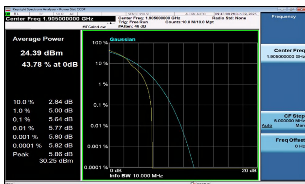
Band2-10MHz-16QAM-19150-1RB#0-PASS
