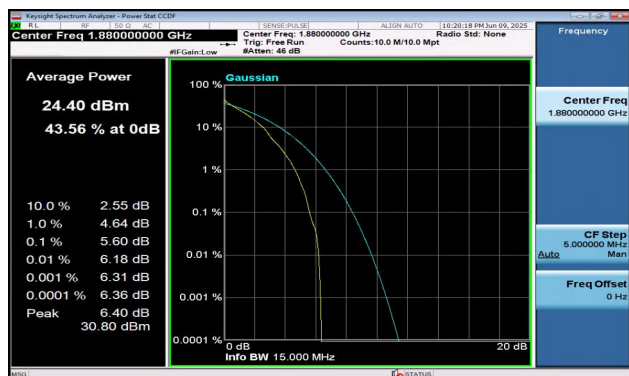
Band2-15MHz-QPSK-18900-1RB#0-PASS
