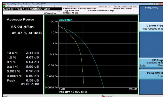
Band2-15MHz-QPSK-18675-75RB#0-PASS
