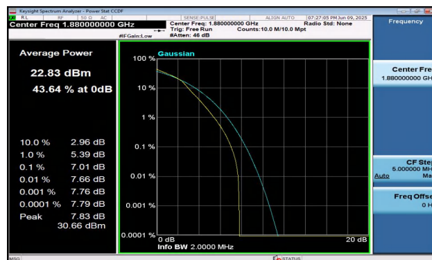
Band2-1.4MHz-16QAM-18900-6RB#0-PASS
