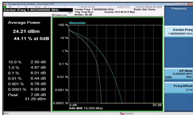
Band2-15MHz-QPSK-19125-75RB#0-PASS
