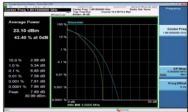
Band2-3MHz-16QAM-18615-15RB#0-PASS
