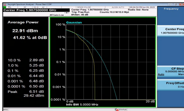
Band2-5MHz-16QAM-19175-1RB#0-PASS
