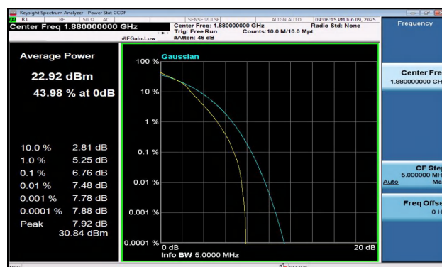
Band2-5MHz-16QAM-18900-25RB#0-PASS
