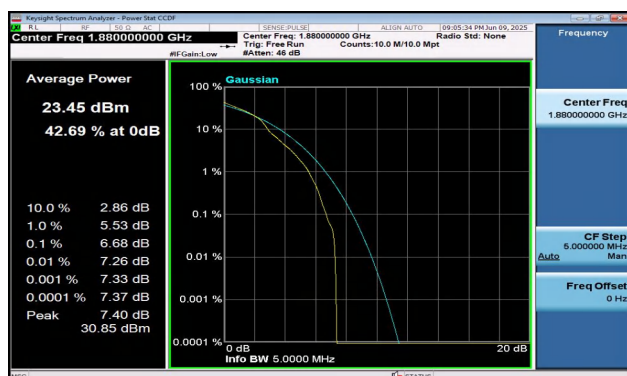
Band2-5MHz-16QAM-18900-1RB#0-PASS
