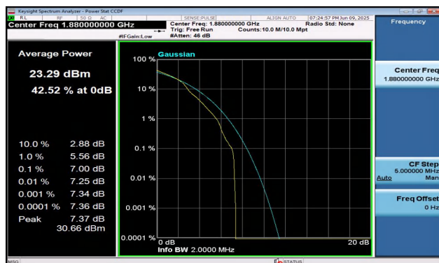
Band2-1.4MHz-16QAM-18900-1RB#0-PASS
