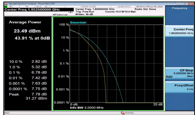
Band2-5MHz-16QAM-18625-25RB#0-PASS
