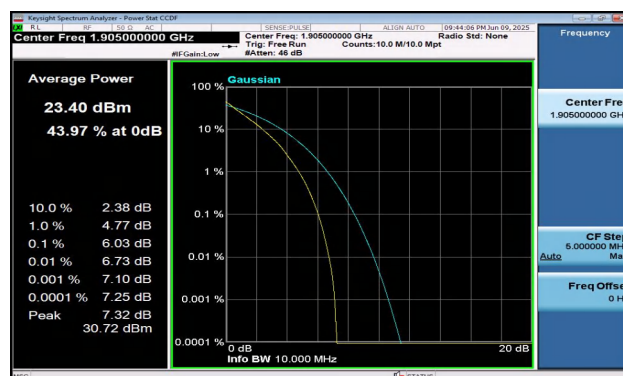
Band2-10MHz-QPSK-19150-50RB#0-PASS
