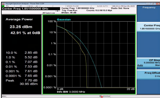
Band2-3MHz-16QAM-18615-1RB#0-PASS
