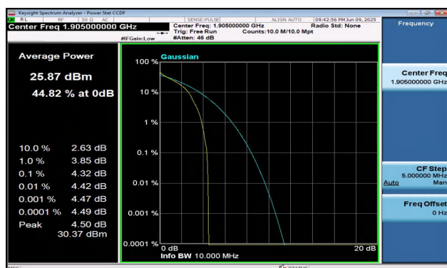
Band2-10MHz-QPSK-19150-1RB#0-PASS
