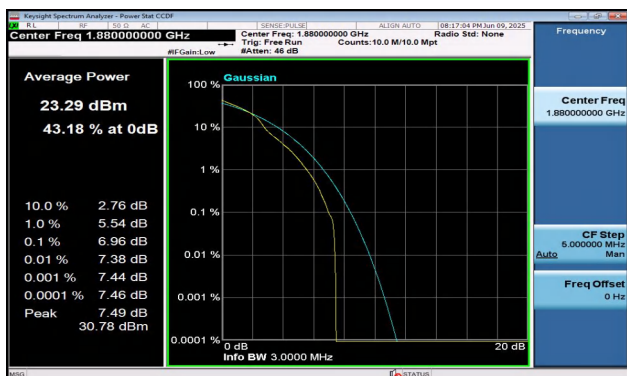
Band2-3MHz-16QAM-18900-1RB#0-PASS
