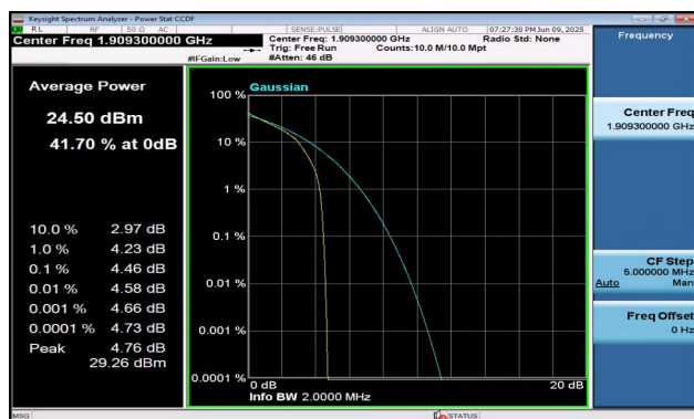
Band2-1.4MHz-QPSK-19193-1RB#0-PASS
