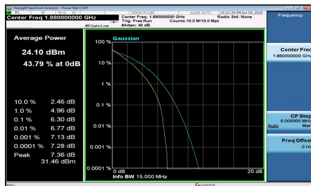
Band2-15MHz-QPSK-18900-75RB#0-PASS
