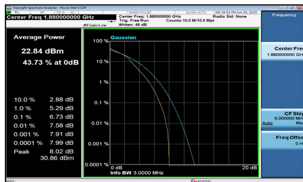
Band2-3MHz-16QAM-18900-15RB#0-PASS
