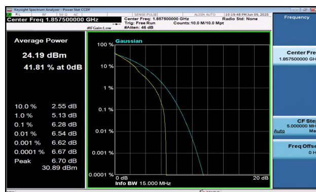
Band2-15MHz-QPSK-18675-1RB#0-PASS
