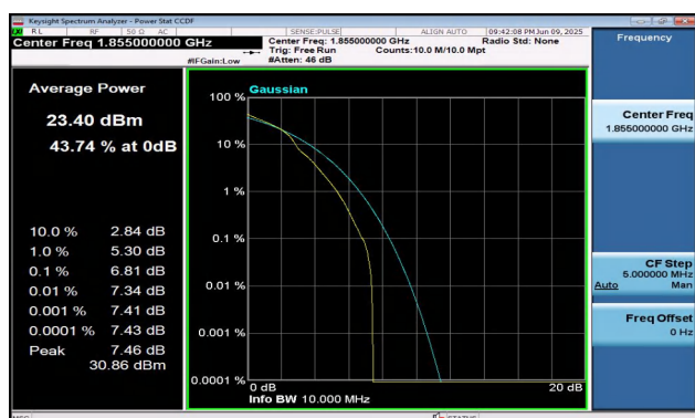
Band2-10MHz-16QAM-18650-1RB#0-PASS
