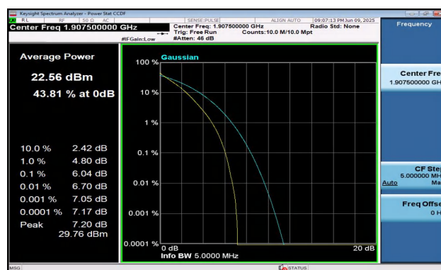
Band2-5MHz-QPSK-19175-25RB#0-PASS
