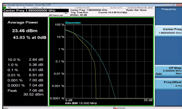
Band2-15MHz-16QAM-18900-1RB#0-PASS
