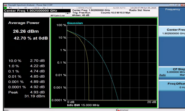
Band2-15MHz-QPSK-19125-1RB#0-PASS
