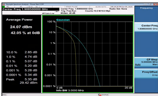
Band2-3MHz-QPSK-19185-1RB#0-PASS
