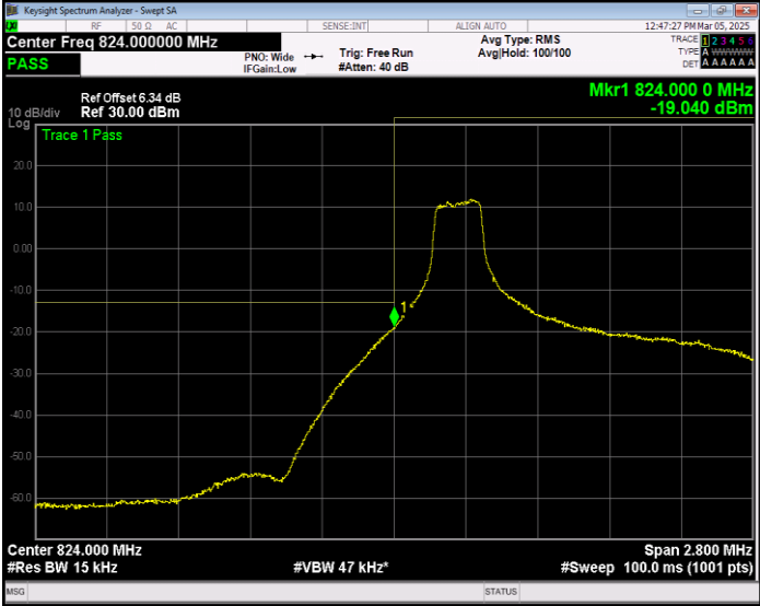
Band5 16QAM BW=1.4MHz Channel=20643 RB Size=1 Position=#0 Normal
