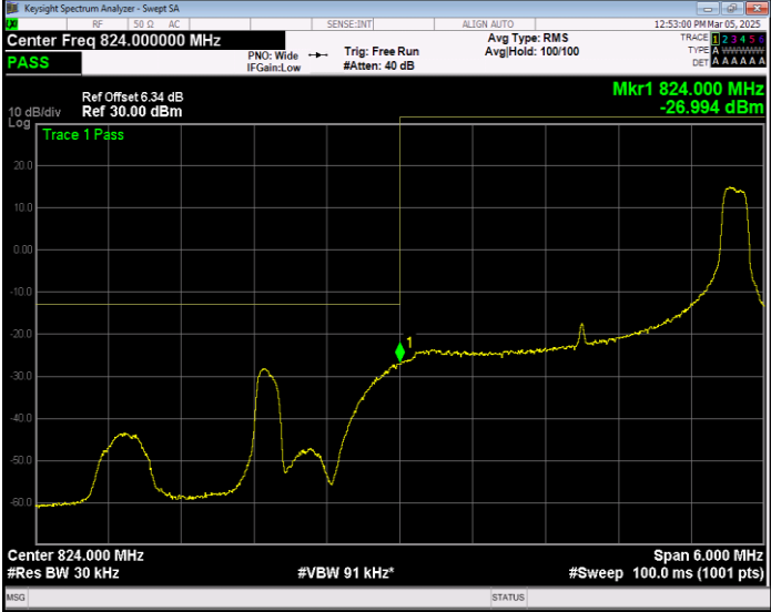
Band5 16QAM BW=3MHz Channel=20415 RB Size=15 Position=#0 Extended
