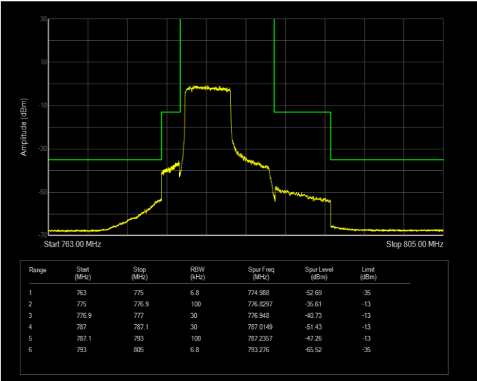
Band13 16QAM BW=10MHz Channel=23230 RB Size=27 Position=#0 Normal
