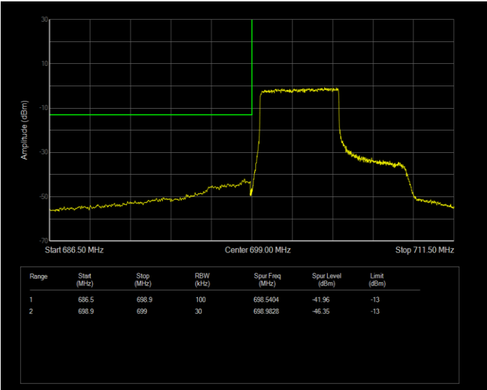
Band12 16QAM BW=10MHz Channel=23060 RB Size=27 Position=#0 Normal
