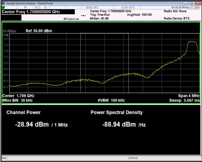
Band66 16QAM BW=15MHz Channel=132047 RB Size=1 Position=#0 Normal
