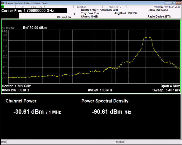
Band66 16QAM BW=3MHz Channel=131987 RB Size=1 Position=#0 Normal
