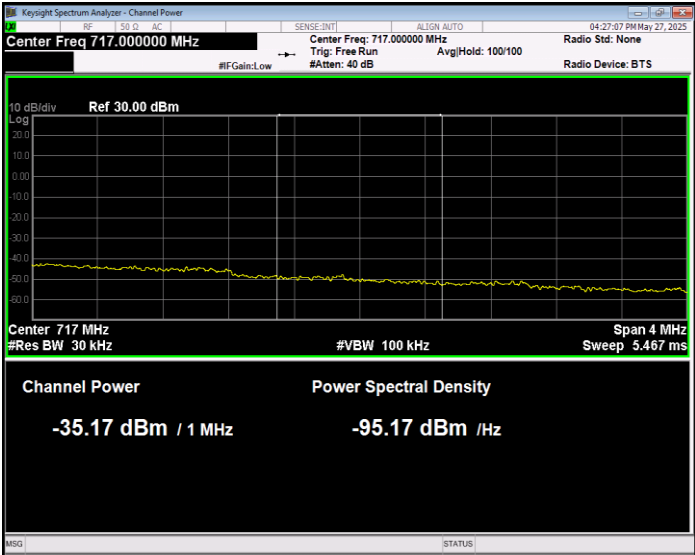
Band17 16QAM BW=10MHz Channel=23800 RB Size=27 Position=#0 Normal
