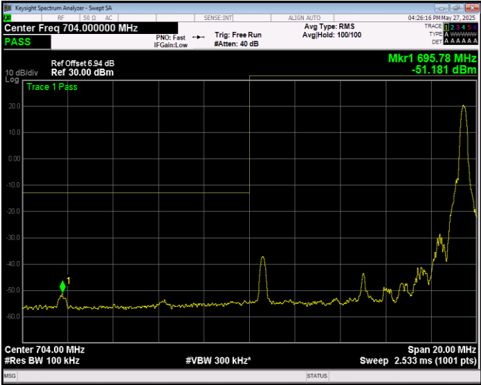
Band17 16QAM BW=10MHz Channel=23780 RB Size=27 Position=#0 Extended
