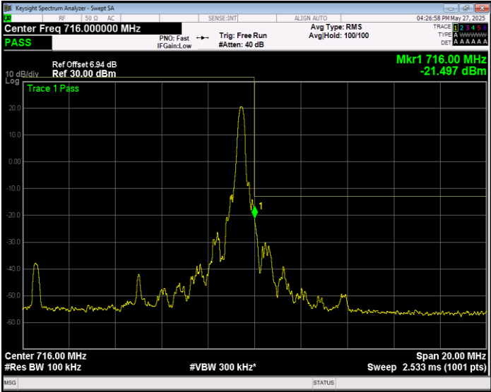
Band17 16QAM BW=10MHz Channel=23800 RB Size=27 Position=#0 Extended
