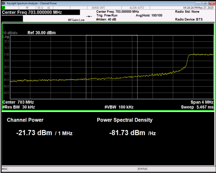
Band17 16QAM BW=10MHz Channel=23780 RB Size=27 Position=#0 Normal
