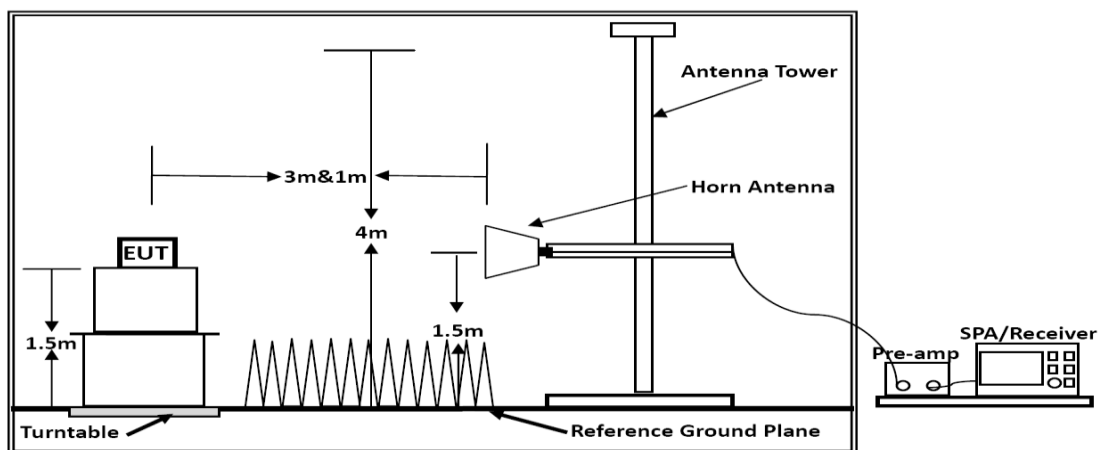
Above 1GHz
