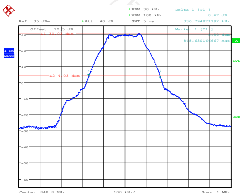
26dB&99% Occupied Bandwidth Plot on Channel 251
