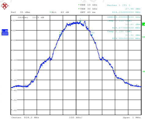
26dB&99% Occupied Bandwidth Plot on Channel 128
