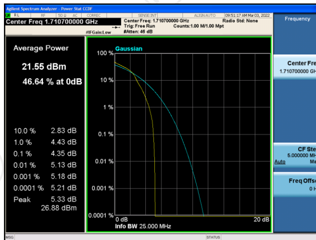
Band4-1.4MHz-16QAM-20175-1RB#0
