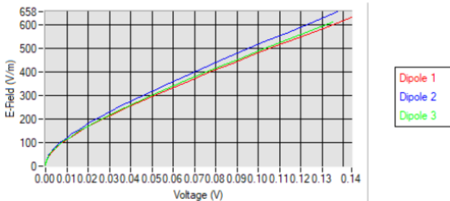
Calibration curves
