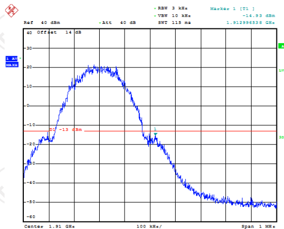
Higher Band Edge Plot on Channel 810
