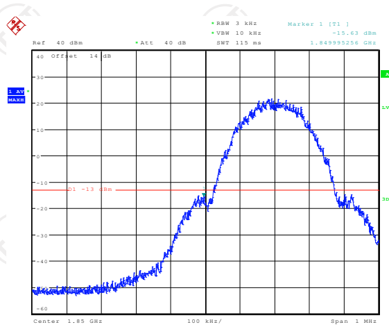
Lower Band Edge Plot on Channel 512
