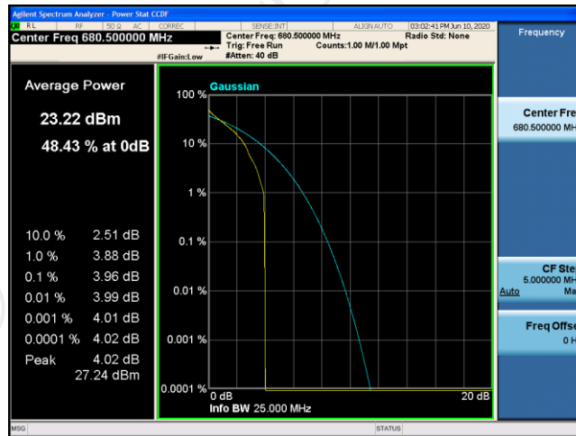
Band71-15MHz-QPSK-133297-75RB#0
