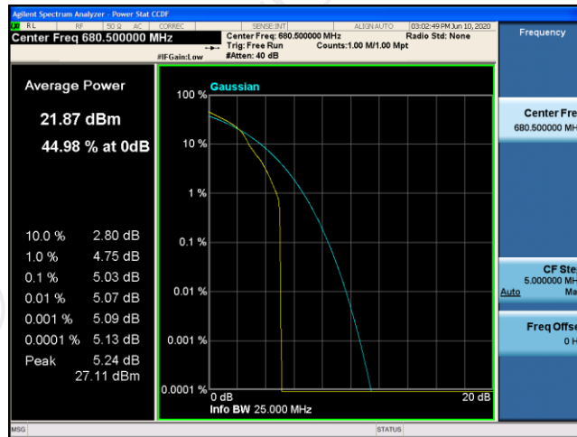
Band71-15MHz-16QAM-133297-75RB#0
