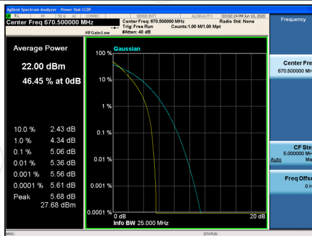
Band71-15MHz-QPSK-133297-1RB#0
