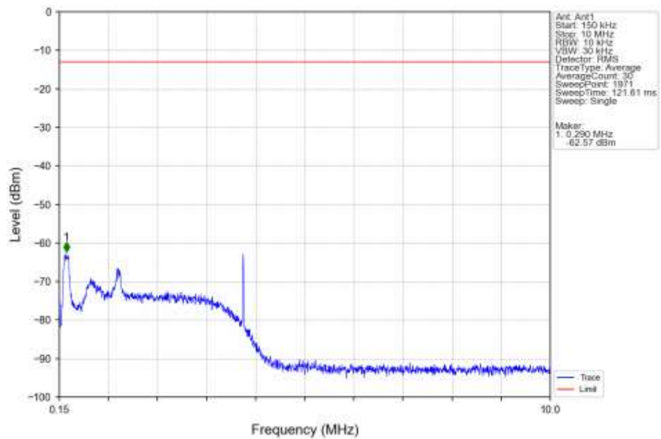
Band2_RMC_MCH_1880MHz_12.2kbps_RMC_NTNV
