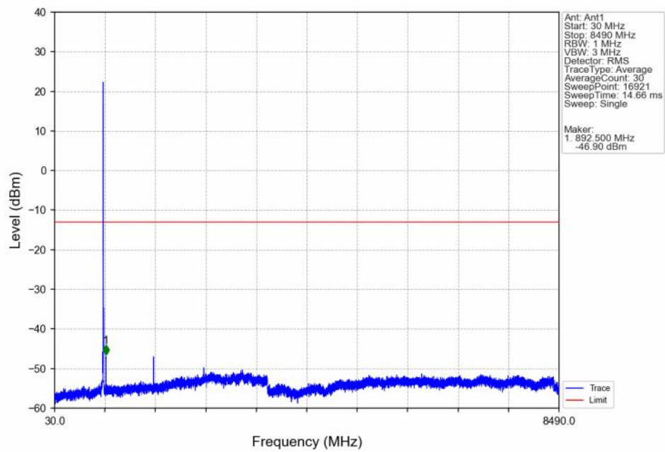
Band5_5MHz_QPSK_HCH_846.5MHz_RB_1_0_NTN
