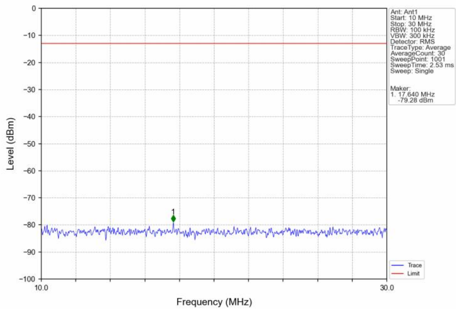
Band5_10MHz_16QAM_LCH_829MHz_RB_1_0_NTNV
