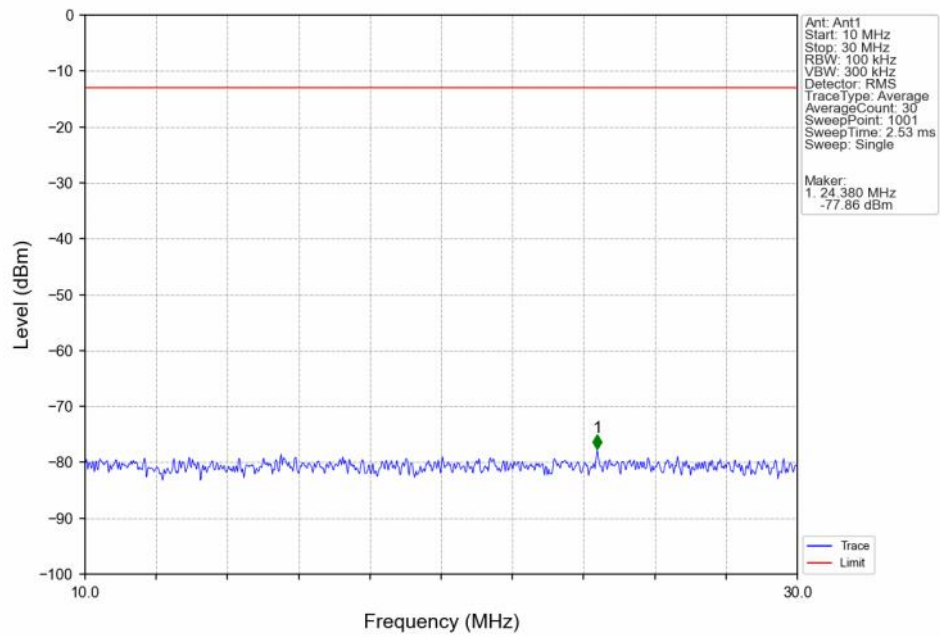
Band5_5MHz_QPSK_HCH_846.5MHz_RB_1_0_NTN
