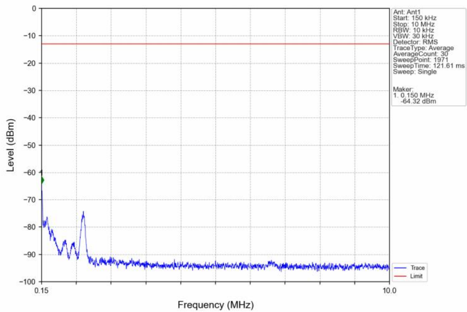
Band4_15MHz_16QAM_MCH_1732.5MHz_RB_1_0_NTNV
