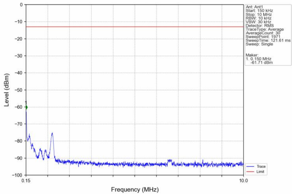
Band4 15MHz QPSK HCH 1747.5MHz RB 1 0 NTN
