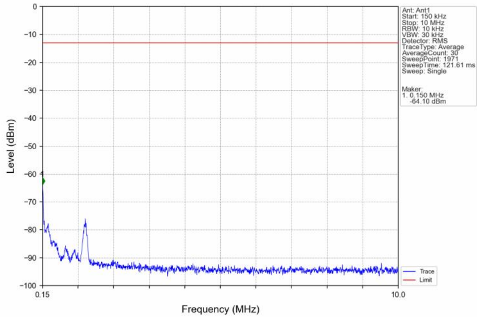
Band4 5MHz 16QAM HCH 1752.5MHz RB 1 0 NTN
