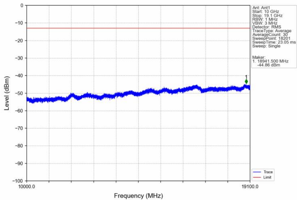
Band2_3MHz_16QAM_HCH_1908.5MHz_RB_1_0_NTN
