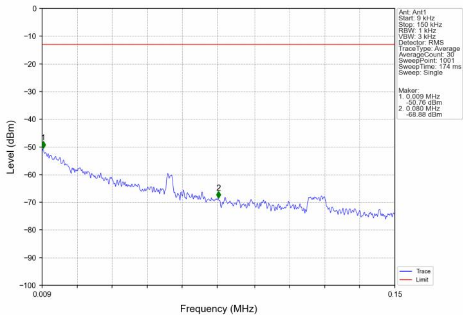
Band2_3MHz_16QAM_HCH_1908.5MHz_RB_1_0_NTN
