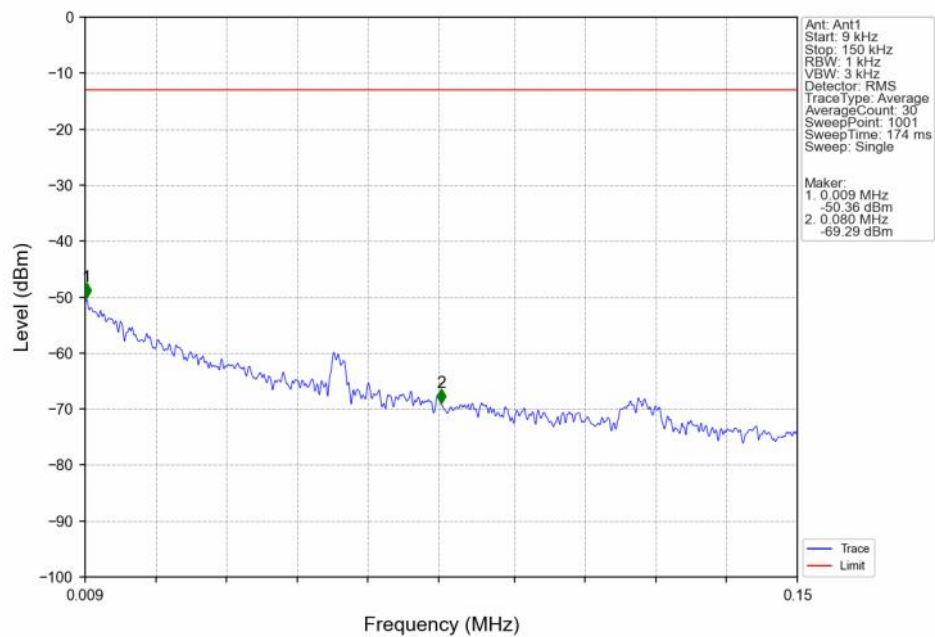
Band2_5MHz_16QAM_HCH_1907.5MHz_RB_1_0_NTN
