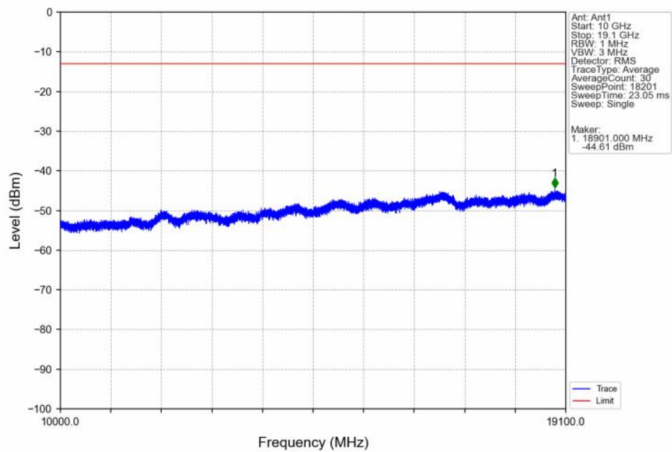
Band2_5MHz_16QAM_HCH_1907.5MHz_RB_1_0_NTN
