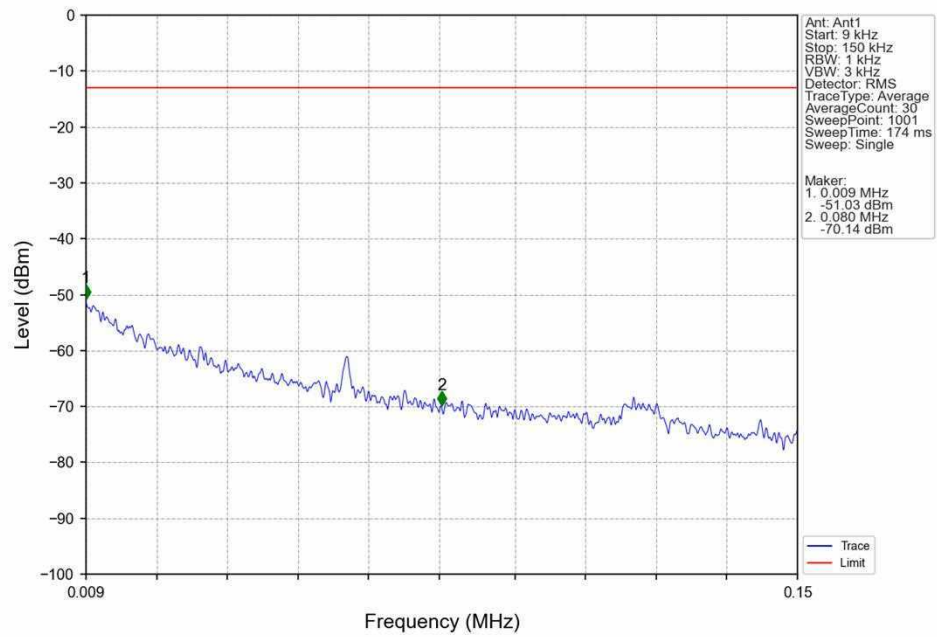
Band5 3MHz 16QAM MCH 836.5MHz RB 1 0 NTN
