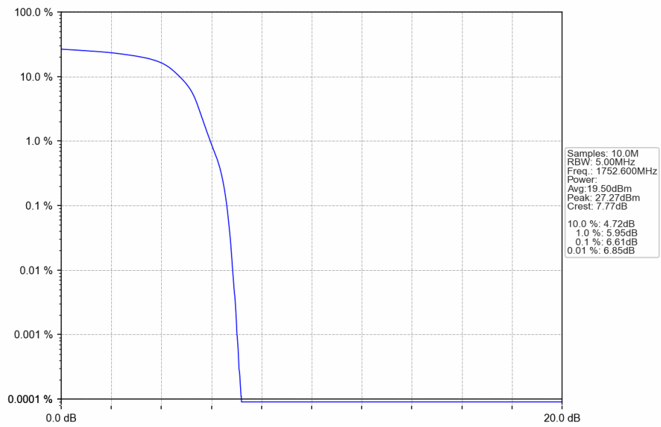
Band4_HSUPA_HCH_1752.6MHz_Subtest 1_NTNV
