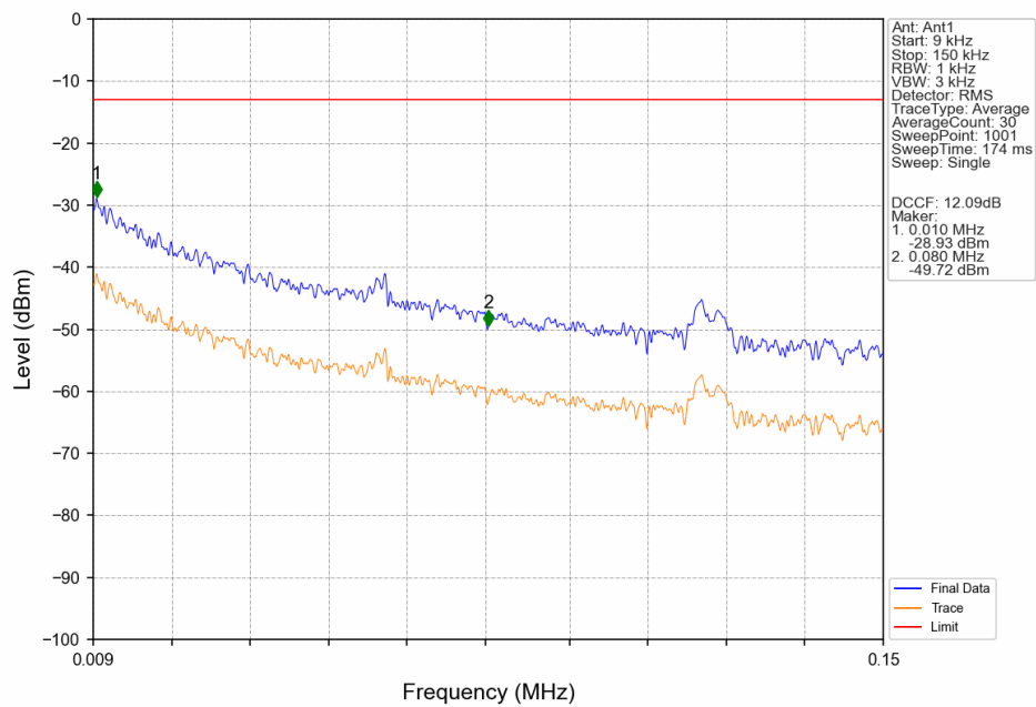
GSM850_GPRS_MCH_836.6MHz_1 TX Slot_NTNV
