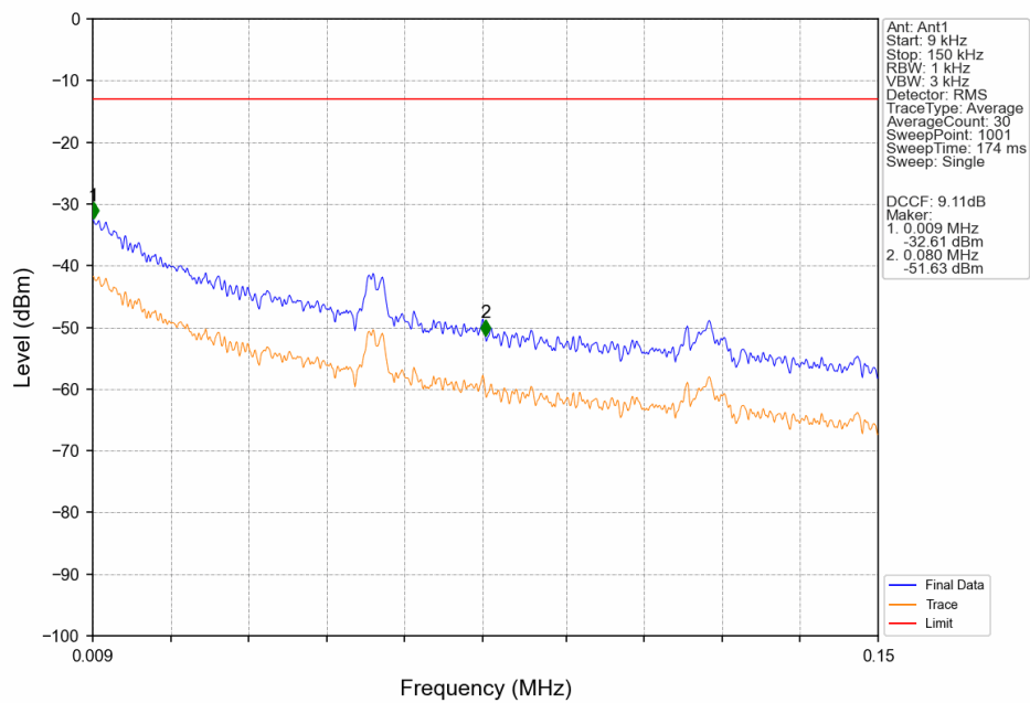
GSM850_EGPRS_MCH_836.6MHz_1 TX Slot_NTNV
