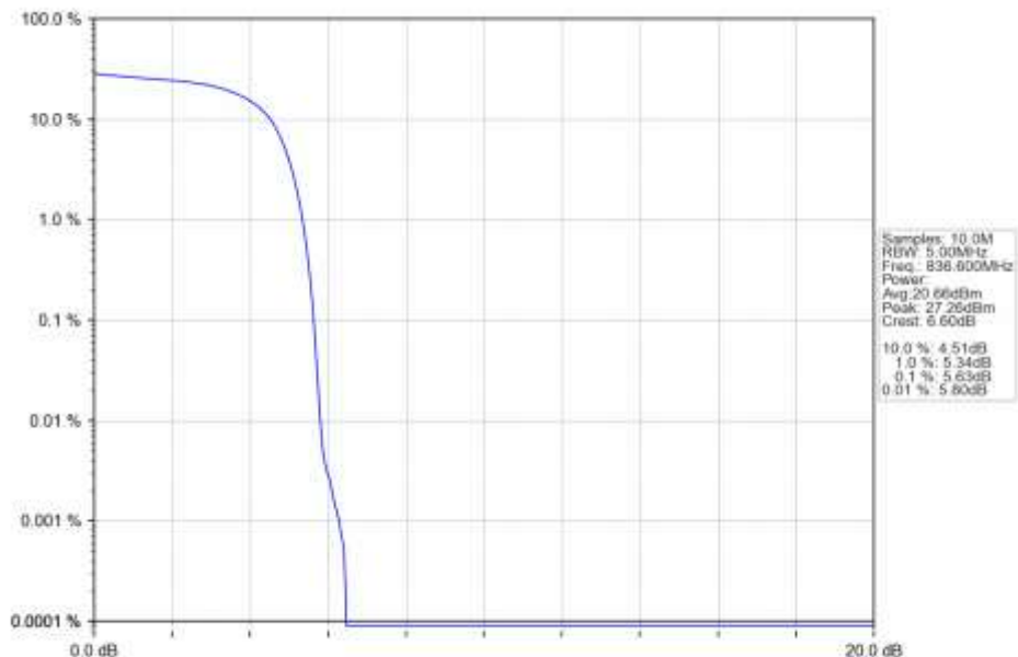
Band5 HSDPA MCH 836.6MHz Subtest 1 NTV
