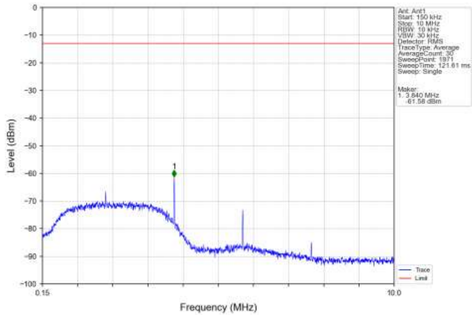
Band5 RMC MCH 836.6MHz 12.2kbps RMC NTN
