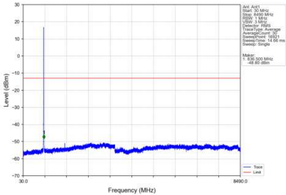
Band5 RMC MCH 836.6MHz 12.2kbps RMC NTNV
