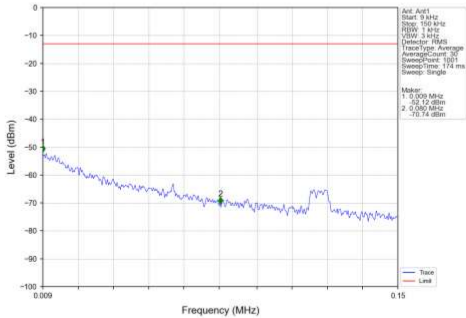
Band5 HSUPA HCH 846.6MHz Subtest 1 NTNV
