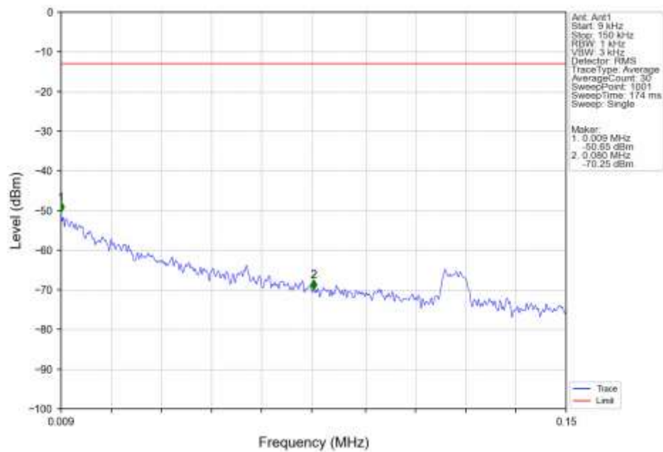
Band5 HSDPA MCH 836.6MHz Subtest 1 NTN
