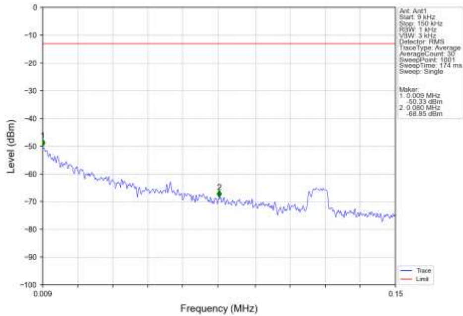
Band5 RMC HCH 846.6MHz 12.2kbps RMC NTN
