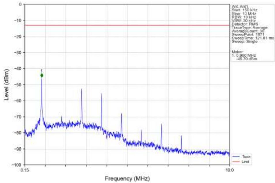
Band5 HSDPA LCH 826.4MHz Subtest 1 NTNV
