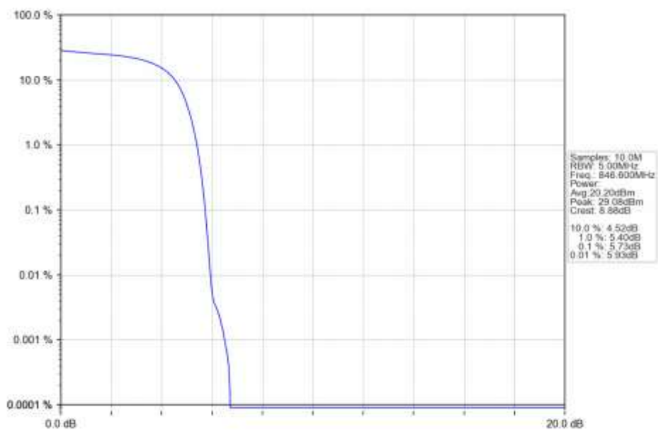
Band5 HSDPA HCH 846.6MHz Subtest 1 NTV
