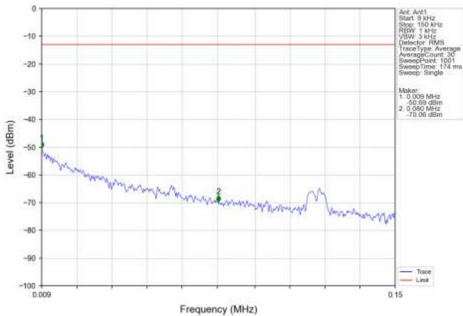
Band5 RMC MCH 836.6MHz 12.2kbps RMC NTNV
