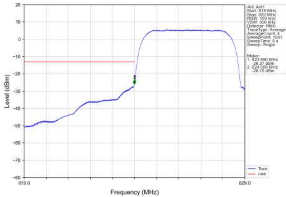
Band5 HSDPA LCH 826.4MHz Subtest 1 NTNV
