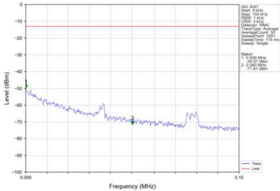
Band4 HSUPA MCH 1732.6MHz Subtest 1 NTV
