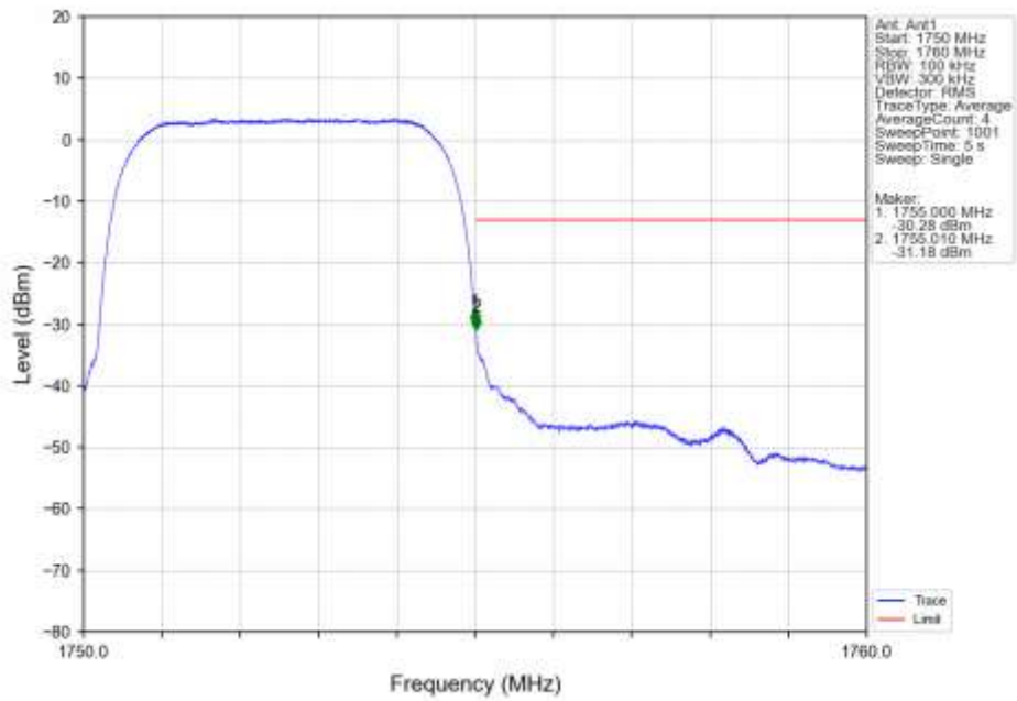
Band4 HSDPA HCH 1752.6MHz Subtest 1 NTNV
