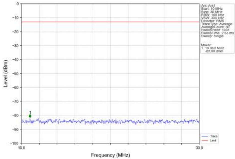
Band4 HSUPA MCH 1732.6MHz Subtest 1 NTV
