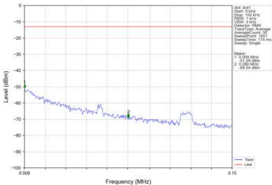
Band4 HSDPA MCH 1732.6MHz Subtest 1 NTN
