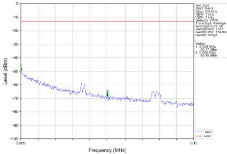
Band2 HSUPA HCH 1907.6MHz Subtest 1 NTN
