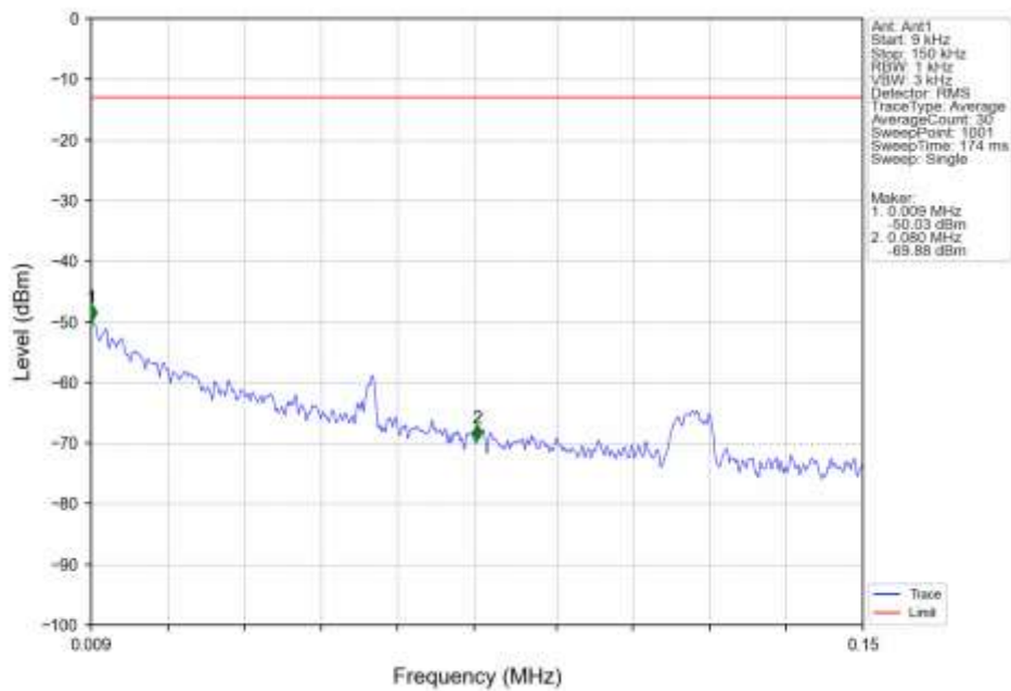
Band2 HSDPA HCH 1907.6MHz Subtest 1 NTNV
