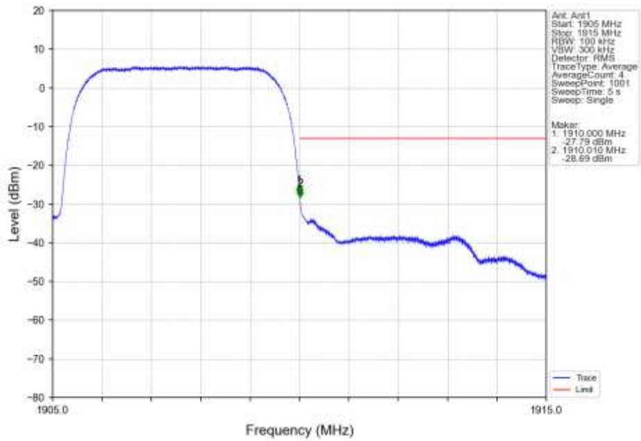
Band2 HSDPA HCH 1907.6MHz Subtest 1 NTNV
