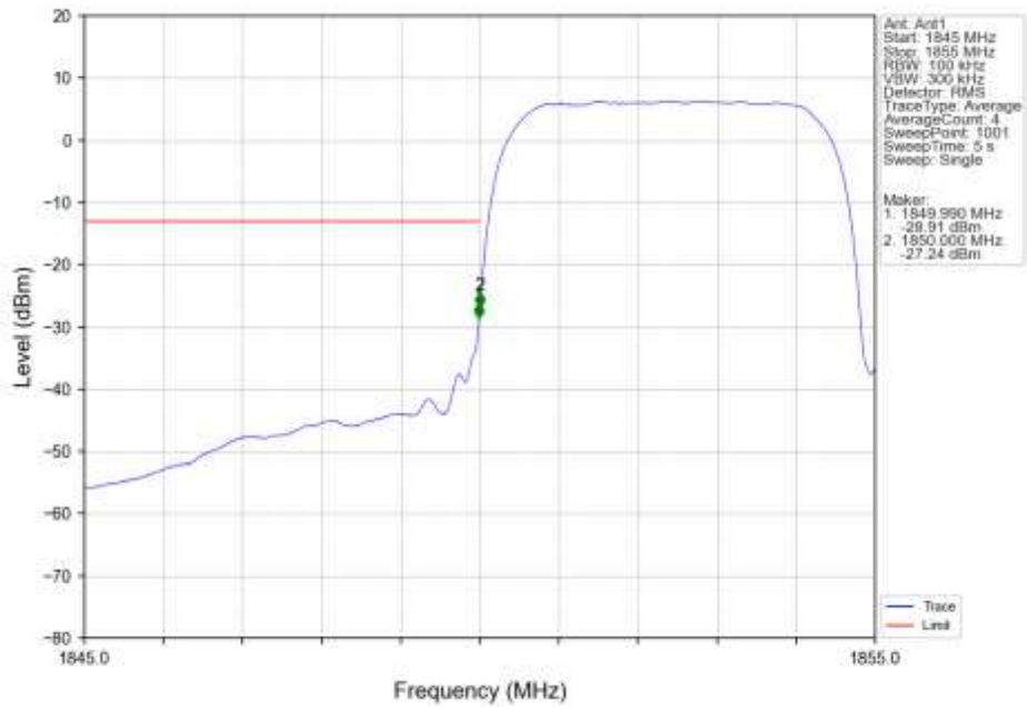
Band2_RMC_LCH_1852.4MHz_12.2kbps RMC_NTNV
