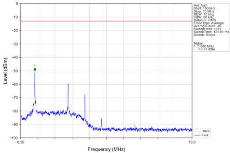
Band2 HSDPA MCH 1880MHz Subtest 1 NTN
