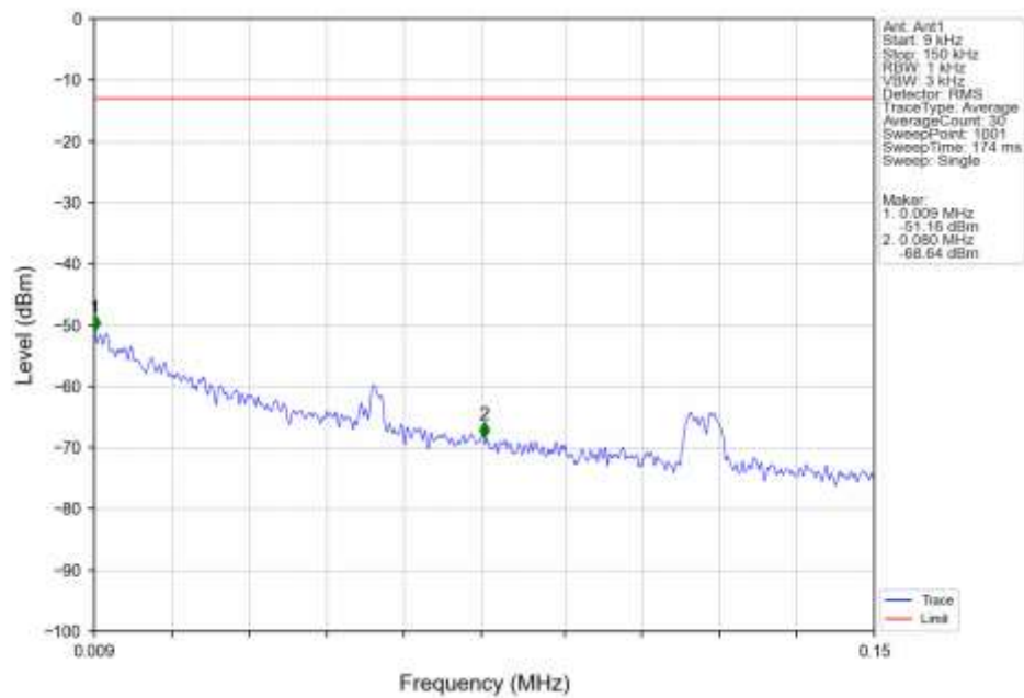
Band2 HSDPA MCH 1880MHz Subtest 1 NTN
