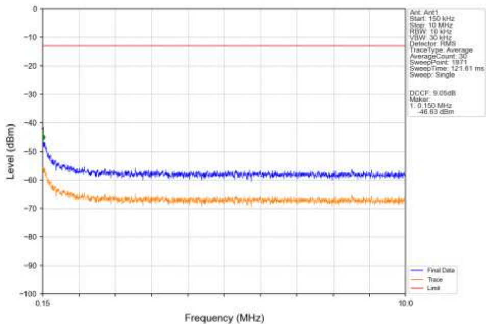
GSM850 GPRS MCH 836.6MHz 1 TX Slot NTV
