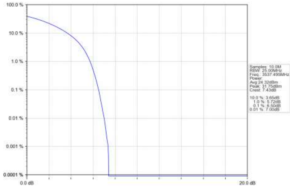
n78e 15kHz SISO NTN 25MHz CP-OFDM 64 QAM 3537.495MHz Outer Full Ant1
