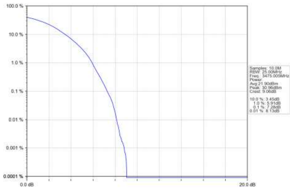
n78e 15kHz SISO NTN 50MHz DFT-s-OFDM 16 QAM 3475.005MHz Outer Full Ant1
