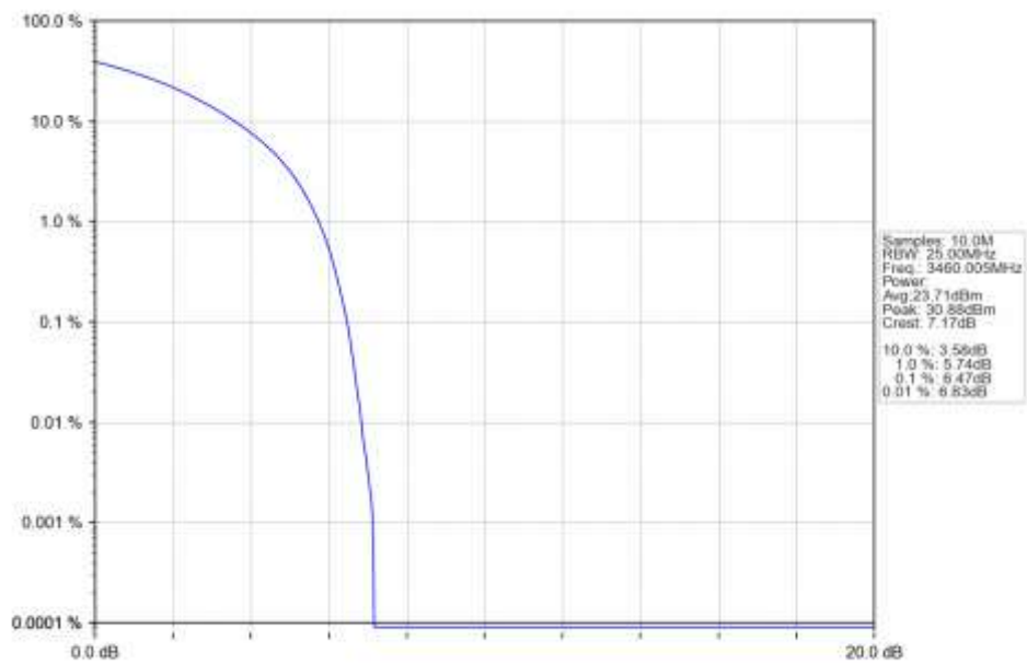
n78e 15kHz SISO NTN 20MHz CP-OFDM 16 QAM 3460.005MHz Outer Full Ant1
