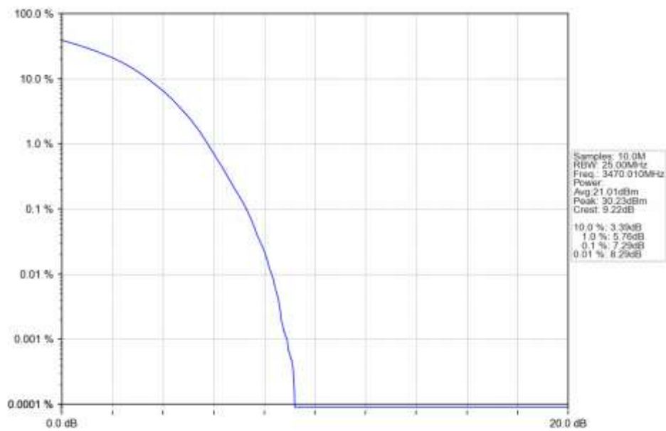
n78e 15kHz SISO NTN 40MHz DFT-s-OFDM 256 QAM 3470.01MHz Outer Full Ant1
