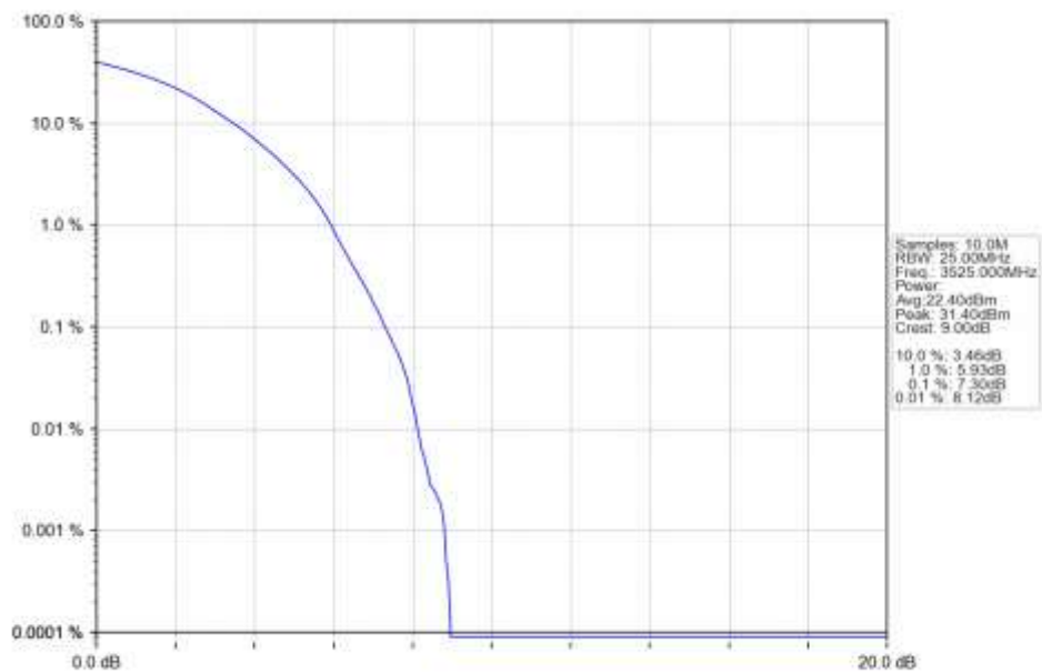
n78e 15kHz SISO NTN 50MHz DFT-s-OFDM 16 QAM 3525MHz Outer Full Ant1
