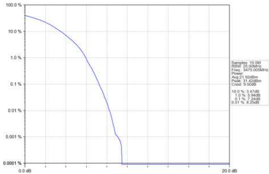
n78e 15kHz SISO NTN 50MHz DFT-s-OFDM 64 QAM 3475.005MHz Outer Full Ant1
