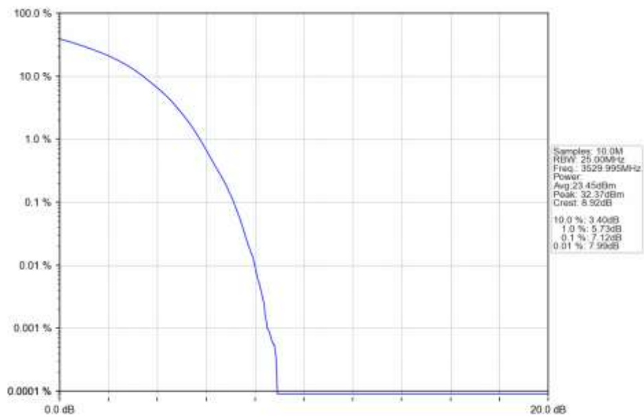
n78e 15kHz SISO NTN 40MHz DFT-s-OFDM 16 QAM 3529.995MHz Outer Full Ant1
