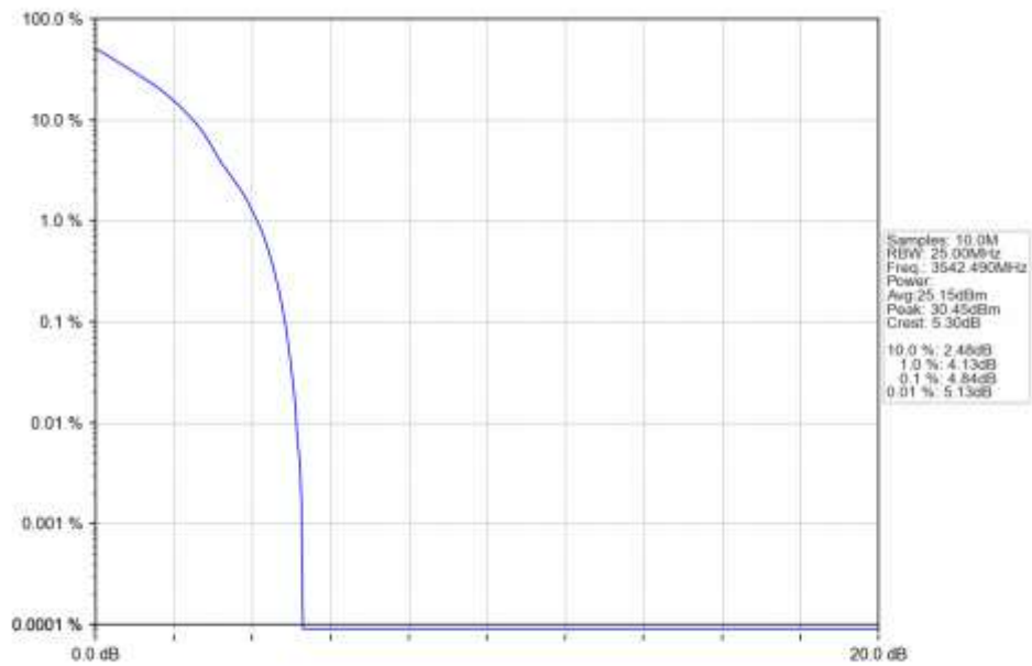
n78e 30kHz SISO NTN 15MHz DFT-s-OFDM QPSK 3542.49MHz Outer Full Ant1
