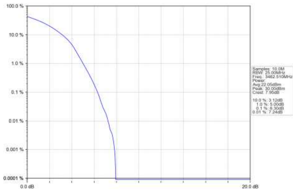
n78e 15kHz SISO NTN 25MHz DFT-s-OFDM 256 QAM 3462.51MHz Outer Full Ant1
