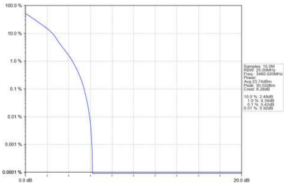
n78e_30kHz_SISO_NTNV_20MHz_DFT-s-OFDM QPSK_3460.02MHz_Outer_Full_Ant1
