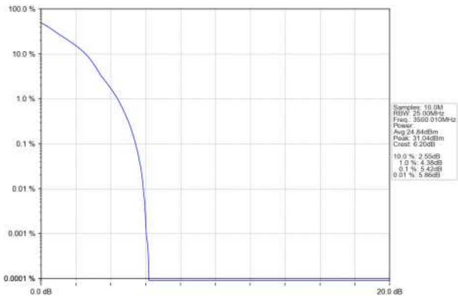
n78e_30kHz_SISO_NTNV_20MHz_DFT-s-OFDM QPSK_3500.01MHz_Outer_Full_Ant1
