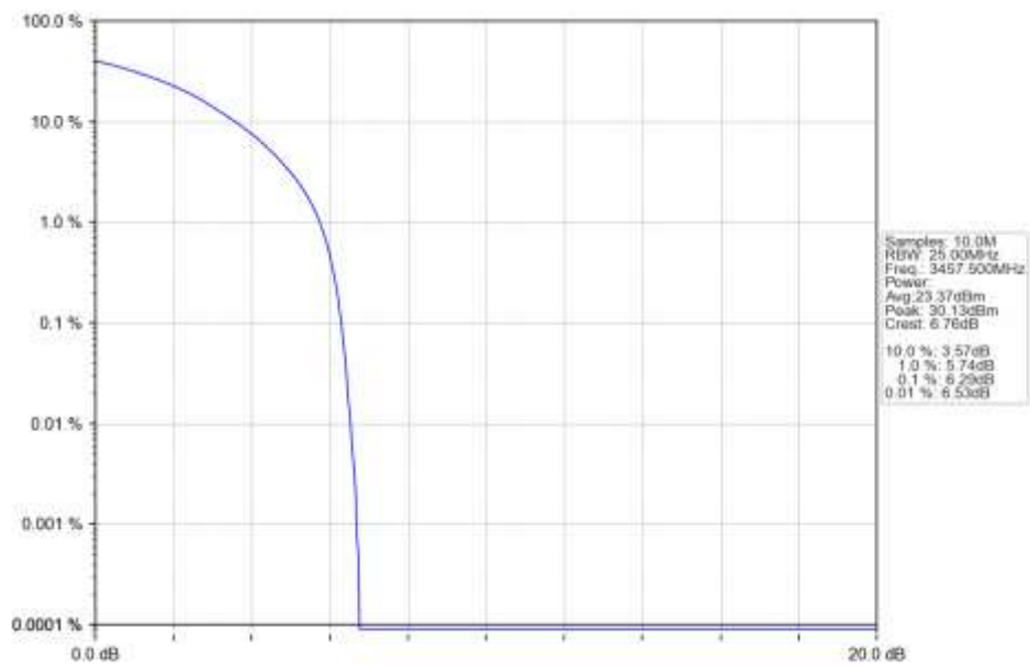
n78e 30kHz SISO NTN 15MHz CP-OFDM 16 QAM 3457.5MHz Outer Full Ant1
