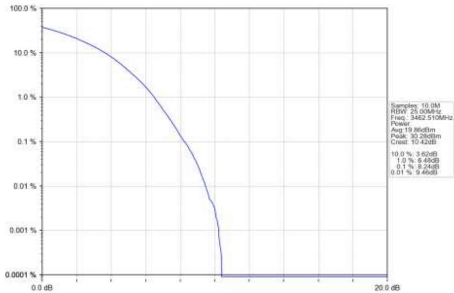
n78e 15kHz SISO NTN 25MHz CP-OFDM 256 QAM 3462.51MHz Outer Full Ant1
