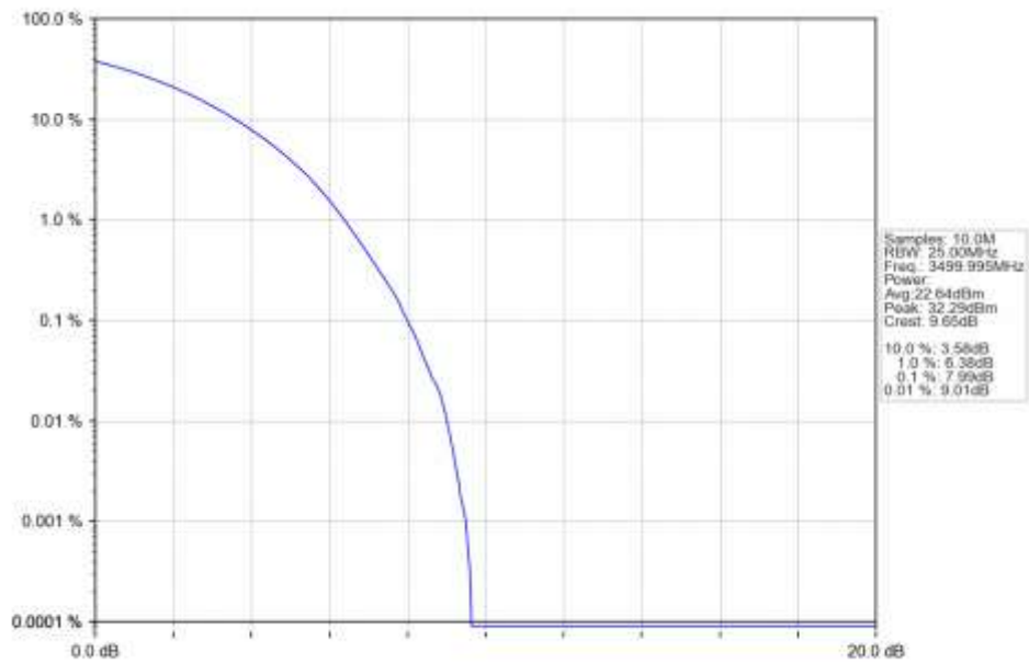
n78e 15kHz SISO NTN 50MHz CP-OFDM 16 QAM 3499.995MHz Outer Full Ant1
