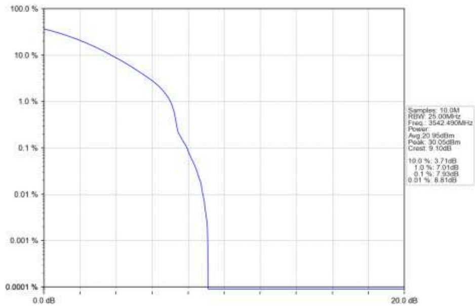
n78e 30kHz SISO NTN 15MHz CP-OFDM 256 QAM 3542.49MHz Outer Full Ant1
