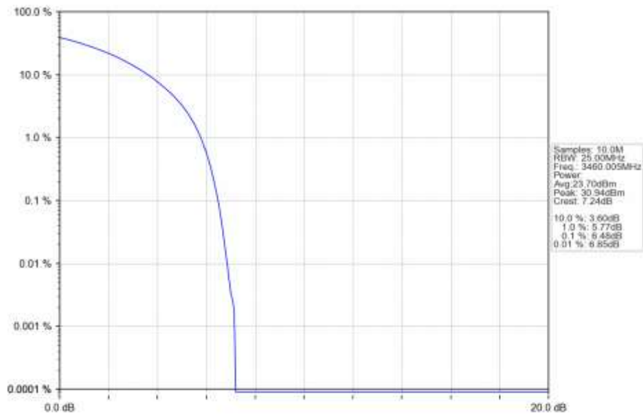
n78e 15kHz SISO NTV 20MHz CP-OFDM QPSK 3460.005MHz Outer Full Ant1
