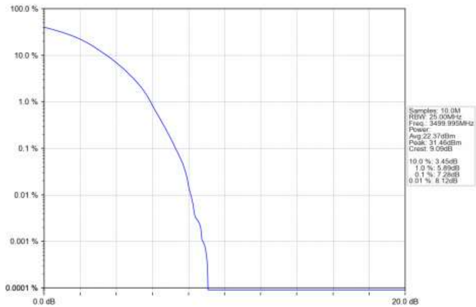
n78e 15kHz SISO NTN 50MHz DFT-s-OFDM 16 QAM 3499.995MHz Outer Full Ant1
