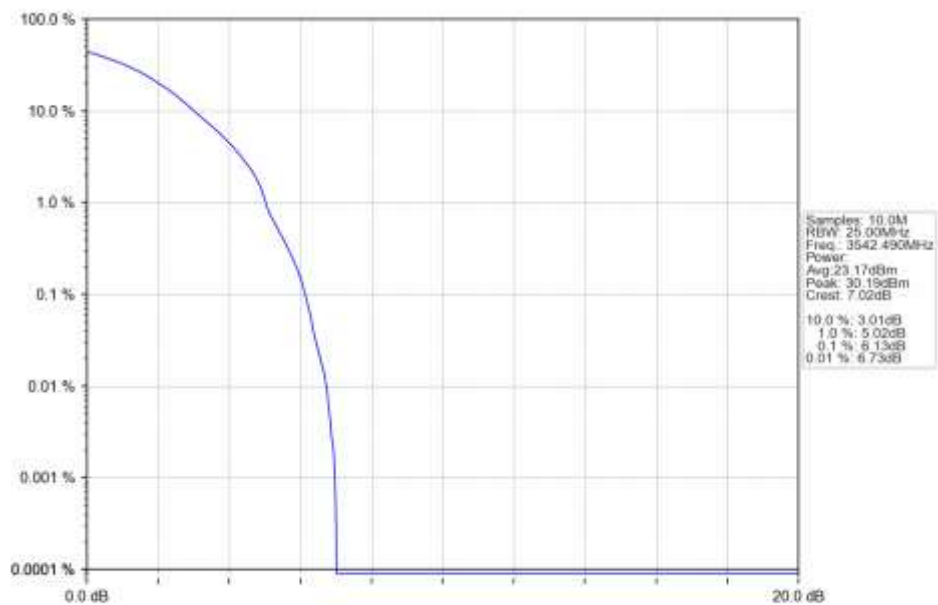
n78e 30kHz SISO NTN 15MHz DFT-s-OFDM 256 QAM 3542.49MHz Outer Full Ant1
