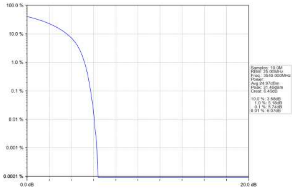
n78e 15kHz SISO NTN 20MHz CP-OFDM 16 QAM 3540MHz Outer Full Ant1
