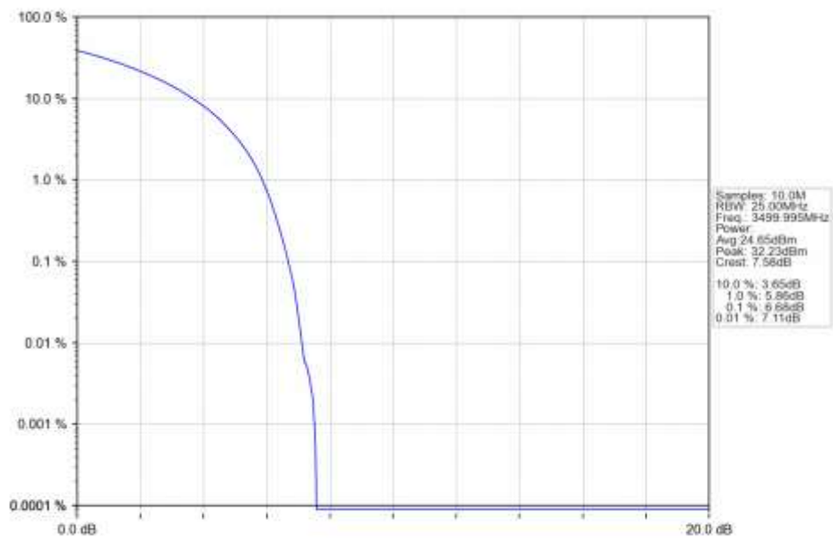
n78e 15kHz SISO NTN 25MHz CP-OFDM QPSK 3499.995MHz Outer Full Ant1
