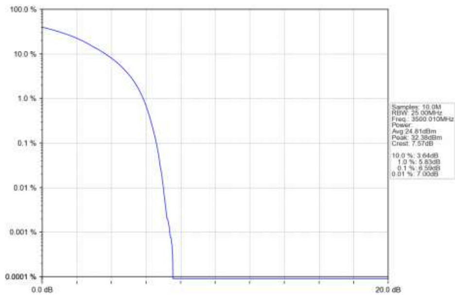
n78e 30kHz SISO NTN 25MHz CP-OFDM QPSK 3500.01MHz Outer Full Ant1
