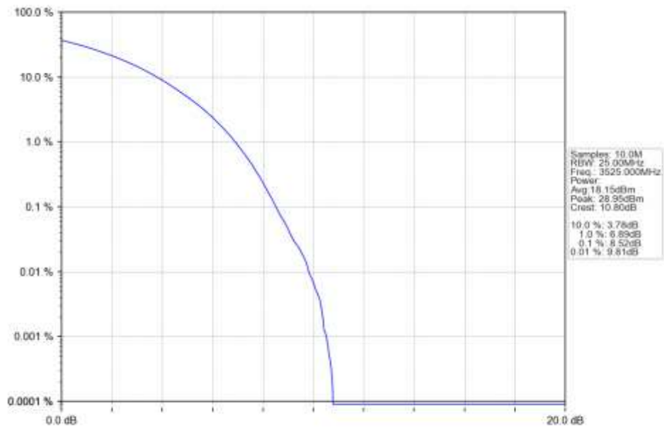
n78e 30kHz SISO NTN 50MHz CP-OFDM 256 QAM 3525MHz Outer Full Ant1
