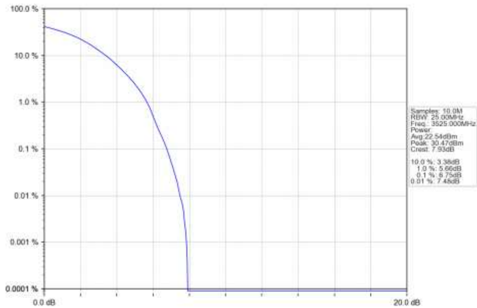
n78e 15kHz SISO NTN 50MHz DFT-s-OFDM QPSK 3525MHz Outer Full Ant1
