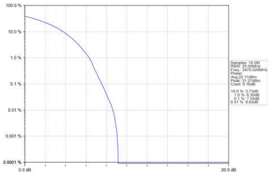
n78e 30kHz SISO NTN 50MHz DFT-s-OFDM 16 QAM 3475.02MHz Outer Full Ant1
