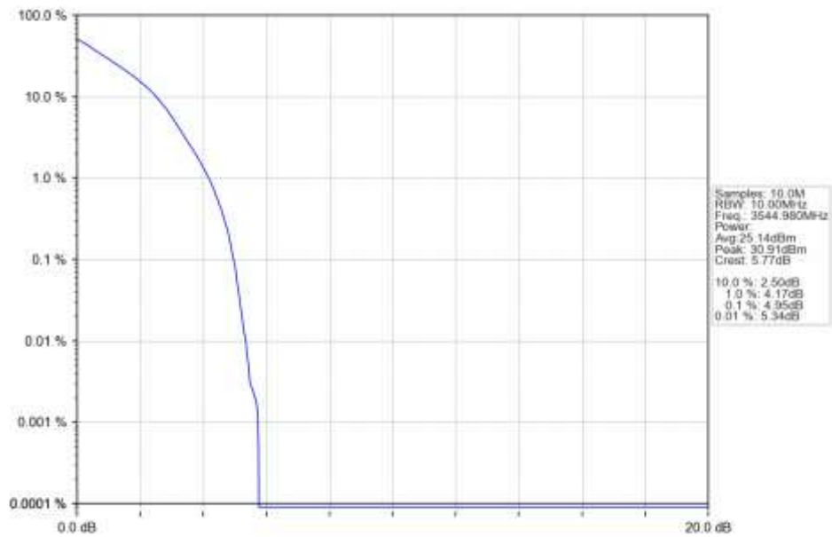
n78e 30kHz SISO NTN 10MHz DFT-s-OFDM QPSK 3544.98MHz Outer Full Ant1
