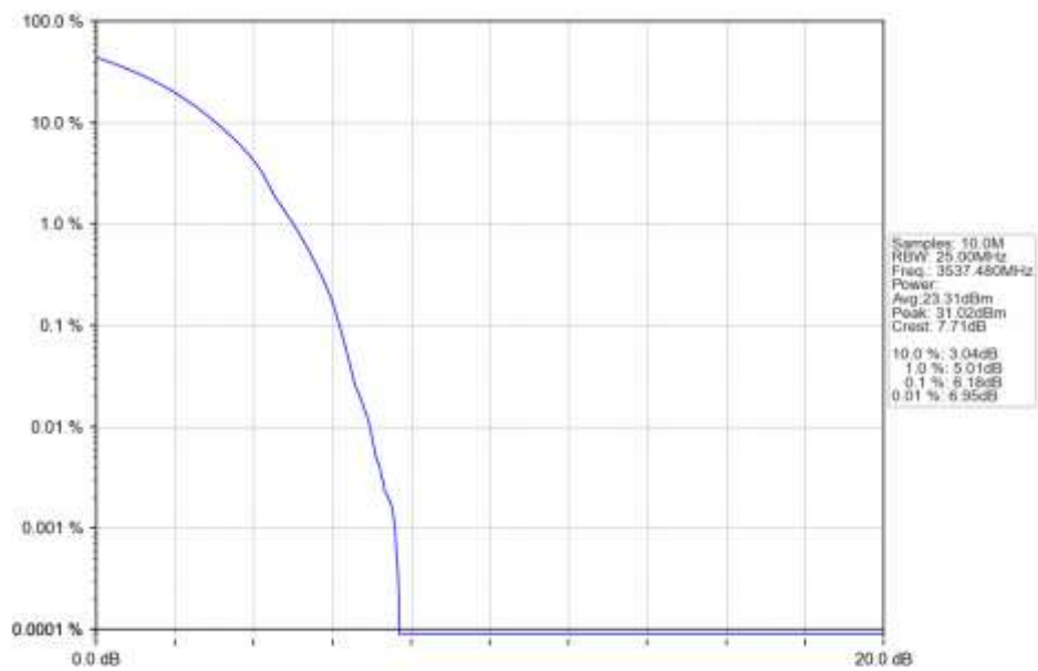
n78e 30kHz SISO NTN 25MHz DFT-s-OFDM 256 QAM 3537.48MHz Outer Full Ant1
