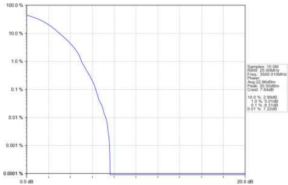
n78e 30kHz SISO NTN 15MHz DFT-s-OFDM 256 QAM 3500.01MHz Outer Full Ant1
