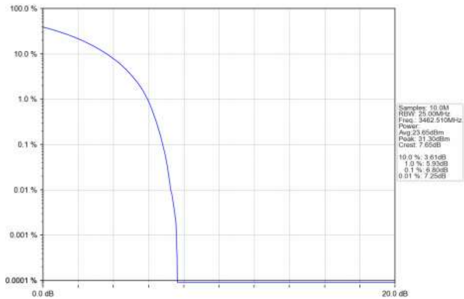
n78e 15kHz SISO NTN 25MHz CP-OFDM QPSK 3462.51MHz Outer Full Ant1
