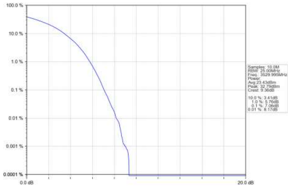
n78e 15kHz SISO NTN 40MHz DFT-s-OFDM 64 QAM 3529.995MHz Outer Full Ant1
