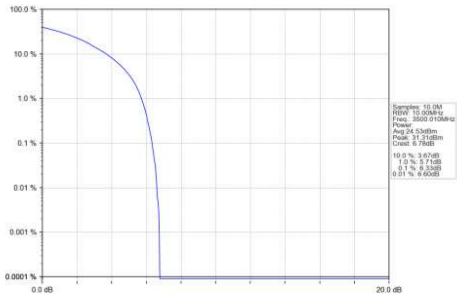
n78e 30kHz SISO NTN 10MHz CP-OFDM QPSK 3500.01MHz Outer Full Ant1
