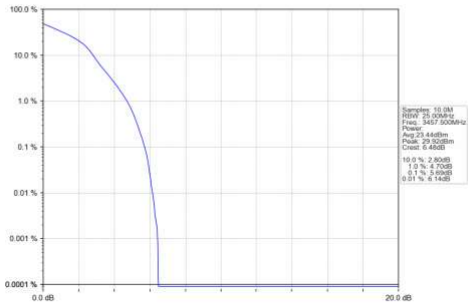
n78e 30kHz SISO NTN 15MHz DFT-s-OFDM 16 QAM 3457.5MHz Outer Full Ant1
