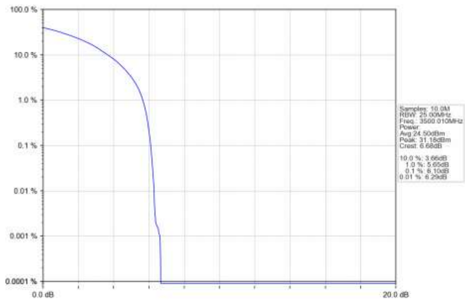
n78e 30kHz SISO NTN 15MHz CP-OFDM QPSK 3500.01MHz Outer Full Ant1
