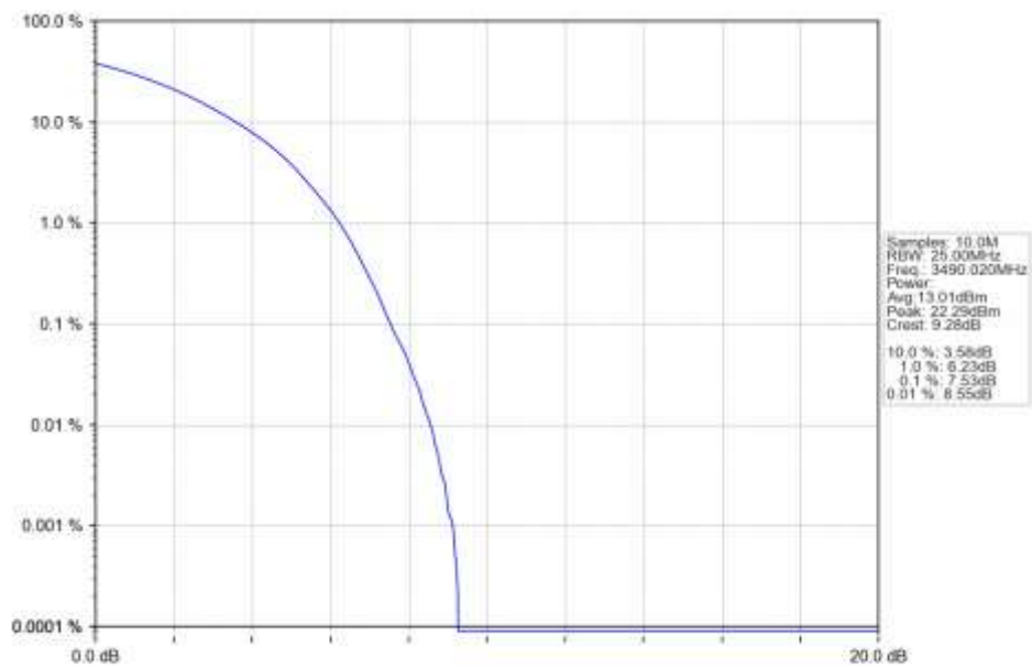
n78e 30kHz SISO NTN 80MHz DFT-s-OFDM 16 QAM 3490.02MHz Outer Full Ant1
