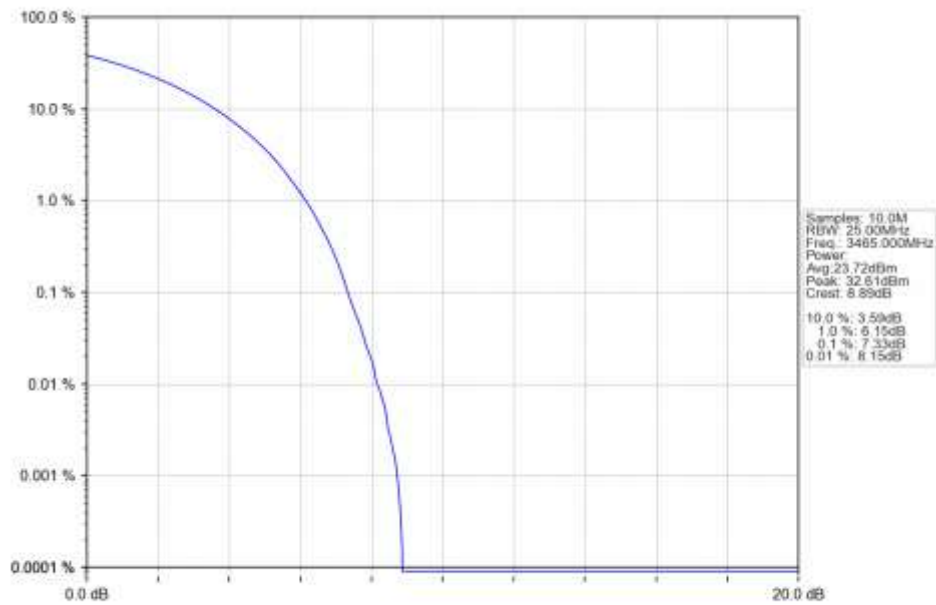
n78e 15kHz SISO NTN 30MHz CP-OFDM QPSK 3465MHz Outer Full Ant1
