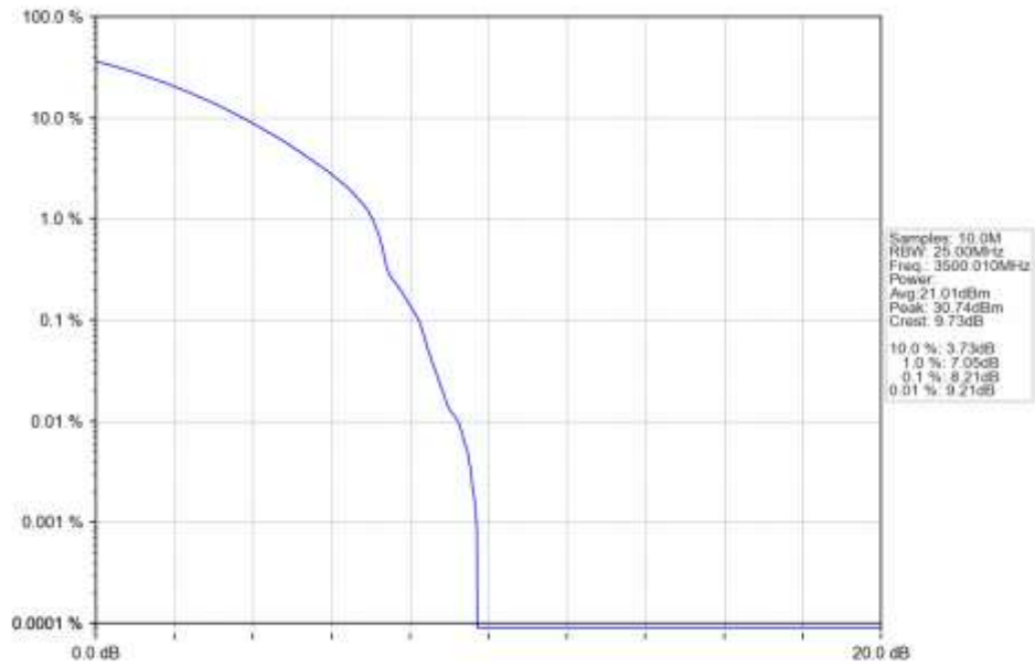
n78e 30kHz SISO NTN 20MHz CP-OFDM 256 QAM 3500.01MHz Outer Full Ant1
