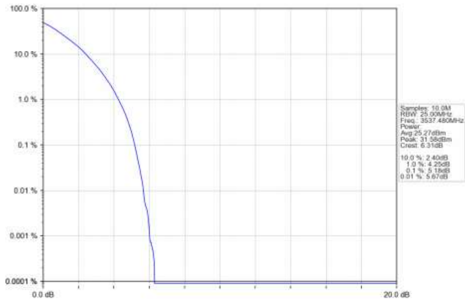
n78e 30kHz SISO NTN 25MHz DFT-s-OFDM QPSK 3537.48MHz Outer Full Ant1
