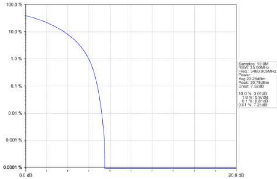
n78e 15kHz SISO NTN 20MHz CP-OFDM 64 QAM 3460.005MHz Outer Full Ant1
