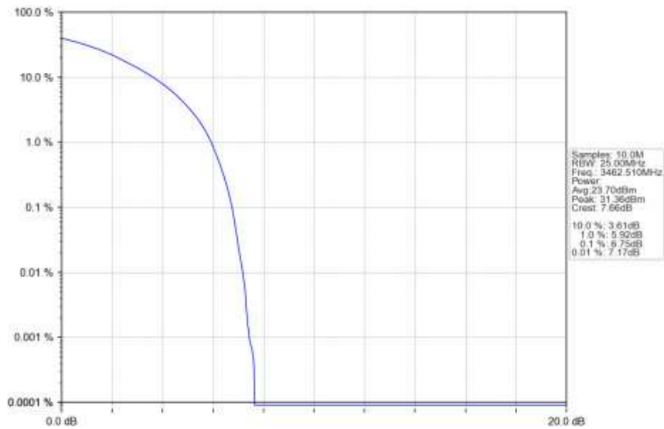
n78e 30kHz SISO NTN 25MHz CP-OFDM QPSK 3462.51MHz Outer Full Ant1
