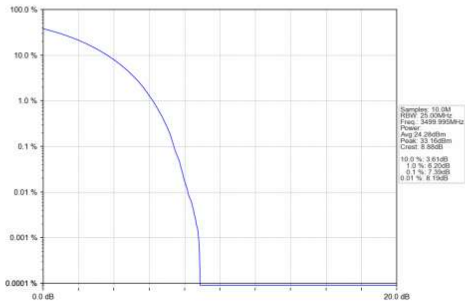
n78e 15kHz SISO NTN 30MHz CP-OFDM QPSK 3499.995MHz Outer Full Ant1
