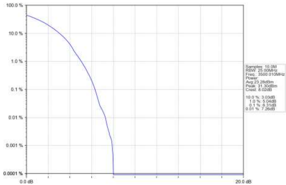
n78e 30kHz SISO NTN 25MHz DFT-s-OFDM 256 QAM 3500.01MHz Outer Full Ant1
