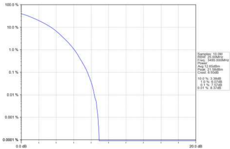
n78e 30kHz SISO NTN 90MHz DFT-s-OFDM 16 QAM 3495MHz Outer Full Ant1
