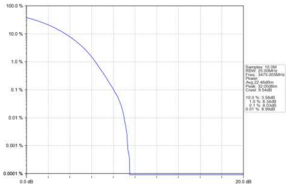
n78e 15kHz SISO NTN 50MHz CP-OFDM 16 QAM 3475.005MHz Outer Full Ant1
