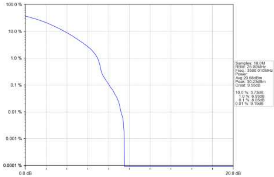
n78e 30kHz SISO NTN 15MHz CP-OFDM 256 QAM 3500.01MHz Outer Full Ant1
