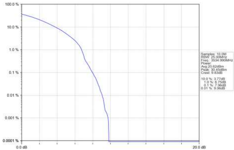
n78e 30kHz SISO NTN 30MHz CP-OFDM 256 QAM 3534.99MHz Outer Full Ant1
