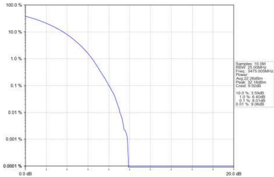
n78e 15kHz SISO NTN 50MHz CP-OFDM QPSK 3475.005MHz Outer Full Ant1
