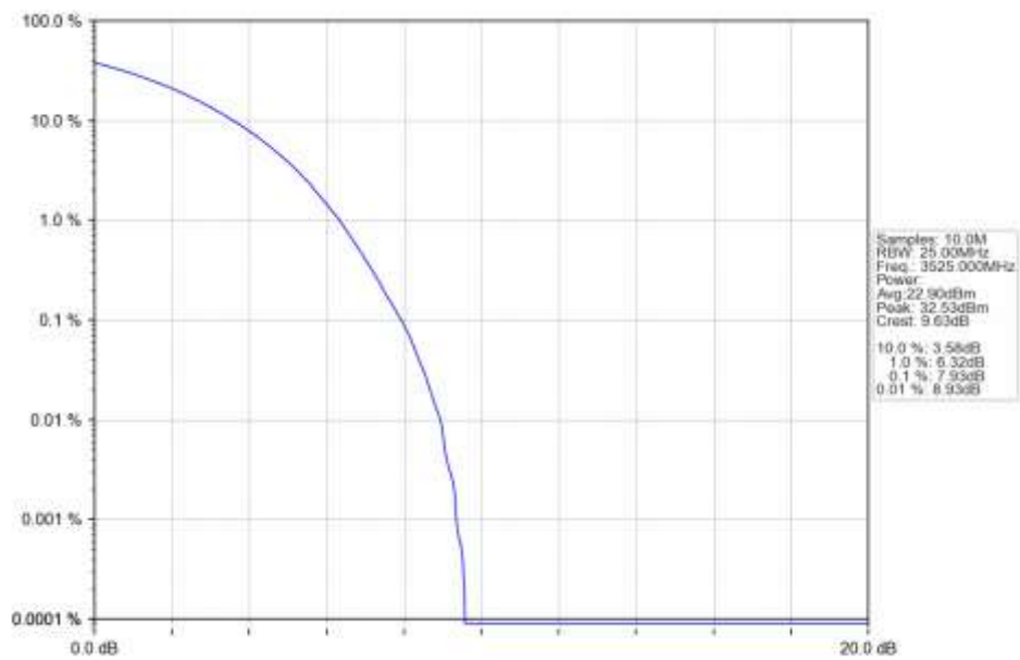
n78e 15kHz SISO NTN 50MHz CP-OFDM 16 QAM 3525MHz Outer Full Ant1
