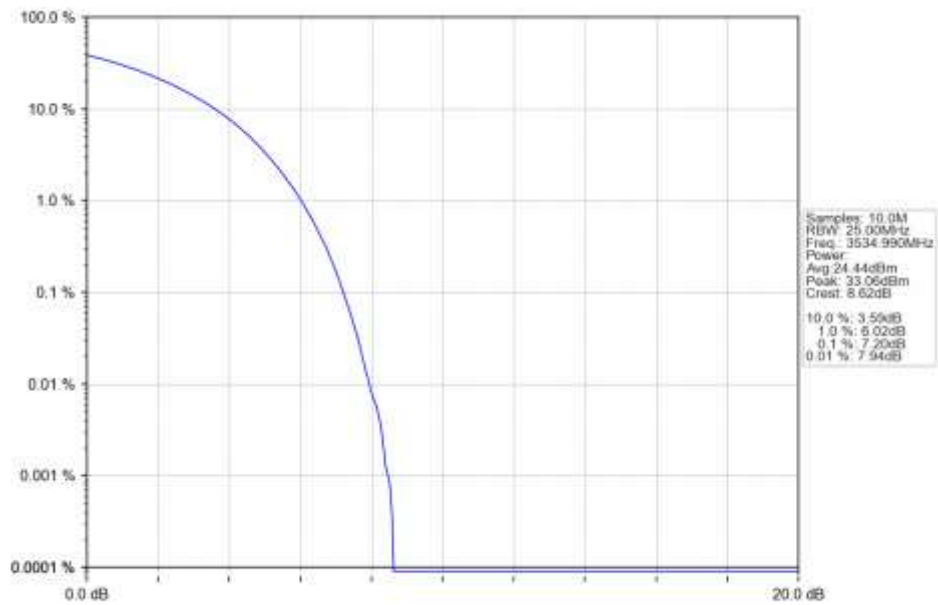
n78e 15kHz SISO NTN 30MHz CP-OFDM QPSK 3534.99MHz Outer Full Ant1
