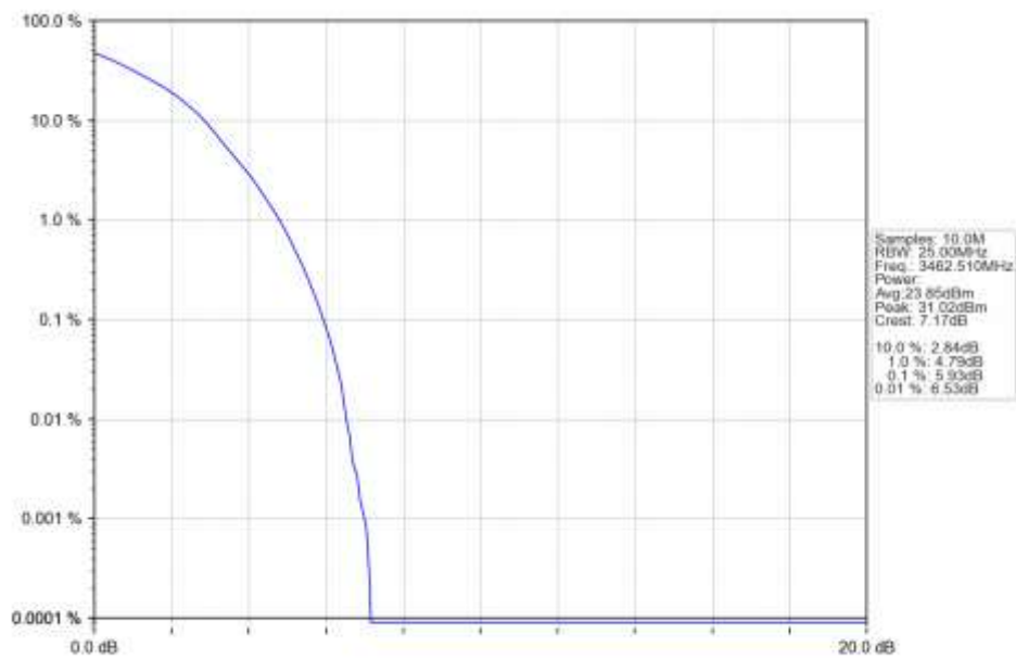
n78e 30kHz SISO NTN 25MHz DFT-s-OFDM 16 QAM 3462.51MHz Outer Full Ant1
