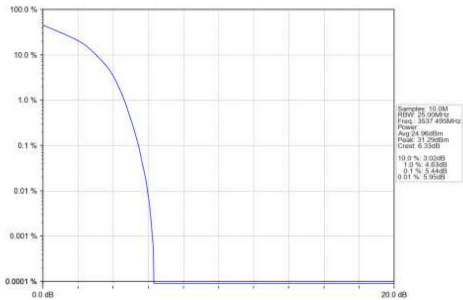
n78e 15kHz SISO NTN 25MHz DFT-s-OFDM 16 QAM 3537.495MHz Outer Full Ant1
