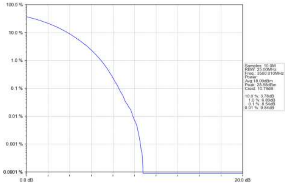
n78e 30kHz SISO NTN 50MHz CP-OFDM 256 QAM 3500.01MHz Outer Full Ant1
