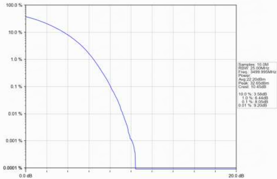
n78e 15kHz SISO NTN 50MHz CP-OFDM 64 QAM 3499.995MHz Outer Full Ant1
