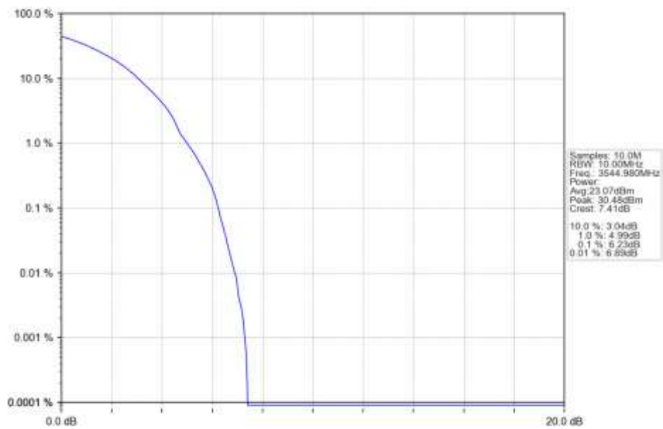
n78e 30kHz SISO NTN 10MHz DFT-s-OFDM 256 QAM 3544.98MHz Outer Full Ant1
