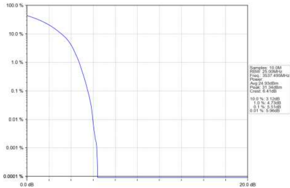
n78e 15kHz SISO NTN 25MHz DFT-s-OFDM 64 QAM 3537.495MHz Outer Full Ant1
