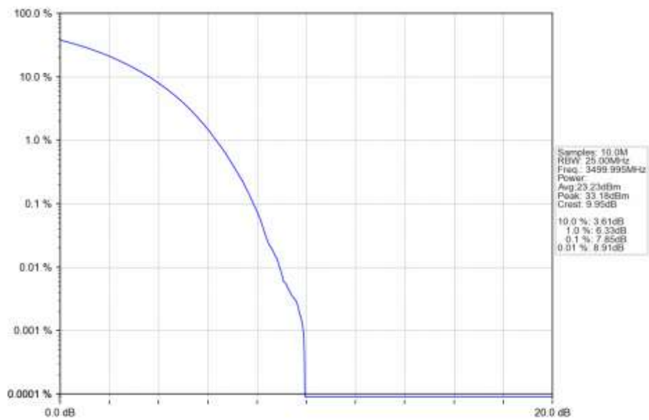
n78e 15kHz SISO NTN 40MHz CP-OFDM QPSK 3499.995MHz Outer Full Ant1
