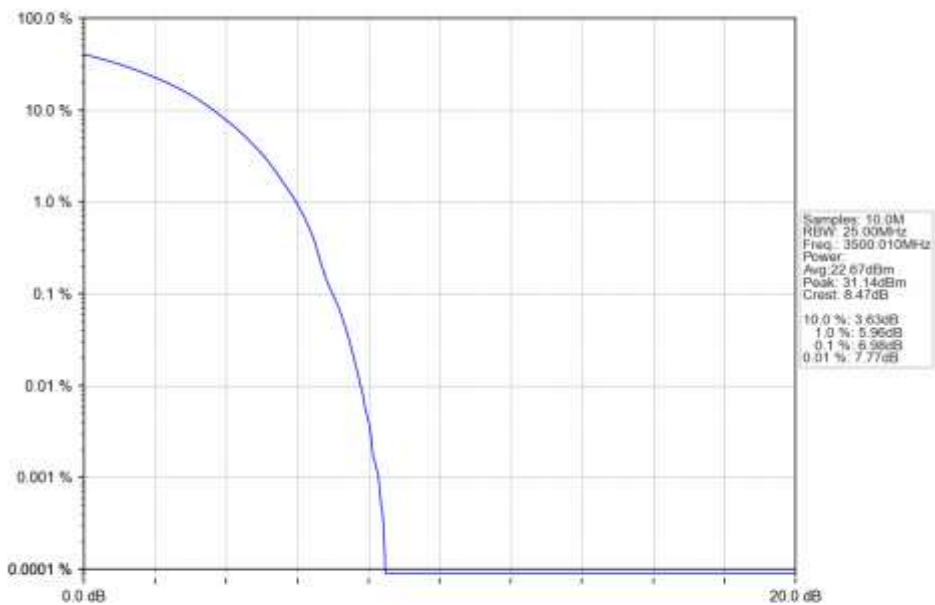
n78e_30kHz_SISO_NTNV_50MHz_DFT-s-OFDM QPSK_3500.01MHz_Outer_Full_Ant1
