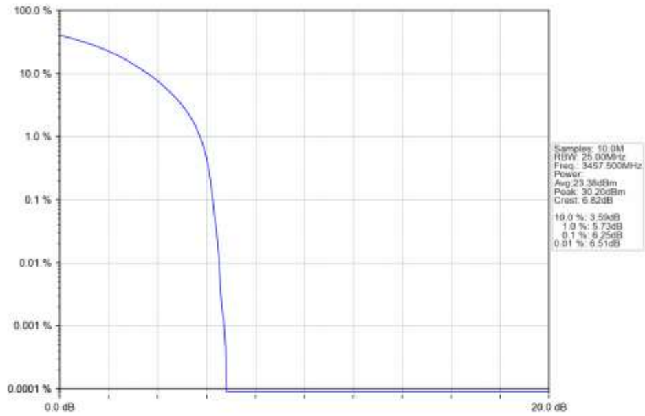
n78e 30kHz SISO NTN 15MHz CP-OFDM QPSK 3457.5MHz Outer Full Ant1
