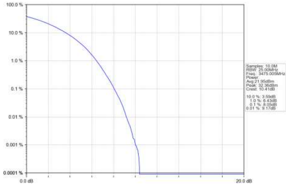
n78e 15kHz SISO NTN 50MHz CP-OFDM 64 QAM 3475.005MHz Outer Full Ant1
