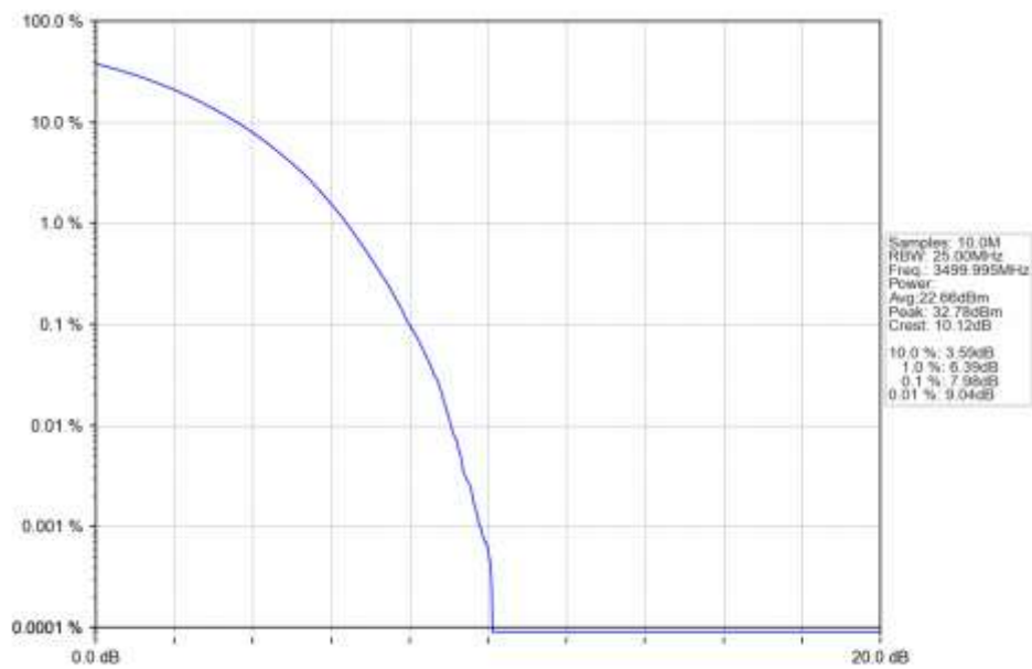
n78e 15kHz SISO NTN 50MHz CP-OFDM QPSK 3499.995MHz Outer Full Ant1
