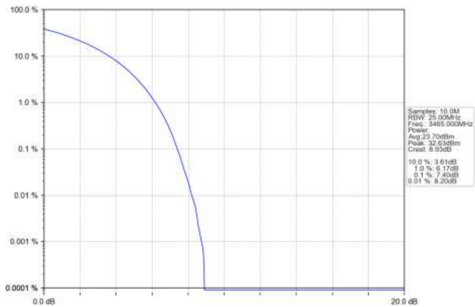
n78e 15kHz SISO NTN 30MHz CP-OFDM 16 QAM 3465MHz Outer Full Ant1
