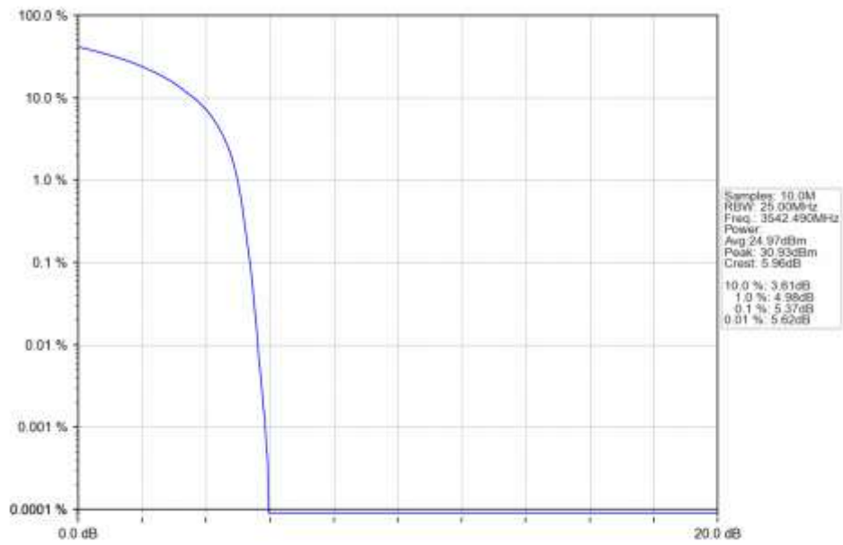
n78e 30kHz SISO NTN 15MHz CP-OFDM QPSK 3542.49MHz Outer Full Ant1
