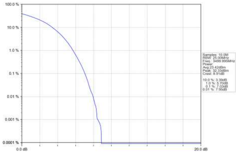
n78e 15kHz SISO NTN 40MHz DFT-s-OFDM 16 QAM 3499.995MHz Outer Full Ant1
