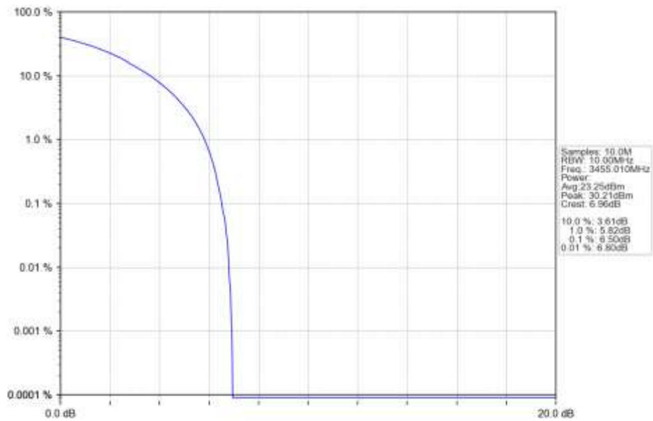
n78e 30kHz SISO NTN 10MHz CP-OFDM QPSK 3455.01MHz Outer Full Ant1
