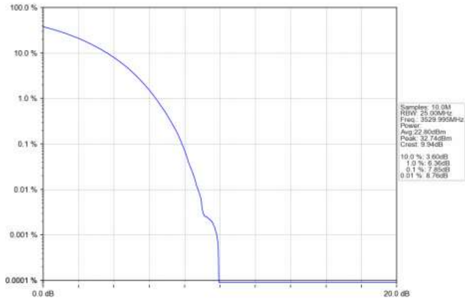
n78e 15kHz SISO NTN 40MHz CP-OFDM 64 QAM 3529.995MHz Outer Full Ant1
