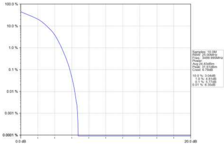
n78e 15kHz SISO NTN 25MHz DFT-s-OFDM 16 QAM 3499.995MHz Outer Full Ant1
