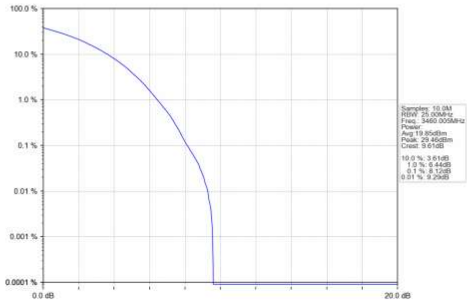
n78e 15kHz SISO NTN 20MHz CP-OFDM 256 QAM 3460.005MHz Outer Full Ant1
