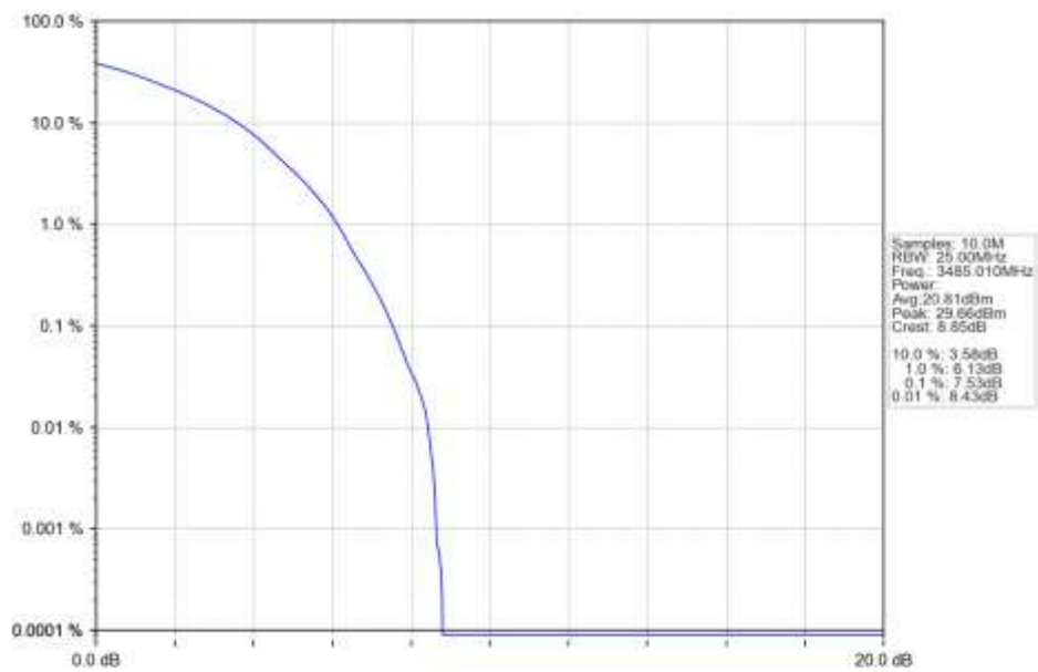
n78e 30kHz SISO NTN 70MHz DFT-s-OFDM 16 QAM 3485.01MHz Outer Full Ant1
