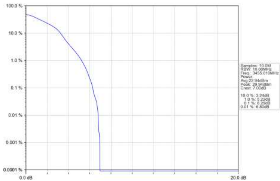
n78e 30kHz SISO NTN 10MHz DFT-s-OFDM 16 QAM 3455.01MHz Outer Full Ant1
