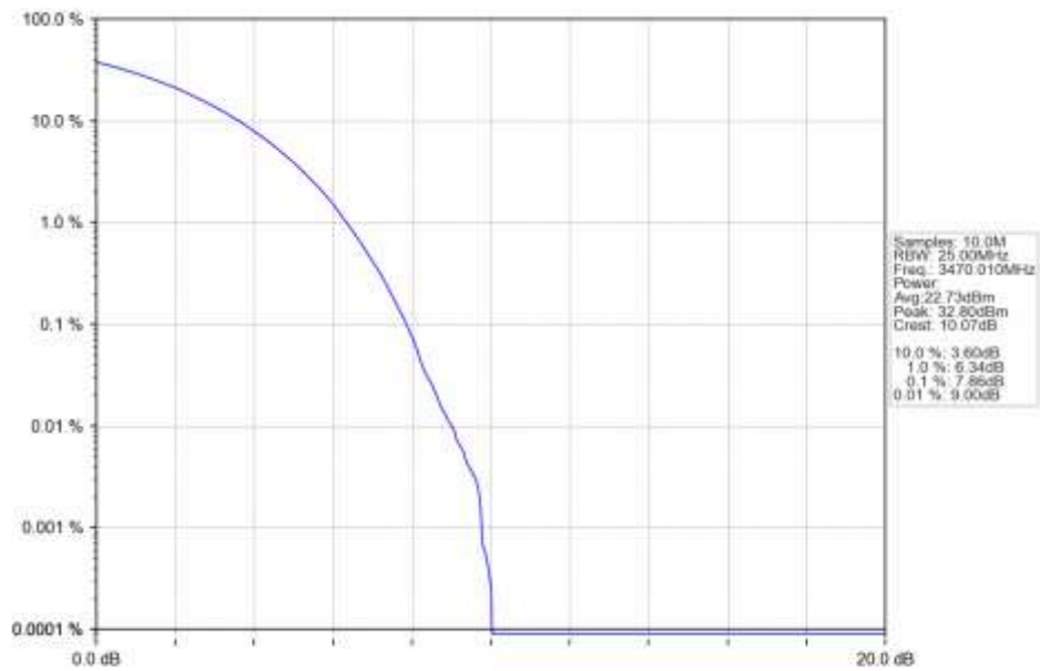
n78e 15kHz SISO NTN 40MHz CP-OFDM QPSK 3470.01MHz Outer Full Ant1
