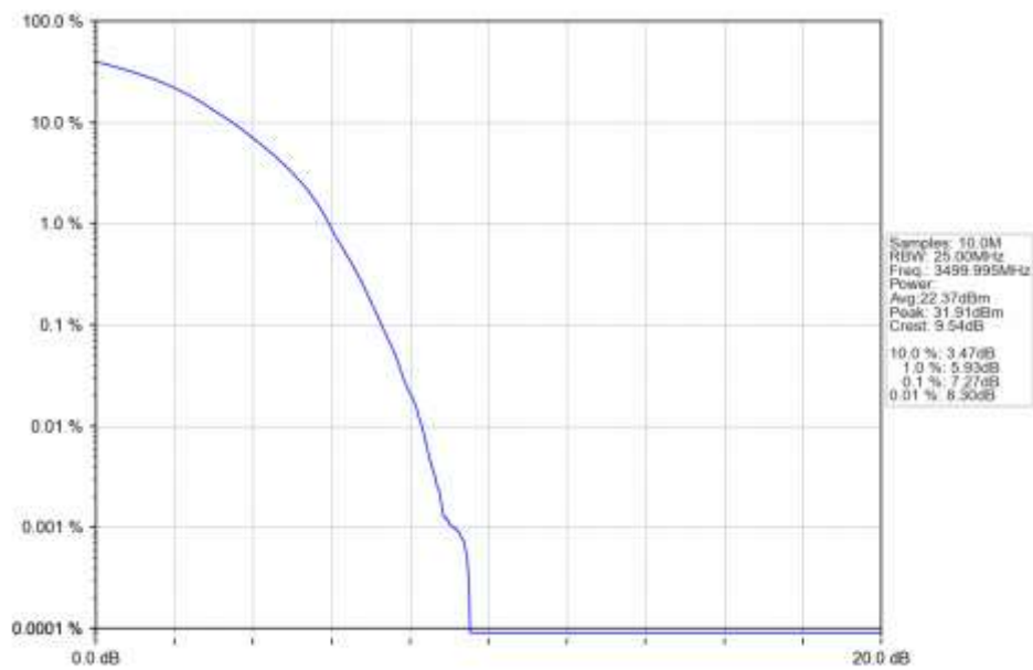
n78e 15kHz SISO NTN 50MHz DFT-s-OFDM 64 QAM 3499.995MHz Outer Full Ant1
