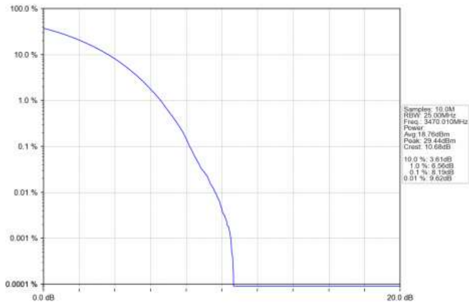
n78e 15kHz SISO NTN 40MHz CP-OFDM 256 QAM 3470.01MHz Outer Full Ant1
