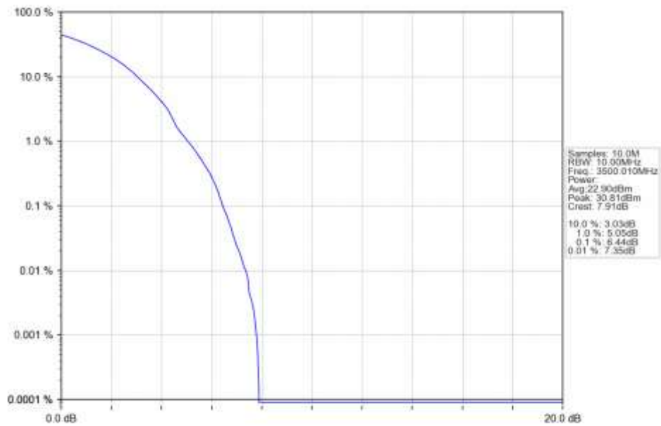
n78e 30kHz SISO NTN 10MHz DFT-s-OFDM 256 QAM 3500.01MHz Outer Full Ant1
