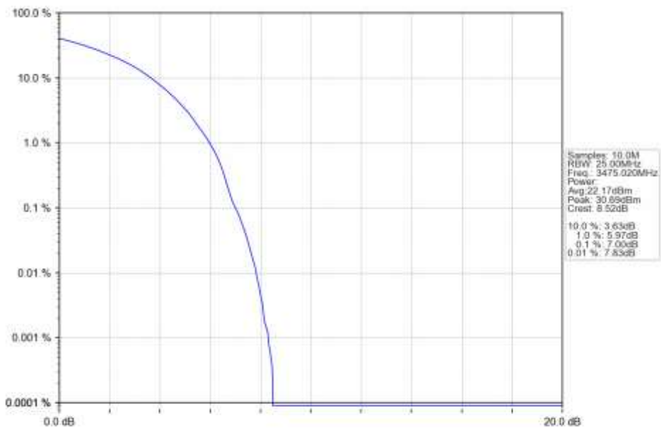
n78e_30kHz_SISO_NTNV_50MHz_DFT-s-OFDM QPSK_3475.02MHz_Outer_Full_Ant1
