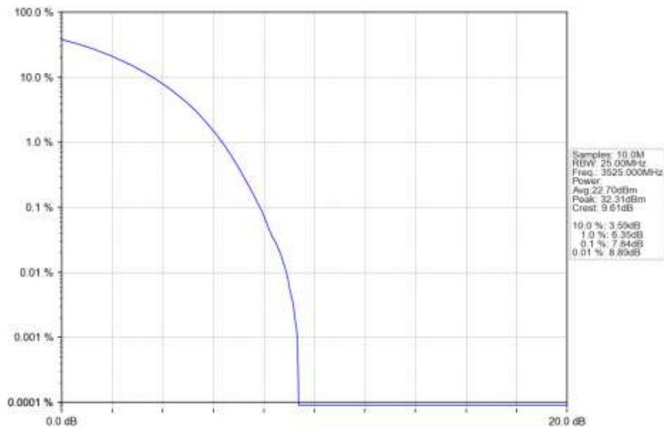
n78e 15kHz SISO NTN 50MHz CP-OFDM QPSK 3525MHz Outer Full Ant1
