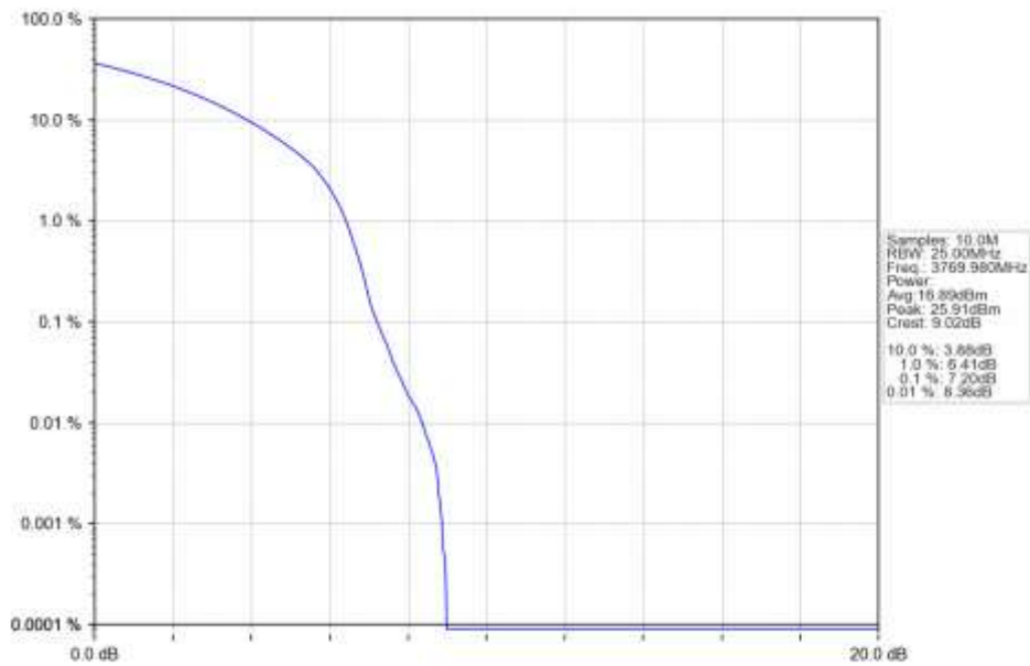
n78a 30kHz SISO NTN 60MHz DFT-s-OFDM 16 QAM 3769.98MHz Outer Full Ant1
