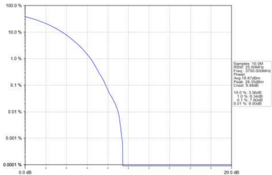
n78a 15kHz SISO NTN 50MHz CP-OFDM QPSK 3750MHz Outer Full Ant1
