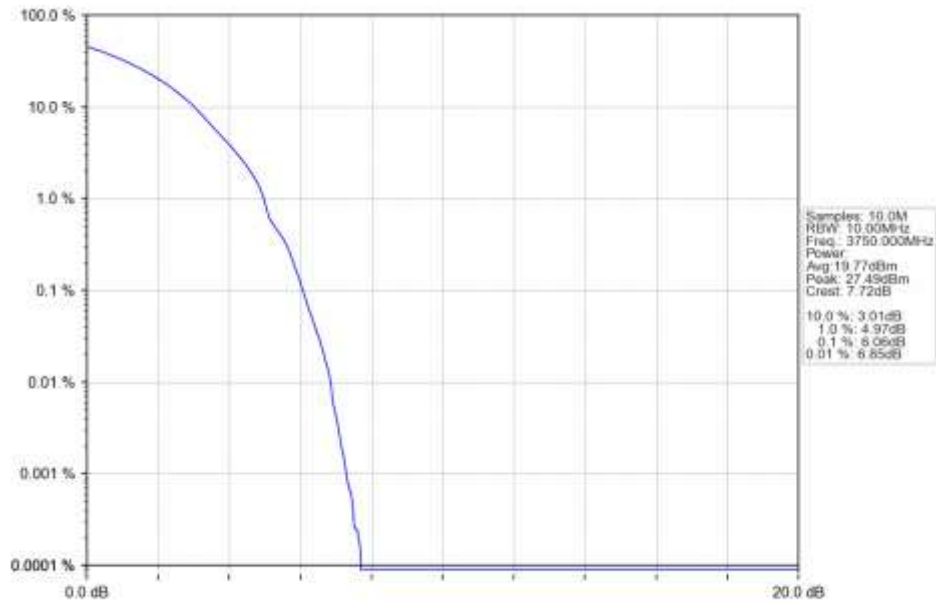
n78a 30kHz SISO NTN 10MHz DFT-s-OFDM 256 QAM 3750MHz Outer Full Ant1
