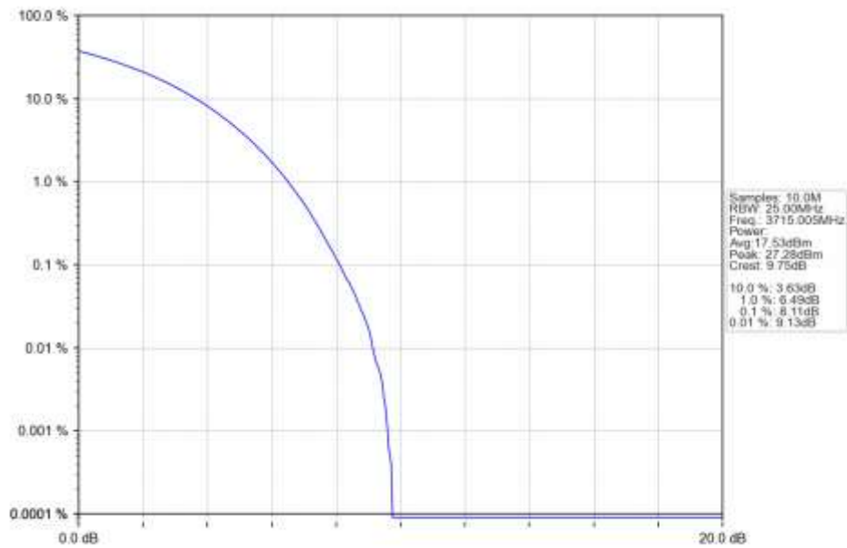
n78a 15kHz SISO NTN 30MHz CP-OFDM 256 QAM 3715.005MHz Outer Full Ant1
