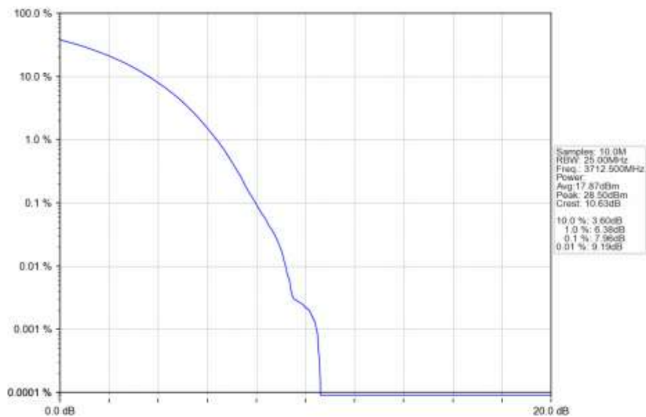
n78a 15kHz SISO NTN 25MHz CP-OFDM 256 QAM 3712.5MHz Outer Full Ant1
