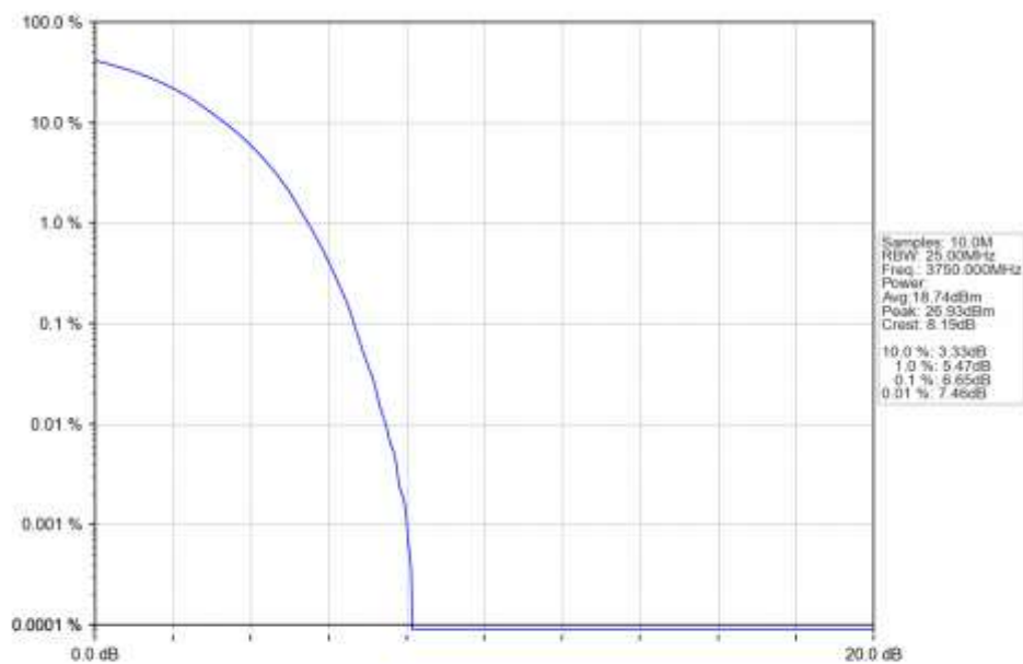
n78a_15kHz_SISO_NTNV_50MHz_DFT-s-OFDM QPSK_3750MHz_Outer_Full_Ant1
