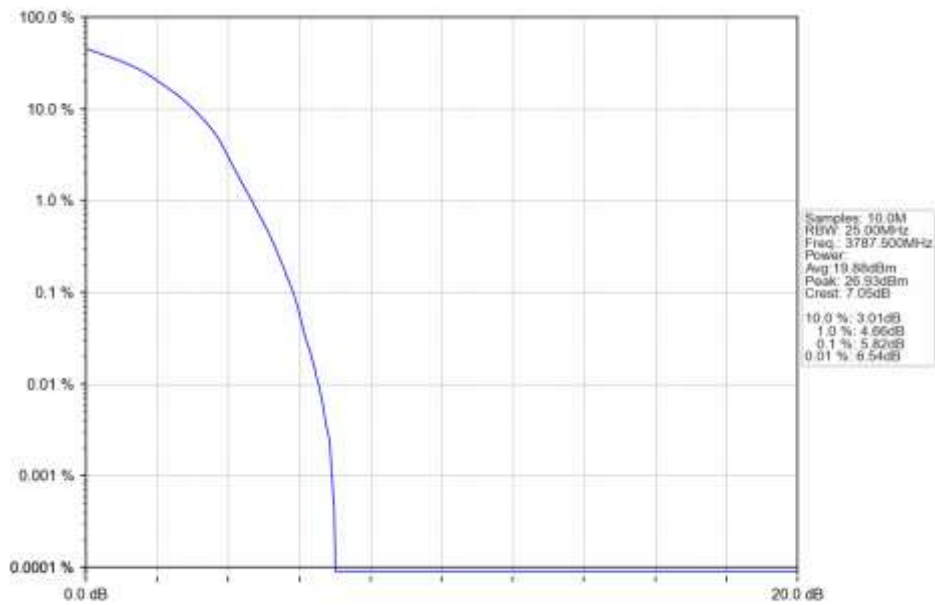
n78a 30kHz SISO NTN 25MHz DFT-s-OFDM 16 QAM 3787.5MHz Outer Full Ant1
