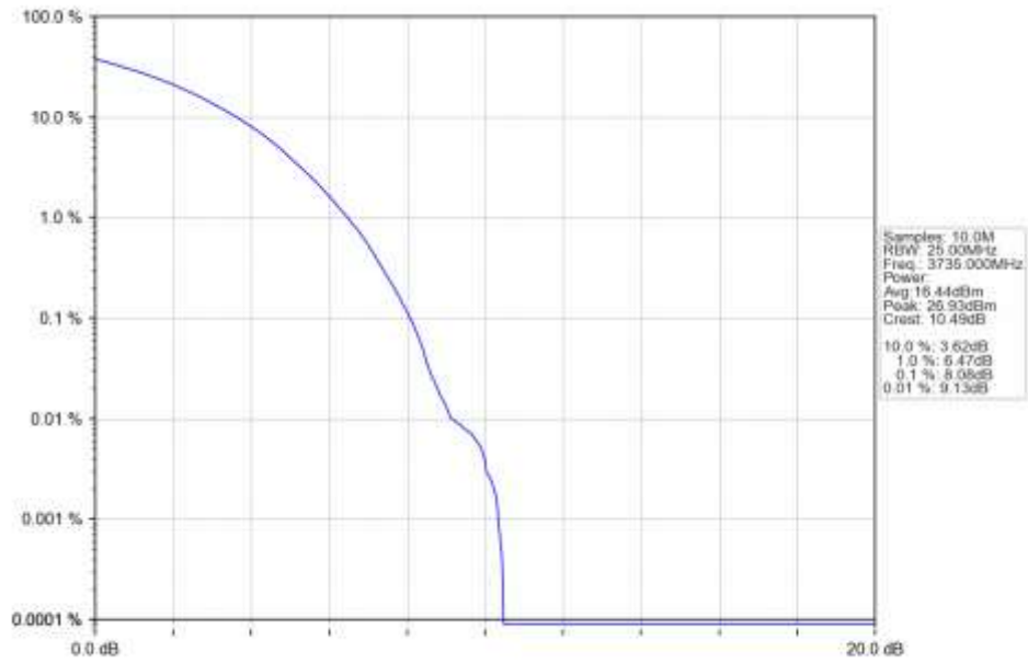
n78a 30kHz SISO NTN 70MHz CP-OFDM 64 QAM 3735MHz Outer Full Ant1
