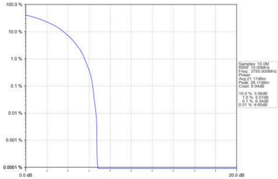
n78a 30kHz SISO NTN 10MHz CP-OFDM 16 QAM 3750MHz Outer Full Ant1
