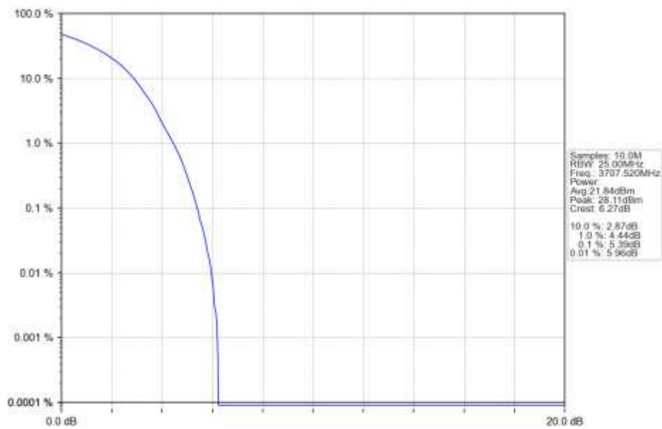
n78a 30kHz SISO NTN 15MHz DFT-s-OFDM 16 QAM 3707.52MHz Outer Full Ant1
