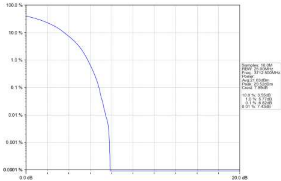
n78a 30kHz SISO NTN 25MHz CP-OFDM 16 QAM 3712.5MHz Outer Full Ant1
