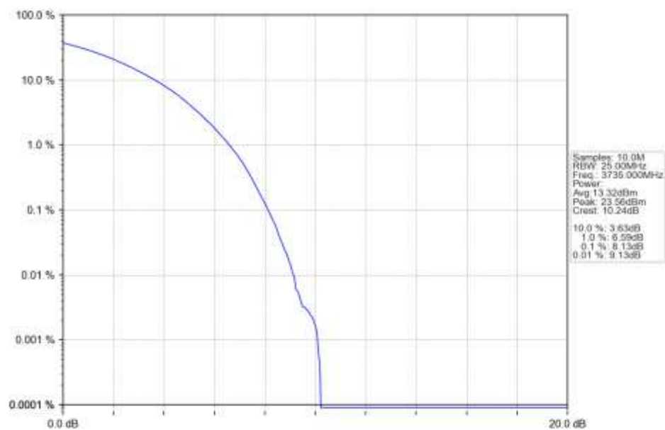
n78a 30kHz SISO NTN 70MHz CP-OFDM 256 QAM 3735MHz Outer Full Ant1
