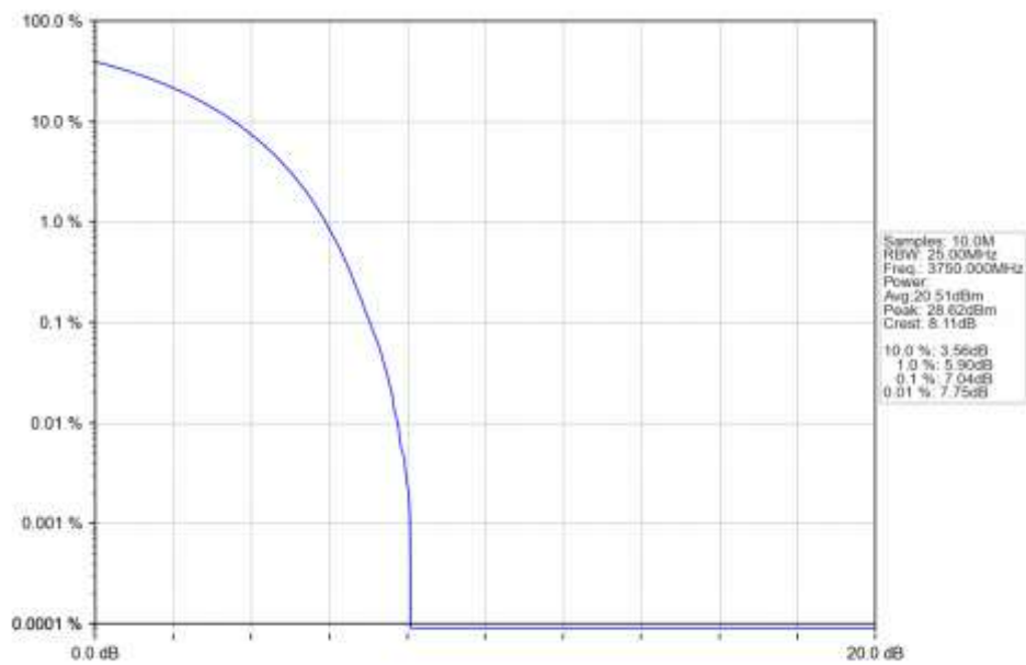
n78a 15kHz SISO NTN 25MHz CP-OFDM 64 QAM 3750MHz Outer Full Ant1
