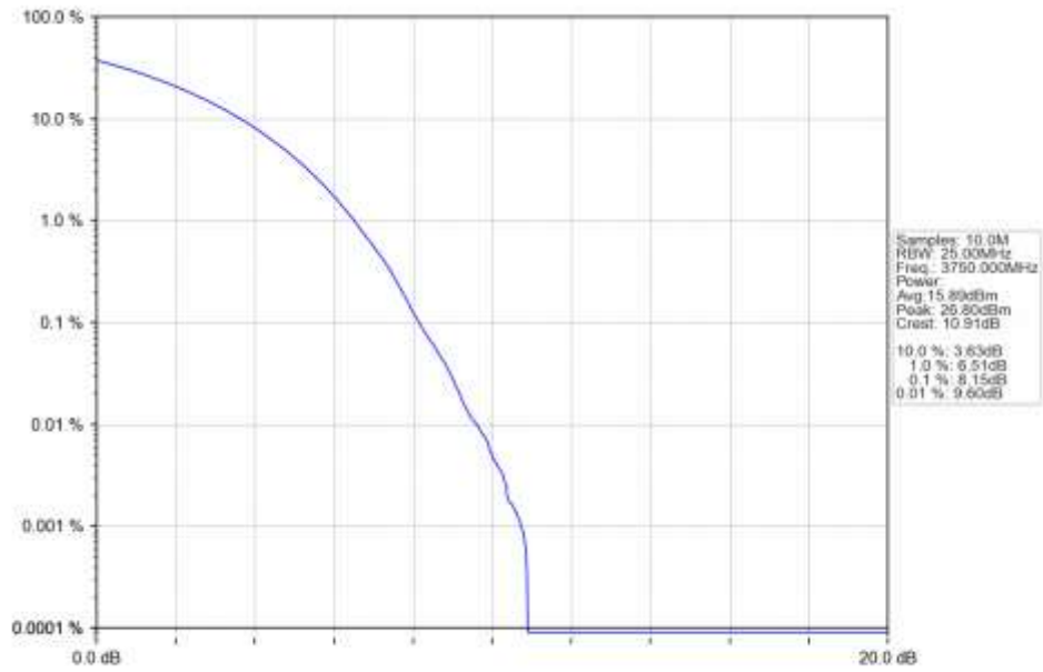
n78a 15kHz SISO NTN 40MHz CP-OFDM 256 QAM 3750MHz Outer Full Ant1
