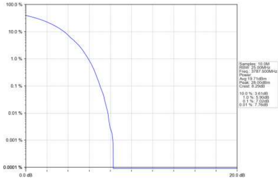
n78a 30kHz SISO NTN 25MHz CP-OFDM QPSK 3787.5MHz Outer Full Ant1
