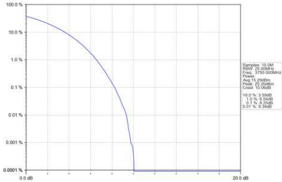
n78a 15kHz SISO NTN 50MHz CP-OFDM 256 QAM 3750MHz Outer Full Ant1
