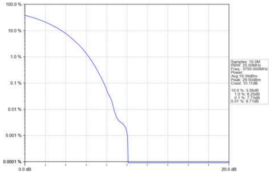
n78a 15kHz SISO NTN 40MHz CP-OFDM 16 QAM 3750MHz Outer Full Ant1
