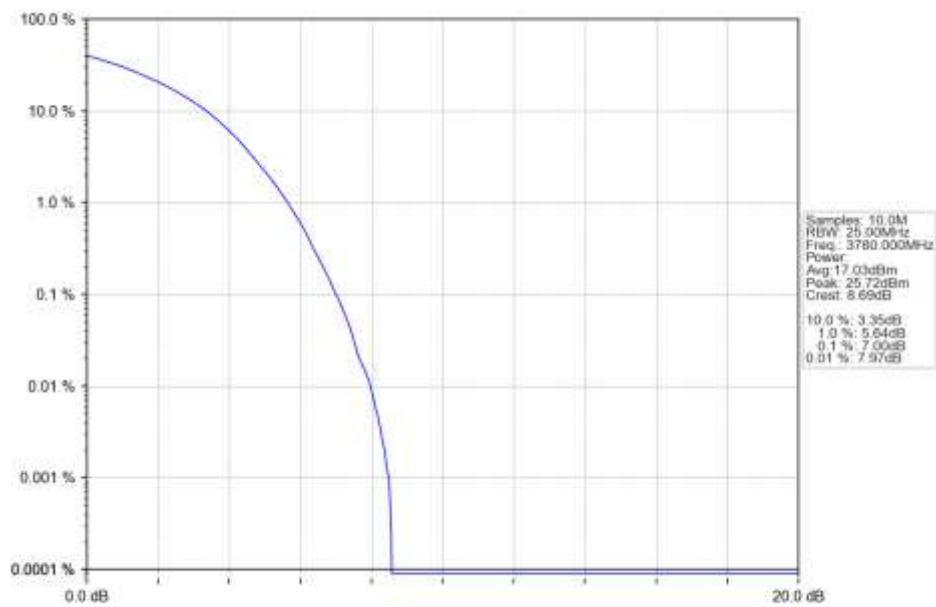
n78a 15kHz SISO NTN 40MHz DFT-s-OFDM 256 QAM 3780MHz Outer Full Ant1
