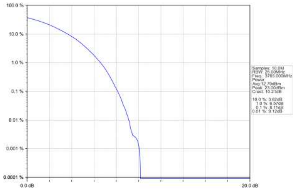
n78a 30kHz SISO NTN 70MHz CP-OFDM 256 QAM 3765MHz Outer Full Ant1
