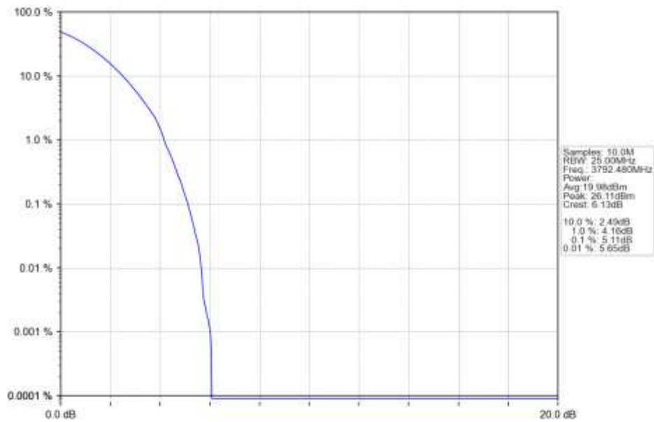
n78a 30kHz SISO NTN 15MHz DFT-s-OFDM QPSK 3792.48MHz Outer Full Ant1
