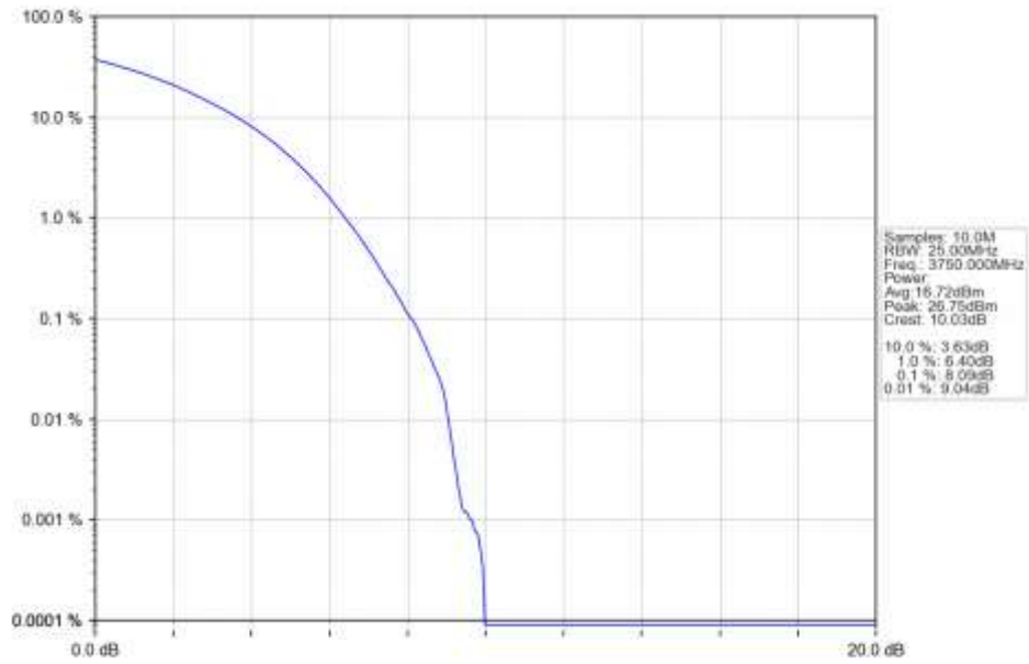
n78a 30kHz SISO NTN 70MHz CP-OFDM 16 QAM 3750MHz Outer Full Ant1
