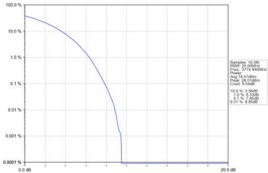
n78a 15kHz SISO NTN 50MHz CP-OFDM 16 QAM 3774.99MHz Outer Full Ant1
