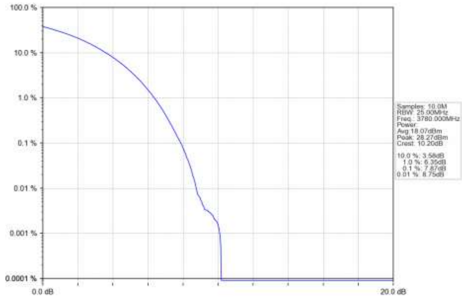
n78a 15kHz SISO NTN 40MHz CP-OFDM 64 QAM 3780MHz Outer Full Ant1
