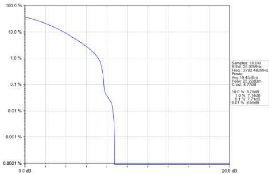
n78a 30kHz SISO NTN 15MHz CP-OFDM 256 QAM 3792.48MHz Outer Full Ant1
