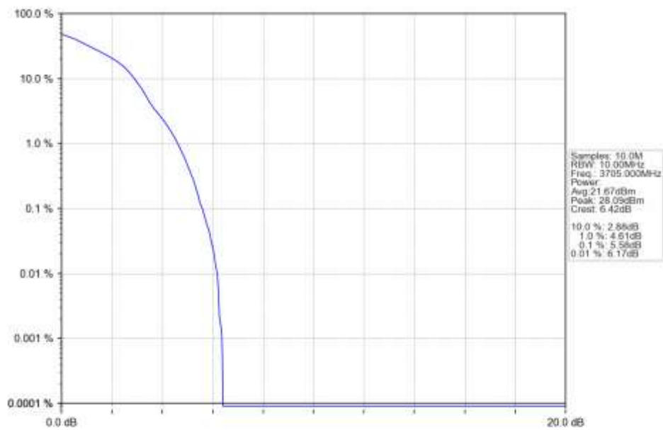
n78a 30kHz SISO NTN 10MHz DFT-s-OFDM 16 QAM 3705MHz Outer Full Ant1
