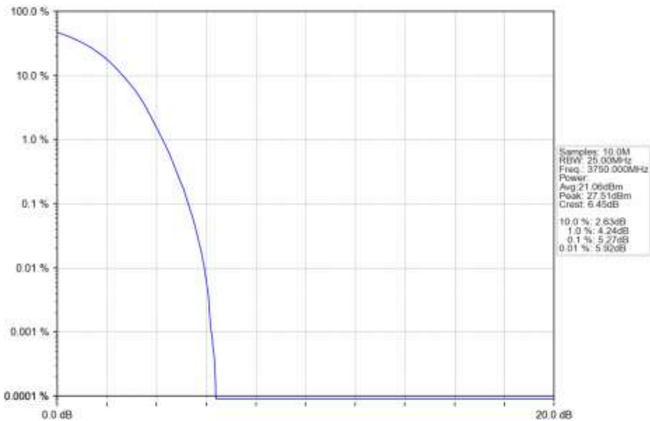
n78a_30kHz_SISO_NTNV_30MHz_DFT-s-OFDM QPSK_3750MHz_Outer_Full_Ant1
