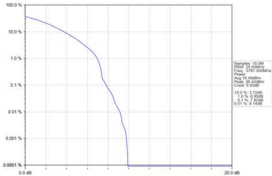
n78a 30kHz SISO NTN 25MHz CP-OFDM 256 QAM 3787.5MHz Outer Full Ant1
