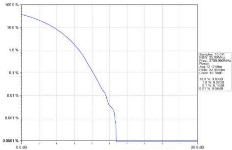
n78a 30kHz SISO NTN 80MHz CP-OFDM 256 QAM 3759.99MHz Outer Full Ant1
