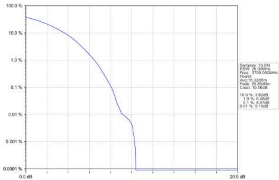
n78a 30kHz SISO NTN 70MHz CP-OFDM 64 QAM 3750MHz Outer Full Ant1
