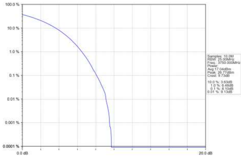
n78a 15kHz SISO NTN 30MHz CP-OFDM 256 QAM 3750MHz Outer Full Ant1
