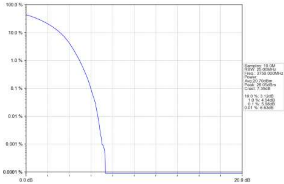
n78a 15kHz SISO NTN 30MHz DFT-s-OFDM 16 QAM 3750MHz Outer Full Ant1
