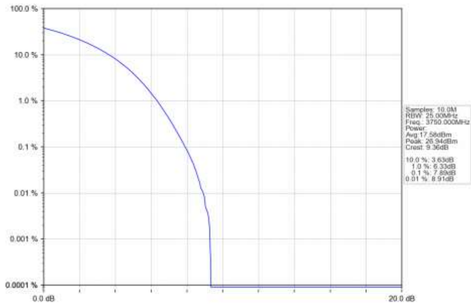
n78a 15kHz SISO NTN 20MHz CP-OFDM 256 QAM 3750MHz Outer Full Ant1
