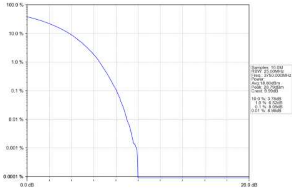
n78a 30kHz SISO NTN 40MHz CP-OFDM 16 QAM 3750MHz Outer Full Ant1
