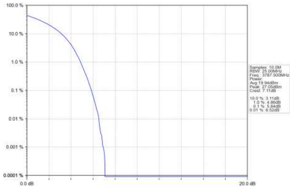
n78a 15kHz SISO NTN 25MHz DFT-s-OFDM 64 QAM 3787.5MHz Outer Full Ant1
