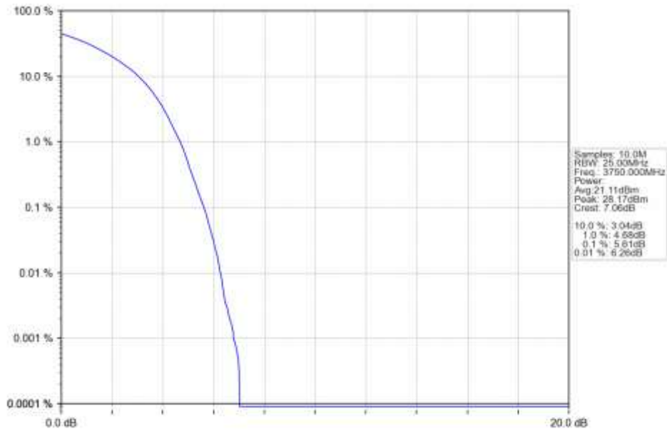
n78a 15kHz SISO NTN 25MHz DFT-s-OFDM 16 QAM 3750MHz Outer Full Ant1
