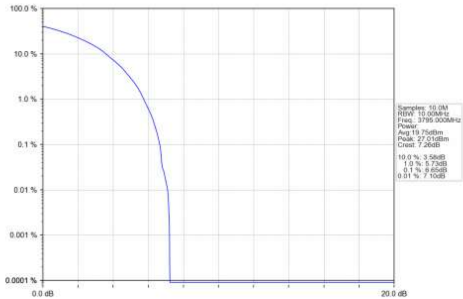
n78a 30kHz SISO NTN 10MHz CP-OFDM 16 QAM 3795MHz Outer Full Ant1
