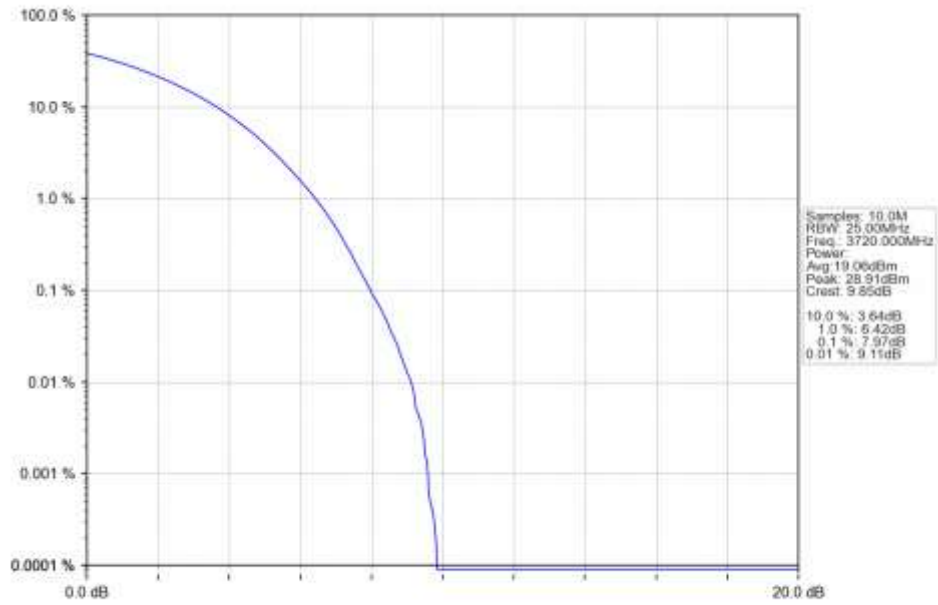
n78a 30kHz SISO NTN 40MHz CP-OFDM 64 QAM 3720MHz Outer Full Ant1
