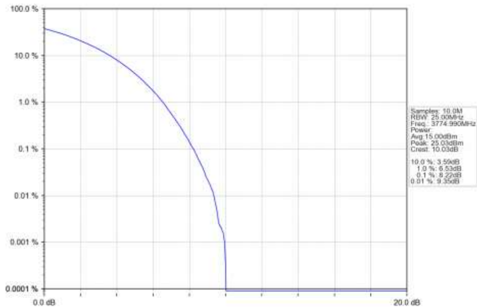
n78a 15kHz SISO NTN 50MHz CP-OFDM 256 QAM 3774.99MHz Outer Full Ant1
