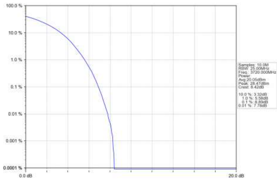
n78a 15kHz SISO NTN 40MHz DFT-s-OFDM 16 QAM 3720MHz Outer Full Ant1
