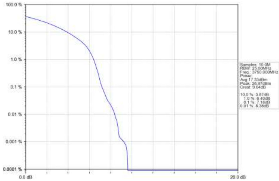
n78a 30kHz SISO NTN 60MHz DFT-s-OFDM 16 QAM 3750MHz Outer Full Ant1
