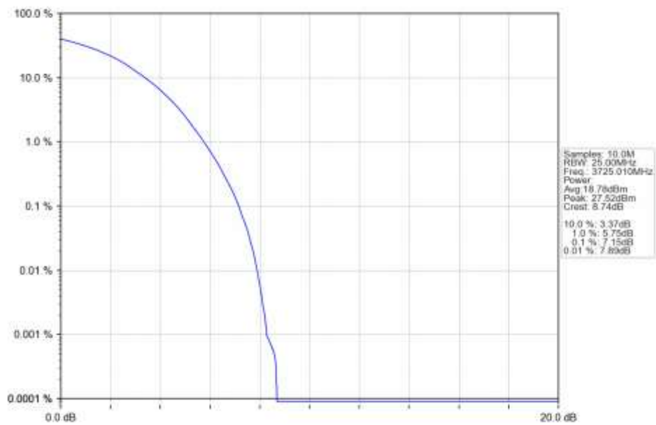
n78a 15kHz SISO NTN 50MHz DFT-s-OFDM 16 QAM 3725.01MHz Outer Full Ant1
