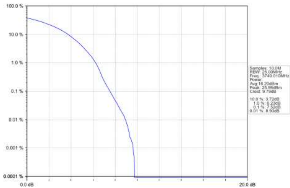
n78a 30kHz SISO NTN 80MHz DFT-s-OFDM 16 QAM 3740.01MHz Outer Full Ant1
