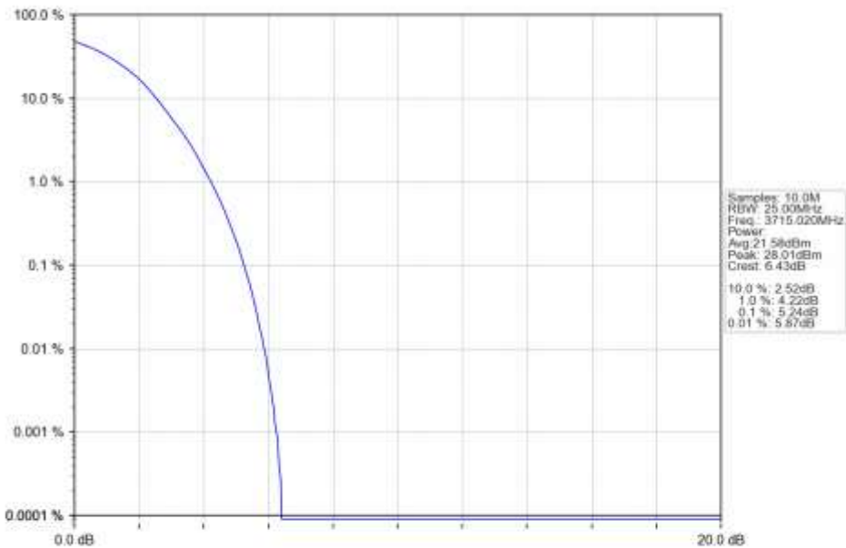
n78a_30kHz_SISO_NTNV_30MHz_DFT-s-OFDM QPSK_3715.02MHz_Outer_Full_Ant1
