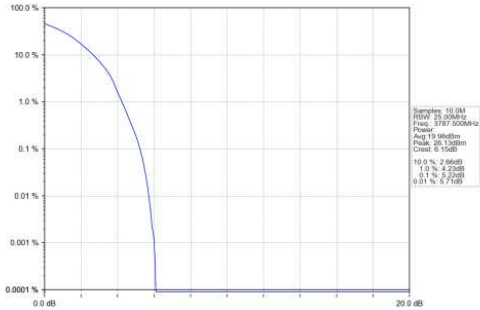
n78a 30kHz SISO NTN 25MHz DFT-s-OFDM QPSK 3787.5MHz Outer Full Ant1
