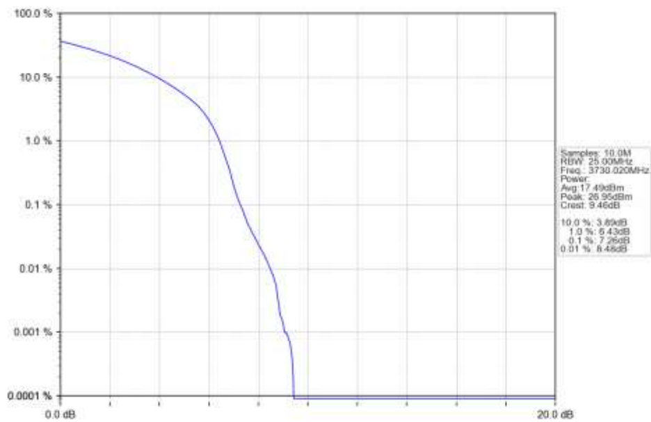
n78a 30kHz SISO NTN 60MHz DFT-s-OFDM 16 QAM 3730.02MHz Outer Full Ant1
