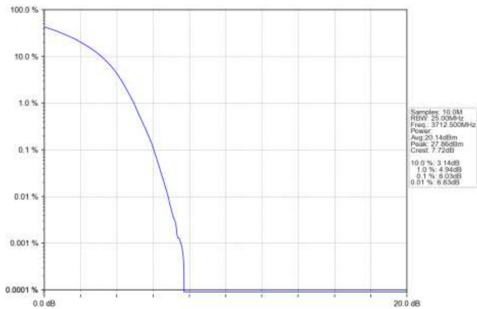
n78a 15kHz SISO NTN 25MHz DFT-s-OFDM 256 QAM 3712.5MHz Outer Full Ant1
