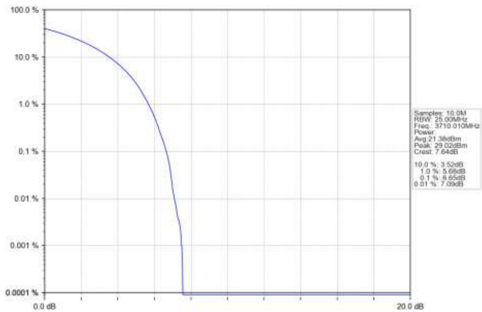
n78a 15kHz SISO NTN 20MHz CP-OFDM 16 QAM 3710.01MHz Outer Full Ant1
