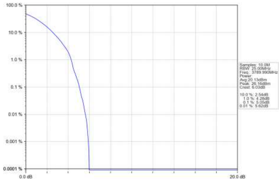
n78a 30kHz SISO NTN 20MHz DFT-s-OFDM QPSK 3789.99MHz Outer Full Ant1
