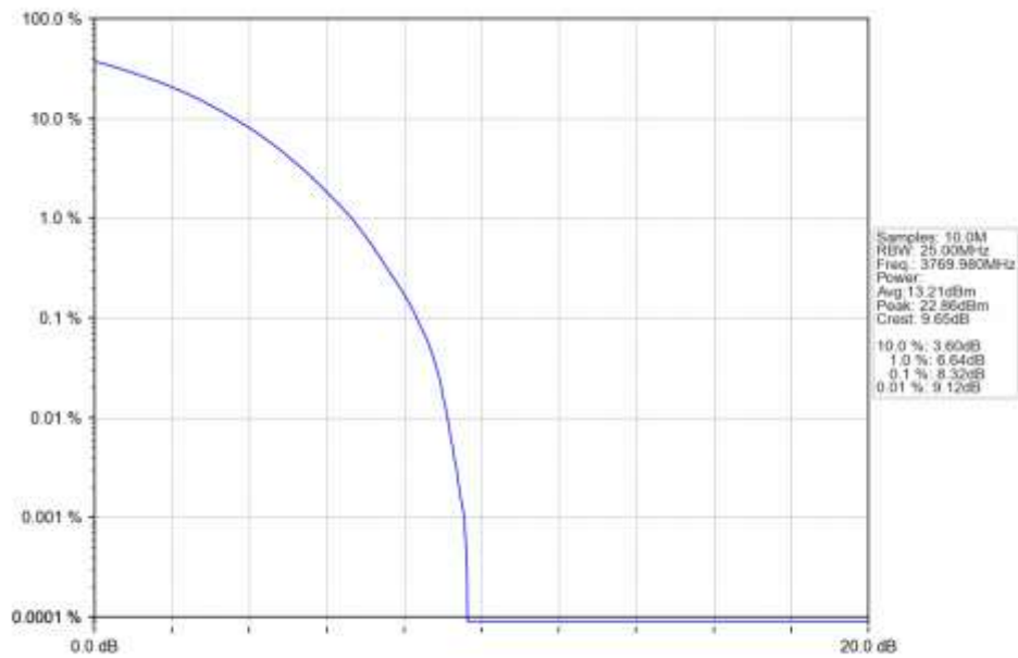
n78a 30kHz SISO NTN 60MHz CP-OFDM 256 QAM 3769.98MHz Outer Full Ant1
