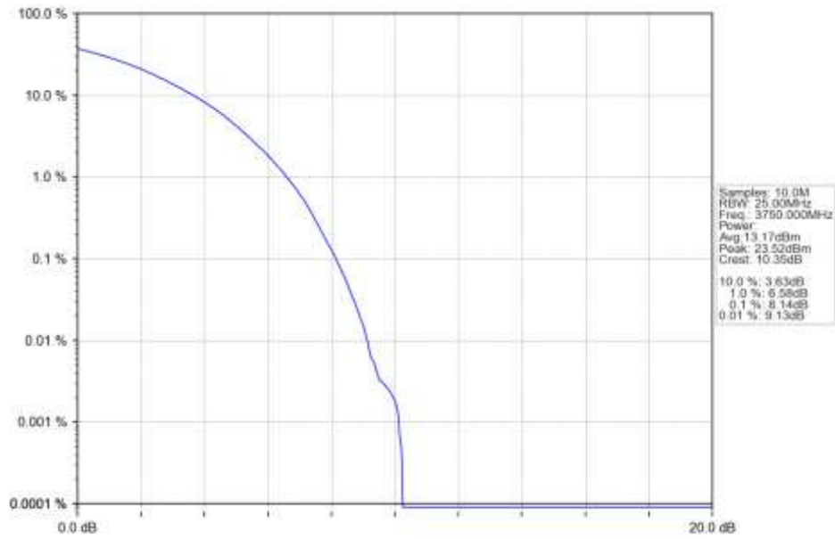
n78a 30kHz SISO NTN 70MHz CP-OFDM 256 QAM 3750MHz Outer Full Ant1
