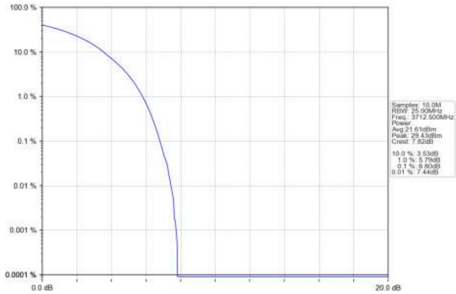
n78a 30kHz SISO NTN 25MHz CP-OFDM QPSK 3712.5MHz Outer Full Ant1
