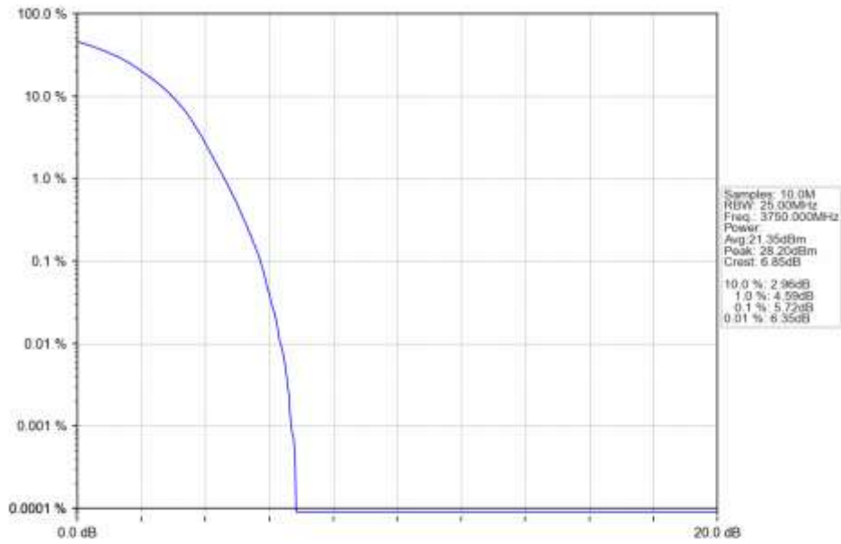
n78a 30kHz SISO NTN 25MHz DFT-s-OFDM 16 QAM 3750MHz Outer Full Ant1
