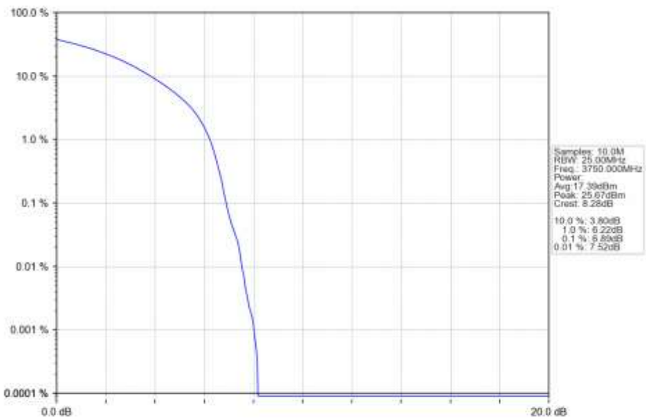
n78a_30kHz_SISO_NTNV_60MHz_DFT-s-OFDM QPSK_3750MHz_Outer_Full_Ant1
