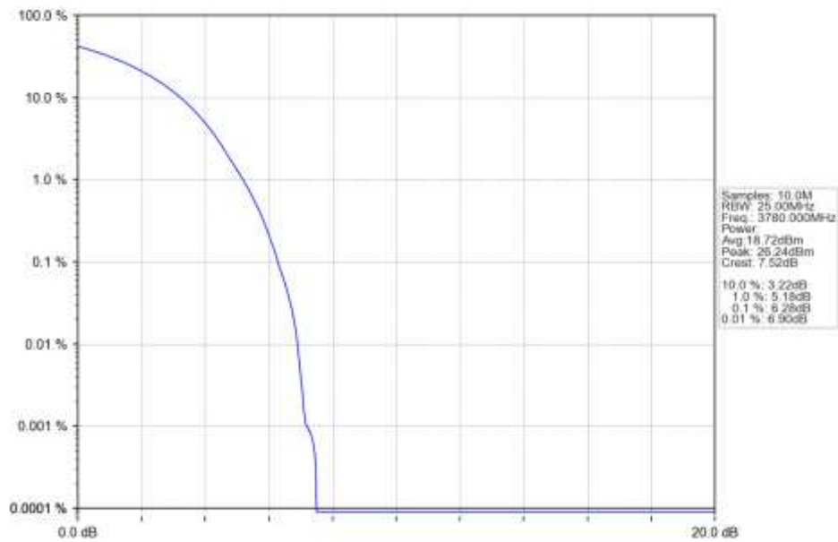
n78a 15kHz SISO NTN 40MHz DFT-s-OFDM QPSK 3780MHz Outer Full Ant1
