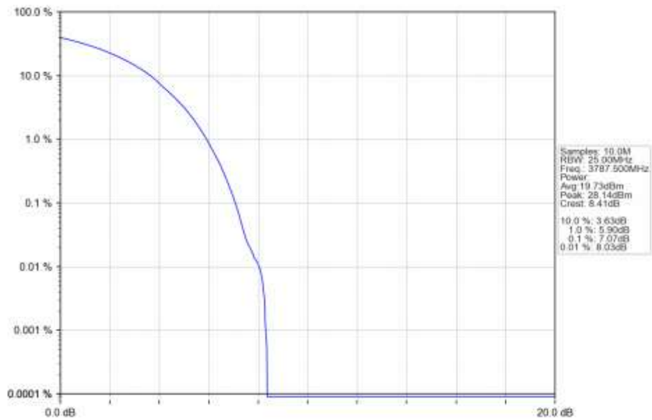
n78a 30kHz SISO NTN 25MHz CP-OFDM 16 QAM 3787.5MHz Outer Full Ant1
