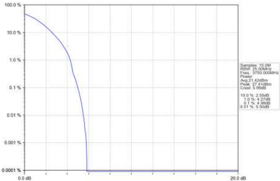
n78a_30kHz_SISO_NTNV_20MHz_DFT-s-OFDM QPSK_3750MHz_Outer_Full_Ant1
