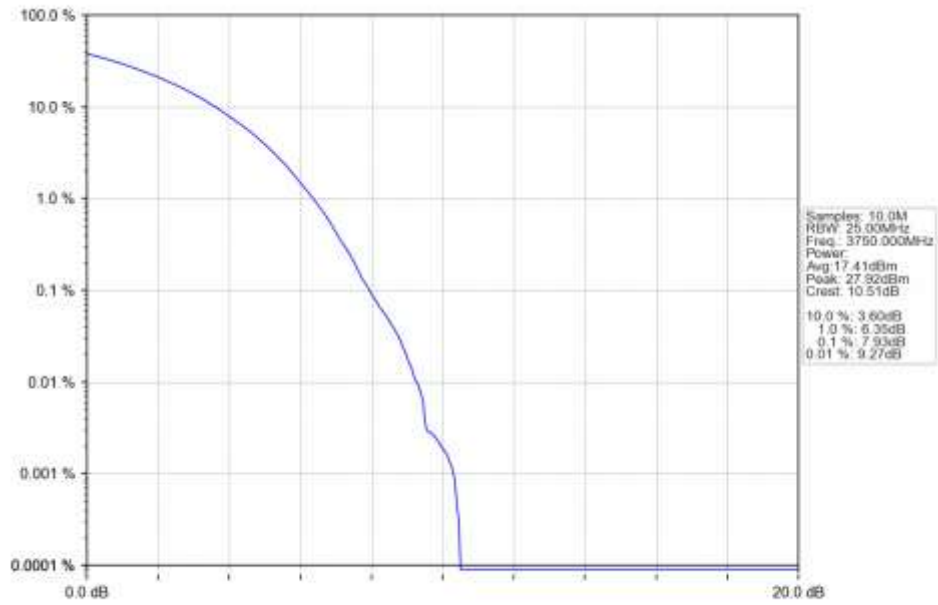
n78a 15kHz SISO NTN 25MHz CP-OFDM 256 QAM 3750MHz Outer Full Ant1
