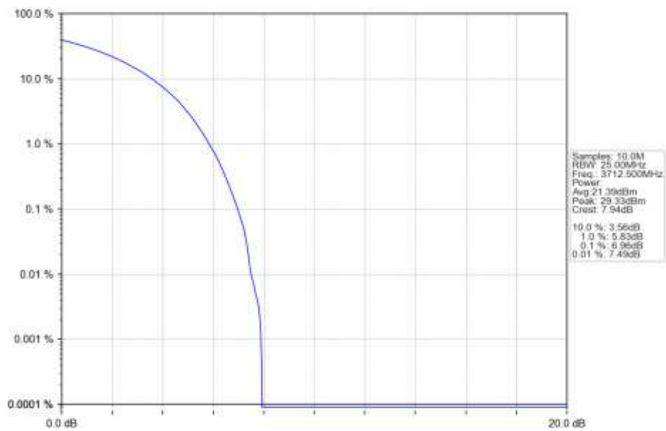
n78a 15kHz SISO NTN 25MHz CP-OFDM 16 QAM 3712.5MHz Outer Full Ant1
