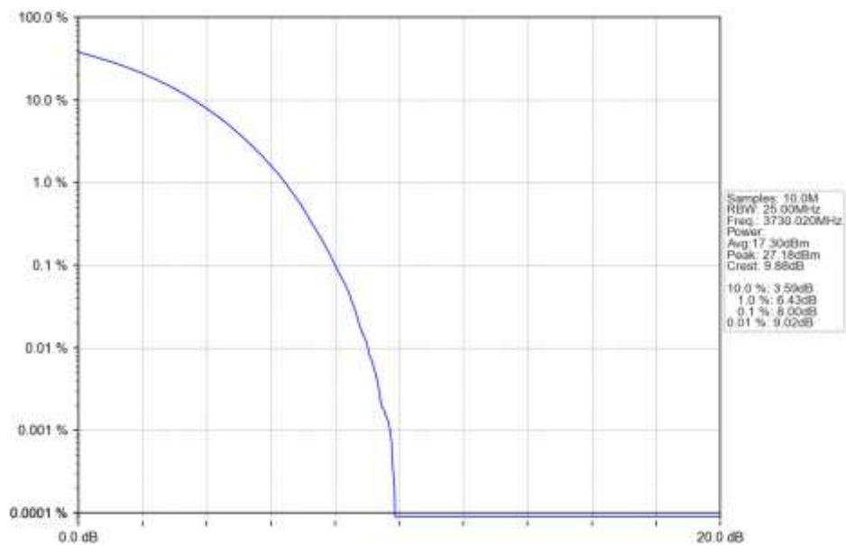
n78a 30kHz SISO NTN 60MHz CP-OFDM 16 QAM 3730.02MHz Outer Full Ant1
