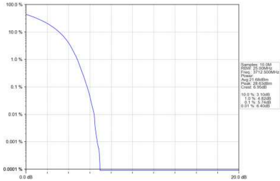
n78a 15kHz SISO NTN 25MHz DFT-s-OFDM 64 QAM 3712.5MHz Outer Full Ant1
