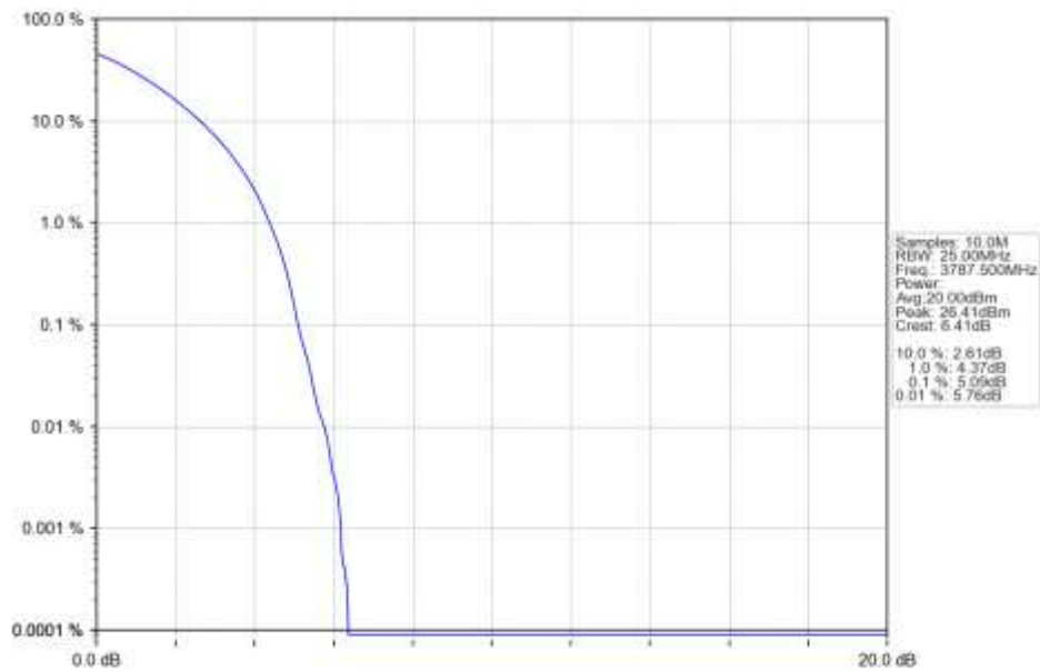
n78a 15kHz SISO NTN 25MHz DFT-s-OFDM QPSK 3787.5MHz Outer Full Ant1
