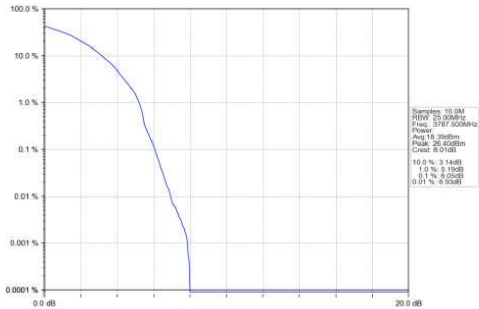
n78a 30kHz SISO NTN 25MHz DFT-s-OFDM 256 QAM 3787.5MHz Outer Full Ant1
