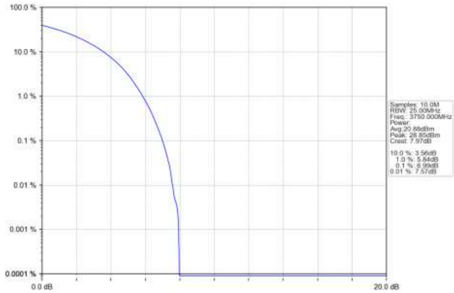
n78a 15kHz SISO NTN 25MHz CP-OFDM 16 QAM 3750MHz Outer Full Ant1
