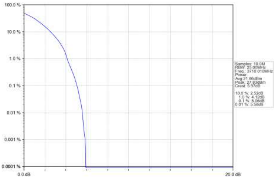
n78a_30kHz_SISO_NTNV_20MHz_DFT-s-OFDM QPSK_3710.01MHz_Outer_Full_Ant1
