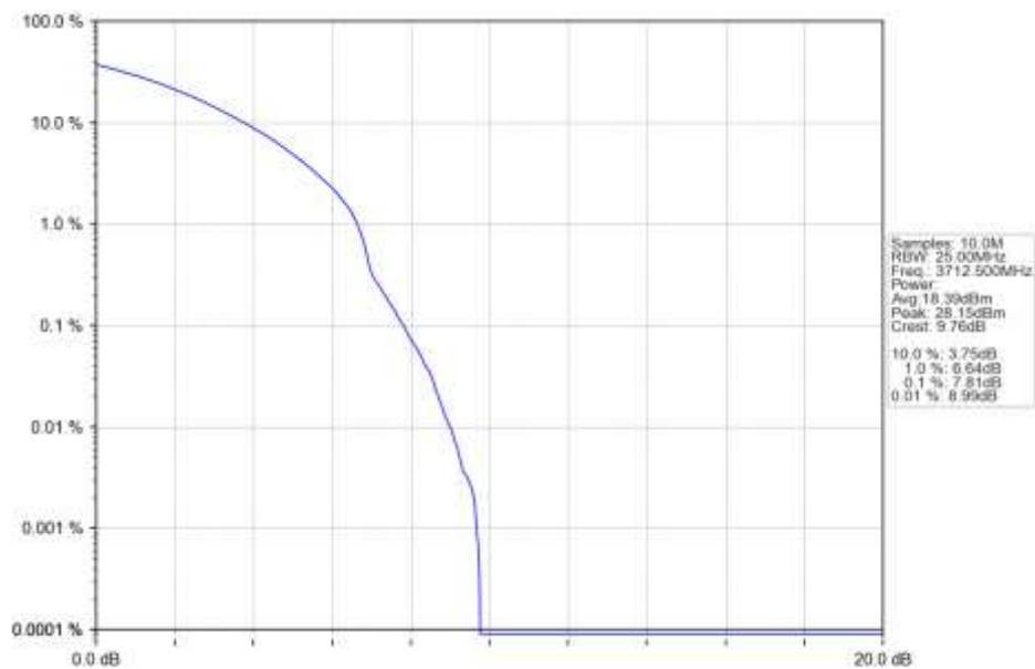
n78a 30kHz SISO NTN 25MHz CP-OFDM 256 QAM 3712.5MHz Outer Full Ant1
