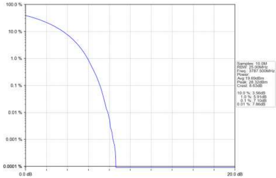
n78a 15kHz SISO NTN 25MHz CP-OFDM QPSK 3787.5MHz Outer Full Ant1
