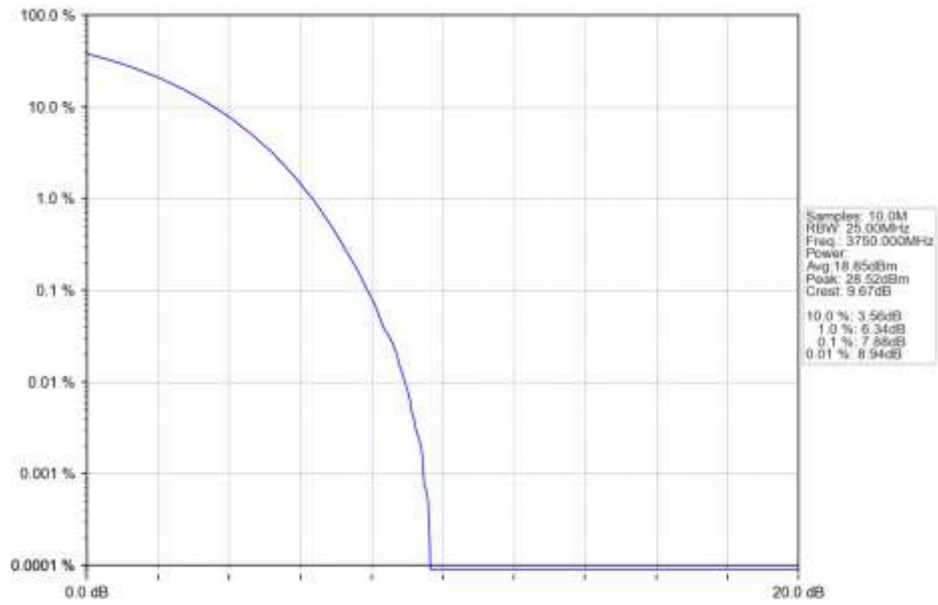
n78a 15kHz SISO NTN 50MHz CP-OFDM 16 QAM 3750MHz Outer Full Ant1
