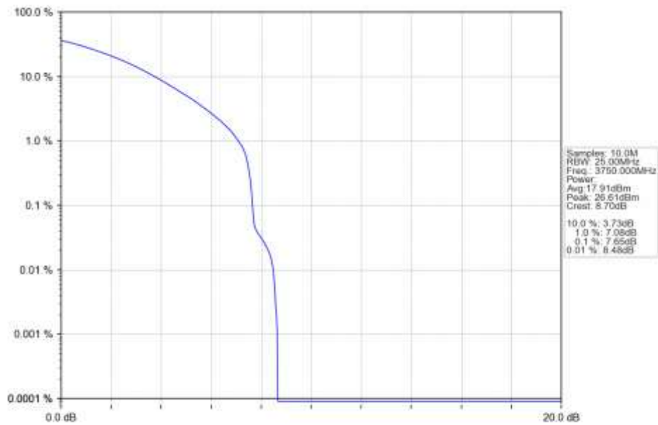
n78a 30kHz SISO NTN 15MHz CP-OFDM 256 QAM 3750MHz Outer Full Ant1
