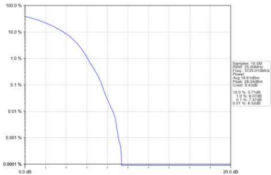
n78a 30kHz SISO NTN 50MHz DFT-s-OFDM 16 QAM 3725.01MHz Outer Full Ant1
