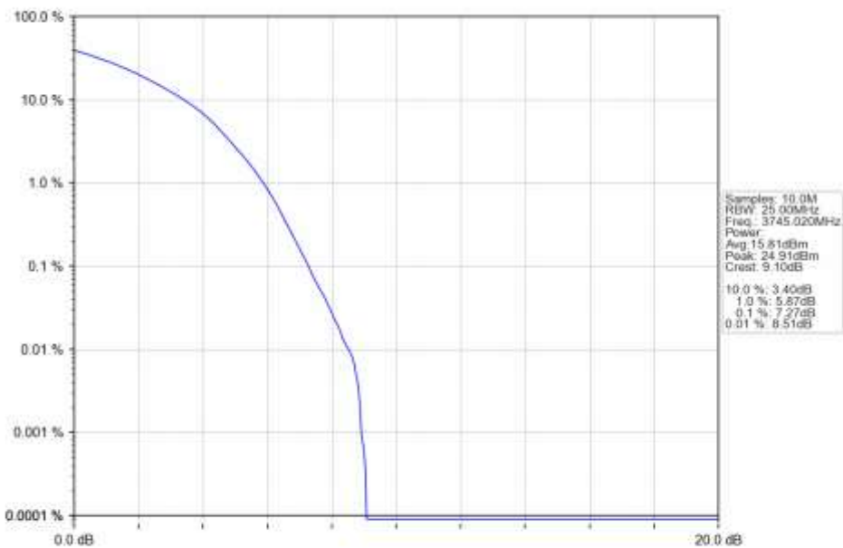
n78a_30kHz_SISO_NTNV_90MHz_DFT-s-OFDM QPSK_3745.02MHz_Outer_Full_Ant1
