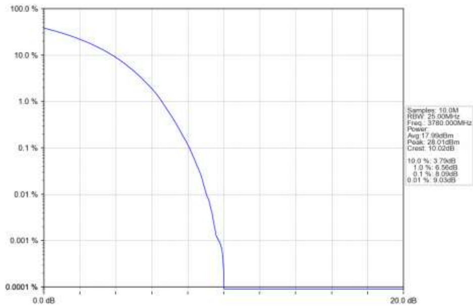
n78a 30kHz SISO NTN 40MHz CP-OFDM 16 QAM 3780MHz Outer Full Ant1
