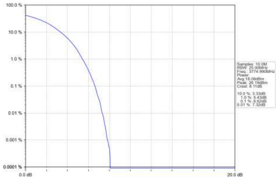
n78a 15kHz SISO NTN 50MHz DFT-s-OFDM QPSK 3774.99MHz Outer Full Ant1
