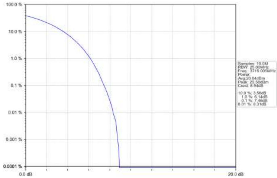
n78a 15kHz SISO NTN 30MHz CP-OFDM 64 QAM 3715.005MHz Outer Full Ant1
