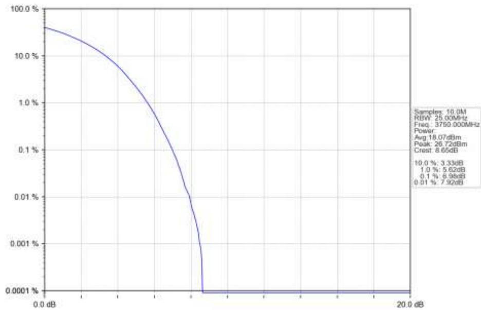
n78a 15kHz SISO NTN 40MHz DFT-s-OFDM 256 QAM 3750MHz Outer Full Ant1
