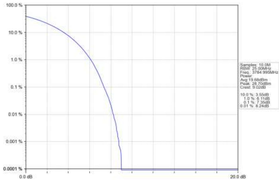
n78a 15kHz SISO NTN 30MHz CP-OFDM QPSK 3784.995MHz Outer Full Ant1
