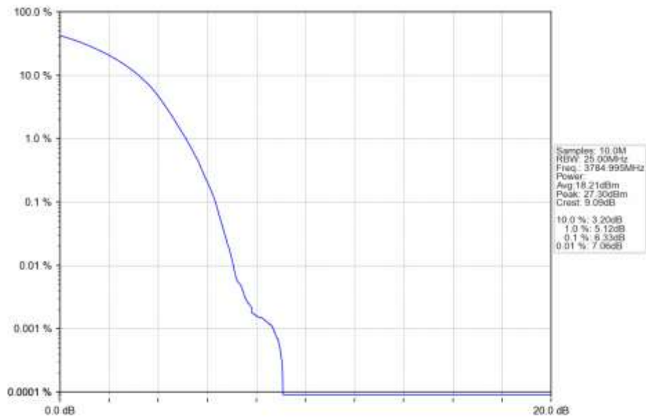
n78a 15kHz SISO NTN 30MHz DFT-s-OFDM 256 QAM 3784.995MHz Outer Full Ant1
