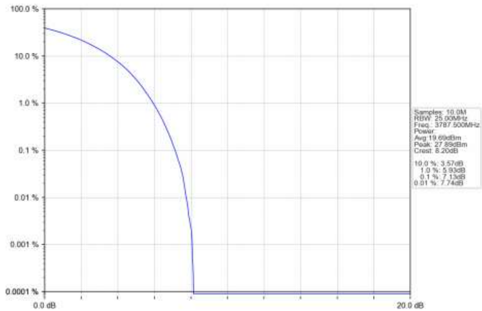
n78a 15kHz SISO NTN 25MHz CP-OFDM 16 QAM 3787.5MHz Outer Full Ant1
