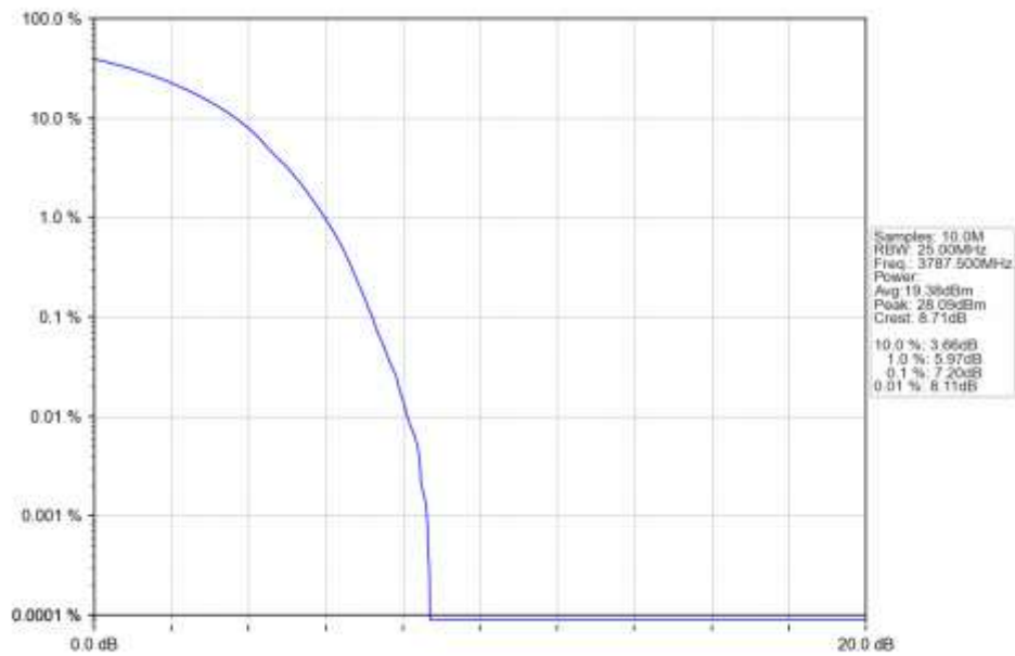
n78a 30kHz SISO NTN 25MHz CP-OFDM 64 QAM 3787.5MHz Outer Full Ant1
