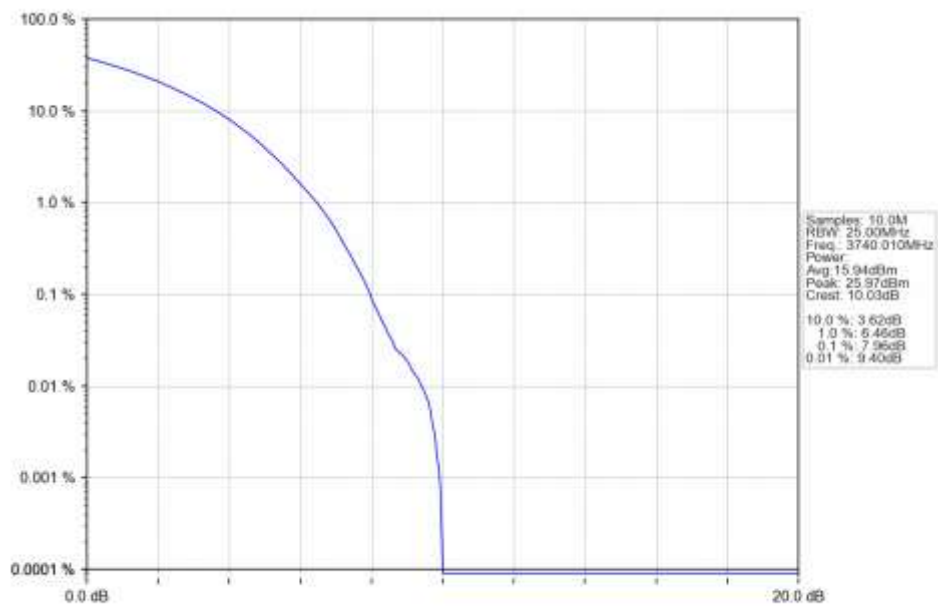
n78a 30kHz SISO NTN 80MHz CP-OFDM 16 QAM 3740.01MHz Outer Full Ant1
