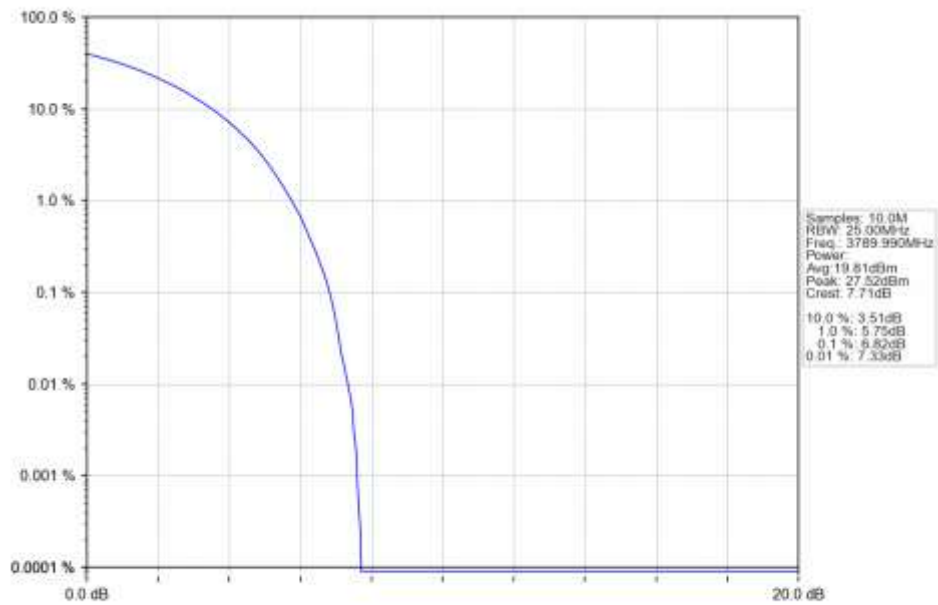
n78a 15kHz SISO NTN 20MHz CP-OFDM QPSK 3789.99MHz Outer Full Ant1
