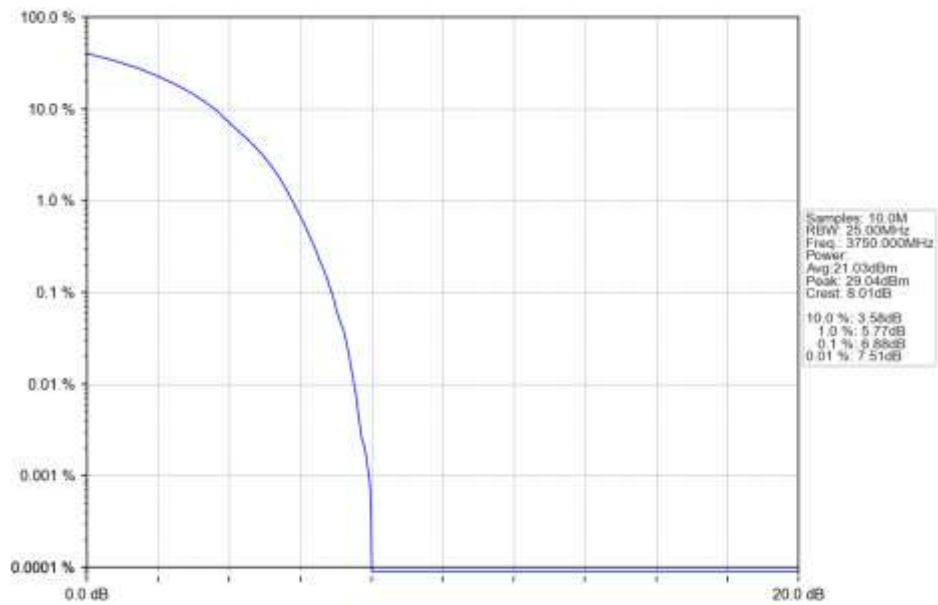
n78a 30kHz SISO NTN 25MHz CP-OFDM QPSK 3750MHz Outer Full Ant1
