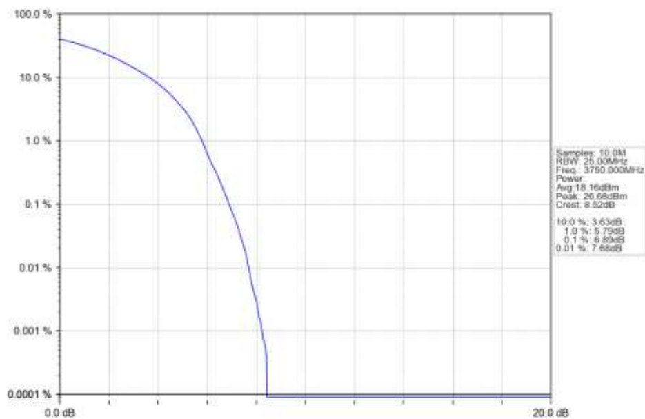
n78a_30kHz_SISO_NTNV_50MHz_DFT-s-OFDM QPSK_3750MHz_Outer_Full_Ant1
