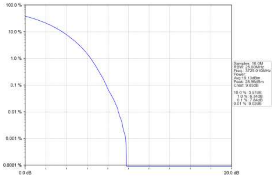
n78a 15kHz SISO NTN 50MHz CP-OFDM QPSK 3725.01MHz Outer Full Ant1
