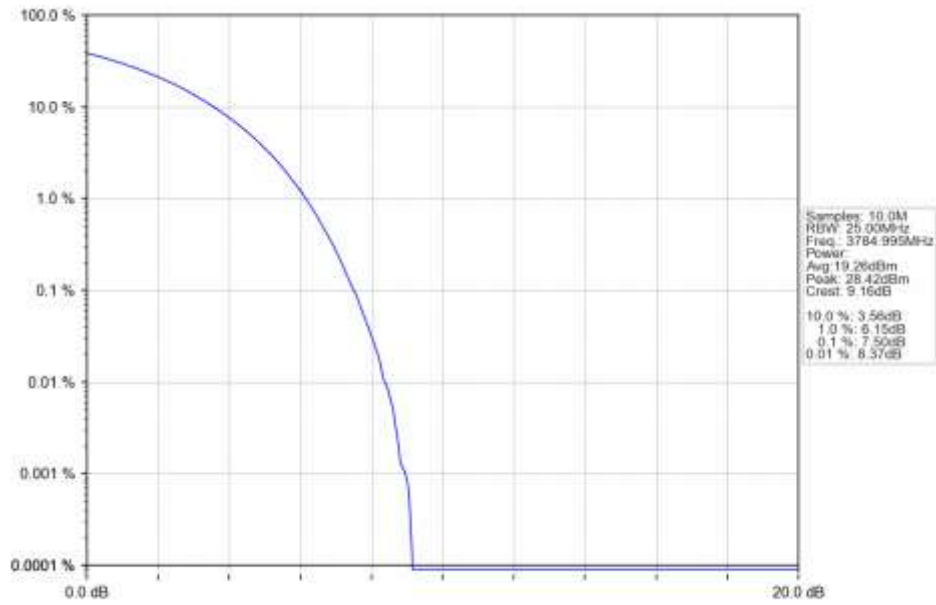
n78a 15kHz SISO NTN 30MHz CP-OFDM 64 QAM 3784.995MHz Outer Full Ant1
