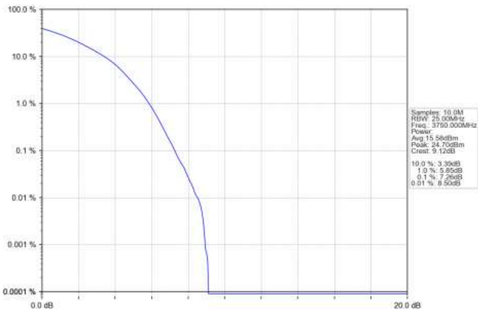
n78a_30kHz_SISO_NTNV_90MHz_DFT-s-OFDM QPSK_3750MHz_Outer_Full_Ant1
