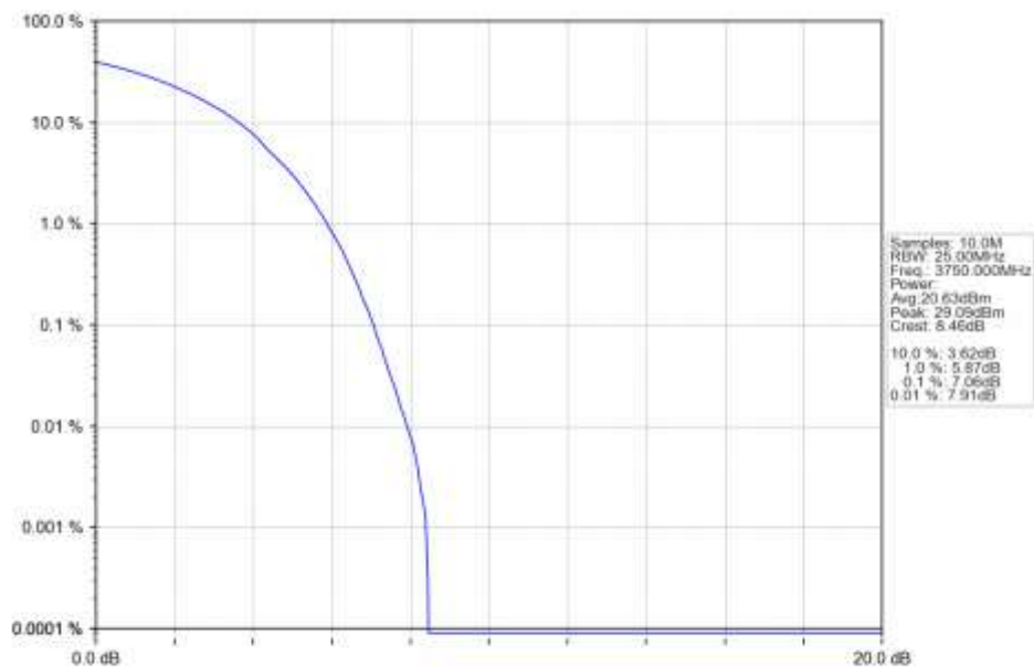
n78a 30kHz SISO NTN 25MHz CP-OFDM 64 QAM 3750MHz Outer Full Ant1
