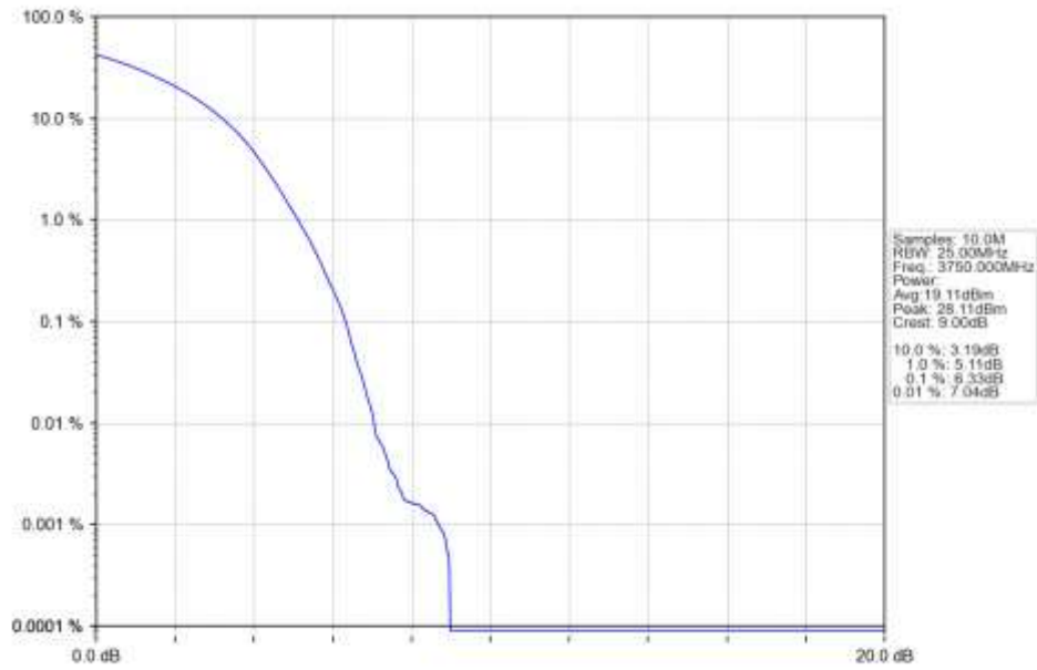
n78a 15kHz SISO NTN 30MHz DFT-s-OFDM 256 QAM 3750MHz Outer Full Ant1
