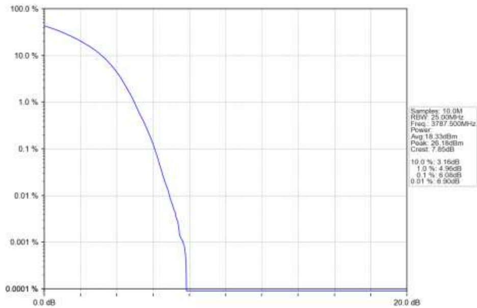
n78a 15kHz SISO NTN 25MHz DFT-s-OFDM 256 QAM 3787.5MHz Outer Full Ant1
