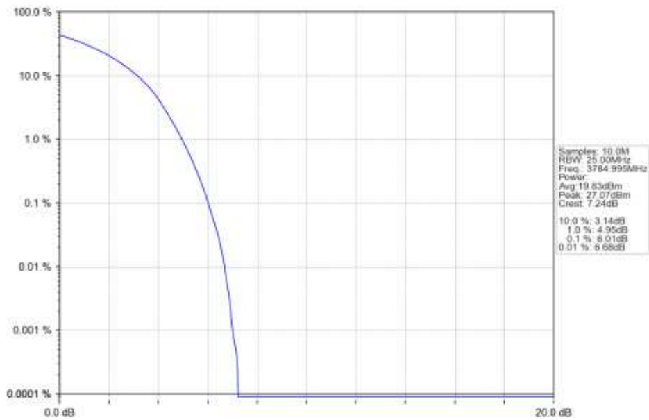
n78a 15kHz SISO NTN 30MHz DFT-s-OFDM 16 QAM 3784.995MHz Outer Full Ant1
