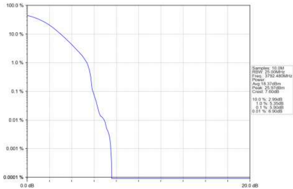
n78a 30kHz SISO NTN 15MHz DFT-s-OFDM 256 QAM 3792.48MHz Outer Full Ant1
