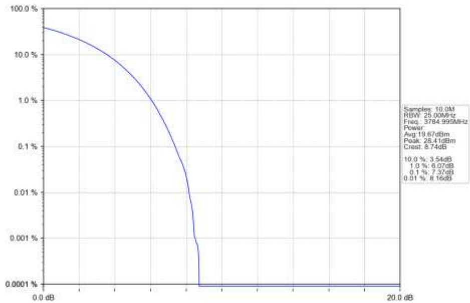
n78a 15kHz SISO NTN 30MHz CP-OFDM 16 QAM 3784.995MHz Outer Full Ant1
