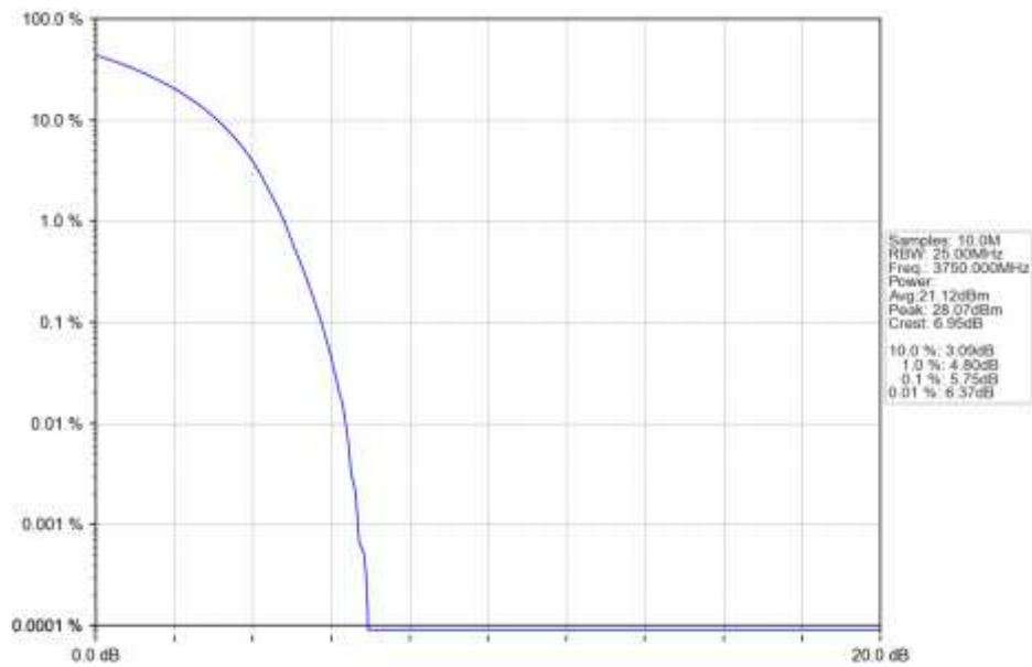
n78a 15kHz SISO NTN 25MHz DFT-s-OFDM 64 QAM 3750MHz Outer Full Ant1
