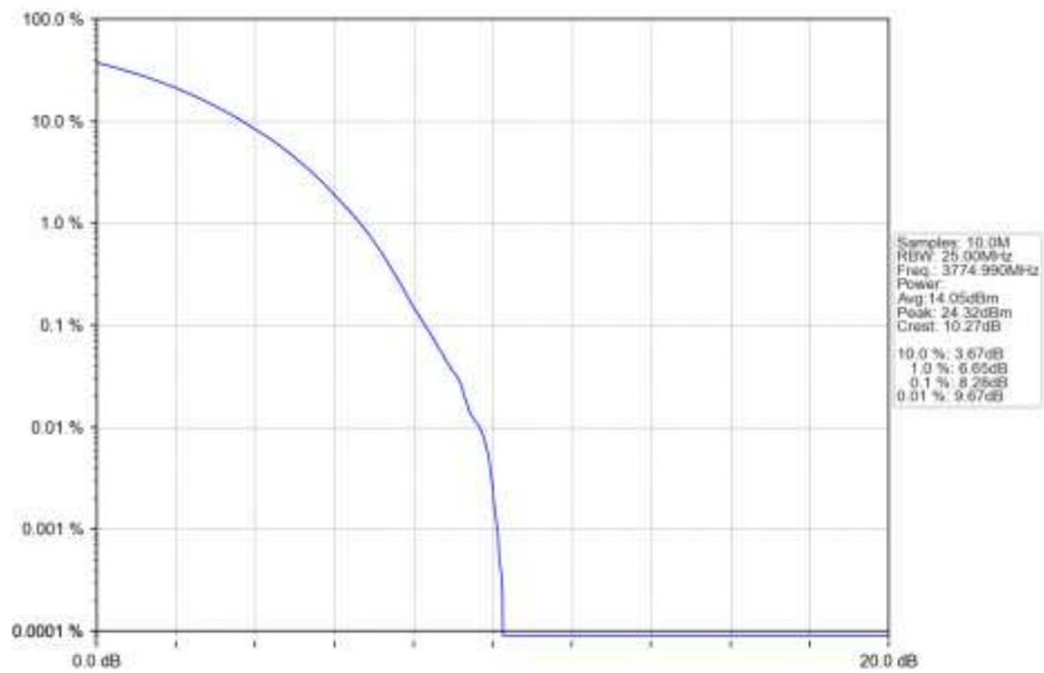
n78a 30kHz SISO NTN 50MHz CP-OFDM 256 QAM 3774.99MHz Outer Full Ant1
