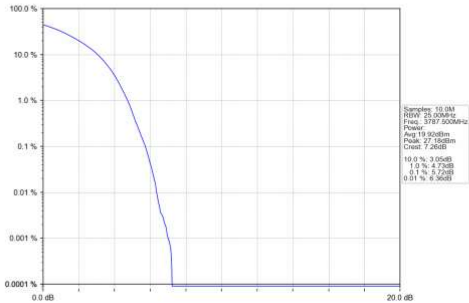
n78a 15kHz SISO NTN 25MHz DFT-s-OFDM 16 QAM 3787.5MHz Outer Full Ant1
