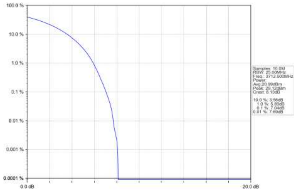
n78a 15kHz SISO NTN 25MHz CP-OFDM 64 QAM 3712.5MHz Outer Full Ant1
