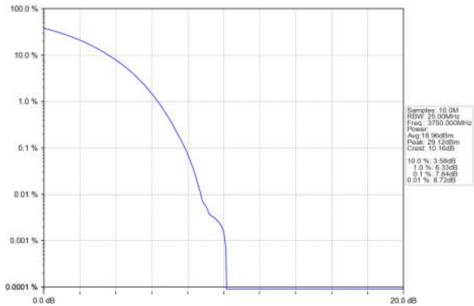
n78a 15kHz SISO NTN 40MHz CP-OFDM 64 QAM 3750MHz Outer Full Ant1
