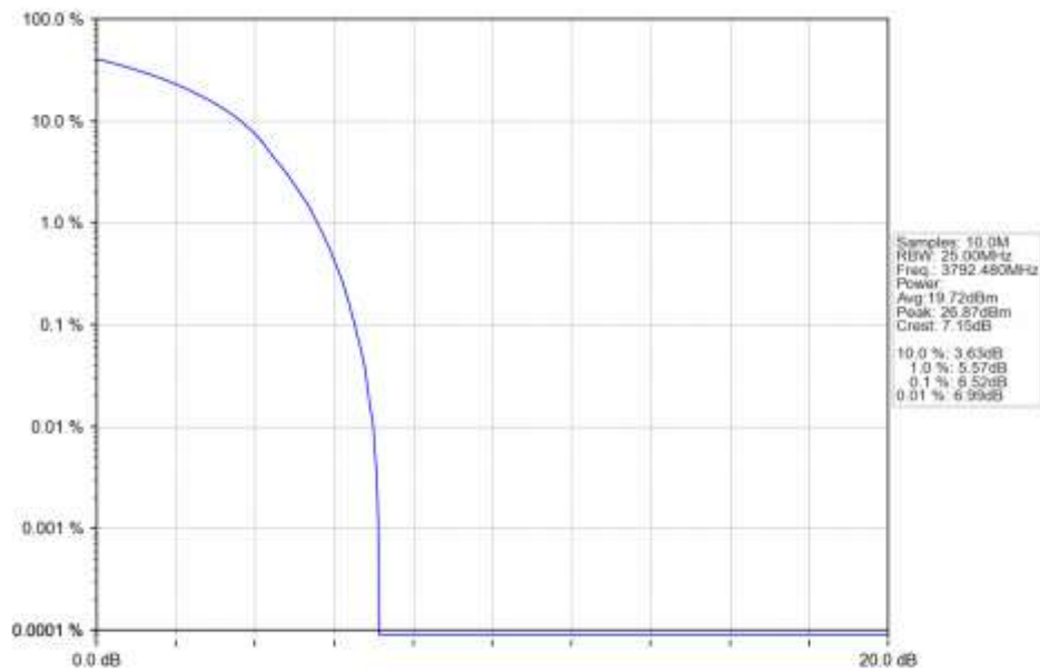
n78a 30kHz SISO NTN 15MHz CP-OFDM QPSK 3792.48MHz Outer Full Ant1
