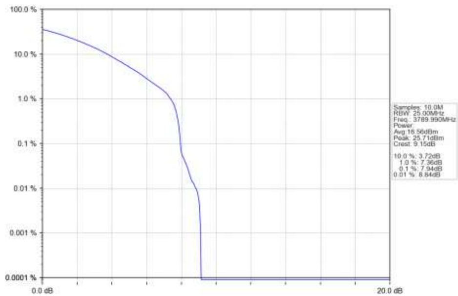
n78a 30kHz SISO NTN 20MHz CP-OFDM 256 QAM 3789.99MHz Outer Full Ant1
