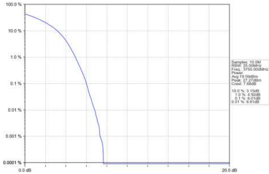
n78a 15kHz SISO NTN 25MHz DFT-s-OFDM 256 QAM 3750MHz Outer Full Ant1
