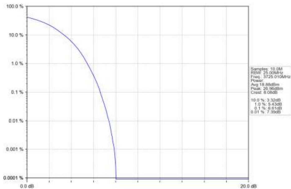
n78a_15kHz_SISO_NTNV_50MHz_DFT-s-OFDM QPSK_3725.01MHz_Outer_Full_Ant1
