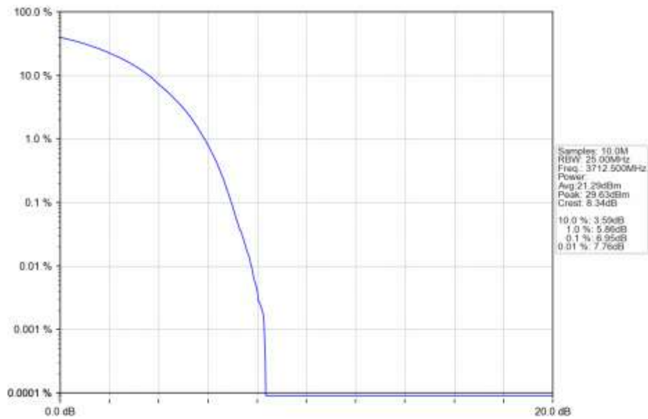
n78a 30kHz SISO NTN 25MHz CP-OFDM 64 QAM 3712.5MHz Outer Full Ant1
