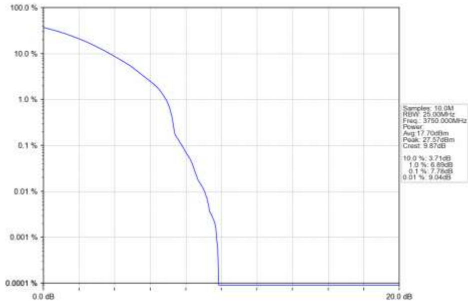
n78a 30kHz SISO NTN 25MHz CP-OFDM 256 QAM 3750MHz Outer Full Ant1
