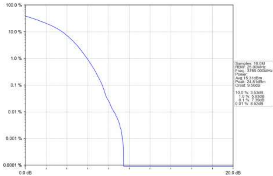
n78a 30kHz SISO NTN 70MHz DFT-s-OFDM 256 QAM 3765MHz Outer Full Ant1
