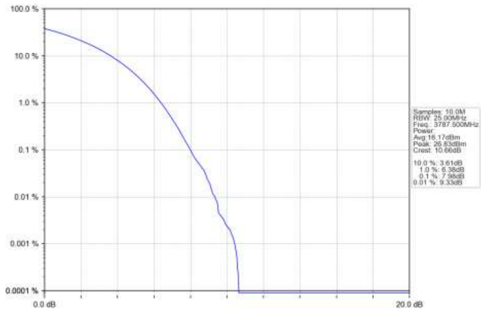
n78a 15kHz SISO NTN 25MHz CP-OFDM 256 QAM 3787.5MHz Outer Full Ant1
