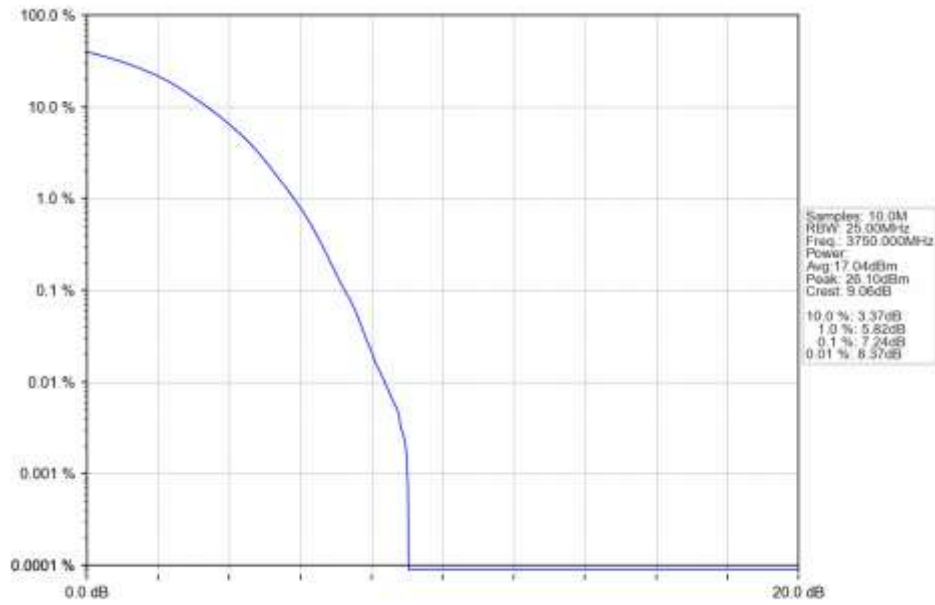
n78a 15kHz SISO NTN 50MHz DFT-s-OFDM 256 QAM 3750MHz Outer Full Ant1
