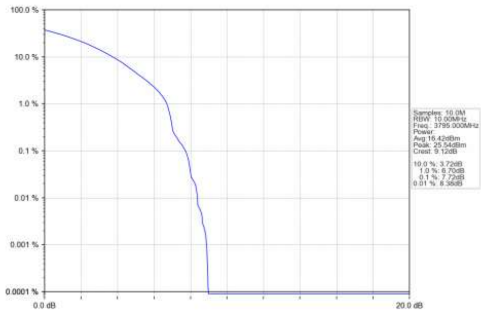
n78a 30kHz SISO NTN 10MHz CP-OFDM 256 QAM 3795MHz Outer Full Ant1
