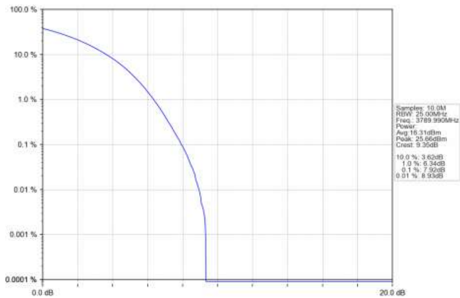
n78a 15kHz SISO NTN 20MHz CP-OFDM 256 QAM 3789.99MHz Outer Full Ant1
