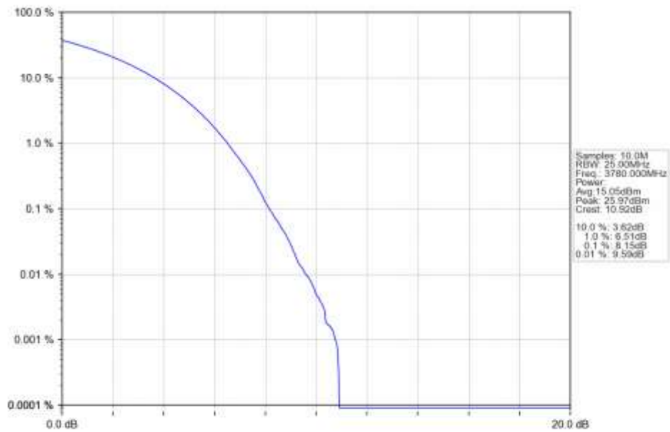
n78a 15kHz SISO NTN 40MHz CP-OFDM 256 QAM 3780MHz Outer Full Ant1
