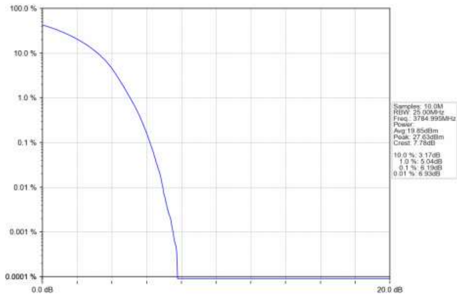
n78a 15kHz SISO NTN 30MHz DFT-s-OFDM 64 QAM 3784.995MHz Outer Full Ant1
