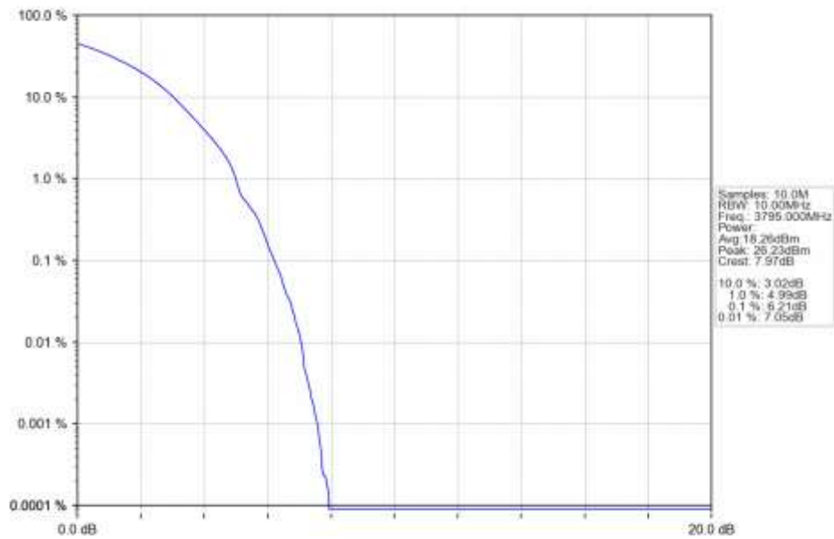
n78a 30kHz SISO NTN 10MHz DFT-s-OFDM 256 QAM 3795MHz Outer Full Ant1
