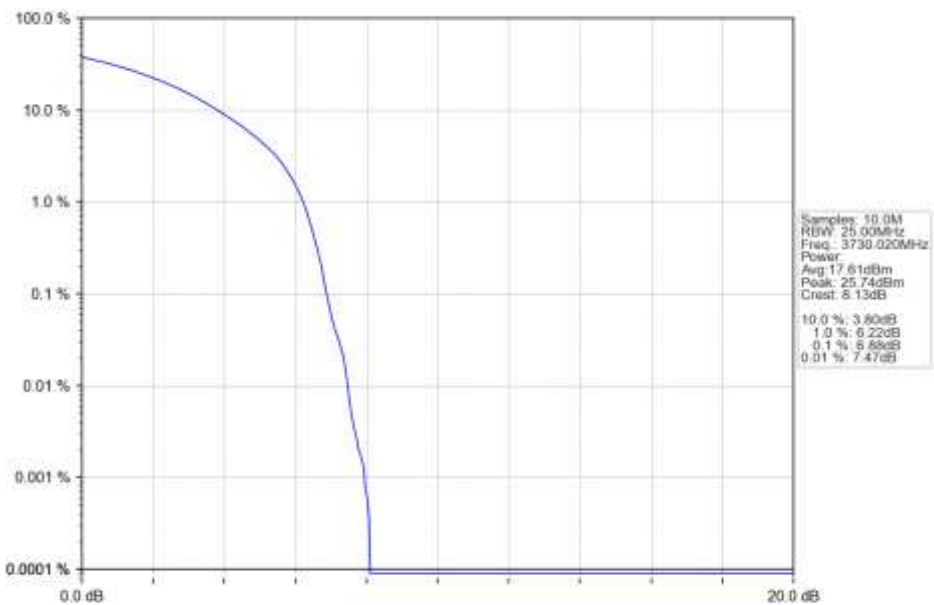
n78a_30kHz_SISO_NTNV_60MHz_DFT-s-OFDM QPSK_3730.02MHz_Outer_Full_Ant1
