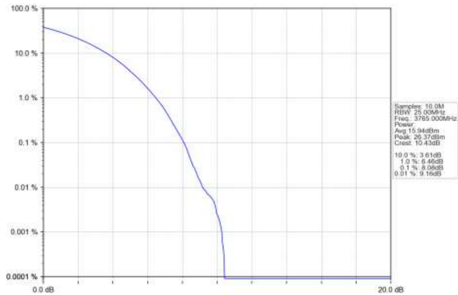
n78a 30kHz SISO NTN 70MHz CP-OFDM 64 QAM 3765MHz Outer Full Ant1
