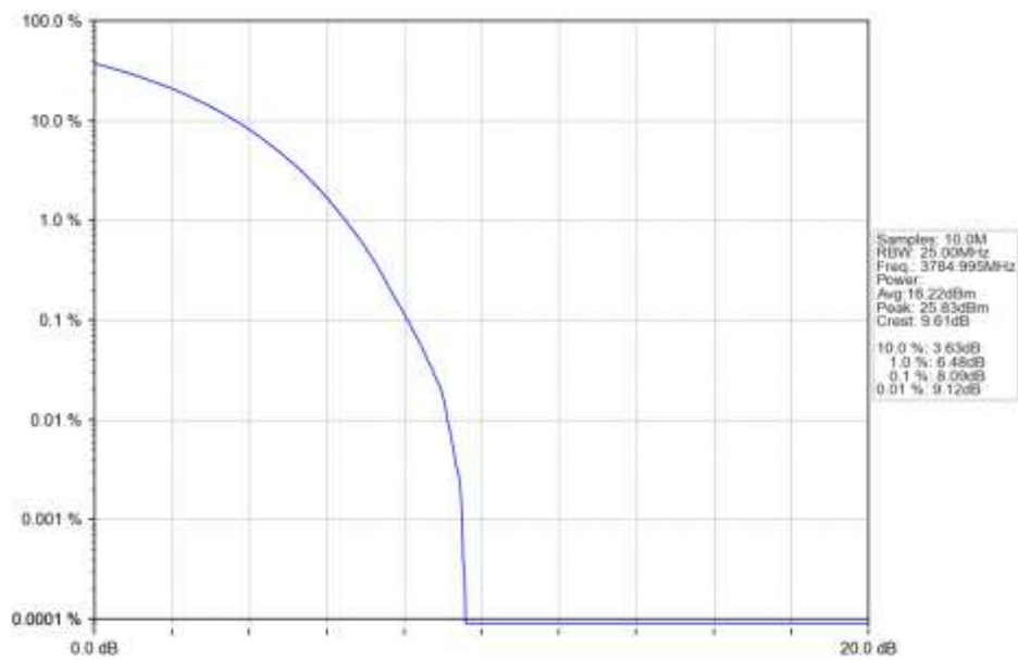
n78a 15kHz SISO NTN 30MHz CP-OFDM 256 QAM 3784.995MHz Outer Full Ant1
