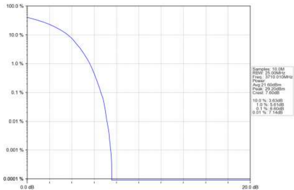
n78a 30kHz SISO NTN 20MHz CP-OFDM 16 QAM 3710.01MHz Outer Full Ant1
