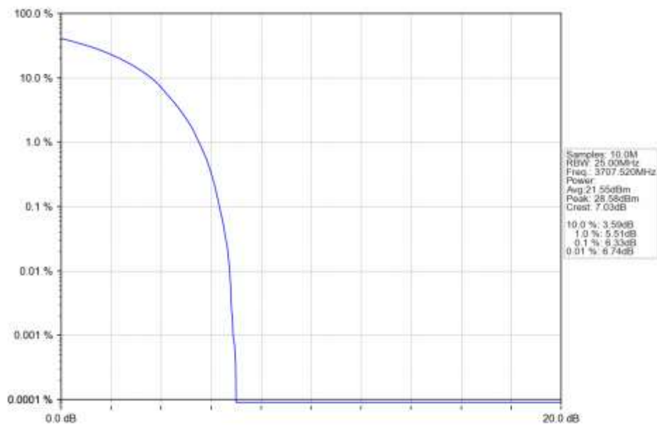
n78a 30kHz SISO NTN 15MHz CP-OFDM 16 QAM 3707.52MHz Outer Full Ant1
