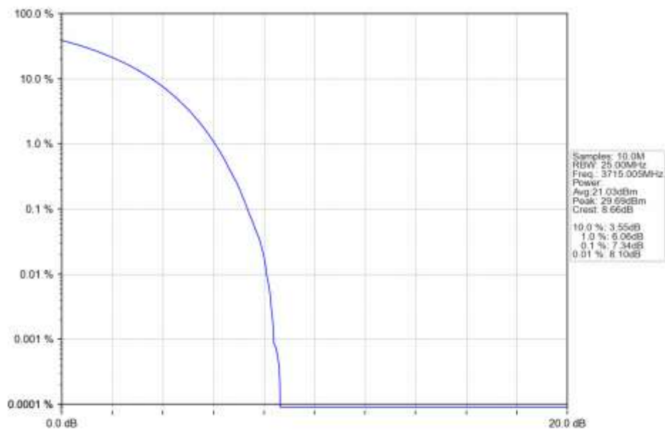
n78a 15kHz SISO NTN 30MHz CP-OFDM 16 QAM 3715.005MHz Outer Full Ant1
