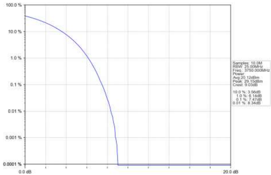
n78a 15kHz SISO NTN 30MHz CP-OFDM 64 QAM 3750MHz Outer Full Ant1
