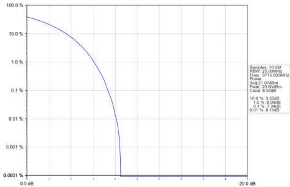
n78a 15kHz SISO NTN 30MHz CP-OFDM QPSK 3715.005MHz Outer Full Ant1
