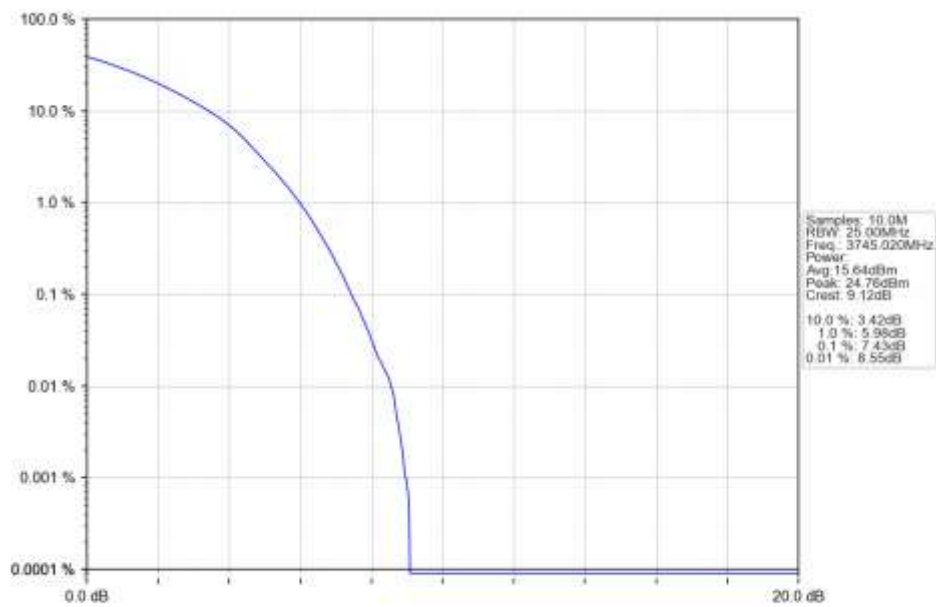
n78a 30kHz SISO NTN 90MHz DFT-s-OFDM 16 QAM 3745.02MHz Outer Full Ant1
