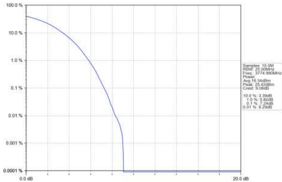
n78a 15kHz SISO NTN 50MHz DFT-s-OFDM 256 QAM 3774.99MHz Outer Full Ant1
