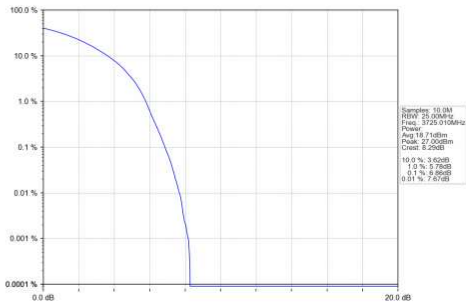
n78a_30kHz_SISO_NTNV_50MHz_DFT-s-OFDM QPSK_3725.01MHz_Outer_Full_Ant1
