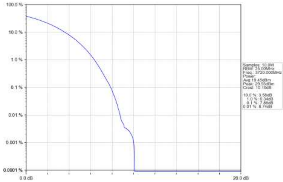
n78a 15kHz SISO NTN 40MHz CP-OFDM 64 QAM 3720MHz Outer Full Ant1
