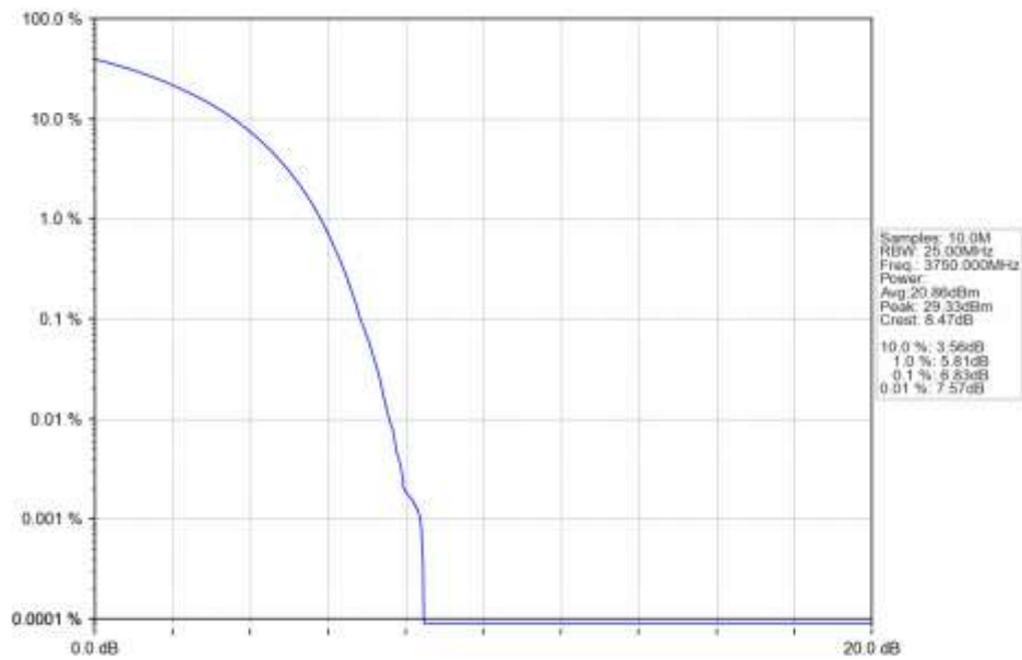
n78a 15kHz SISO NTN 25MHz CP-OFDM QPSK 3750MHz Outer Full Ant1
