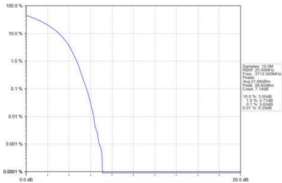
n78a 15kHz SISO NTN 25MHz DFT-s-OFDM 16 QAM 3712.5MHz Outer Full Ant1
