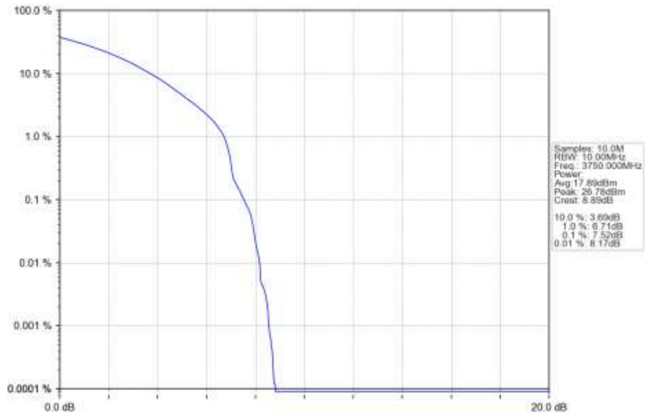
n78a 30kHz SISO NTN 10MHz CP-OFDM 256 QAM 3750MHz Outer Full Ant1
