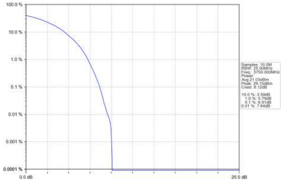
n78a 30kHz SISO NTN 25MHz CP-OFDM 16 QAM 3750MHz Outer Full Ant1
