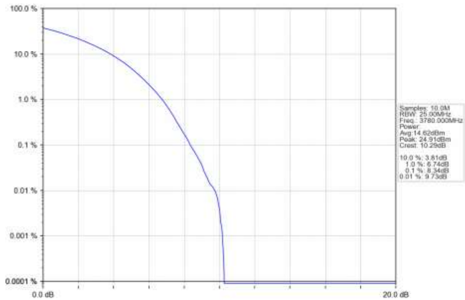
n78a 30kHz SISO NTN 40MHz CP-OFDM 256 QAM 3780MHz Outer Full Ant1
