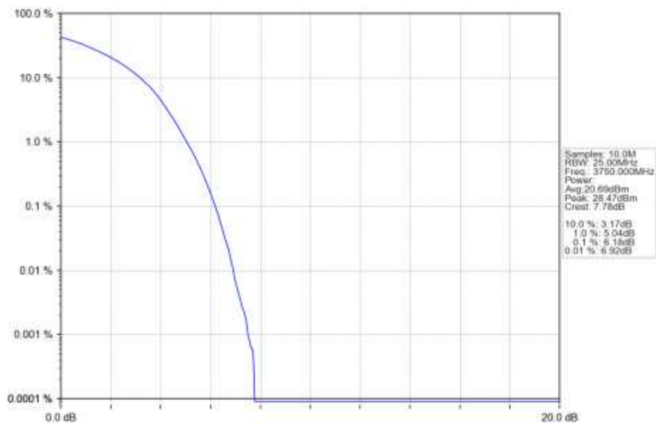
n78a 15kHz SISO NTN 30MHz DFT-s-OFDM 64 QAM 3750MHz Outer Full Ant1
