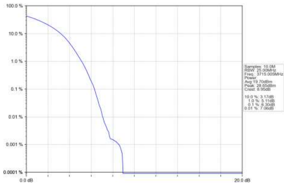
n78a 15kHz SISO NTN 30MHz DFT-s-OFDM 256 QAM 3715.005MHz Outer Full Ant1
