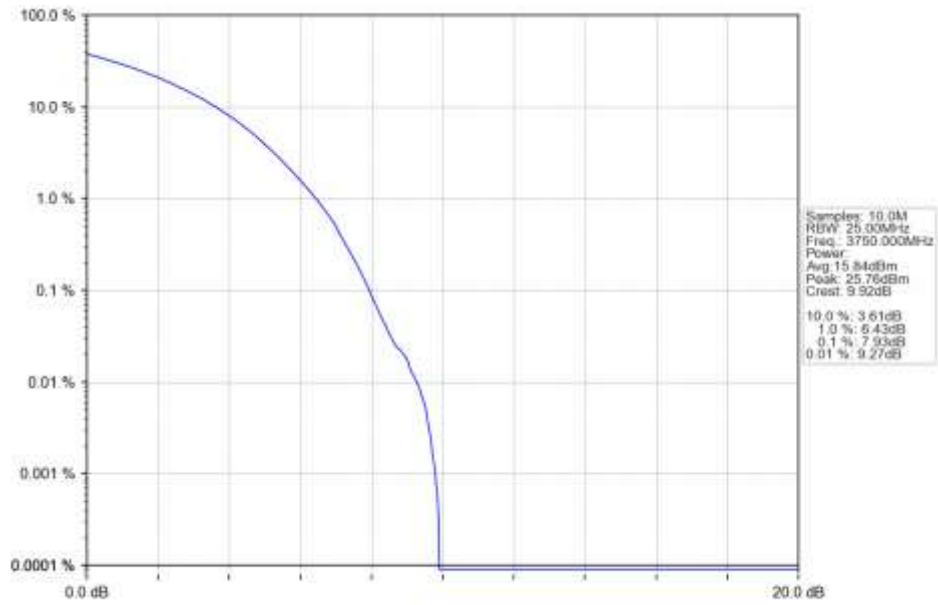
n78a 30kHz SISO NTN 80MHz CP-OFDM 16 QAM 3750MHz Outer Full Ant1
