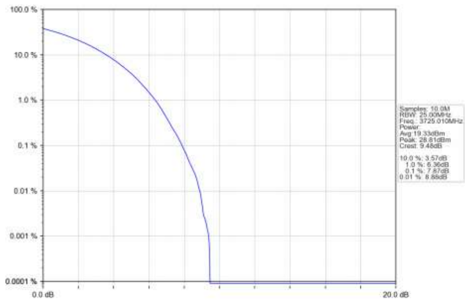
n78a 15kHz SISO NTN 50MHz CP-OFDM 16 QAM 3725.01MHz Outer Full Ant1
