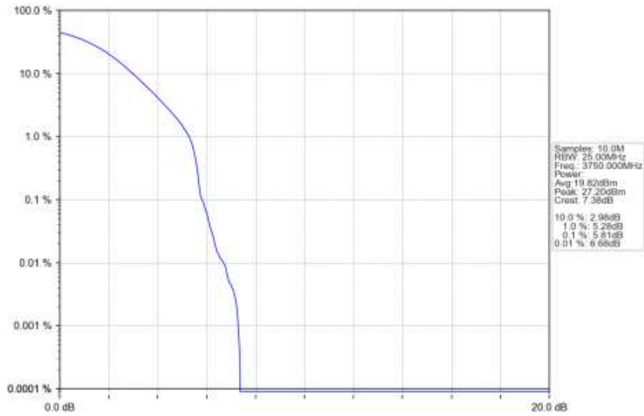
n78a 30kHz SISO NTN 15MHz DFT-s-OFDM 256 QAM 3750MHz Outer Full Ant1
