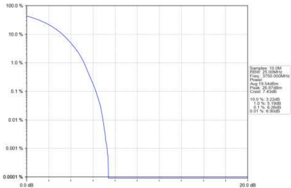
n78a_30kHz_SISO_NTNV_40MHz_DFT-s-OFDM QPSK_3750MHz_Outer_Full_Ant1
