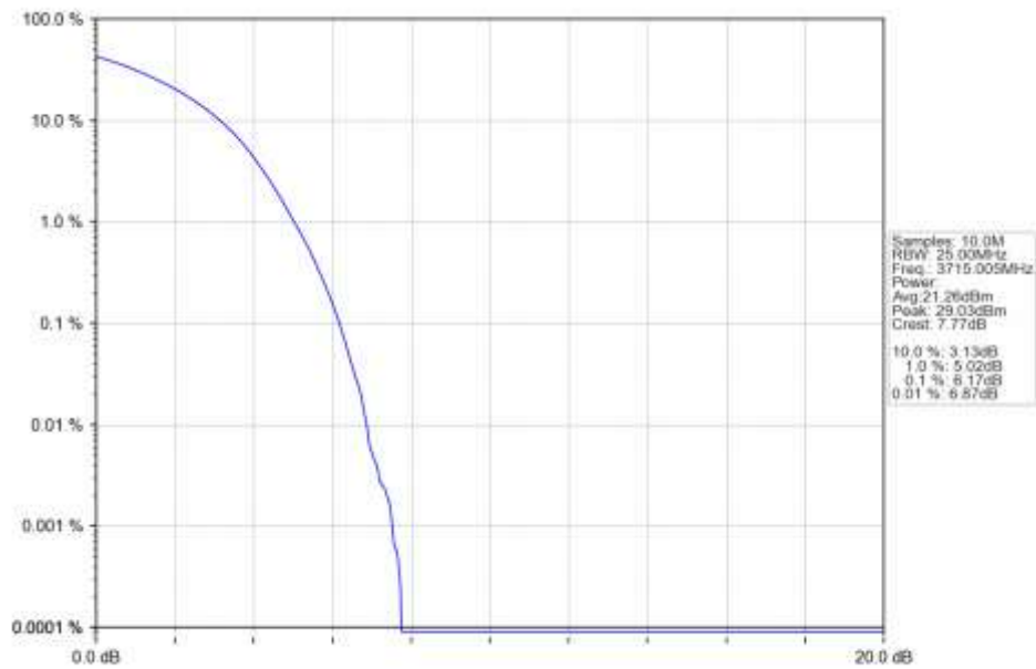
n78a 15kHz SISO NTN 30MHz DFT-s-OFDM 64 QAM 3715.005MHz Outer Full Ant1
