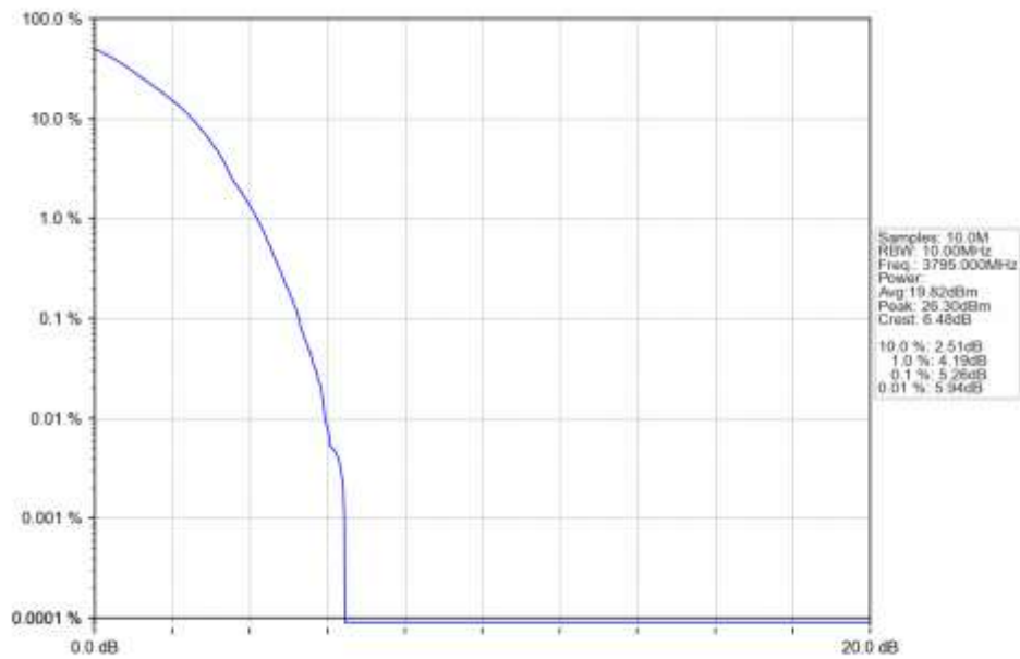
n78a 30kHz SISO NTN 10MHz DFT-s-OFDM QPSK 3795MHz Outer Full Ant1
