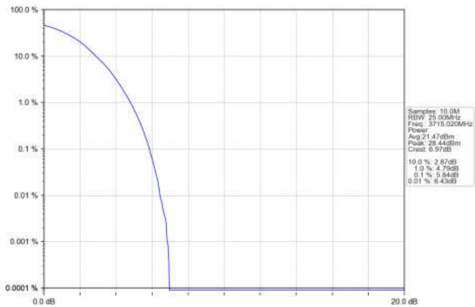
n78a 30kHz SISO NTN 30MHz DFT-s-OFDM 16 QAM 3715.02MHz Outer Full Ant1
