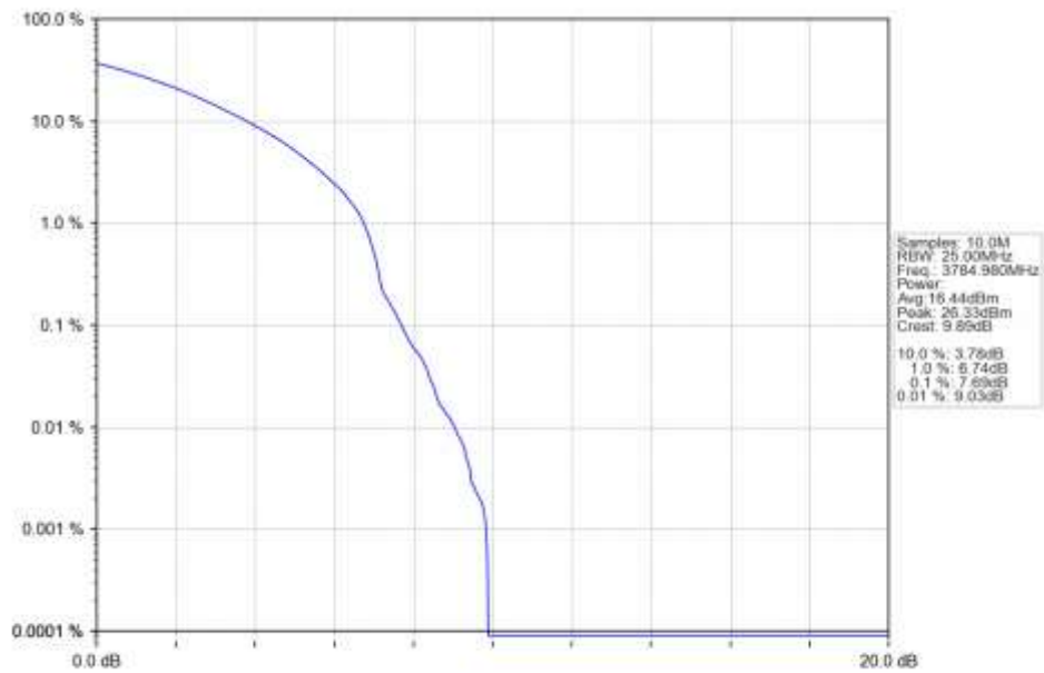
n78a 30kHz SISO NTN 30MHz CP-OFDM 256 QAM 3784.98MHz Outer Full Ant1
