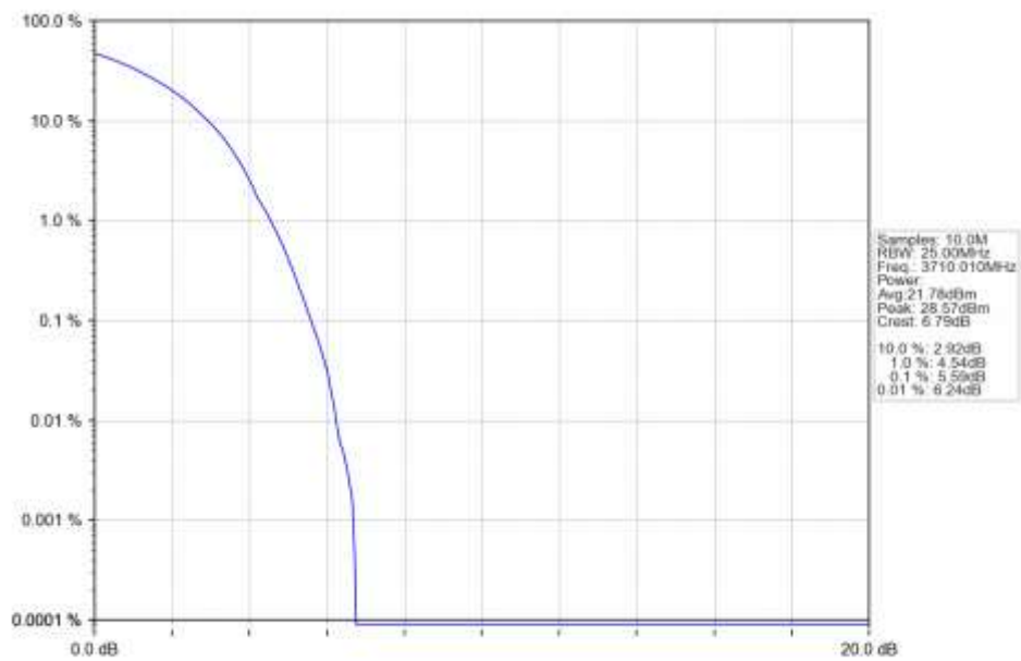
n78a 30kHz SISO NTN 20MHz DFT-s-OFDM 16 QAM 3710.01MHz Outer Full Ant1
