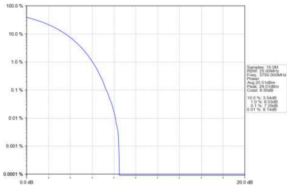
n78a 15kHz SISO NTN 30MHz CP-OFDM QPSK 3750MHz Outer Full Ant1
