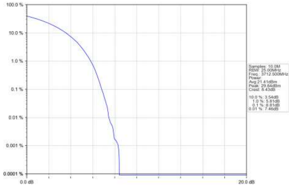
n78a 15kHz SISO NTN 25MHz CP-OFDM QPSK 3712.5MHz Outer Full Ant1
