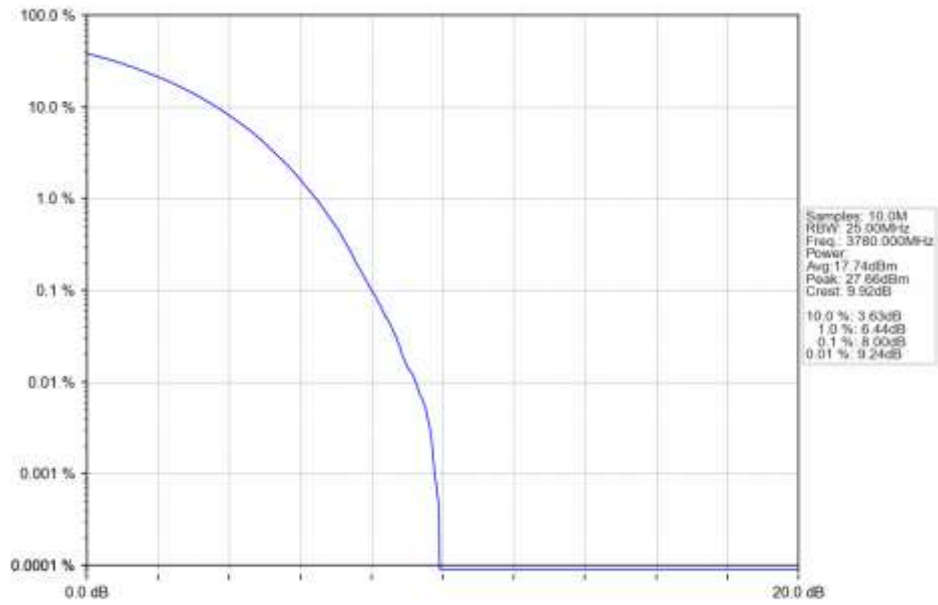
n78a 30kHz SISO NTN 40MHz CP-OFDM 64 QAM 3780MHz Outer Full Ant1
