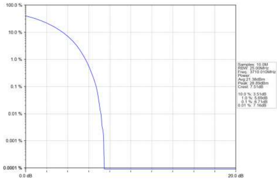
n78a 15kHz SISO NTN 20MHz CP-OFDM QPSK 3710.01MHz Outer Full Ant1
