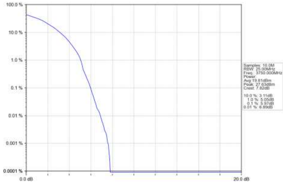
n78a 30kHz SISO NTN 25MHz DFT-s-OFDM 256 QAM 3750MHz Outer Full Ant1
