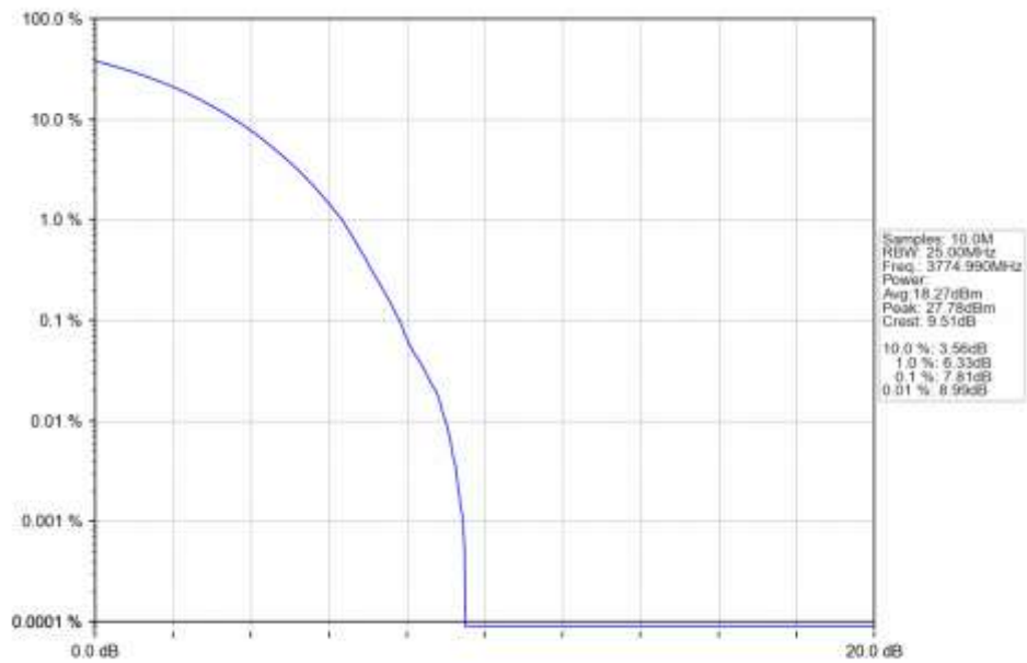
n78a 15kHz SISO NTN 50MHz CP-OFDM QPSK 3774.99MHz Outer Full Ant1
