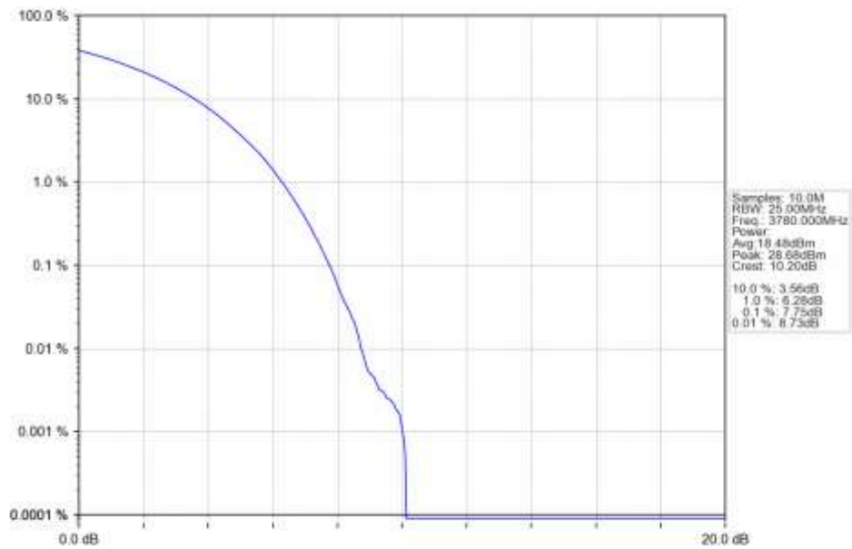
n78a 15kHz SISO NTN 40MHz CP-OFDM 16 QAM 3780MHz Outer Full Ant1
