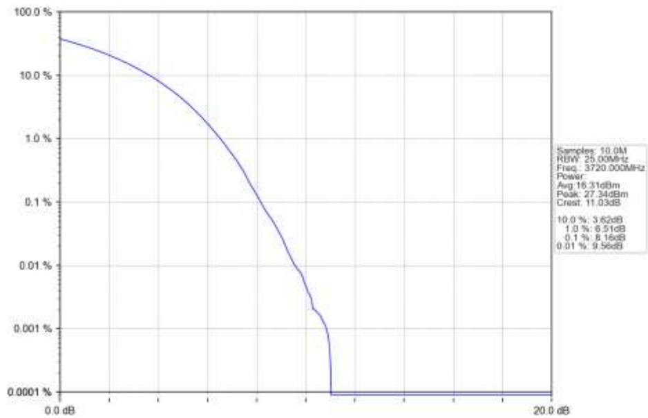
n78a 15kHz SISO NTN 40MHz CP-OFDM 256 QAM 3720MHz Outer Full Ant1
