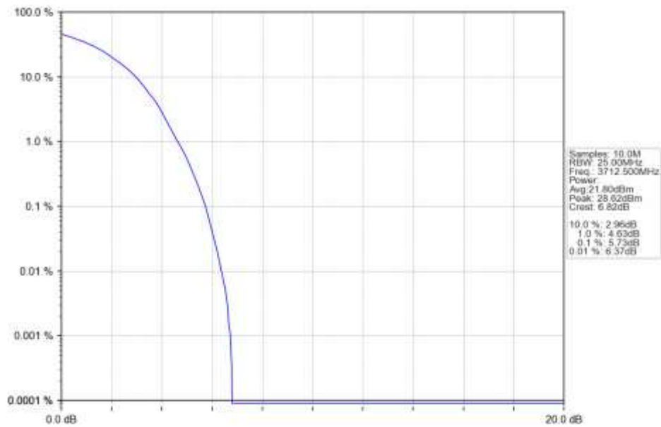
n78a 30kHz SISO NTN 25MHz DFT-s-OFDM 16 QAM 3712.5MHz Outer Full Ant1
