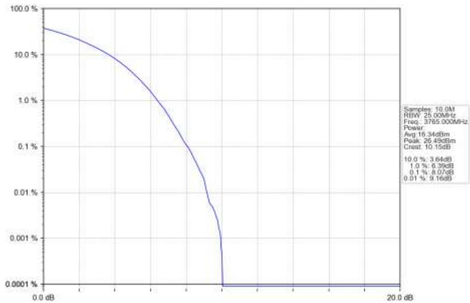
n78a 30kHz SISO NTN 70MHz CP-OFDM 16 QAM 3765MHz Outer Full Ant1
