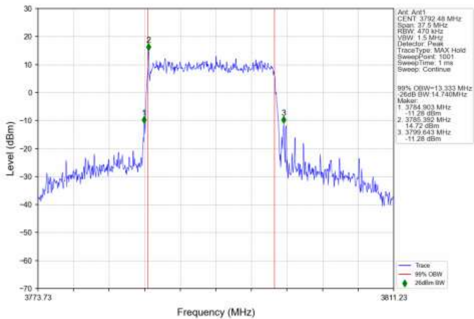
n78a 30kHz SISO NTN 15MHz DFT-s-OFDM 256 QAM 3792.48MHz Outer Full Ant1
