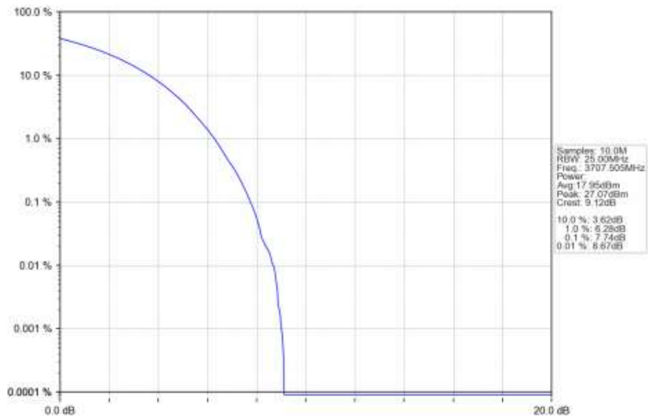
n78a 15kHz SISO NTN 15MHz CP-OFDM 256 QAM 3707.505MHz Outer Full Ant1
