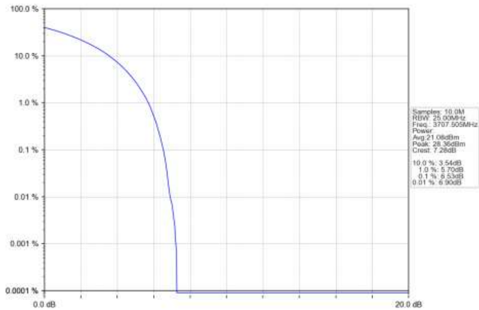
n78a 15kHz SISO NTN 15MHz CP-OFDM 64 QAM 3707.505MHz Outer Full Ant1
