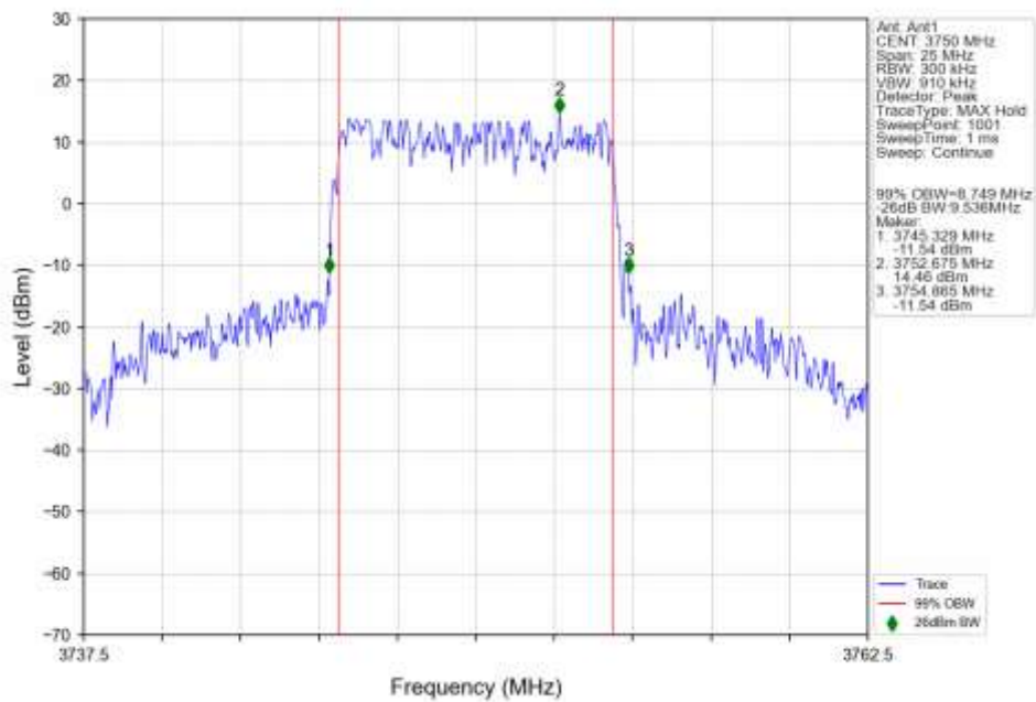
n78a 30kHz SISO NTN 10MHz DFT-s-OFDM 64 QAM 3750MHz Outer Full Ant1
