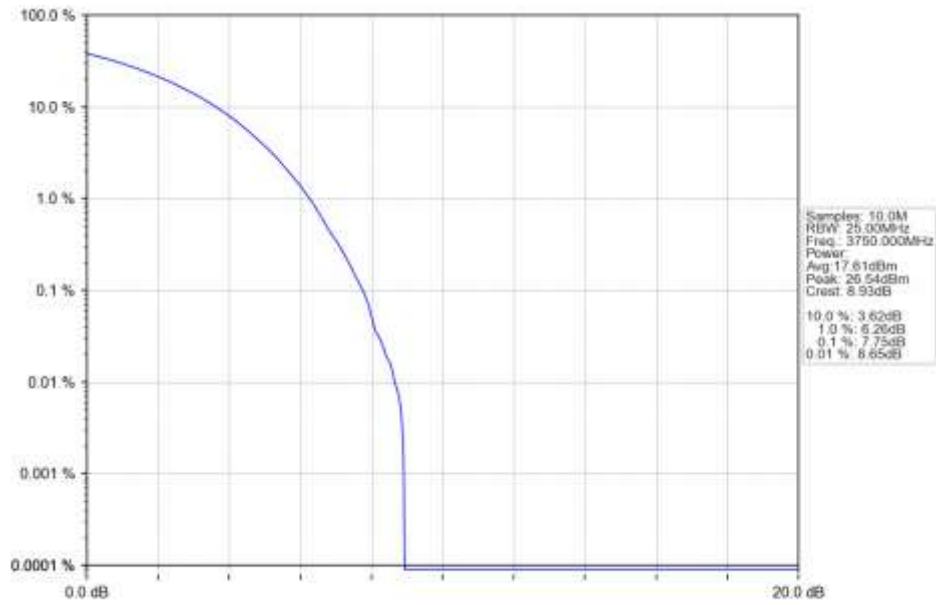
n78a 15kHz SISO NTN 15MHz CP-OFDM 256 QAM 3750MHz Outer Full Ant1
