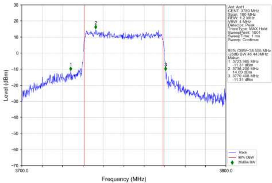
n78a 30kHz SISO NTN 40MHz CP-OFDM 64 QAM 3750MHz Outer Full Ant1
