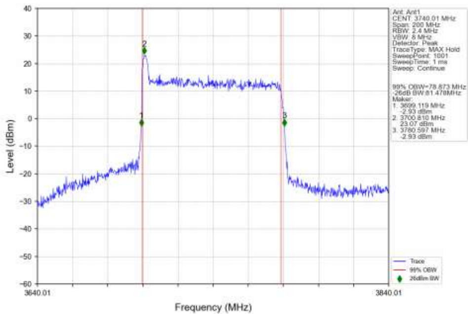
n78a 30kHz SISO NTN 80MHz DFT-s-OFDM 16 QAM 3740.01MHz Outer Full Ant1
