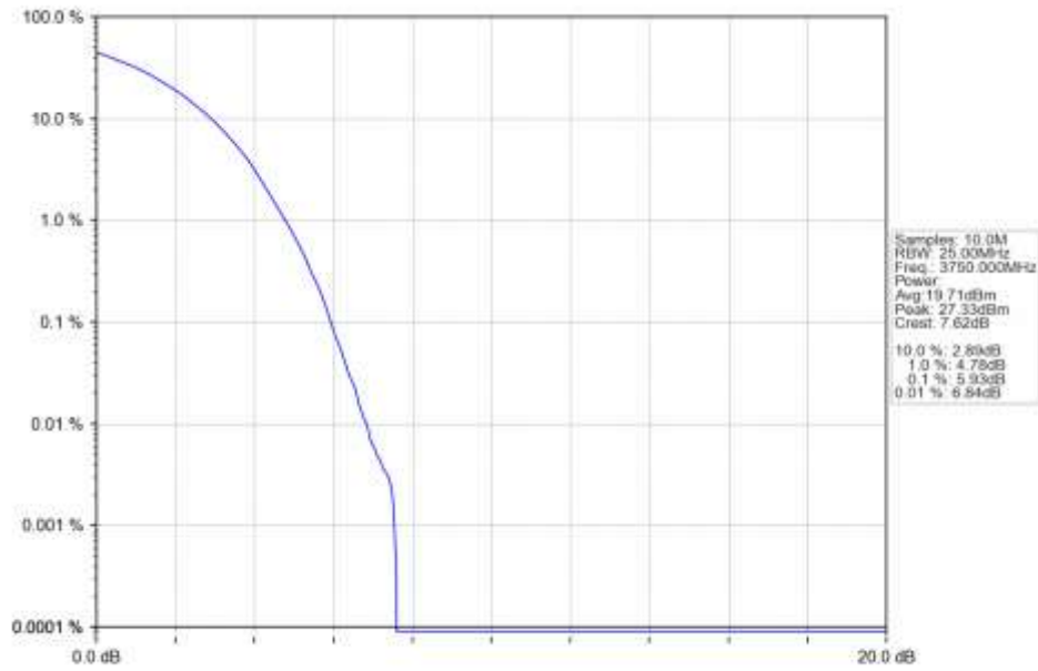
n78a 15kHz SISO NTN 20MHz DFT-s-OFDM 256 QAM 3750MHz Outer Full Ant1
