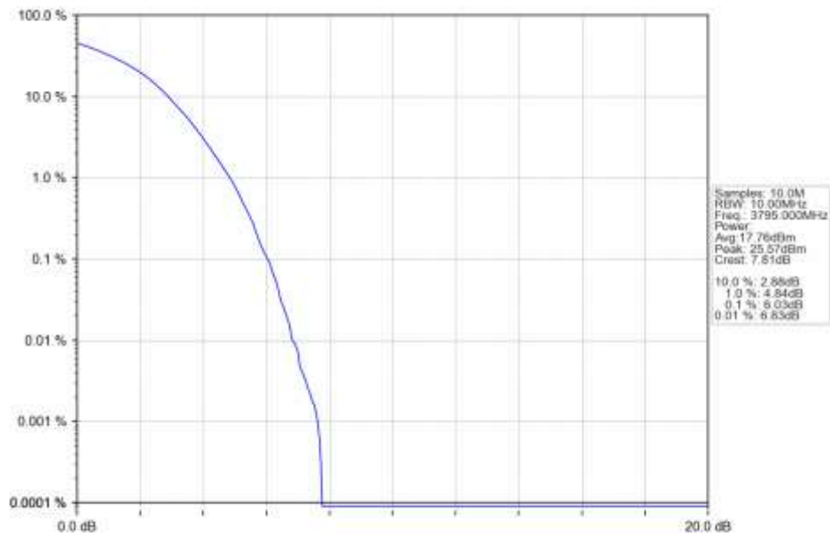
n78a 15kHz SISO NTN 10MHz DFT-s-OFDM 256 QAM 3795MHz Outer Full Ant1
