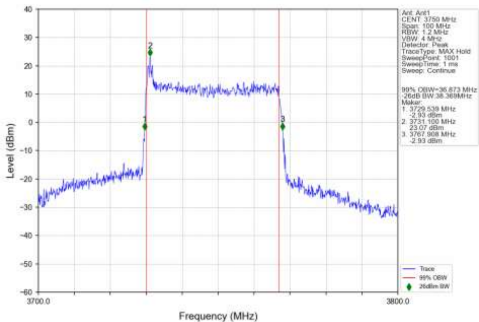
n78a_30kHz_SISO_NTNV_40MHz_DFT-s-OFDM QPSK_3750MHz_Outer_Full_Ant1
