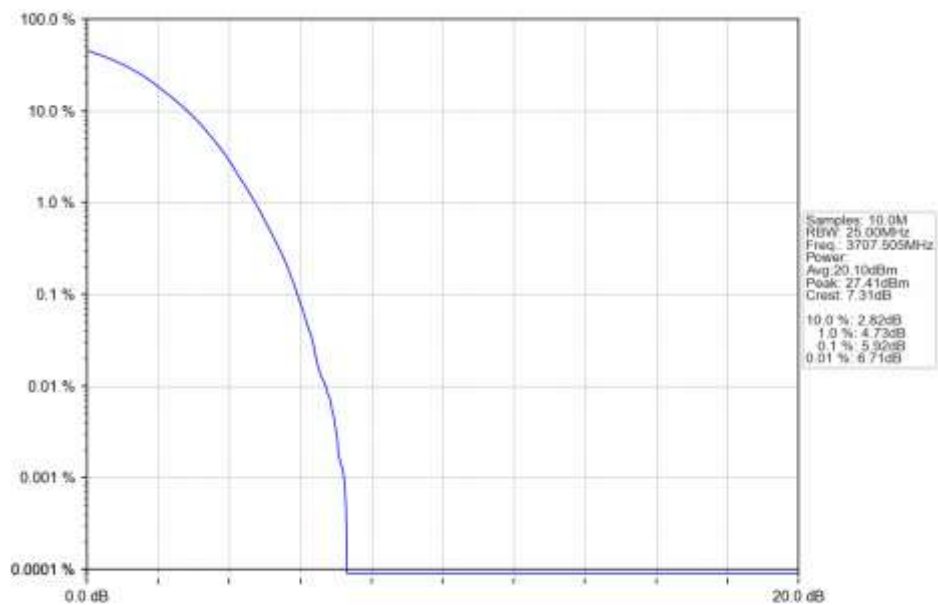
n78a 15kHz SISO NTN 15MHz DFT-s-OFDM 256 QAM 3707.505MHz Outer Full Ant1
