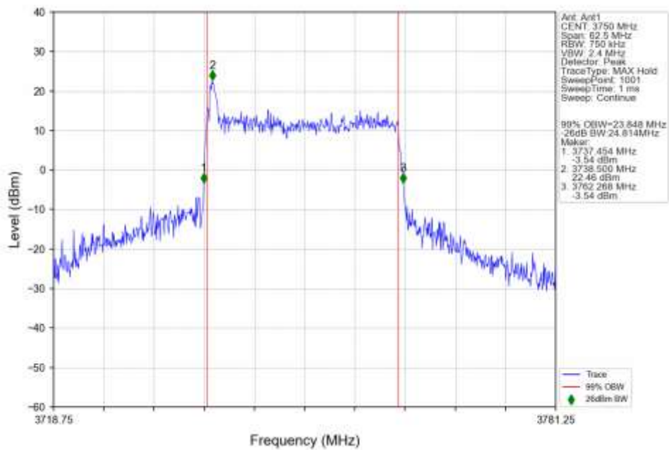
n78a 30kHz SISO NTN 25MHz CP-OFDM QPSK 3750MHz Outer Full Ant1
