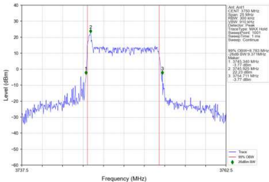
n78a_30kHz_SISO_NTNV_10MHz_DFT-s-OFDM_QPSK_3750MHz_Outer_Full_Ant1
