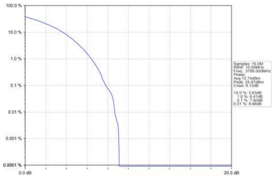
n78a 15kHz SISO NTN 10MHz CP-OFDM 256 QAM 3795MHz Outer Full Ant1
