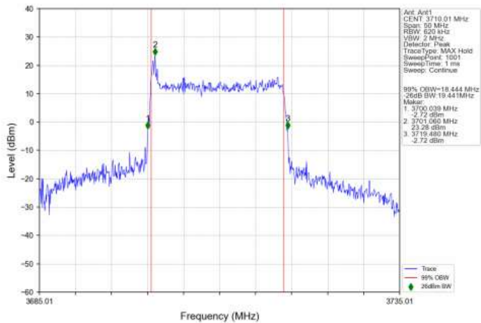
n78a 30kHz SISO NTN 20MHz DFT-s-OFDM 16 QAM 3710.01MHz Outer Full Ant1
