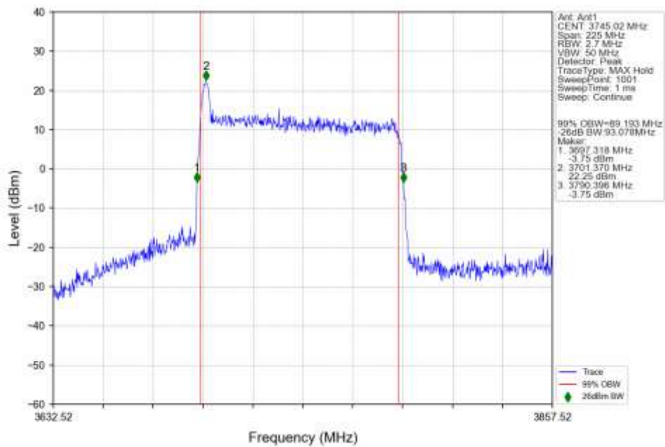
n78a 30kHz SISO NTN 90MHz DFT-s-OFDM 16 QAM 3745.02MHz Outer Full Ant1
