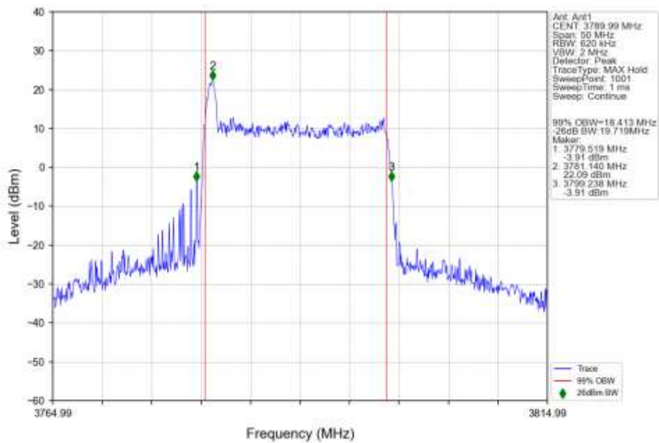
n78a 30kHz SISO NTN 20MHz DFT-s-OFDM 256 QAM 3789.99MHz Outer Full Ant1
