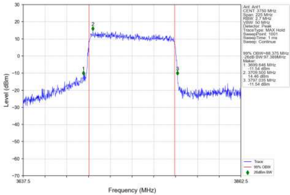
n78a 30kHz SISO NTN 90MHz CP-OFDM 16 QAM 3754.98MHz Outer Full Ant1
