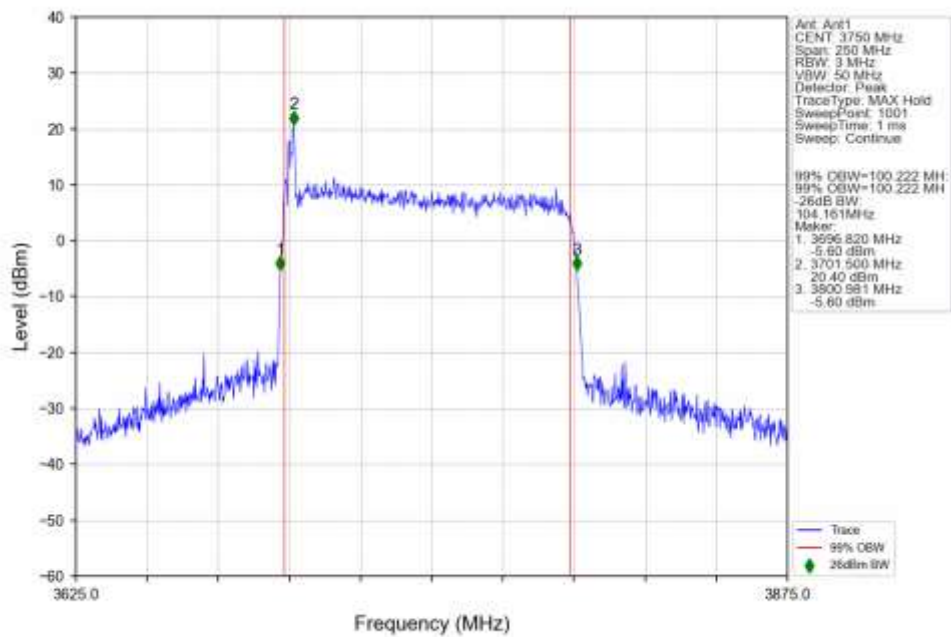
n78a 30kHz SISO NTN 100MHz CP-OFDM 256 QAM 3750MHz Outer Full Ant1
