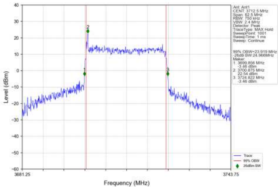
n78a 30kHz SISO NTN 25MHz CP-OFDM 16 QAM 3712.5MHz Outer Full Ant1
