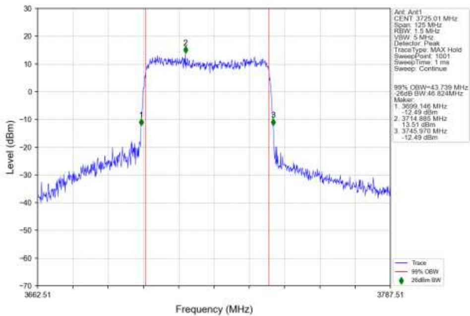
n78a 15kHz SISO NTN 50MHz CP-OFDM 256 QAM 3725.01MHz Outer Full Ant1
