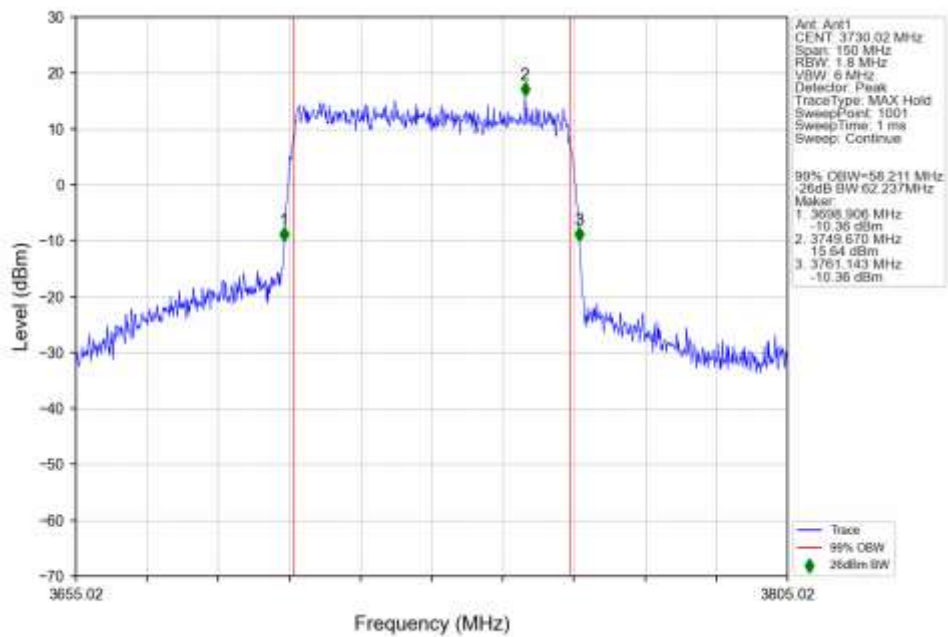
n78a 30kHz SISO NTN 60MHz DFT-s-OFDM 16 QAM 3730.02MHz Outer Full Ant1
