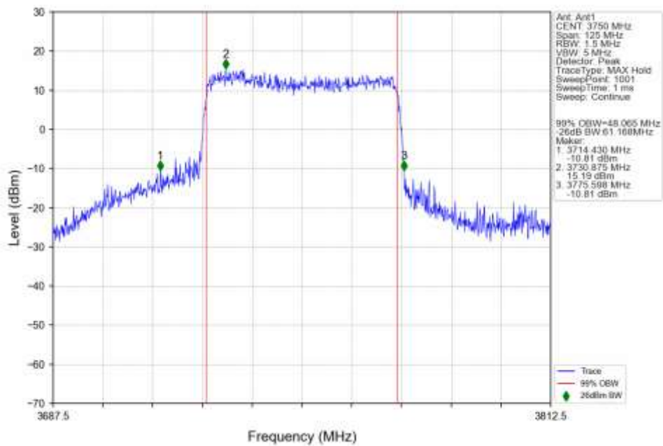
n78a 30kHz SISO NTN 50MHz CP-OFDM QPSK 3750MHz Outer Full Ant1
