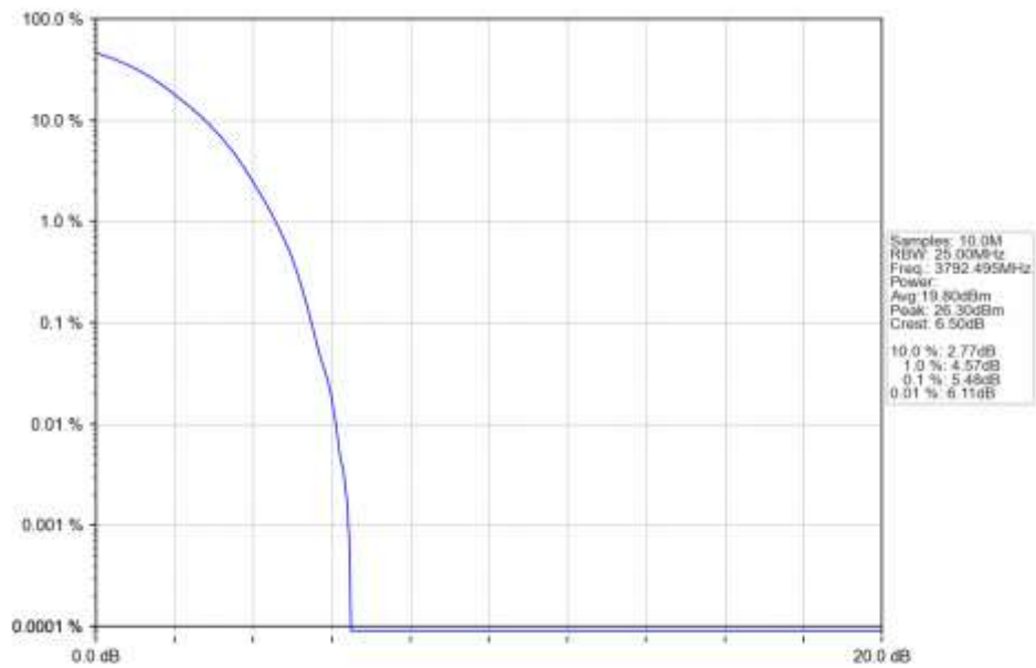
n78a 15kHz SISO NTN 15MHz DFT-s-OFDM 64 QAM 3792.495MHz Outer Full Ant1
