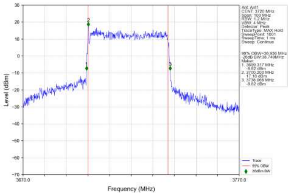
n78a 30kHz SISO NTN 40MHz DFT-s-OFDM 16 QAM 3720MHz Outer Full Ant1
