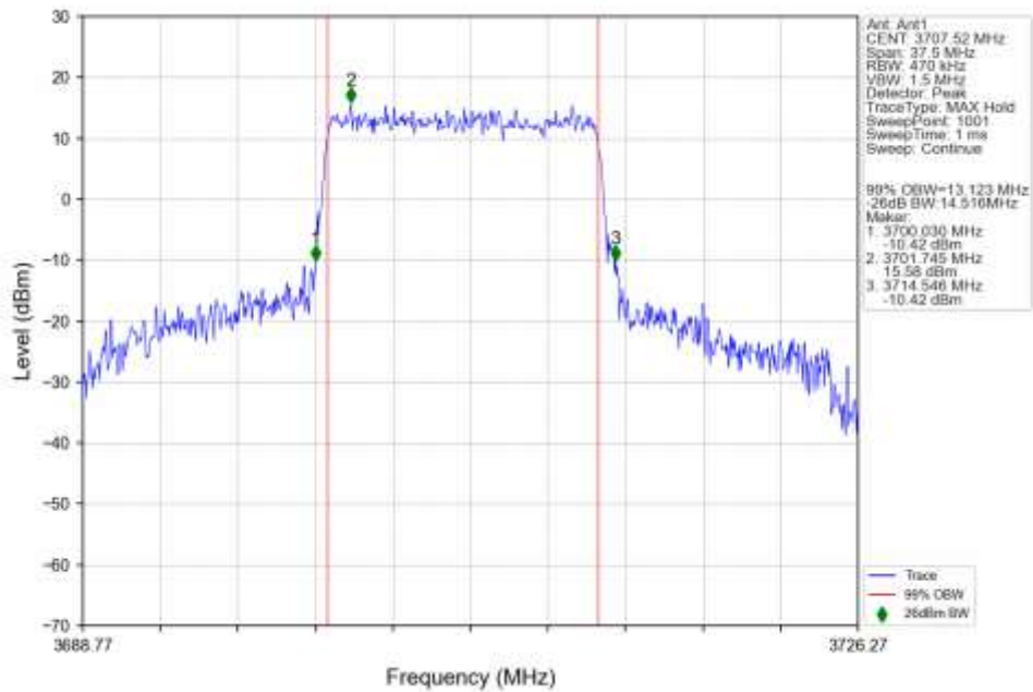
n78a 30kHz SISO NTN 15MHz DFT-s-OFDM 16 QAM 3707.52MHz Outer Full Ant1
