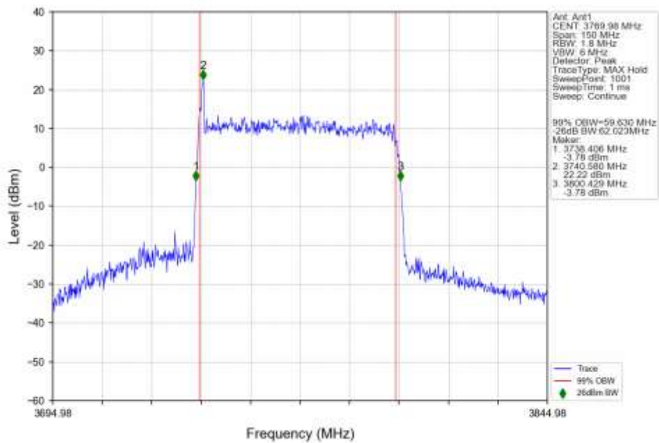
n78a 30kHz SISO NTN 60MHz DFT-s-OFDM 256 QAM 3769.98MHz Outer Full Ant1
