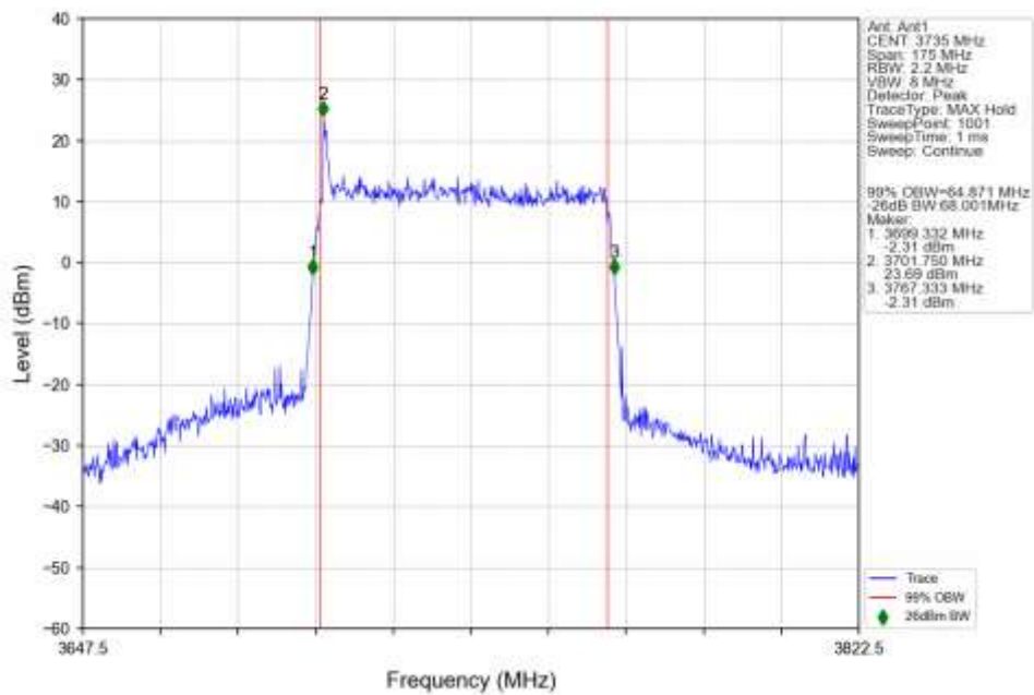
n78a 30kHz SISO NTN 70MHz DFT-s-OFDM 256 QAM 3735MHz Outer Full Ant1
