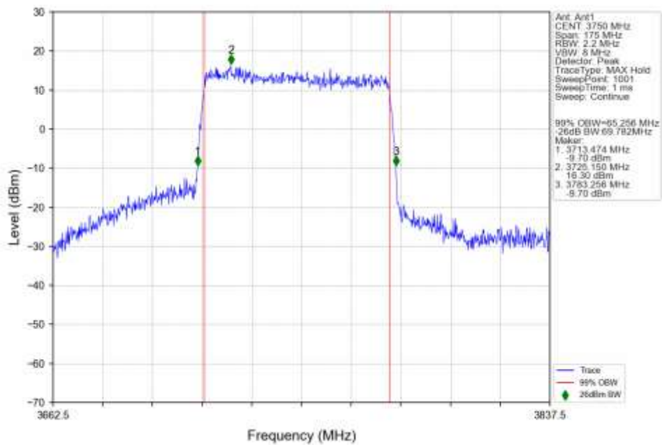
n78a 30kHz SISO NTN 70MHz DFT-s-OFDM 64 QAM 3750MHz Outer Full Ant1
