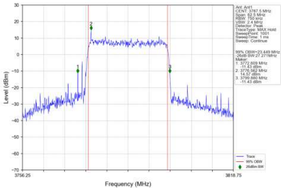
n78a 30kHz SISO NTN 25MHz CP-OFDM 256 QAM 3787.5MHz Outer Full Ant1
