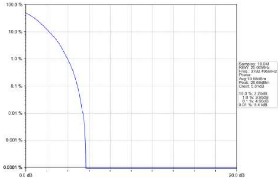
n78a 15kHz SISO NTN 15MHz DFT-s-OFDM QPSK 3792.495MHz Outer Full Ant1
