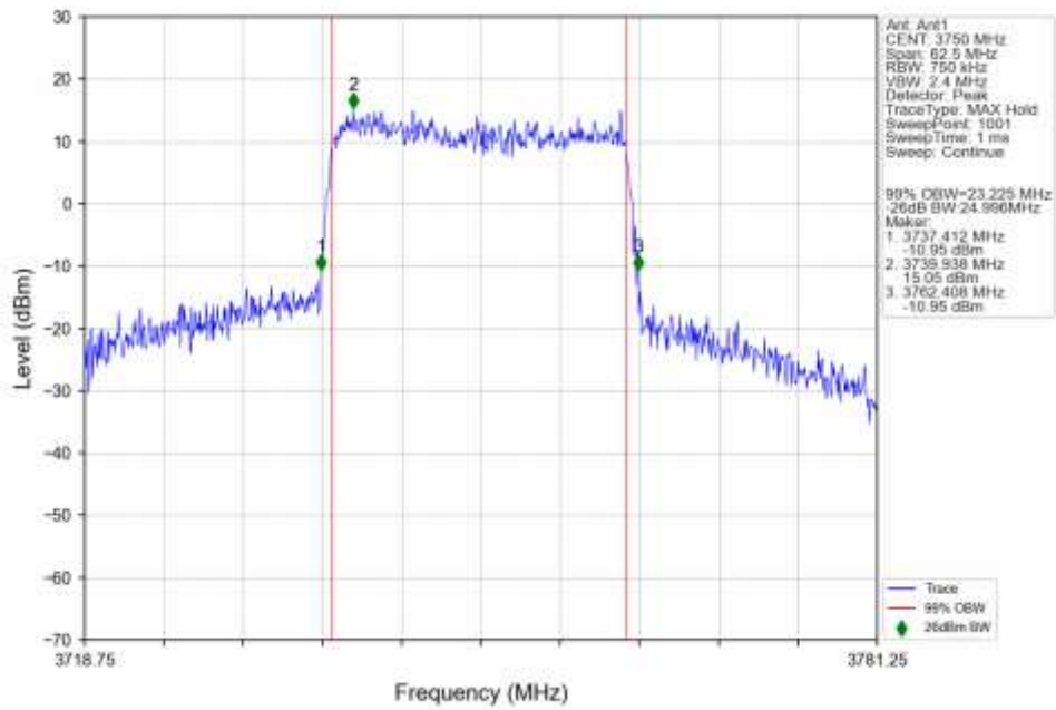
n78a 30kHz SISO NTN 25MHz DFT-s-OFDM 64 QAM 3750MHz Outer Full Ant1
