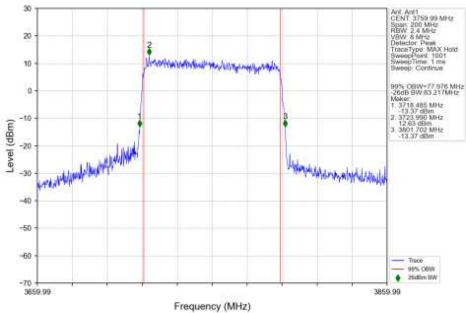
n78a 30kHz SISO NTN 80MHz CP-OFDM 256 QAM 3759.99MHz Outer Full Ant1
