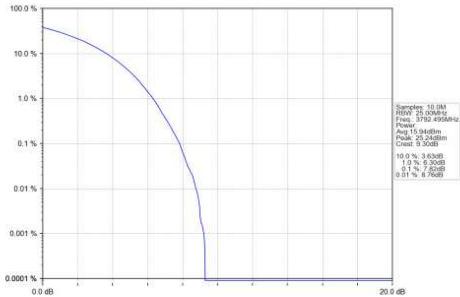
n78a 15kHz SISO NTN 15MHz CP-OFDM 256 QAM 3792.495MHz Outer Full Ant1
