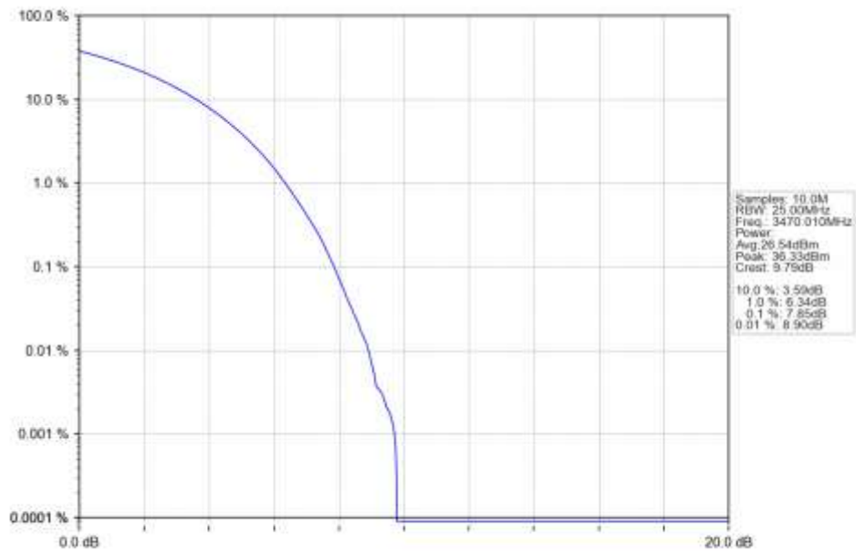
n77d 15kHz SISO NTN 40MHz CP-OFDM QPSK 3470.01MHz Outer Full Ant1
