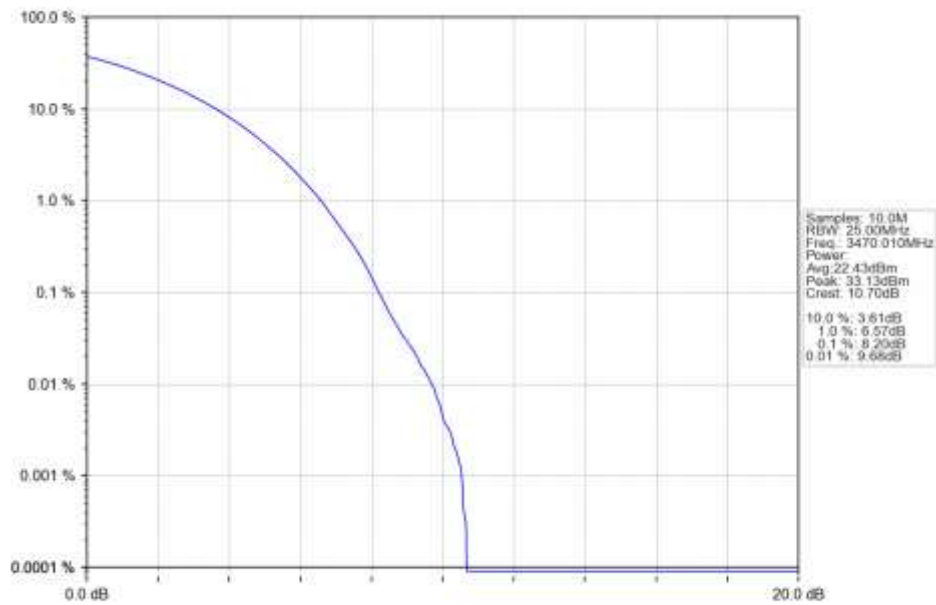
n77d 15kHz SISO NTN 40MHz CP-OFDM 256 QAM 3470.01MHz Outer Full Ant1
