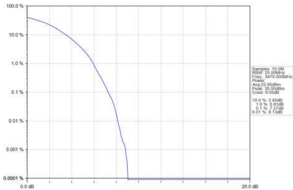
n77d 15kHz SISO NTN 50MHz DFT-s-OFDM 16 QAM 3475.005MHz Outer Full Ant1
