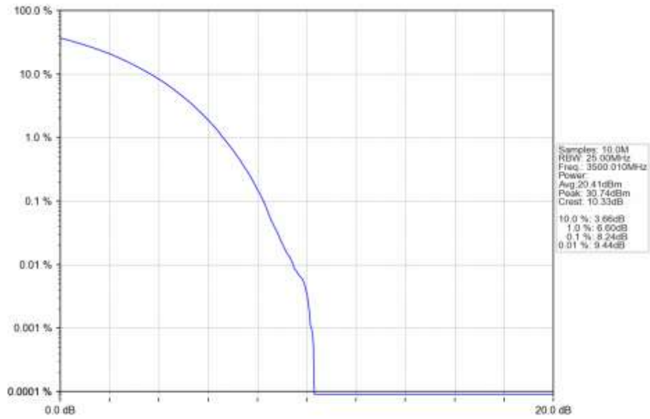
n77d 30kHz SISO NTN 70MHz CP-OFDM 256 QAM 3500.01MHz Outer Full Ant1
