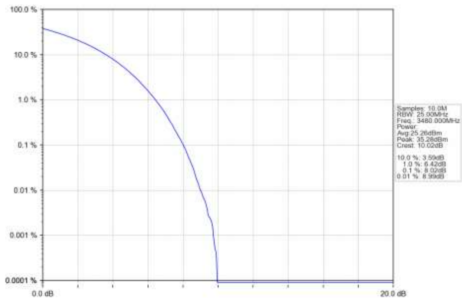
n77d 30kHz SISO NTN 60MHz CP-OFDM 16 QAM 3480MHz Outer Full Ant1
