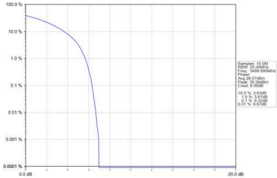
n77d 15kHz SISO NTN 20MHz CP-OFDM 16 QAM 3499.995MHz Outer Full Ant1
