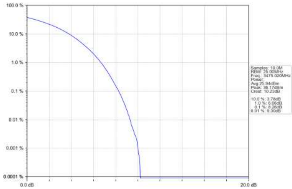
n77d 30kHz SISO NTN 50MHz CP-OFDM QPSK 3475.02MHz Outer Full Ant1
