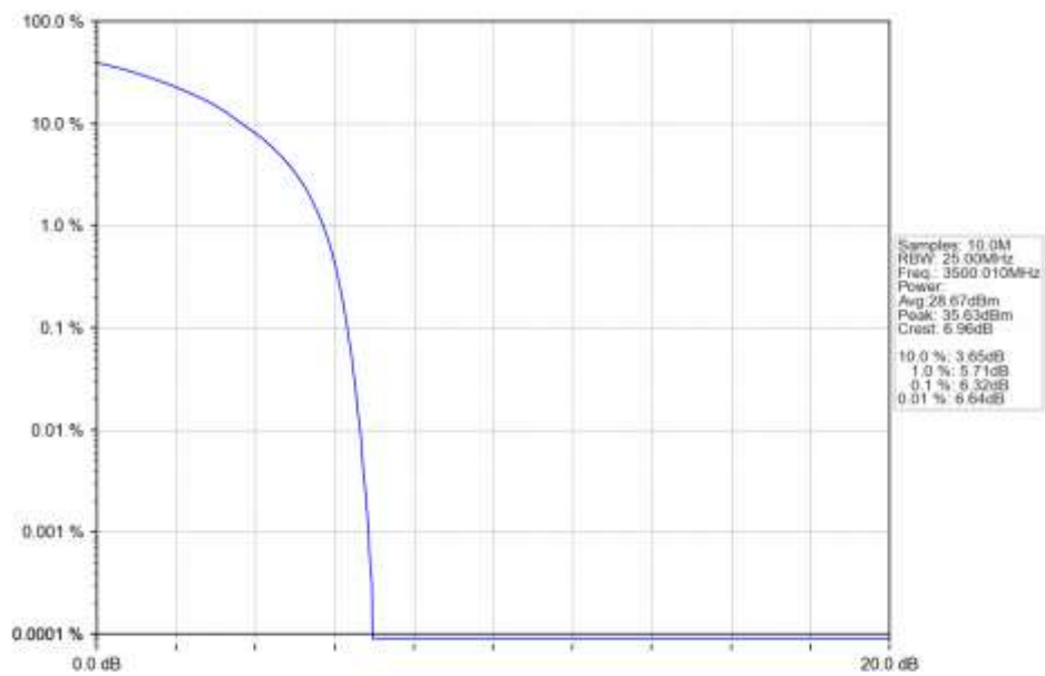
n77d 30kHz SISO NTN 20MHz CP-OFDM QPSK 3500.01MHz Outer Full Ant1
