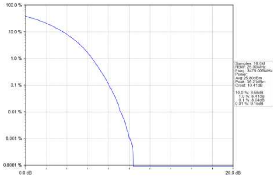
n77d 15kHz SISO NTN 50MHz CP-OFDM 64 QAM 3475.005MHz Outer Full Ant1
