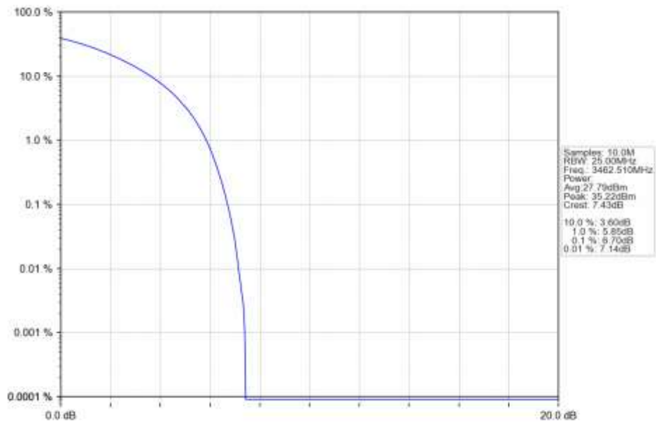
n77d 15kHz SISO NTN 25MHz CP-OFDM QPSK 3462.51MHz Outer Full Ant1
