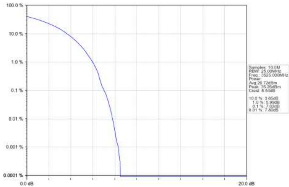
n77d 30kHz SISO NTN 50MHz DFT-s-OFDM QPSK 3525MHz Outer Full Ant1
