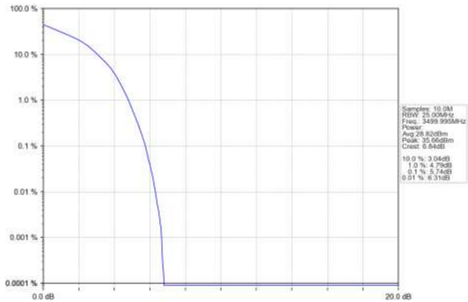
n77d 15kHz SISO NTN 25MHz DFT-s-OFDM 16 QAM 3499.995MHz Outer Full Ant1
