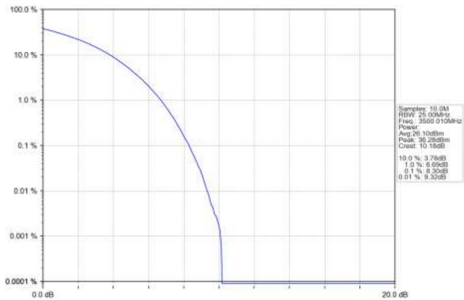
n77d 30kHz SISO NTN 50MHz CP-OFDM QPSK 3500.01MHz Outer Full Ant1
