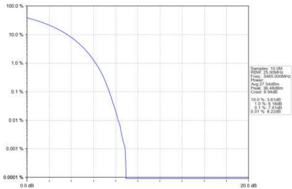
n77d 15kHz SISO NTN 30MHz CP-OFDM 16 QAM 3465MHz Outer Full Ant1
