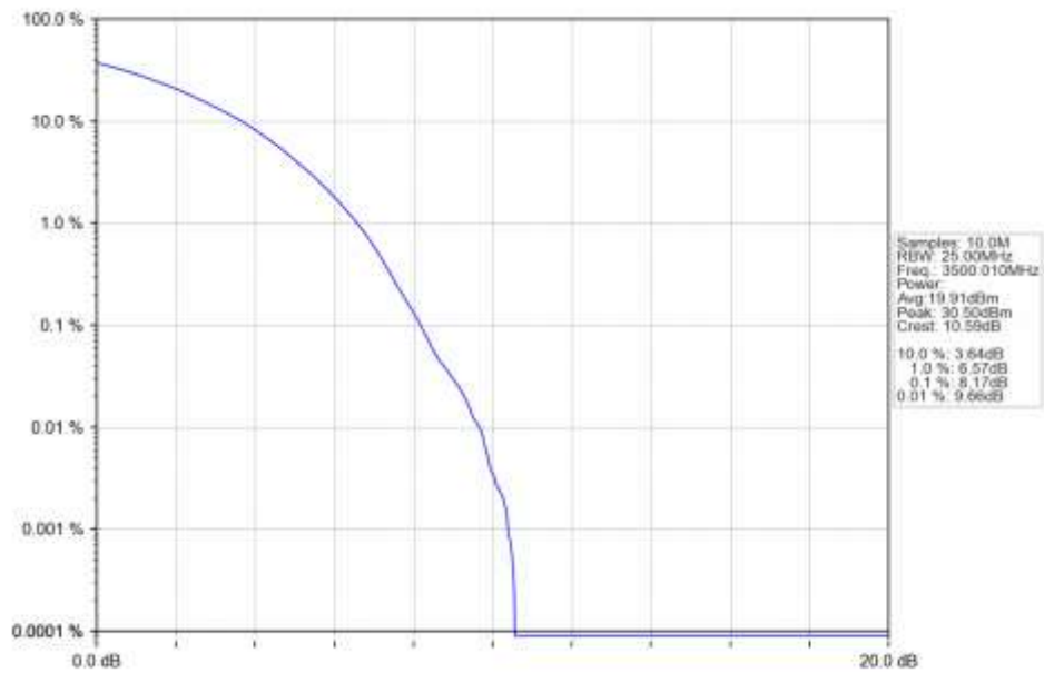
n77d 30kHz SISO NTN 80MHz CP-OFDM 256 QAM 3500.01MHz Outer Full Ant1
