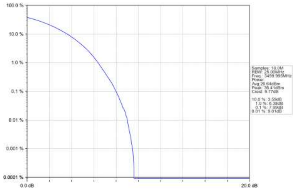
n77d 15kHz SISO NTN 50MHz CP-OFDM 16 QAM 3499.995MHz Outer Full Ant1
