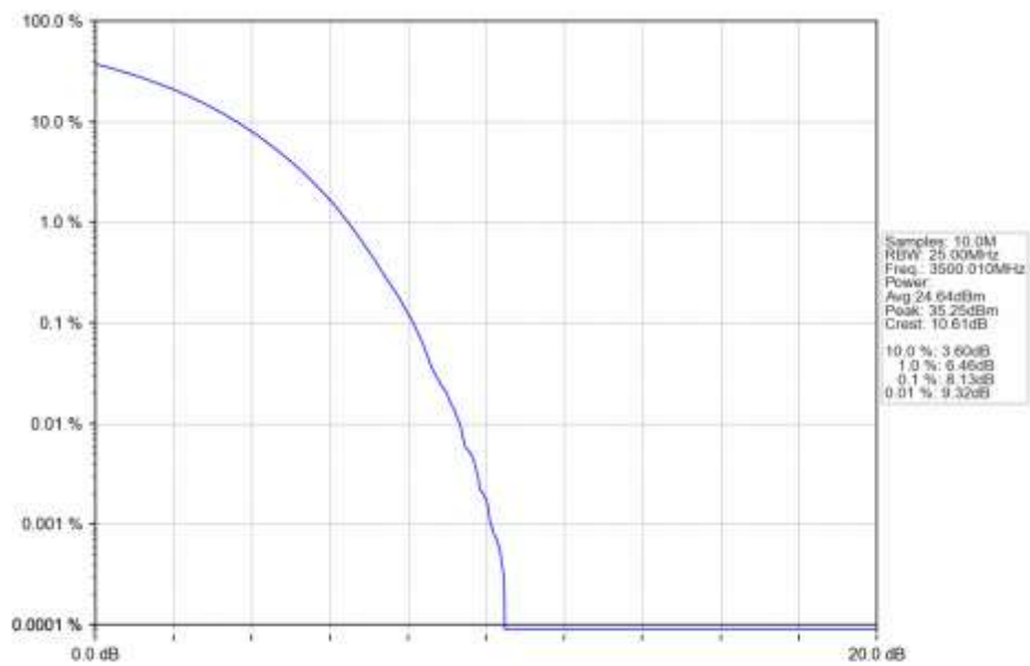
n77d 30kHz SISO NTN 70MHz CP-OFDM QPSK 3500.01MHz Outer Full Ant1
