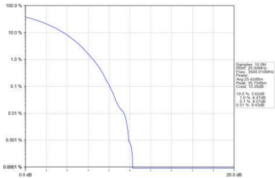
n77d 30kHz SISO NTN 60MHz CP-OFDM QPSK 3500.01MHz Outer Full Ant1
