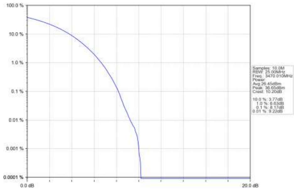
n77d 30kHz SISO NTN 40MHz CP-OFDM QPSK 3470.01MHz Outer Full Ant1
