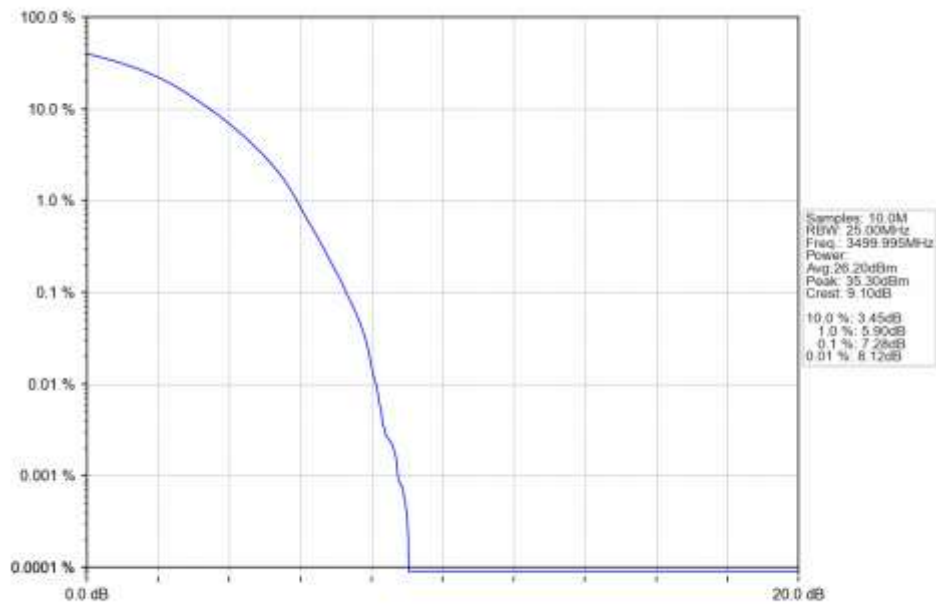
n77d 15kHz SISO NTN 50MHz DFT-s-OFDM 16 QAM 3499.995MHz Outer Full Ant1
