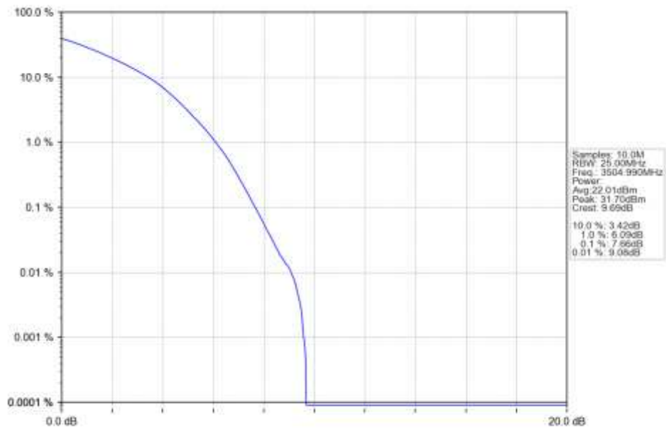
n77d 30kHz SISO NTN 90MHz DFT-s-OFDM 256 QAM 3504.99MHz Outer Full Ant1
