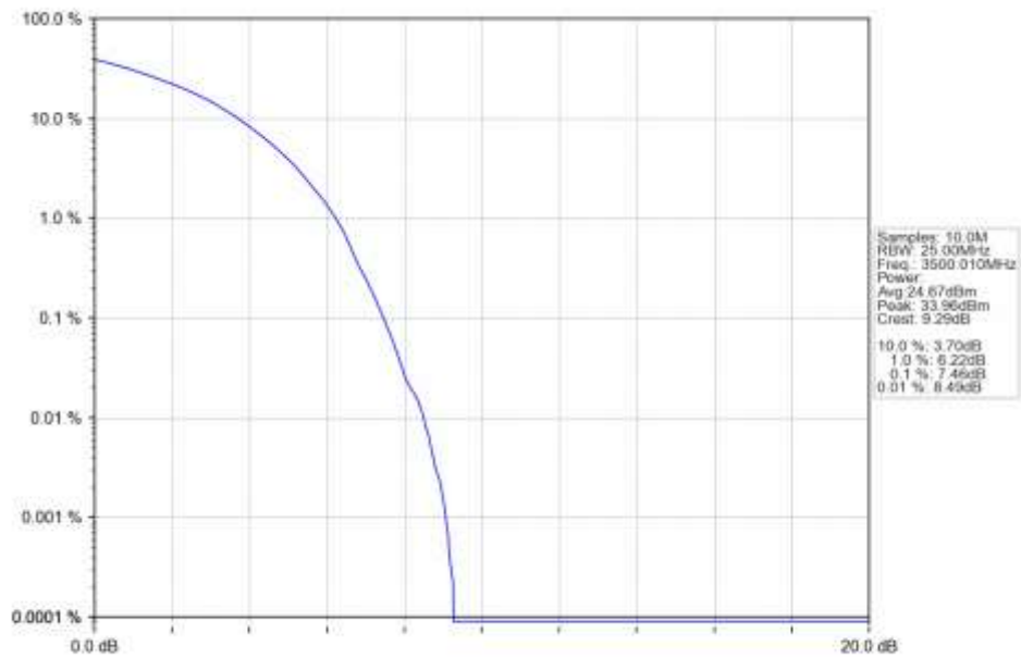
n77d 30kHz SISO NTN 50MHz DFT-s-OFDM 256 QAM 3500.01MHz Outer Full Ant1
