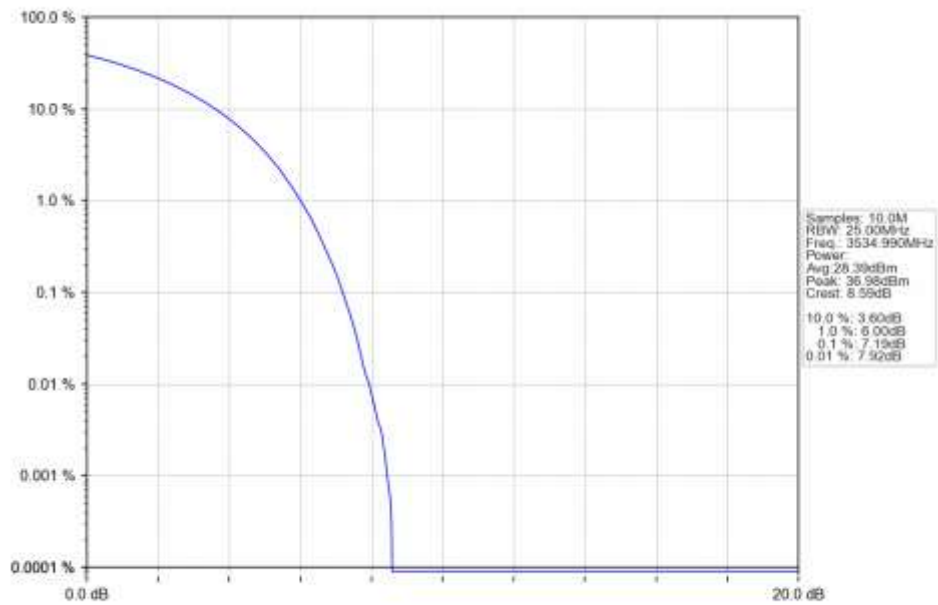
n77d 15kHz SISO NTN 30MHz CP-OFDM QPSK 3534.99MHz Outer Full Ant1
