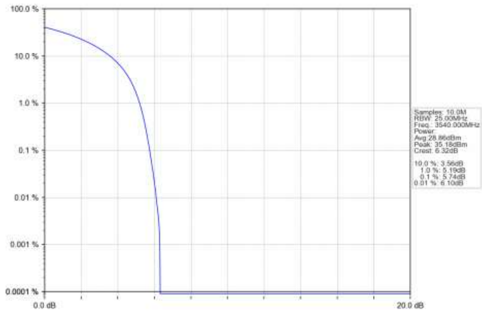
n77d 15kHz SISO NTN 20MHz CP-OFDM QPSK 3540MHz Outer Full Ant1
