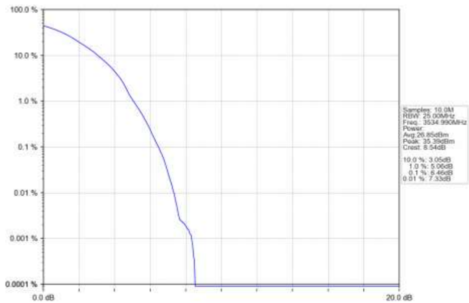
n77d 30kHz SISO NTN 30MHz DFT-s-OFDM 256 QAM 3534.99MHz Outer Full Ant1
