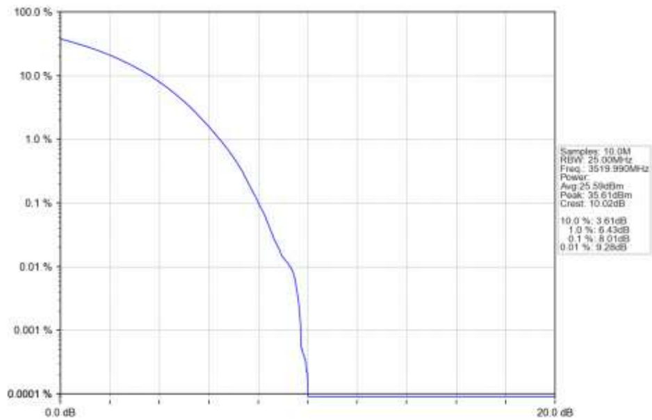
n77d 30kHz SISO NTN 60MHz CP-OFDM QPSK 3519.99MHz Outer Full Ant1
