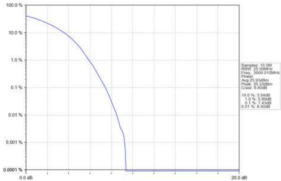
n77d 30kHz SISO NTN 40MHz DFT-s-OFDM 256 QAM 3500.01MHz Outer Full Ant1
