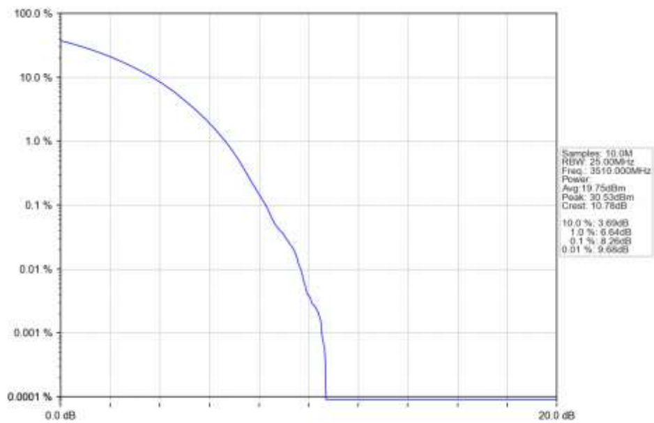
n77d 30kHz SISO NTN 80MHz CP-OFDM 256 QAM 3510MHz Outer Full Ant1
