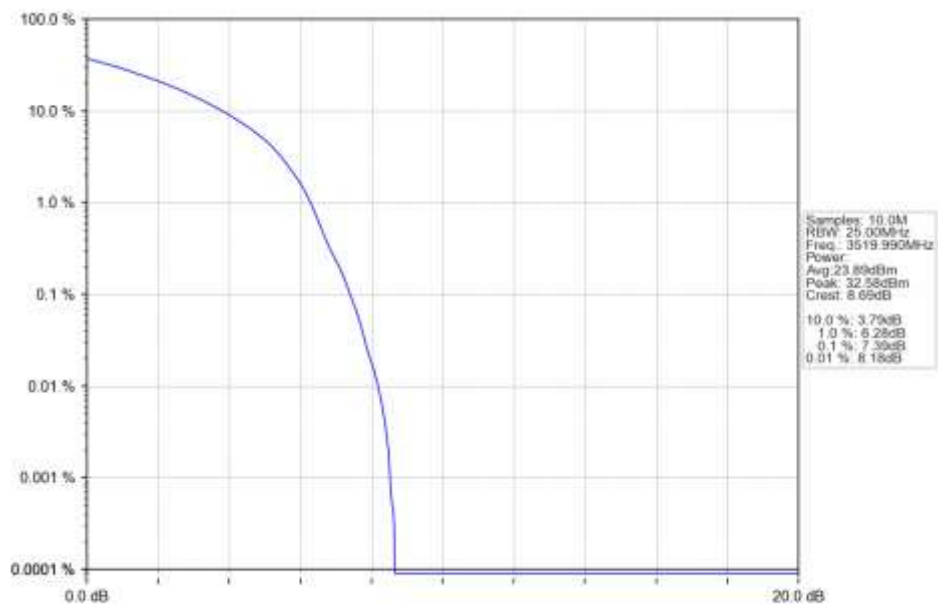
n77d 30kHz SISO NTN 60MHz DFT-s-OFDM 256 QAM 3519.99MHz Outer Full Ant1
