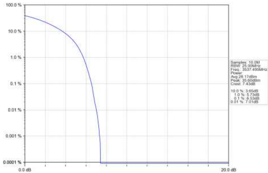
n77d 15kHz SISO NTN 25MHz CP-OFDM 64 QAM 3537.495MHz Outer Full Ant1
