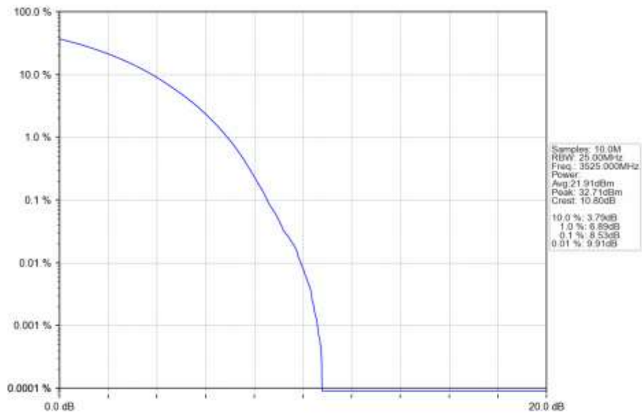
n77d 30kHz SISO NTN 50MHz CP-OFDM 256 QAM 3525MHz Outer Full Ant1
