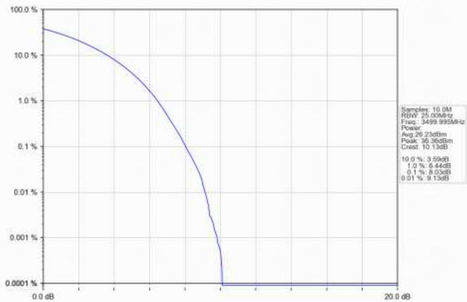
n77d 15kHz SISO NTN 50MHz CP-OFDM 64 QAM 3499.995MHz Outer Full Ant1
