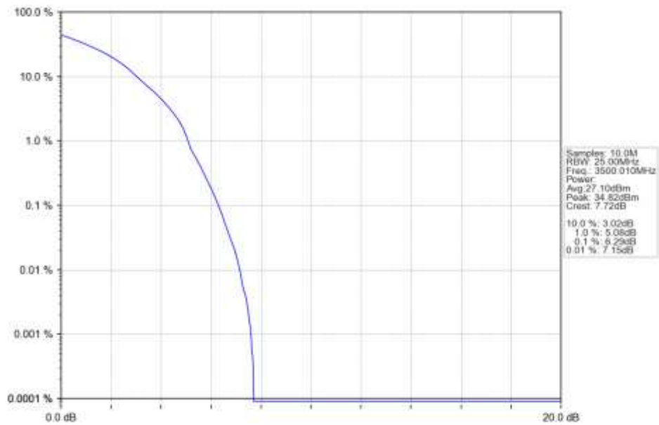
n77d 30kHz SISO NTN 20MHz DFT-s-OFDM 256 QAM 3500.01MHz Outer Full Ant1
