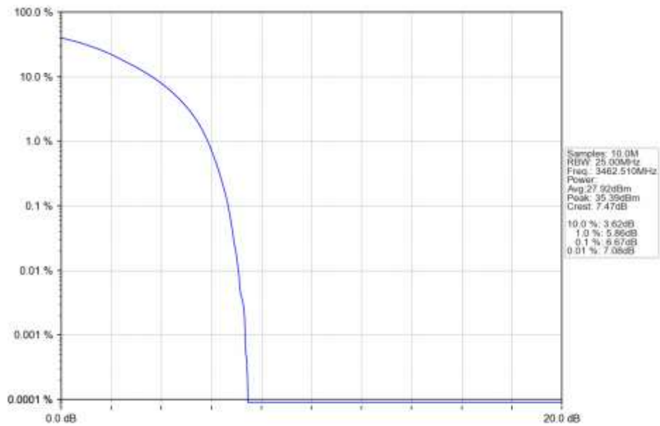
n77d 30kHz SISO NTN 25MHz CP-OFDM QPSK 3462.51MHz Outer Full Ant1
