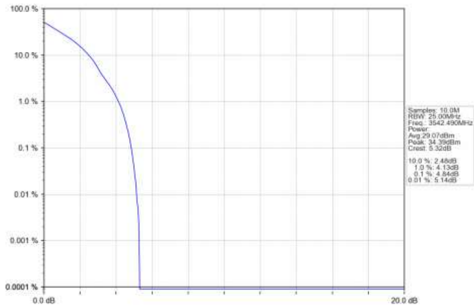
n77d 30kHz SISO NTN 15MHz DFT-s-OFDM QPSK 3542.49MHz Outer Full Ant1
