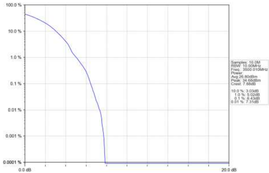
n77d 30kHz SISO NTN 10MHz DFT-s-OFDM 256 QAM 3500.01MHz Outer Full Ant1
