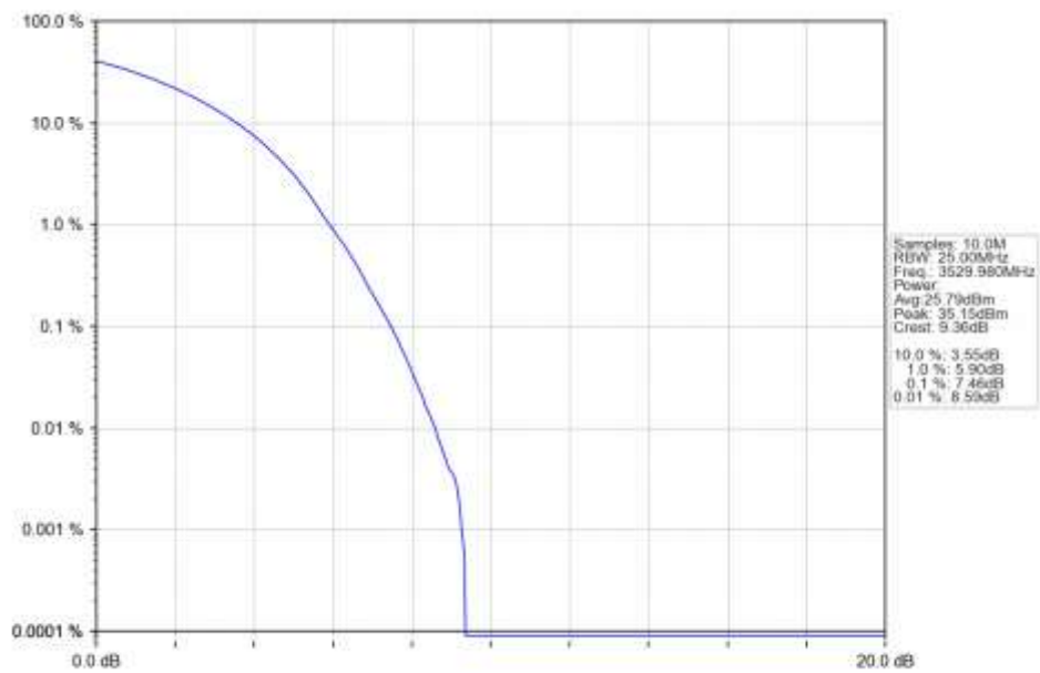
n77d 30kHz SISO NTN 40MHz DFT-s-OFDM 256 QAM 3529.98MHz Outer Full Ant1
