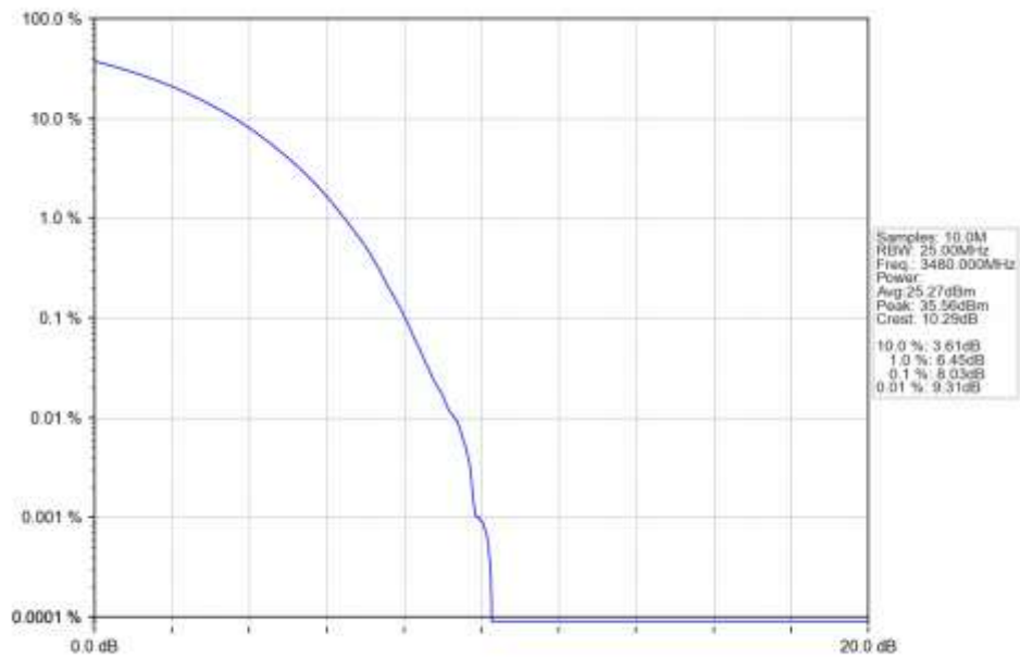
n77d 30kHz SISO NTN 60MHz CP-OFDM QPSK 3480MHz Outer Full Ant1
