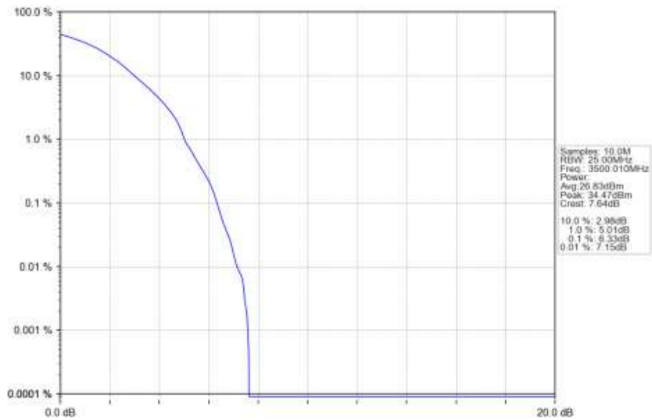
n77d 30kHz SISO NTN 15MHz DFT-s-OFDM 256 QAM 3500.01MHz Outer Full Ant1
