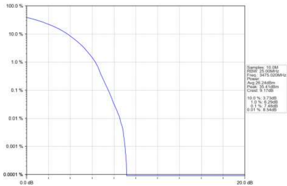
n77d 30kHz SISO NTN 50MHz DFT-s-OFDM 16 QAM 3475.02MHz Outer Full Ant1
