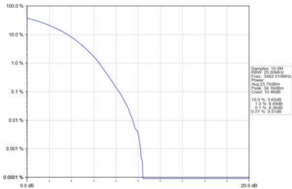
n77d 15kHz SISO NTN 25MHz CP-OFDM 256 QAM 3462.51MHz Outer Full Ant1
