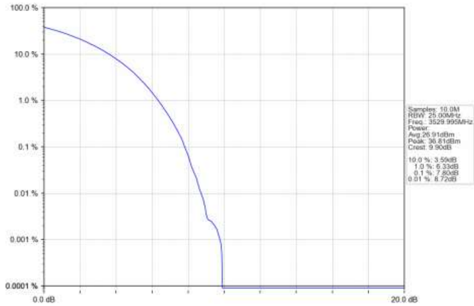
n77d 15kHz SISO NTN 40MHz CP-OFDM 64 QAM 3529.995MHz Outer Full Ant1
