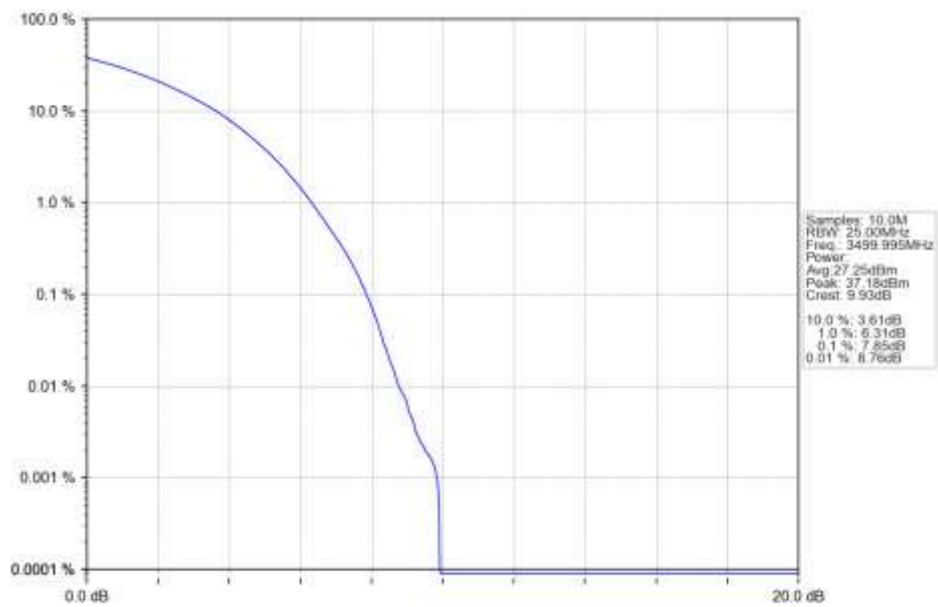
n77d 15kHz SISO NTN 40MHz CP-OFDM QPSK 3499.995MHz Outer Full Ant1
