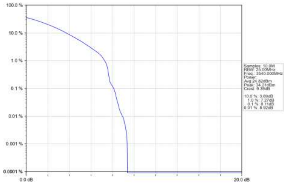
n77d 30kHz SISO NTN 20MHz CP-OFDM 256 QAM 3540MHz Outer Full Ant1
