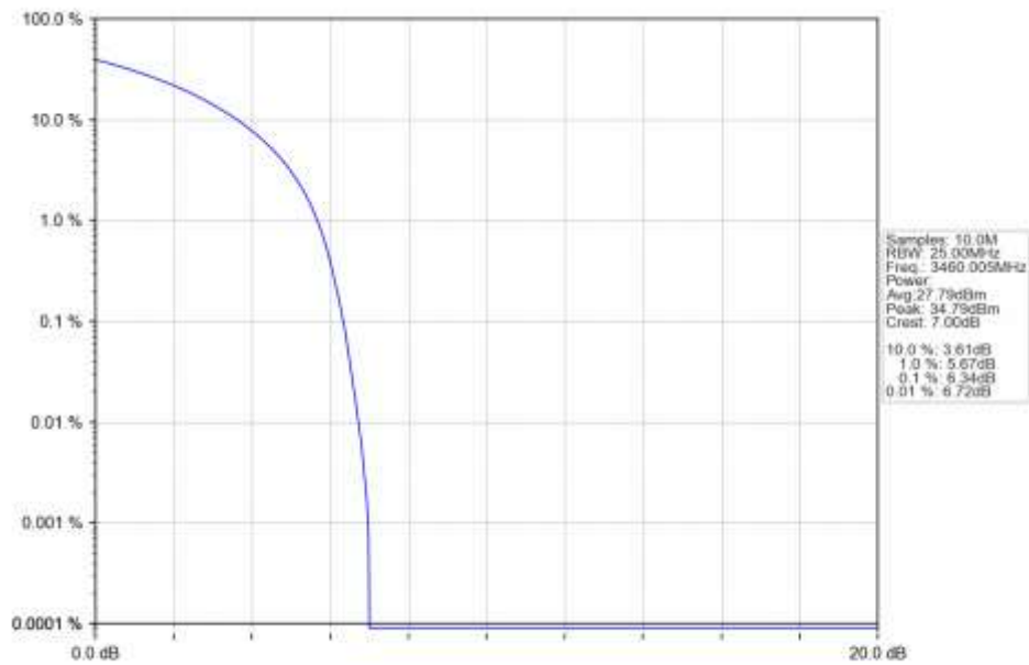
n77d 15kHz SISO NTV 20MHz CP-OFDM QPSK 3460.005MHz Outer Full Ant1
