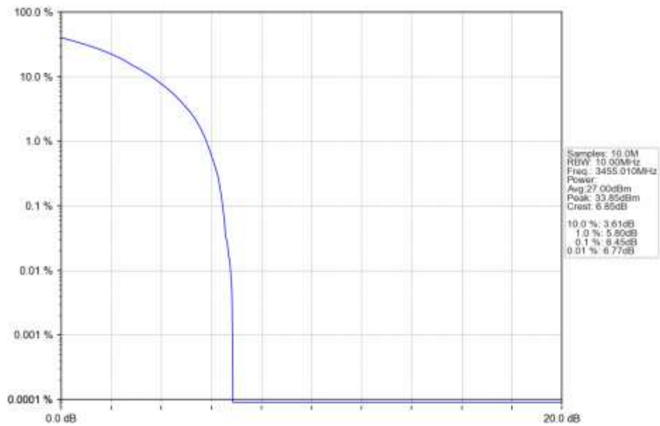
n77d 30kHz SISO NTN 10MHz CP-OFDM QPSK 3455.01MHz Outer Full Ant1
