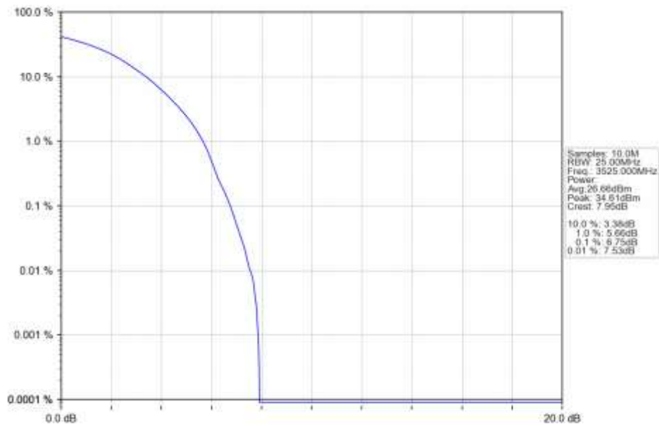
n77d 15kHz SISO NTN 50MHz DFT-s-OFDM QPSK 3525MHz Outer Full Ant1
