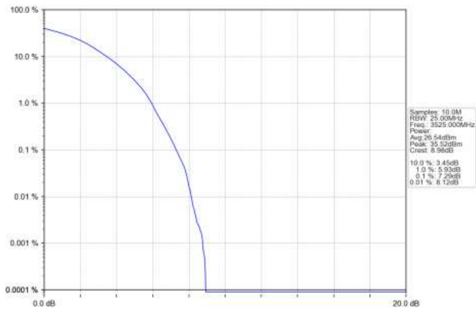
n77d 15kHz SISO NTN 50MHz DFT-s-OFDM 16 QAM 3525MHz Outer Full Ant1
