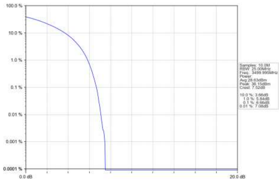
n77d 15kHz SISO NTN 25MHz CP-OFDM QPSK 3499.995MHz Outer Full Ant1
