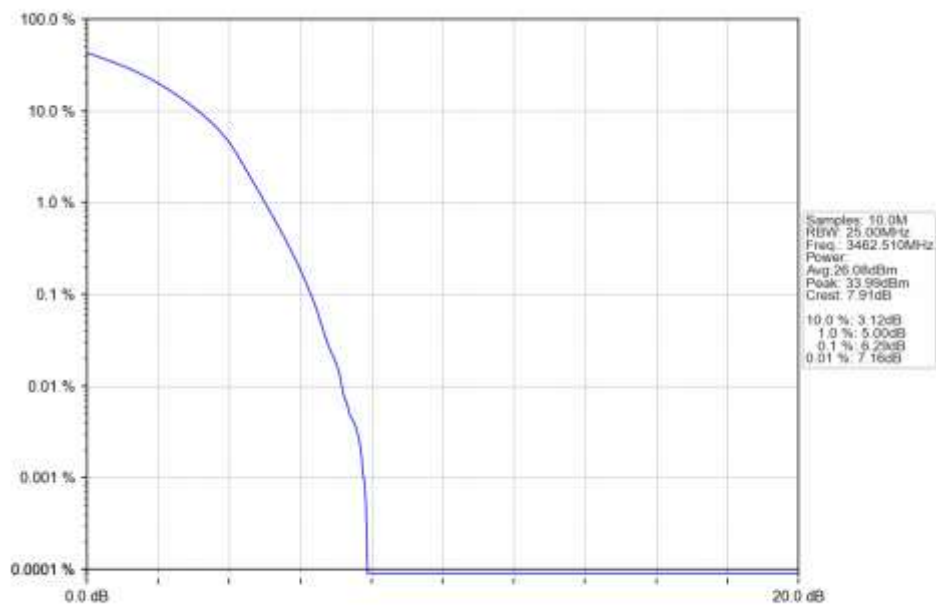
n77d 15kHz SISO NTN 25MHz DFT-s-OFDM 256 QAM 3462.51MHz Outer Full Ant1
