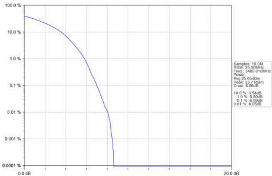
n77d_30kHz_SISO_NTNV_70MHz_DFT-s-OFDM QPSK_3485.01MHz_Outer_Full_Ant1
