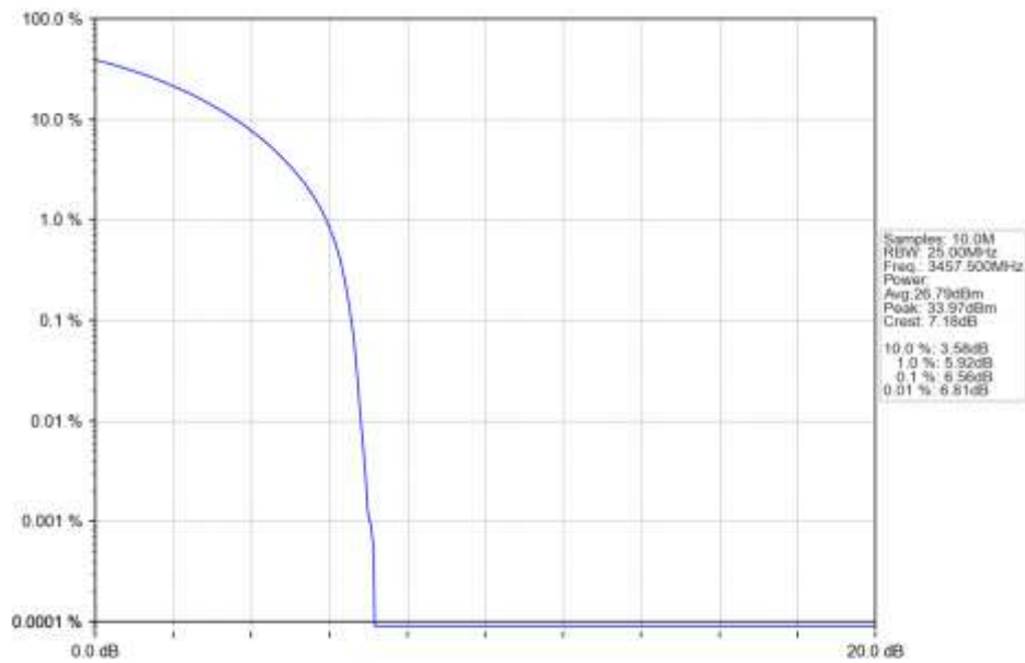
n77d 15kHz SISO NTN 15MHz CP-OFDM 64 QAM 3457.5MHz Outer Full Ant1
