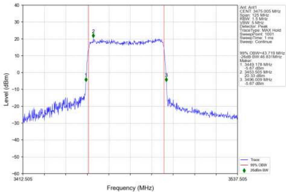
n77d 15kHz SISO NTN 50MHz CP-OFDM 256 QAM 3475.005MHz Outer Full Ant1
