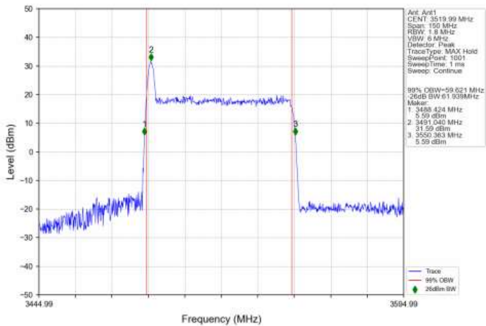
n77d 30kHz SISO NTN 60MHz CP-OFDM 256 QAM 3519.99MHz Outer Full Ant1
