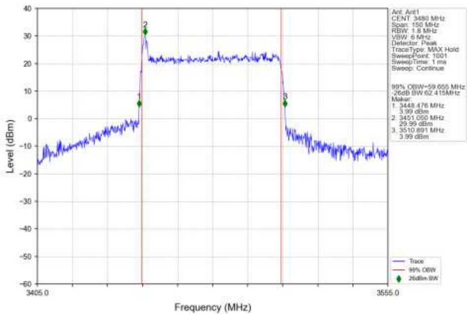
n77d 30kHz SISO NTN 60MHz CP-OFDM 16 QAM 3480MHz Outer Full Ant1
