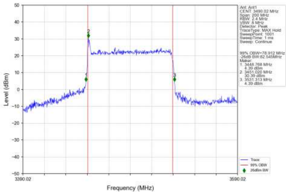
n77d 30kHz SISO NTN 80MHz CP-OFDM 16 QAM 3490.02MHz Outer Full Ant1
