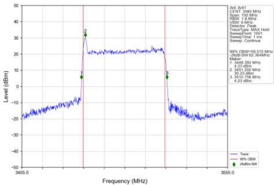
n77d 30kHz SISO NTN 60MHz DFT-s-OFDM 16 QAM 3480MHz Outer Full Ant1
