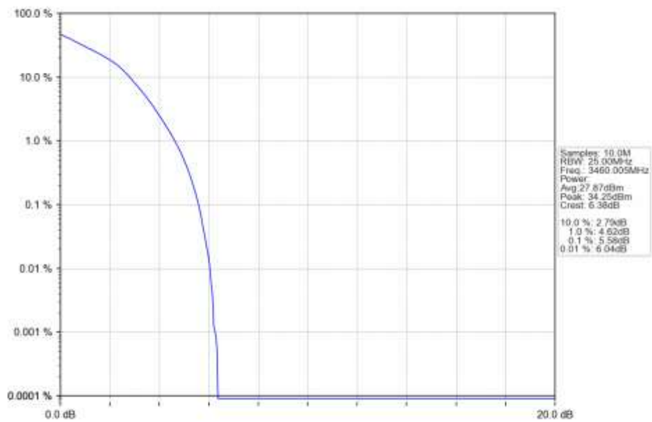
n77d 15kHz SISO NTN 20MHz DFT-s-OFDM 16 QAM 3460.005MHz Outer Full Ant1
