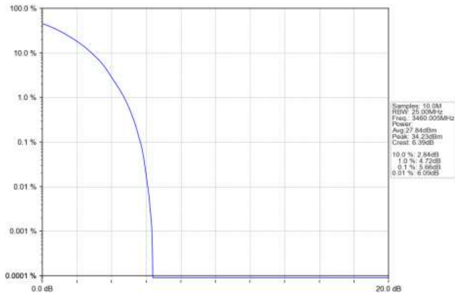
n77d 15kHz SISO NTN 20MHz DFT-s-OFDM 64 QAM 3460.005MHz Outer Full Ant1
