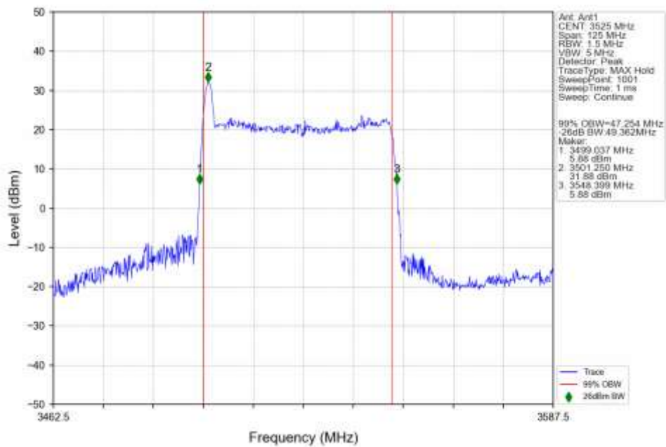
n77d 30kHz SISO NTN 50MHz DFT-s-OFDM 256 QAM 3525MHz Outer Full Ant1
