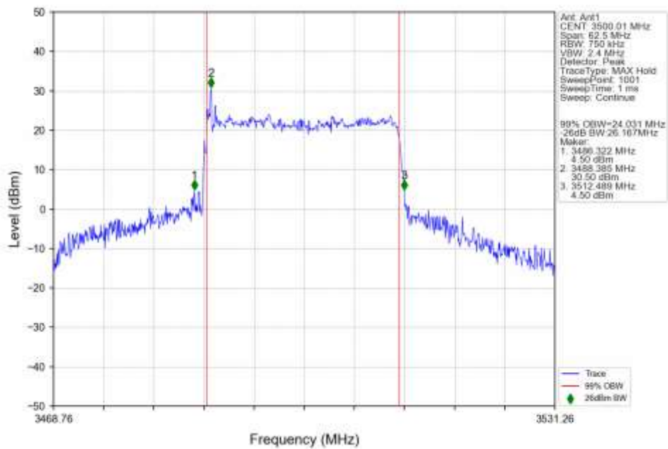
n77d 30kHz SISO NTN 25MHz CP-OFDM QPSK 3500.01MHz Outer Full Ant1
