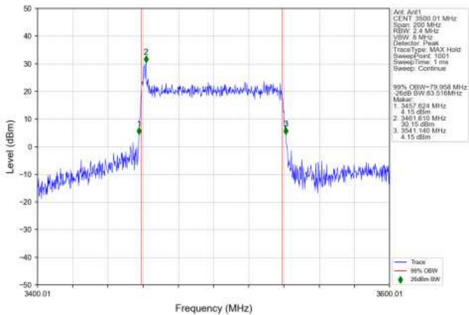
n77d 30kHz SISO NTN 80MHz CP-OFDM QPSK 3500.01MHz Outer Full Ant1
