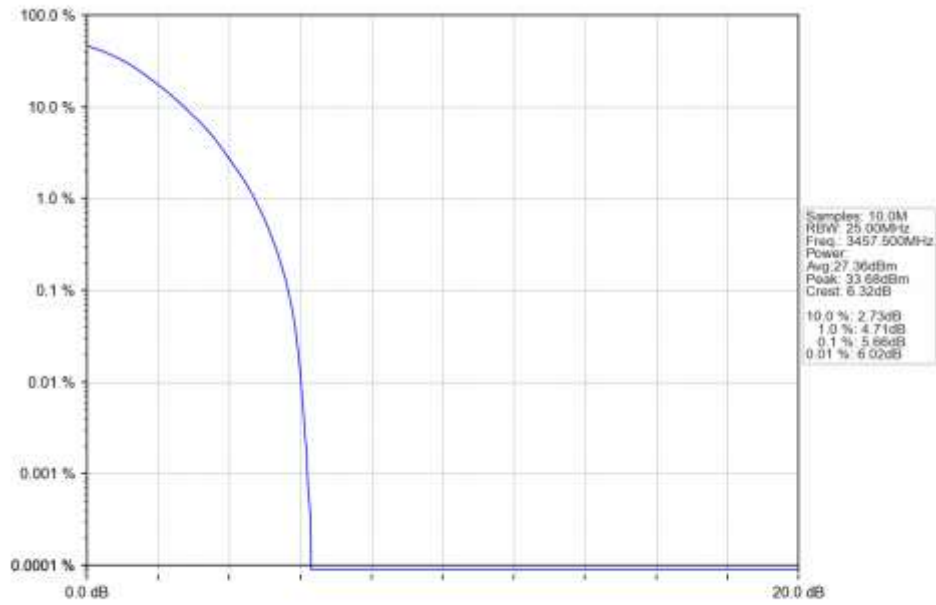
n77d 15kHz SISO NTN 15MHz DFT-s-OFDM 64 QAM 3457.5MHz Outer Full Ant1
