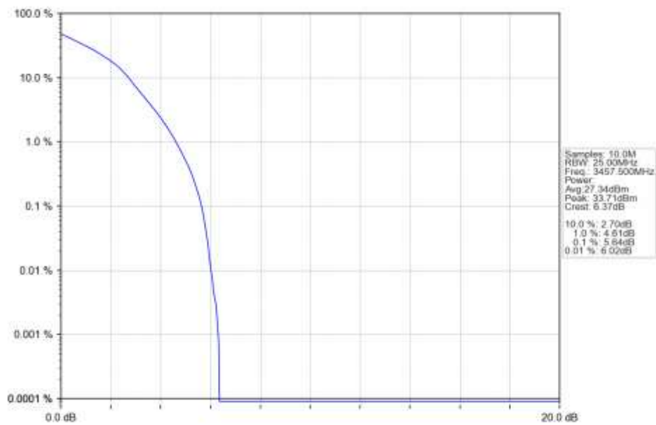
n77d 15kHz SISO NTN 15MHz DFT-s-OFDM 16 QAM 3457.5MHz Outer Full Ant1
