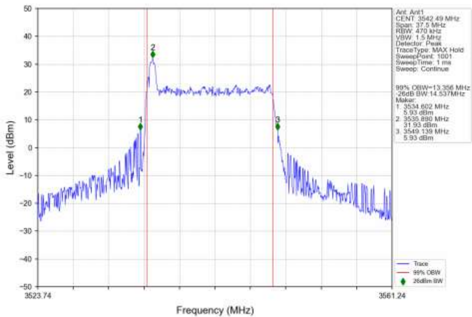
n77d 30kHz SISO NTN 15MHz DFT-s-OFDM 256 QAM 3542.49MHz Outer Full Ant1
