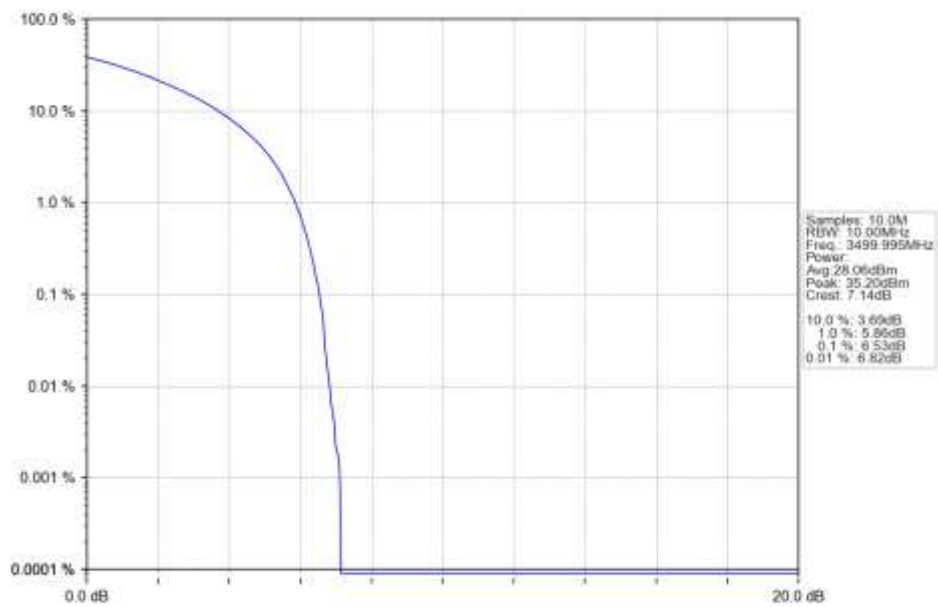
n77d 15kHz SISO NTN 10MHz CP-OFDM QPSK 3499.995MHz Outer Full Ant1
