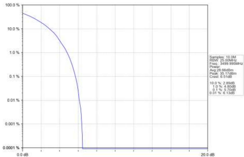
n77d 15kHz SISO NTN 20MHz DFT-s-OFDM 64 QAM 3499.995MHz Outer Full Ant1
