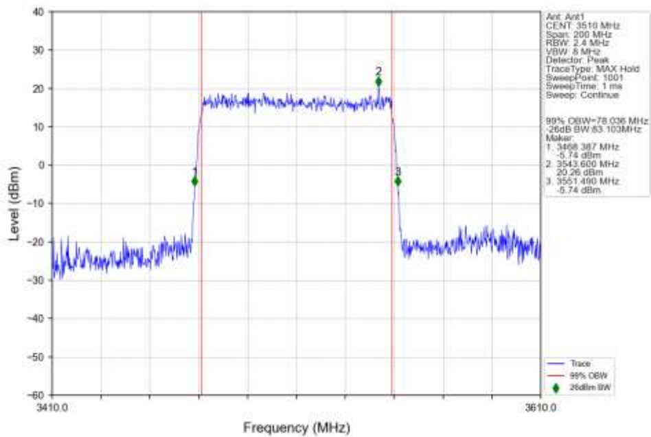
n77d 30kHz SISO NTN 80MHz CP-OFDM 256 QAM 3510MHz Outer Full Ant1
