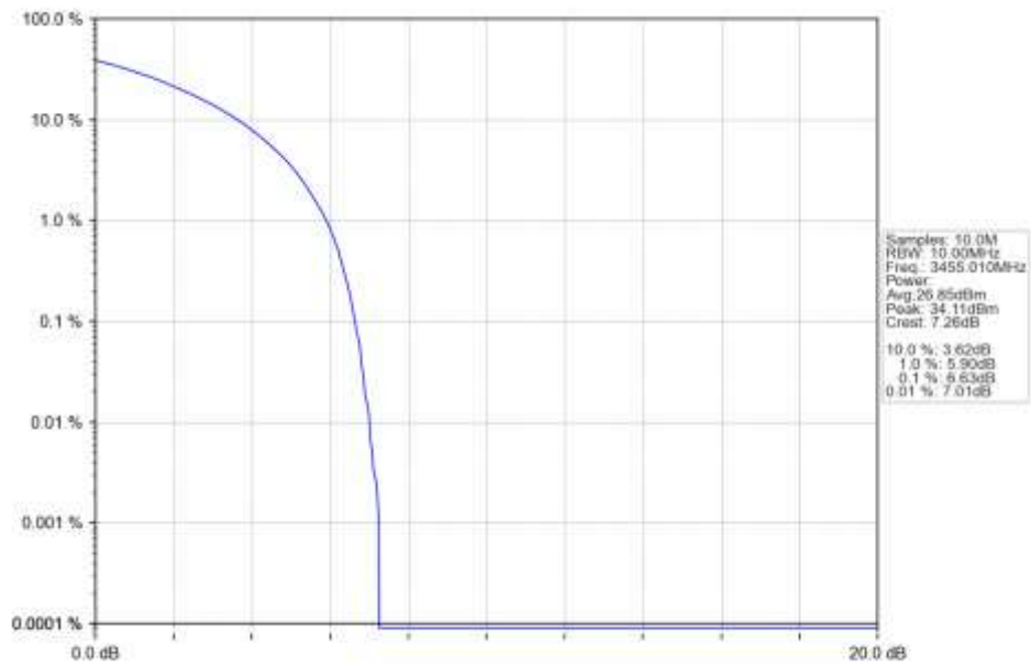
n77d 15kHz SISO NTN 10MHz CP-OFDM QPSK 3455.01MHz Outer Full Ant1
