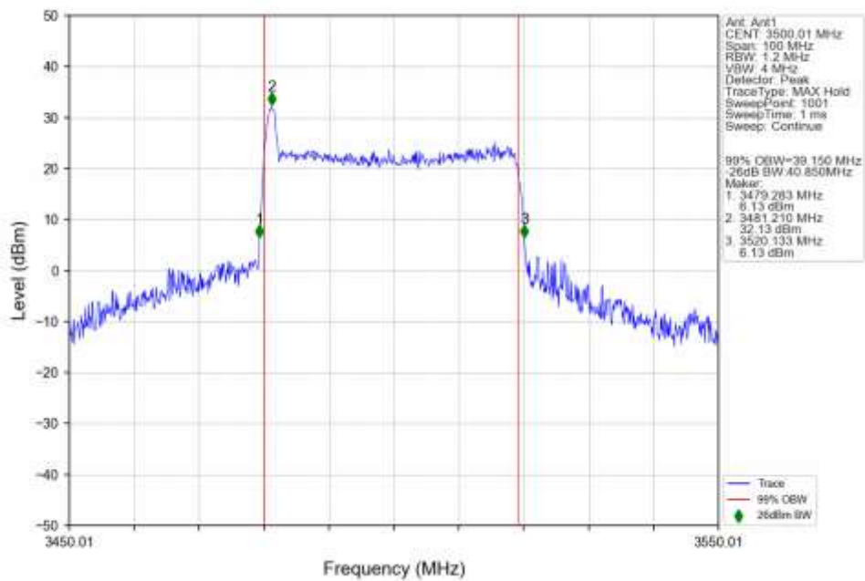
n77d 30kHz SISO NTN 40MHz CP-OFDM QPSK 3500.01MHz Outer Full Ant1
