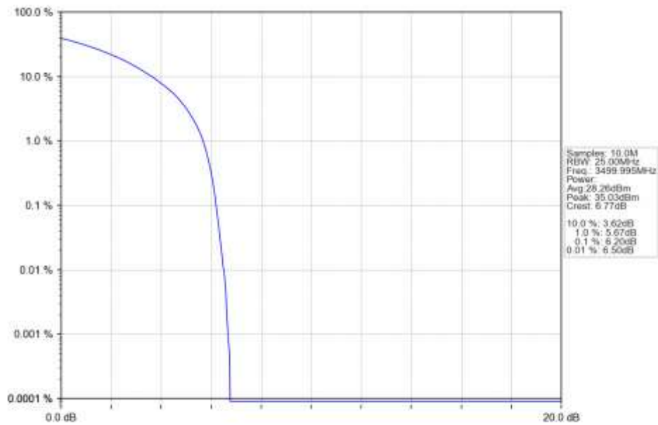
n77d 15kHz SISO NTN 15MHz CP-OFDM QPSK 3499.995MHz Outer Full Ant1
