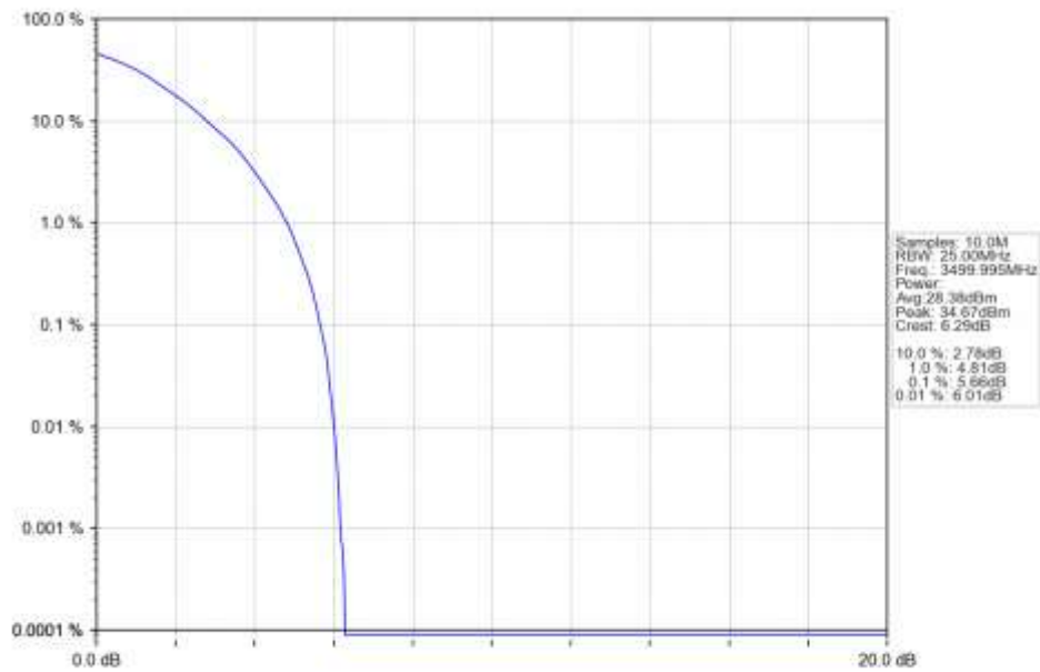
n77d 15kHz SISO NTN 15MHz DFT-s-OFDM 64 QAM 3499.995MHz Outer Full Ant1
