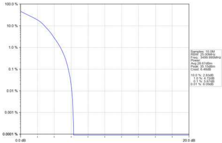
n77d 15kHz SISO NTN 20MHz DFT-s-OFDM 16 QAM 3499.995MHz Outer Full Ant1
