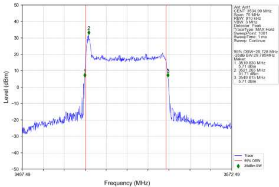
n77d 30kHz SISO NTN 30MHz CP-OFDM 256 QAM 3534.99MHz Outer Full Ant1
