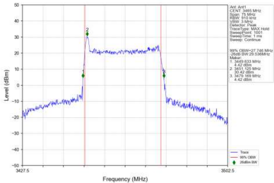
n77d 30kHz SISO NTN 30MHz DFT-s-OFDM 16 QAM 3465MHz Outer Full Ant1
