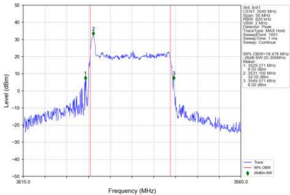
n77d 30kHz SISO NTN 20MHz DFT-s-OFDM 256 QAM 3540MHz Outer Full Ant1
