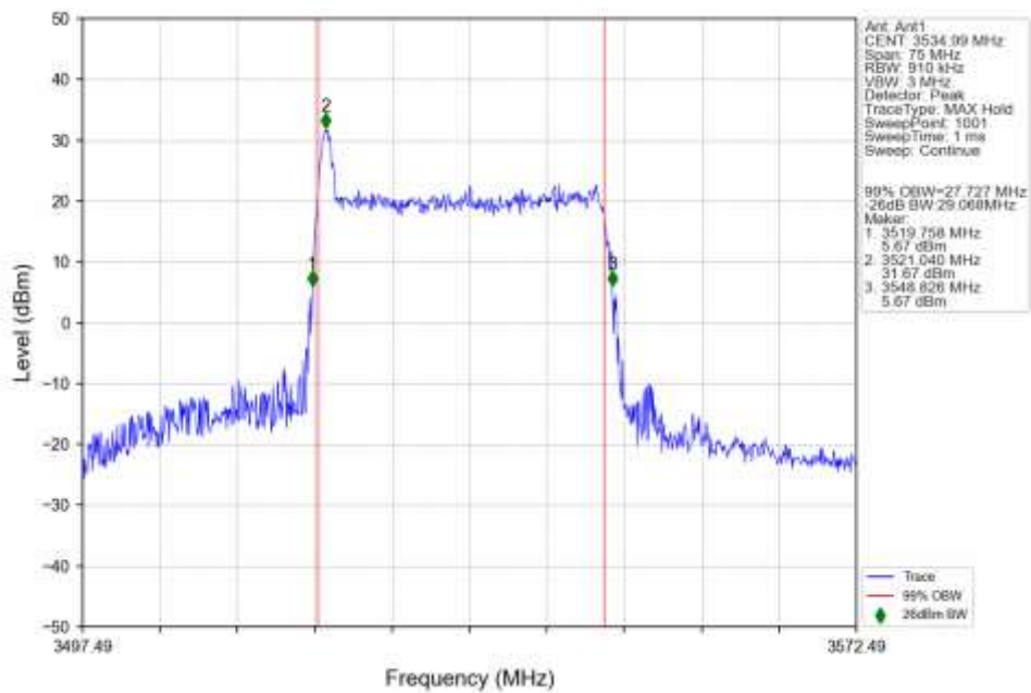
n77d 30kHz SISO NTN 30MHz DFT-s-OFDM 256 QAM 3534.99MHz Outer Full Ant1
