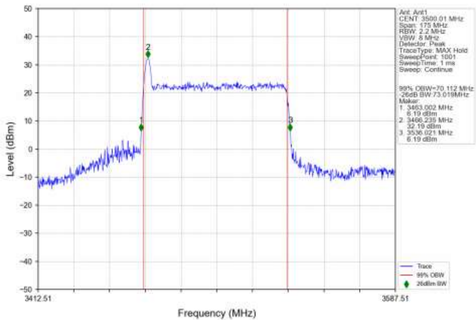
n77d 30kHz SISO NTN 70MHz CP-OFDM QPSK 3500.01MHz Outer Full Ant1
