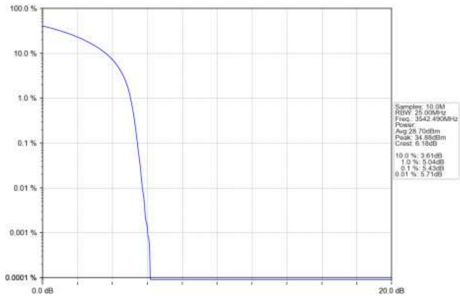
n77d 15kHz SISO NTN 15MHz CP-OFDM QPSK 3542.49MHz Outer Full Ant1
