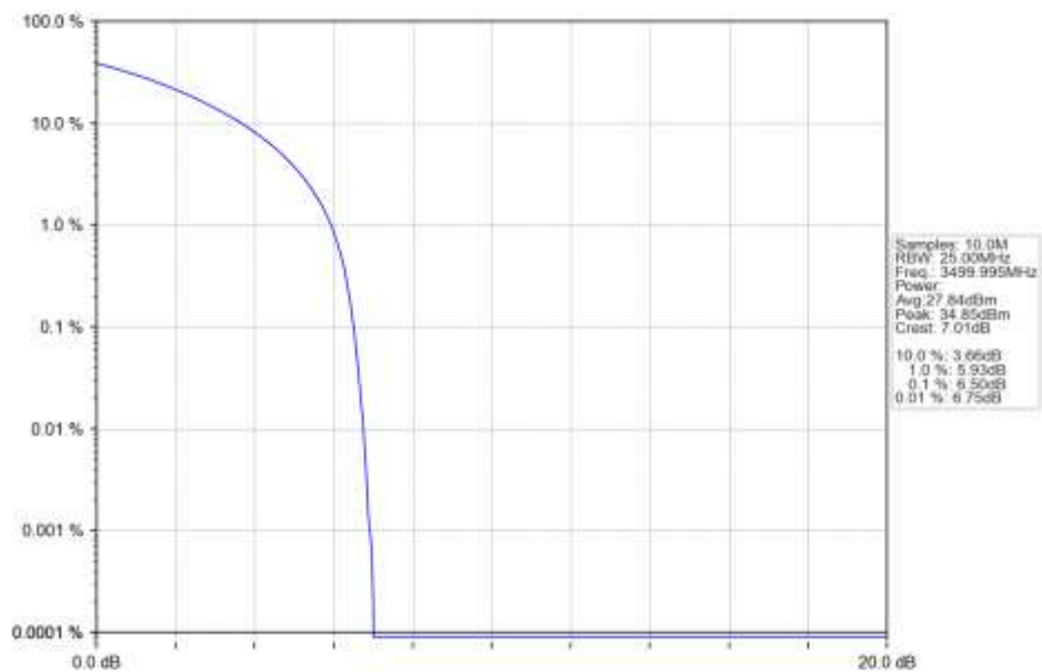
n77d 15kHz SISO NTN 15MHz CP-OFDM 64 QAM 3499.995MHz Outer Full Ant1
