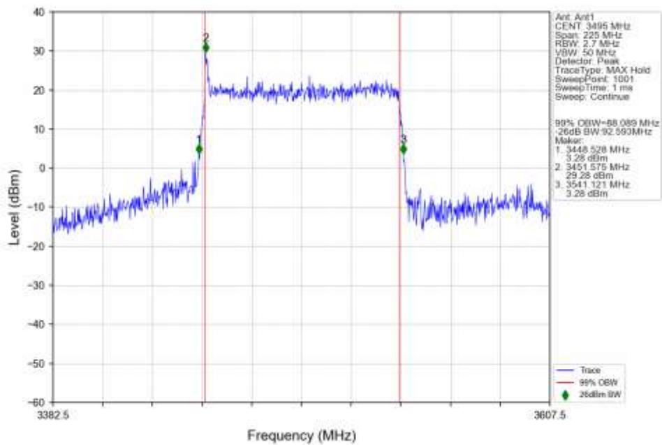
n77d 30kHz SISO NTN 90MHz CP-OFDM 16 QAM 3495MHz Outer Full Ant1
