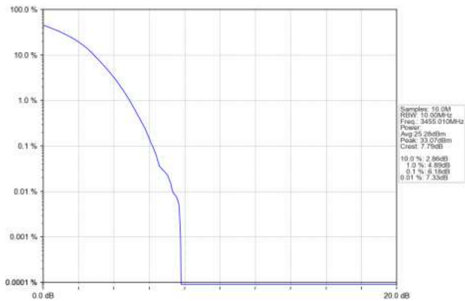
n77d 15kHz SISO NTN 10MHz DFT-s-OFDM 256 QAM 3455.01MHz Outer Full Ant1
