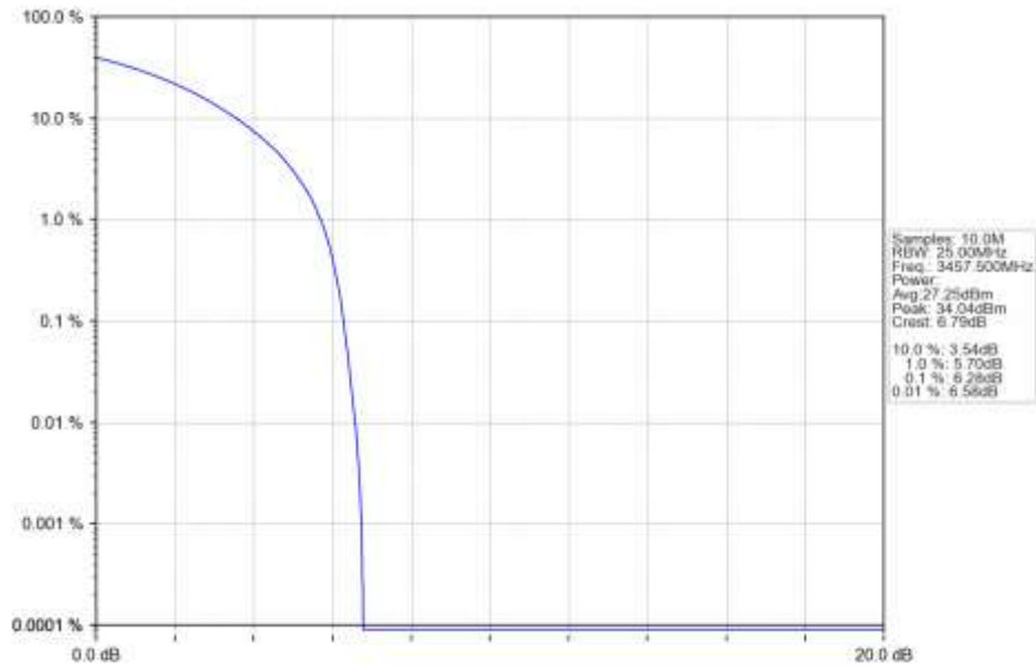
n77d 15kHz SISO NTN 15MHz CP-OFDM QPSK 3457.5MHz Outer Full Ant1
