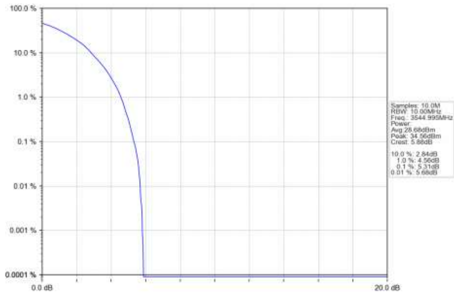
n77d 15kHz SISO NTN 10MHz DFT-s-OFDM 64 QAM 3544.995MHz Outer Full Ant1
