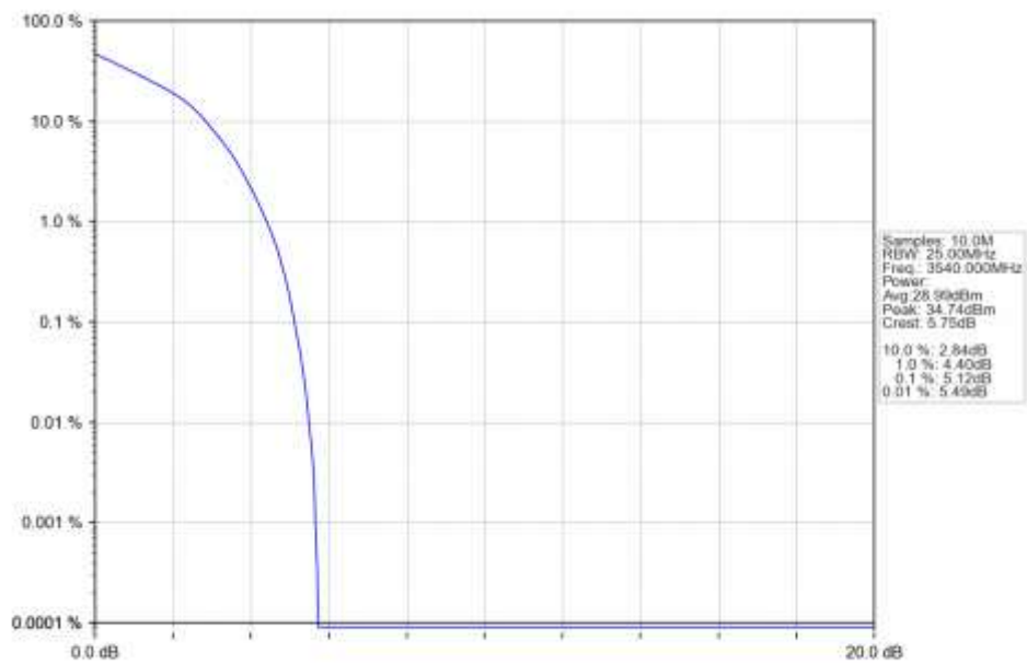
n77d 15kHz SISO NTN 20MHz DFT-s-OFDM 16 QAM 3540MHz Outer Full Ant1
