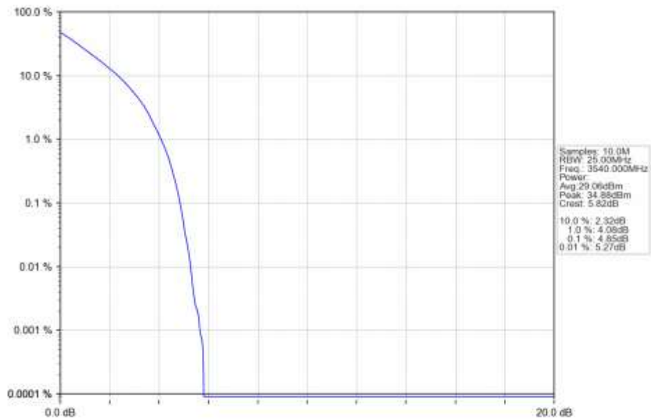
n77d 15kHz SISO NTN 20MHz DFT-s-OFDM QPSK 3540MHz Outer Full Ant1
