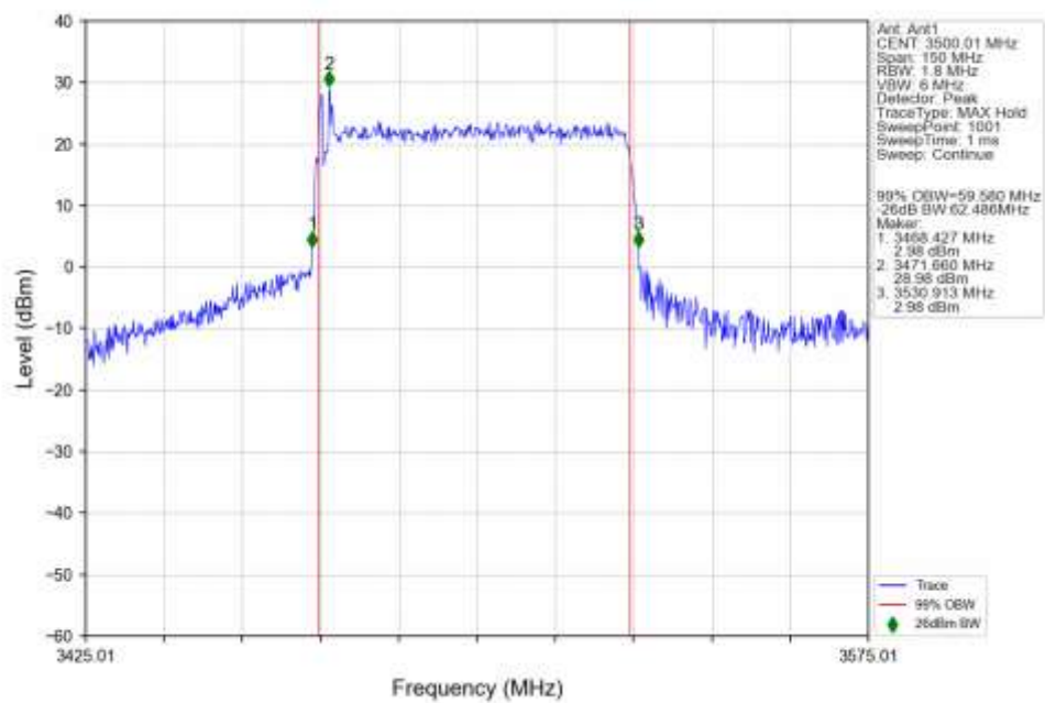
n77d 30kHz SISO NTN 60MHz CP-OFDM QPSK 3500.01MHz Outer Full Ant1
