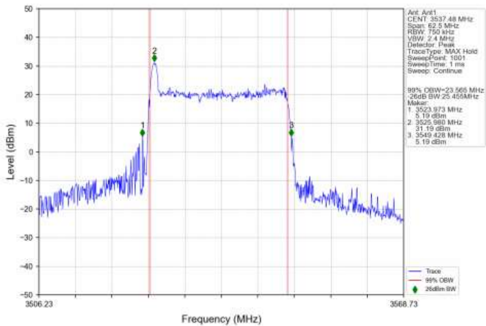
n77d 30kHz SISO NTN 25MHz DFT-s-OFDM 256 QAM 3537.48MHz Outer Full Ant1
