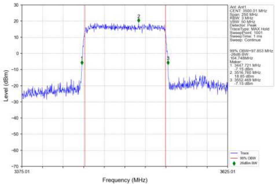
n77d 30kHz SISO NTN 100MHz CP-OFDM 256 QAM 3500.01MHz Outer Full Ant1
