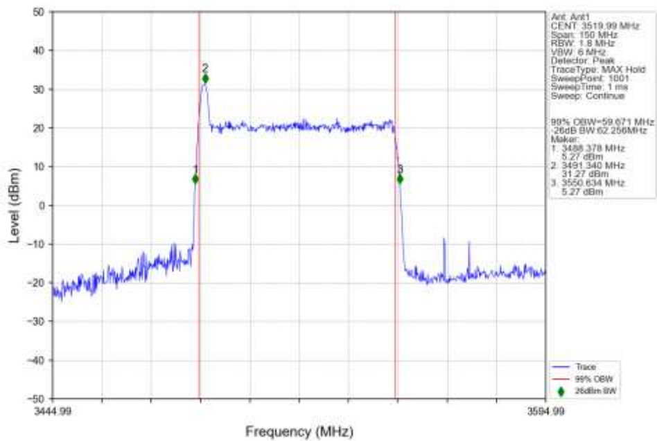
n77d 30kHz SISO NTN 60MHz DFT-s-OFDM 256 QAM 3519.99MHz Outer Full Ant1
