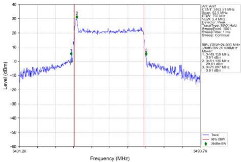
n77d 30kHz SISO NTN 25MHz CP-OFDM 16 QAM 3462.51MHz Outer Full Ant1
