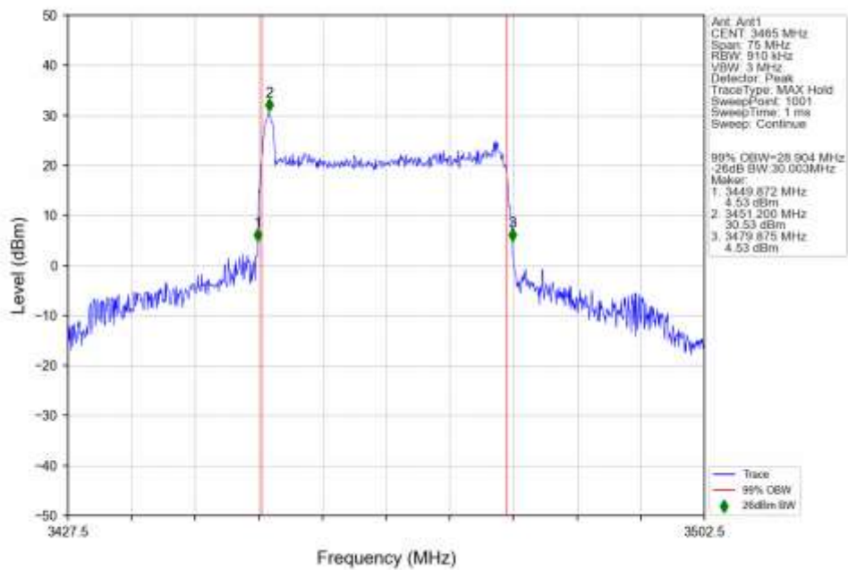
n77d 30kHz SISO NTN 30MHz CP-OFDM 16 QAM 3465MHz Outer Full Ant1
