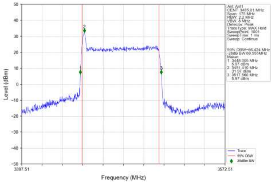
n77d 30kHz SISO NTN 70MHz DFT-s-OFDM 16 QAM 3485.01MHz Outer Full Ant1
