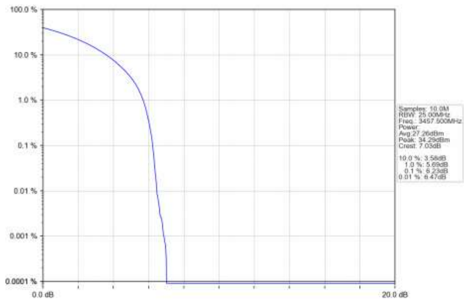
n77d 15kHz SISO NTN 15MHz CP-OFDM 16 QAM 3457.5MHz Outer Full Ant1
