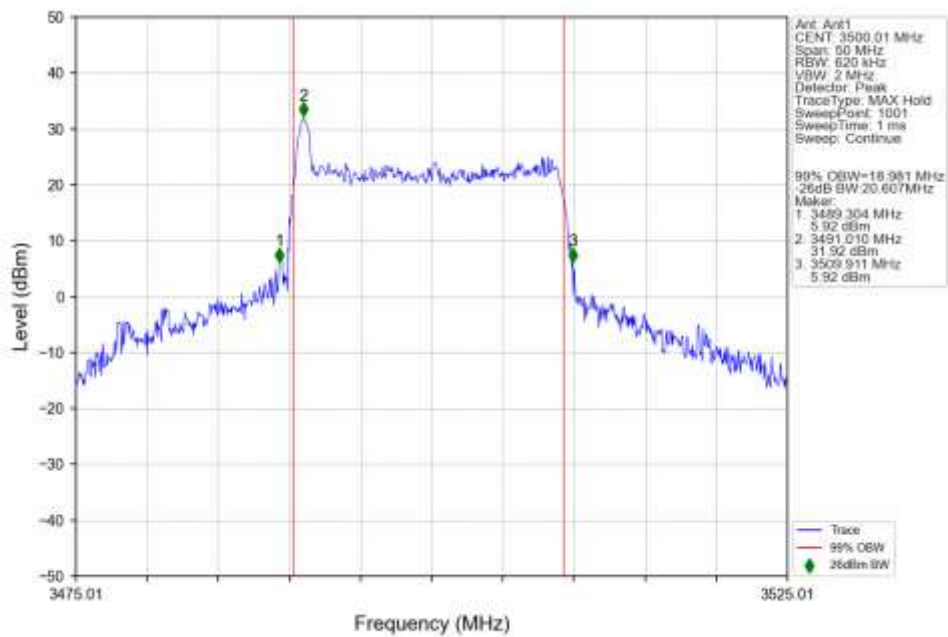
n77d 30kHz SISO NTN 20MHz CP-OFDM QPSK 3500.01MHz Outer Full Ant1
