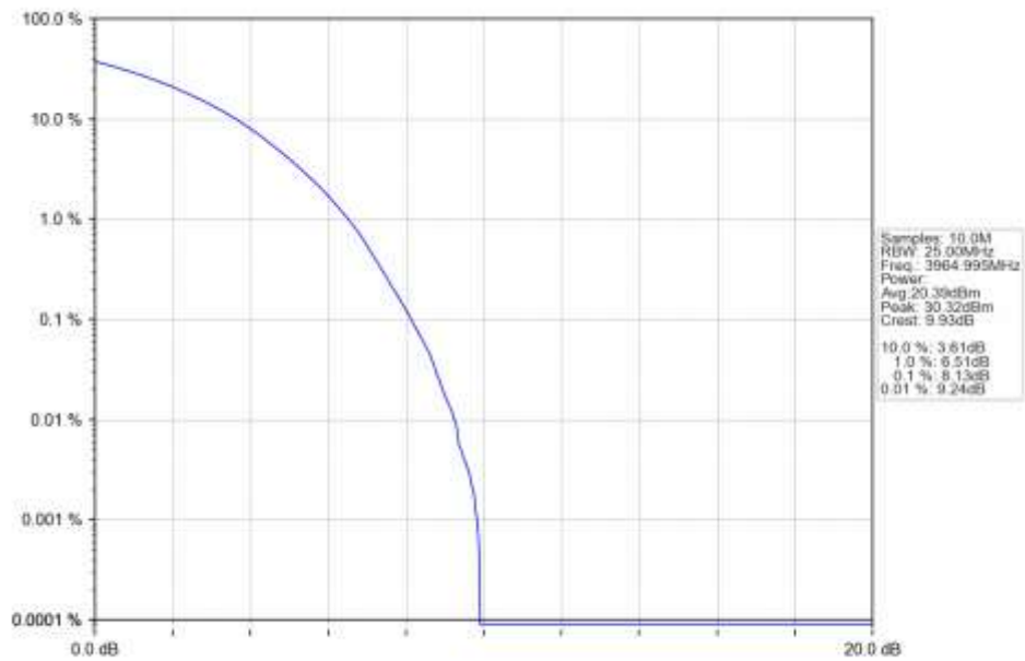
n77a 15kHz SISO NTN 30MHz CP-OFDM 256 QAM 3964.995MHz Outer Full Ant1
