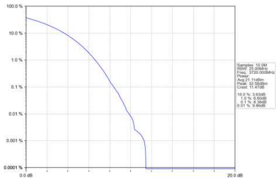
n77a 15kHz SISO NTN 40MHz CP-OFDM 256 QAM 3720MHz Outer Full Ant1
