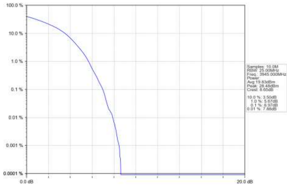
n77a 30kHz SISO NTN 70MHz DFT-s-OFDM QPSK 3945MHz Outer Full Ant1
