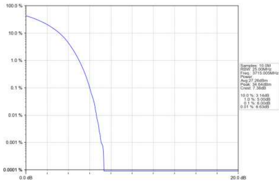
n77a 15kHz SISO NTN 30MHz DFT-s-OFDM 16 QAM 3715.005MHz Outer Full Ant1
