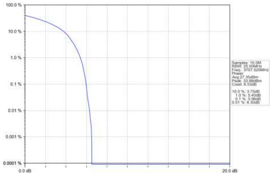
n77a 30kHz SISO NTN 15MHz CP-OFDM QPSK 3707.52MHz Outer Full Ant1
