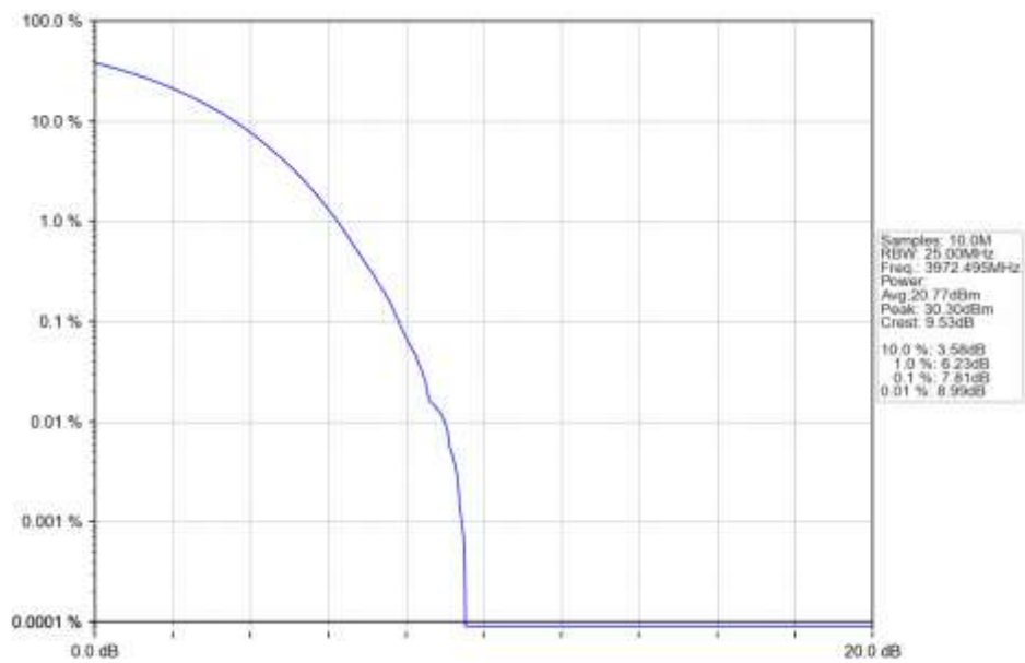
n77a 15kHz SISO NTN 15MHz CP-OFDM 256 QAM 3972.495MHz Outer Full Ant1
