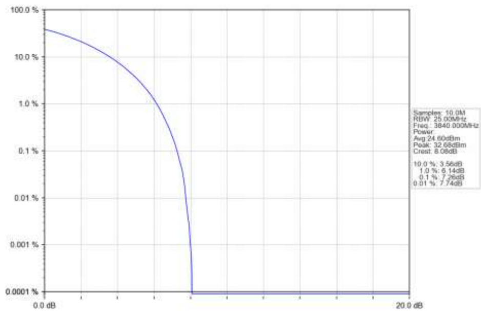
n77a 15kHz SISO NTN 20MHz CP-OFDM QPSK 3840MHz Outer Full Ant1
