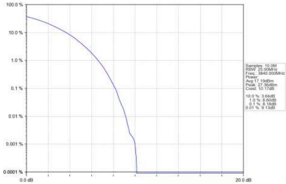
n77a 30kHz SISO NTN 70MHz CP-OFDM 256 QAM 3840MHz Outer Full Ant1
