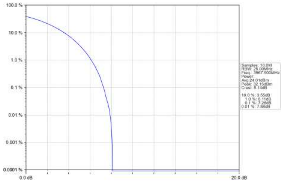
n77a 15kHz SISO NTN 25MHz CP-OFDM 16 QAM 3967.5MHz Outer Full Ant1
