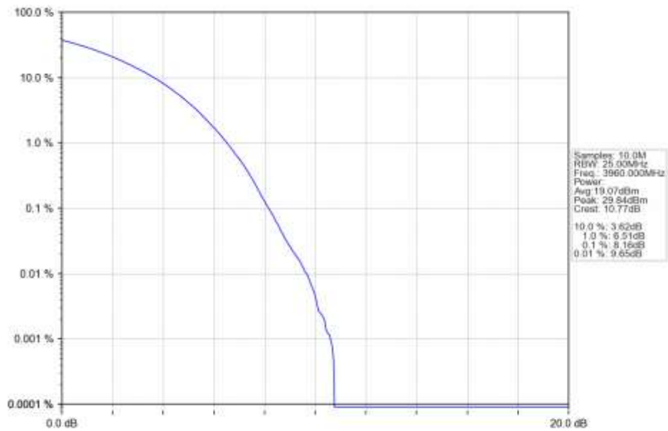
n77a 15kHz SISO NTN 40MHz CP-OFDM 256 QAM 3960MHz Outer Full Ant1
