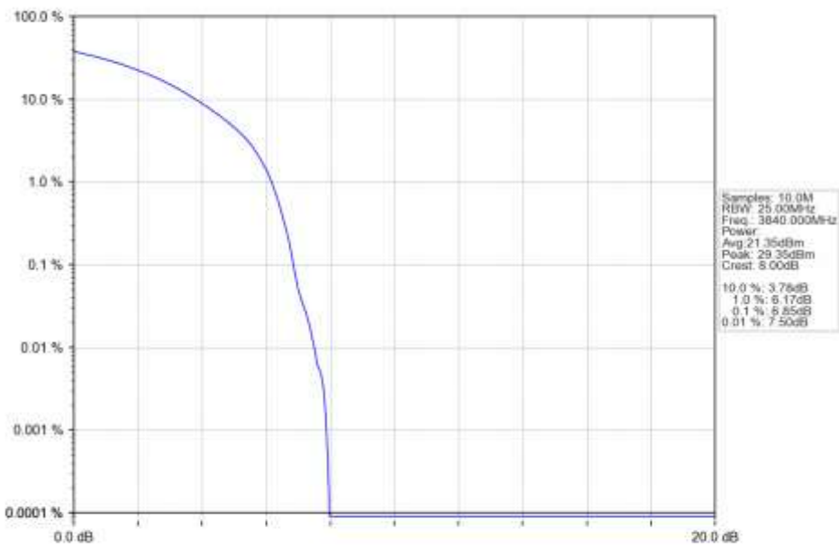
n77a_30kHz_SISO_NTNV_60MHz_DFT-s-OFDM QPSK_3840MHz_Outer_Full_Ant1
