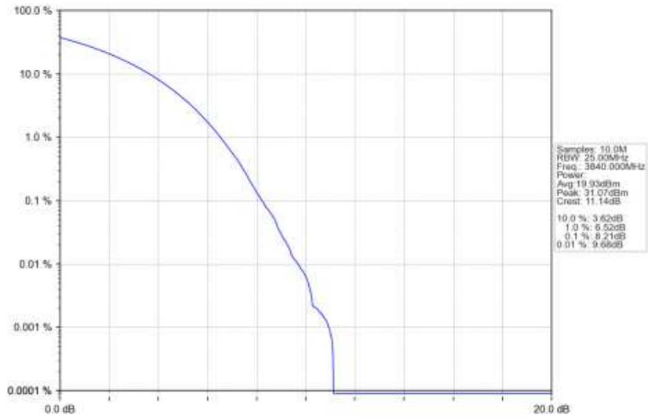
n77a 15kHz SISO NTN 40MHz CP-OFDM 256 QAM 3840MHz Outer Full Ant1
