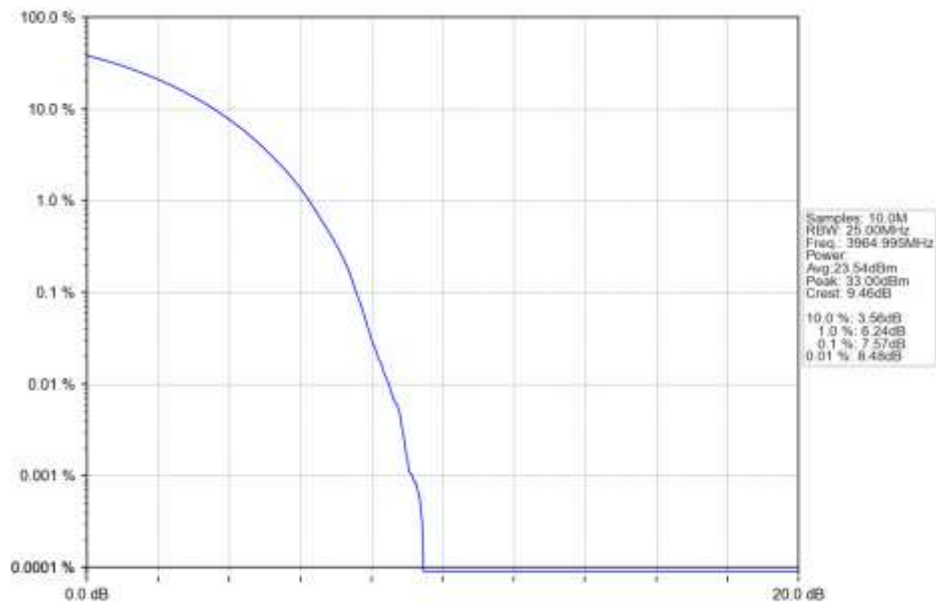
n77a 15kHz SISO NTN 30MHz CP-OFDM QPSK 3964.995MHz Outer Full Ant1
