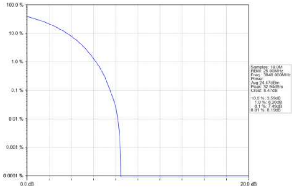
n77a 15kHz SISO NTN 25MHz CP-OFDM 16 QAM 3840MHz Outer Full Ant1
