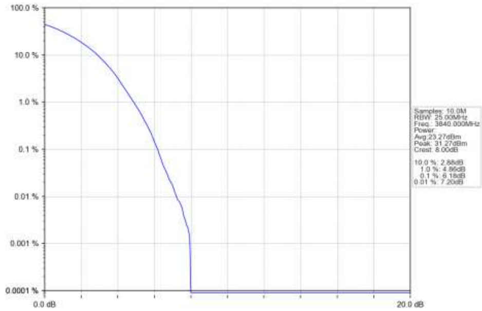
n77a 15kHz SISO NTN 20MHz DFT-s-OFDM 256 QAM 3840MHz Outer Full Ant1
