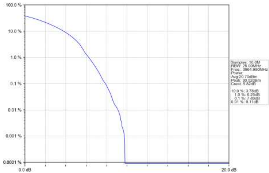
n77a 30kHz SISO NTN 30MHz CP-OFDM 256 QAM 3964.98MHz Outer Full Ant1
