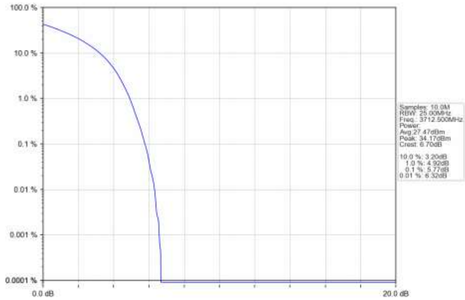
n77a 15kHz SISO NTN 25MHz DFT-s-OFDM 64 QAM 3712.5MHz Outer Full Ant1
