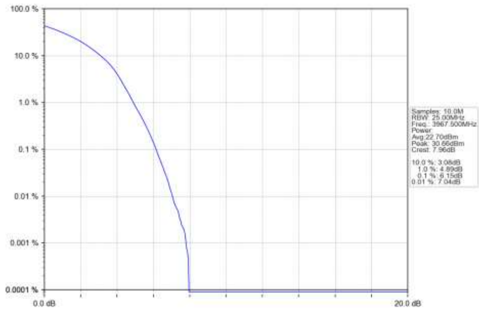
n77a 15kHz SISO NTN 25MHz DFT-s-OFDM 256 QAM 3967.5MHz Outer Full Ant1
