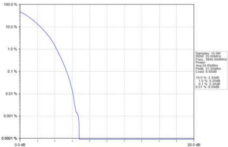
n77a_15kHz_SISO_NTNV_20MHz_DFT-s-OFDM QPSK_3840MHz_Outer_Full_Ant1
