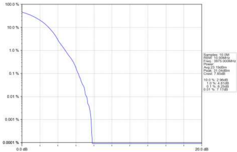
n77a 30kHz SISO NTN 10MHz DFT-s-OFDM 256 QAM 3975MHz Outer Full Ant1
