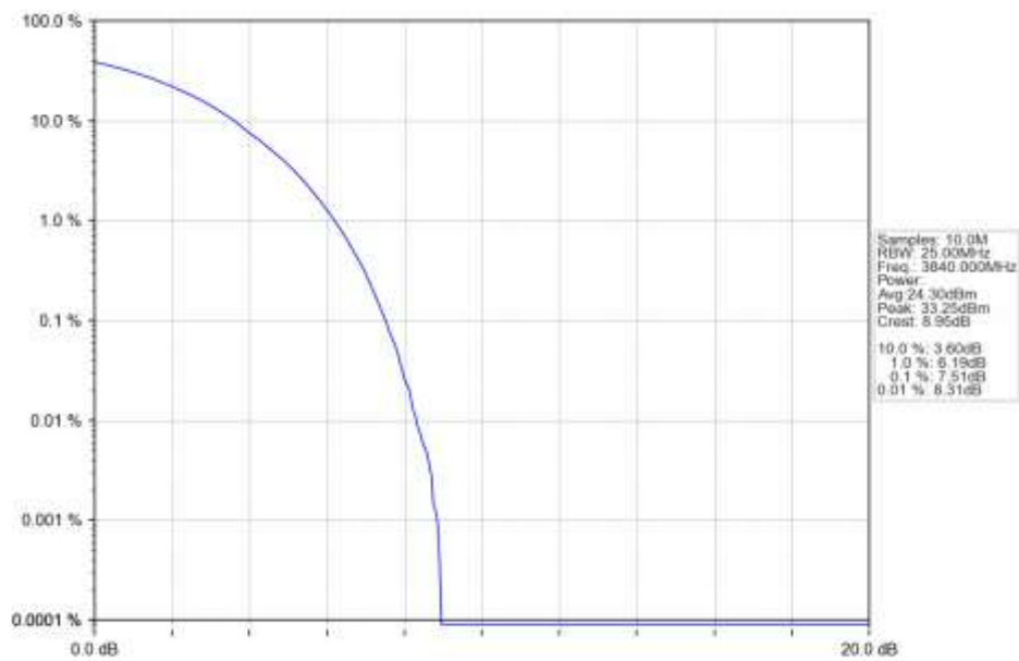
n77a 30kHz SISO NTN 25MHz CP-OFDM 64 QAM 3840MHz Outer Full Ant1
