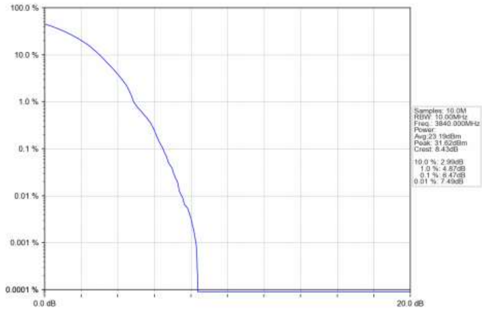
n77a 30kHz SISO NTN 10MHz DFT-s-OFDM 256 QAM 3840MHz Outer Full Ant1
