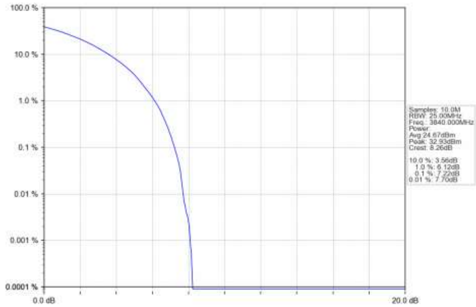
n77a 15kHz SISO NTN 20MHz CP-OFDM 16 QAM 3840MHz Outer Full Ant1
