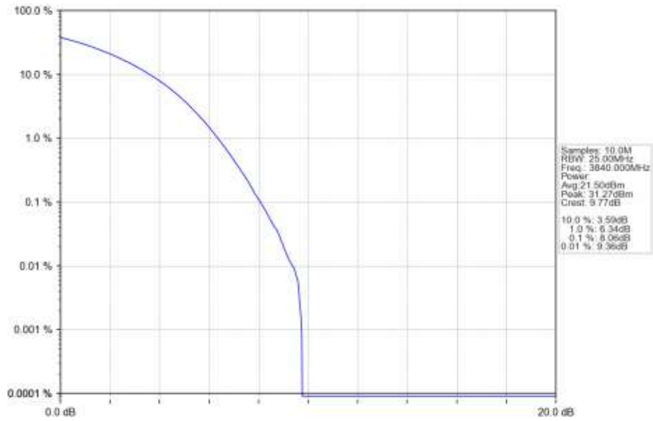
n77a 15kHz SISO NTN 20MHz CP-OFDM 256 QAM 3840MHz Outer Full Ant1
