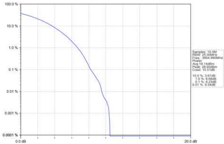
n77a 30kHz SISO NTN 50MHz CP-OFDM 256 QAM 3954.99MHz Outer Full Ant1
