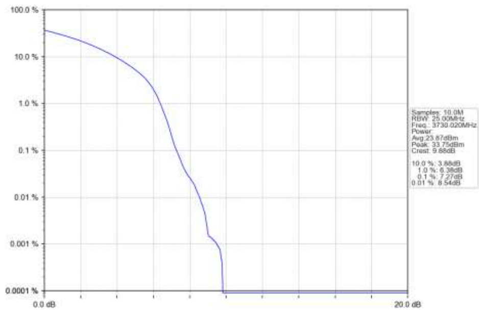
n77a 30kHz SISO NTN 60MHz DFT-s-OFDM 16 QAM 3730.02MHz Outer Full Ant1
