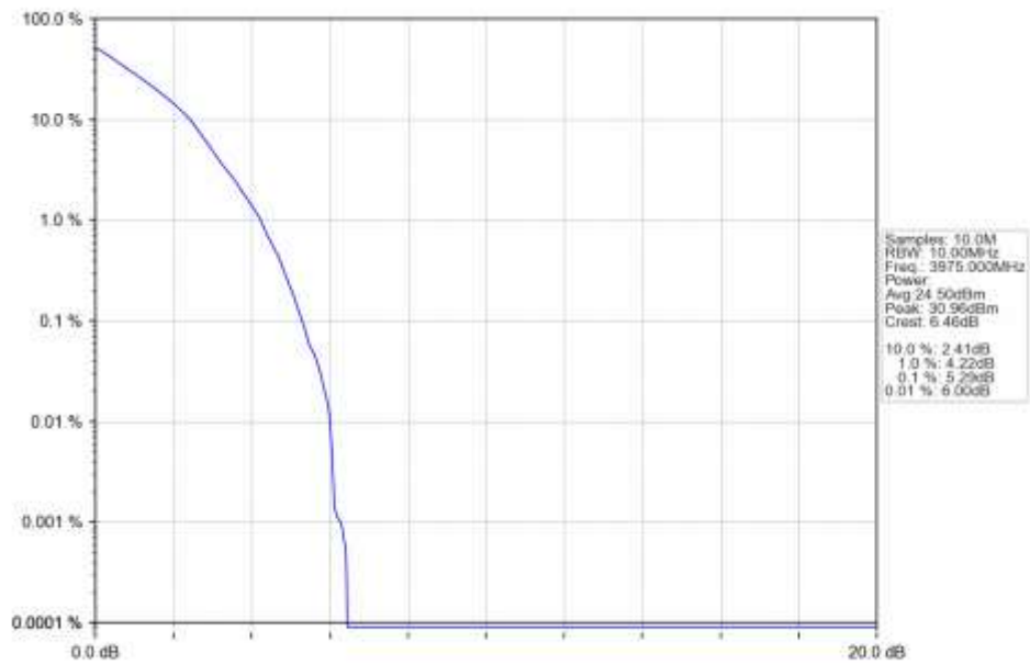
n77a 30kHz SISO NTN 10MHz DFT-s-OFDM QPSK 3975MHz Outer Full Ant1
