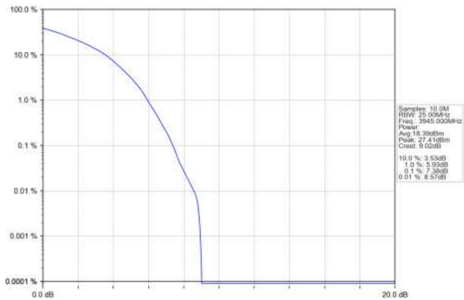
n77a 30kHz SISO NTN 70MHz DFT-s-OFDM 256 QAM 3945MHz Outer Full Ant1
