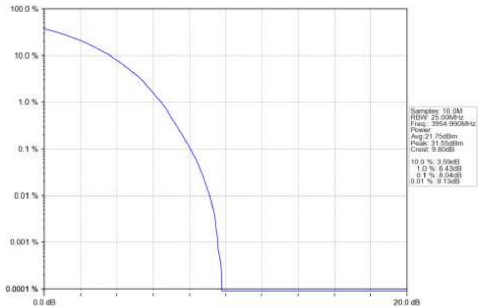
n77a 15kHz SISO NTN 50MHz CP-OFDM QPSK 3954.99MHz Outer Full Ant1
