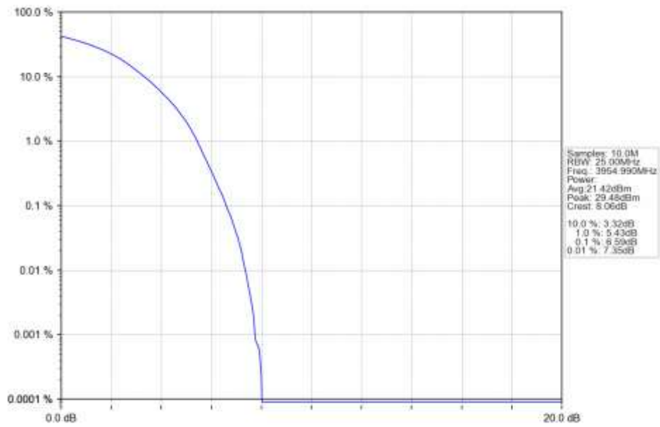
n77a 15kHz SISO NTN 50MHz DFT-s-OFDM QPSK 3954.99MHz Outer Full Ant1
