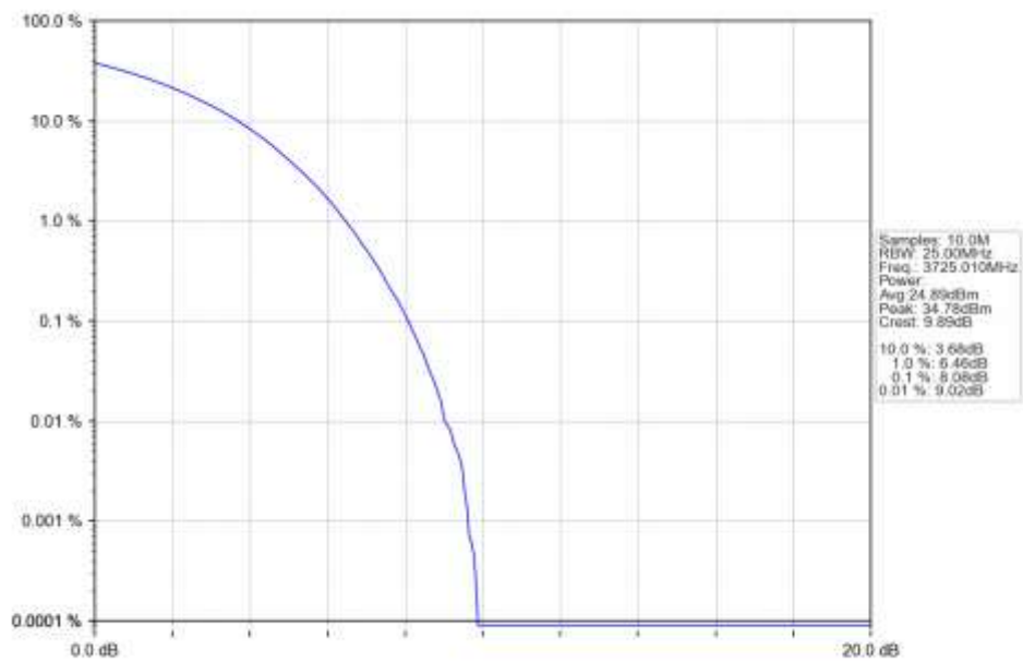
n77a 30kHz SISO NTN 50MHz CP-OFDM 16 QAM 3725.01MHz Outer Full Ant1
