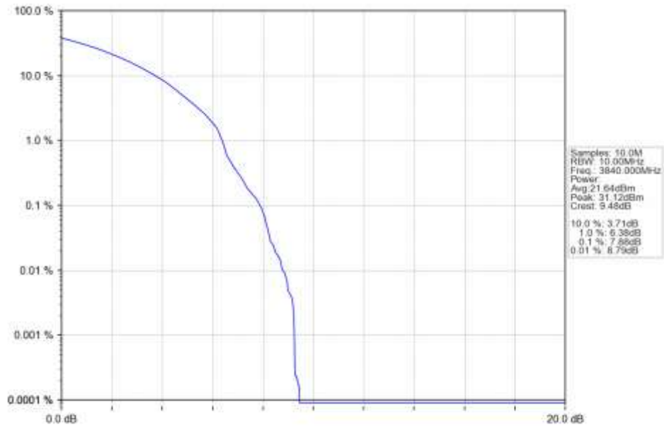
n77a 30kHz SISO NTN 10MHz CP-OFDM 256 QAM 3840MHz Outer Full Ant1
