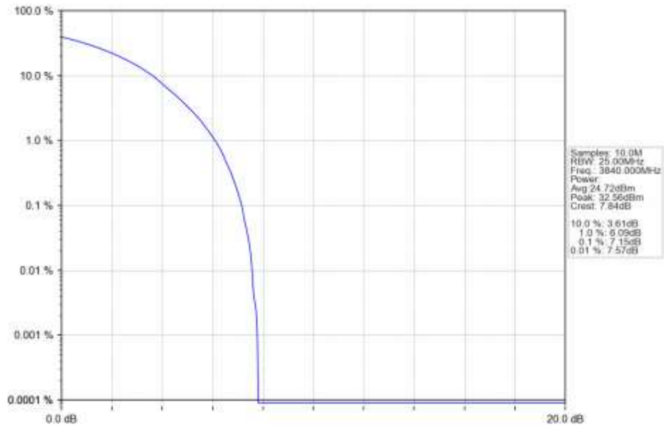
n77a 30kHz SISO NTN 15MHz CP-OFDM 16 QAM 3840MHz Outer Full Ant1
