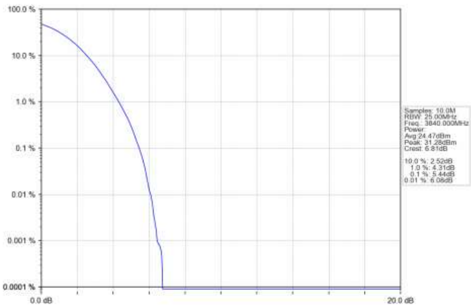
n77a_30kHz_SISO_NTNV_30MHz_DFT-s-OFDM QPSK_3840MHz_Outer_Full_Ant1
