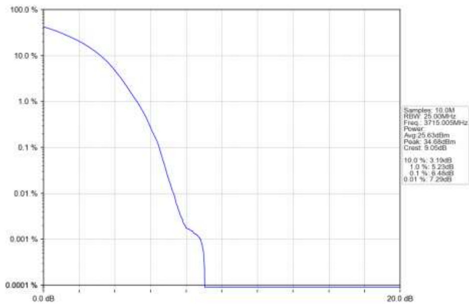
n77a 15kHz SISO NTN 30MHz DFT-s-OFDM 256 QAM 3715.005MHz Outer Full Ant1
