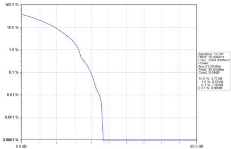
n77a 30kHz SISO NTN 20MHz CP-OFDM 256 QAM 3969.99MHz Outer Full Ant1
