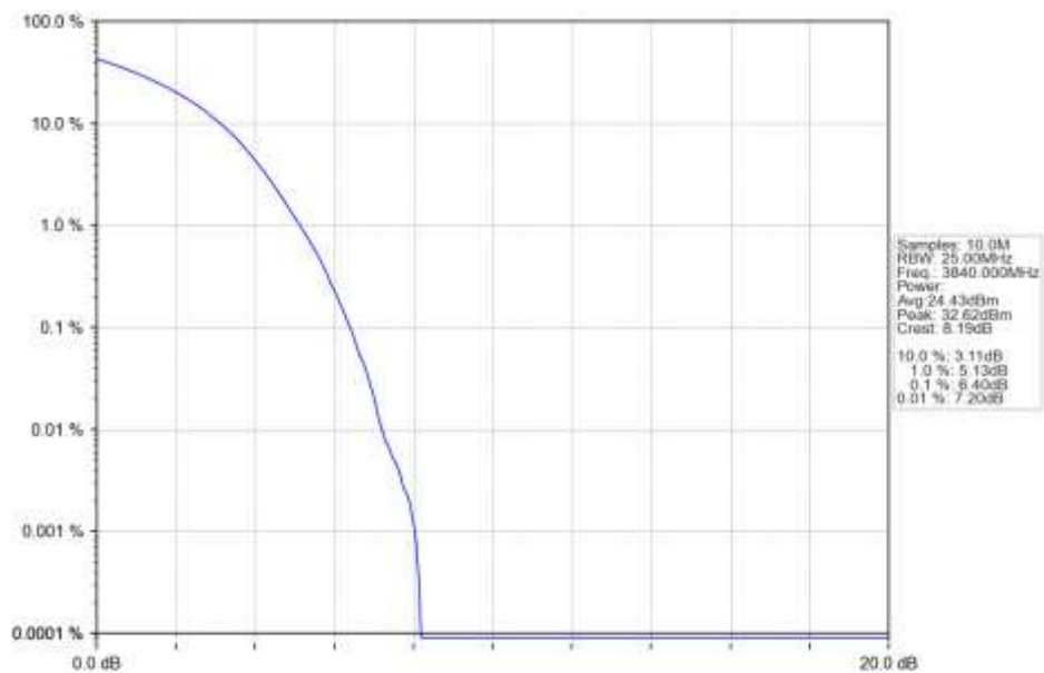
n77a 15kHz SISO NTN 30MHz DFT-s-OFDM 64 QAM 3840MHz Outer Full Ant1
