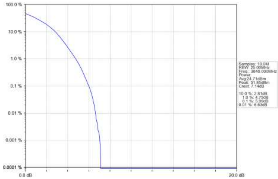
n77a 15kHz SISO NTN 20MHz DFT-s-OFDM 16 QAM 3840MHz Outer Full Ant1
