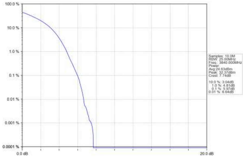
n77a 15kHz SISO NTN 25MHz DFT-s-OFDM 16 QAM 3840MHz Outer Full Ant1
