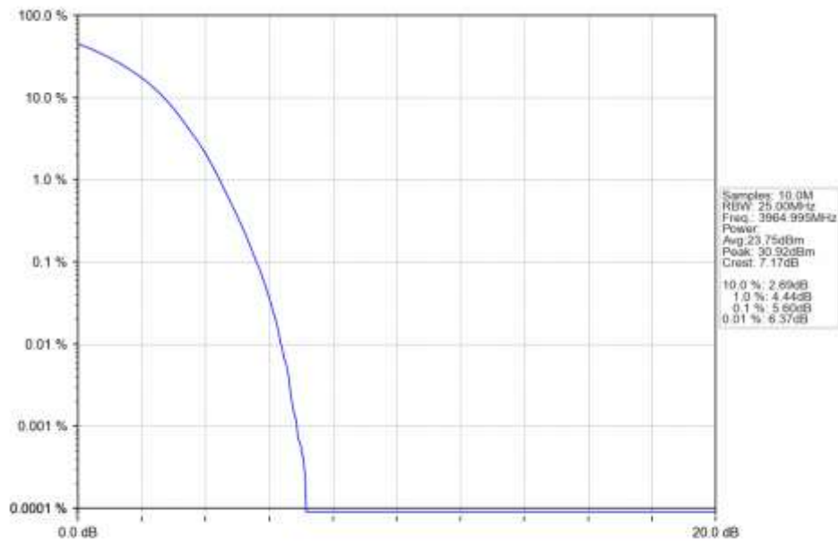
n77a 15kHz SISO NTN 30MHz DFT-s-OFDM QPSK 3964.995MHz Outer Full Ant1
