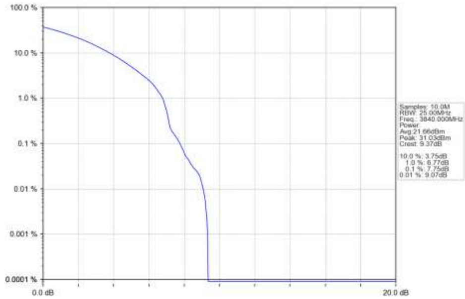
n77a 30kHz SISO NTN 15MHz CP-OFDM 256 QAM 3840MHz Outer Full Ant1
