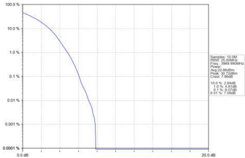
n77a 15kHz SISO NTN 20MHz DFT-s-OFDM 256 QAM 3969.99MHz Outer Full Ant1
