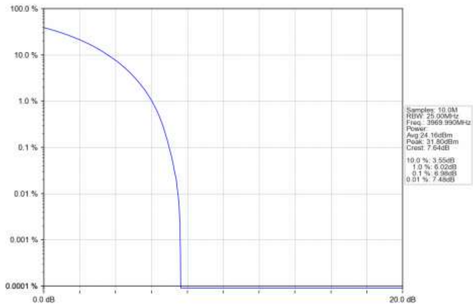
n77a 15kHz SISO NTN 20MHz CP-OFDM QPSK 3969.99MHz Outer Full Ant1
