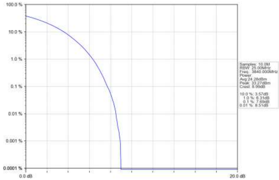
n77a 15kHz SISO NTN 30MHz CP-OFDM 16 QAM 3840MHz Outer Full Ant1
