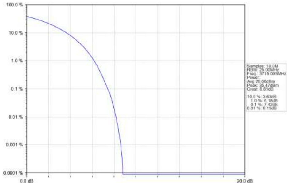
n77a 15kHz SISO NTN 30MHz CP-OFDM 64 QAM 3715.005MHz Outer Full Ant1
