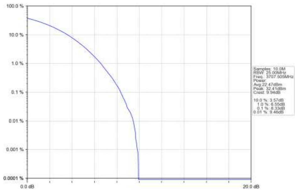
n77a 15kHz SISO NTN 15MHz CP-OFDM 256 QAM 3707.505MHz Outer Full Ant1
