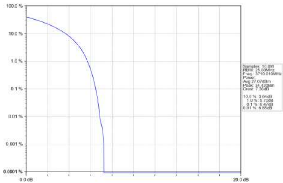
n77a 15kHz SISO NTN 20MHz CP-OFDM 16 QAM 3710.01MHz Outer Full Ant1
