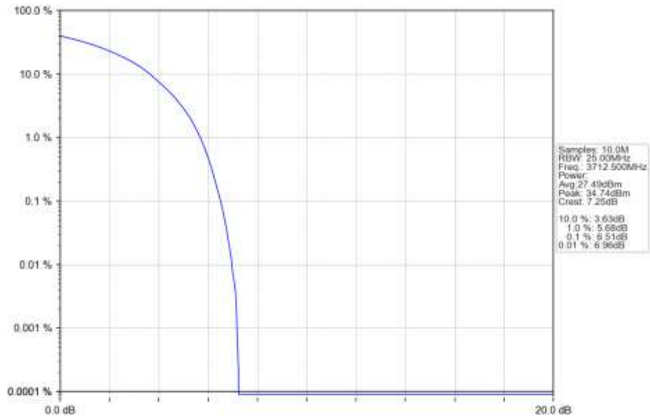
n77a 30kHz SISO NTN 25MHz CP-OFDM QPSK 3712.5MHz Outer Full Ant1
