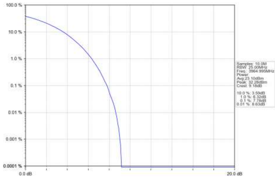
n77a 15kHz SISO NTN 30MHz CP-OFDM 64 QAM 3964.995MHz Outer Full Ant1
