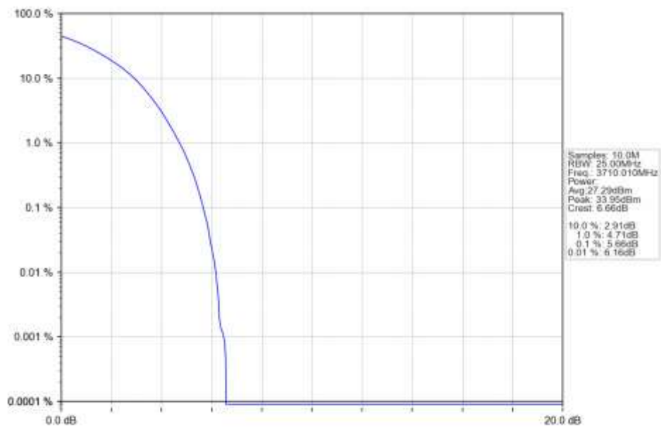
n77a 15kHz SISO NTN 20MHz DFT-s-OFDM 16 QAM 3710.01MHz Outer Full Ant1
