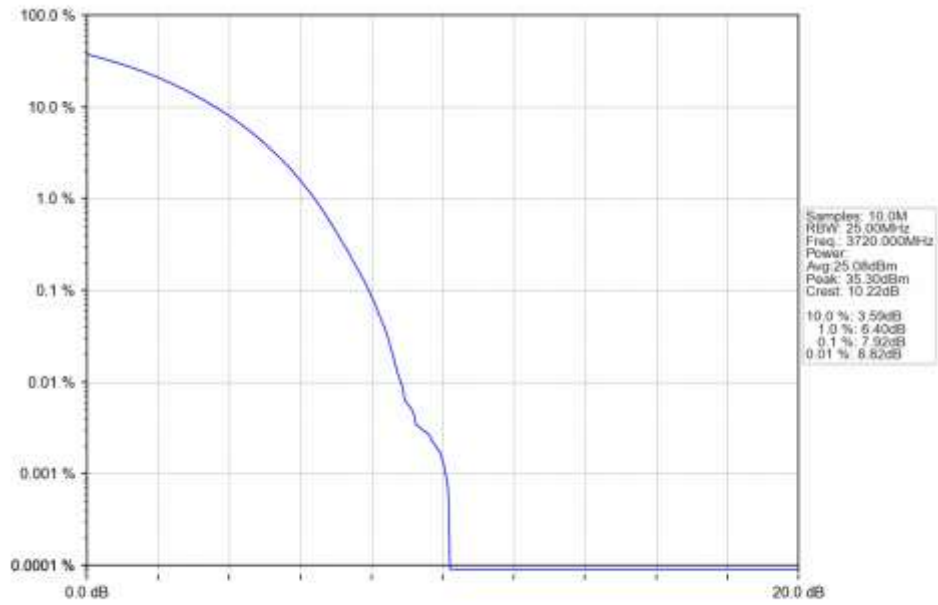
n77a 15kHz SISO NTN 40MHz CP-OFDM 64 QAM 3720MHz Outer Full Ant1
