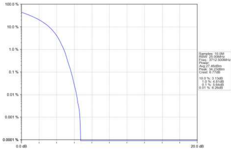
n77a 15kHz SISO NTN 25MHz DFT-s-OFDM 16 QAM 3712.5MHz Outer Full Ant1
