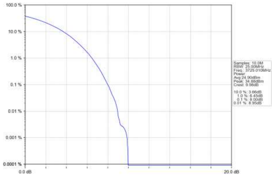
n77a 30kHz SISO NTN 50MHz CP-OFDM QPSK 3725.01MHz Outer Full Ant1
