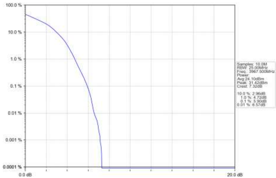
n77a 15kHz SISO NTN 25MHz DFT-s-OFDM 16 QAM 3967.5MHz Outer Full Ant1
