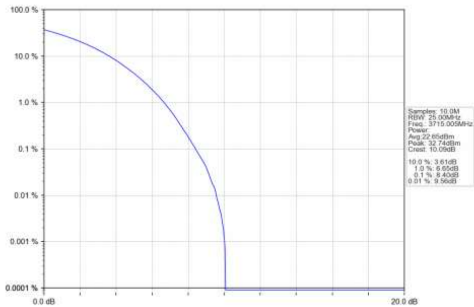
n77a 15kHz SISO NTN 30MHz CP-OFDM 256 QAM 3715.005MHz Outer Full Ant1
