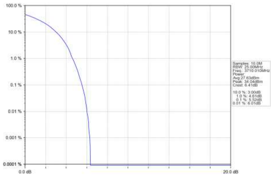
n77a 30kHz SISO NTN 20MHz DFT-s-OFDM 16 QAM 3710.01MHz Outer Full Ant1
