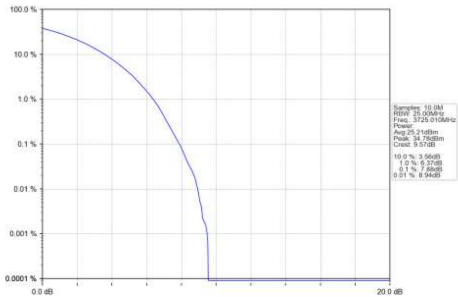
n77a 15kHz SISO NTN 50MHz CP-OFDM 16 QAM 3725.01MHz Outer Full Ant1
