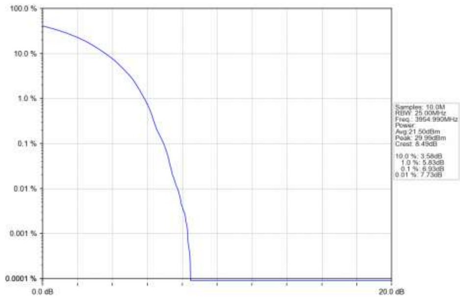
n77a 30kHz SISO NTN 50MHz DFT-s-OFDM QPSK 3954.99MHz Outer Full Ant1
