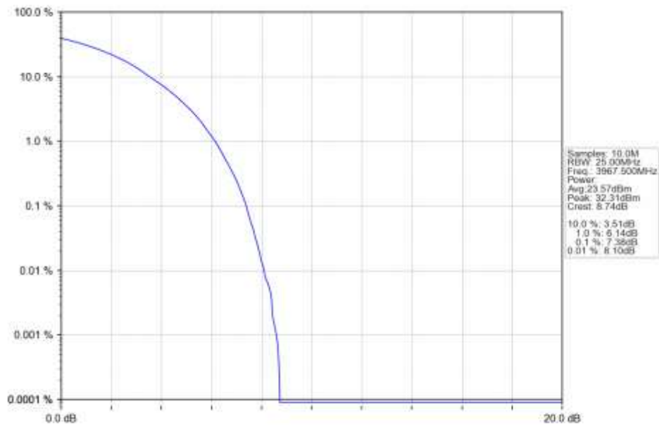
n77a 30kHz SISO NTN 25MHz CP-OFDM 64 QAM 3967.5MHz Outer Full Ant1
