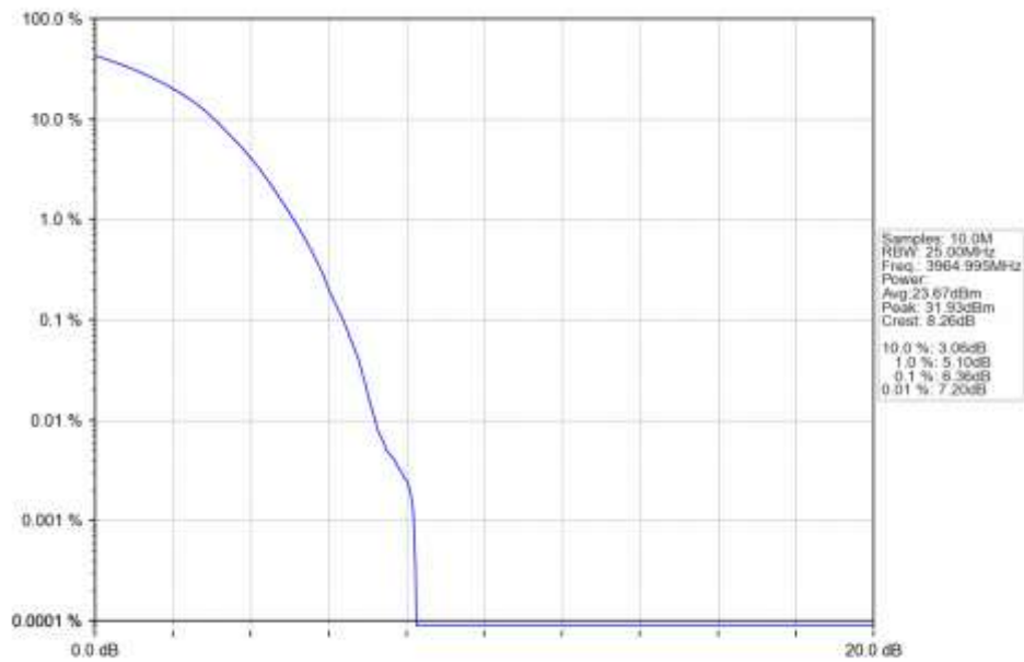
n77a 15kHz SISO NTN 30MHz DFT-s-OFDM 64 QAM 3964.995MHz Outer Full Ant1
