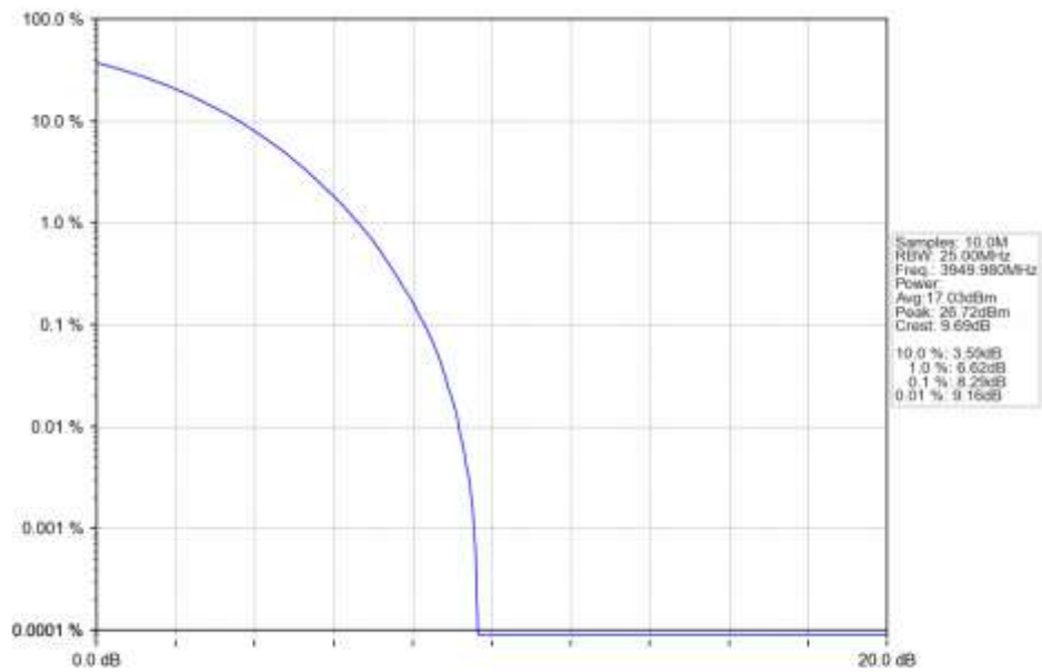
n77a 30kHz SISO NTN 60MHz CP-OFDM 256 QAM 3949.98MHz Outer Full Ant1
