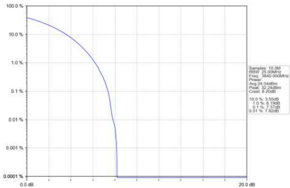
n77a 15kHz SISO NTN 15MHz CP-OFDM 64 QAM 3840MHz Outer Full Ant1
