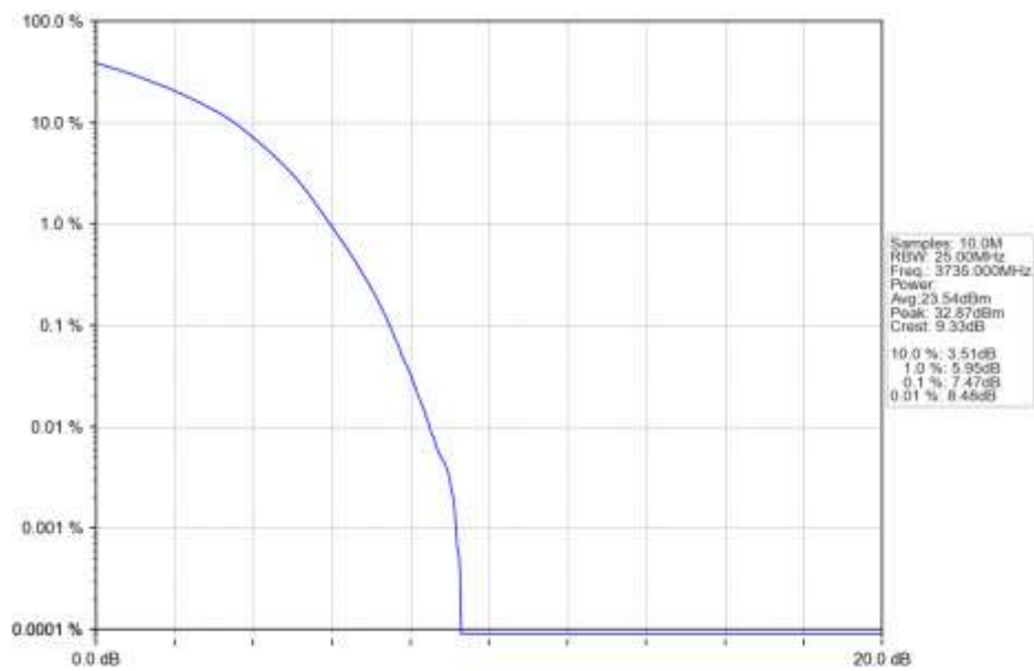
n77a 30kHz SISO NTN 70MHz DFT-s-OFDM 16 QAM 3735MHz Outer Full Ant1
