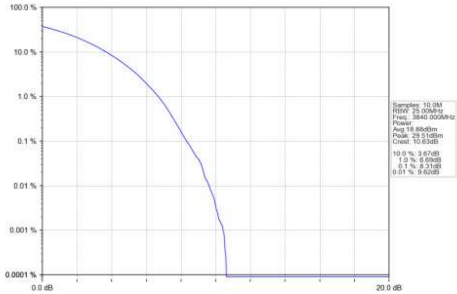
n77a 30kHz SISO NTN 50MHz CP-OFDM 256 QAM 3840MHz Outer Full Ant1
