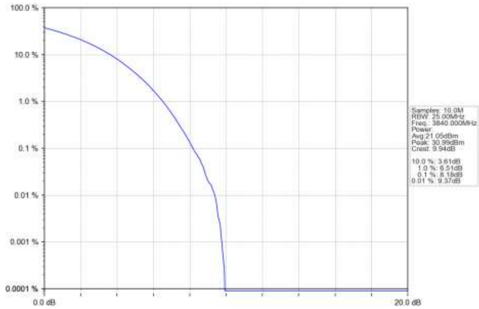
n77a 15kHz SISO NTN 30MHz CP-OFDM 256 QAM 3840MHz Outer Full Ant1
