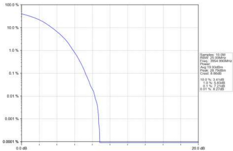
n77a 15kHz SISO NTN 50MHz DFT-s-OFDM 256 QAM 3954.99MHz Outer Full Ant1
