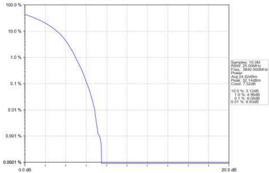
n77a 15kHz SISO NTN 25MHz DFT-s-OFDM 64 QAM 3840MHz Outer Full Ant1
