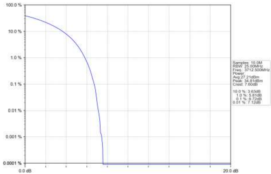
n77a 15kHz SISO NTN 25MHz CP-OFDM 16 QAM 3712.5MHz Outer Full Ant1
