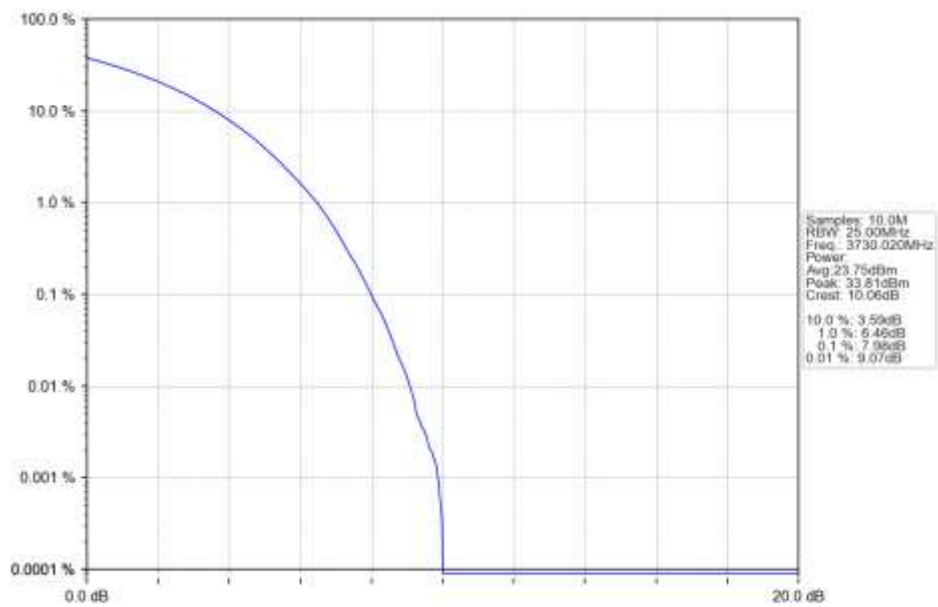
n77a 30kHz SISO NTN 60MHz CP-OFDM 16 QAM 3730.02MHz Outer Full Ant1
