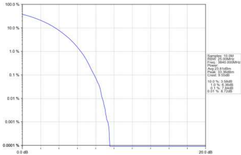
n77a 15kHz SISO NTN 30MHz CP-OFDM 64 QAM 3840MHz Outer Full Ant1
