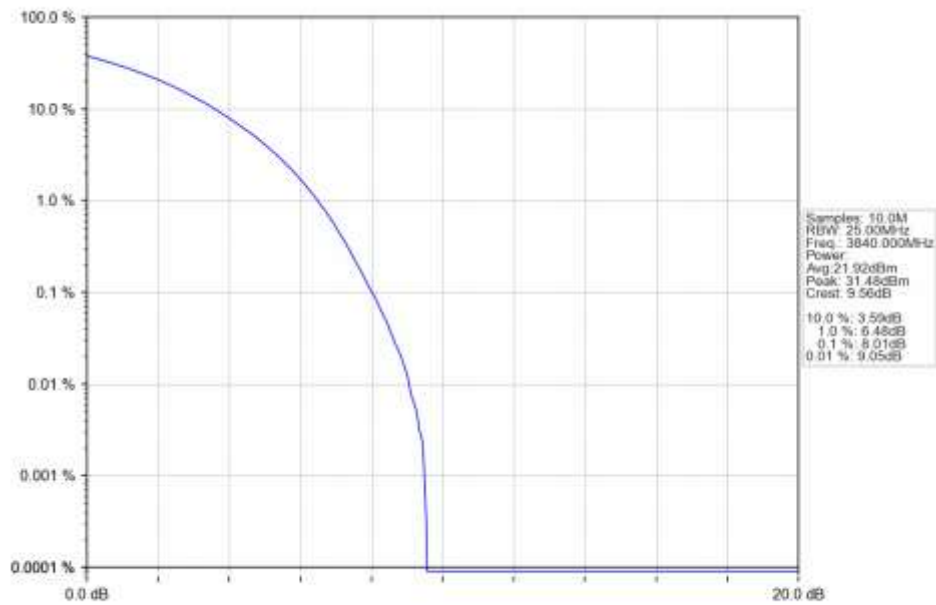
n77a 15kHz SISO NTN 50MHz CP-OFDM 64 QAM 3840MHz Outer Full Ant1
