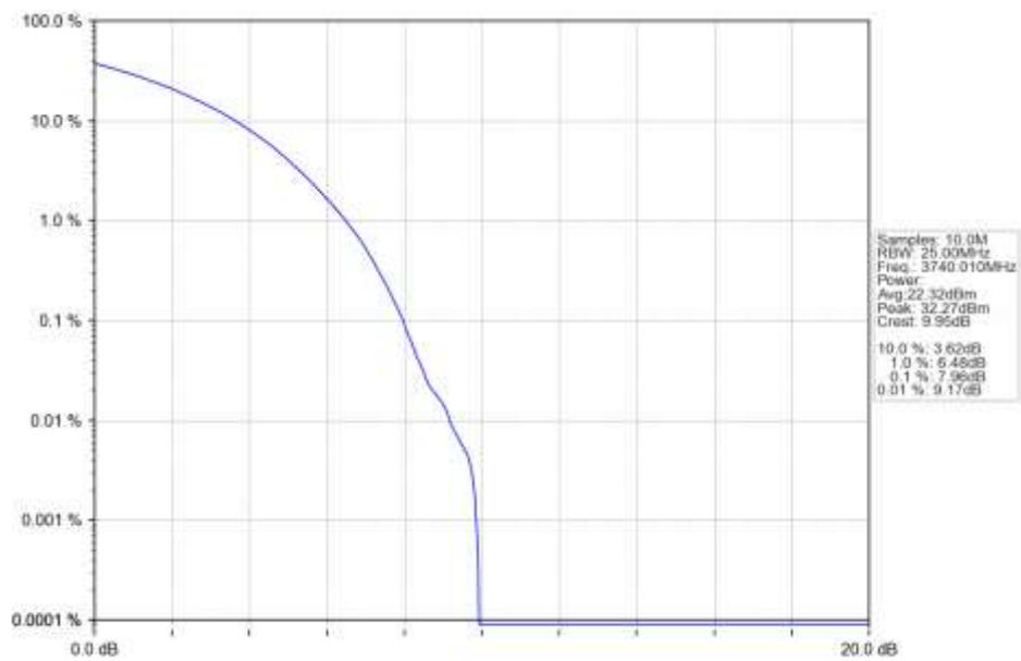
n77a 30kHz SISO NTN 80MHz CP-OFDM 16 QAM 3740.01MHz Outer Full Ant1
