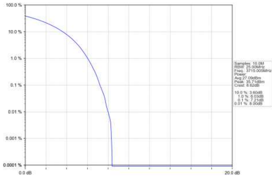
n77a 15kHz SISO NTN 30MHz CP-OFDM QPSK 3715.005MHz Outer Full Ant1
