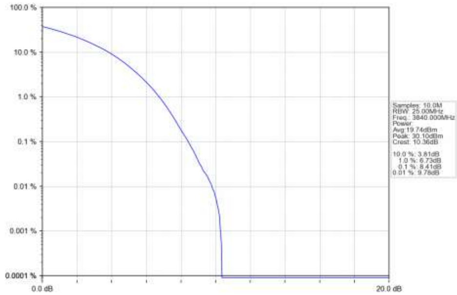
n77a 30kHz SISO NTN 40MHz CP-OFDM 256 QAM 3840MHz Outer Full Ant1
