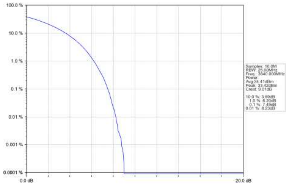
n77a 15kHz SISO NTN 25MHz CP-OFDM QPSK 3840MHz Outer Full Ant1
