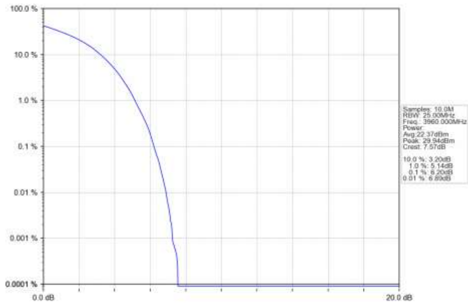
n77a 15kHz SISO NTN 40MHz DFT-s-OFDM QPSK 3960MHz Outer Full Ant1
