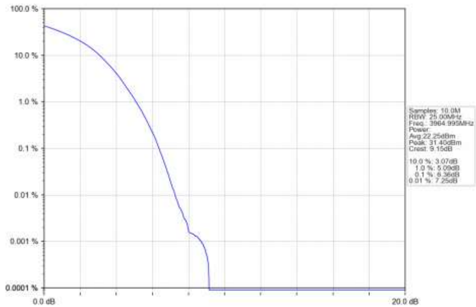
n77a 15kHz SISO NTN 30MHz DFT-s-OFDM 256 QAM 3964.995MHz Outer Full Ant1
