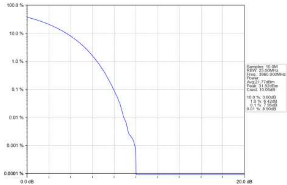
n77a 15kHz SISO NTN 40MHz CP-OFDM 64 QAM 3960MHz Outer Full Ant1
