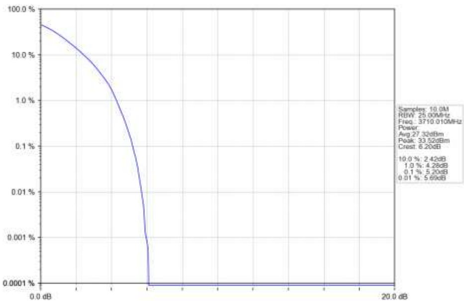
n77a_15kHz_SISO_NTNV_20MHz_DFT-s-OFDM QPSK_3710.01MHz_Outer_Full_Ant1
