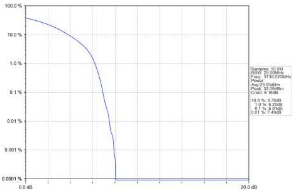
n77a_30kHz_SISO_NTNV_60MHz_DFT-s-OFDM QPSK_3730.02MHz_Outer_Full_Ant1
