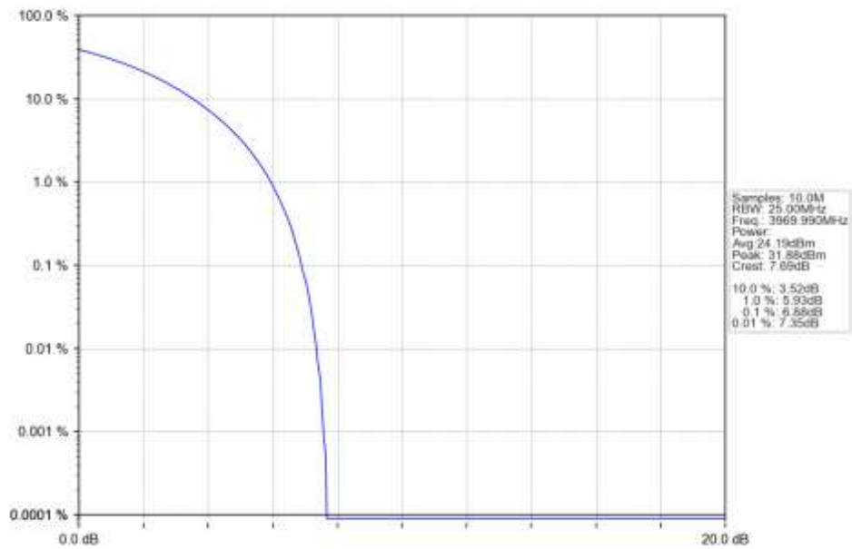
n77a 15kHz SISO NTN 20MHz CP-OFDM 16 QAM 3969.99MHz Outer Full Ant1
