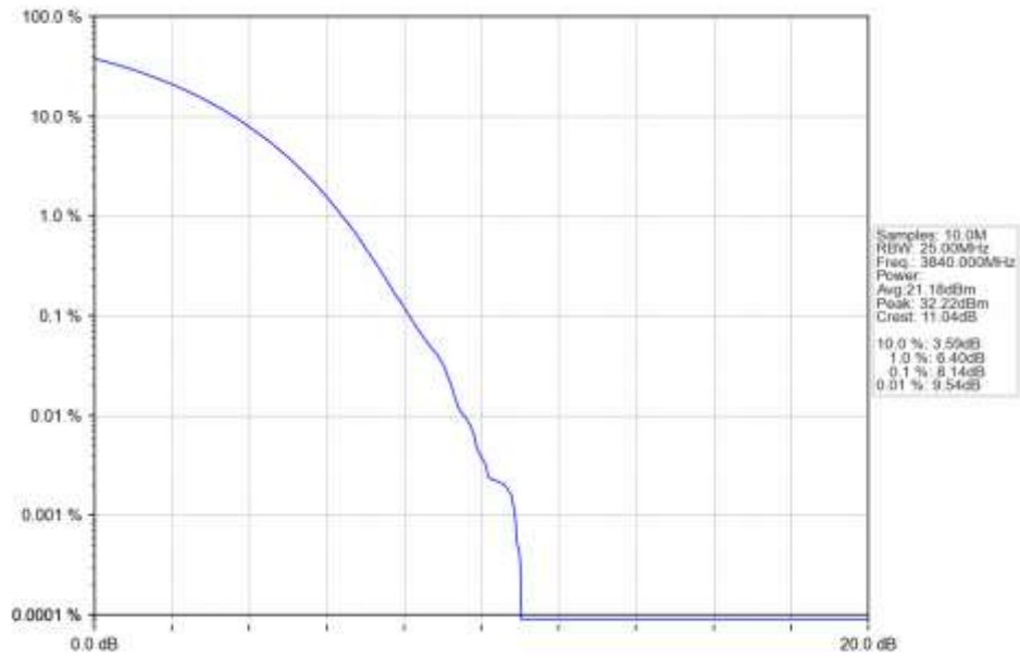
n77a 15kHz SISO NTN 25MHz CP-OFDM 256 QAM 3840MHz Outer Full Ant1
