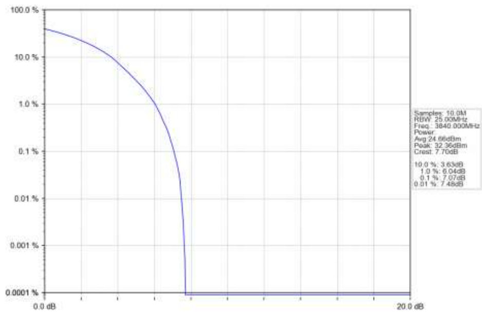
n77a 30kHz SISO NTN 15MHz CP-OFDM QPSK 3840MHz Outer Full Ant1
