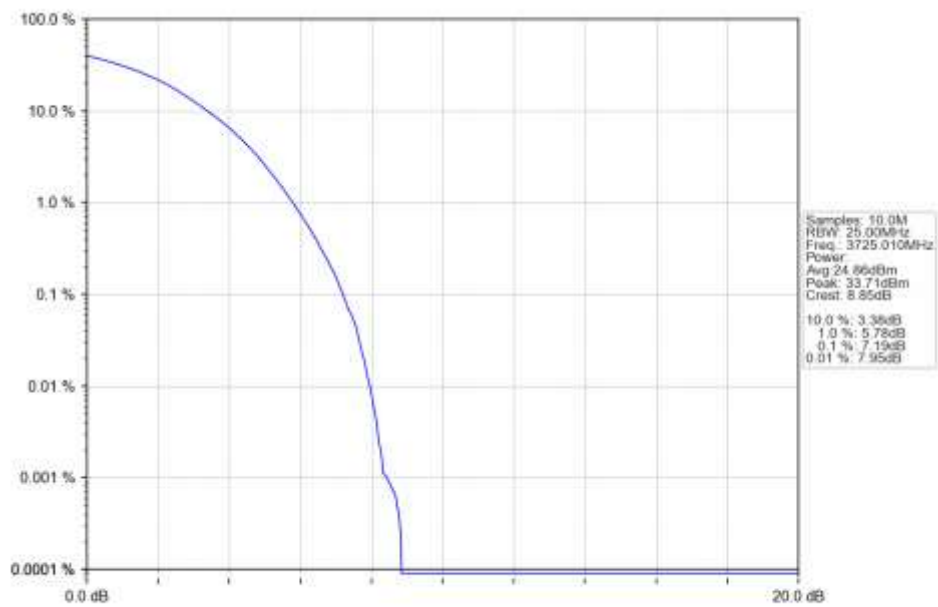
n77a 15kHz SISO NTN 50MHz DFT-s-OFDM 16 QAM 3725.01MHz Outer Full Ant1
