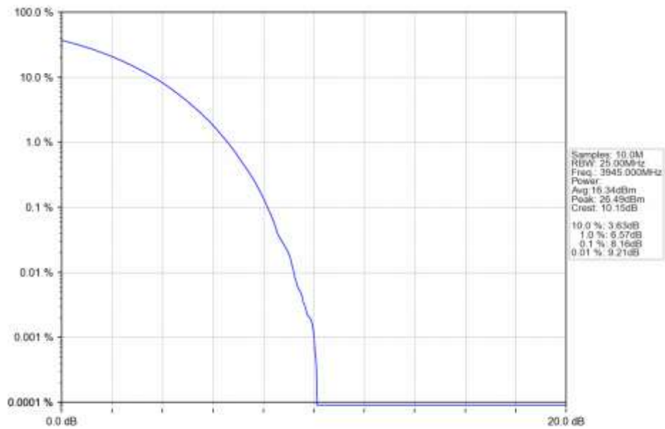
n77a 30kHz SISO NTN 70MHz CP-OFDM 256 QAM 3945MHz Outer Full Ant1
