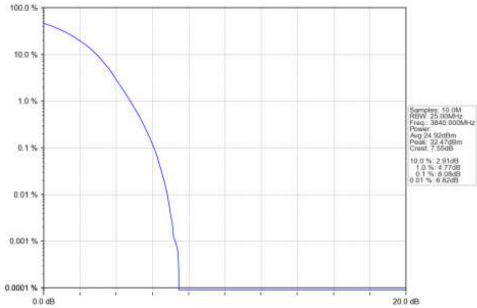
n77a 30kHz SISO NTN 25MHz DFT-s-OFDM 16 QAM 3840MHz Outer Full Ant1
