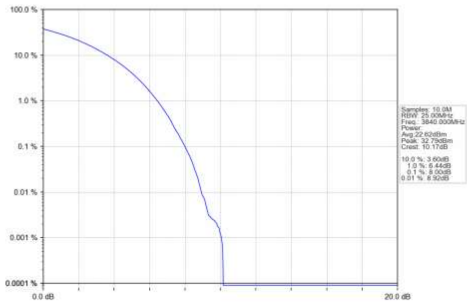
n77a 15kHz SISO NTN 40MHz CP-OFDM 64 QAM 3840MHz Outer Full Ant1
