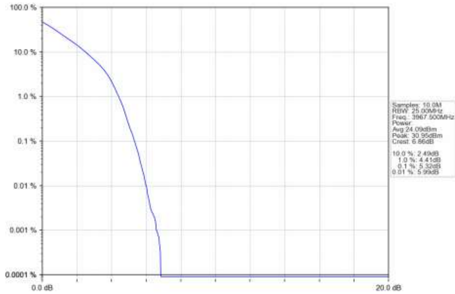
n77a 15kHz SISO NTN 25MHz DFT-s-OFDM QPSK 3967.5MHz Outer Full Ant1
