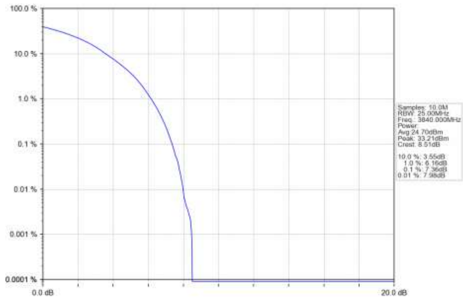
n77a 30kHz SISO NTN 25MHz CP-OFDM QPSK 3840MHz Outer Full Ant1
