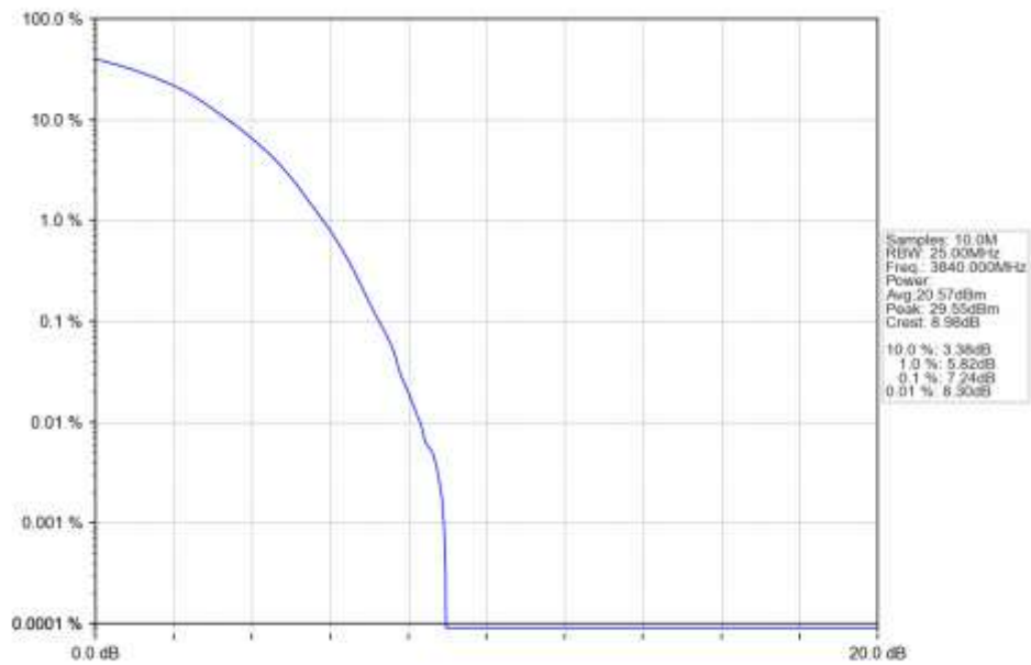
n77a 15kHz SISO NTN 50MHz DFT-s-OFDM 256 QAM 3840MHz Outer Full Ant1
