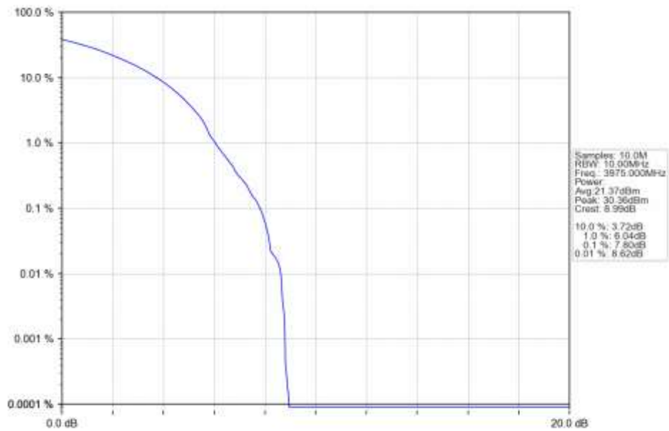
n77a 30kHz SISO NTN 10MHz CP-OFDM 256 QAM 3975MHz Outer Full Ant1
