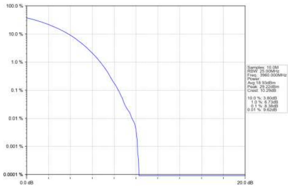
n77a 30kHz SISO NTN 40MHz CP-OFDM 256 QAM 3960MHz Outer Full Ant1
