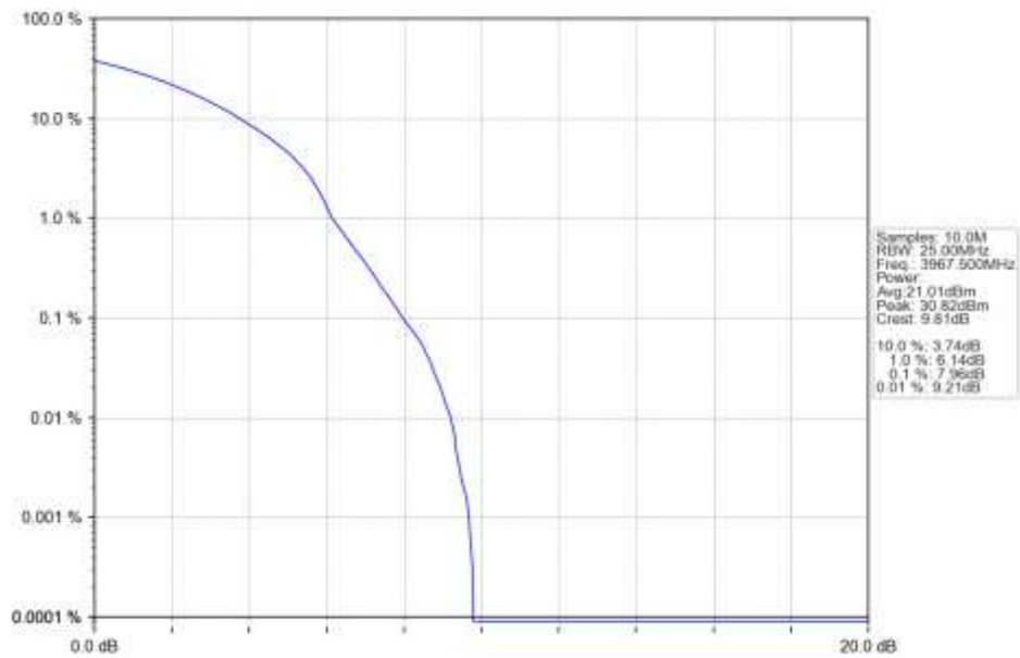
n77a 30kHz SISO NTN 25MHz CP-OFDM 256 QAM 3967.5MHz Outer Full Ant1
