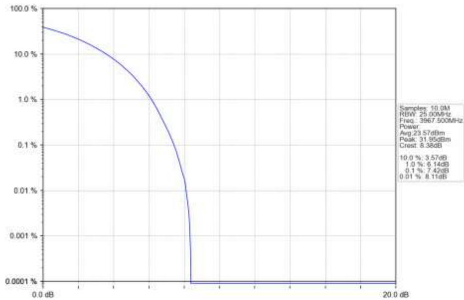
n77a 15kHz SISO NTN 25MHz CP-OFDM 64 QAM 3967.5MHz Outer Full Ant1
