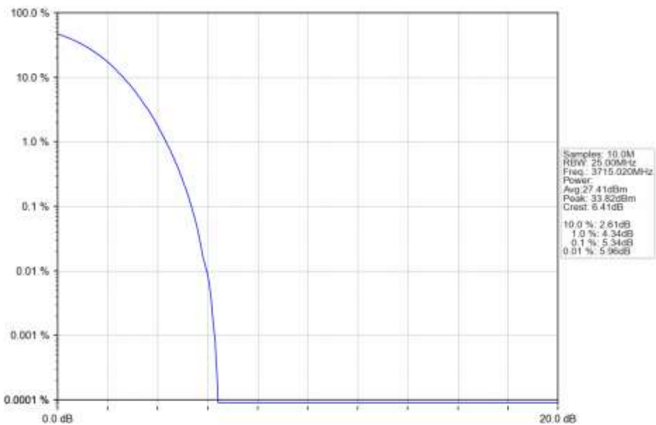
n77a_30kHz_SISO_NTNV_30MHz_DFT-s-OFDM QPSK_3715.02MHz_Outer_Full_Ant1
