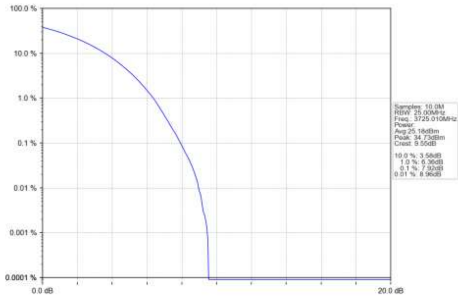
n77a 15kHz SISO NTN 50MHz CP-OFDM QPSK 3725.01MHz Outer Full Ant1
