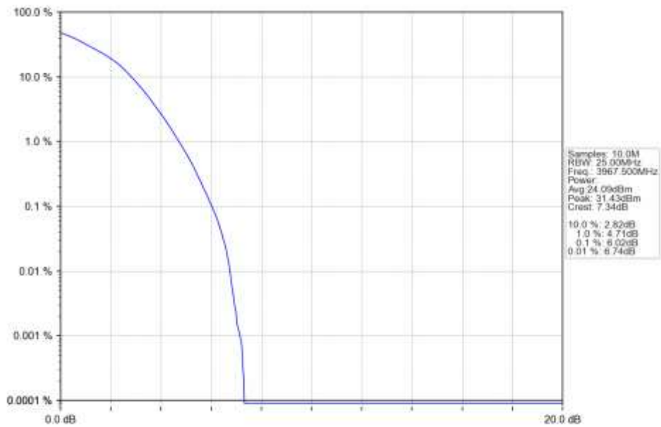
n77a 30kHz SISO NTN 25MHz DFT-s-OFDM 16 QAM 3967.5MHz Outer Full Ant1
