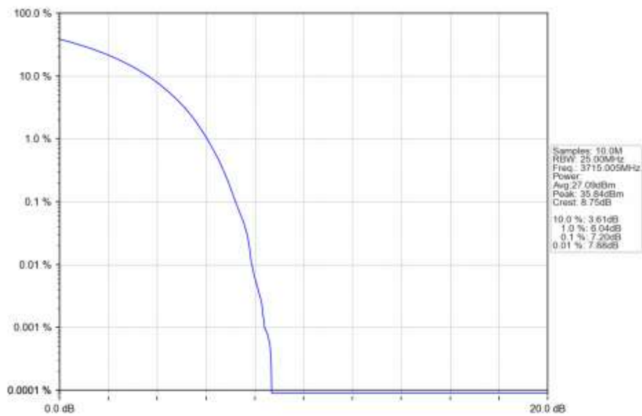
n77a 15kHz SISO NTN 30MHz CP-OFDM 16 QAM 3715.005MHz Outer Full Ant1
