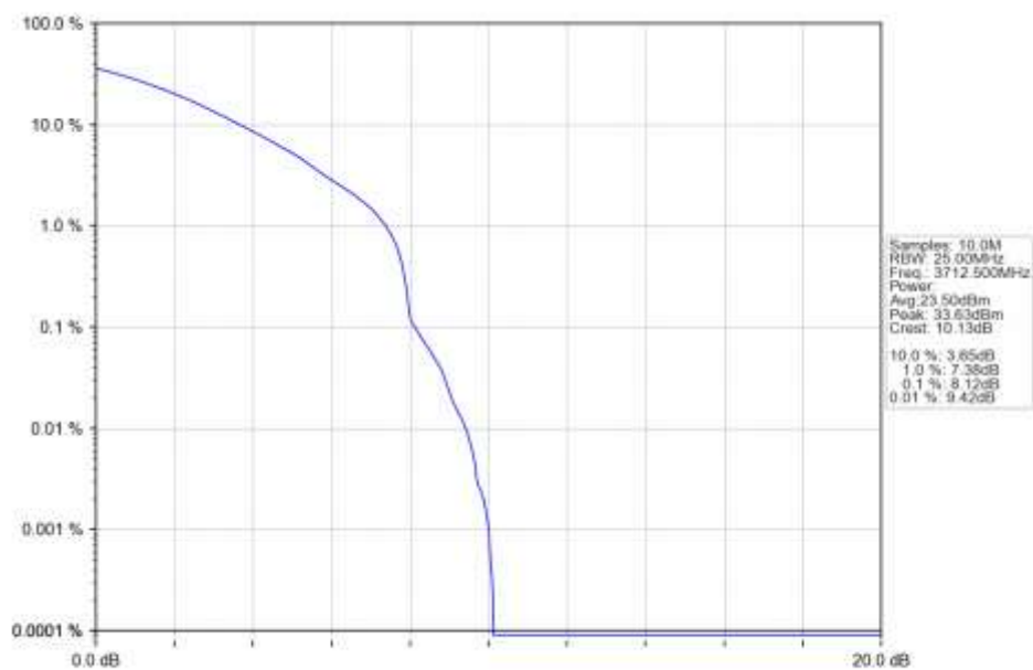
n77a 30kHz SISO NTN 25MHz CP-OFDM 256 QAM 3712.5MHz Outer Full Ant1
