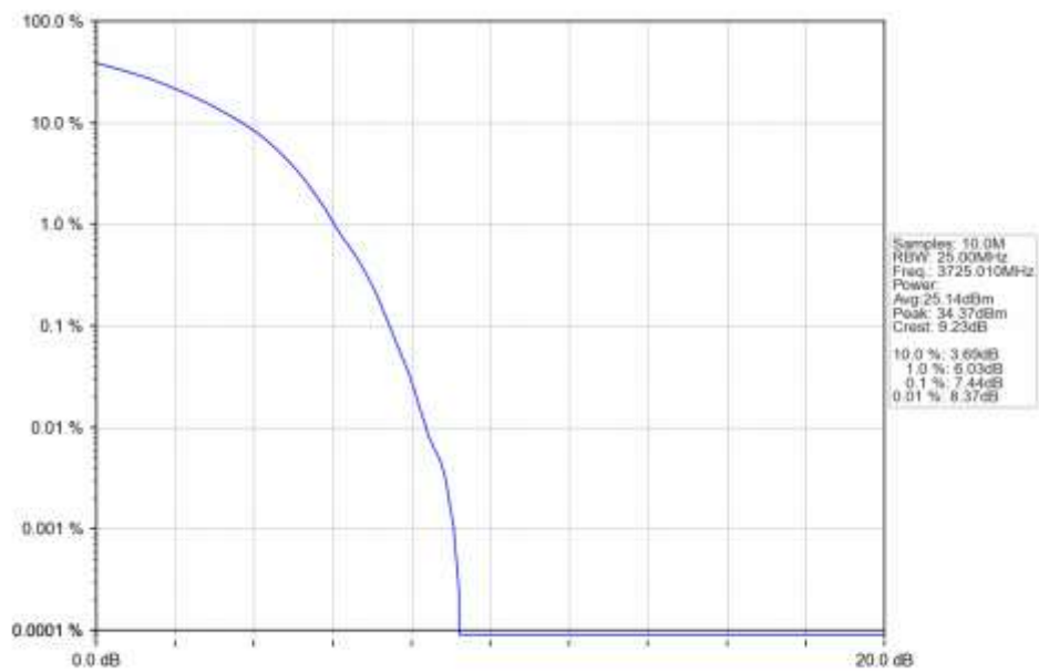
n77a 30kHz SISO NTN 50MHz DFT-s-OFDM 16 QAM 3725.01MHz Outer Full Ant1
