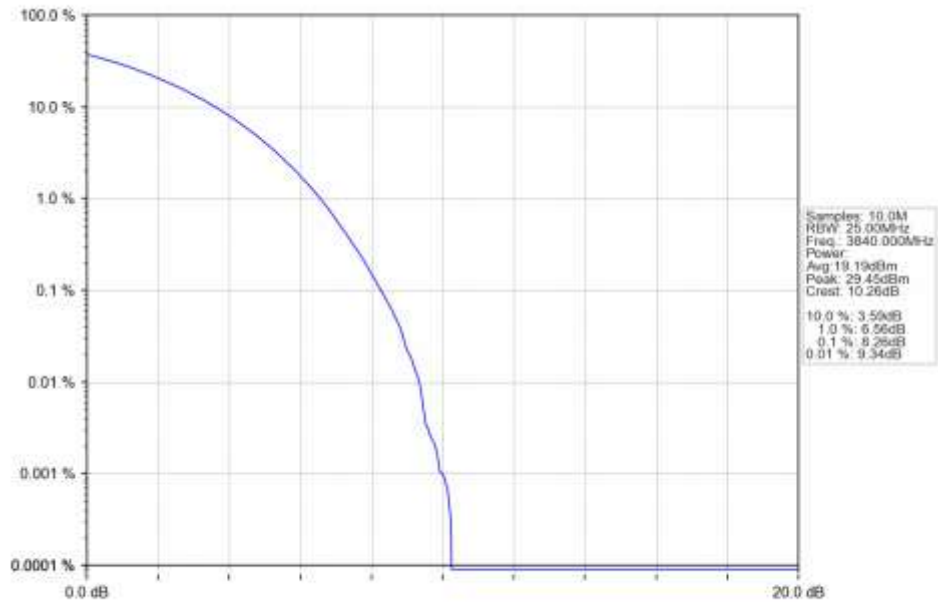
n77a 15kHz SISO NTN 50MHz CP-OFDM 256 QAM 3840MHz Outer Full Ant1
