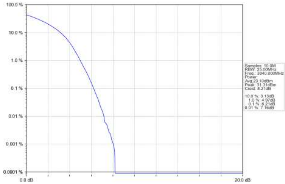
n77a 15kHz SISO NTN 25MHz DFT-s-OFDM 256 QAM 3840MHz Outer Full Ant1
