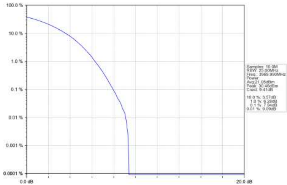
n77a 15kHz SISO NTN 20MHz CP-OFDM 256 QAM 3969.99MHz Outer Full Ant1
