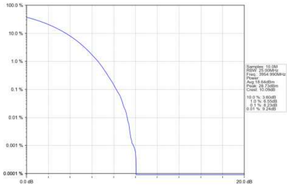
n77a 15kHz SISO NTN 50MHz CP-OFDM 256 QAM 3954.99MHz Outer Full Ant1
