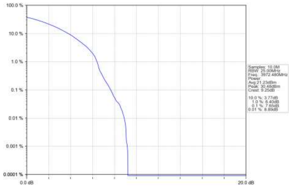
n77a 30kHz SISO NTN 15MHz CP-OFDM 256 QAM 3972.48MHz Outer Full Ant1
