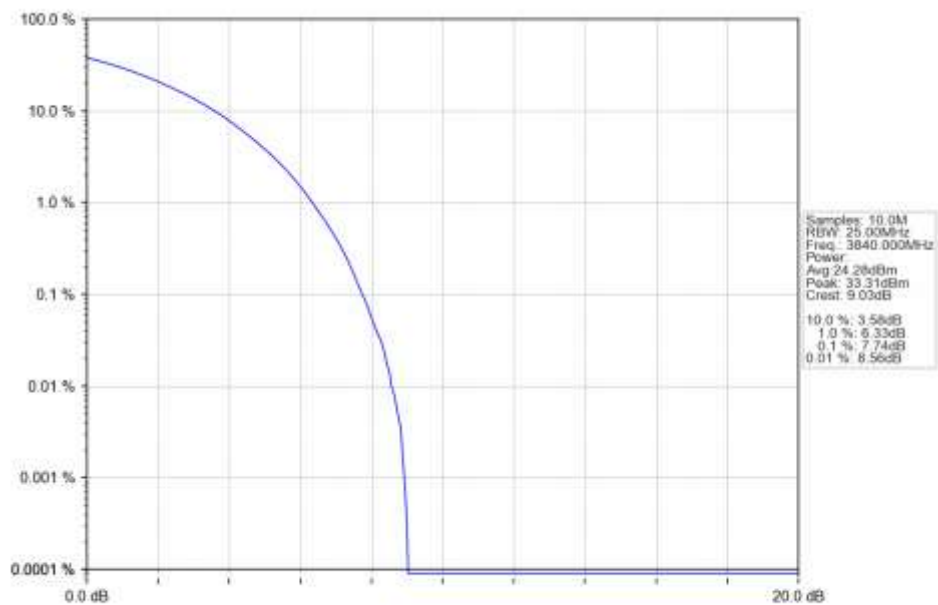
n77a 15kHz SISO NTN 30MHz CP-OFDM QPSK 3840MHz Outer Full Ant1
