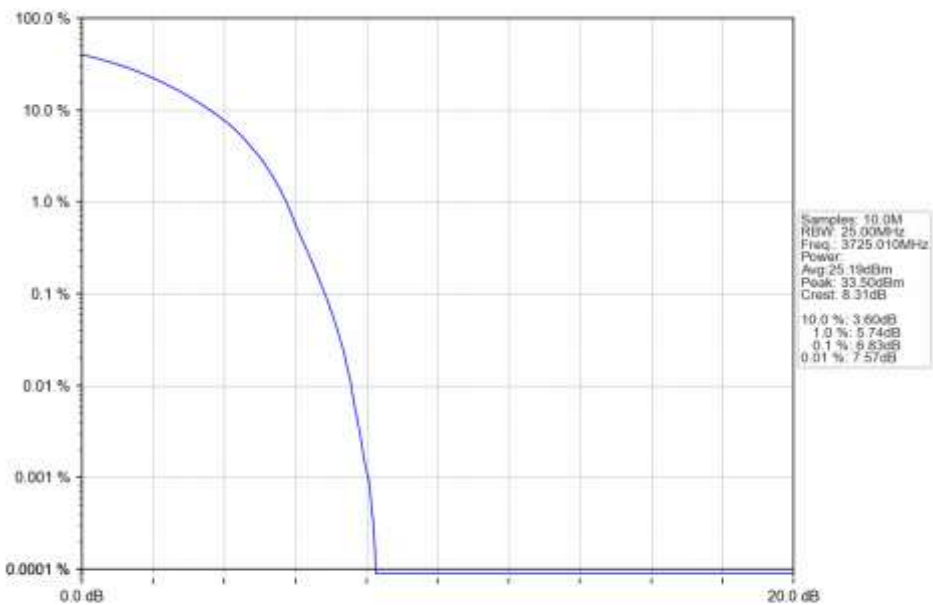
n77a_30kHz_SISO_NTNV_50MHz_DFT-s-OFDM QPSK_3725.01MHz_Outer_Full_Ant1
