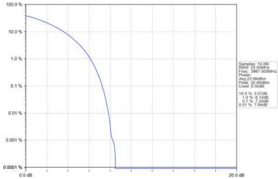
n77a 15kHz SISO NTN 25MHz CP-OFDM QPSK 3967.5MHz Outer Full Ant1
