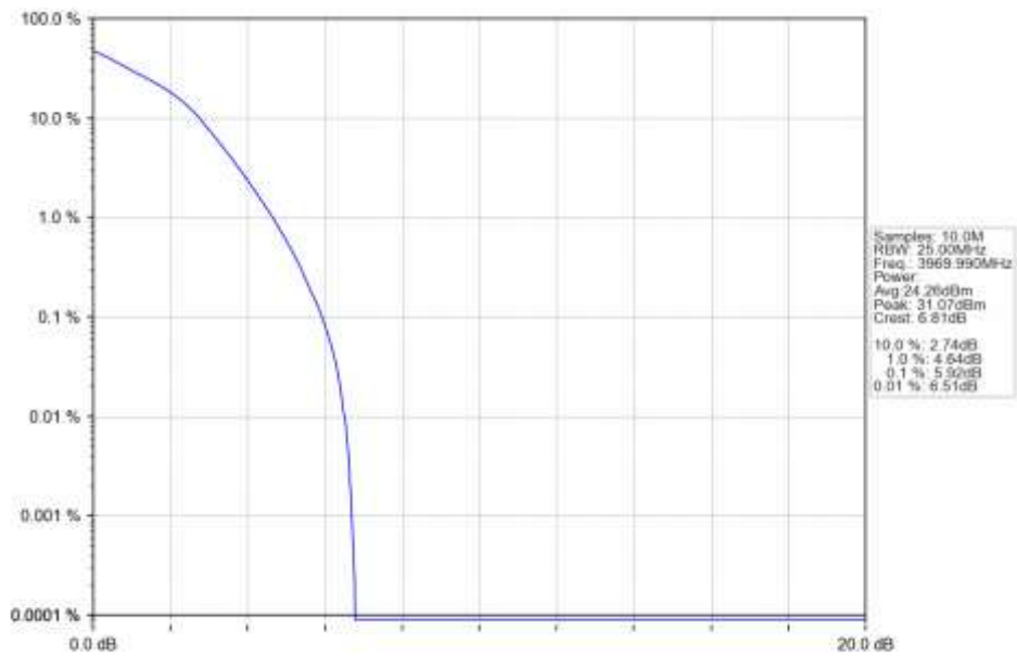
n77a 15kHz SISO NTN 20MHz DFT-s-OFDM 16 QAM 3969.99MHz Outer Full Ant1
