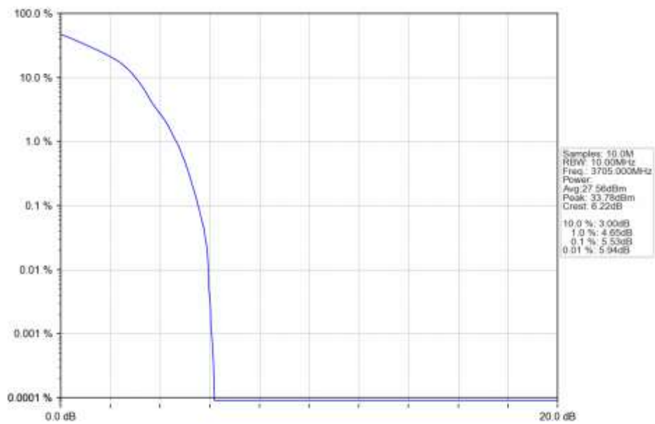
n77a 30kHz SISO NTN 10MHz DFT-s-OFDM 16 QAM 3705MHz Outer Full Ant1
