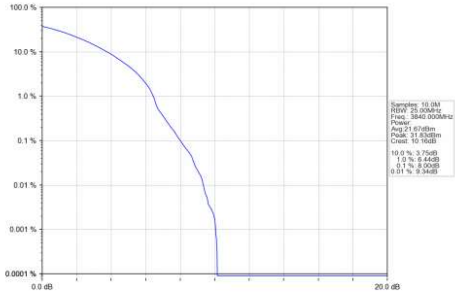
n77a 30kHz SISO NTN 25MHz CP-OFDM 256 QAM 3840MHz Outer Full Ant1
