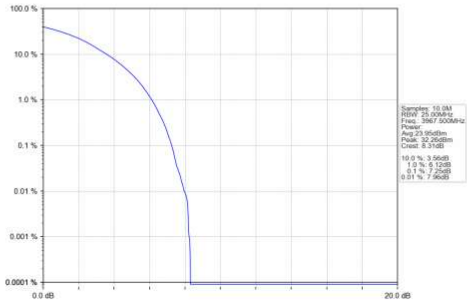
n77a 30kHz SISO NTN 25MHz CP-OFDM 16 QAM 3967.5MHz Outer Full Ant1
