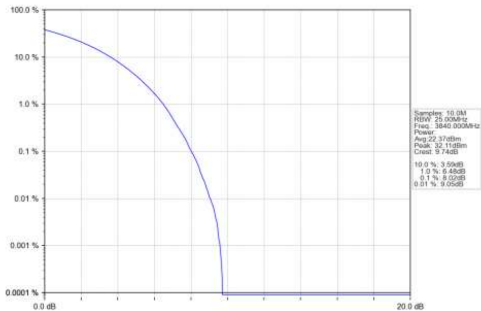
n77a 15kHz SISO NTN 50MHz CP-OFDM QPSK 3840MHz Outer Full Ant1
