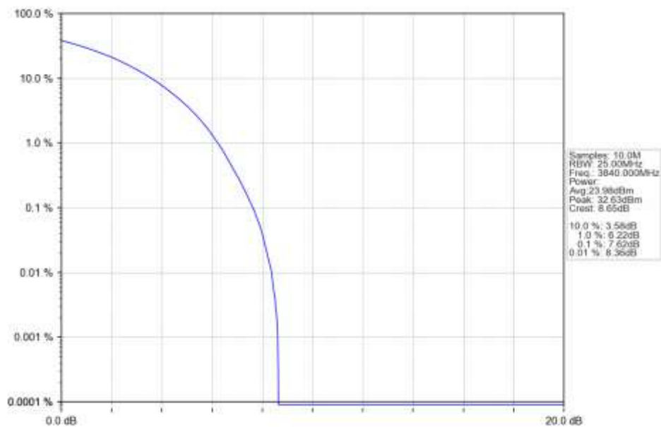
n77a 15kHz SISO NTN 25MHz CP-OFDM 64 QAM 3840MHz Outer Full Ant1
