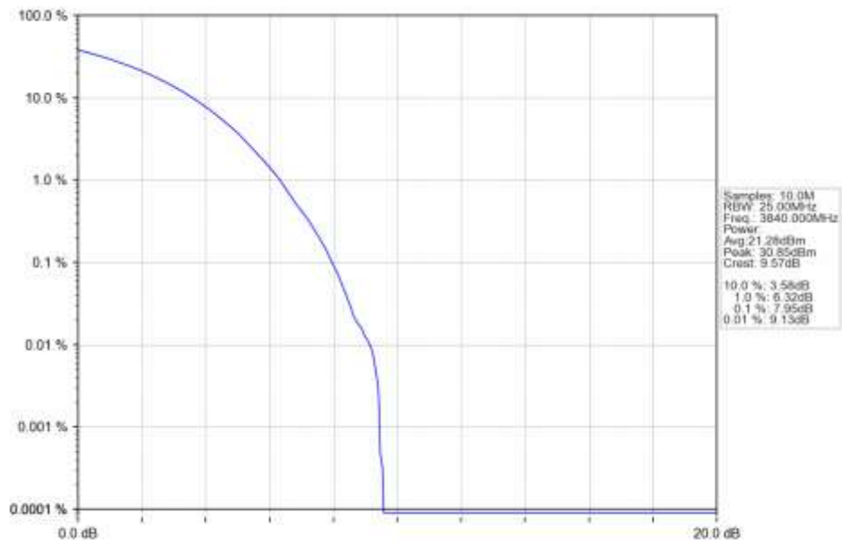
n77a 15kHz SISO NTN 15MHz CP-OFDM 256 QAM 3840MHz Outer Full Ant1
