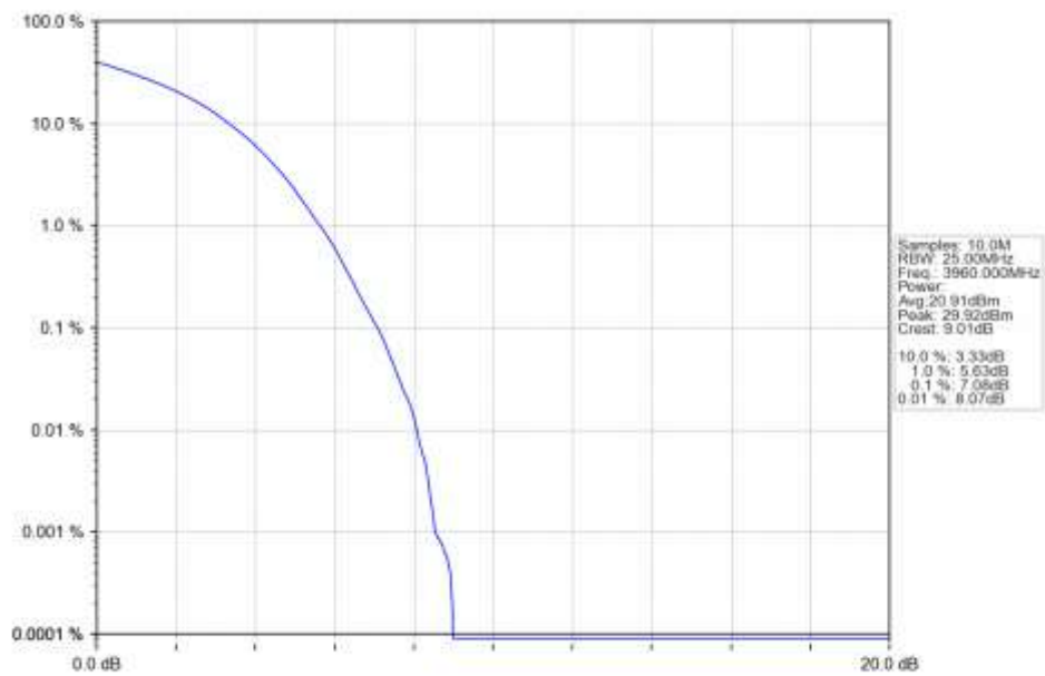
n77a 15kHz SISO NTN 40MHz DFT-s-OFDM 256 QAM 3960MHz Outer Full Ant1
