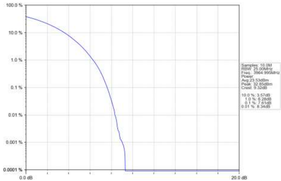
n77a 15kHz SISO NTN 30MHz CP-OFDM 16 QAM 3964.995MHz Outer Full Ant1
