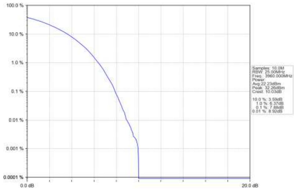
n77a 15kHz SISO NTN 40MHz CP-OFDM 16 QAM 3960MHz Outer Full Ant1
