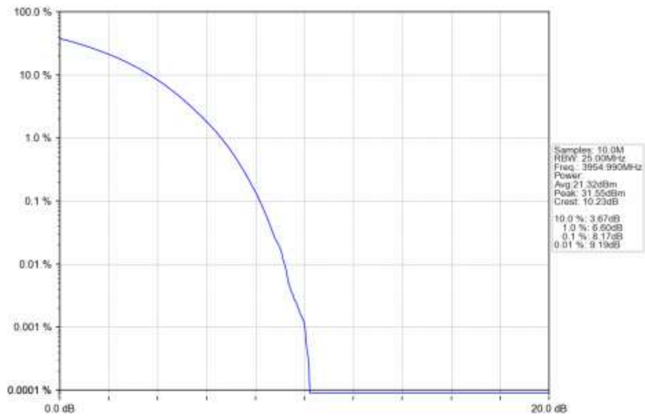
n77a 30kHz SISO NTN 50MHz CP-OFDM QPSK 3954.99MHz Outer Full Ant1
