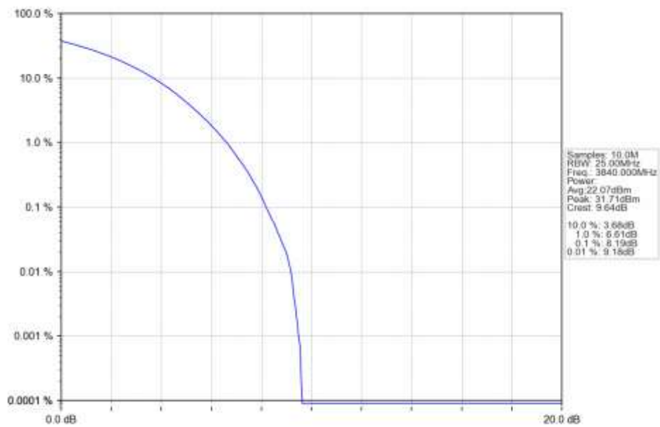
n77a 30kHz SISO NTN 50MHz CP-OFDM QPSK 3840MHz Outer Full Ant1
