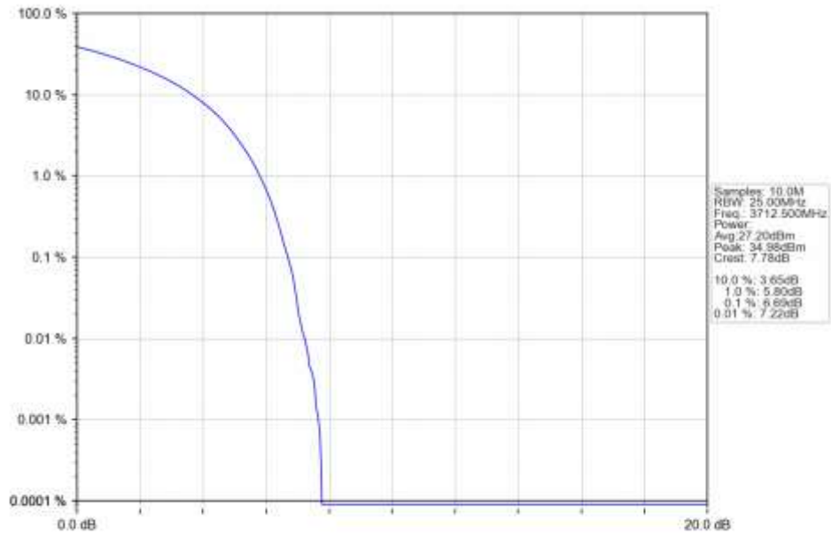
n77a 15kHz SISO NTN 25MHz CP-OFDM QPSK 3712.5MHz Outer Full Ant1
