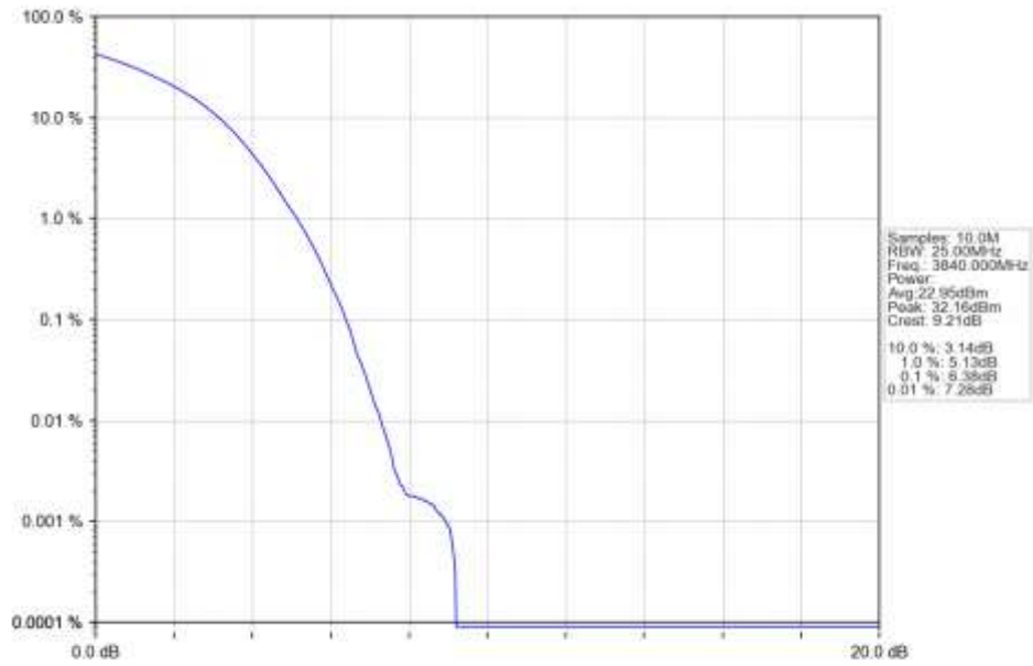
n77a 15kHz SISO NTN 30MHz DFT-s-OFDM 256 QAM 3840MHz Outer Full Ant1
