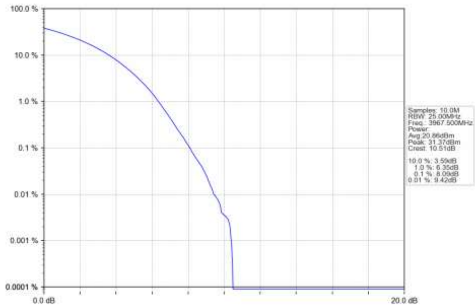
n77a 15kHz SISO NTN 25MHz CP-OFDM 256 QAM 3967.5MHz Outer Full Ant1
