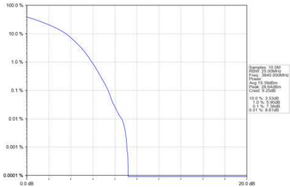
n77a 30kHz SISO NTN 70MHz DFT-s-OFDM 256 QAM 3840MHz Outer Full Ant1
