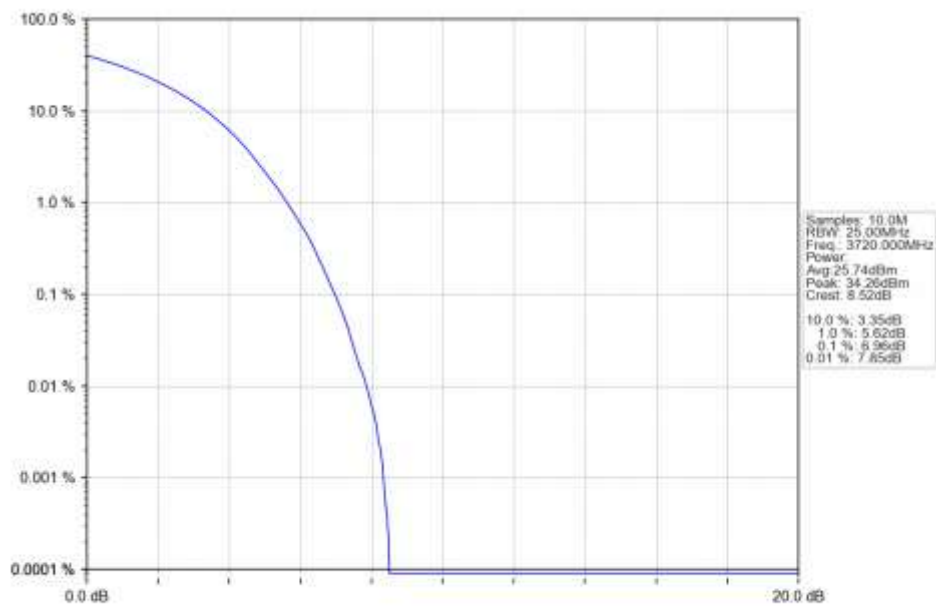
n77a 15kHz SISO NTN 40MHz DFT-s-OFDM 16 QAM 3720MHz Outer Full Ant1
