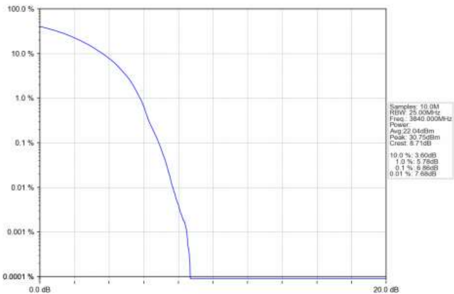
n77a_30kHz_SISO_NTNV_50MHz_DFT-s-OFDM QPSK_3840MHz_Outer_Full_Ant1
