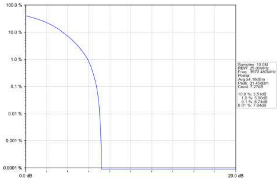
n77a 30kHz SISO NTN 15MHz CP-OFDM 16 QAM 3972.48MHz Outer Full Ant1
