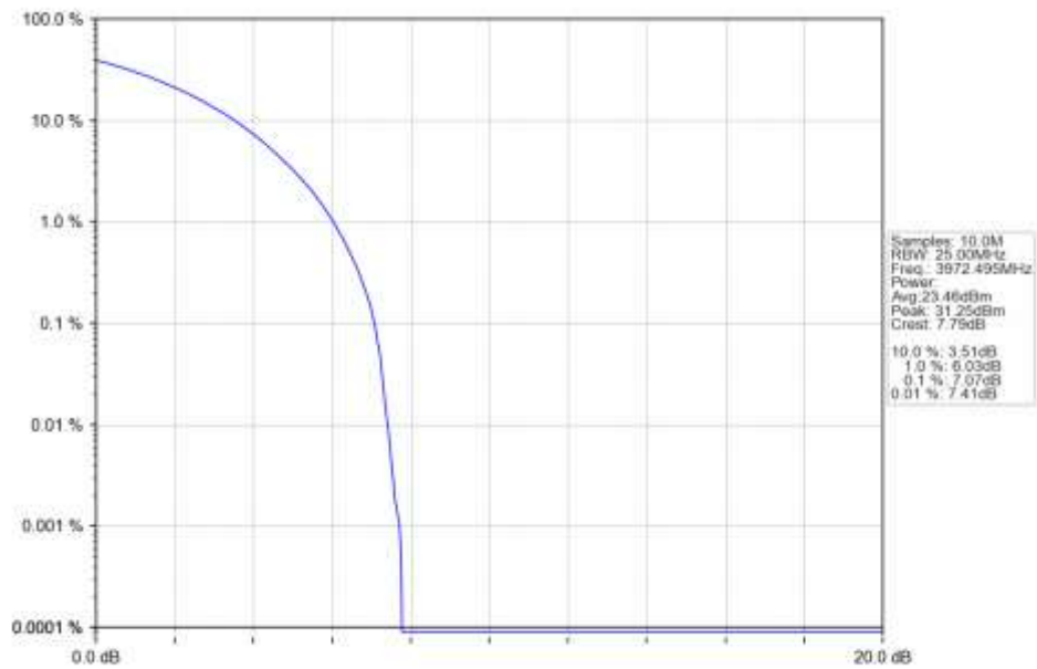
n77a 15kHz SISO NTN 15MHz CP-OFDM 64 QAM 3972.495MHz Outer Full Ant1
