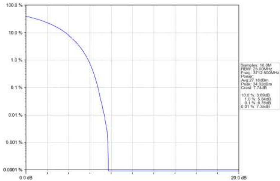
n77a 30kHz SISO NTN 25MHz CP-OFDM 64 QAM 3712.5MHz Outer Full Ant1
