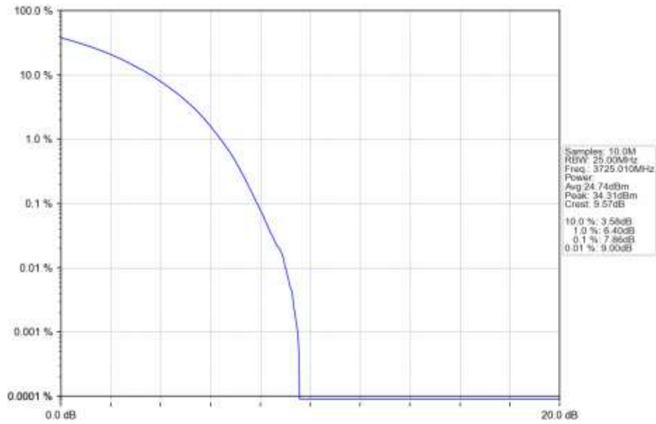
n77a 15kHz SISO NTN 50MHz CP-OFDM 64 QAM 3725.01MHz Outer Full Ant1
