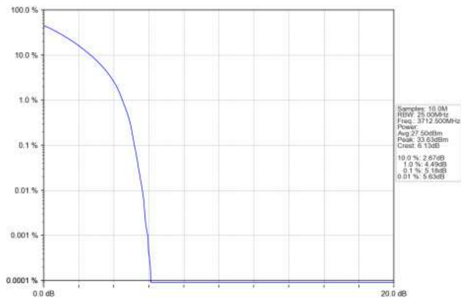
n77a_15kHz_SISO_NTNV_25MHz_DFT-s-OFDM QPSK_3712.5MHz_Outer_Full_Ant1
