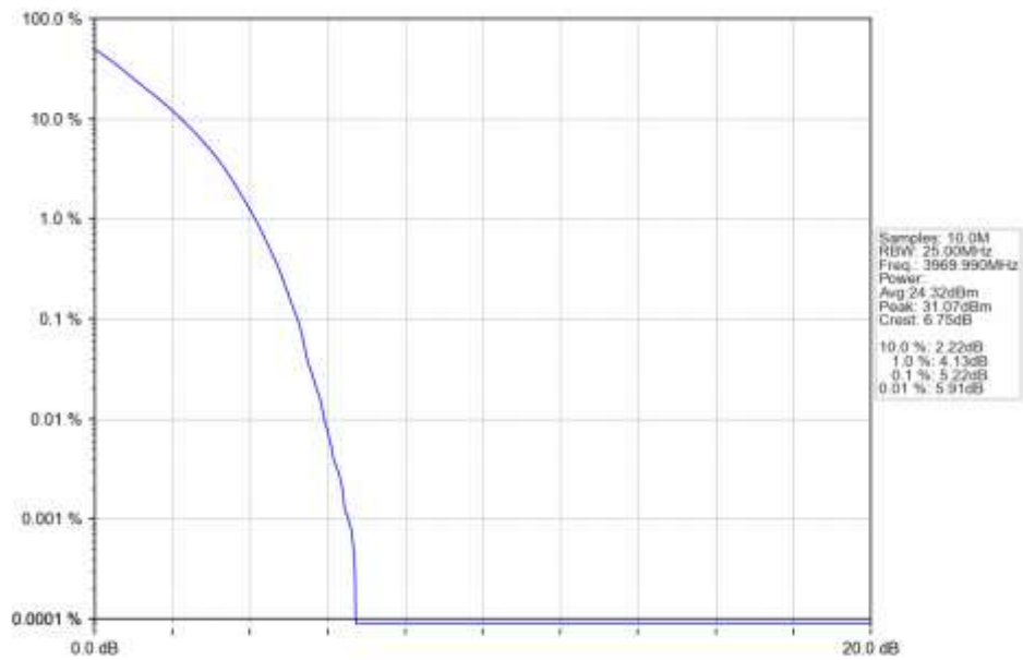
n77a 15kHz SISO NTN 20MHz DFT-s-OFDM QPSK 3969.99MHz Outer Full Ant1
