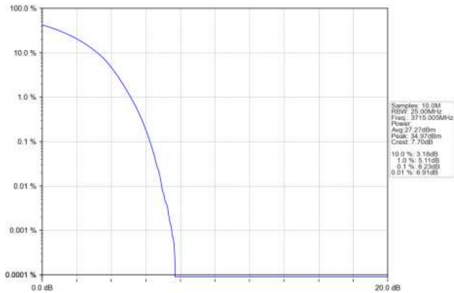
n77a 15kHz SISO NTN 30MHz DFT-s-OFDM 64 QAM 3715.005MHz Outer Full Ant1
