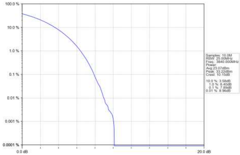
n77a 15kHz SISO NTN 40MHz CP-OFDM 16 QAM 3840MHz Outer Full Ant1
