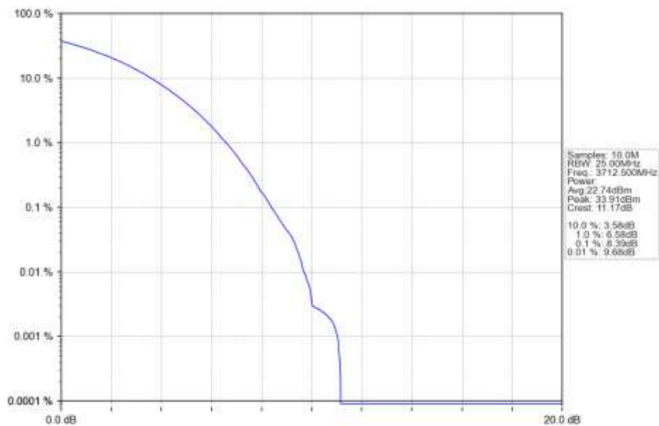
n77a 15kHz SISO NTN 25MHz CP-OFDM 256 QAM 3712.5MHz Outer Full Ant1
