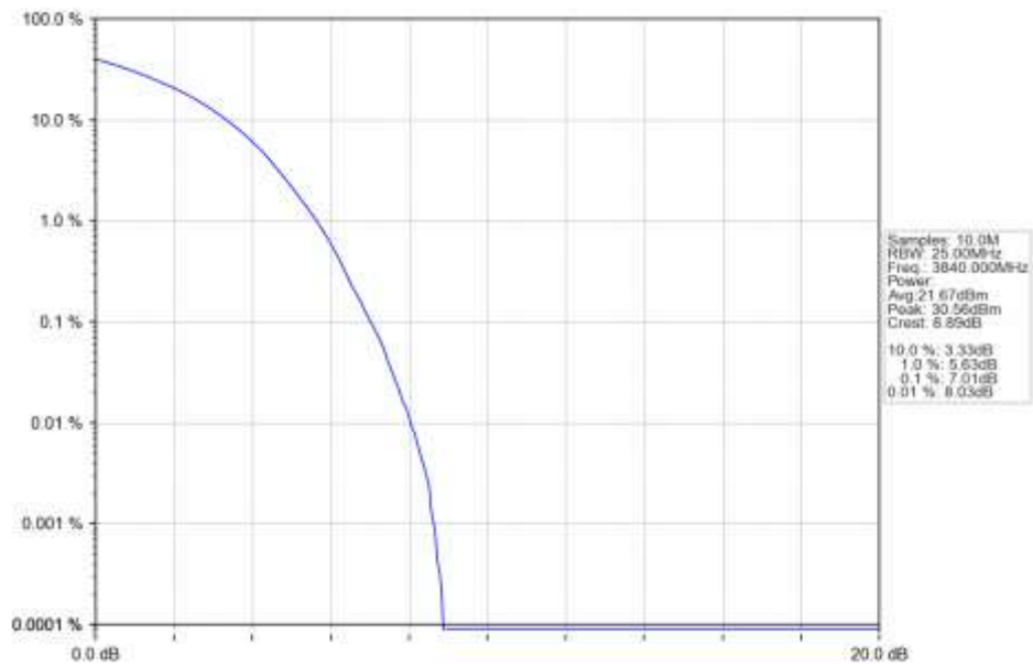
n77a 15kHz SISO NTN 40MHz DFT-s-OFDM 256 QAM 3840MHz Outer Full Ant1
