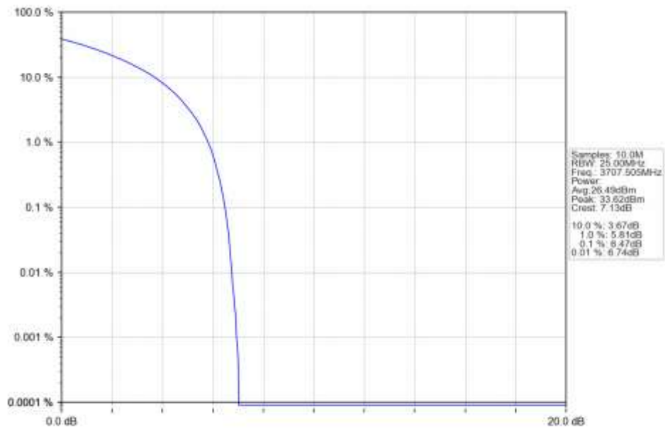
n77a 15kHz SISO NTN 15MHz CP-OFDM 64 QAM 3707.505MHz Outer Full Ant1
