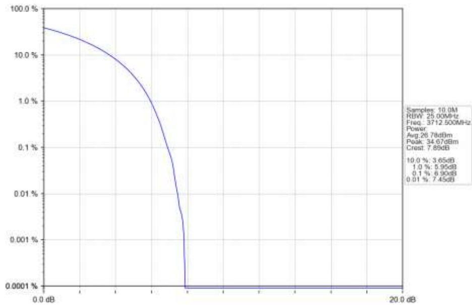
n77a 15kHz SISO NTN 25MHz CP-OFDM 64 QAM 3712.5MHz Outer Full Ant1
