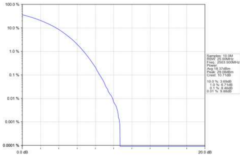
n41 15kHz SISO NTN 15MHz CP-OFDM 256 QAM 2503.5MHz Outer Full Ant1
