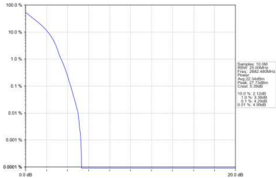
n41 30kHz SISO NTN 15MHz DFT-s-OFDM PI/2 BPSK 2682.48MHz Outer Full Ant1
