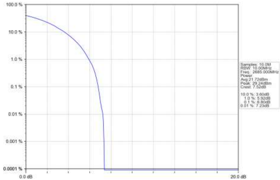
n41 30kHz SISO NTN 10MHz CP-OFDM 16 QAM 2685MHz Outer Full Ant1
