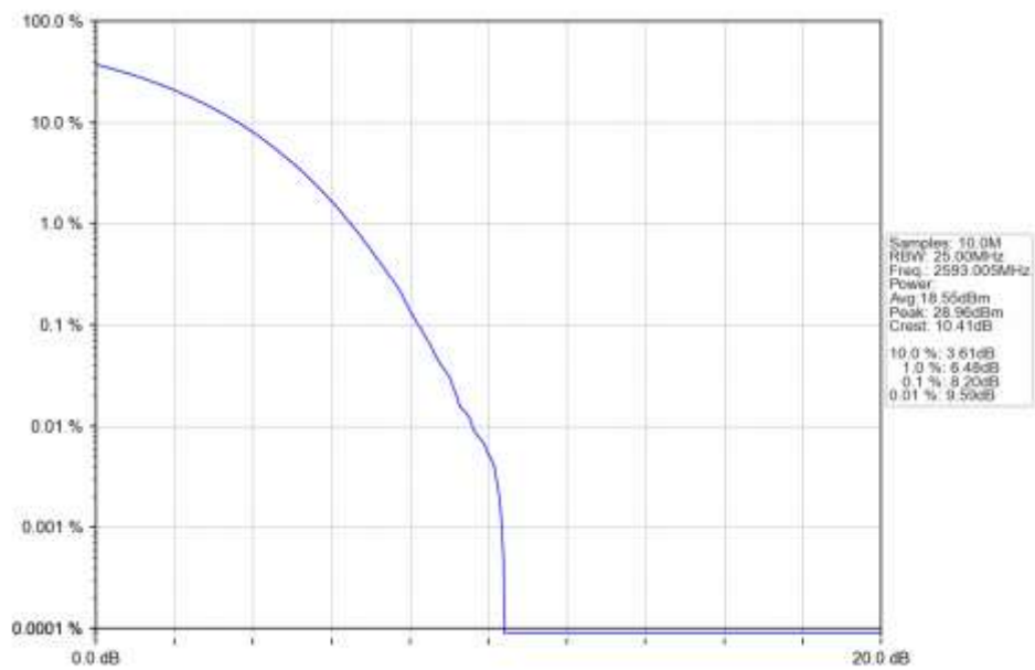
n41 15kHz SISO NTN 15MHz CP-OFDM 256 QAM 2593.005MHz Outer Full Ant1
