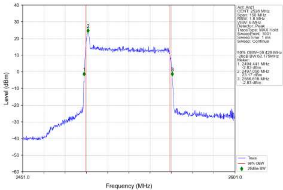
n41 30kHz SISO NTN 60MHz DFT-s-OFDM QPSK 2526MHz Outer Full Ant1
