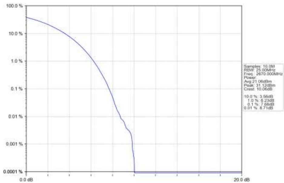
n41 15kHz SISO NTN 40MHz CP-OFDM QPSK 2670MHz Outer Full Ant1
