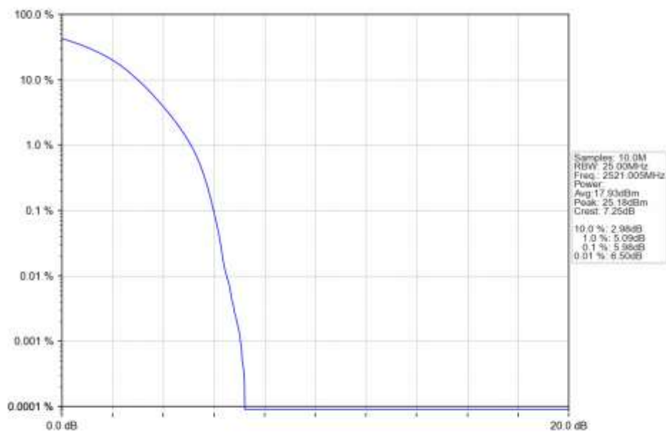
n41_15kHz_SISO_NTNV_50MHz_DFT-s-OFDM PI/2 BPSK_2521.005MHz_Outer_Full_Ant1
