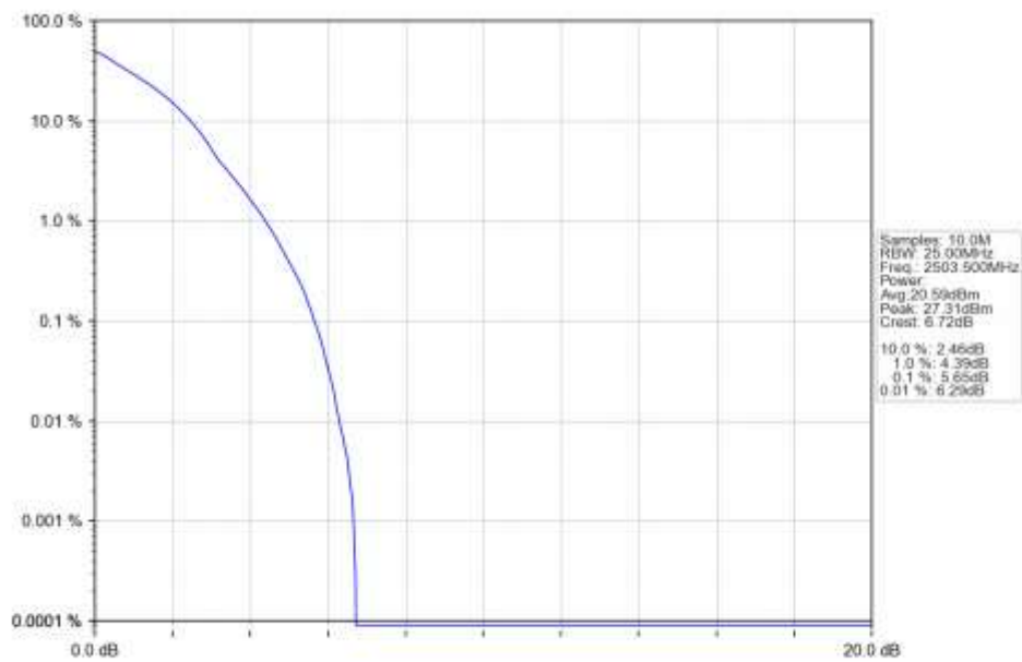
n41 30kHz SISO NTN 15MHz DFT-s-OFDM QPSK 2503.5MHz Outer Full Ant1
