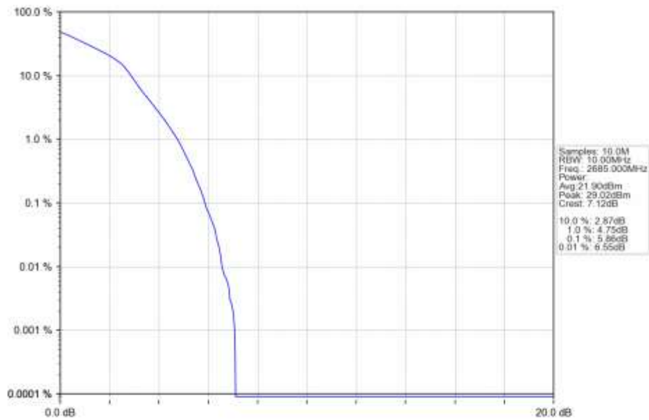
n41 30kHz SISO NTN 10MHz DFT-s-OFDM 16 QAM 2685MHz Outer Full Ant1
