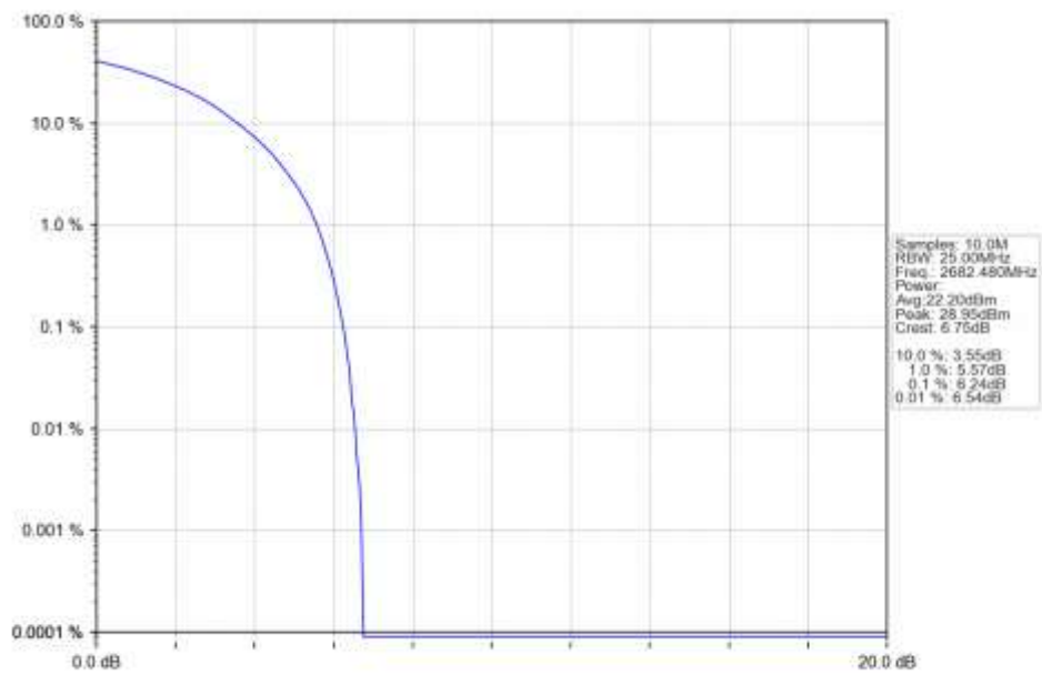
n41 30kHz SISO NTN 15MHz CP-OFDM QPSK 2682.48MHz Outer Full Ant1
