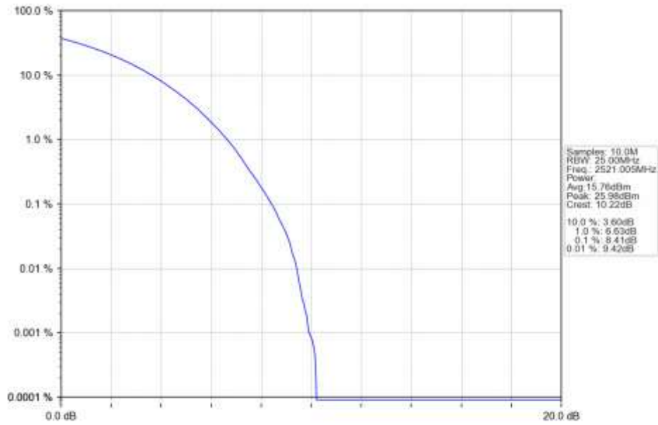
n41 15kHz SISO NTN 50MHz CP-OFDM 256 QAM 2521.005MHz Outer Full Ant1
