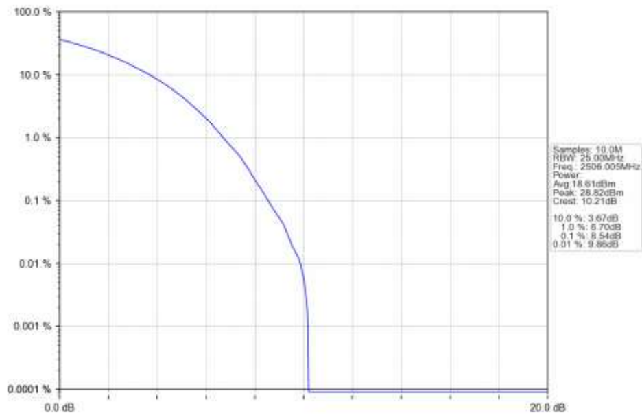
n41 15kHz SISO NTN 20MHz CP-OFDM 256 QAM 2506.005MHz Outer Full Ant1
