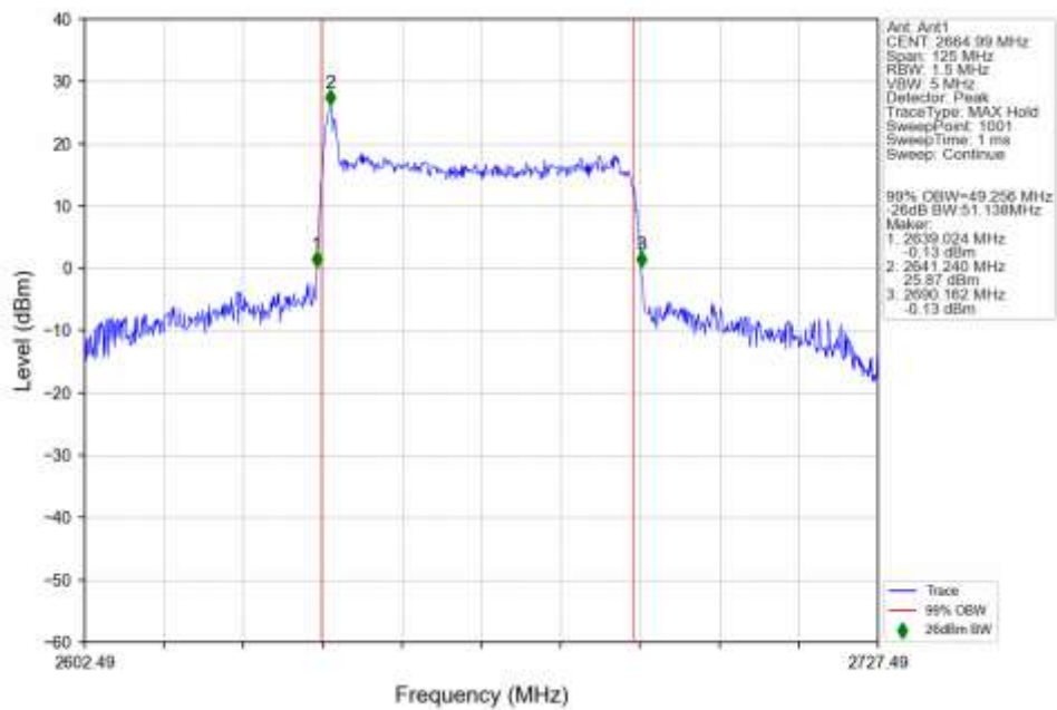
n41 30kHz SISO NTN 50MHz CP-OFDM 64 QAM 2664.99MHz Outer Full Ant1
