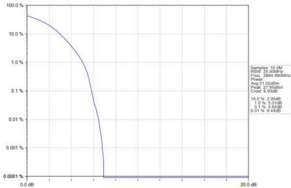
n41 15kHz SISO NTN 50MHz DFT-s-OFDM PI/2 BPSK 2664.99MHz Outer Full Ant1
