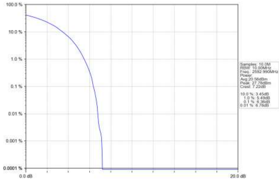
n41 30kHz SISO NTN 10MHz CP-OFDM QPSK 2592.99MHz Outer Full Ant1
