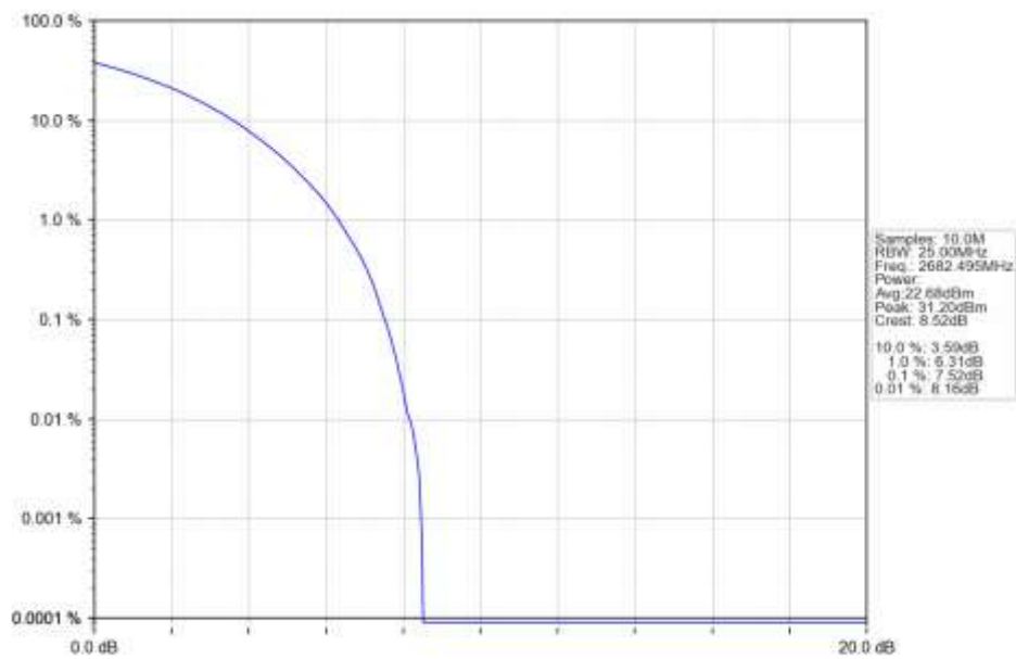
n41 15kHz SISO NTN 15MHz CP-OFDM QPSK 2682.495MHz Outer Full Ant1
