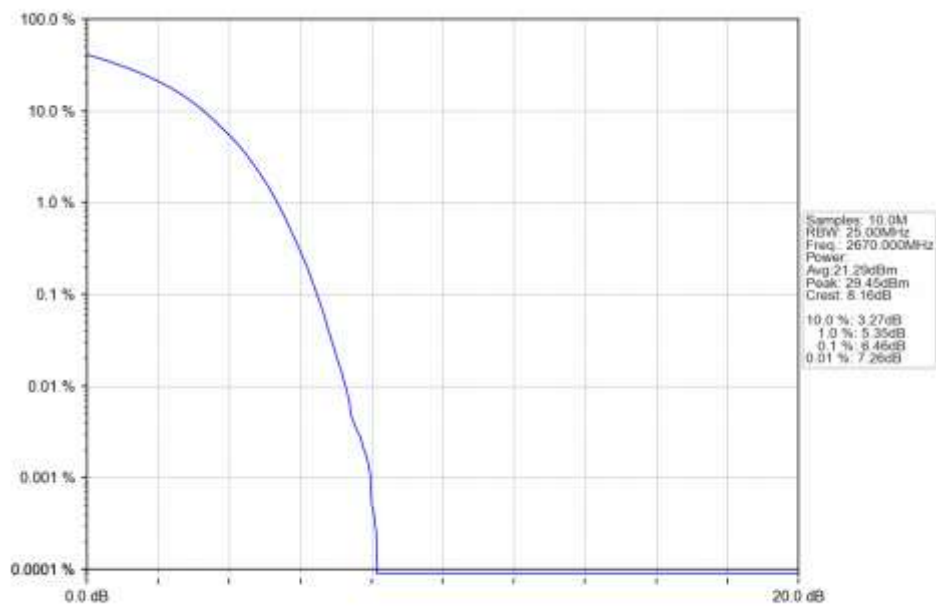
n41 15kHz SISO NTN 40MHz DFT-s-OFDM QPSK 2670MHz Outer Full Ant1
