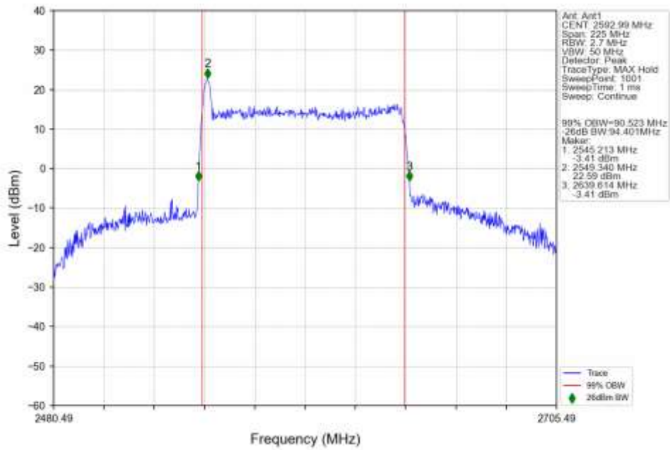
n41 30kHz SISO NTN 90MHz CP-OFDM 16 QAM 2592.99MHz Outer Full Ant1
