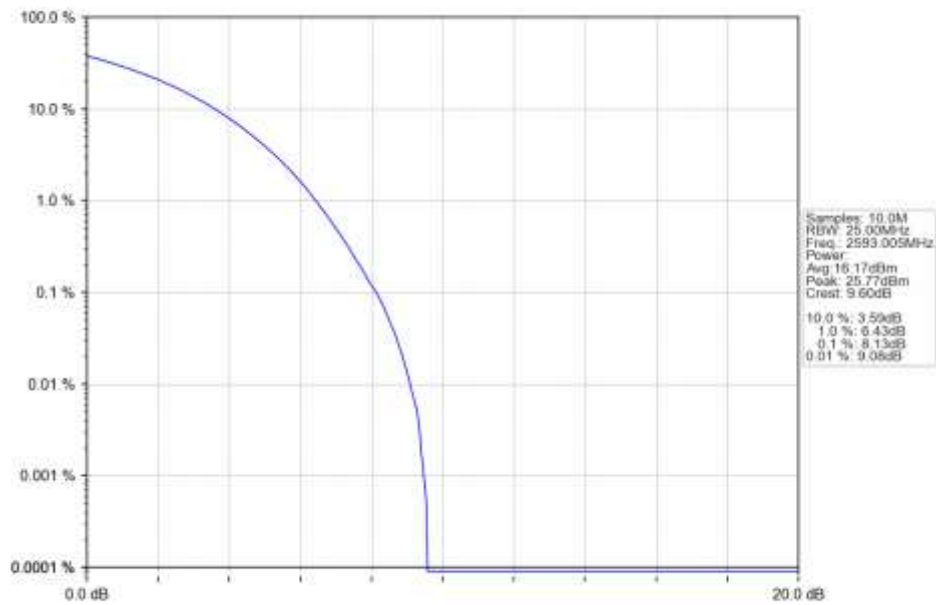
n41 15kHz SISO NTN 50MHz CP-OFDM 256 QAM 2593.005MHz Outer Full Ant1
