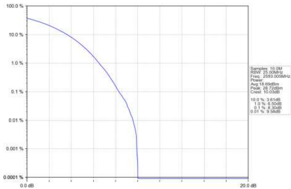
n41 15kHz SISO NTN 20MHz CP-OFDM 256 QAM 2593.005MHz Outer Full Ant1
