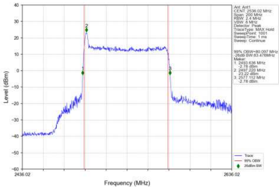
n41 30kHz SISO NTN 80MHz CP-OFDM 64 QAM 2536.02MHz Outer Full Ant1
