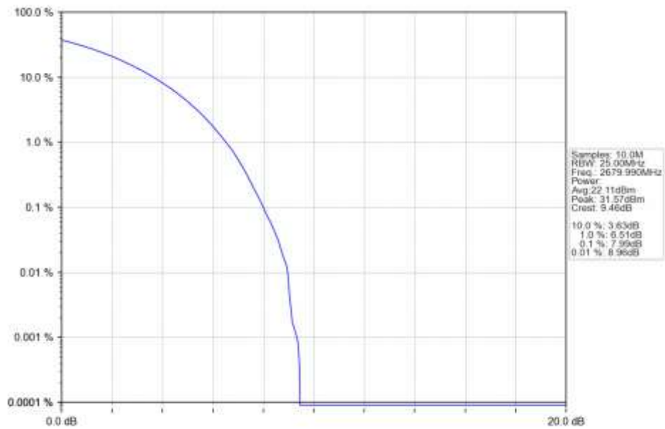
n41 15kHz SISO NTN 20MHz CP-OFDM 64 QAM 2679.99MHz Outer Full Ant1
