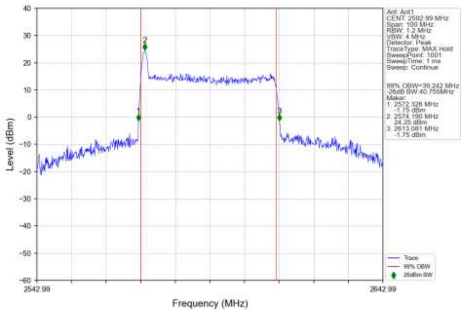
n41 30kHz SISO NTN 40MHz CP-OFDM 16 QAM 2592.99MHz Outer Full Ant1
