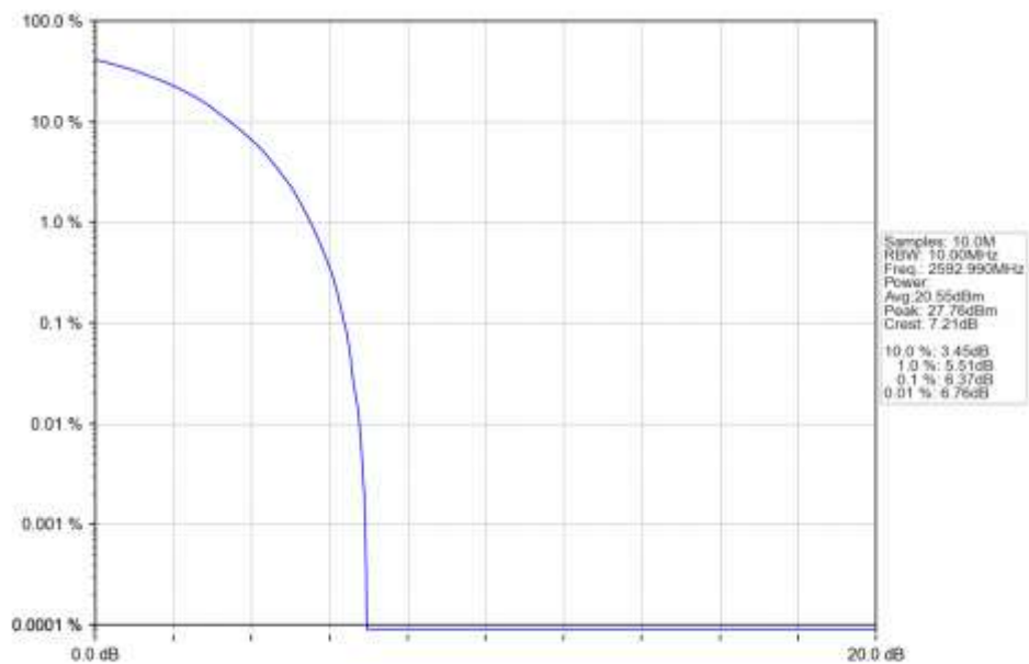
n41 30kHz SISO NTN 10MHz CP-OFDM 16 QAM 2592.99MHz Outer Full Ant1
