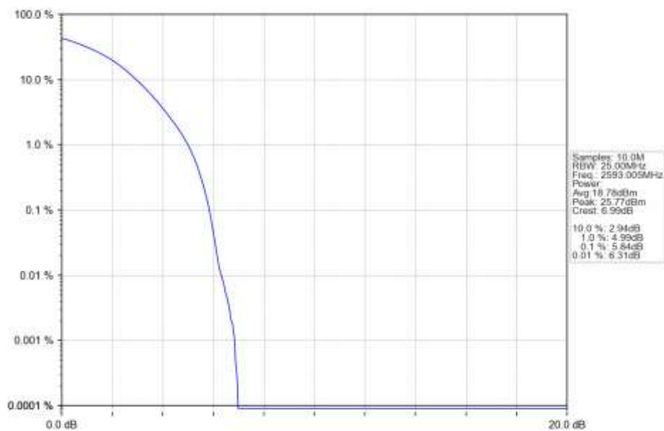
n41_15kHz_SISO_NTNV_50MHz_DFT-s-OFDM PI/2 BPSK_2593.005MHz_Outer_Full_Ant1
