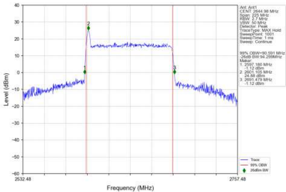
n41 30kHz SISO NTN 90MHz CP-OFDM 64 QAM 2644.98MHz Outer Full Ant1
