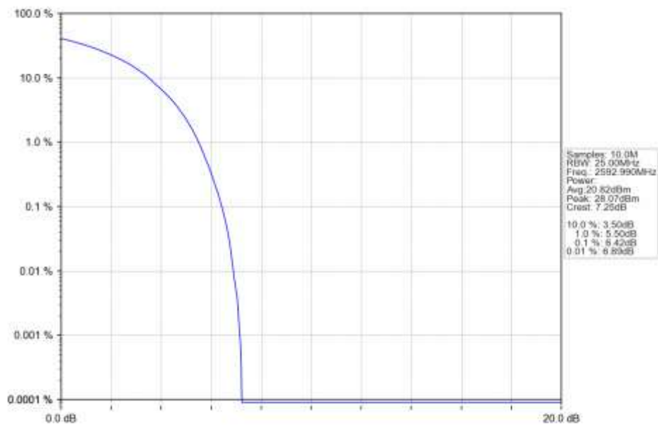
n41 30kHz SISO NTN 20MHz CP-OFDM 16 QAM 2592.99MHz Outer Full Ant1
