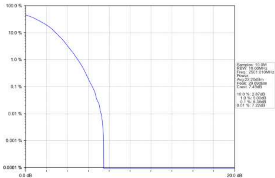
n41 15kHz SISO NTN 10MHz DFT-s-OFDM 64 QAM 2501.01MHz Outer Full Ant1
