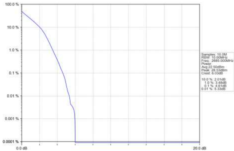
n41 15kHz SISO NTN 10MHz DFT-s-OFDM PI/2 BPSK 2685MHz Outer Full Ant1
