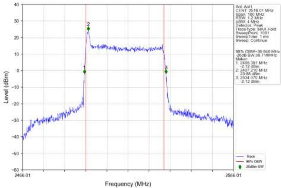
n41 30kHz SISO NTN 40MHz DFT-s-OFDM 64 QAM 2516.01MHz Outer Full Ant1
