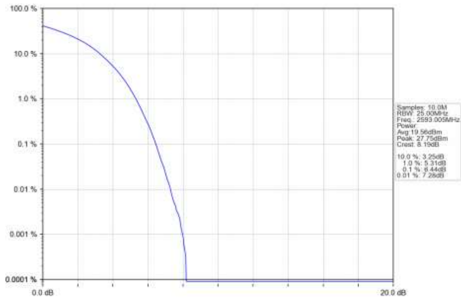
n41 15kHz SISO NTN 40MHz DFT-s-OFDM QPSK 2593.005MHz Outer Full Ant1
