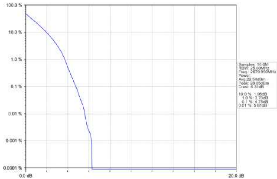
n41 15kHz SISO NTN 20MHz DFT-s-OFDM PI/2 BPSK 2679.99MHz Outer Full Ant1
