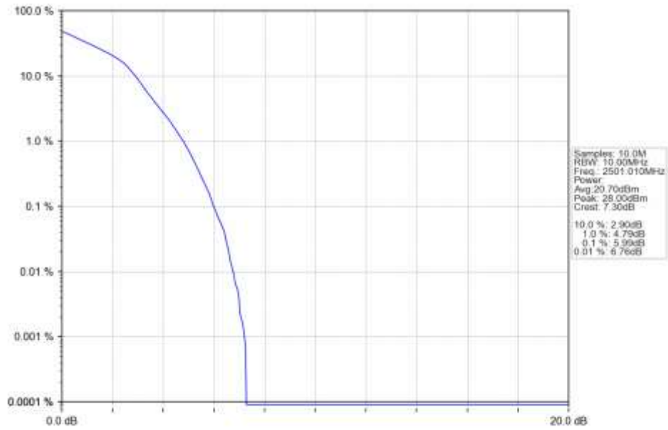
n41 30kHz SISO NTN 10MHz DFT-s-OFDM 16 QAM 2501.01MHz Outer Full Ant1
