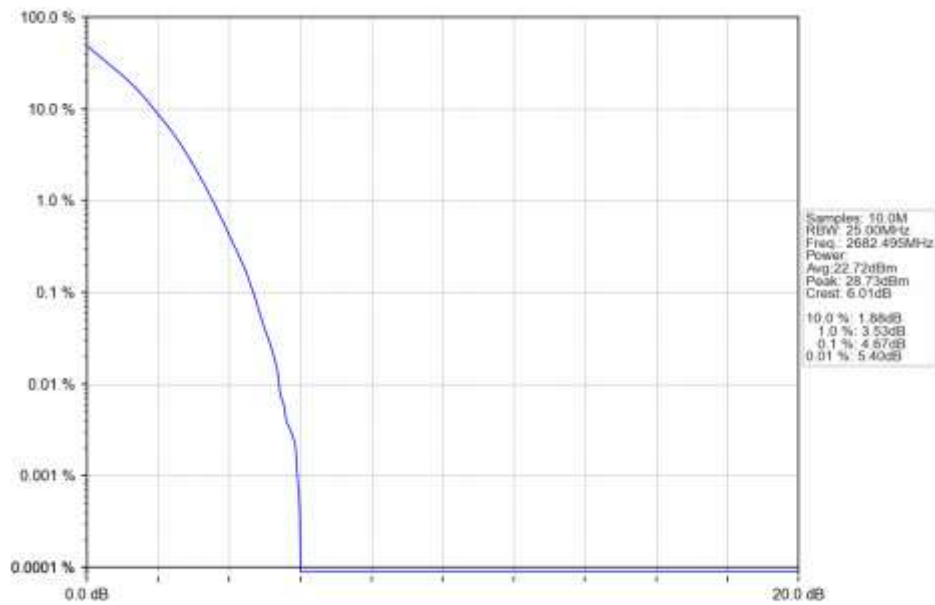
n41 15kHz SISO NTN 15MHz DFT-s-OFDM PI/2 BPSK 2682.495MHz Outer Full Ant1
