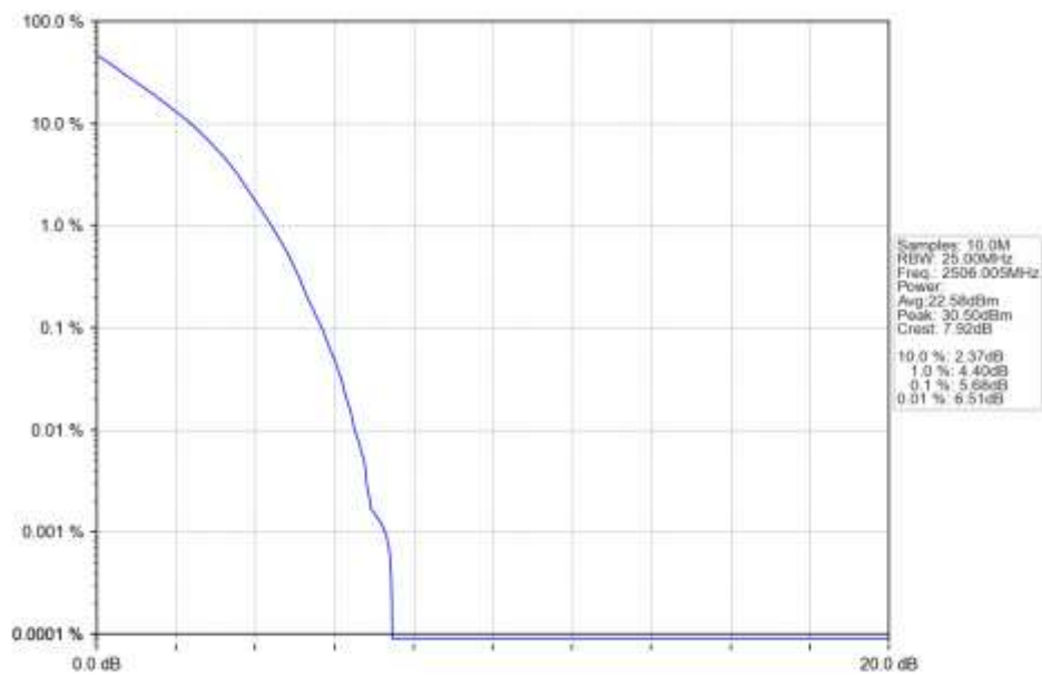
n41 15kHz SISO NTN 20MHz DFT-s-OFDM QPSK 2506.005MHz Outer Full Ant1
