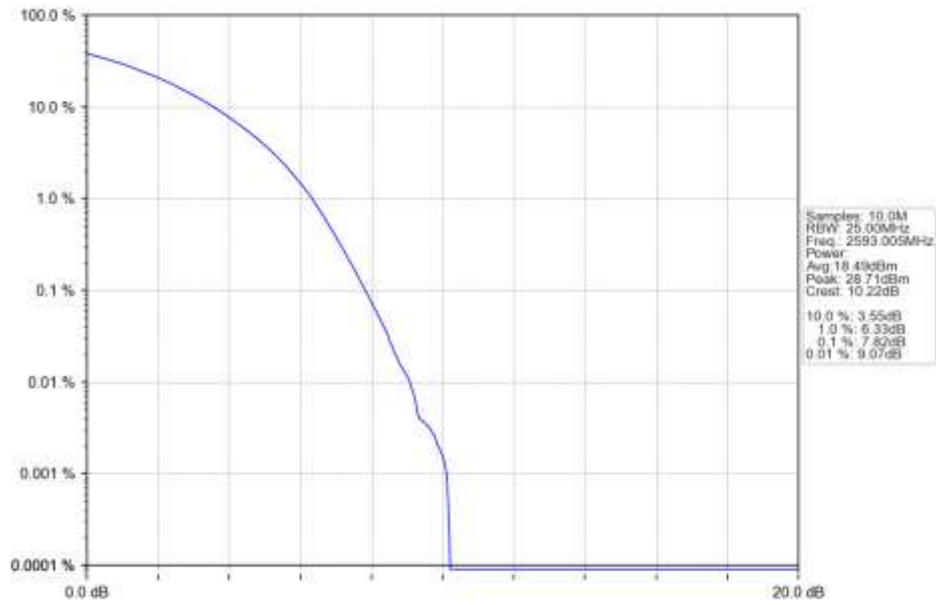
n41 15kHz SISO NTN 50MHz CP-OFDM 64 QAM 2593.005MHz Outer Full Ant1
