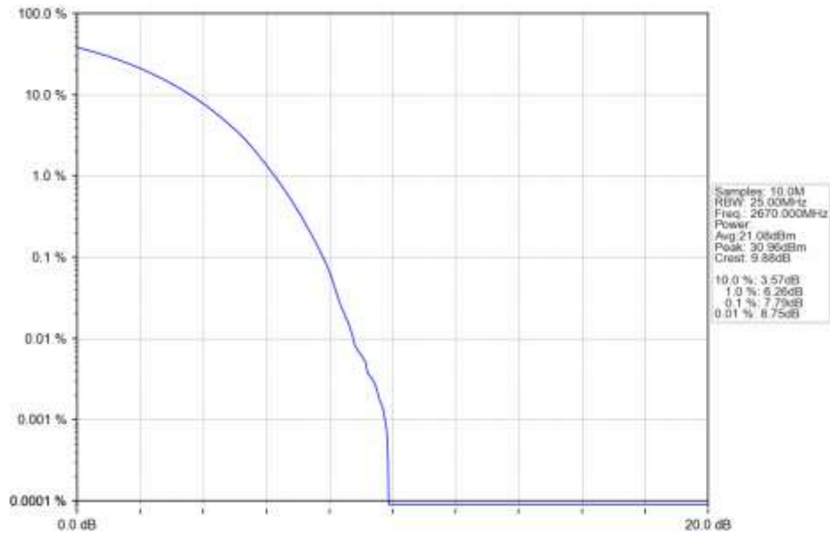
n41 15kHz SISO NTN 40MHz CP-OFDM 16 QAM 2670MHz Outer Full Ant1
