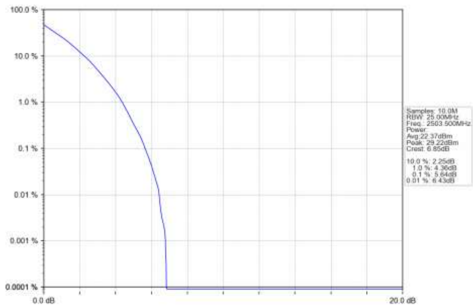
n41 15kHz SISO NTN 15MHz DFT-s-OFDM QPSK 2503.5MHz Outer Full Ant1
