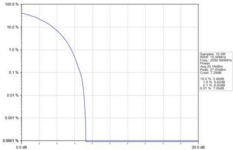
n41 30kHz SISO NTN 10MHz CP-OFDM 64 QAM 2592.99MHz Outer Full Ant1
