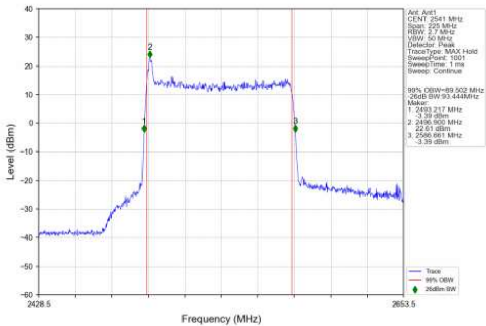
n41 30kHz SISO NTN 90MHz DFT-s-OFDM QPSK 2541MHz Outer Full Ant1
