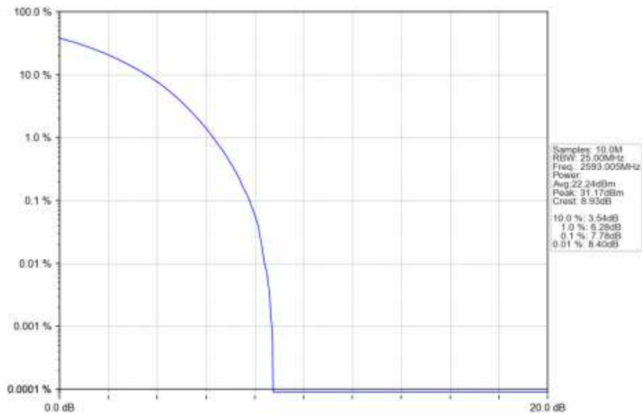
n41 15kHz SISO NTN 15MHz CP-OFDM QPSK 2593.005MHz Outer Full Ant1
