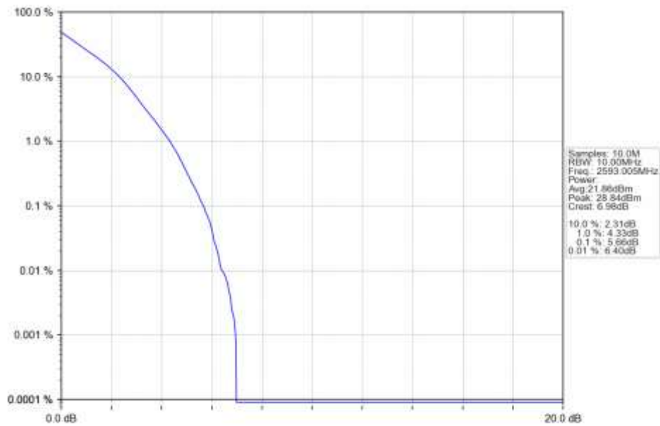
n41 15kHz SISO NTN 10MHz DFT-s-OFDM QPSK 2593.005MHz Outer Full Ant1
