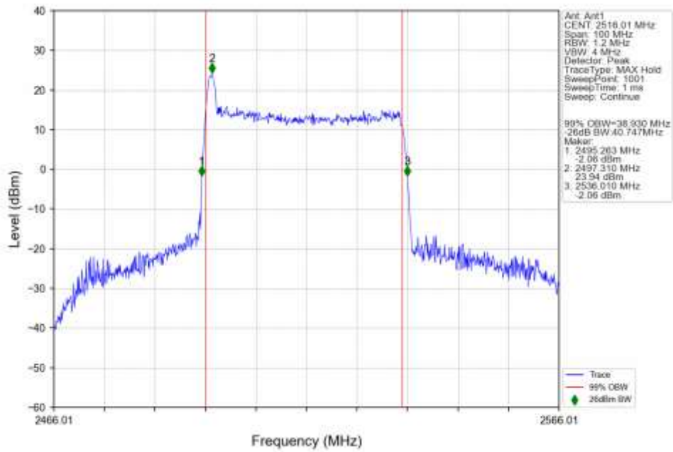
n41 30kHz SISO NTN 40MHz CP-OFDM 64 QAM 2516.01MHz Outer Full Ant1
