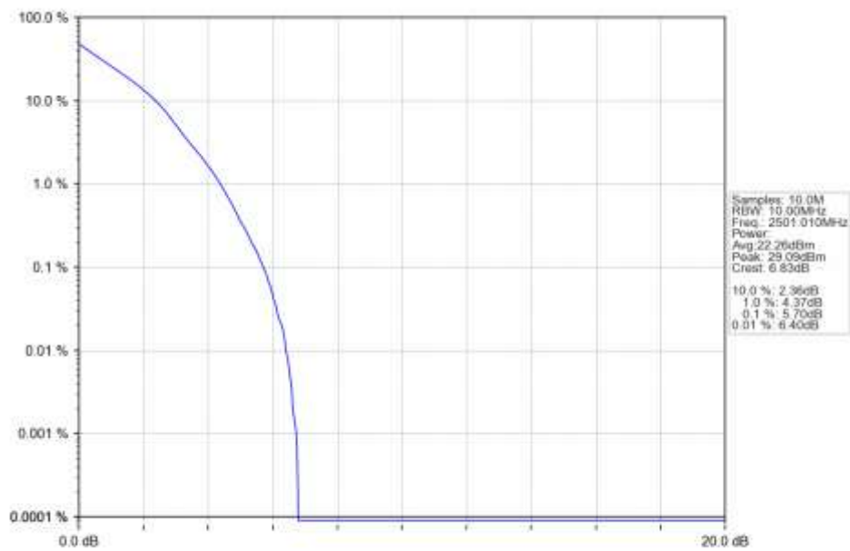
n41 15kHz SISO NTN 10MHz DFT-s-OFDM QPSK 2501.01MHz Outer Full Ant1
