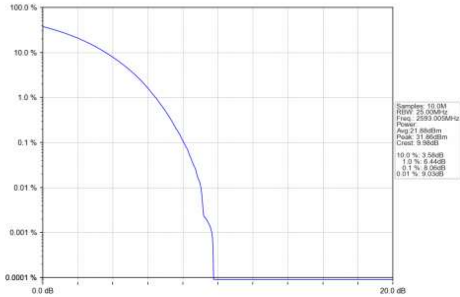
n41 15kHz SISO NTN 20MHz CP-OFDM 64 QAM 2593.005MHz Outer Full Ant1
