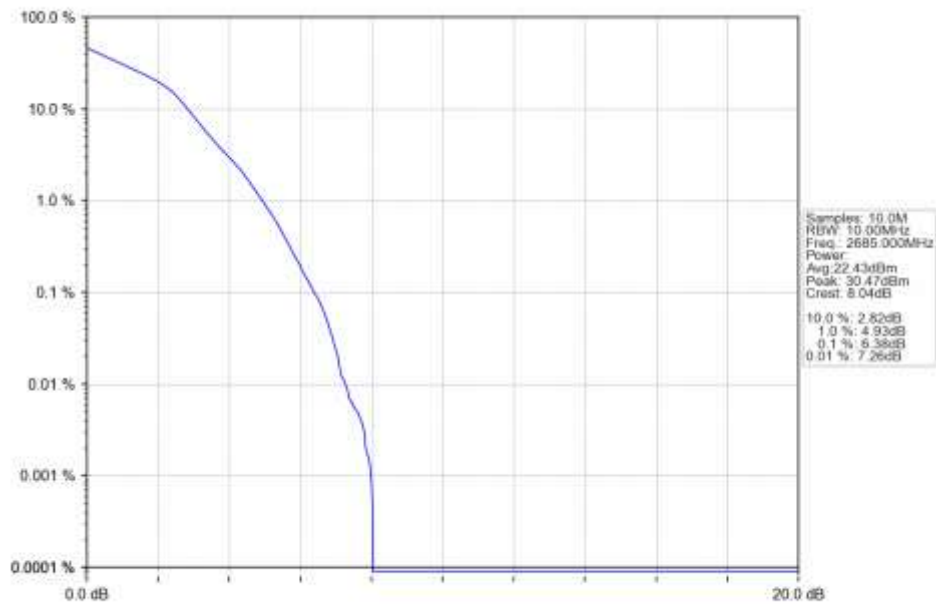
n41 15kHz SISO NTN 10MHz DFT-s-OFDM 16 QAM 2685MHz Outer Full Ant1
