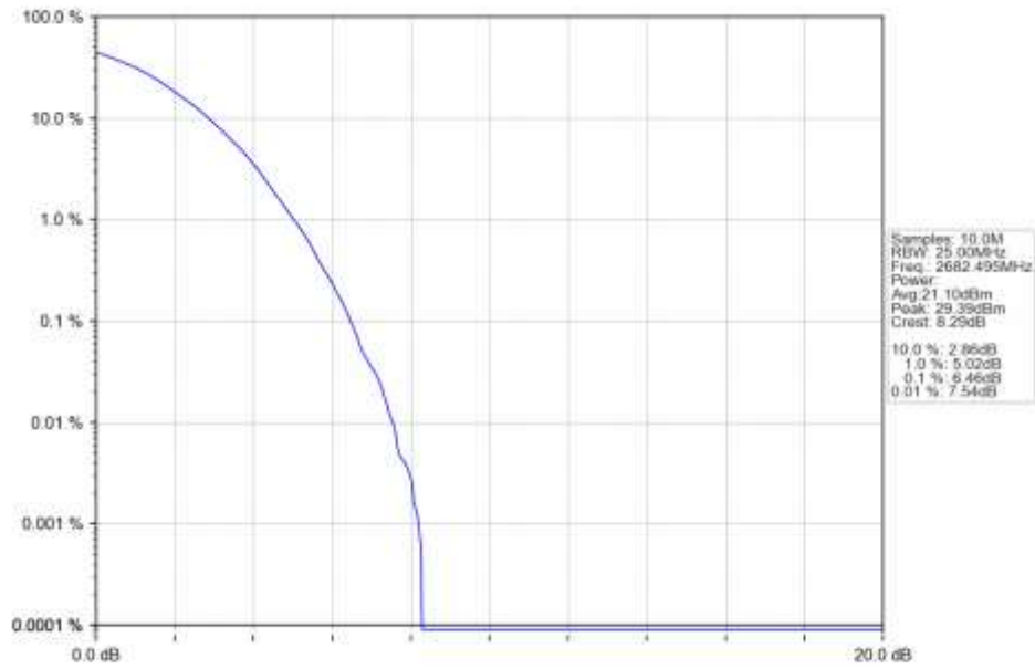
n41 15kHz SISO NTN 15MHz DFT-s-OFDM 256 QAM 2682.495MHz Outer Full Ant1
