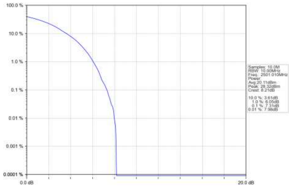
n41 30kHz SISO NTN 10MHz CP-OFDM 64 QAM 2501.01MHz Outer Full Ant1
