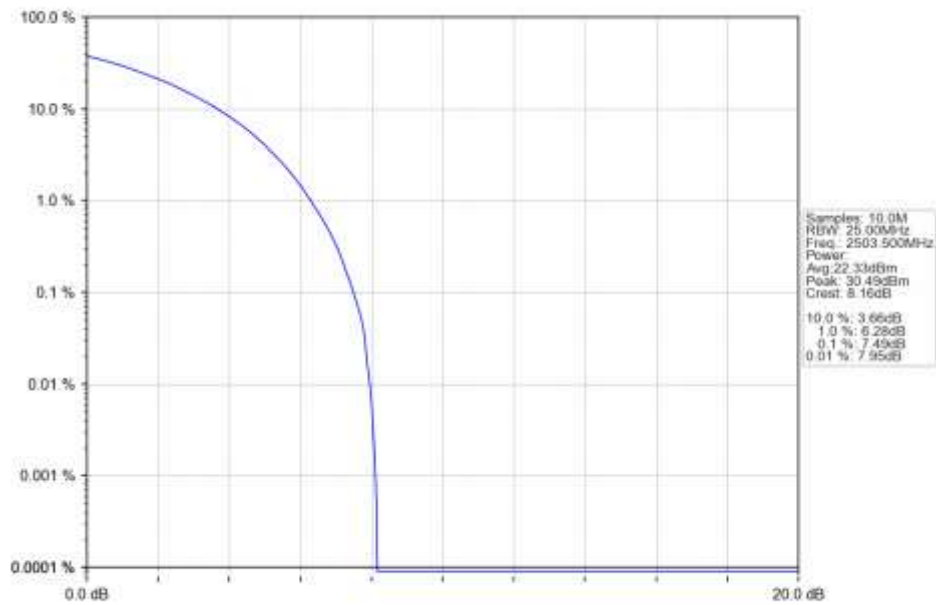
n41 15kHz SISO NTN 15MHz CP-OFDM QPSK 2503.5MHz Outer Full Ant1
