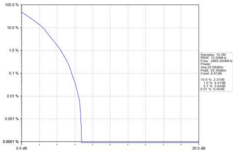
n41 15kHz SISO NTN 10MHz DFT-s-OFDM QPSK 2685MHz Outer Full Ant1
