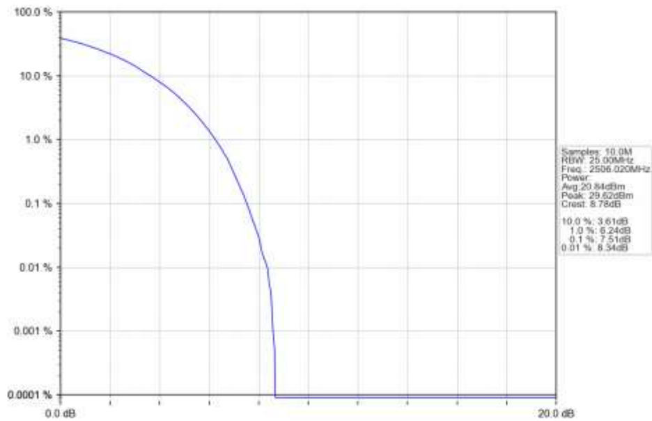
n41 30kHz SISO NTN 20MHz CP-OFDM 16 QAM 2506.02MHz Outer Full Ant1
