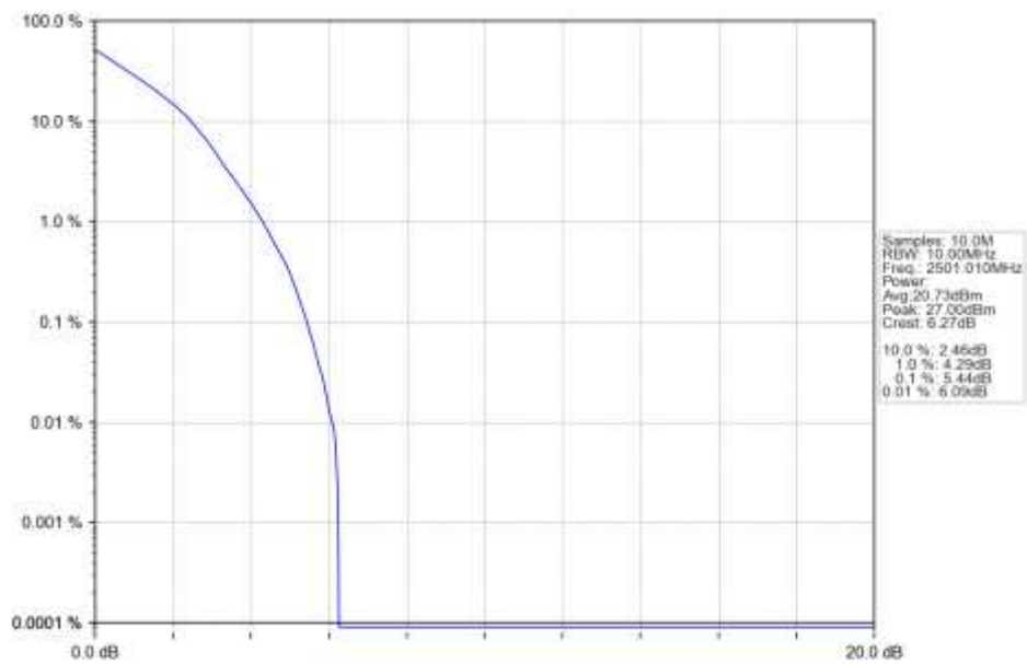
n41 30kHz SISO NTN 10MHz DFT-s-OFDM QPSK 2501.01MHz Outer Full Ant1
