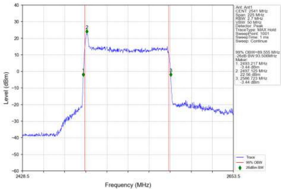
n41 30kHz SISO NTN 90MHz DFT-s-OFDM 64 QAM 2541MHz Outer Full Ant1
