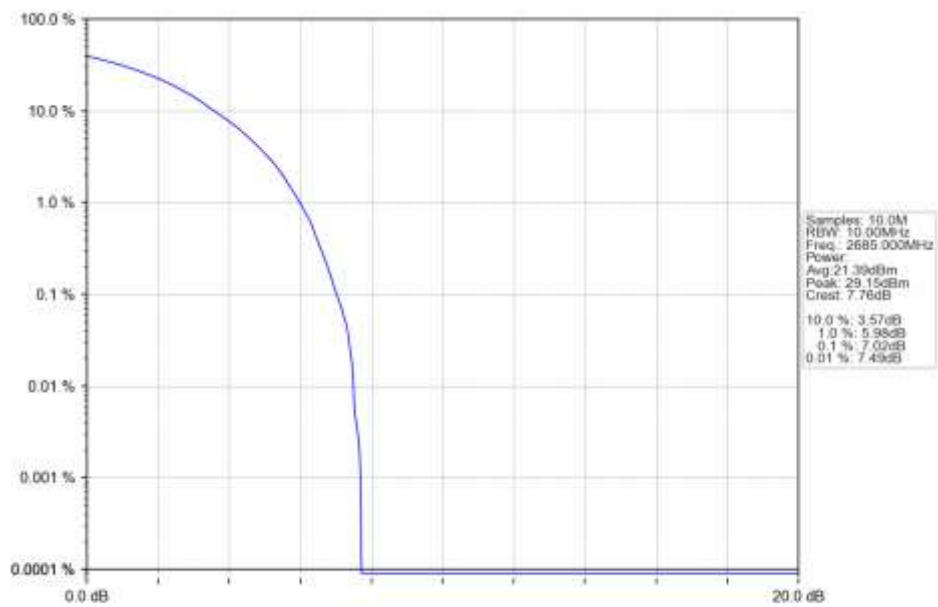
n41 30kHz SISO NTN 10MHz CP-OFDM 64 QAM 2685MHz Outer Full Ant1
