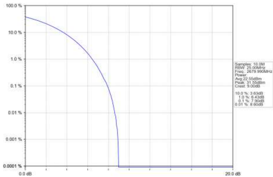
n41 15kHz SISO NTN 20MHz CP-OFDM QPSK 2679.99MHz Outer Full Ant1
