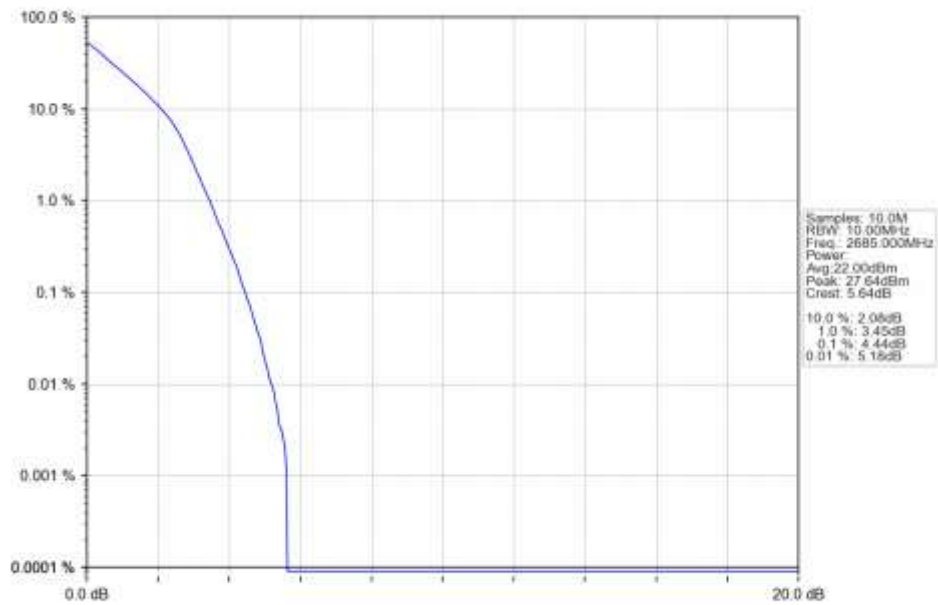
n41 30kHz SISO NTN 10MHz DFT-s-OFDM PI/2 BPSK 2685MHz Outer Full Ant1
