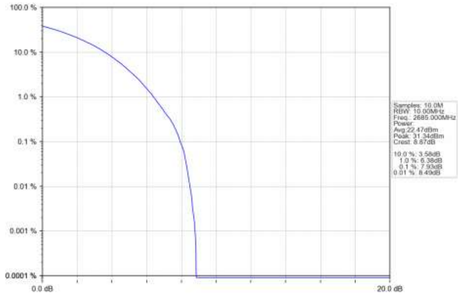
n41 15kHz SISO NTN 10MHz CP-OFDM 16 QAM 2685MHz Outer Full Ant1
