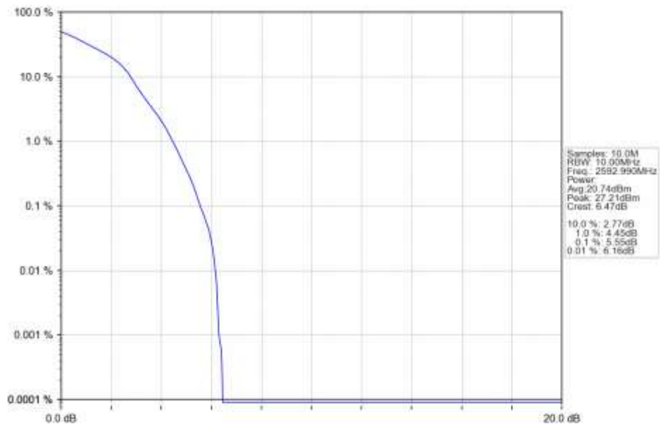
n41 30kHz SISO NTN 10MHz DFT-s-OFDM 16 QAM 2592.99MHz Outer Full Ant1
