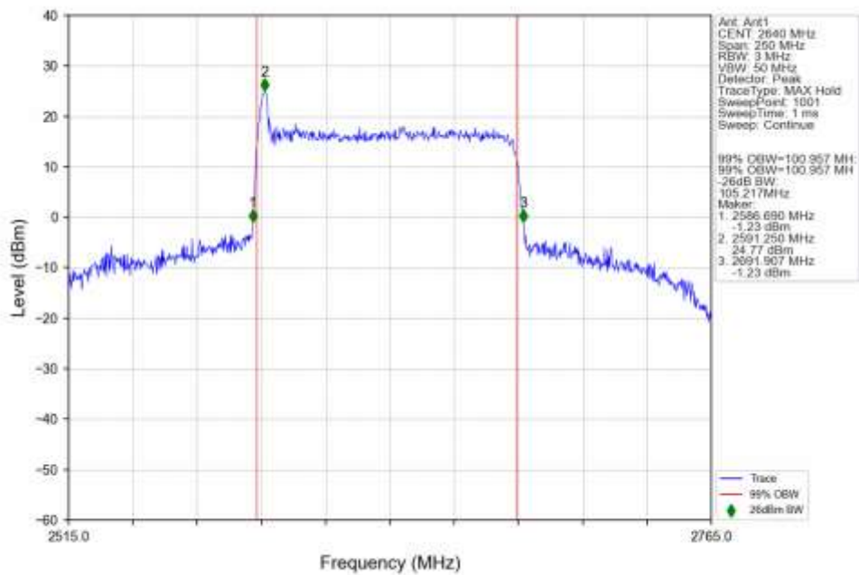
n41 30kHz SISO NTN 100MHz CP-OFDM QPSK 2640MHz Outer Full Ant1
