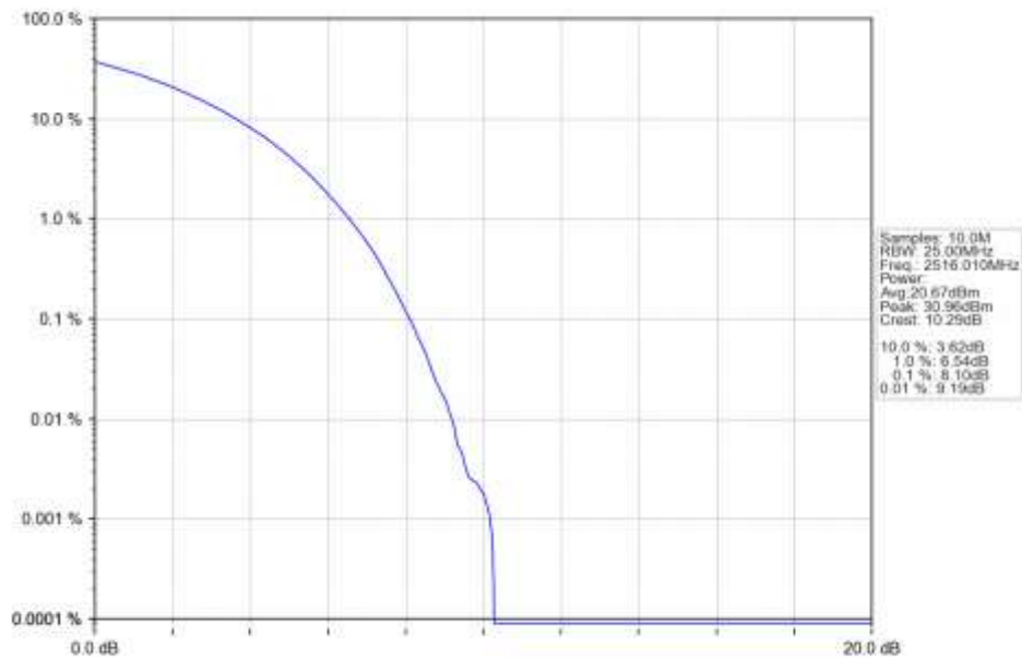
n41 15kHz SISO NTN 40MHz CP-OFDM 64 QAM 2516.01MHz Outer Full Ant1
