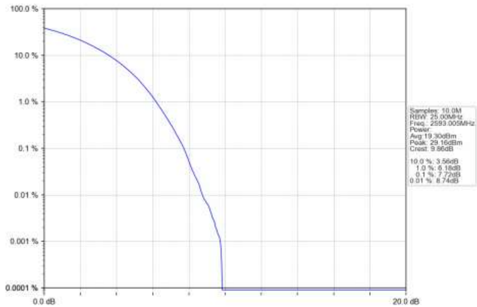
n41 15kHz SISO NTN 40MHz CP-OFDM QPSK 2593.005MHz Outer Full Ant1
