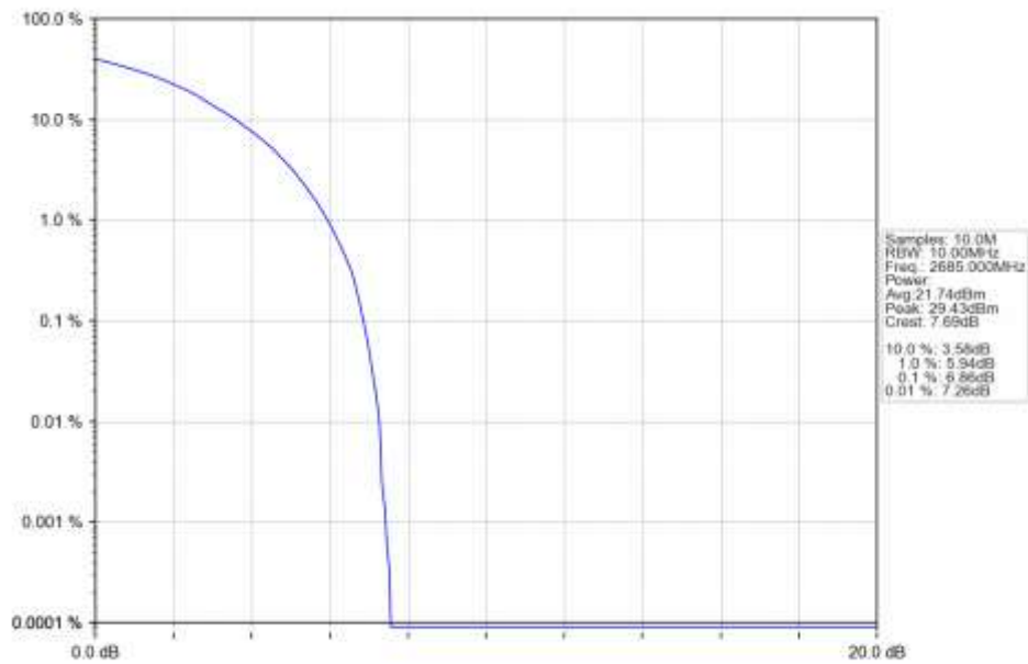
n41 30kHz SISO NTN 10MHz CP-OFDM QPSK 2685MHz Outer Full Ant1
