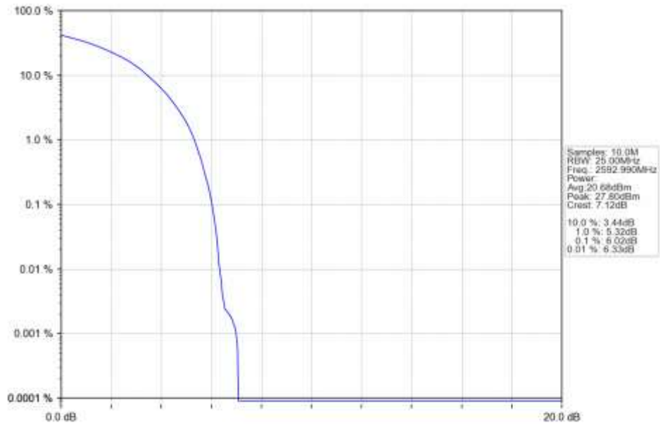
n41 30kHz SISO NTN 15MHz CP-OFDM QPSK 2592.99MHz Outer Full Ant1
