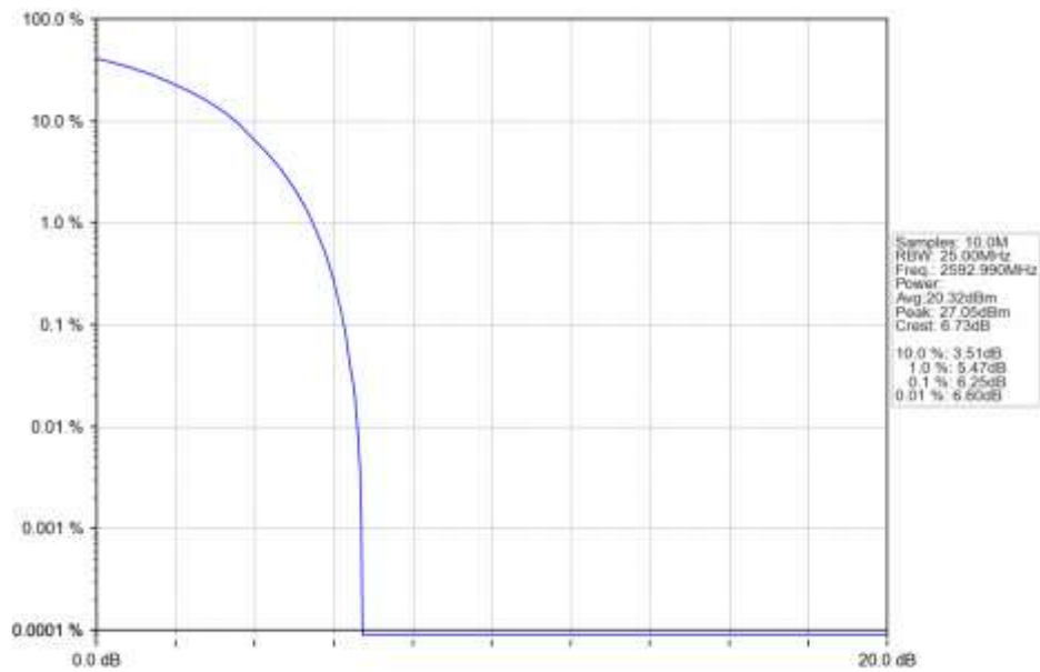
n41 30kHz SISO NTN 15MHz CP-OFDM 64 QAM 2592.99MHz Outer Full Ant1
