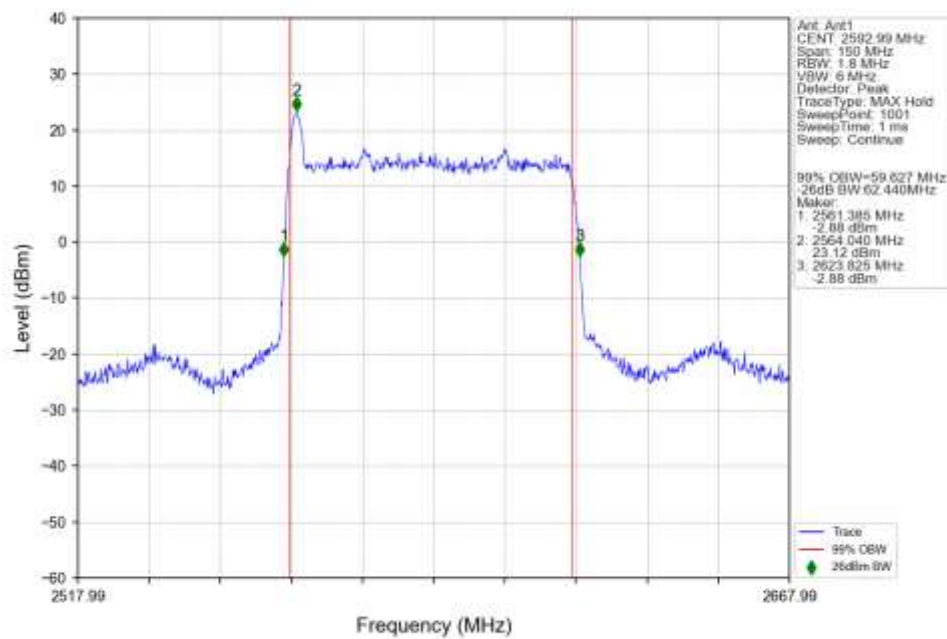
n41_30kHz_SISO_NTNV_60MHz_DFT-s-OFDM PI/2 BPSK_2592.99MHz_Outer_Full_Ant1
