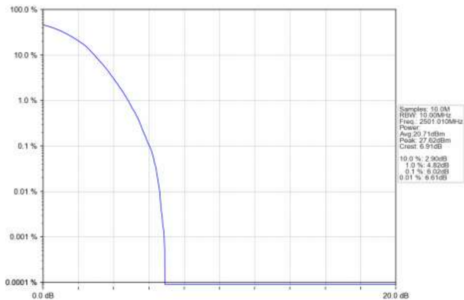
n41 30kHz SISO NTN 10MHz DFT-s-OFDM 64 QAM 2501.01MHz Outer Full Ant1
