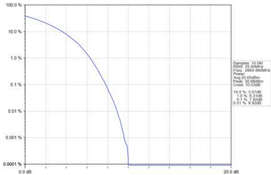
n41 15kHz SISO NTN 50MHz CP-OFDM 64 QAM 2664.99MHz Outer Full Ant1
