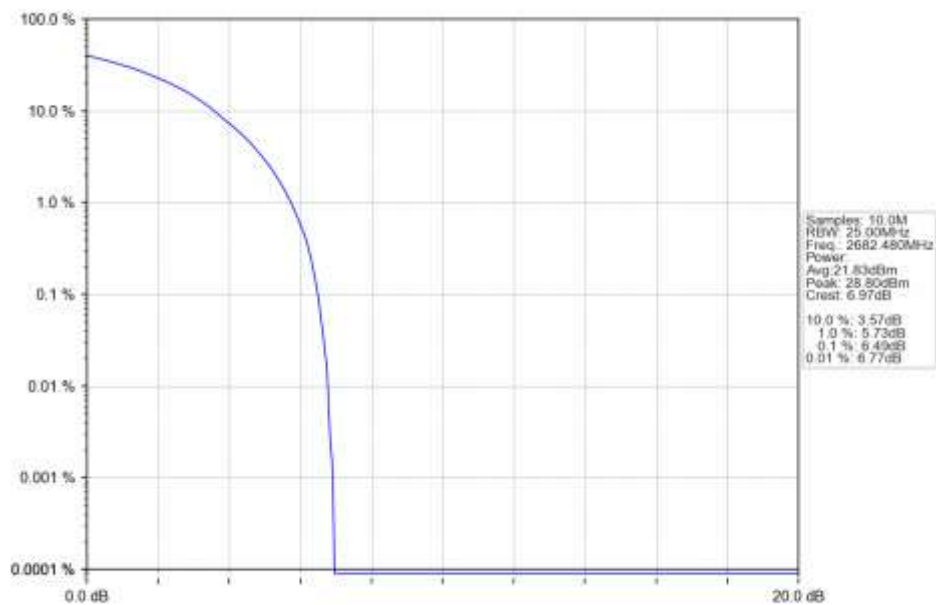
n41 30kHz SISO NTN 15MHz CP-OFDM 64 QAM 2682.48MHz Outer Full Ant1
