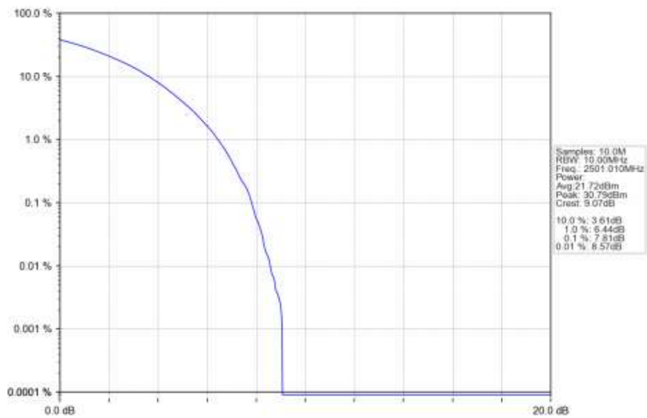
n41 15kHz SISO NTN 10MHz CP-OFDM 64 QAM 2501.01MHz Outer Full Ant1
