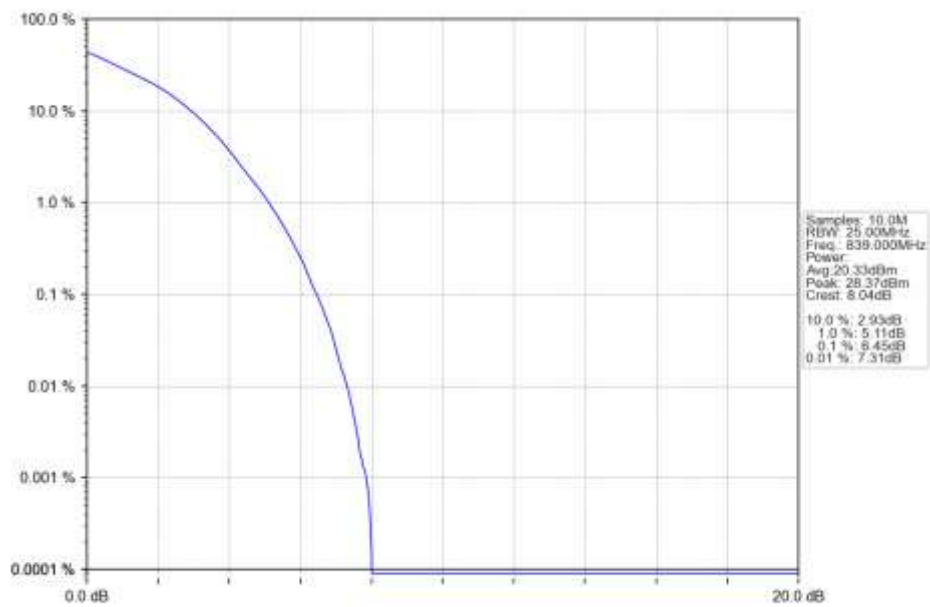
n5 15kHz SISO NTN 20MHz DFT-s-OFDM 16 QAM 839MHz Outer Full Ant1
