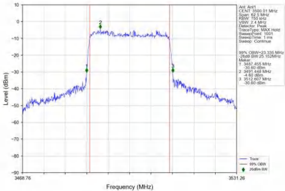
n78e 30kHz SISO NTN 25MHz CP-OFDM 64 QAM 3500.01MHz Outer Full Ant1
