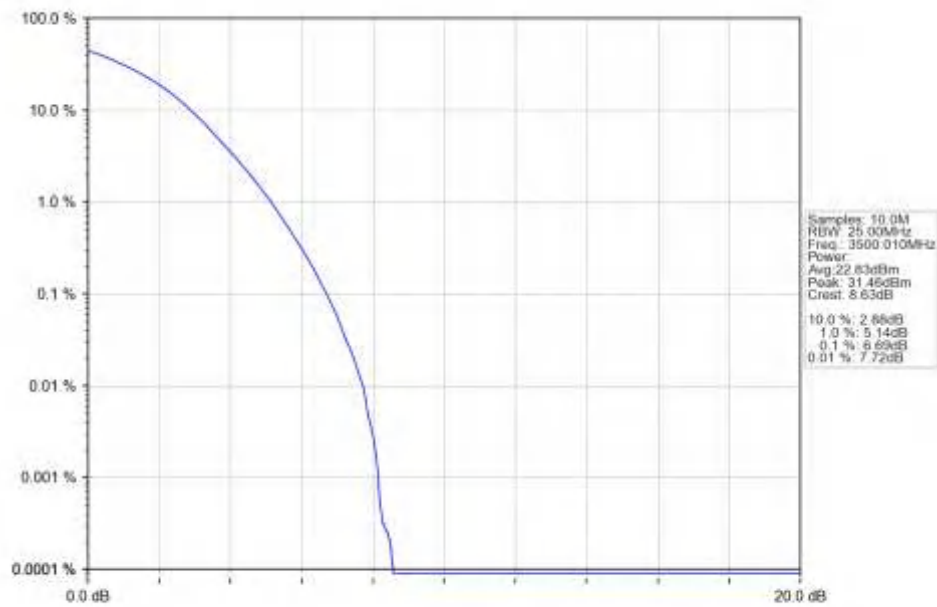
n78e 30kHz SISO NTN 20MHz DFT-s-OFDM 64 QAM 3500.01MHz Outer Full Ant1
