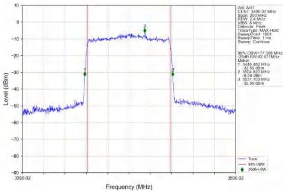
n78e 30kHz SISO NTN 80MHz DFT-s-OFDM 256 QAM 3490.02MHz Outer Full Ant1
