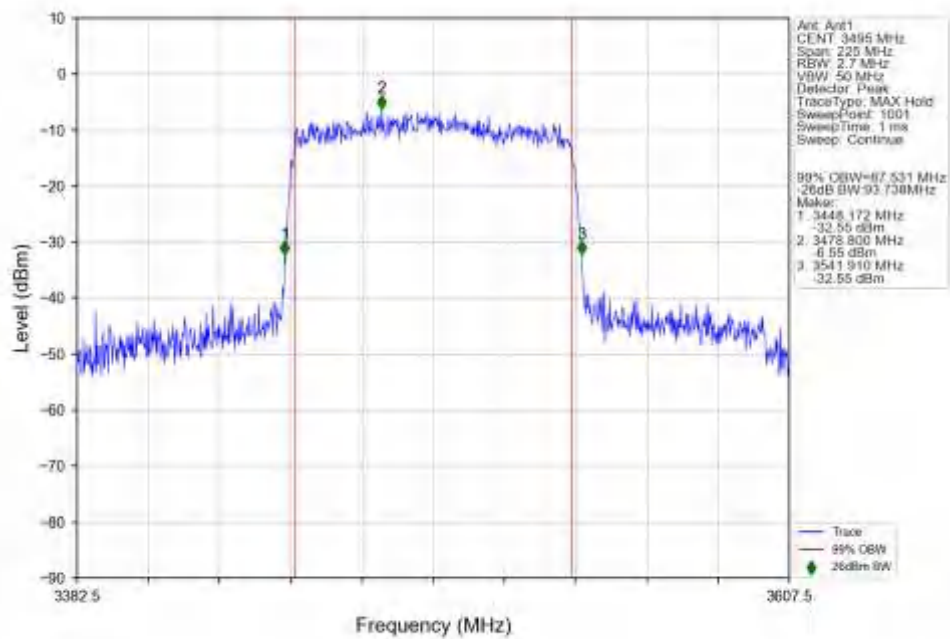
n78e 30kHz SISO NTV 90MHz CP-OFDM 16 QAM 3495MHz Outer Full Ant1
