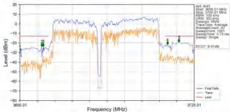
n78a 30kHz SISO NTN 20MHz DFT-s-OFDM QPSK 3710.01MHz Outer Full Ant1
