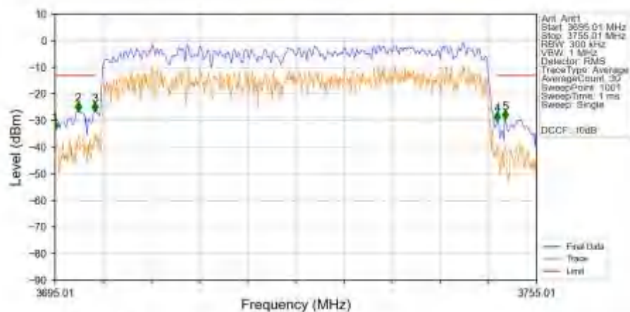
n78a_30kHz_SISO_NTNV_50MHz_CP-OFDM_QPSK_3725.01MHz_Outer_Full_Ant1
