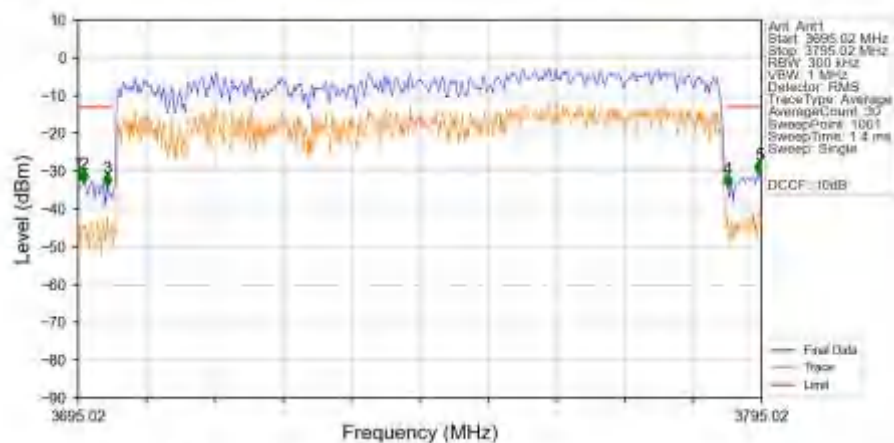
n78a_30kHz_SISO_NTNV_90MHz_CP-OFDM_QPSK_3745.02MHz_Outer_Full_Ant1
