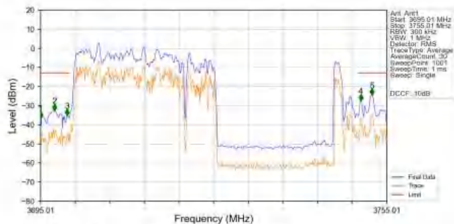
n78a 30kHz SISO NTN 50MHz DFT-s-OFDM QPSK 3725.01MHz Outer Full Ant1
