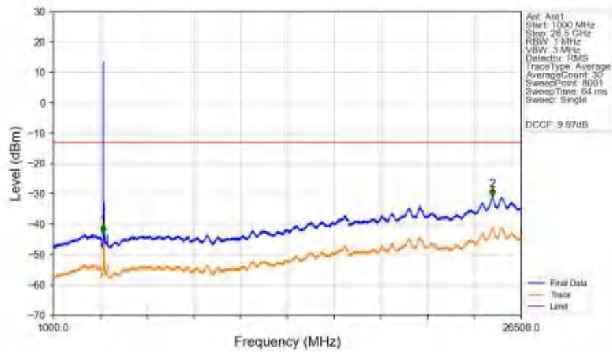
n78a_30kHz_SISO_NTNV_70MHz_DFT-s-OFDM_QPSK_3750MHz_Edge_1RB_Left_Ant1
