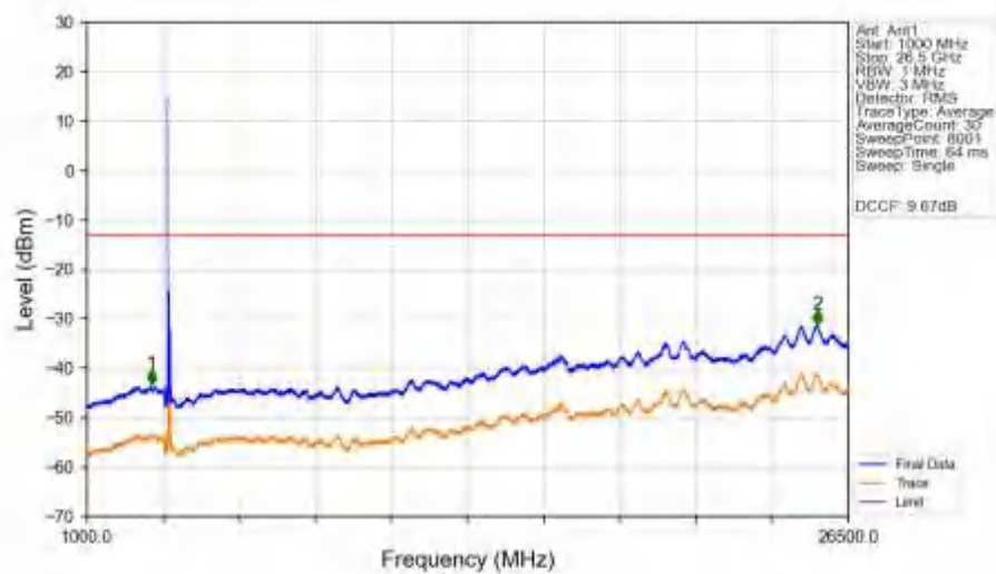
n78a_30kHz_SISO_NTNV_50MHz_CP-OFDM_QPSK_3725.01MHz_Edge_1RB_Left_Ant1
