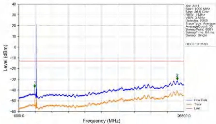
n78a_30kHz_SISO_NTNV_25MHz_DFT-s-OFDM_QPSK_3712.5MHz_Edge_1RB_Left_Ant1
