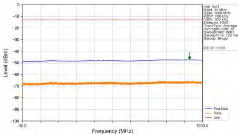
n78a_30kHz_SISO_NTNV_25MHz_DFT-s-OFDM_QPSK_3750MHz_Edge_1RB_Left_Ant1
