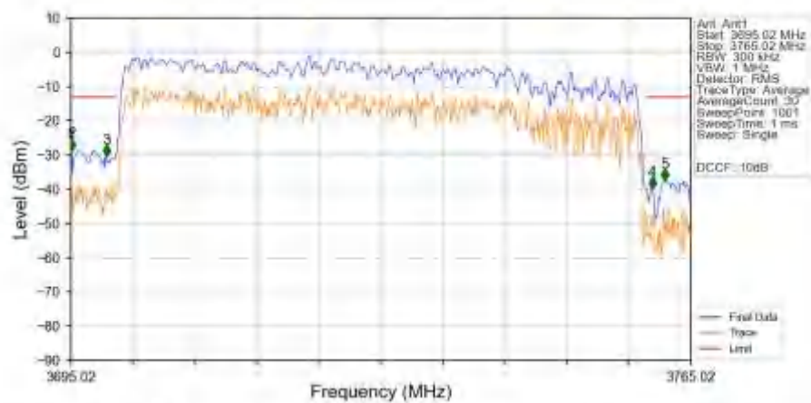
n78a_30kHz_SISO_NTNV_60MHz_CP-OFDM_QPSK_3730.02MHz_Outer_Full_Ant1
