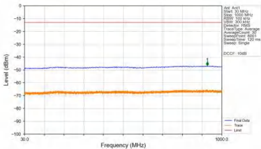
n78a_30kHz_SISO_NTNV_50MHz_DFT-s-OFDM_QPSK_3774.99MHz_Edge_1RB_Right_Ant1
