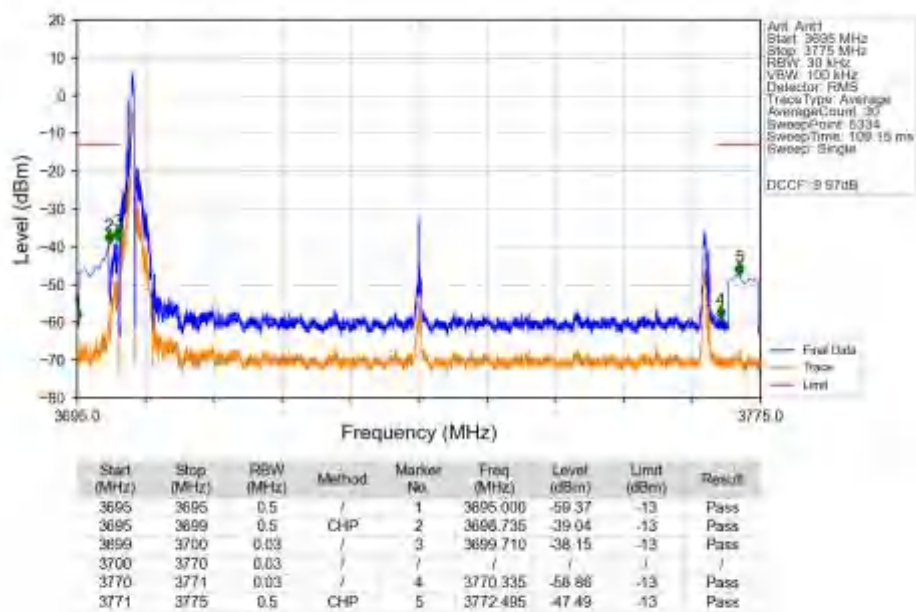
n78a_30kHz_SISO_NTNV_70MHz_CP-OFDM_QPSK_3735MHz_Inner_1RB_Left_Ant1
