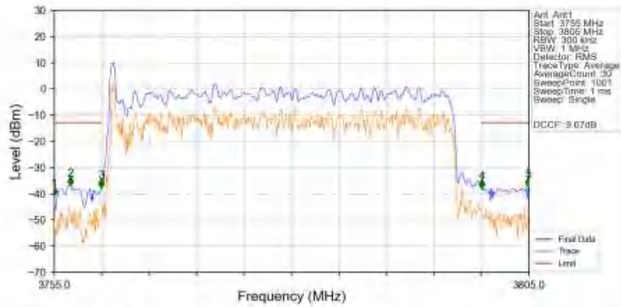
n78a 30kHz SISO NTN 40MHz DFT-s-OFDM QPSK 3780MHz Outer Full Ant1
