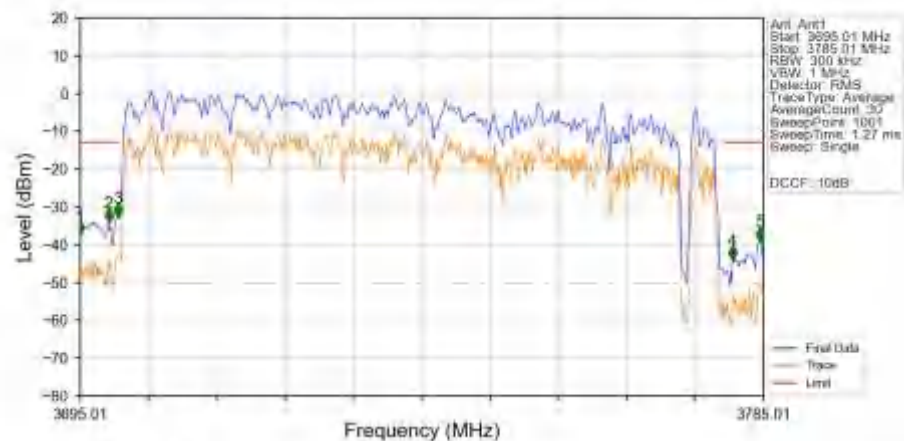
n78a 30kHz SISO NTN 80MHz DFT-s-OFDM QPSK 3740.01MHz Outer Full Ant1
