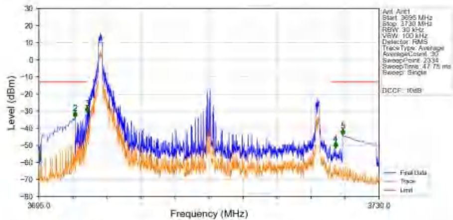
n78a_30kHz_SISO_NTNV_25MHz_CP-OFDM_QPSK_3712.5MHz_Inner_1RB_Left_Ant1
