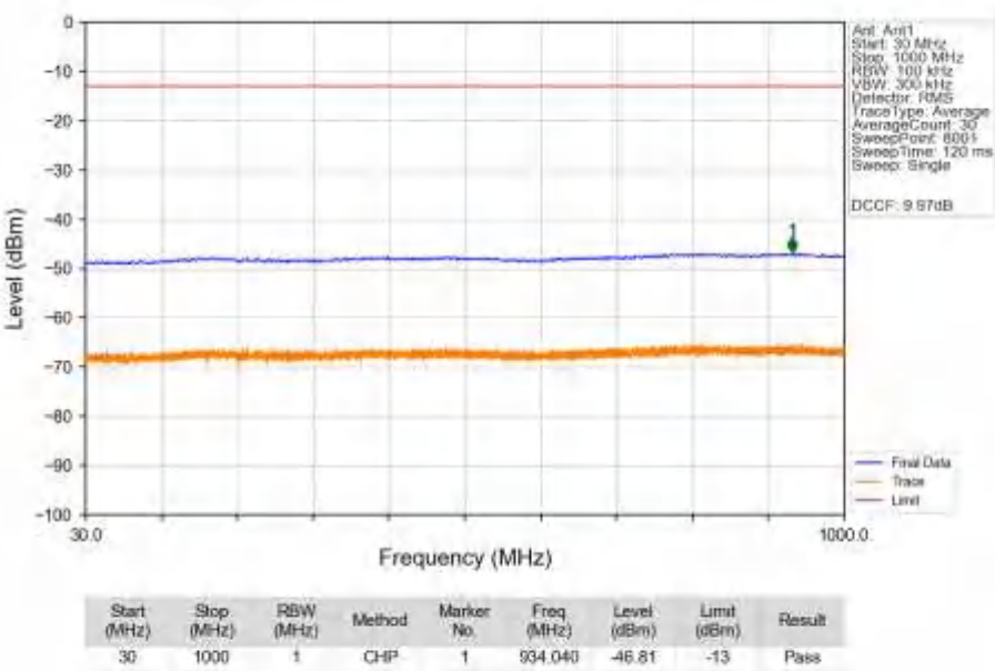
n78a_30kHz_SISO_NTNV_70MHz_CP-OFDM_QPSK_3750MHz_Edge_1RB_Left_Ant1
