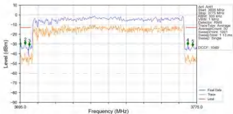
n78a_30kHz_SISO_NTNV_70MHz_CP-OFDM_QPSK_3735MHz_Outer_Full_Ant1
