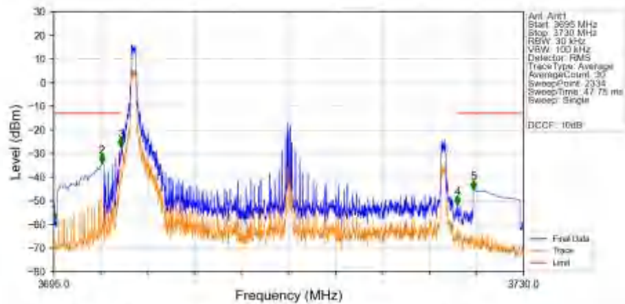
n78a_30kHz_SISO_NTNV_25MHz_CP-OFDM_QPSK_3712.5MHz_Edge_1RB_Left_Ant1
