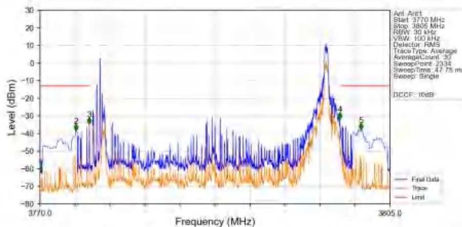
n78a 30kHz SISO NTN 25MHz DFT-s-OFDM QPSK 3787.5MHz Inner_1RB_Right_Ant1
