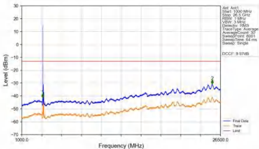
n78a_30kHz_SISO_NTNV_70MHz_DFT-s-OFDM_QPSK_3735MHz_Edge_1RB_Left_Ant1
