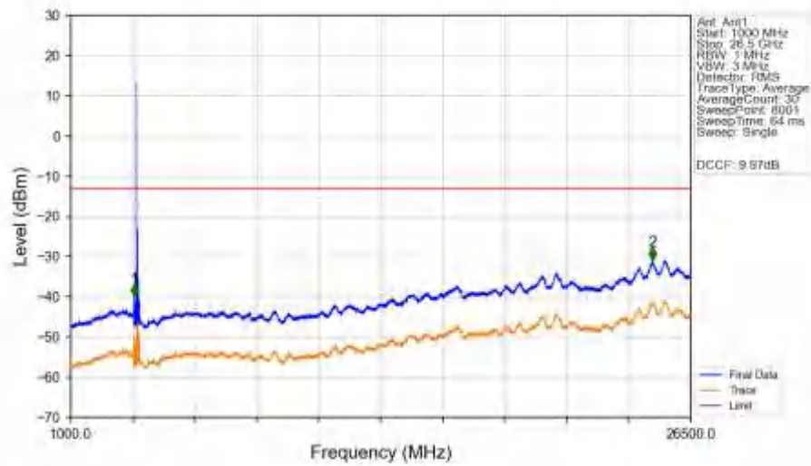
n78a_30kHz_SISO_NTNV_40MHz_DFT-s-OFDM_QPSK_3720MHz_Edge_1RB_Left_Ant1
