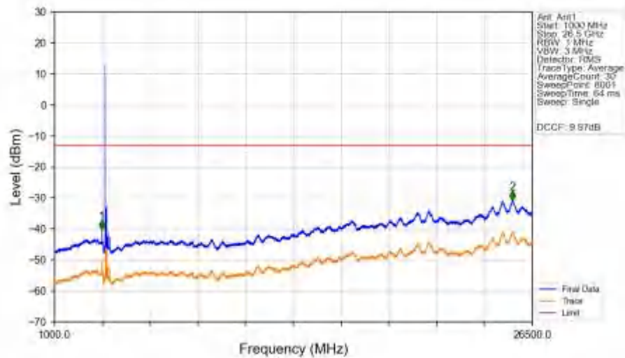
n78a_30kHz_SISO_NTNV_90MHz_CP-OFDM_QPSK_3745.02MHz_Edge_1RB_Left_Ant1
