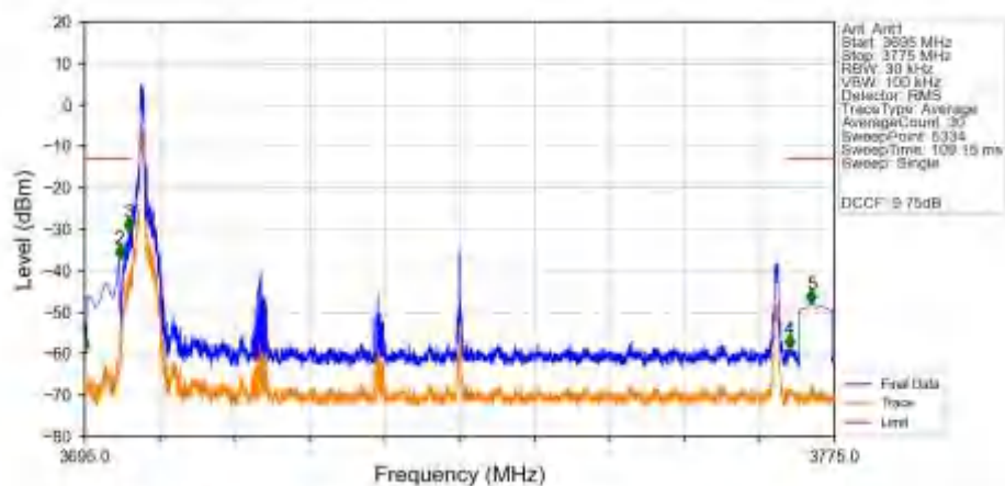
n78a_30kHz_SISO_NTNV_70MHz_CP-OFDM_QPSK_3735MHz_Edge_1RB_Left_Ant1
