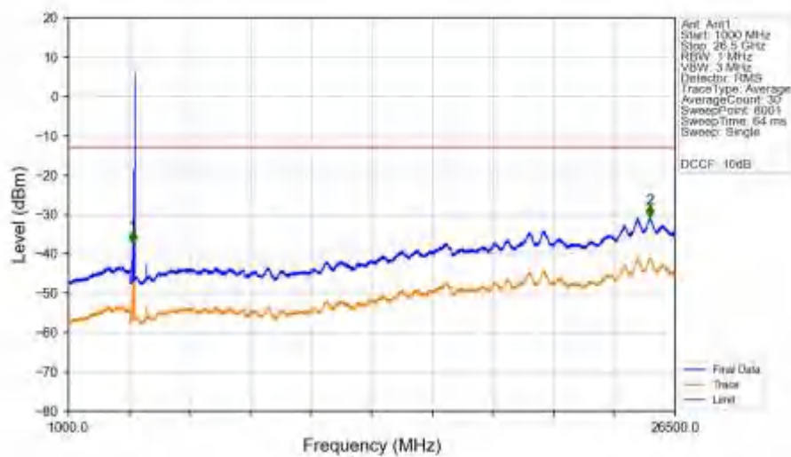
n78a_30kHz_SISO_NTNV_50MHz_DFT-s-OFDM_QPSK_3774.99MHz_Edge_1RB_Right_Ant1
