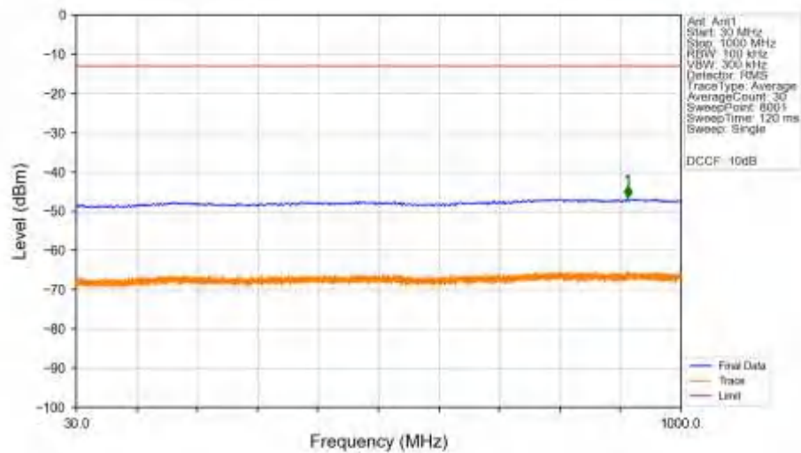
n78a_30kHz_SISO_NTNV_80MHz_DFT-s-OFDM_QPSK_3759.99MHz_Edge_1RB_Right_Ant1
