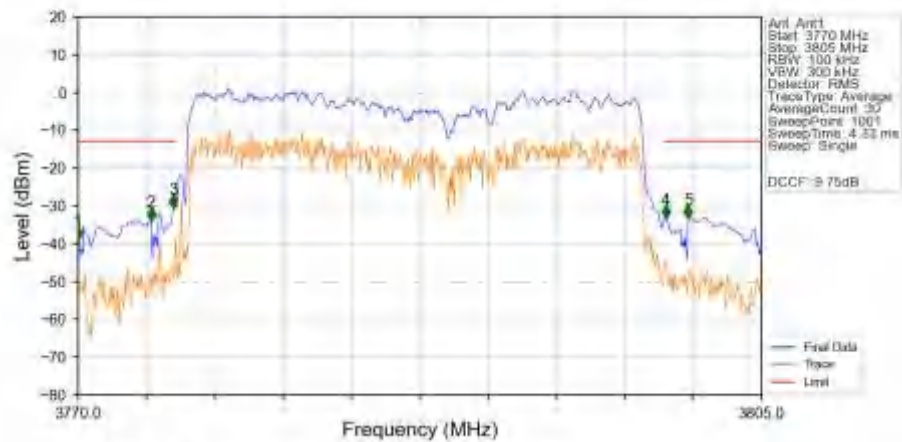
n78a 30kHz SISO NTN 25MHz DFT-s-OFDM QPSK 3787.5MHz Outer_Full_Ant1
