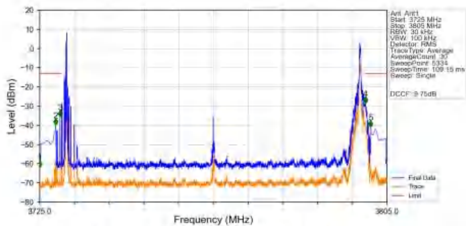
n78a_30kHz_SISO_NTNV_70MHz_DFT-s-OFDM_QPSK_3765MHz_Edge_1RB_Right_Ant1
