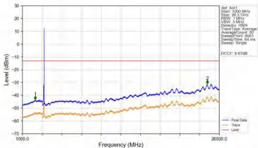
n78a_30kHz_SISO_NTNV_60MHz_DFT-s-OFDM_QPSK_3769.98MHz_Edge_1RB_Right_Ant1
