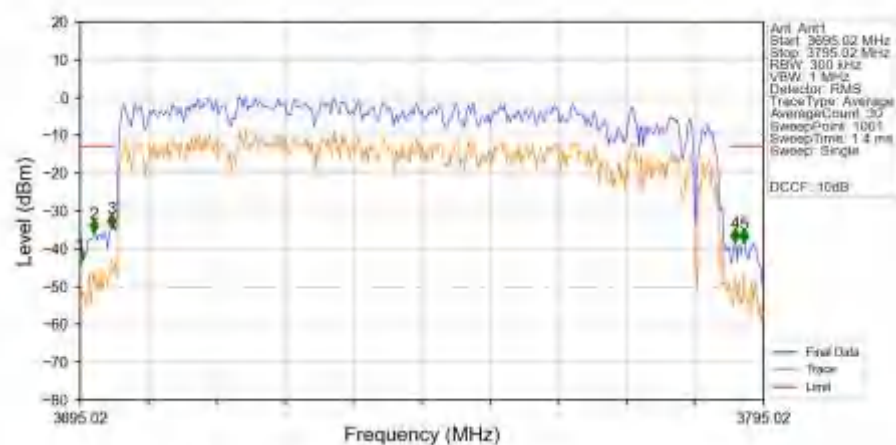
n78a 30kHz SISO NTN 90MHz DFT-s-OFDM QPSK 3745.02MHz Outer Full Ant1
