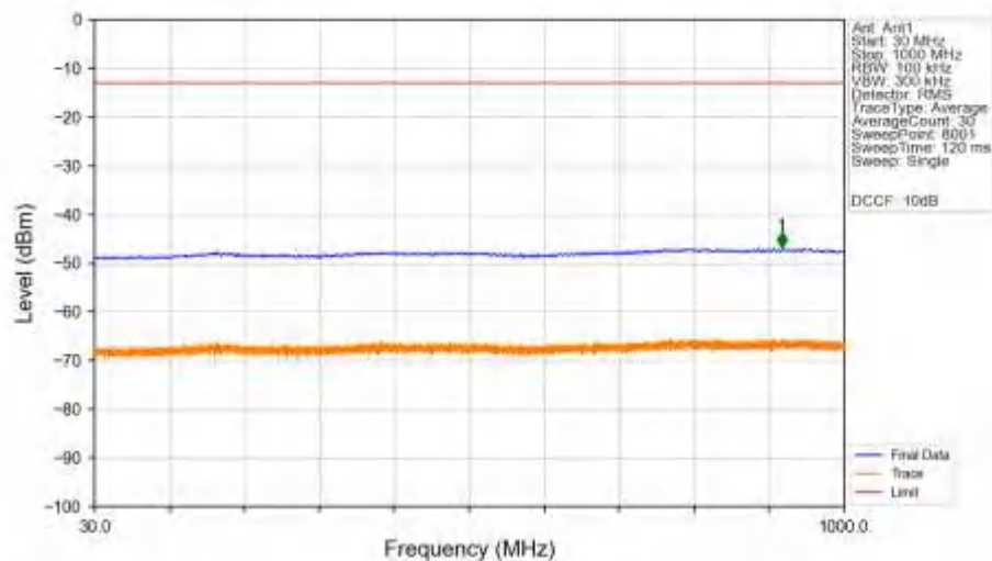
n78a_30kHz_SISO_NTNV_25MHz_CP-OFDM_QPSK_3750MHz_Edge_1RB_Left_Ant1
