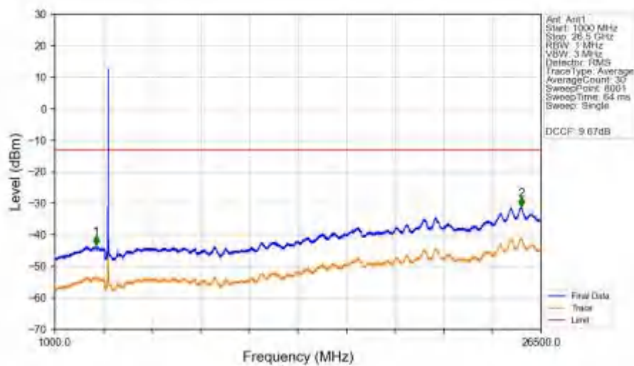
n78a_30kHz_SISO_NTNV_30MHz_DFT-s-OFDM_QPSK_3784.98MHz_Edge_1RB_Right_Ant1
