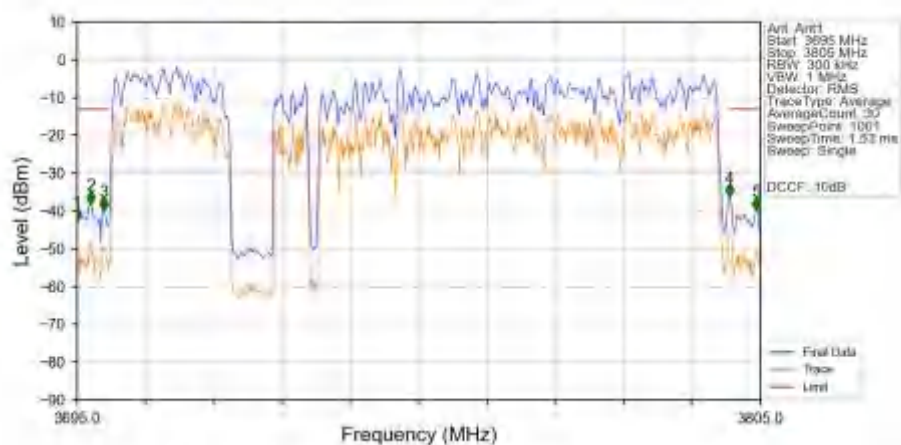
n78a_30kHz_SISO_NTNV_100MHz_DFT-s-OFDM_QPSK_3750MHz_Outer_Full_Ant1
