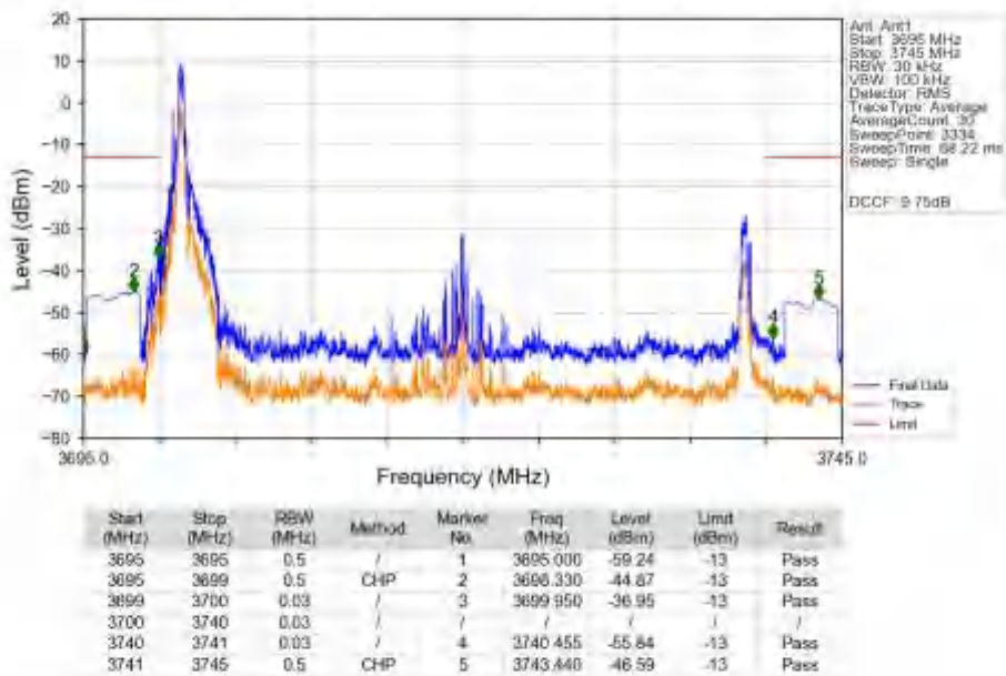
n78a_30kHz_SISO_NTNV_40MHz_CP-OFDM_QPSK_3720MHz_Inner_1RB_Left_Ant1
