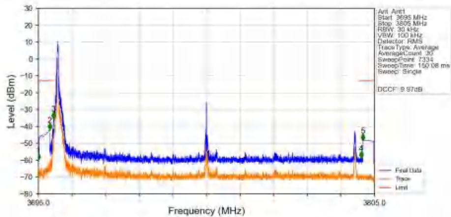
n78a_30kHz_SISO_NTNV_100MHz_DFT-s-OFDM_QPSK_3750MHz_Inner_1RB_Left_Ant1
