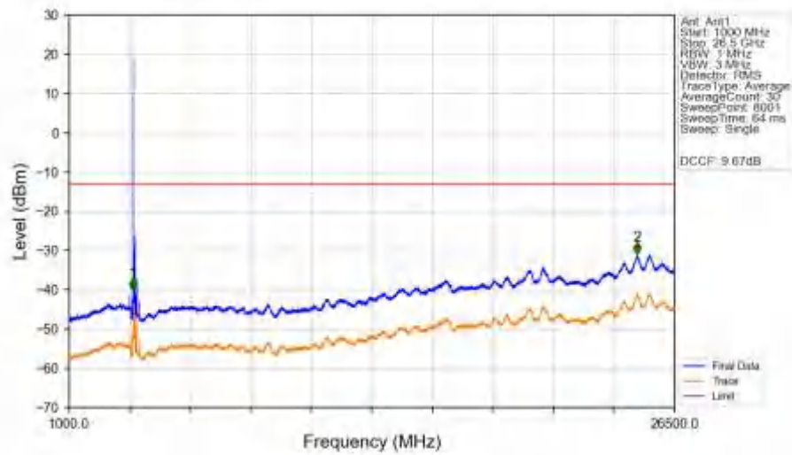
n78a_30kHz_SISO_NTNV_80MHz_CP-OFDM_QPSK_3740.01MHz_Edge_1RB_Left_Ant1
