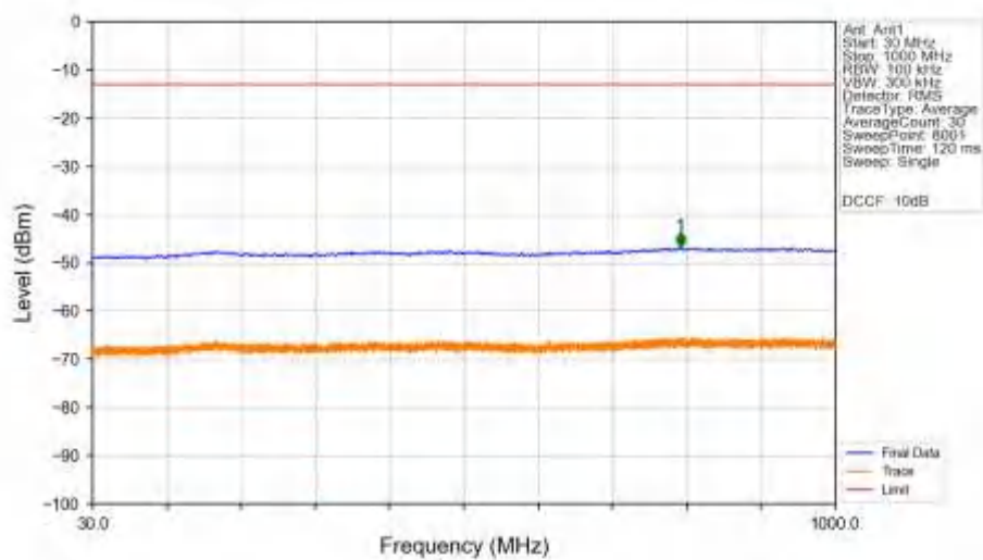
n78a_30kHz_SISO_NTNV_40MHz_DFT-s-OFDM_QPSK_3780MHz_Edge_1RB_Right_Ant1
