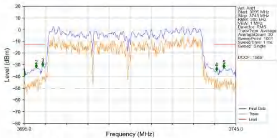
n78a_30kHz_SISO_NTNV_40MHz_DFT-s-OFDM_QPSK_3720MHz_Outer_Full_Ant1
