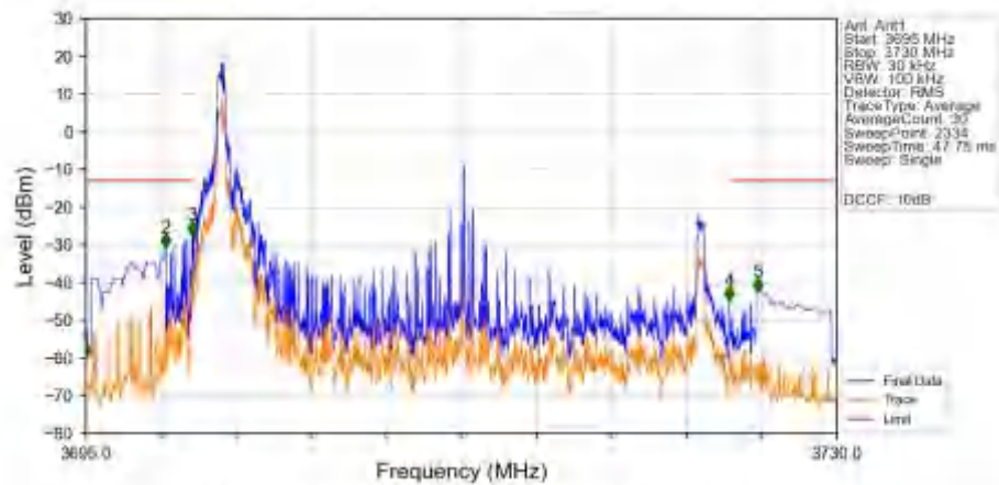
n78a_30kHz_SISO_NTNV_25MHz_DFT-s-OFDM_QPSK_3712.5MHz_Inner_1RB_Left_Ant1
