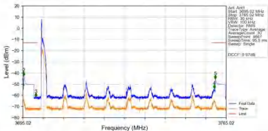
n78a 30kHz SISO NTN 60MHz DFT-s-OFDM QPSK 3730.02MHz Inner 1RB Left Ant1
