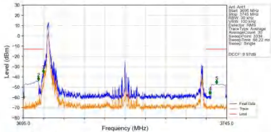
n78a_30kHz_SISO_NTNV_40MHz_CP-OFDM_QPSK_3720MHz_Edge_1RB_Left_Ant1
