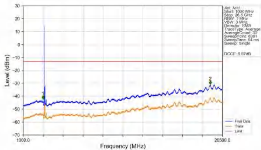
n78a 30kHz SISO NTN 90MHz DFT-s-OFDM QPSK 3745.02MHz Edge 1RB Left Ant1
