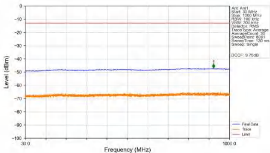
n78a_30kHz_SISO_NTNV_70MHz_CP-OFDM_QPSK_3735MHz_Edge_1RB_Left_Ant1
