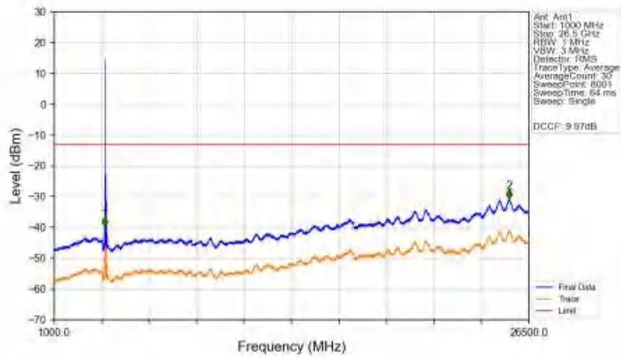
n78a_30kHz_SISO_NTNV_40MHz_CP-OFDM_QPSK_3750MHz_Edge_1RB_Left_Ant1
