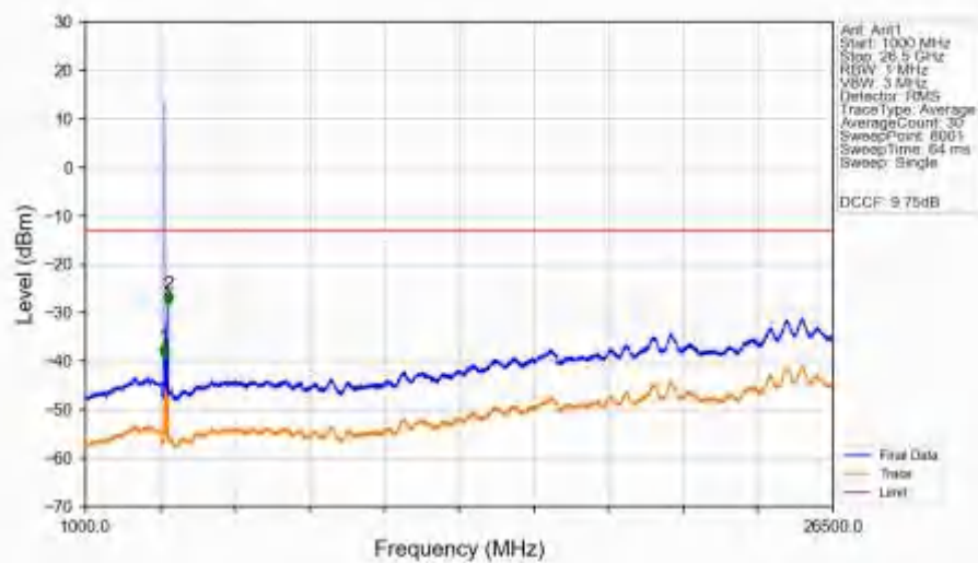
n78a_30kHz_SISO_NTNV_70MHz_CP-OFDM_QPSK_3735MHz_Edge_1RB_Left_Ant1
