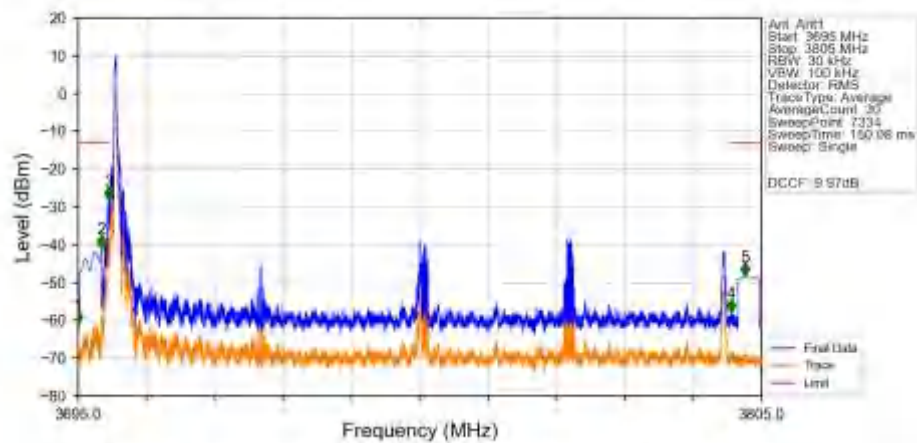
n78a_30kHz_SISO_NTNV_100MHz_CP-OFDM_QPSK_3750MHz_Edge_1RB_Left_Ant1
