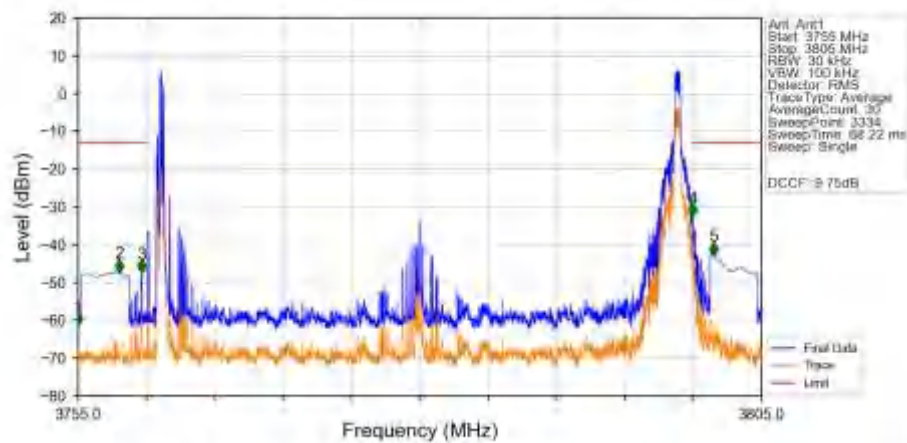
n78a_30kHz_SISO_NTNV_40MHz_CP-OFDM_QPSK_3780MHz_Edge_1RB_Right_Ant1
