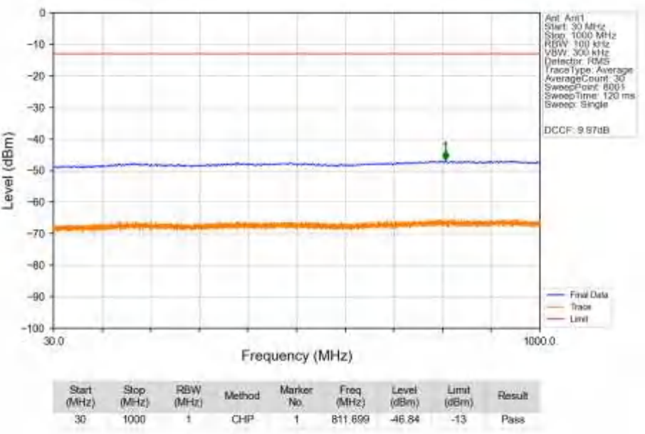
n78a_30kHz_SISO_NTNV_40MHz_CP-OFDM_QPSK_3750MHz_Edge_1RB_Left_Ant1
