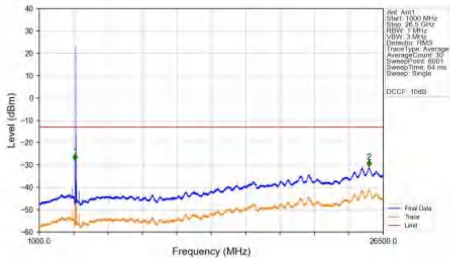
n78a_30kHz_SISO_NTNV_20MHz_CP-OFDM_QPSK_3710.01MHz_Edge_1RB_Left_Ant1
