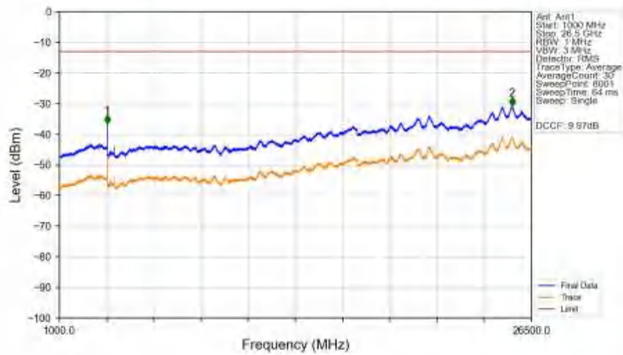
n78a_30kHz_SISO_NTNV_60MHz_CP-OFDM_QPSK_3730.02MHz_Edge_1RB_Left_Ant1
