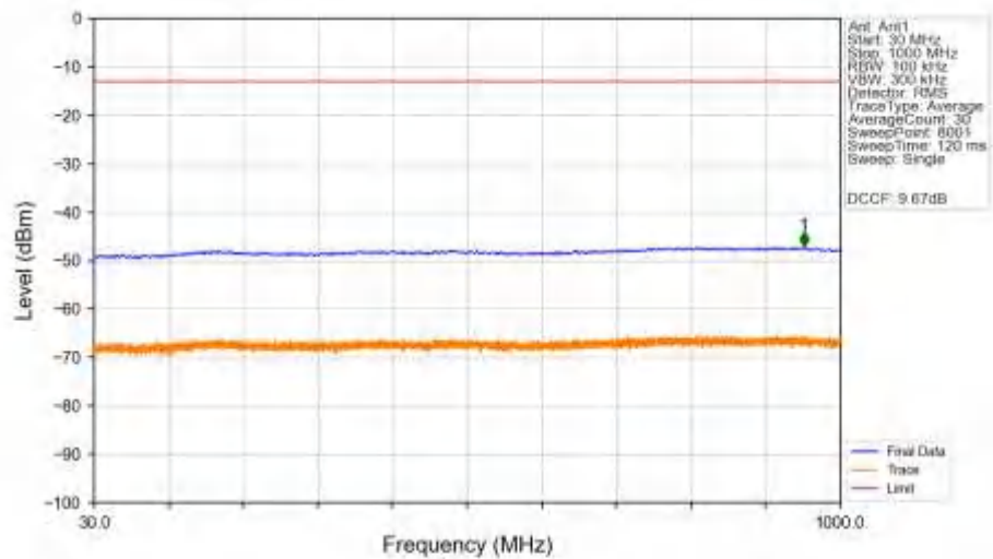
n78a_30kHz_SISO_NTNV_60MHz_DFT-s-OFDM_QPSK_3769.98MHz_Edge_1RB_Right_Ant1
