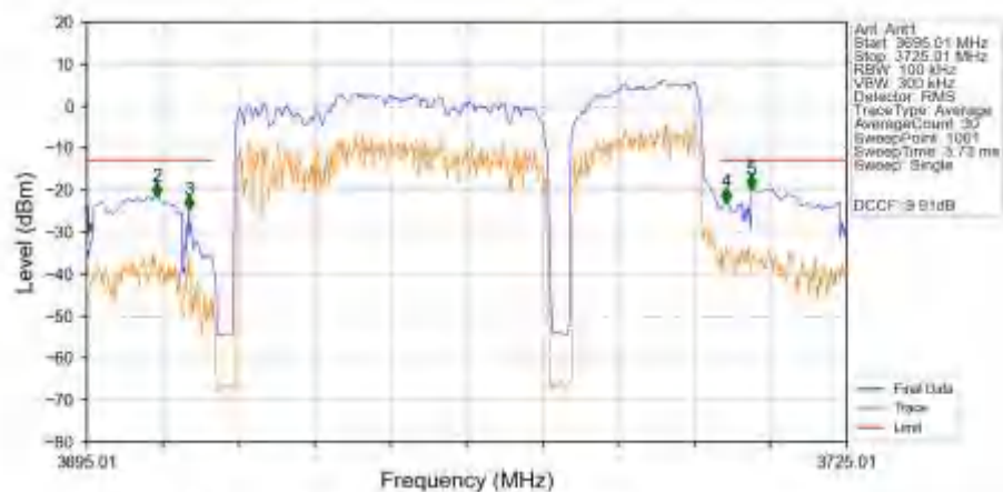
n78a_30kHz_SISO_NTNV_20MHz_CP-OFDM_QPSK_3710.01MHz_Outer_Full_Ant1
