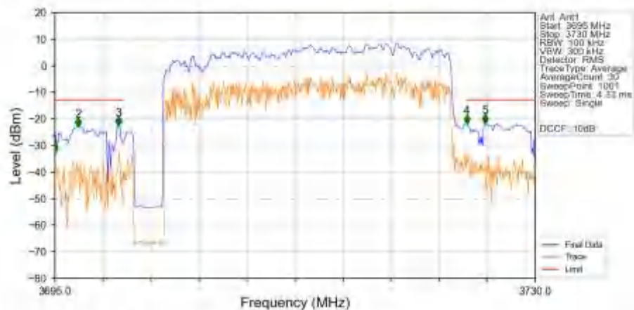
n78a_30kHz_SISO_NTNV_25MHz_DFT-s-OFDM_QPSK_3712.5MHz_Outer_Full_Ant1
