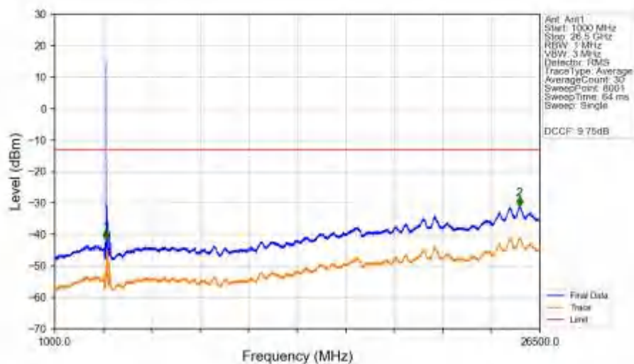
n78a_30kHz_SISO_NTNV_100MHz_DFT-s-OFDM_QPSK_3750MHz_Edge_1RB_Left_Ant1
