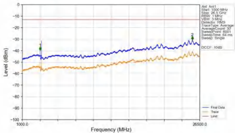
n78a_30kHz_SISO_NTNV_70MHz_CP-OFDM_QPSK_3765MHz_Edge_1RB_Right_Ant1
