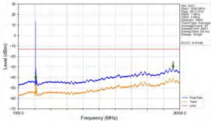
n78a_30kHz_SISO_NTNV_80MHz_DFT-s-OFDM_QPSK_3750MHz_Edge_1RB_Left_Ant1
