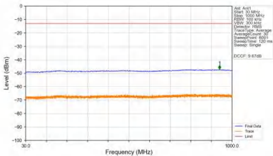
n78a_30kHz_SISO_NTNV_30MHz_DFT-s-OFDM_QPSK_3784.98MHz_Edge_1RB_Right_Ant1
