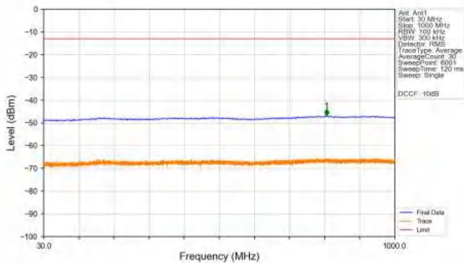
n78a_30kHz_SISO_NTNV_25MHz_CP-OFDM_QPSK_3712.5MHz_Edge_1RB_Left_Ant1
