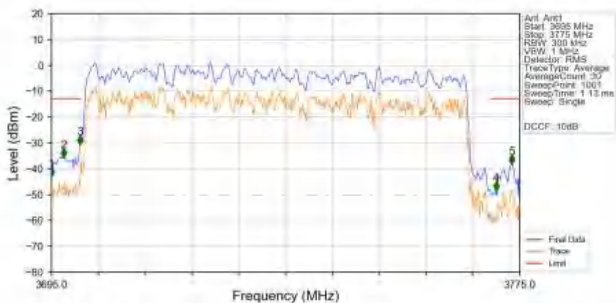
n78a_30kHz_SISO_NTNV_70MHz_DFT-s-OFDM_QPSK_3735MHz_Outer_Full_Ant1
