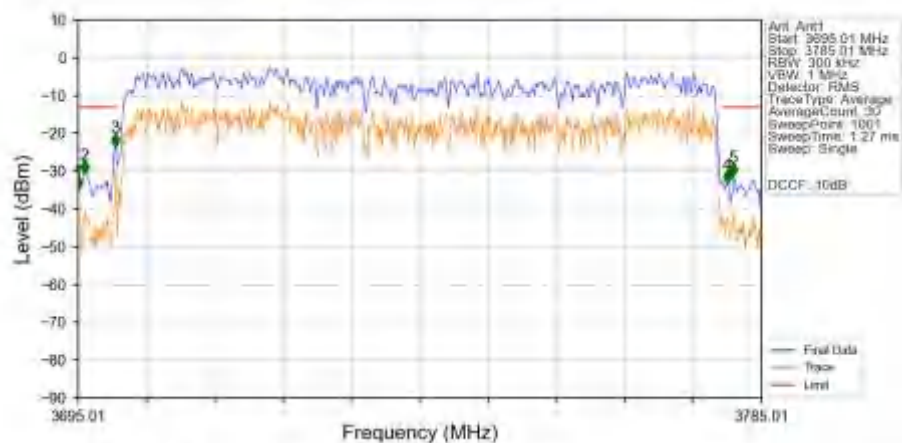
n78a_30kHz_SISO_NTNV_80MHz_CP-OFDM_QPSK_3740.01MHz_Outer_Full_Ant1
