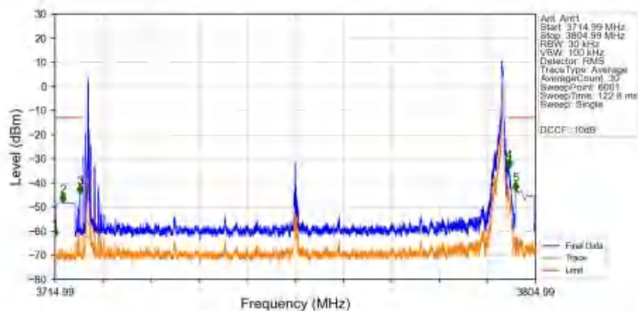
n78a_30kHz_SISO_NTNV_80MHz_DFT-s-OFDM_QPSK_3759.99MHz_Edge_1RB_Right_Ant1
