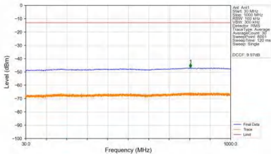
n78a_30kHz_SISO_NTNV_40MHz_CP-OFDM_QPSK_3720MHz_Edge_1RB_Left_Ant1
