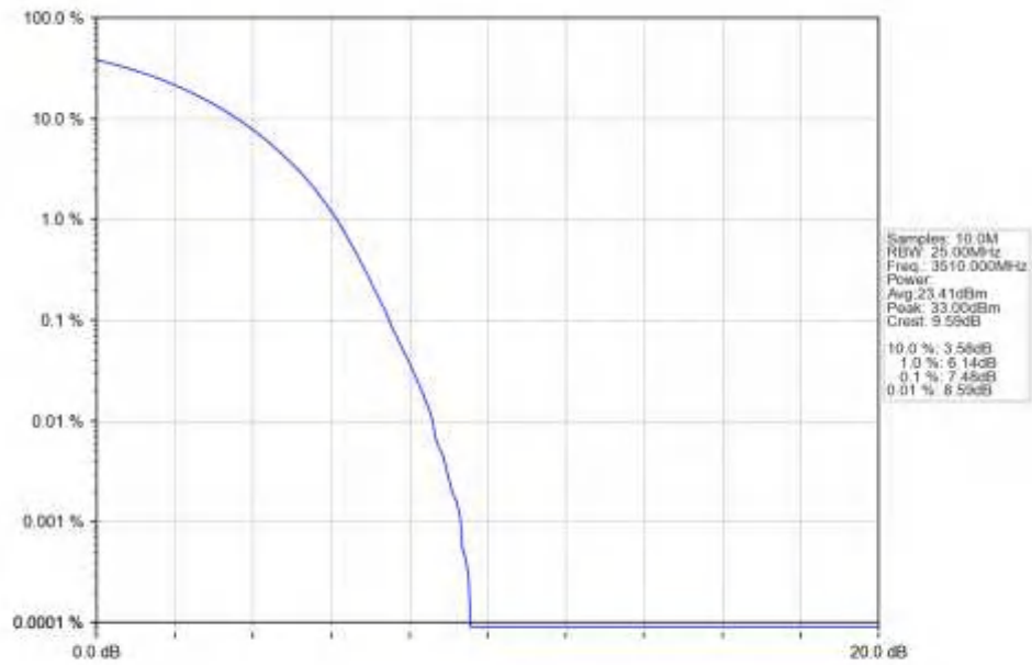
n77d 30kHz SISO_NTNV_80MHz DFT-s-OFDM QPSK 3510MHz_Outer_Full_Ant1
