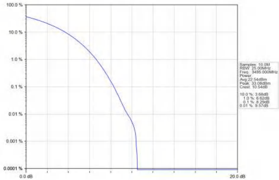
n77d_30kHz_SISO_NTNV_90MHz_CP-OFDM_QPSK_3495MHz_Outer_Full_Ant1
