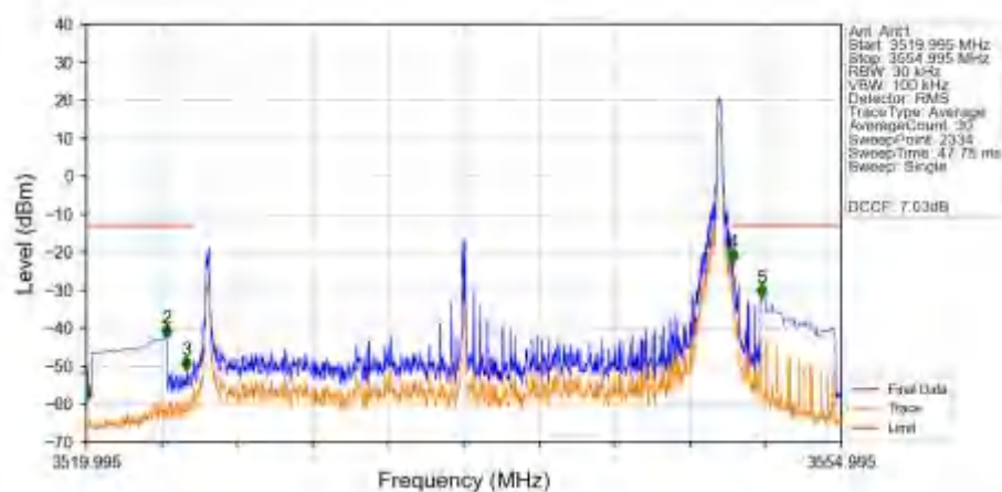
n77d_15kHz_SISO_NTNV_25MHz_DFT-s-OFDM_QPSK_3537.495MHz_Edge_1RB_Right_Ant1
