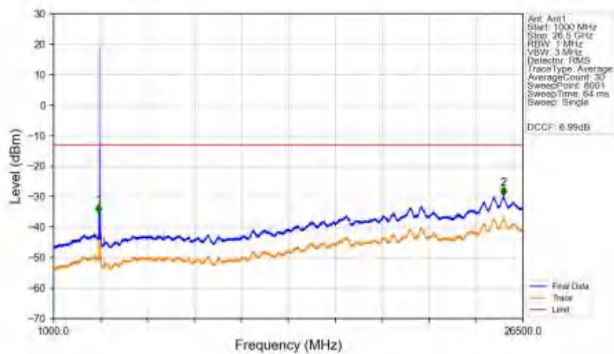
n77d_15kHz_SISO_NTNV_25MHz_DFT-s-OFDM_QPSK_3499.995MHz_Edge_1RB_Left_Ant1
