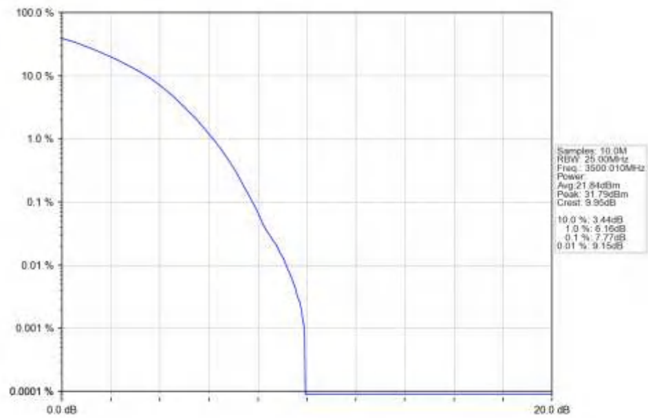
n77d_30kHz_SISO_NTNV_90MHz_DFT-s-OFDM_256_QAM_3500.01MHz_Outer_Full_Ant1
