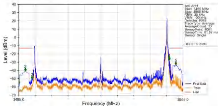
n77d_15kHz_SISO_NTNV_50MHz_DFT-s-OFDM_QPSK_3525MHz_Edge_1RB_Right_Ant1
