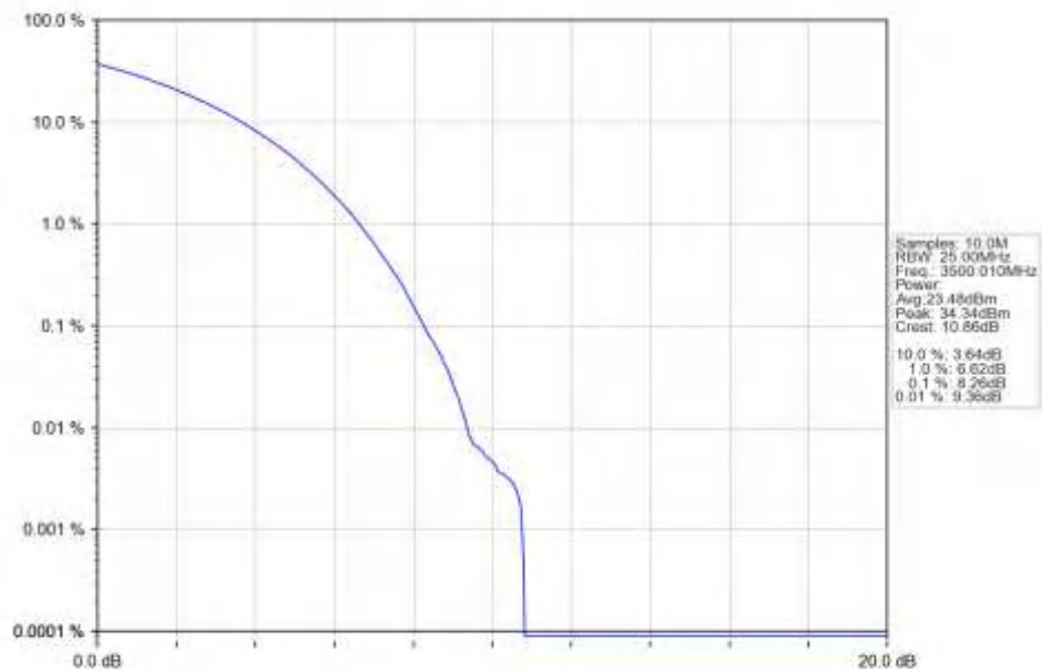
n77d 30kHz SISO_NTNV_80MHz CP-OFDM QPSK 3500.01MHz_Outer_Full_Ant1
