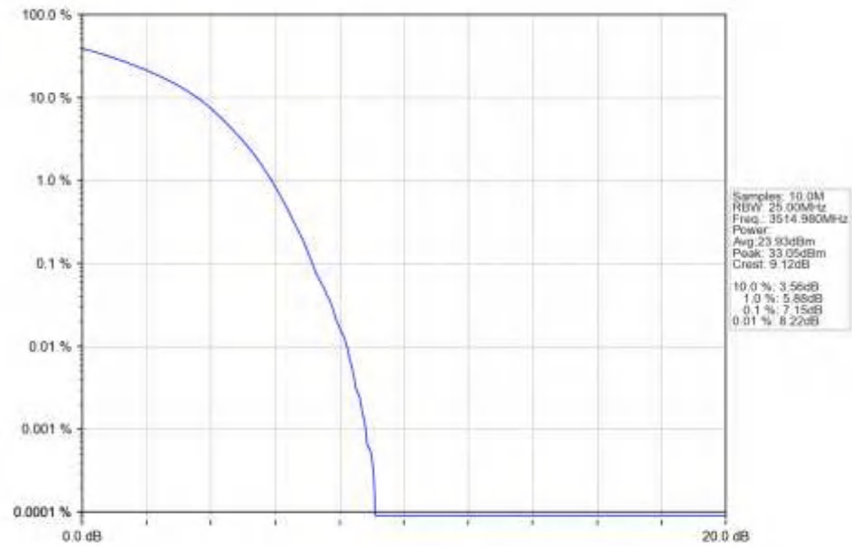
n77d_30kHz_SISO_NTNV_70MHz_DFT-s-OFDM_QPSK_3514.98MHz_Outer_Full_Ant1
