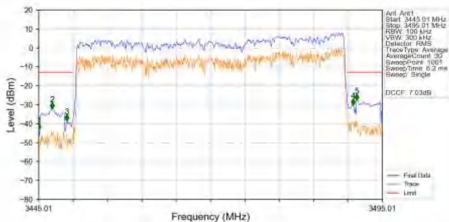
n77d 15kHz SISO NTN 40MHz DFT-s-OFDM QPSK 3470.01MHz Outer Full Ant1
