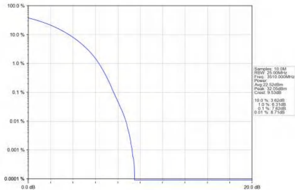
n77d_30kHz_SISO_NTNV_80MHz_DFT-s-OFDM_256_QAM_3510MHz_Outer_Full_Ant1
