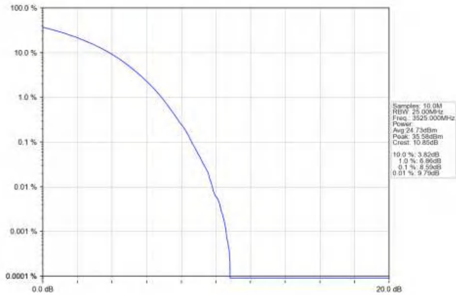
n77d_30kHz_SISO_NTNV_50MHz_CP-OFDM_64_QAM_3525MHz_Outer_Full_Ant1
