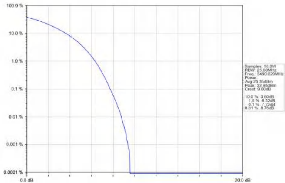
n77d 30kHz SISO_NTNV_80MHz DFT-s-OFDM 16 QAM 3490.02MHz_Outer_Full_Ant1
