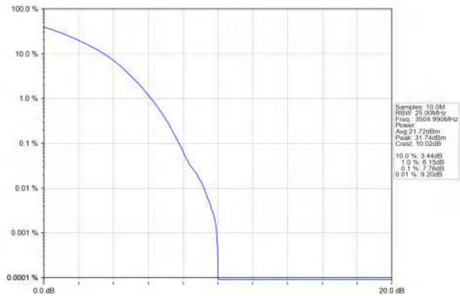
n77d_30kHz_SISO_NTNV_90MHz_DFT-s-OFDM_256_QAM_3504.99MHz_Outer_Full_Ant1
