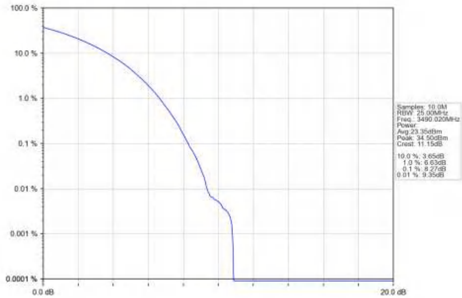
n77d 30kHz SISO_NTNV_80MHz CP-OFDM QPSK 3490.02MHz_Outer_Full_Ant1
