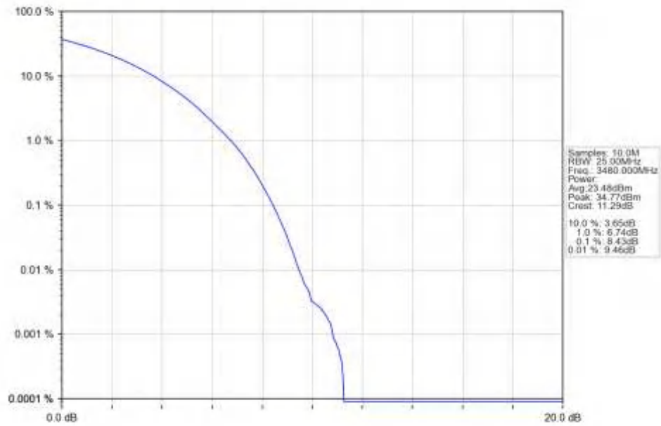
n77d_30kHz_SISO_NTNV_60MHz_CP-OFDM_64_QAM_3480MHz_Outer_Full_Ant1
