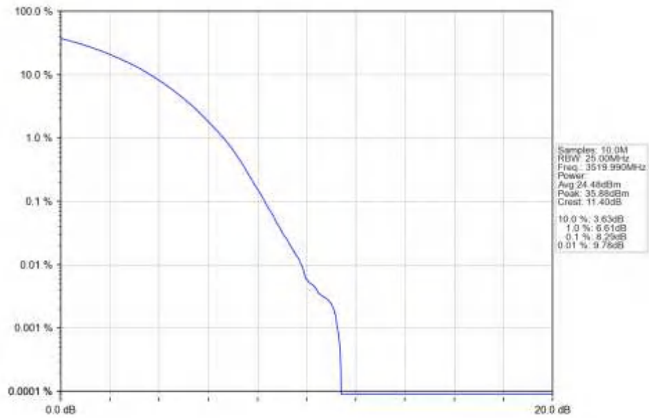
n77d_30kHz_SISO_NTNV_60MHz_CP-OFDM_QPSK_3519.99MHz_Outer_Full_Ant1
