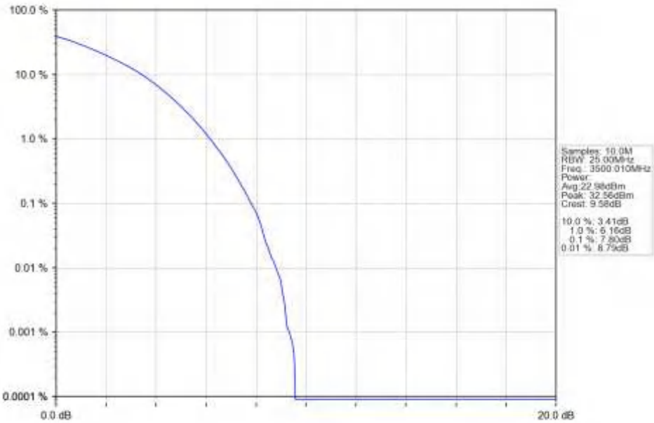
n77d_30kHz_SISO_NTNV_90MHz_DFT-s-OFDM_64_QAM_3500.01MHz_Outer_Full_Ant1
