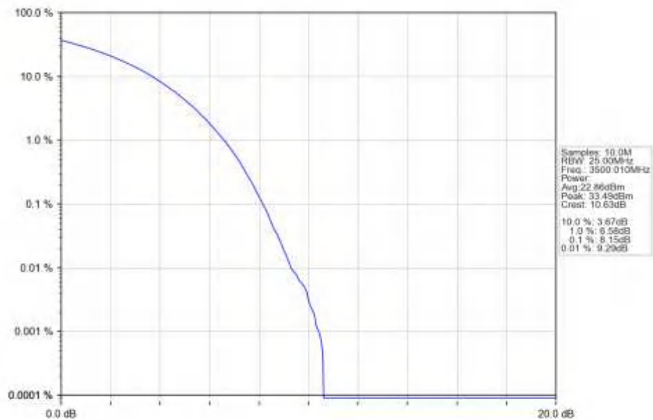
n77d_30kHz_SISO_NTNV_90MHz_CP-OFDM_QPSK_3500.01MHz_Outer_Full_Ant1
