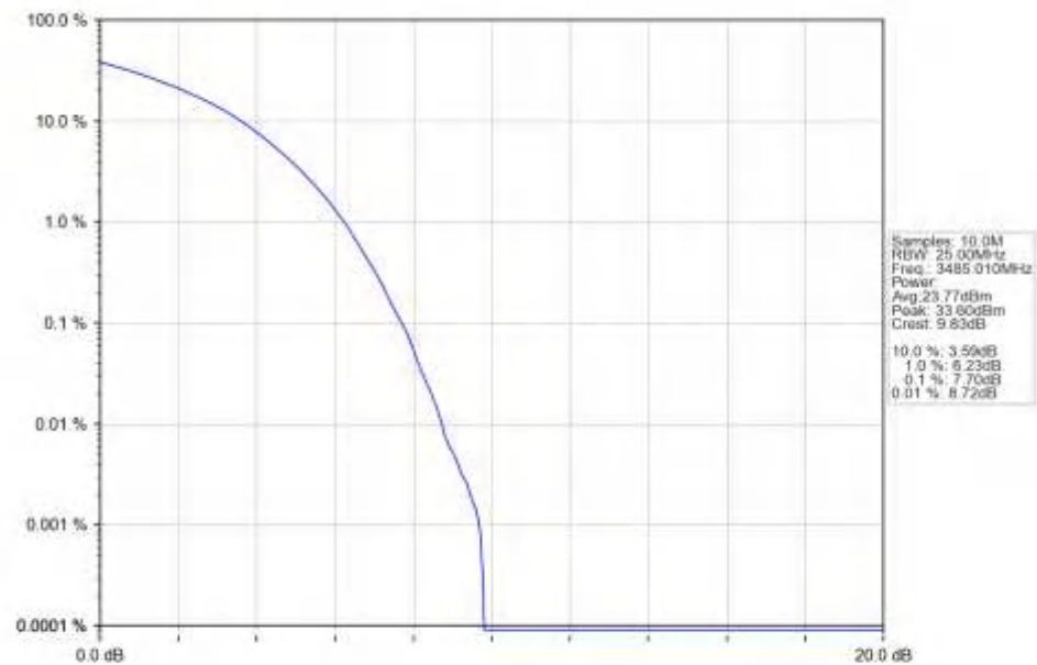
n77d_30kHz_SISO_NTNV_70MHz_DFT-s-OFDM_16_QAM_3485.01MHz_Outer_Full_Ant1
