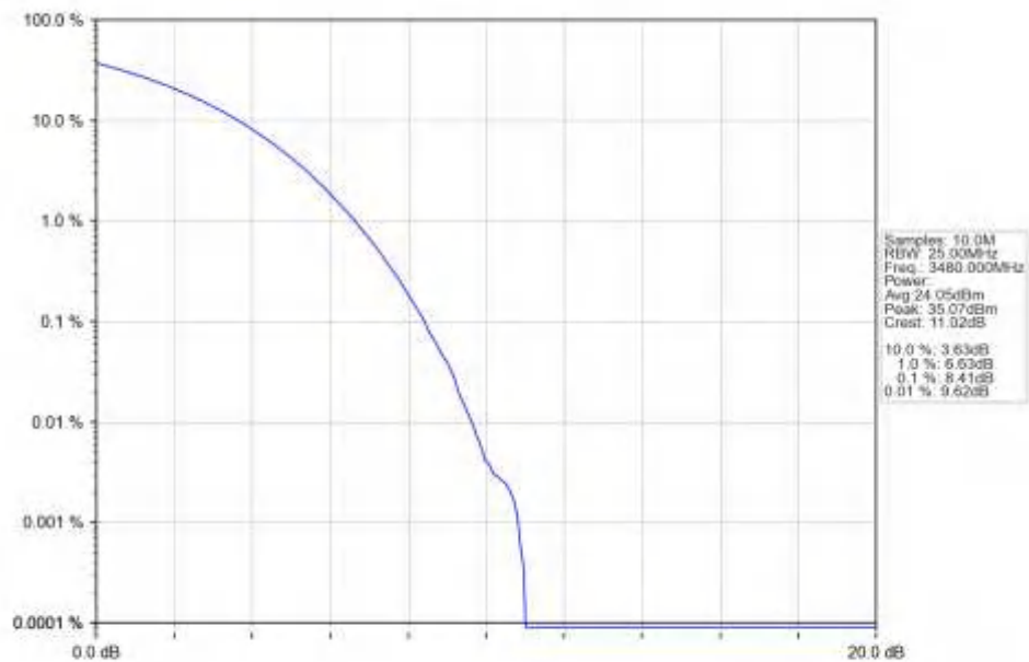
n77d_30kHz_SISO_NTNV_60MHz_CP-OFDM_16_QAM_3480MHz_Outer_Full_Ant1
