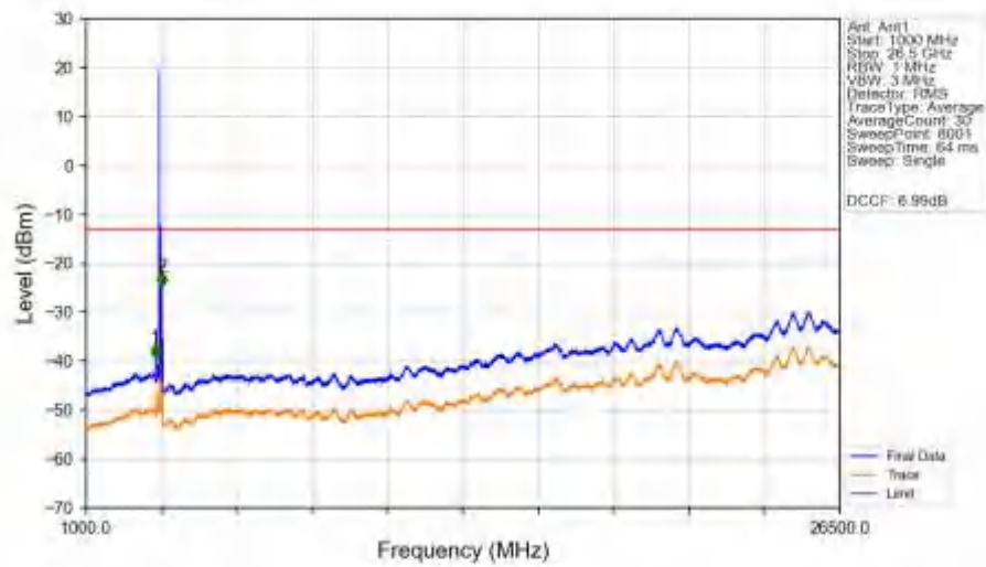
n77d_15kHz_SISO_NTNV_50MHz_CP-OFDM_QPSK_3499.995MHz_Edge_1RB_Left_Ant1
