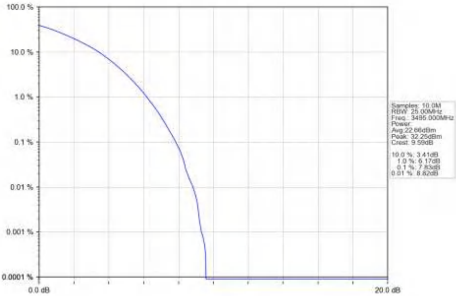
n77d_30kHz_SISO_NTNV_90MHz_DFT-s-OFDM_64_QAM_3495MHz_Outer_Full_Ant1
