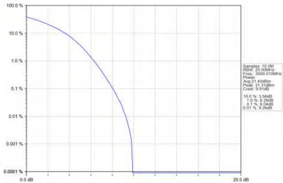
n77d_30kHz_SISO_NTNV_100MHz_DFT-s-OFDM_256_QAM_3500.01MHz_Outer_Full_Ant1
