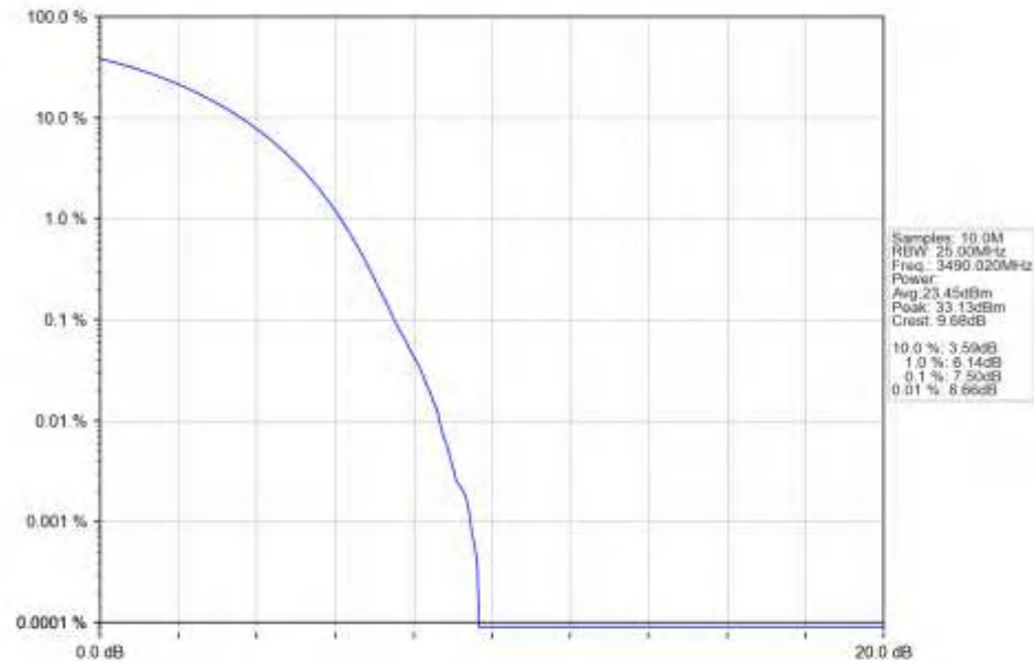
n77d_30kHz_SISO_NTNV_80MHz_DFT-s-OFDM_QPSK_3490.02MHz_Outer_Full_Ant1
