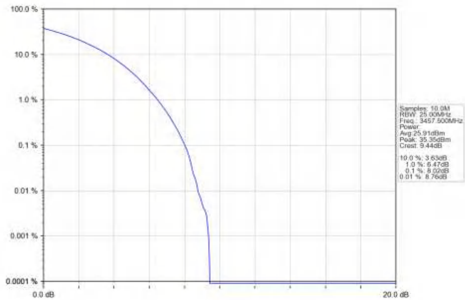
n77d_15kHz_SISO_NTNV_15MHz_CP-OFDM_16_QAM_3457.5MHz_Outer_Full_Ant1
