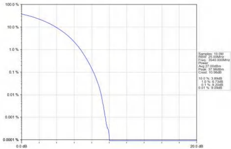
n77d_15kHz_SISO_NTNV_20MHz_CP-OFDM_16_QAM_3540MHz_Outer_Full_Ant1
