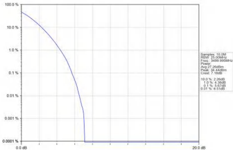
n77d_15kHz_SISO_NTNV_15MHz_DFT-s-OFDM QPSK_3499.995MHz_Outer_Full_Ant1
