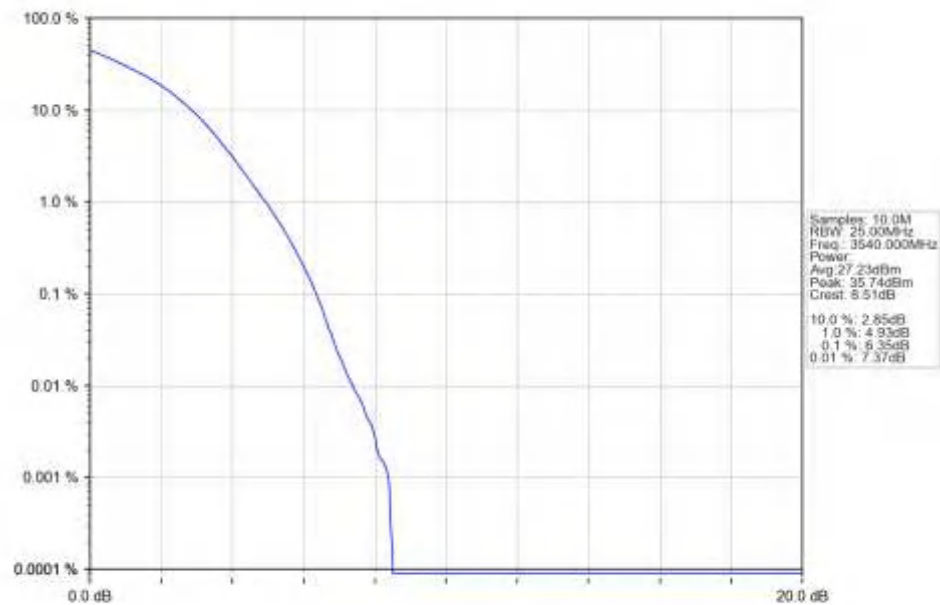
n77d_15kHz_SISO_NTNV_20MHz_DFT-s-OFDM_16_QAM_3540MHz_Outer_Full_Ant1
