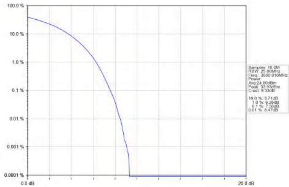
n77d_30kHz_SISO_NTNV_50MHz_DFT-s-OFDM_256_QAM_3500.01MHz_Outer_Full_Ant1
