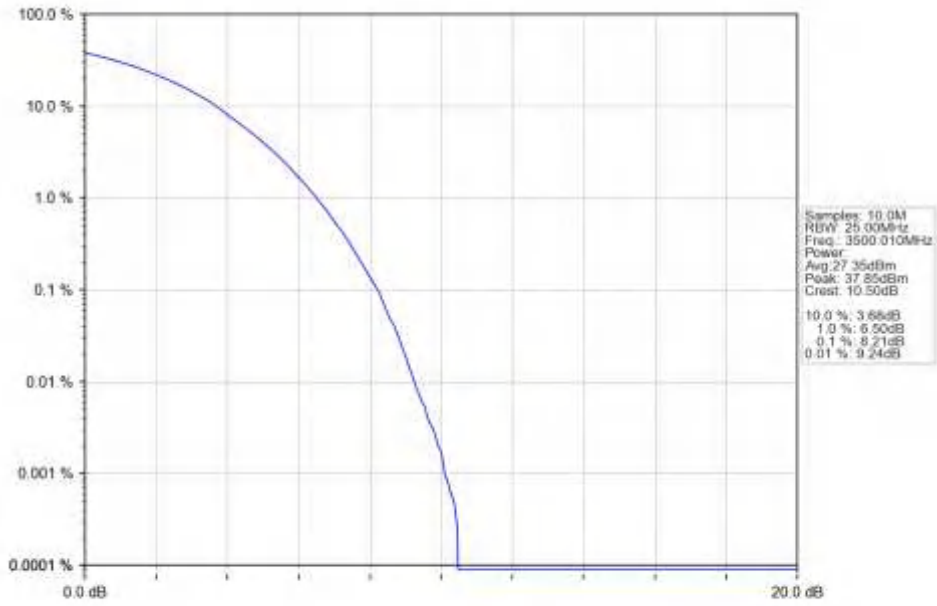
n77d_30kHz_SISO_NTNV_30MHz_CP-OFDM_64_QAM_3500.01MHz_Outer_Full_Ant1
