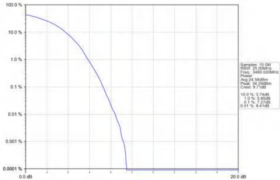
n77d_30kHz_SISO_NTNV_20MHz_DFT-s-OFDM_256_QAM_3460.02MHz_Outer_Full_Ant1
