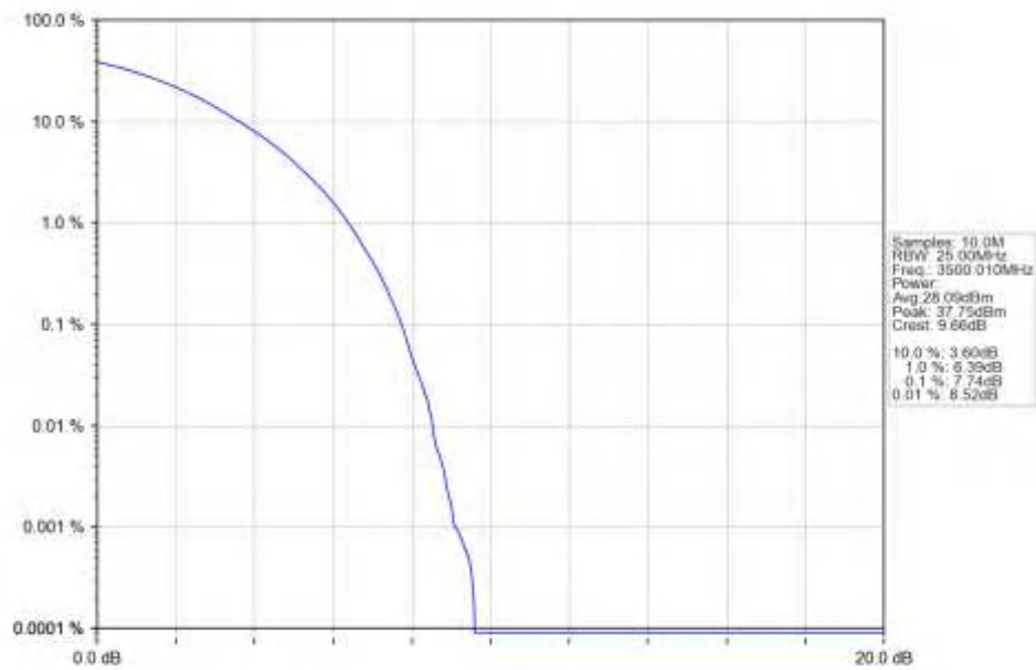
n77d_30kHz_SISO_NTNV_25MHz_CP-OFDM_QPSK_3500.01MHz_Outer_Full_Ant1
