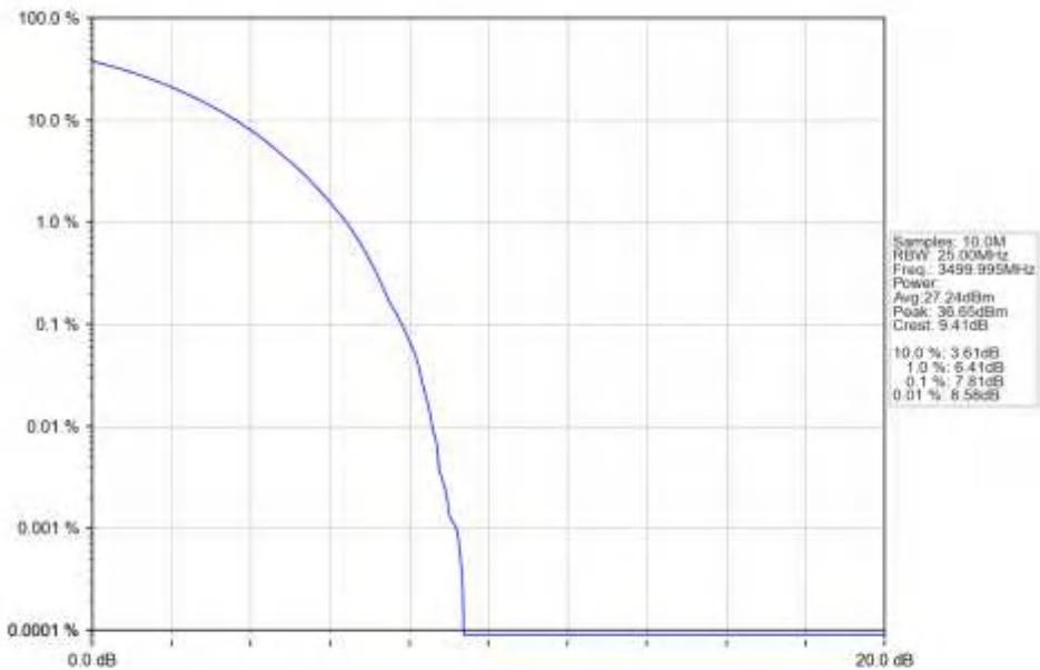
n77d_15kHz_SISO_NTNV_15MHz_CP-OFDM_16_QAM_3499.995MHz_Outer_Full_Ant1
