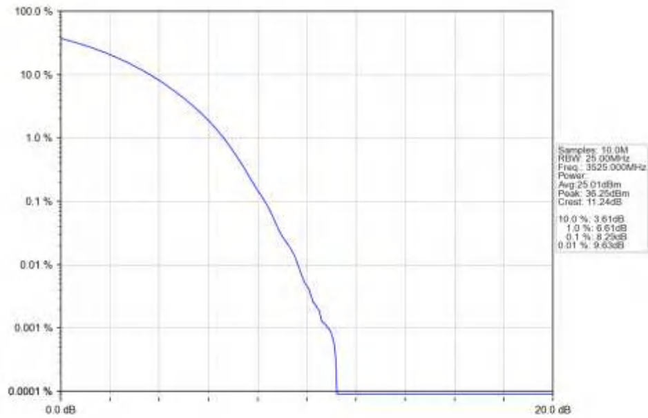
n77d_15kHz_SISO_NTNV_50MHz_CP-OFDM_64_QAM_3525MHz_Outer_Full_Ant1
