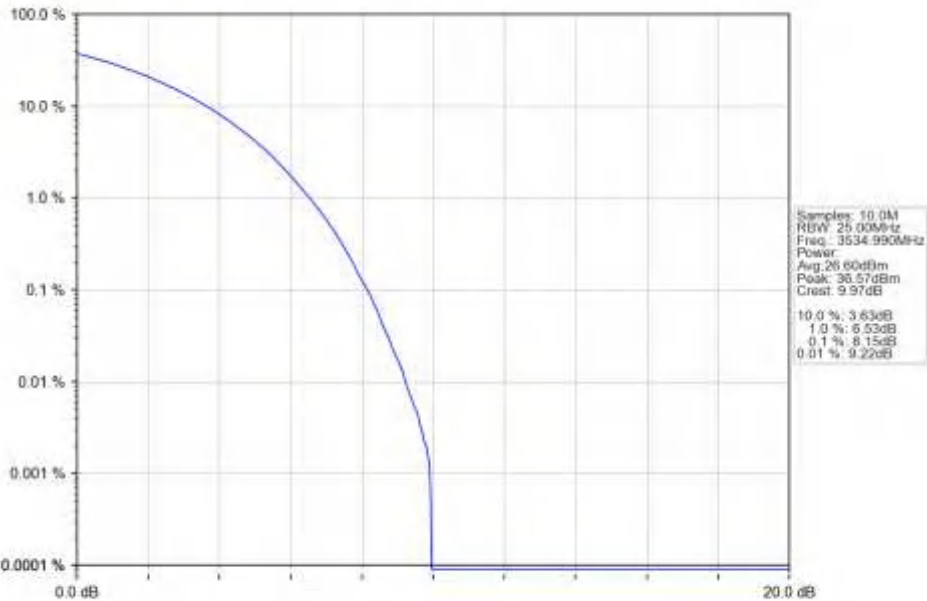
n77d_15kHz_SISO_NTNV_30MHz_CP-OFDM_64_QAM_3534.99MHz_Outer_Full_Ant1
