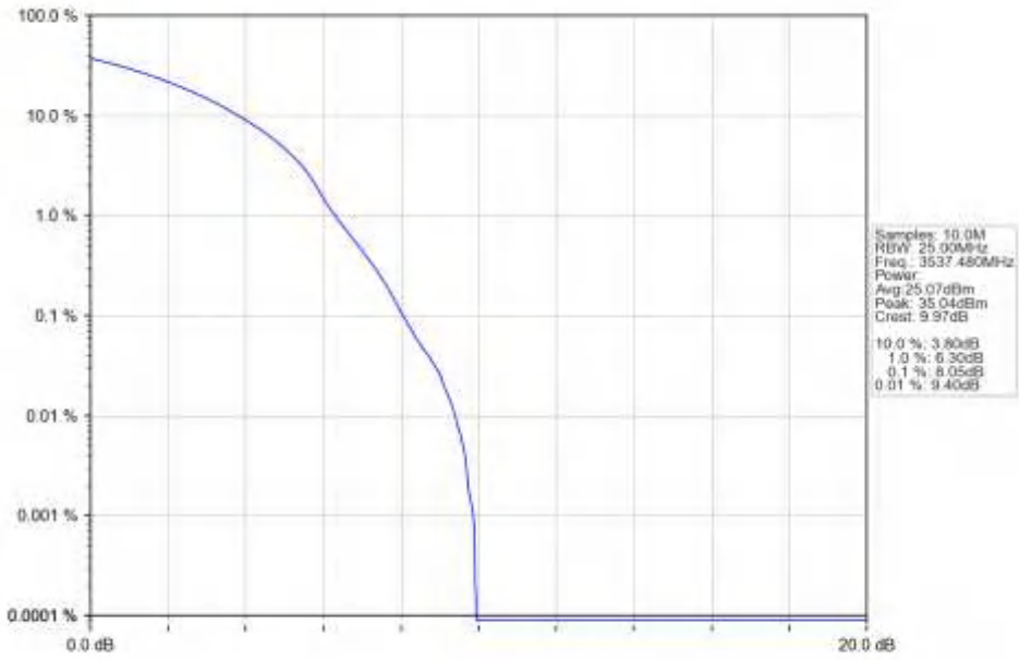
n77d_30kHz_SISO_NTNV_25MHz_CP-OFDM_256_QAM_3537.48MHz_Outer_Full_Ant1
