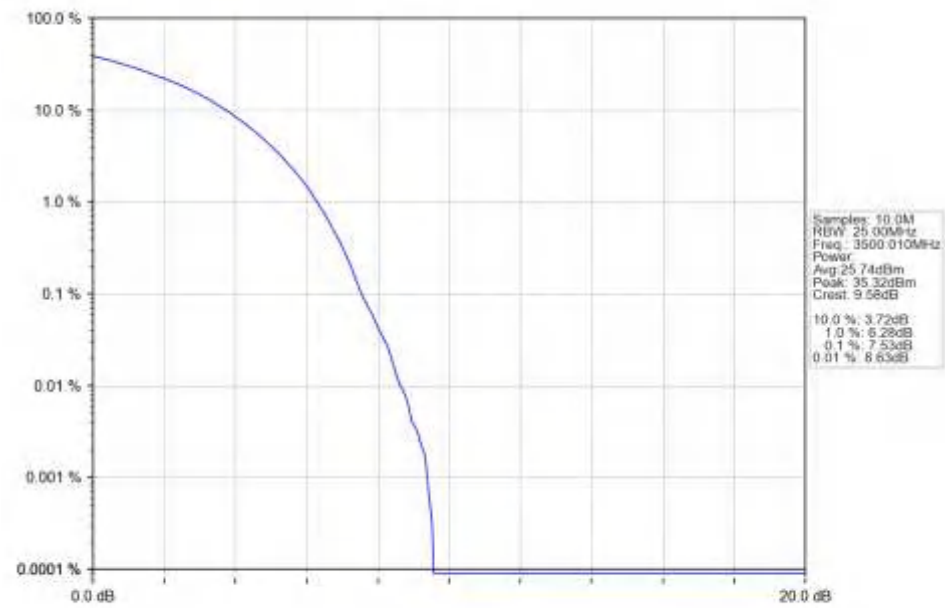
n77d_30kHz_SISO_NTNV_50MHz_DFT-s-OFDM_16_QAM_3500.01MHz_Outer_Full_Ant1
