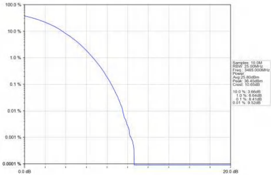
n77d_30kHz_SISO_NTNV_30MHz_CP-OFDM_64_QAM_3465MHz_Outer_Full_Ant1
