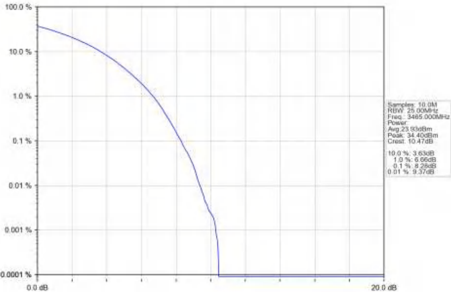
n77d_15kHz_SISO_NTNV_30MHz_CP-OFDM_256_QAM_3465MHz_Outer_Full_Ant1
