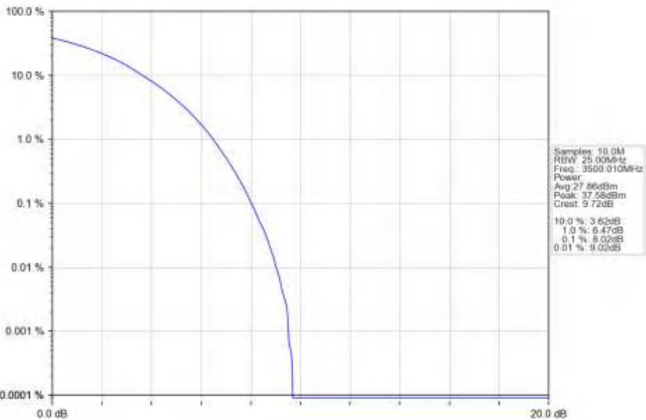
n77d_30kHz_SISO_NTNV_30MHz_CP-OFDM_16_QAM_3500.01MHz_Outer_Full_Ant1
