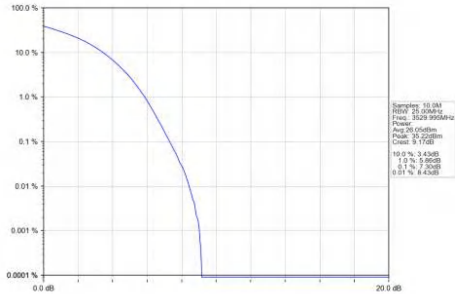
n77d_15kHz_SISO_NTNV_40MHz_DFT-s-OFDM_64_QAM_3529.995MHz_Outer_Full_Ant1
