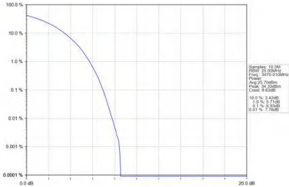
n77d_30kHz_SISO_NTNV_40MHz_DFT-s-OFDM_QPSK_3470.01MHz_Outer_Full_Ant1
