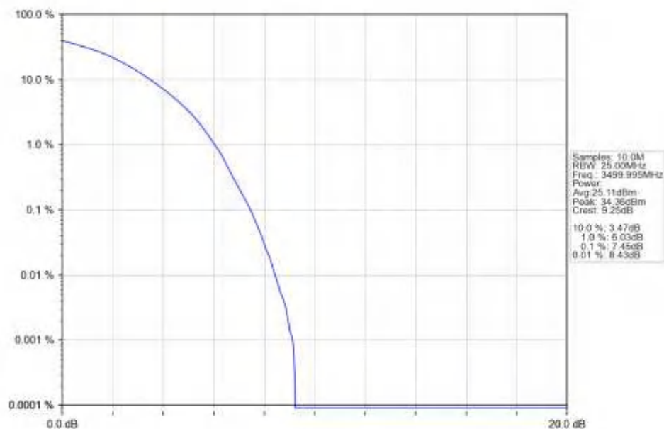
n77d_15kHz_SISO_NTNV_50MHz_DFT-s-OFDM_64_QAM_3499.995MHz_Outer_Full_Ant1
