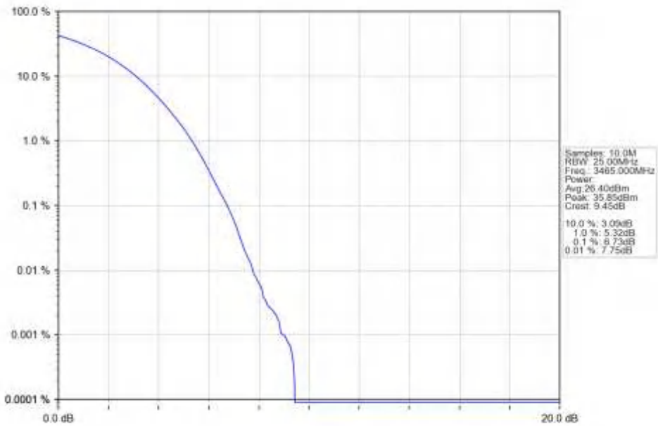
n77d_15kHz_SISO_NTNV_30MHz_DFT-s-OFDM_16_QAM_3465MHz_Outer_Full_Ant1
