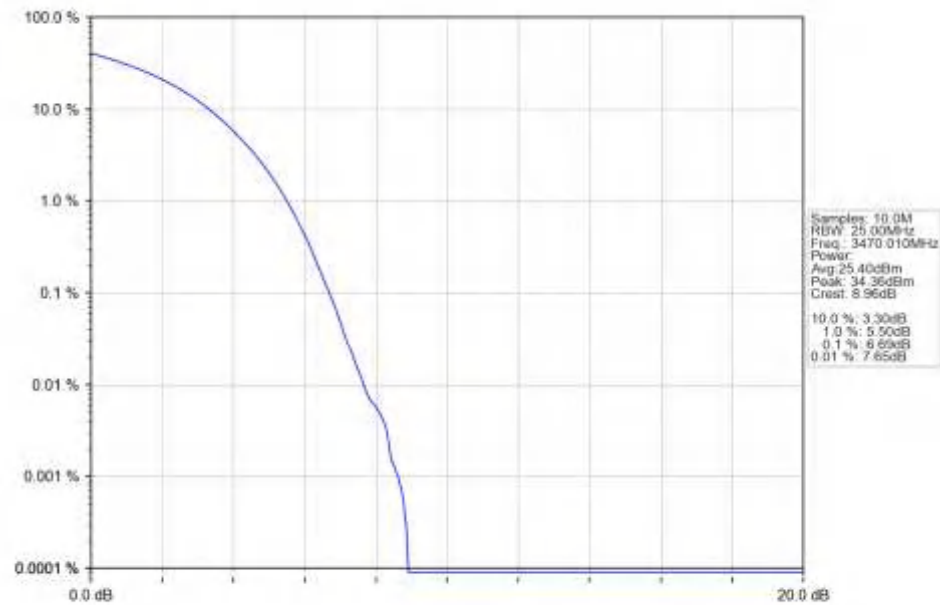
n77d_15kHz_SISO_NTNV_40MHz_DFT-s-OFDM QPSK_3470.01MHz_Outer_Full_Ant1
