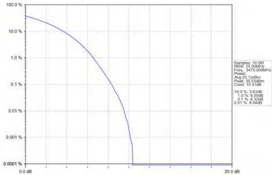
n77d_15kHz_SISO_NTNV_50MHz_CP-OFDM_QPSK_3475.005MHz_Outer_Full_Ant1
