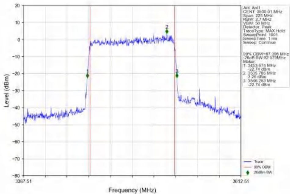
n77d_30kHz_SISO_NTNV_90MHz_DFT-s-OFDM QPSK_3500.01MHz_Outer_Full_Ant1
