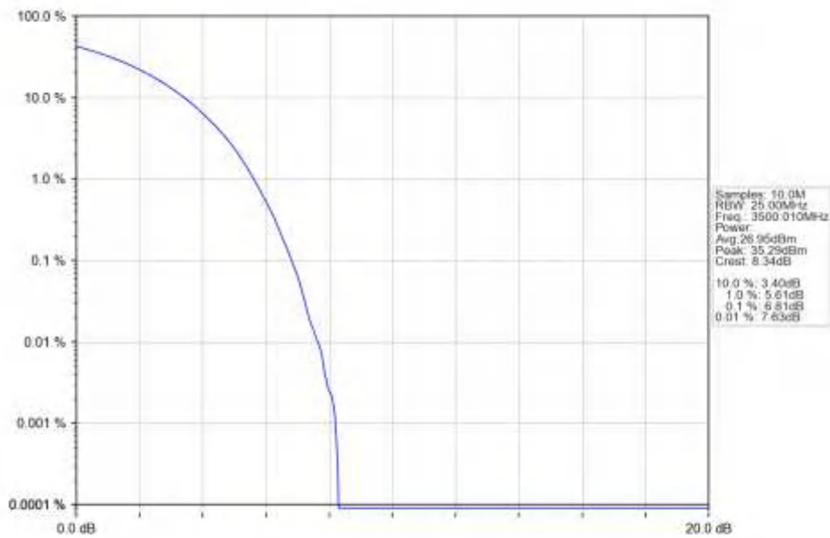
n77d_30kHz_SISO_NTNV_40MHz_DFT-s-OFDM_QPSK_3500.01MHz_Outer_Full_Ant1
