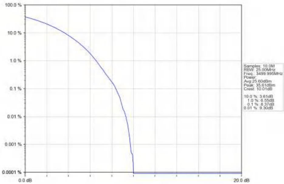
n77d_15kHz_SISO_NTNV_50MHz_CP-OFDM_16_QAM_3499.995MHz_Outer_Full_Ant1
