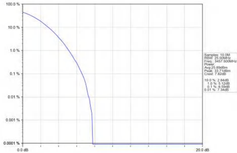
n77d_15kHz_SISO_NTNV_15MHz_DFT-s-OFDM_64_QAM_3457.5MHz_Outer_Full_Ant1
