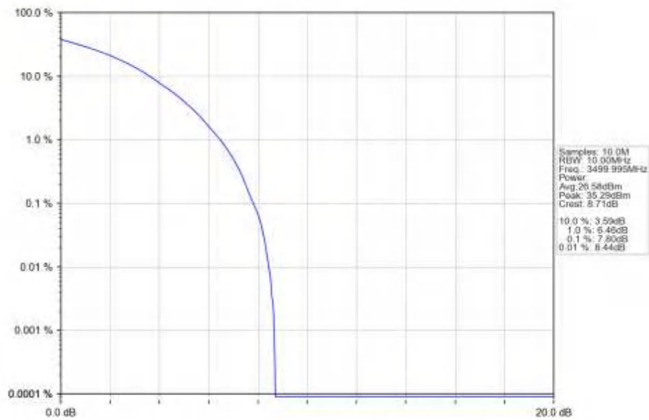
n77d_15kHz_SISO_NTNV_10MHz_CP-OFDM_QPSK_3499.995MHz_Outer_Full_Ant1
