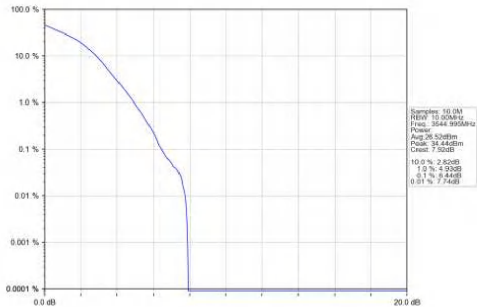
n77d_15kHz_SISO_NTNV_10MHz_DFT-s-OFDM_16_QAM_3544.995MHz_Outer_Full_Ant1
