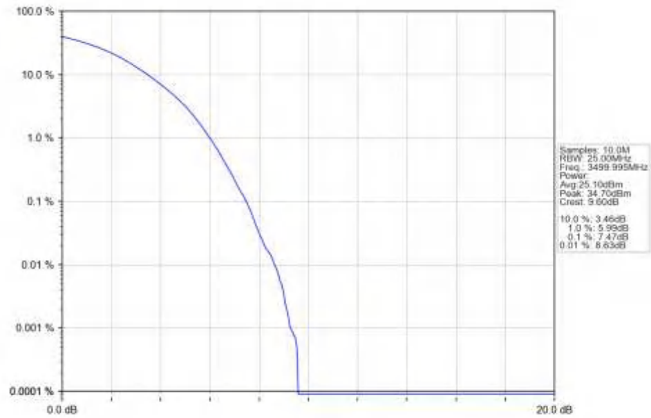
n77d_15kHz_SISO_NTNV_50MHz_DFT-s-OFDM_16_QAM_3499.995MHz_Outer_Full_Ant1
