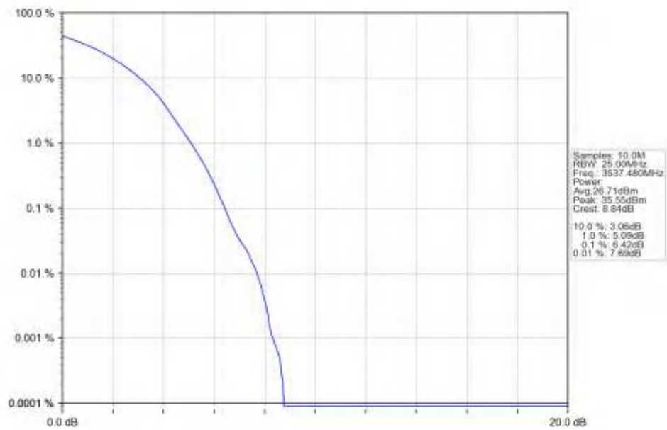
n77d_30kHz_SISO_NTNV_25MHz_DFT-s-OFDM_256_QAM_3537.48MHz_Outer_Full_Ant1
