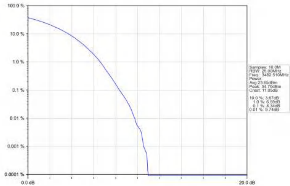
n77d_15kHz_SISO_NTNV_25MHz_CP-OFDM_256_QAM_3462.51MHz_Outer_Full_Ant1
