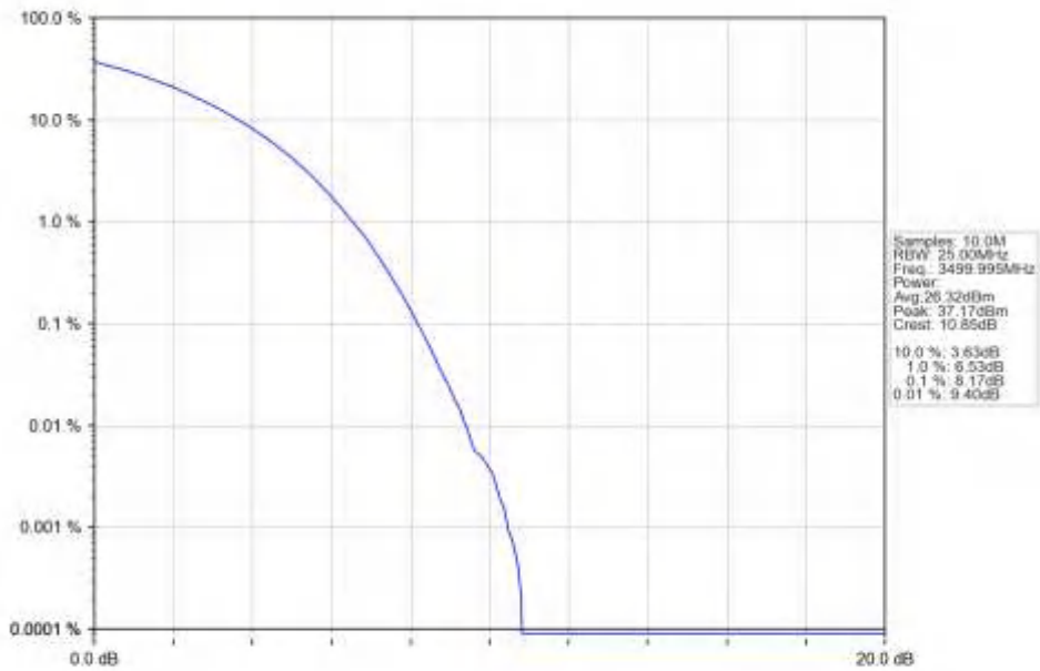
n77d_15kHz_SISO_NTNV_40MHz_CP-OFDM_QPSK_3499.995MHz_Outer_Full_Ant1
