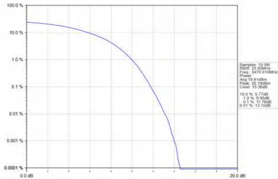
n77d_15kHz_SISO_NTNV_40MHz_DFT-s-OFDM_256_QAM_3470.01MHz_Outer_Full_Ant1
