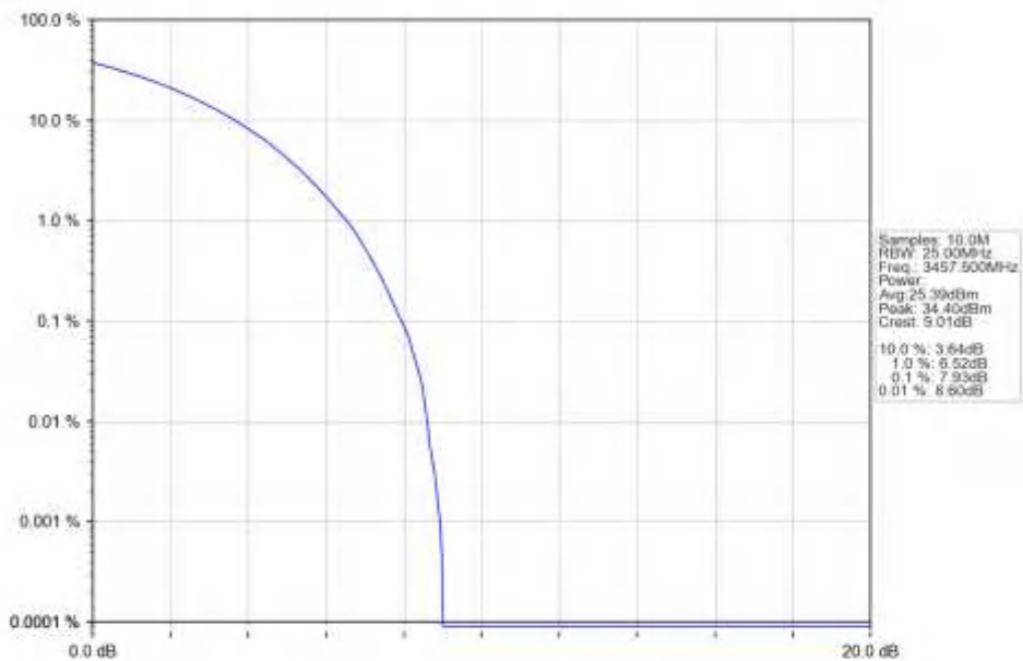
n77d_15kHz_SISO_NTNV_15MHz_CP-OFDM_64_QAM_3457.5MHz_Outer_Full_Ant1
