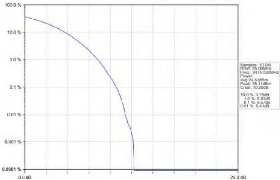
n77d_30kHz_SISO_NTNV_50MHz_CP-OFDM_QPSK_3475.02MHz_Outer_Full_Ant1
