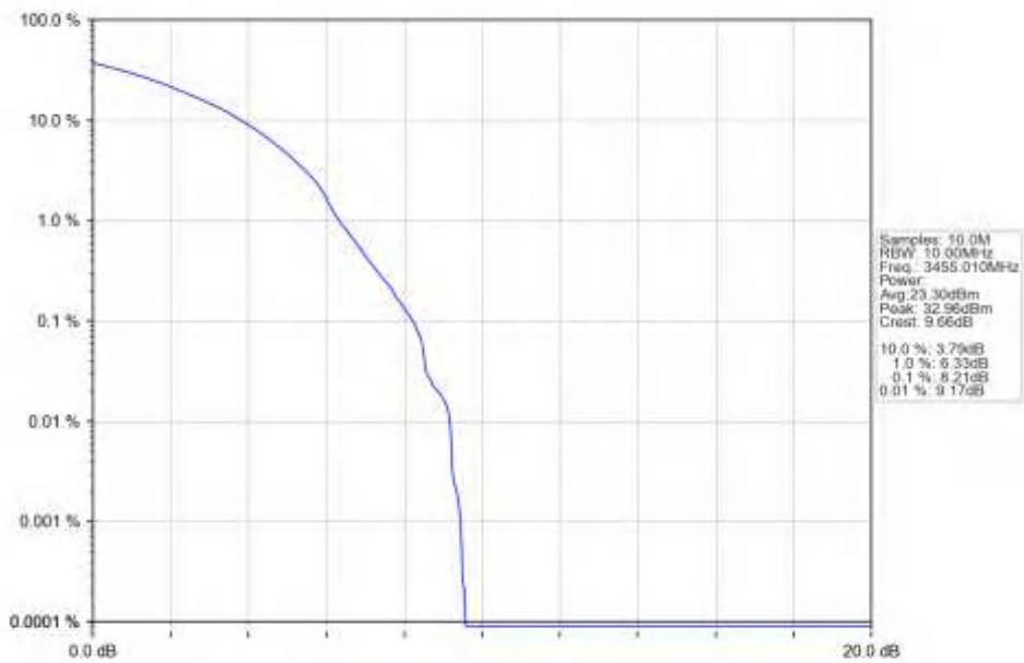
n77d_30kHz_SISO_NTNV_10MHz_CP-OFDM_256_QAM_3455.01MHz_Outer_Full_Ant1
