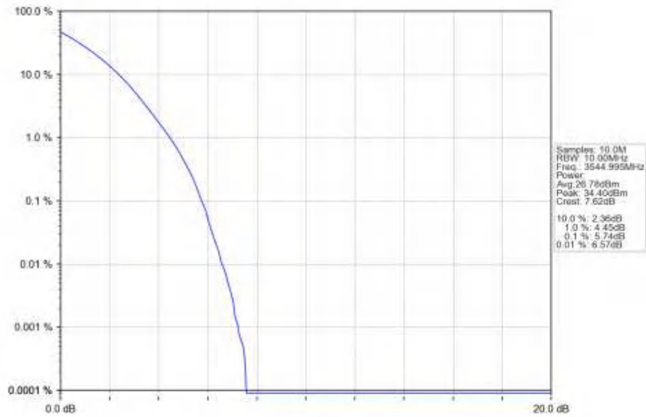
n77d_15kHz_SISO_NTNV_10MHz_DFT-s-OFDM_QPSK_3544.995MHz_Outer_Full_Ant1
