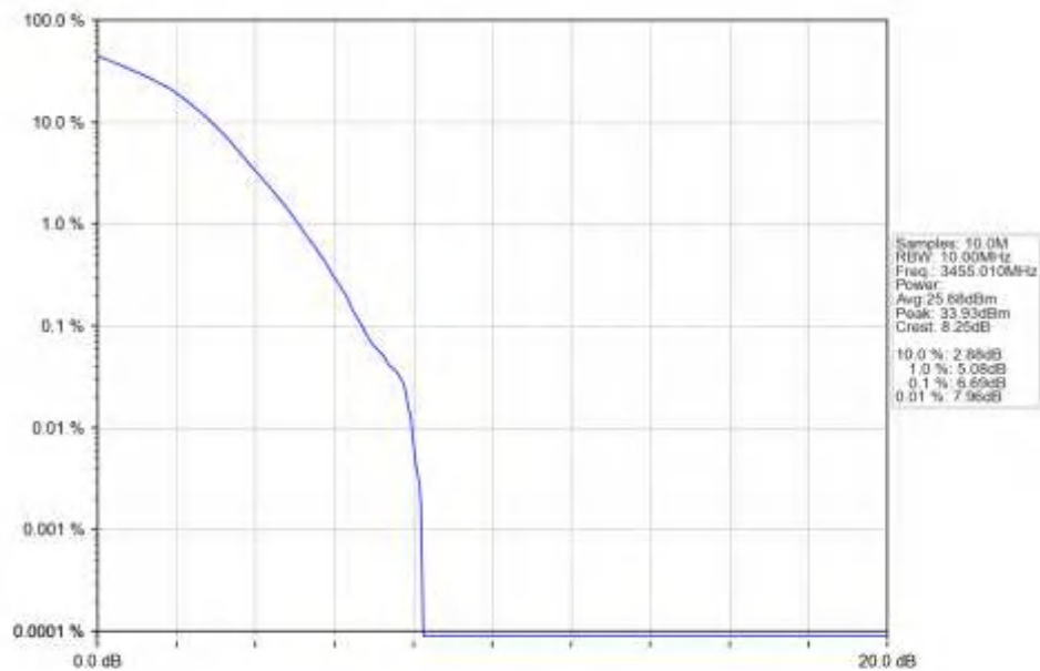
n77d_15kHz_SISO_NTNV_10MHz_DFT-s-OFDM_16_QAM_3455.01MHz_Outer_Full_Ant1
