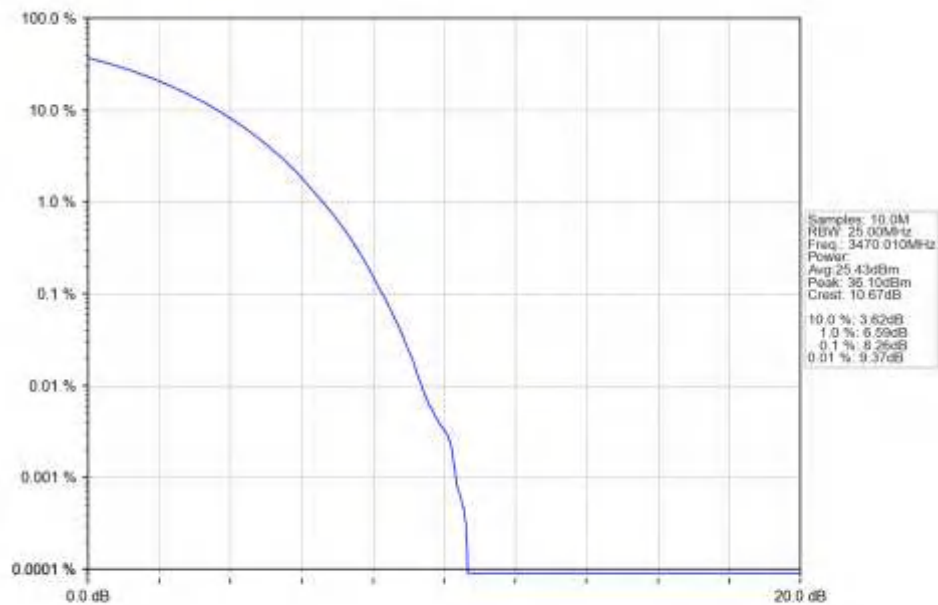
n77d_15kHz_SISO_NTNV_40MHz_CP-OFDM_16_QAM_3470.01MHz_Outer_Full_Ant1
