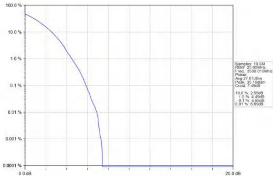
n77d_30kHz_SISO_NTNV_15MHz_DFT-s-OFDM_QPSK_3500.01MHz_Outer_Full_Ant1
