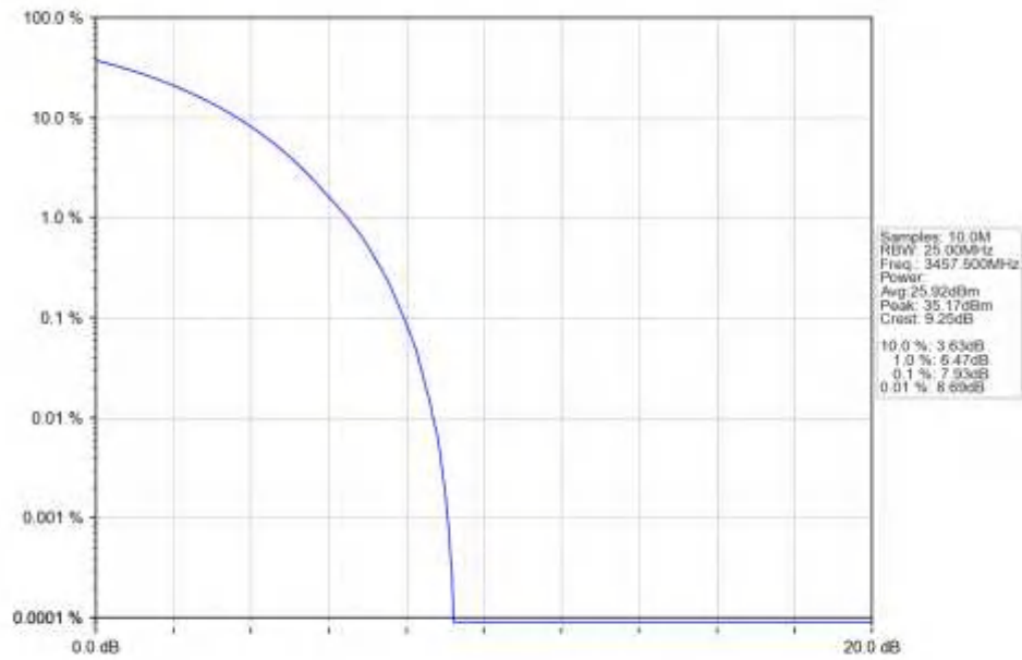
n77d_15kHz_SISO_NTNV_15MHz_CP-OFDM_QPSK_3457.5MHz_Outer_Full_Ant1
