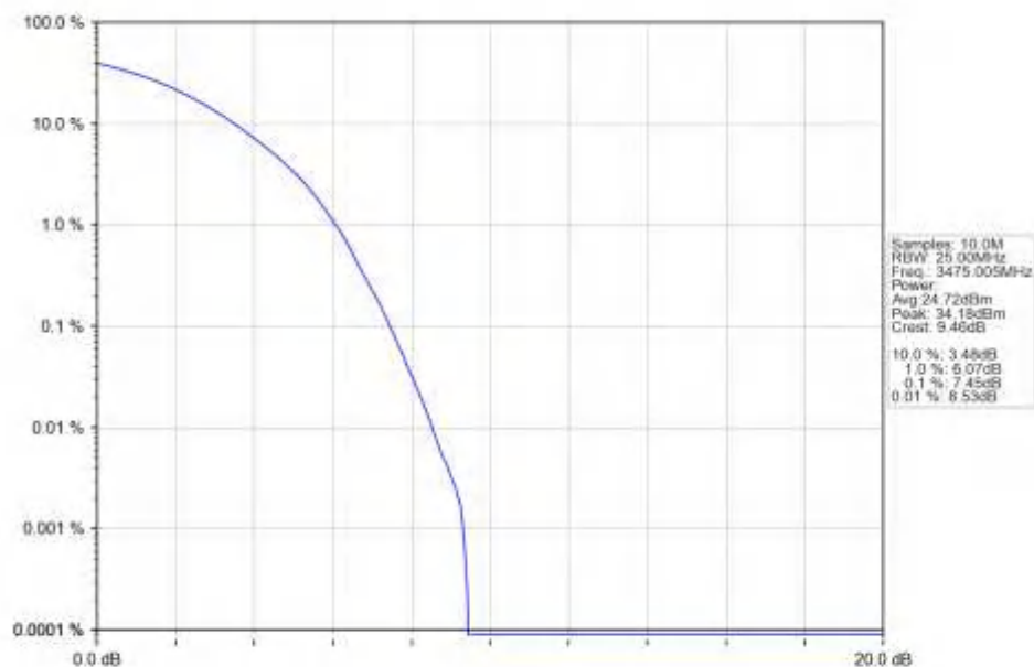
n77d_15kHz_SISO_NTNV_50MHz_DFT-s-OFDM_64_QAM_3475.005MHz_Outer_Full_Ant1
