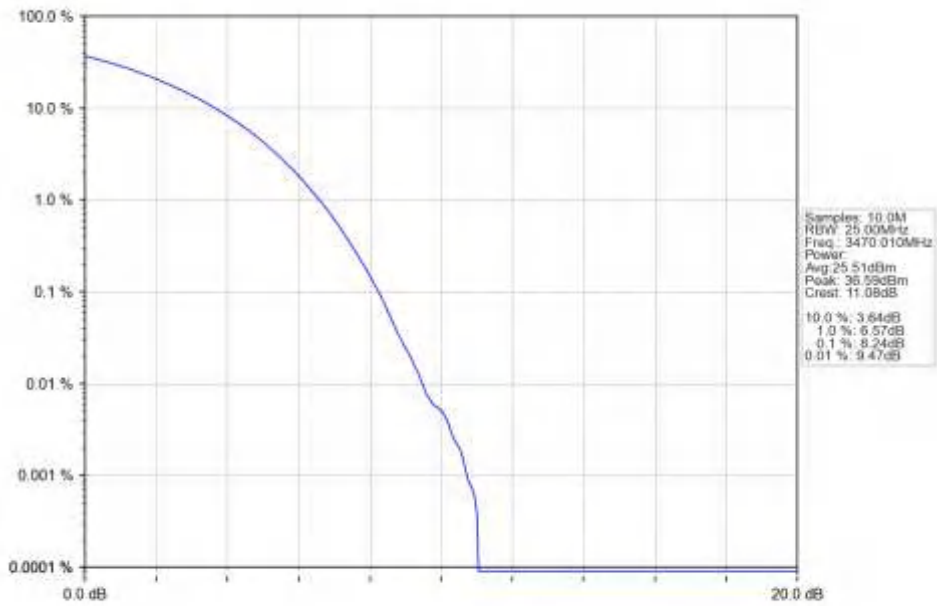
n77d_15kHz_SISO_NTNV_40MHz_CP-OFDM_QPSK_3470.01MHz_Outer_Full_Ant1
