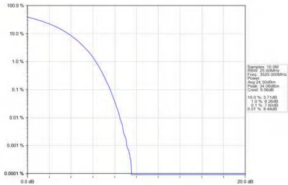
n77d_30kHz_SISO_NTNV_50MHz_DFT-s-OFDM_256_QAM_3525MHz_Outer_Full_Ant1
