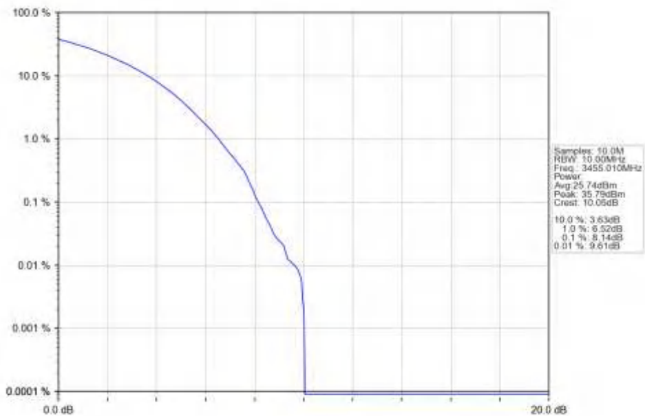
n77d_15kHz_SISO_NTNV_10MHz_CP-OFDM_16QAM_3455.01MHz_Outer_Full_Ant1
