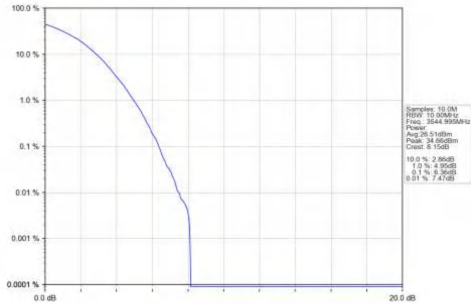
n77d_15kHz_SISO_NTNV_10MHz_DFT-s-OFDM_64_QAM_3544.995MHz_Outer_Full_Ant1
