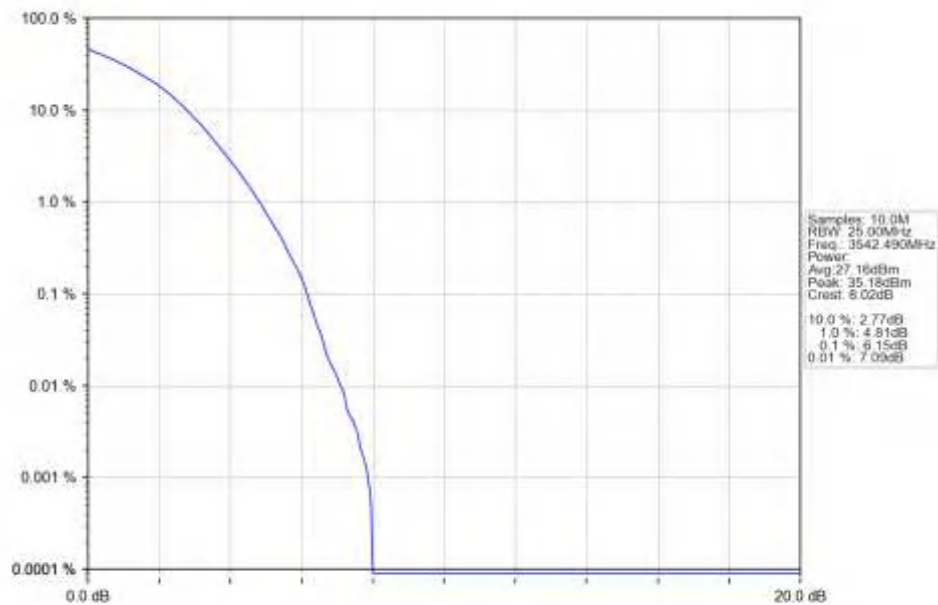
n77d_15kHz_SISO_NTNV_15MHz_DFT-s-OFDM_16_QAM_3542.49MHz_Outer_Full_Ant1
