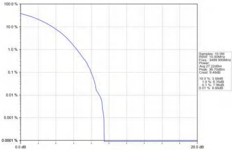
n77d_15kHz_SISO_NTNV_10MHz_CP-OFDM_16_QAM_3499.995MHz_Outer_Full_Ant1
