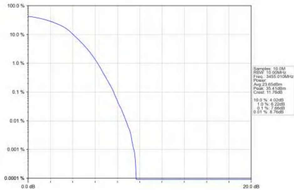
n77d_15kHz_SISO_NTNV_10MHz_DFT-s-OFDM_256_QAM_3455.01MHz_Outer_Full_Ant1
