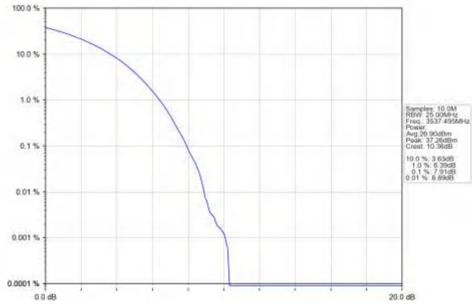
n77d_15kHz_SISO_NTNV_25MHz_CP-OFDM_64_QAM_3537.495MHz_Outer_Full_Ant1
