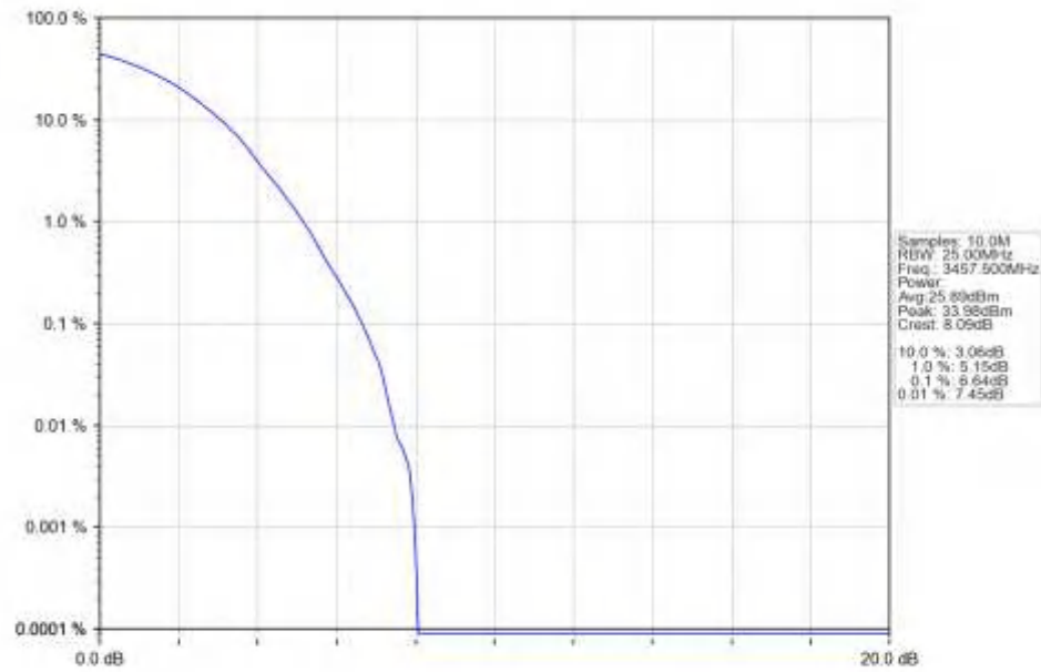
n77d_30kHz_SISO_NTNV_15MHz_DFT-s-OFDM_64_QAM_3457.5MHz_Outer_Full_Ant1
