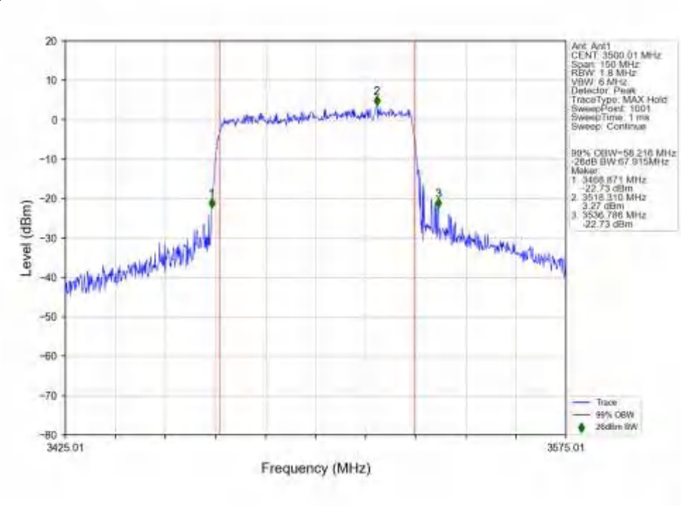
n77d_30kHz_SISO_NTNV_60MHz_CP-OFDM_QPSK_3500.01MHz_Outer_Full_Ant1
