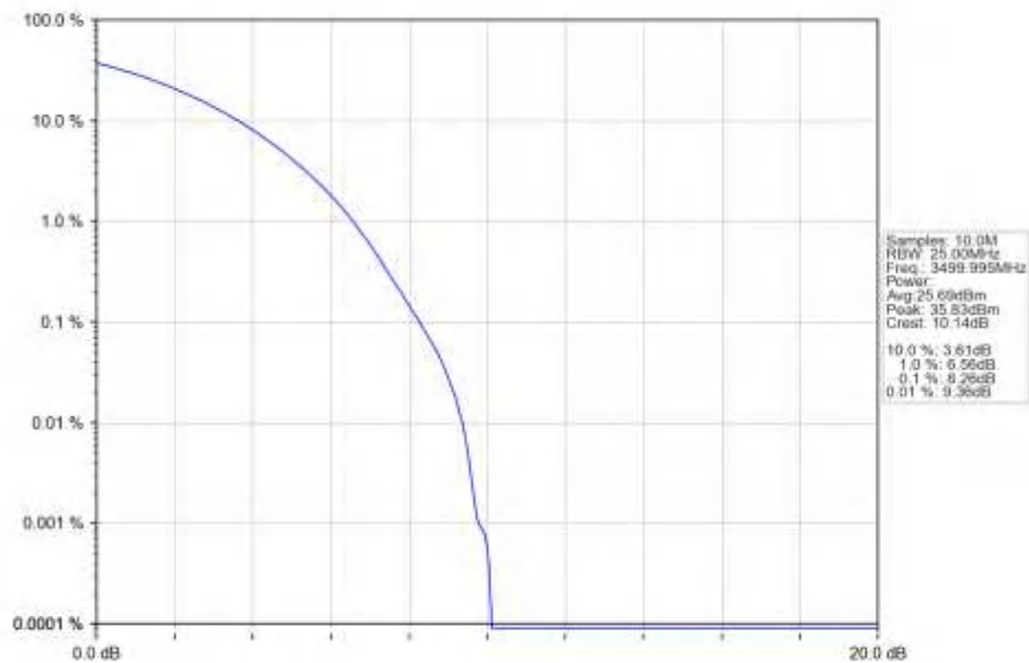
n77d_15kHz_SISO_NTNV_50MHz_CP-OFDM_QPSK_3499.995MHz_Outer_Full_Ant1
