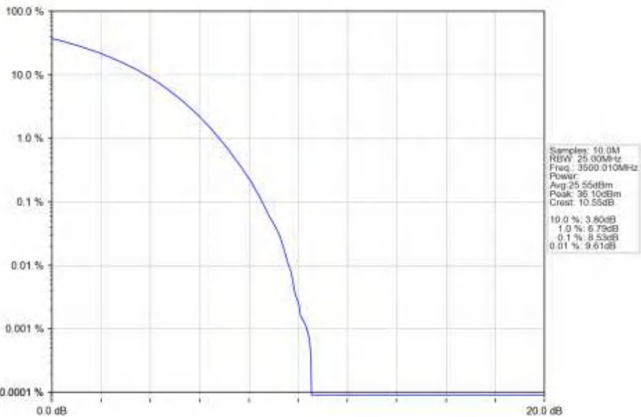
n77d_30kHz_SISO_NTNV_50MHz_CP-OFDM_16_QAM_3500.01MHz_Outer_Full_Ant1
