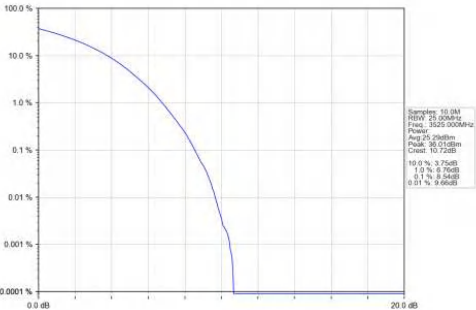
n77d_30kHz_SISO_NTNV_50MHz_CP-OFDM_16_QAM_3525MHz_Outer_Full_Ant1
