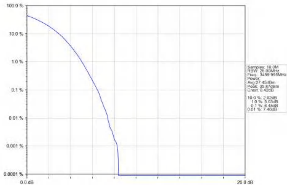
n77d_15kHz_SISO_NTNV_20MHz_DFT-s-OFDM_64_QAM_3499.995MHz_Outer_Full_Ant1
