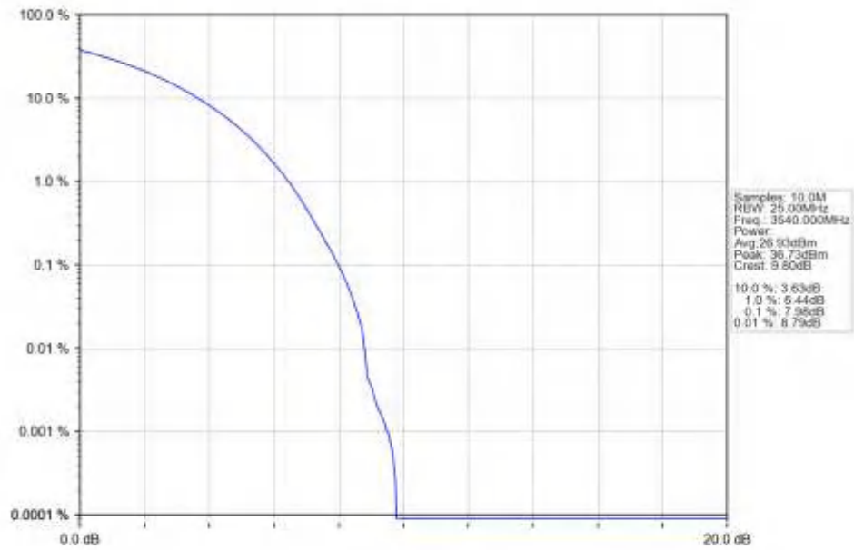
n77d_15kHz_SISO_NTNV_20MHz_CP-OFDM_64_QAM_3540MHz_Outer_Full_Ant1
