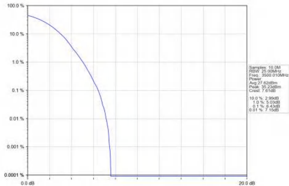
n77d_30kHz_SISO_NTNV_15MHz_DFT-s-OFDM_64_QAM_3500.01MHz_Outer_Full_Ant1
