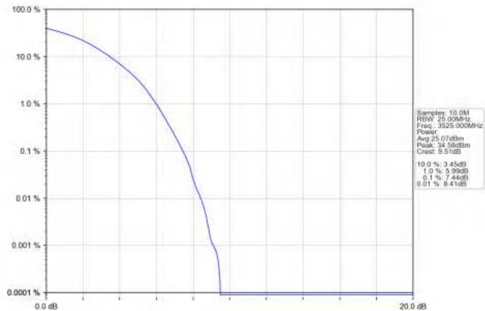
n77d_15kHz_SISO_NTNV_50MHz_DFT-s-OFDM_16_QAM_3525MHz_Outer_Full_Ant1
