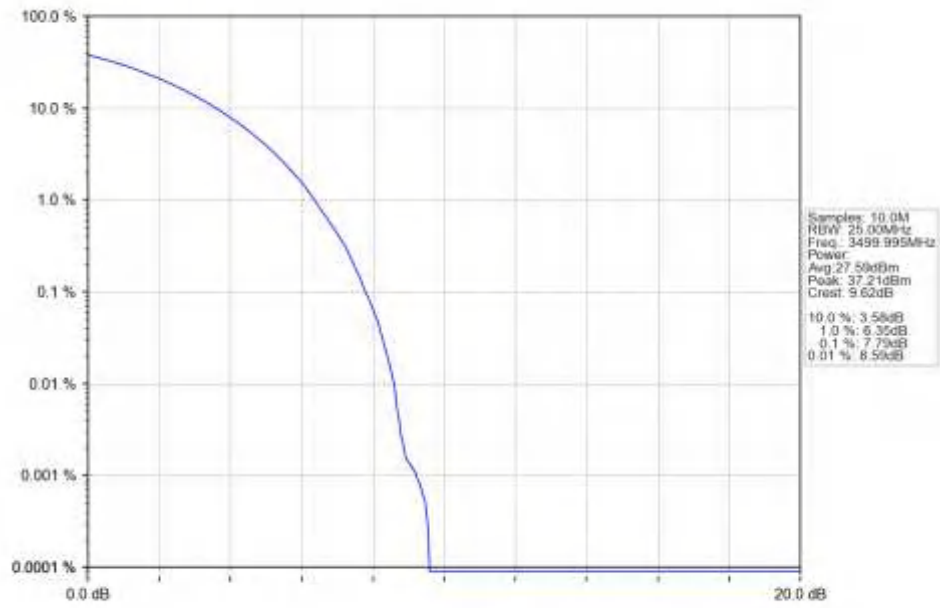
n77d_15kHz_SISO_NTNV_20MHz_CP-OFDM_16_QAM_3499.995MHz_Outer_Full_Ant1
