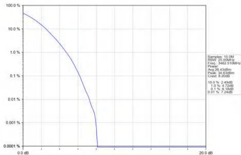
n77d_30kHz_SISO_NTNV_25MHz_DFT-s-OFDM_QPSK_3462.51MHz_Outer_Full_Ant1
