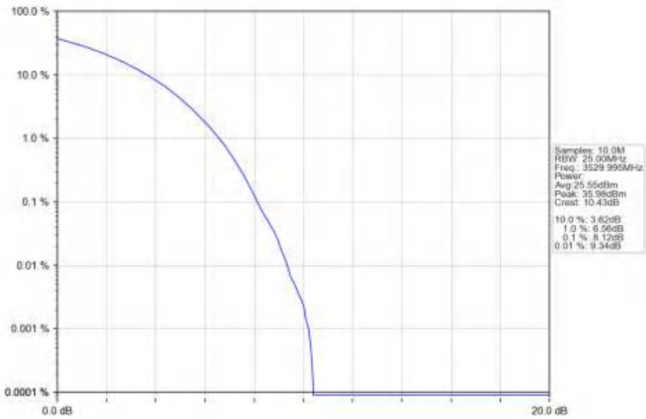
n77d_15kHz_SISO_NTNV_40MHz_CP-OFDM_64_QAM_3529.995MHz_Outer_Full_Ant1
