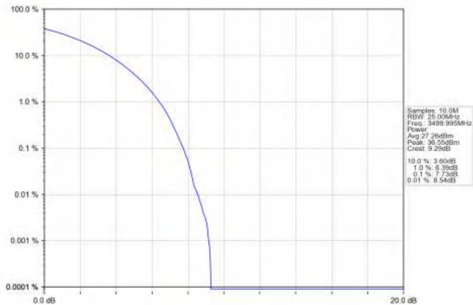
n77d_15kHz_SISO_NTNV_15MHz_CP-OFDM_QPSK_3499.995MHz_Outer_Full_Ant1
