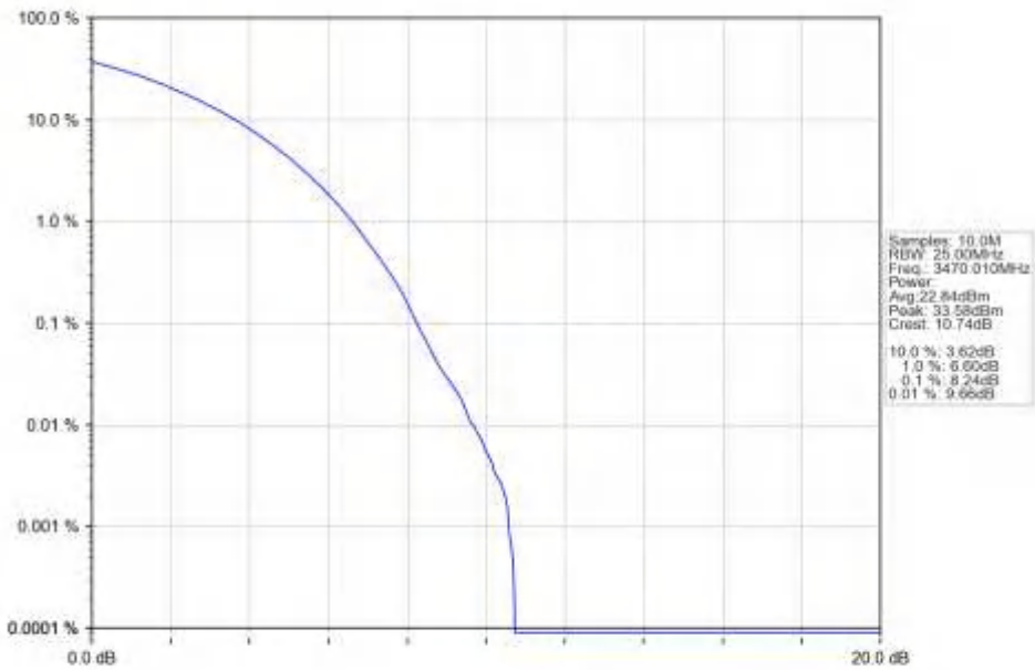
n77d_15kHz_SISO_NTNV_40MHz_CP-OFDM_256_QAM_3470.01MHz_Outer_Full_Ant1
