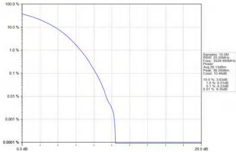
n77d_15kHz_SISO_NTNV_40MHz_CP-OFDM_QPSK_3529.995MHz_Outer_Full_Ant1
