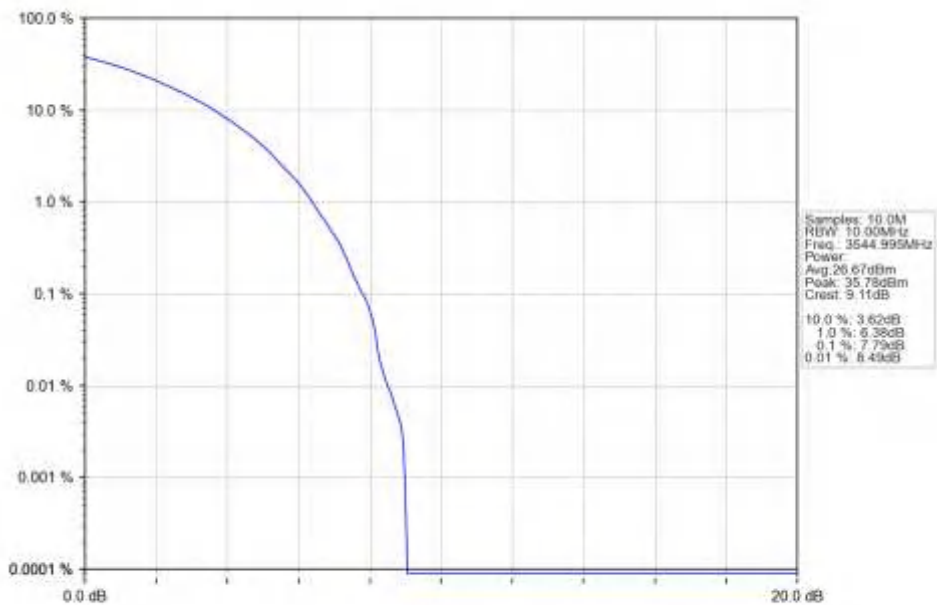
n77d_15kHz_SISO_NTNV_10MHz_CP-OFDM_QPSK_3544.995MHz_Outer_Full_Ant1
