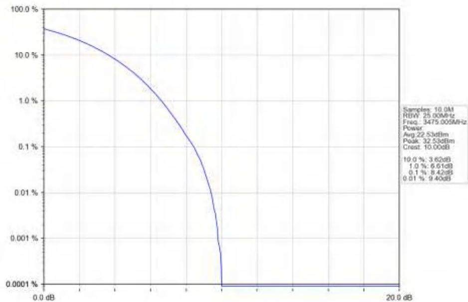
n77d_15kHz_SISO_NTNV_50MHz_CP-OFDM_256_QAM_3475.005MHz_Outer_Full_Ant1
