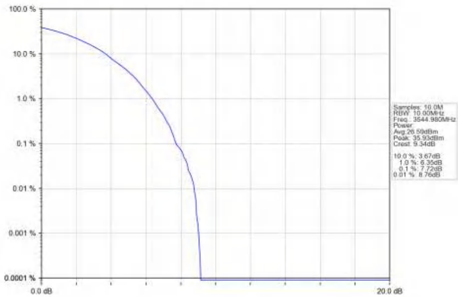
n77d_30kHz_SISO_NTNV_10MHz_CP-OFDM_64_QAM_3544.98MHz_Outer_Full_Ant1
