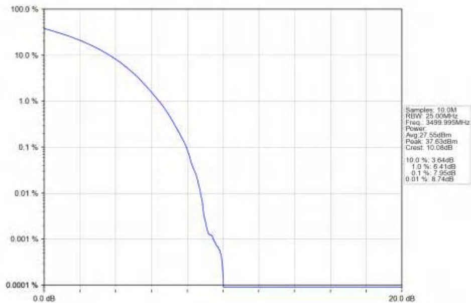
n77d_15kHz_SISO_NTNV_25MHz_CP-OFDM_QPSK_3499.995MHz_Outer_Full_Ant1
