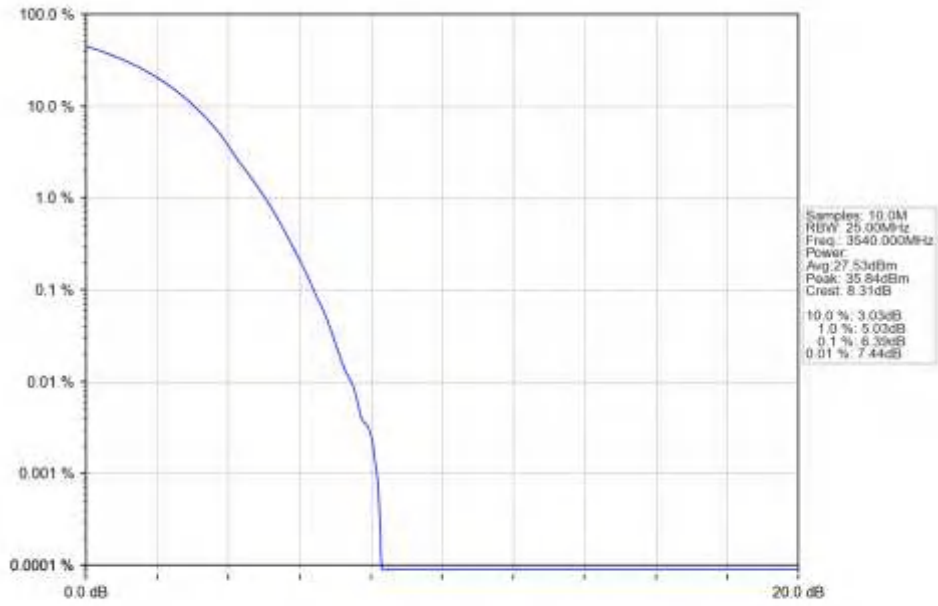
n77d_30kHz_SISO_NTNV_20MHz_DFT-s-OFDM_64_QAM_3540MHz_Outer_Full_Ant1
