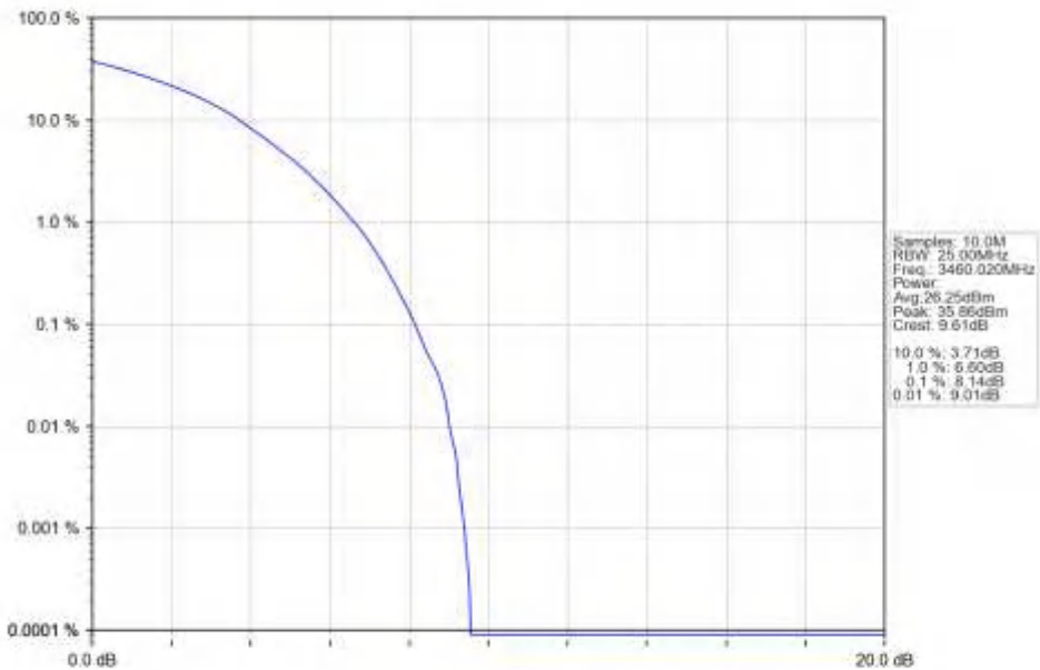
n77d_30kHz_SISO_NTNV_20MHz_CP-OFDM_QPSK_3460.02MHz_Outer_Full_Ant1
