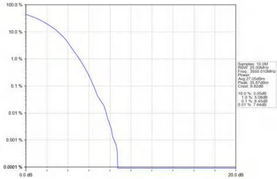
n77d_30kHz_SISO_NTNV_25MHz_DFT-s-OFDM_256_QAM_3500.01MHz_Outer_Full_Ant1
