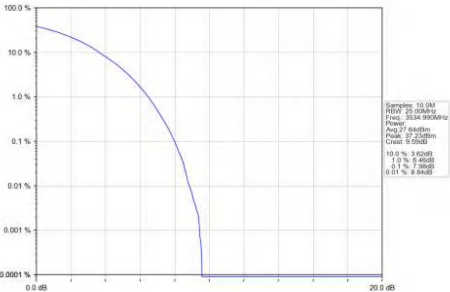
n77d_30kHz_SISO_NTNV_30MHz_CP-OFDM_16_QAM_3534.99MHz_Outer_Full_Ant1
