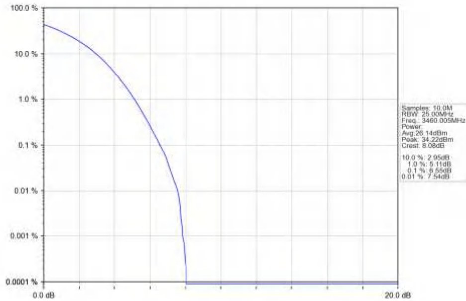
n77d_15kHz_SISO_NTNV_20MHz_DFT-s-OFDM_64_QAM_3460.005MHz_Outer_Full_Ant1
