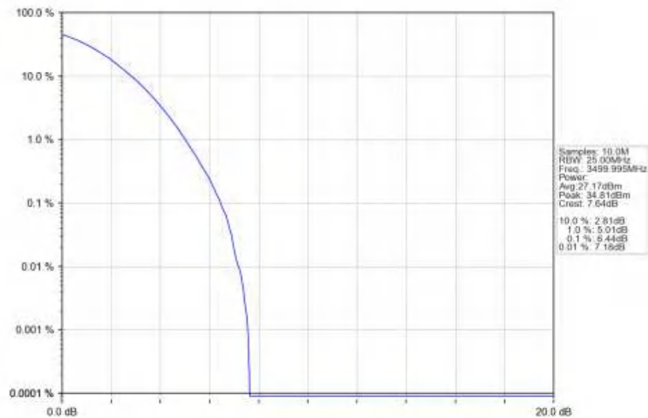
n77d_15kHz_SISO_NTNV_15MHz_DFT-s-OFDM_64_QAM_3499.995MHz_Outer_Full_Ant1
