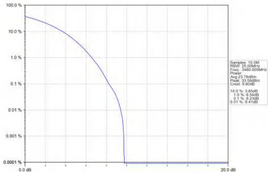
n77d_15kHz_SISO_NTNV_20MHz_CP-OFDM_256_QAM_3460.005MHz_Outer_Full_Ant1
