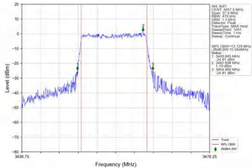
n77d_30kHz_SISO_NTNV_15MHz_DFT-s-OFDM_16_QAM_3457.5MHz_Outer_Full_Ant1
