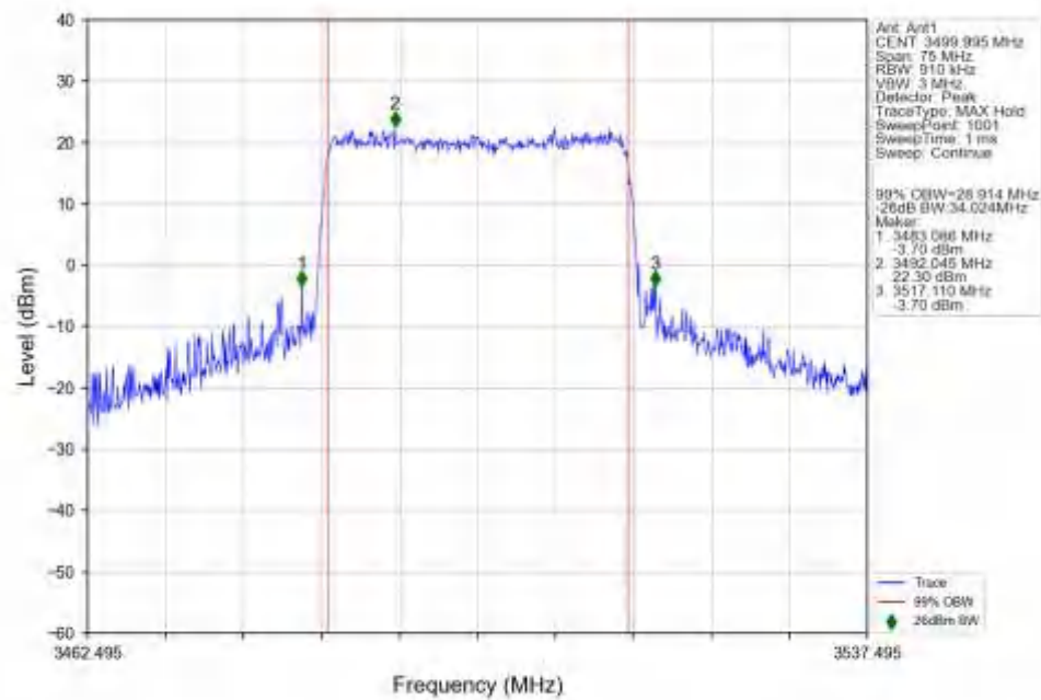
n77d_15kHz_SISO_NTNV_30MHz_CP-OFDM_64_QAM_3499.995MHz_Outer_Full_Ant1
