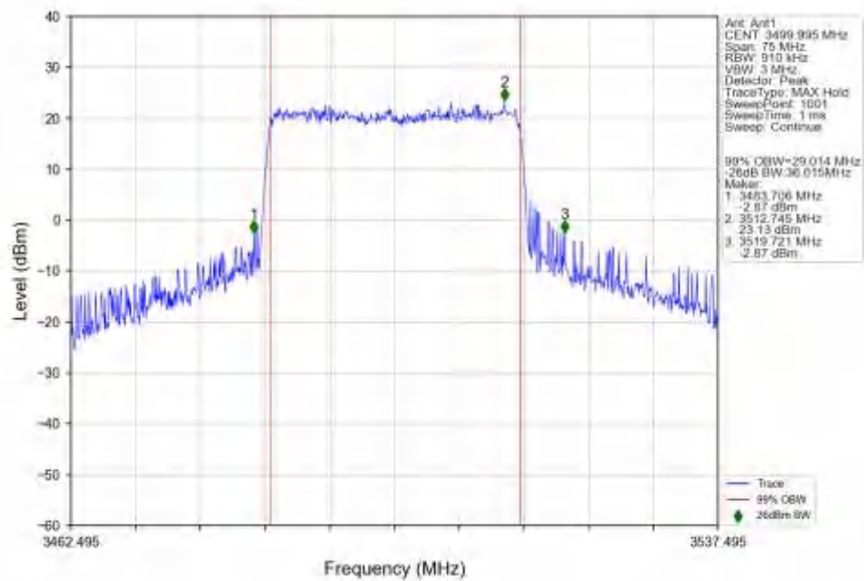
n77d_15kHz_SISO_NTNV_30MHz_CP-OFDM_QPSK_3499.995MHz_Outer_Full_Ant1
