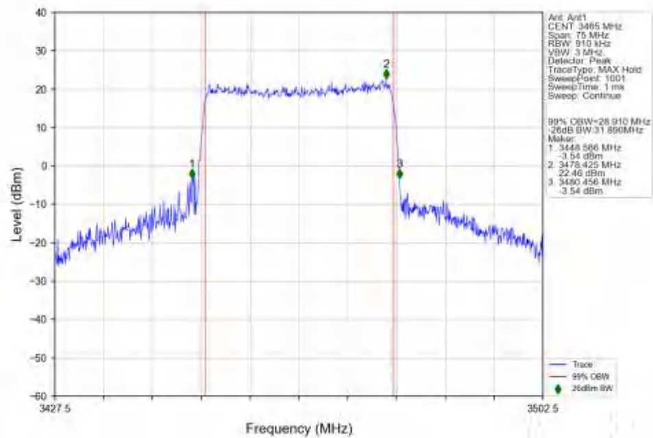
n77d_15kHz_SISO_NTNV_30MHz_CP-OFDM_16_QAM_3465MHz_Outer_Full_Ant1
