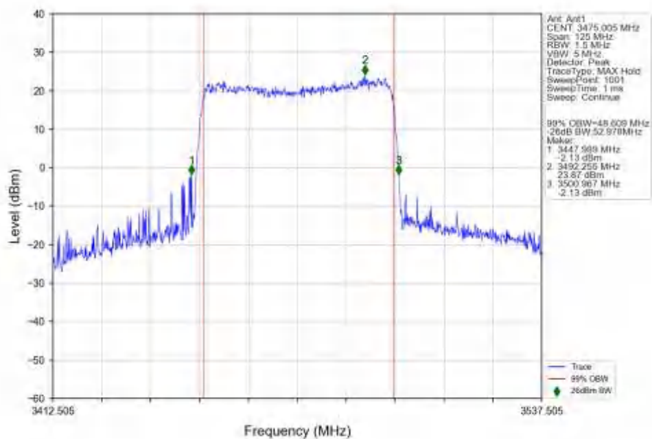
n77d_15kHz_SISO_NTNV_50MHz_DFT-s-OFDM_16_QAM_3475.005MHz_Outer_Full_Ant1
