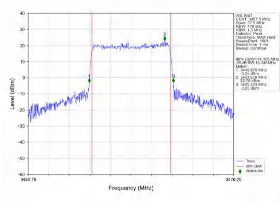
n77d_15kHz_SISO_NTNV_15MHz_CP-OFDM_16_QAM_3457.5MHz_Outer_Full_Ant1
