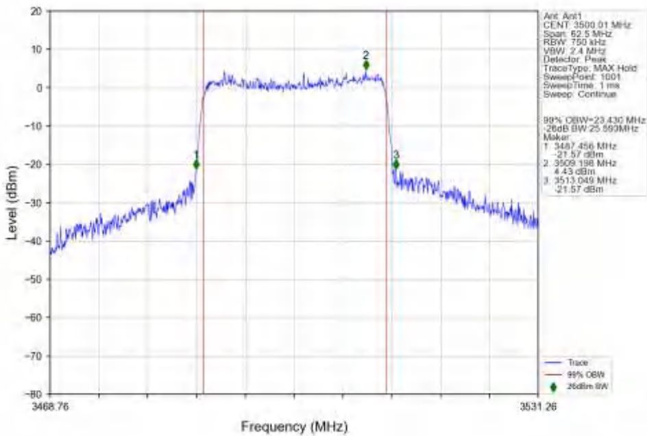
n77d_30kHz_SISO_NTNV_25MHz_CP-OFDM_QPSK_3500.01MHz_Outer_Full_Ant1
