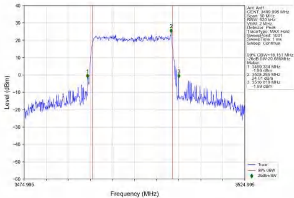
n77d_15kHz_SISO_NTNV_20MHz_DFT-s-OFDM_64_QAM_3499.995MHz_Outer_Full_Ant1
