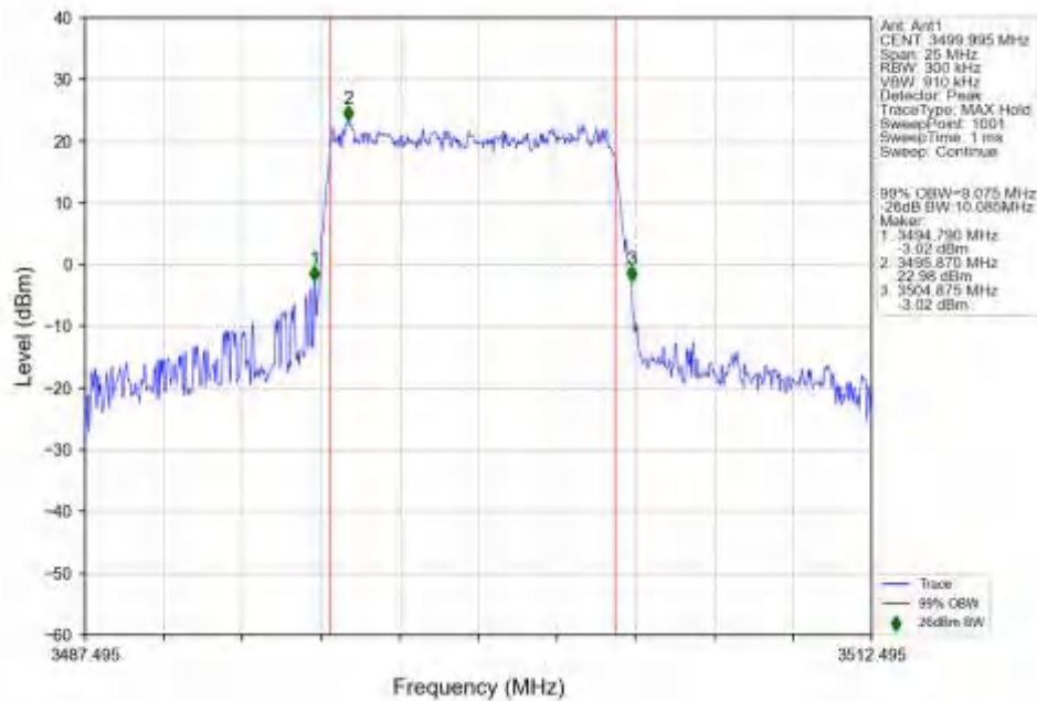
n77d_15kHz_SISO_NTNV_10MHz_DFT-s-OFDM_QPSK_3499.995MHz_Outer_Full_Ant1
