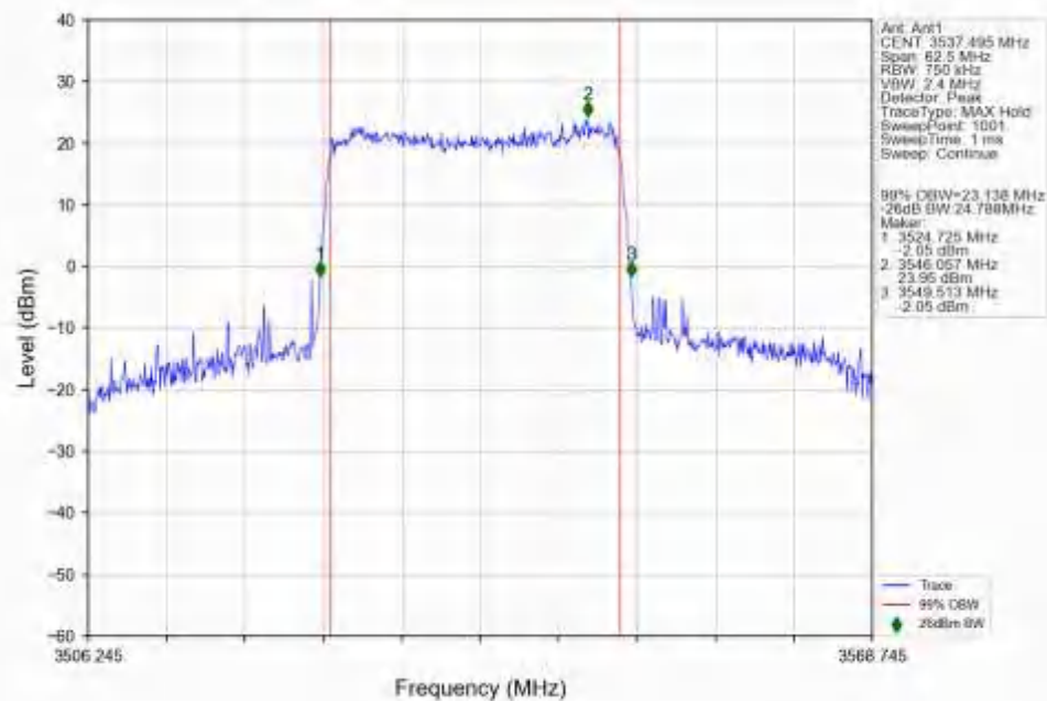
n77d_15kHz_SISO_NTNV_25MHz_DFT-s-OFDM_16_QAM_3537.495MHz_Outer_Full_Ant1
