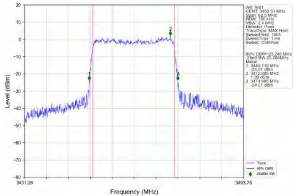
n77d_30kHz_SISO_NTNV_25MHz_DFT-s-OFDM_16_QAM_3462.51MHz_Outer_Full_Ant1
