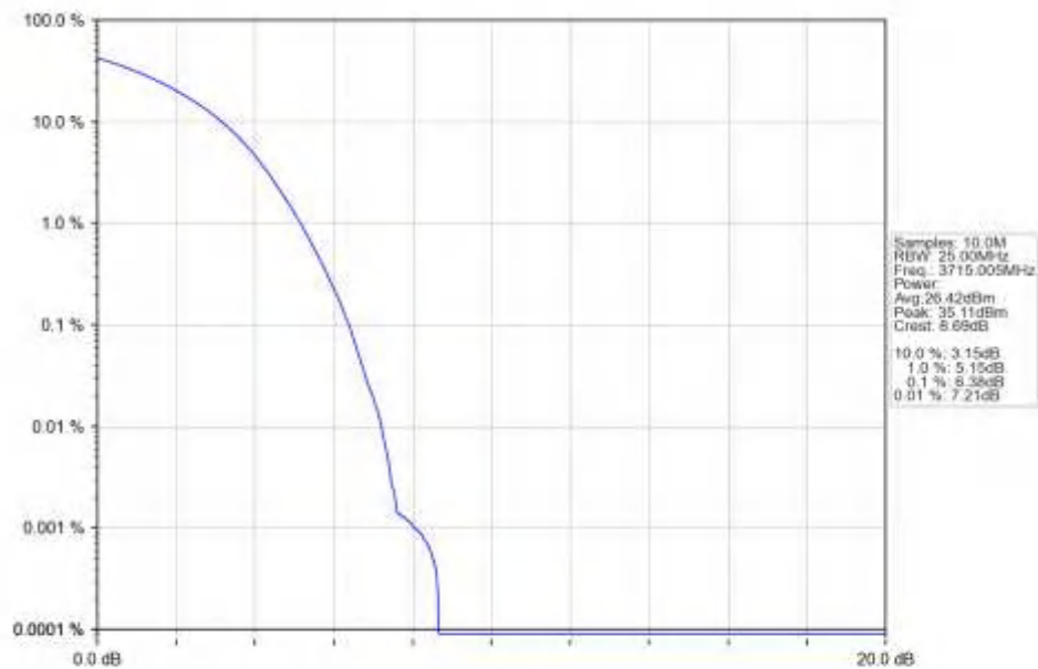
n77a_15kHz_SISO_NTNV_30MHz_DFT-s-OFDM_16_QAM_3715.005MHz_Outer_Full_Ant1
