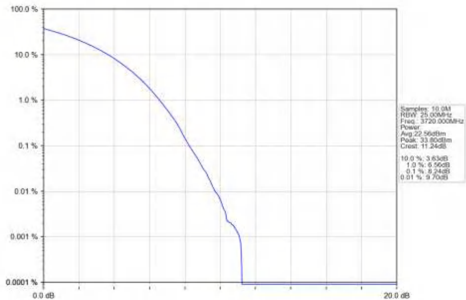
n77a_15kHz_SISO_NTNV_40MHz_CP-OFDM_256_QAM_3720MHz_Outer_Full_Ant1
