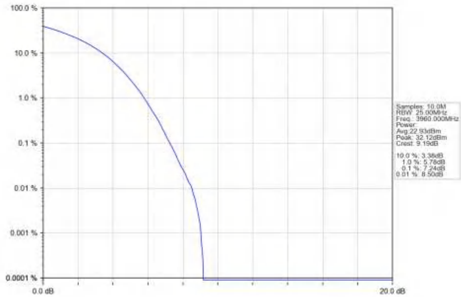
n77a_15kHz_SISO_NTNV_40MHz_DFT-s-OFDM_64_QAM_3960MHz_Outer_Full_Ant1
