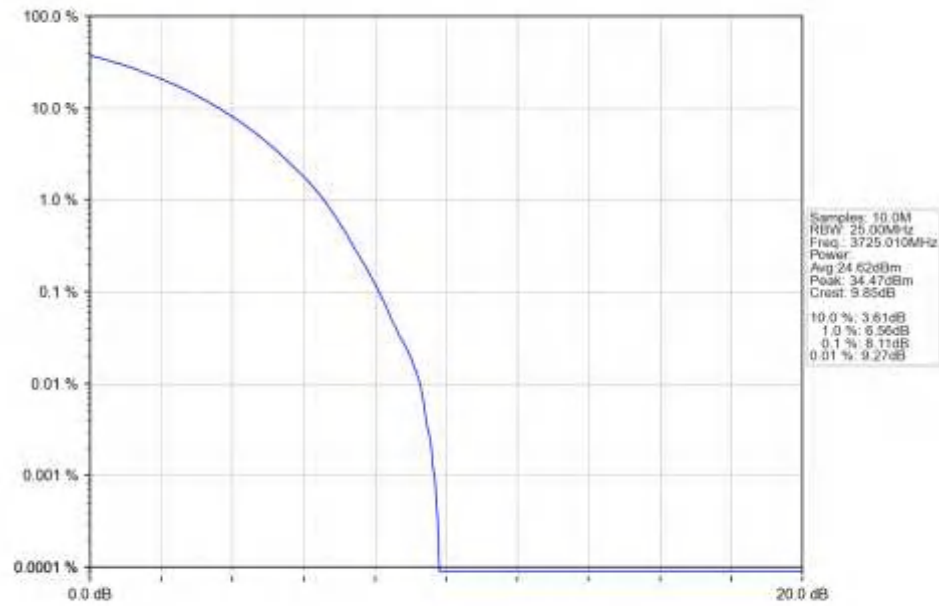
n77a_15kHz_SISO_NTNV_50MHz_CP-OFDM_QPSK_3725.01MHz_Outer_Full_Ant1
