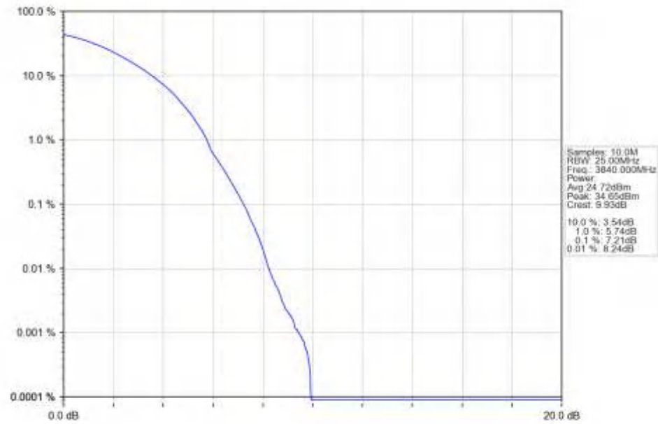
n77a_30kHz_SISO_NTNV_30MHz_DFT-s-OFDM_256_QAM_3840MHz_Outer_Full_Ant1
