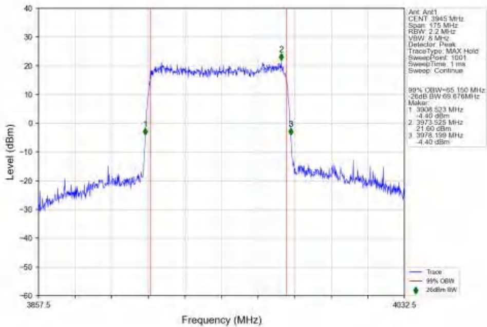
n77a_30kHz_SISO_NTNV_70MHz_DFT-s-OFDM_16_QAM_3945MHz_Outer_Full_Ant1
