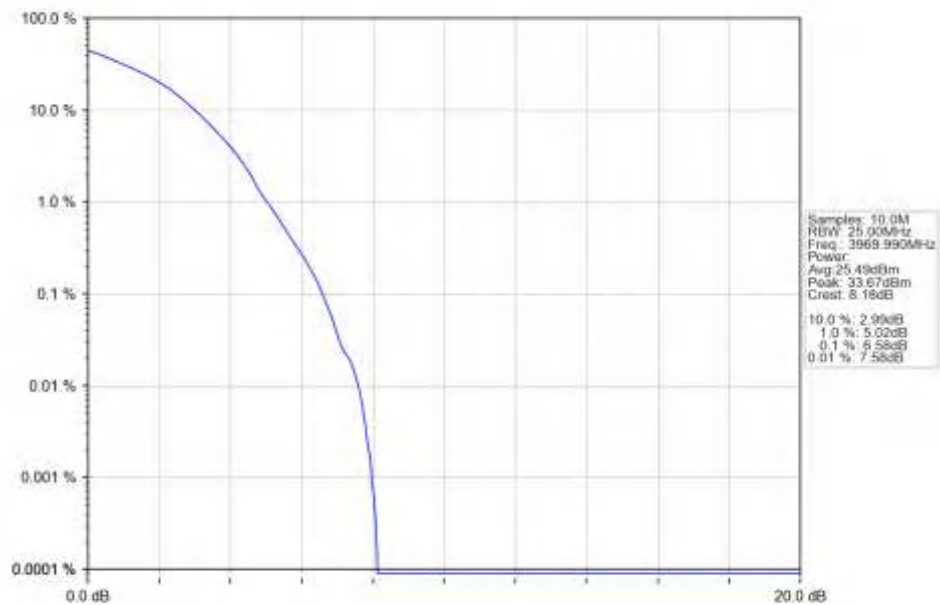
n77a 30kHz SISO NTN 20MHz DFT-s-OFDM 16 QAM 3969.99MHz Outer Full Ant1
