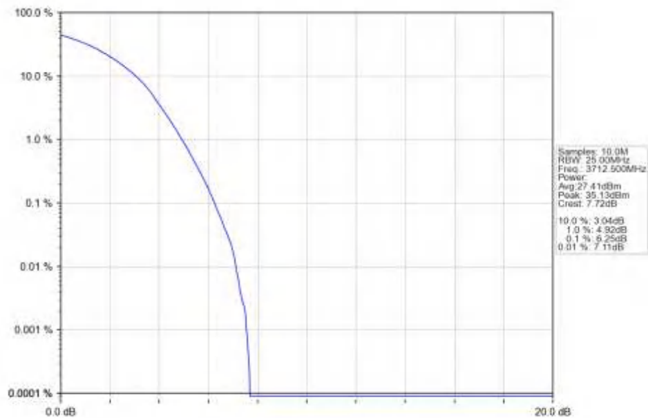
n77a 30kHz SISO NTN 25MHz DFT-s-OFDM 16 QAM 3712.5MHz Outer Full Ant1
