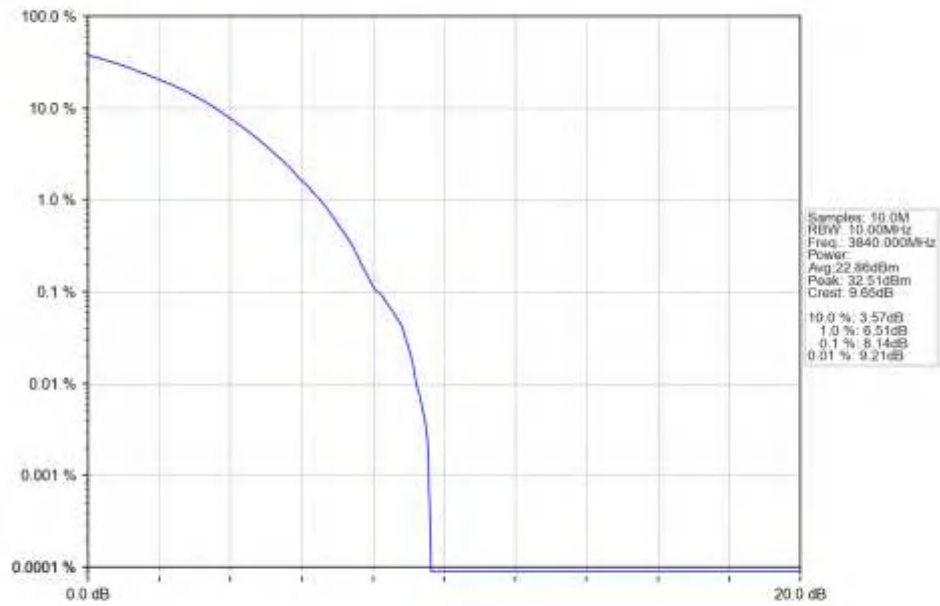
n77a_15kHz_SISO_NTNV_10MHz_CP-OFDM_256_QAM_3840MHz_Outer_Full_Ant1
