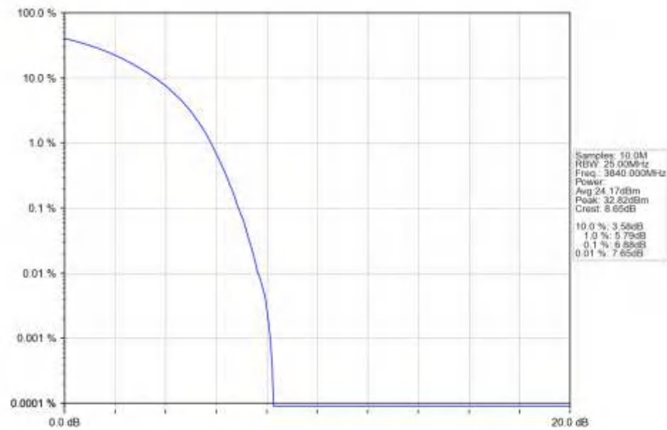
n77a_30kHz_SISO_NTNV_50MHz_DFT-s-OFDM QPSK_3840MHz_Outer_Full_Ant1
