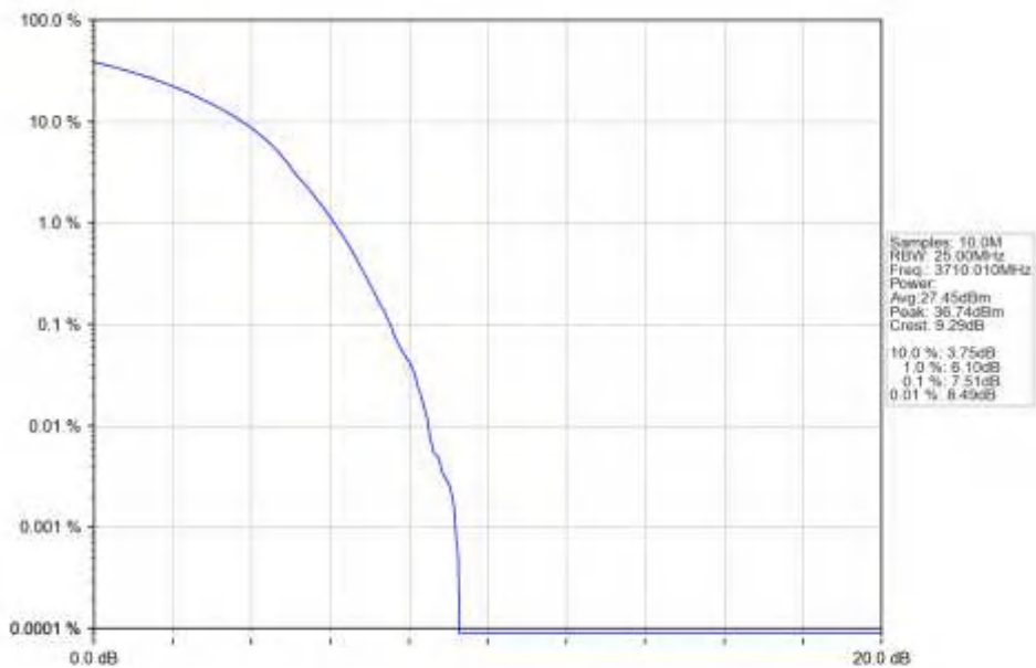
n77a_30kHz_SISO_NTNV_20MHz_CP-OFDM_16QAM_3710.01MHz_Outer_Full_Ant1
