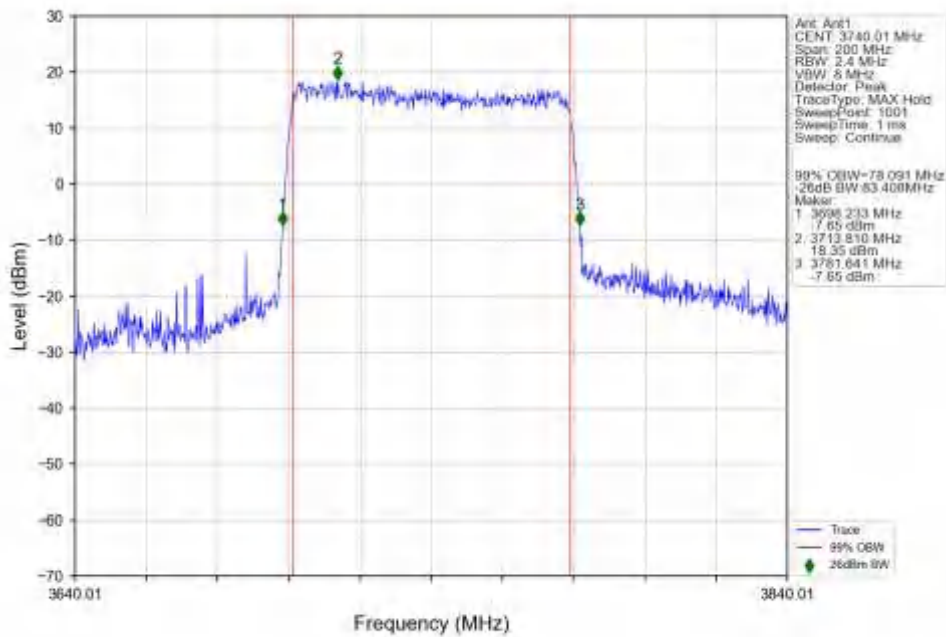
n77a 30kHz SISO NTN 80MHz CP-OFDM 256 QAM 3740.01MHz Outer Full Ant1
