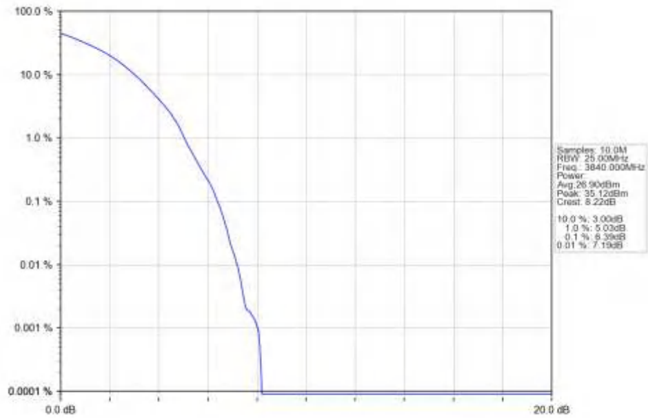
n77a 30kHz SISO NTN 20MHz DFT-s-OFDM 16 QAM 3840MHz Outer Full Ant1
