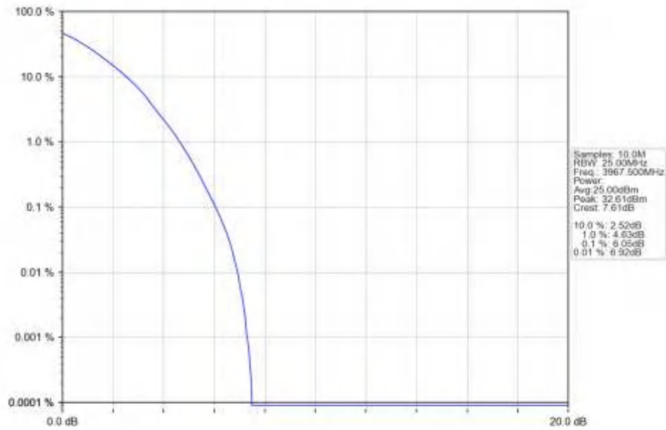
n77a 30kHz SISO NTN 25MHz DFT-s-OFDM QPSK 3967.5MHz Outer Full Ant1
