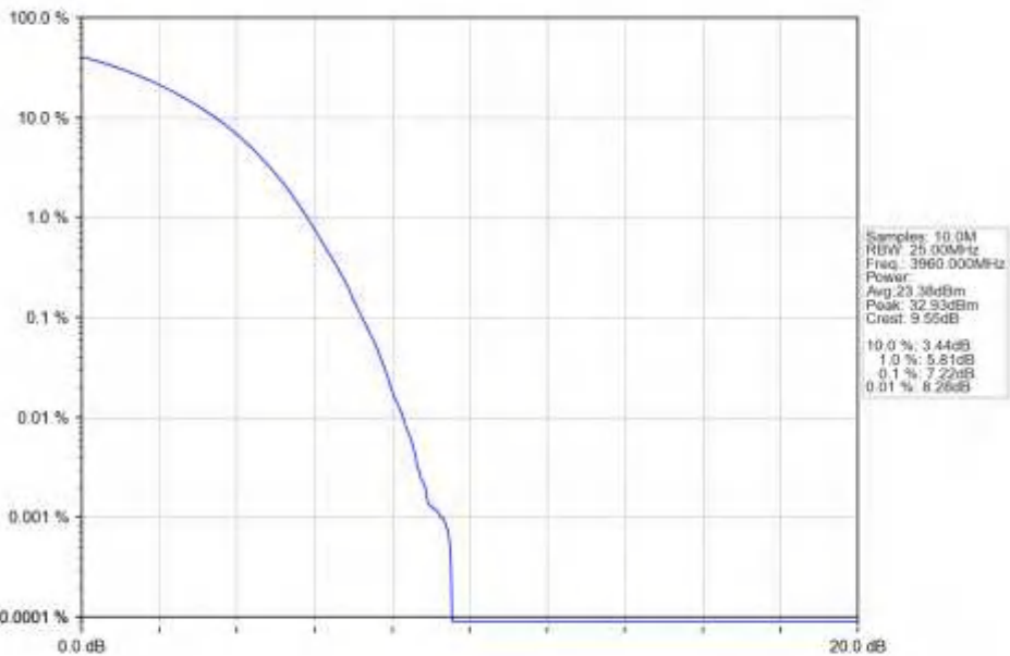
n77a_30kHz_SISO_NTNV_40MHz_DFT-s-OFDM_16_QAM_3960MHz_Outer_Full_Ant1
