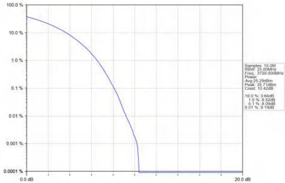
n77a 15kHz SISO NTN 40MHz CP-OFDM QPSK 3720MHz Outer Full Ant1
