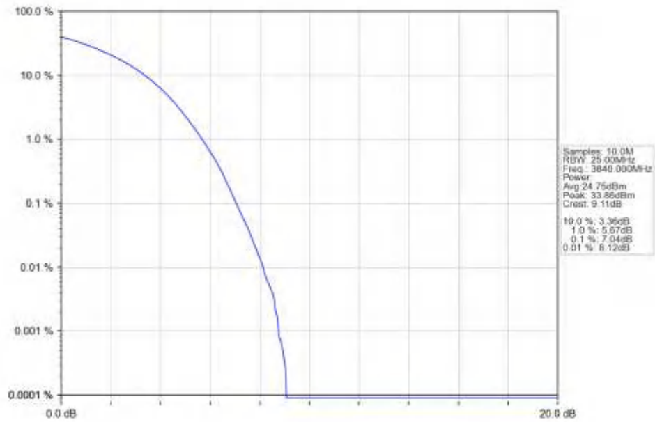
n77a_15kHz_SISO_NTNV_40MHz_DFT-s-OFDM_16_QAM_3840MHz_Outer_Full_Ant1
