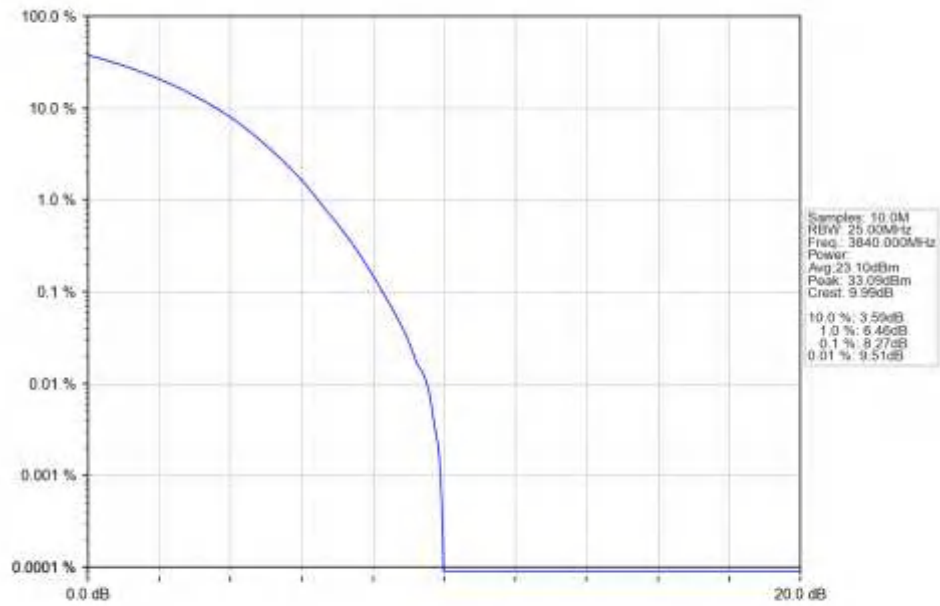
n77a_15kHz_SISO_NTNV_20MHz_CP-OFDM_256_QAM_3840MHz_Outer_Full_Ant1
