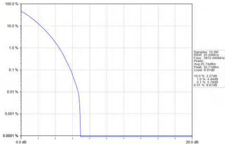
n77a_15kHz_SISO_NTNV_15MHz_DFT-s-OFDM_QPSK_3972.495MHz_Outer_Full_Ant1
