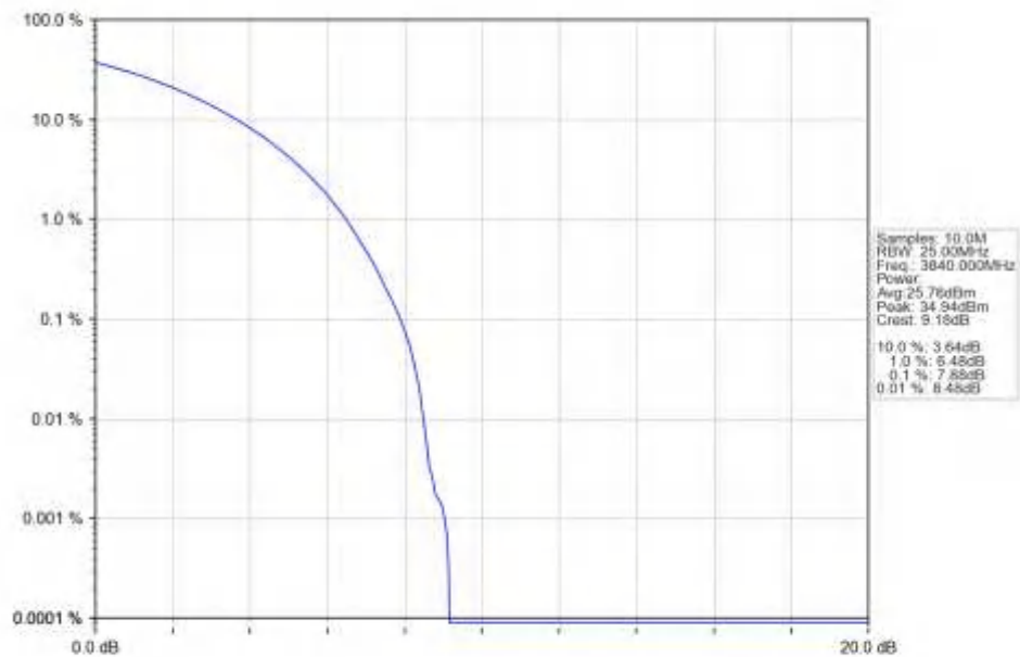
n77a 15kHz SISO NTN 20MHz CP-OFDM 64 QAM 3840MHz Outer Full Ant1
