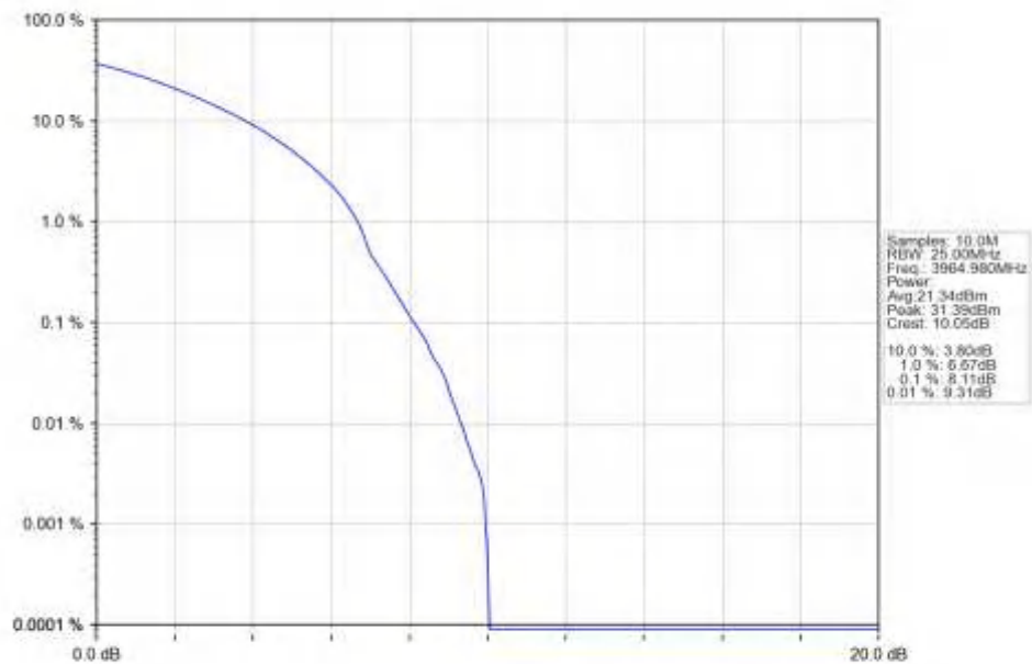
n77a_30kHz_SISO_NTNV_30MHz_CP-OFDM_256_QAM_3964.98MHz_Outer_Full_Ant1
