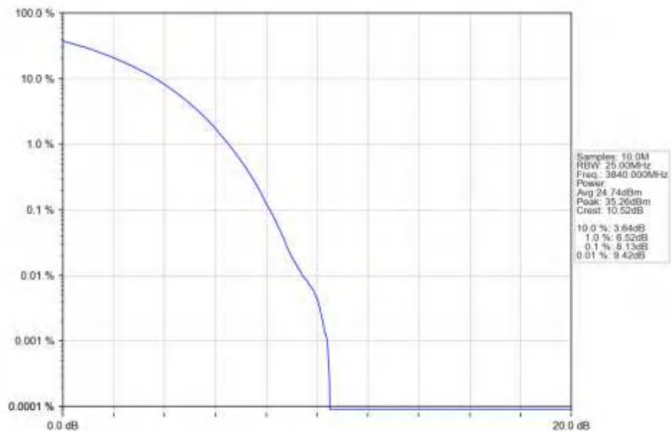
n77a 15kHz SISO NTN 40MHz CP-OFDM QPSK 3840MHz Outer Full Ant1
