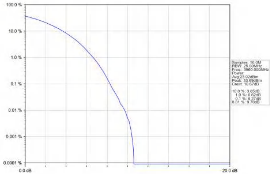
n77a 15kHz SISO NTN 40MHz CP-OFDM QPSK 3960MHz Outer Full Ant1
