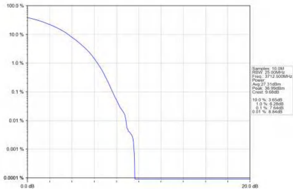
n77a_30kHz_SISO_NTNV_25MHz_CP-OFDM 16 QAM 3712.5MHz_Outer_Full_Ant1
