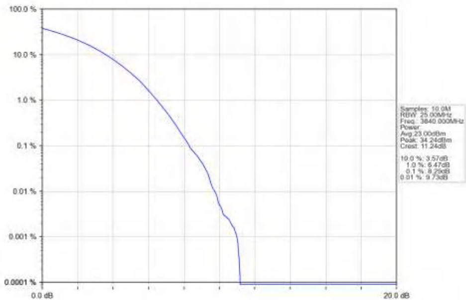
n77a_15kHz_SISO_NTNV_25MHz_CP-OFDM_256_QAM_3840MHz_Outer_Full_Ant1
