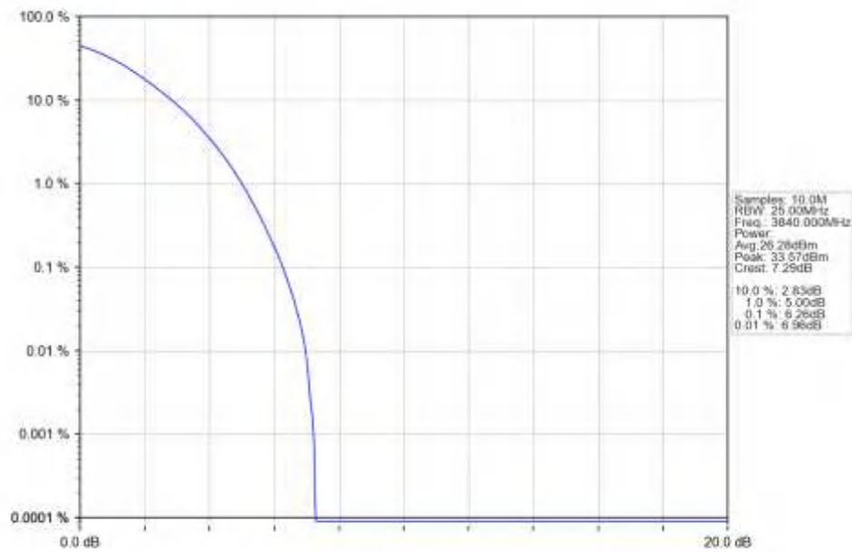
n77a_15kHz_SISO_NTNV_15MHz_DFT-s-OFDM_64_QAM_3840MHz_Outer_Full_Ant1
