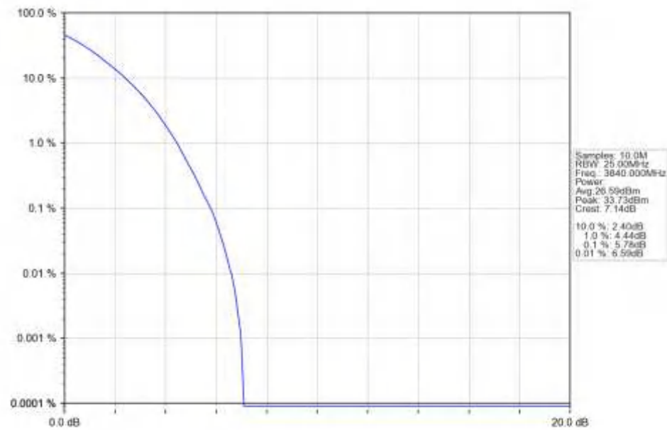
n77a_15kHz_SISO_NTNV_20MHz_DFT-s-OFDM_QPSK_3840MHz_Outer_Full_Ant1
