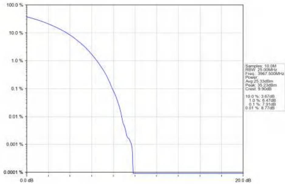
n77a_15kHz_SISO_NTNV_25MHz_CP-OFDM QPSK_3967.5MHz_Outer_Full_Ant1
