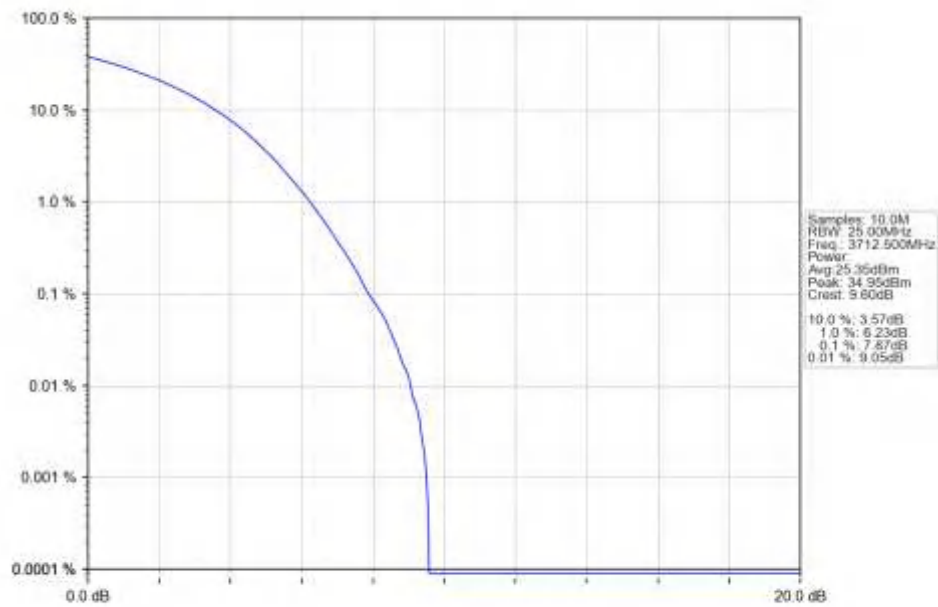
n77a_15kHz_SISO_NTNV_25MHz_CP-OFDM 16 QAM 3712.5MHz_Outer_Full_Ant1
