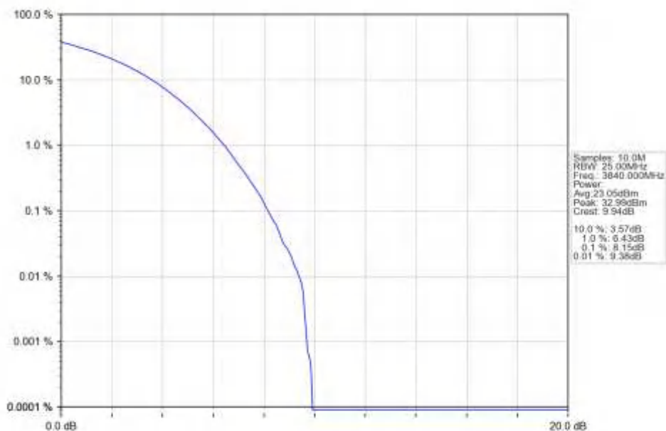
n77a_15kHz_SISO_NTNV_15MHz_CP-OFDM_256_QAM_3840MHz_Outer_Full_Ant1
