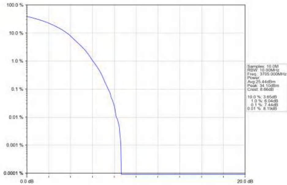
n77a 30kHz SISO NTN 10MHz CP-OFDM QPSK 3705MHz Outer Full Ant1
