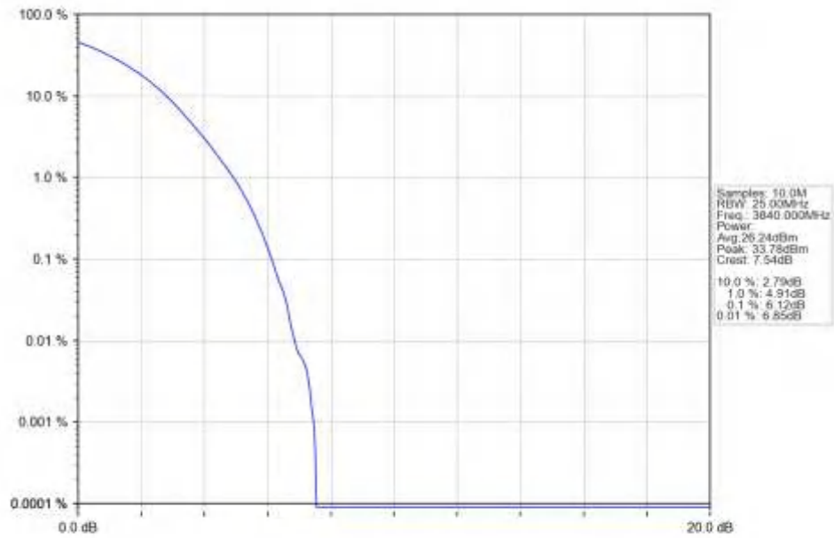
n77a_15kHz_SISO_NTNV_15MHz_DFT-s-OFDM_16_QAM_3840MHz_Outer_Full_Ant1
