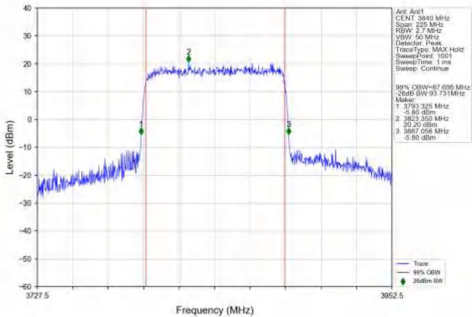
n77a_30kHz_SISO_NTNV_90MHz_CP-OFDM_64_QAM_3840MHz_Outer_Full_Ant1
