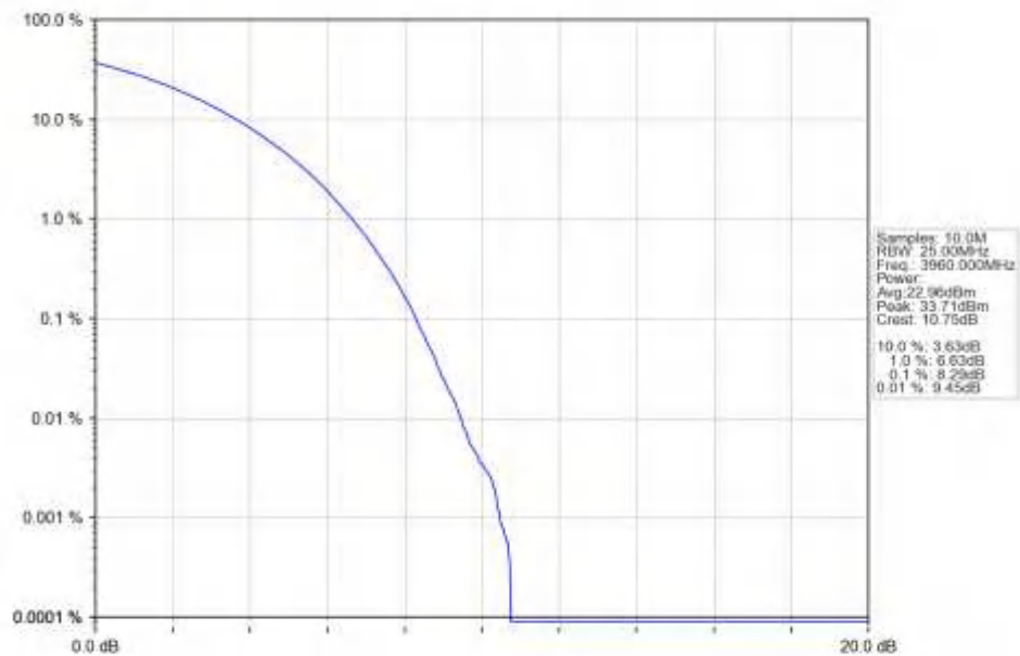
n77a_15kHz_SISO_NTNV_40MHz_CP-OFDM_16_QAM_3960MHz_Outer_Full_Ant1
