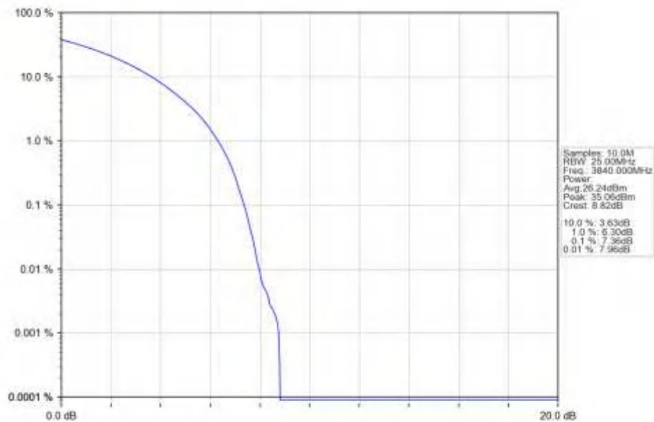
n77a_15kHz_SISO_NTNV_15MHz_CP-OFDM_QPSK_3840MHz_Outer_Full_Ant1
