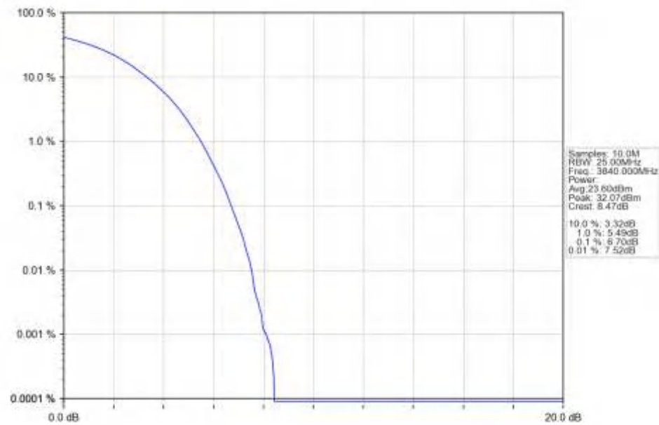
n77a_15kHz_SISO_NTNV_50MHz_DFT-s-OFDM QPSK_3840MHz_Outer_Full_Ant1
