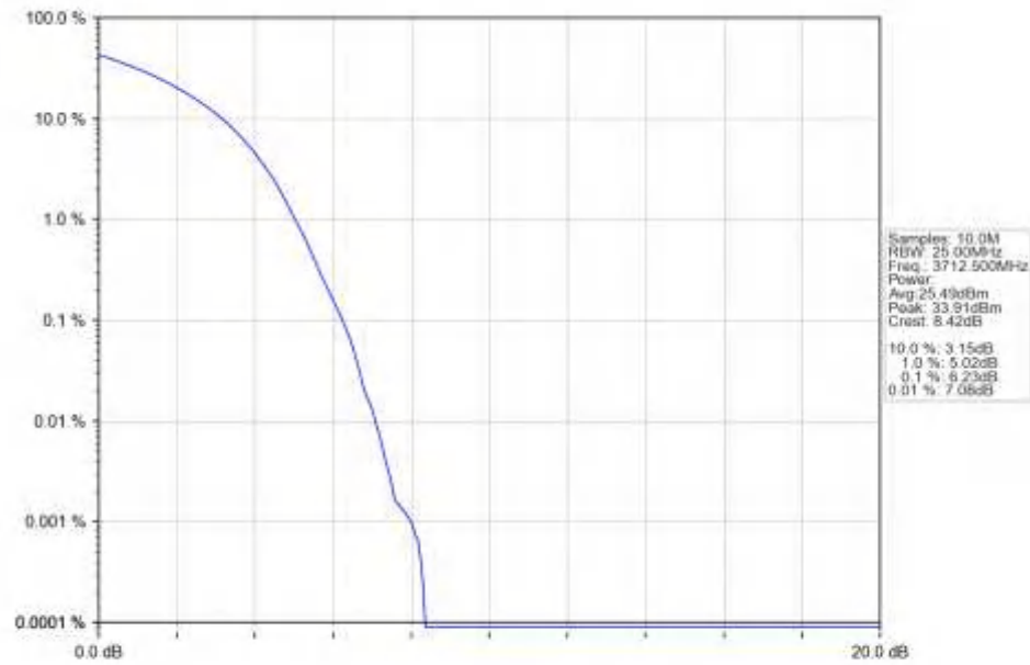
n77a_15kHz_SISO_NTNV_25MHz_DFT-s-OFDM_64_QAM_3712.5MHz_Outer_Full_Ant1
