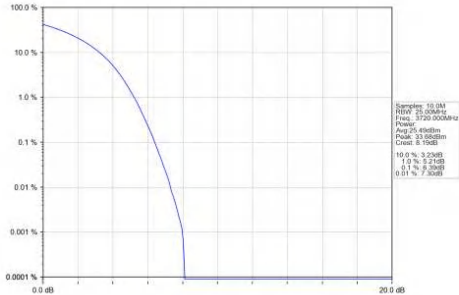
n77a_15kHz_SISO_NTNV_40MHz_DFT-s-OFDM QPSK_3720MHz_Outer_Full_Ant1
