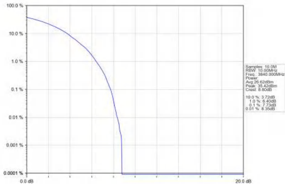
n77a 30kHz SISO NTN 10MHz CP-OFDM QPSK 3840MHz Outer Full Ant1
