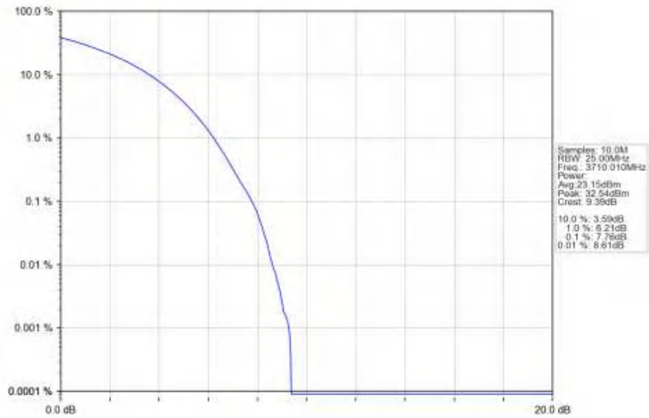
n77a 15kHz SISO NTN 20MHz CP-OFDM 64 QAM 3710.01MHz Outer Full Ant1
