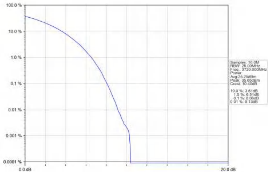
n77a 15kHz SISO NTN 40MHz CP-OFDM 16 QAM 3720MHz Outer Full Ant1
