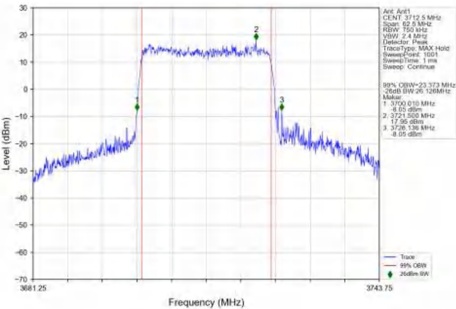
n77a_30kHz_SISO_NTNV_25MHz_CP-OFDM_256_QAM_3712.5MHz_Outer_Full_Ant1
