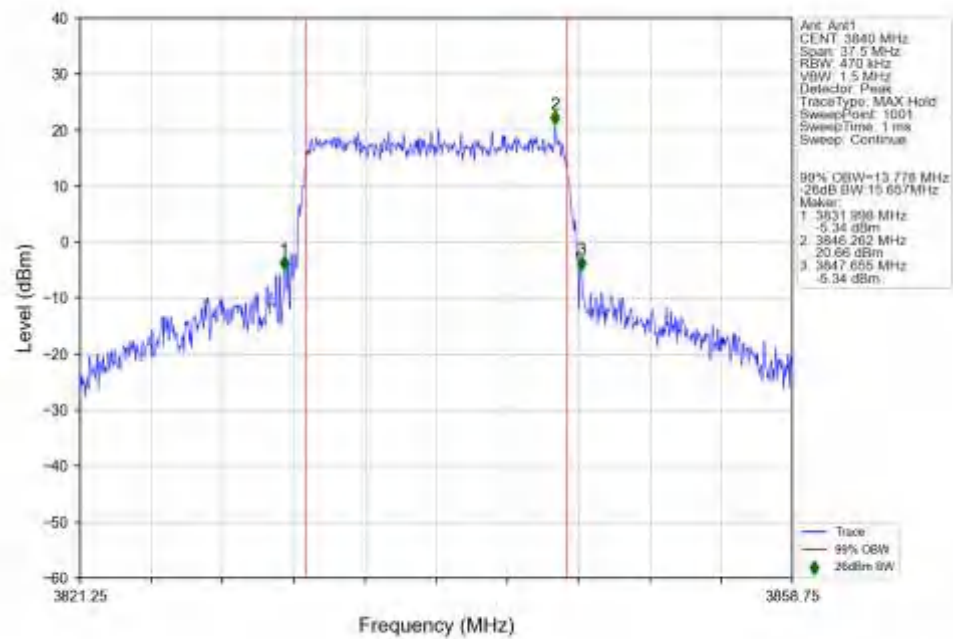
n77a_30kHz_SISO_NTNV_15MHz_CP-OFDM_QPSK_3840MHz_Outer_Full_Ant1
