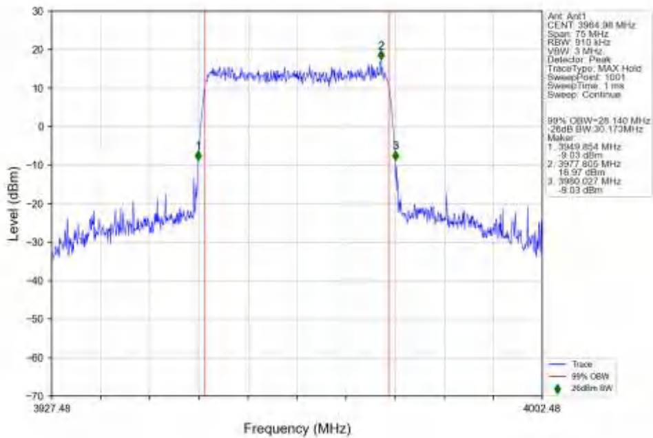
n77a_30kHz_SISO_NTNV_30MHz_CP-OFDM_256_QAM_3964.98MHz_Outer_Full_Ant1
