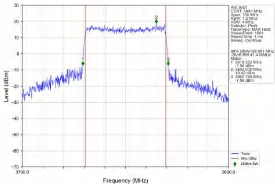
n77a_15kHz_SISO_NTNV_40MHz_CP-OFDM_QPSK_3840MHz_Outer_Full_Ant1
