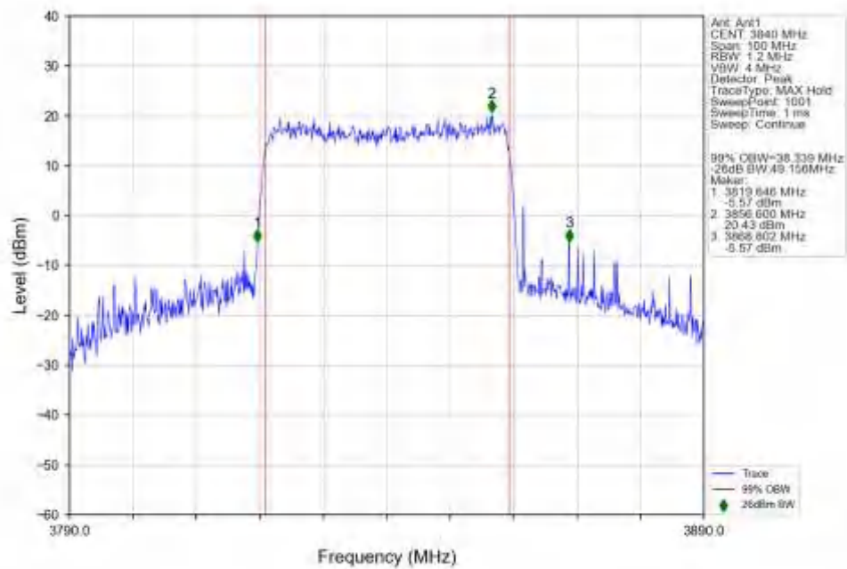
n77a_30kHz_SISO_NTNV_40MHz_CP-OFDM_64_QAM_3840MHz_Outer_Full_Ant1
