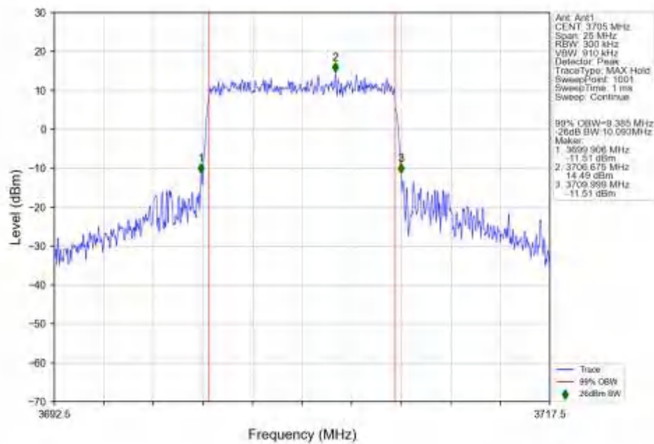
n77a_15kHz_SISO_NTNV_10MHz_CP-OFDM_256_QAM_3705MHz_Outer_Full_Ant1
