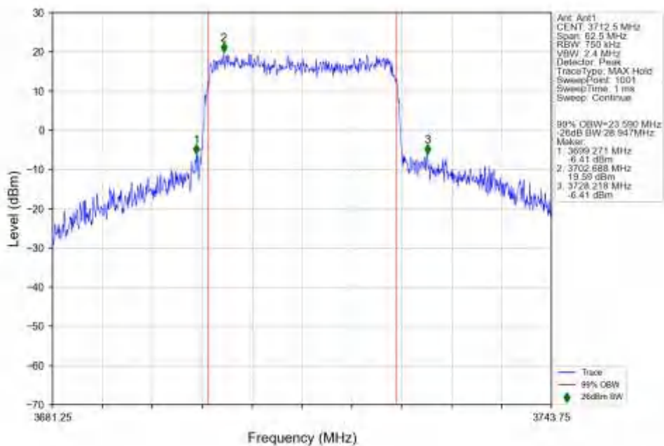
n77a_30kHz_SISO_NTNV_25MHz_CP-OFDM 16 QAM_3712.5MHz_Outer_Full_Ant1
