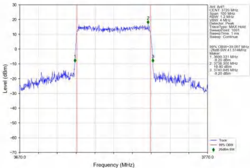
n77a_15kHz_SISO_NTNV_40MHz_DFT-s-OFDM_256_QAM_3720MHz_Outer_Full_Ant1
