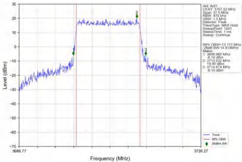
n77a_30kHz_SISO_NTNV_15MHz_DFT-s-OFDM_16_QAM_3707.52MHz_Outer_Full_Ant1
