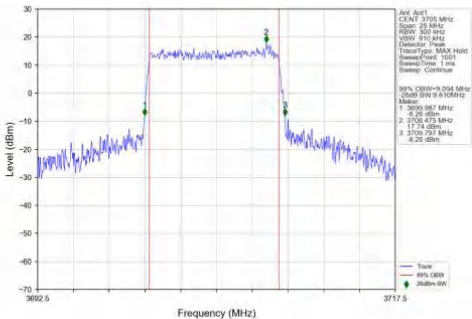
n77a_15kHz_SISO_NTNV_10MHz_DFT-s-OFDM_16_QAM_3705MHz_Outer_Full_Ant1
