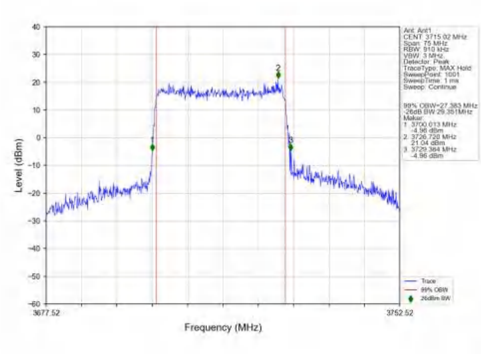
n77a_30kHz_SISO_NTNV_30MHz_DFT-s-OFDM_16_QAM_3715.02MHz_Outer_Full_Ant1
