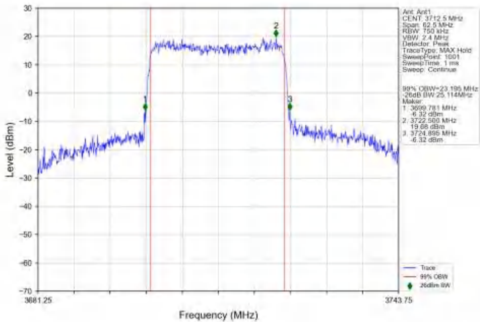
n77a_30kHz_SISO_NTNV_25MHz_DFT-s-OFDM_16_QAM_3712.5MHz_Outer_Full_Ant1
