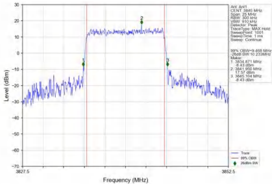
n77a_15kHz_SISO_NTNV_10MHz_CP-OFDM_64_QAM_3840MHz_Outer_Full_Ant1
