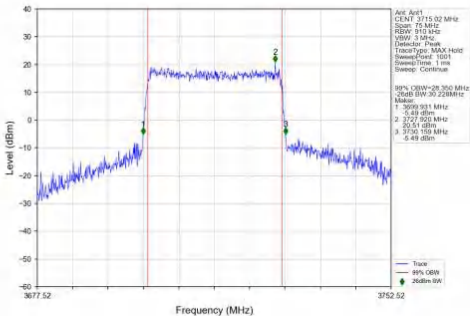
n77a_30kHz_SISO_NTNV_30MHz_CP-OFDM_16_QAM_3715.02MHz_Outer_Full_Ant1
