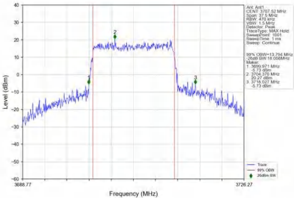
n77a_30kHz_SISO_NTNV_15MHz_CP-OFDM_16QAM_3707.52MHz_Outer_Full_Ant1
