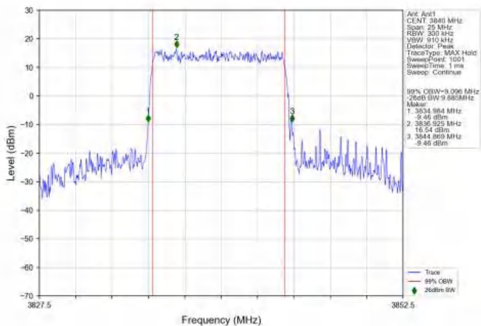
n77a_15kHz_SISO_NTNV_10MHz_DFT-s-OFDM_64_QAM_3840MHz_Outer_Full_Ant1
