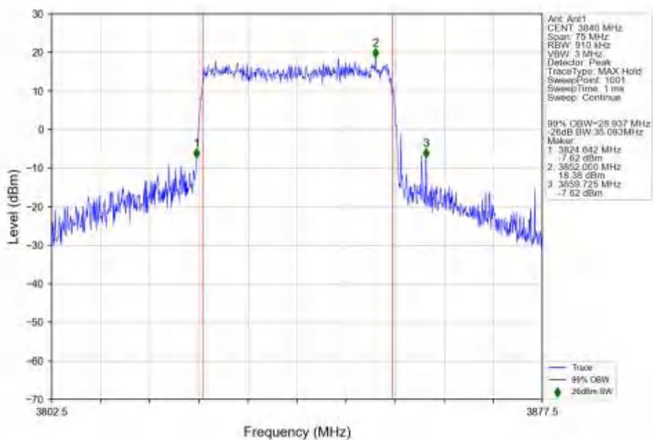
n77a_15kHz_SISO_NTNV_30MHz_CP-OFDM_QPSK_3840MHz_Outer_Full_Ant1
