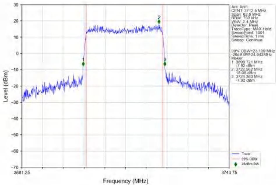
n77a_15kHz_SISO_NTNV_25MHz_DFT-s-OFDM_16_QAM_3712.5MHz_Outer_Full_Ant1
