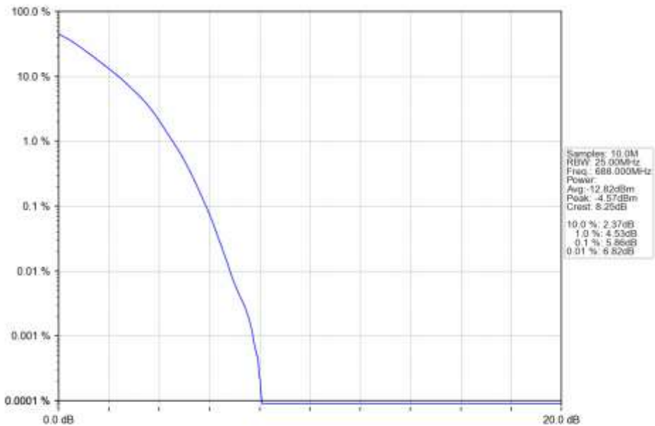
n71_15kHz_SISO_NTNV_20MHz_DFT-s-OFDM_QPSK_688MHz_Outer_Full_Ant1
