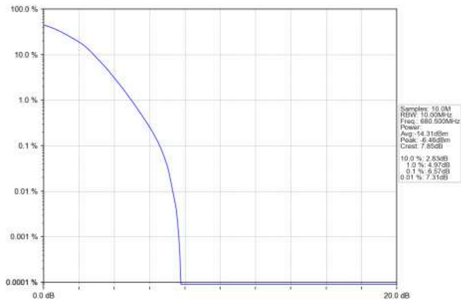
n71_30kHz_SISO_NTNV_10MHz_DFT-s-OFDM_64_QAM_680.5MHz_Outer_Full_Ant1
