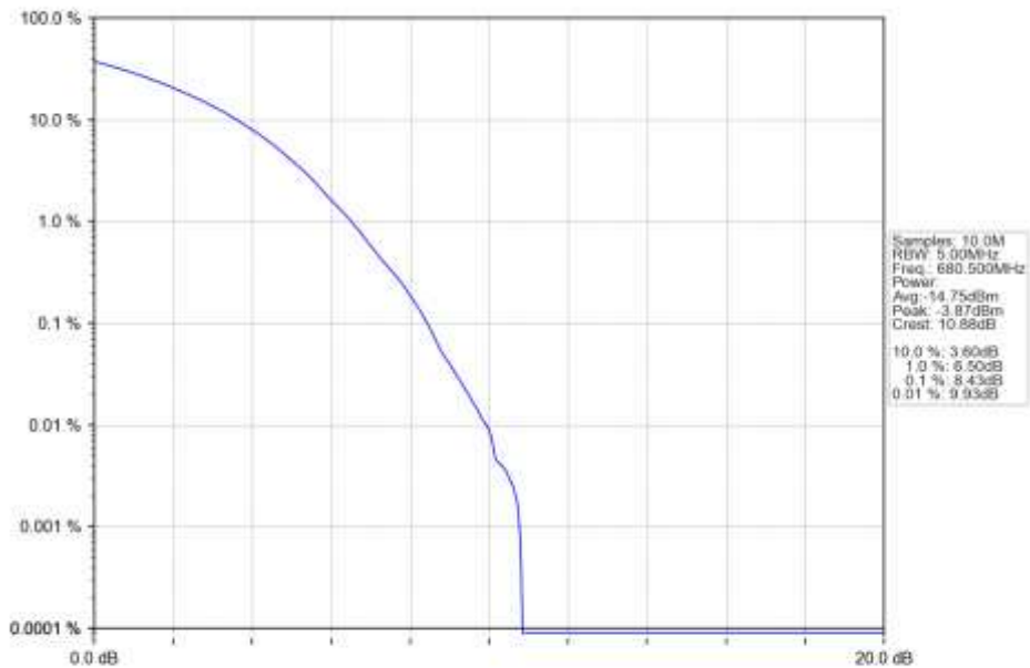
n71_15kHz_SISO_NTNV_5MHz_CP-OFDM_64_QAM_680.5MHz_Outer_Full_Ant1
