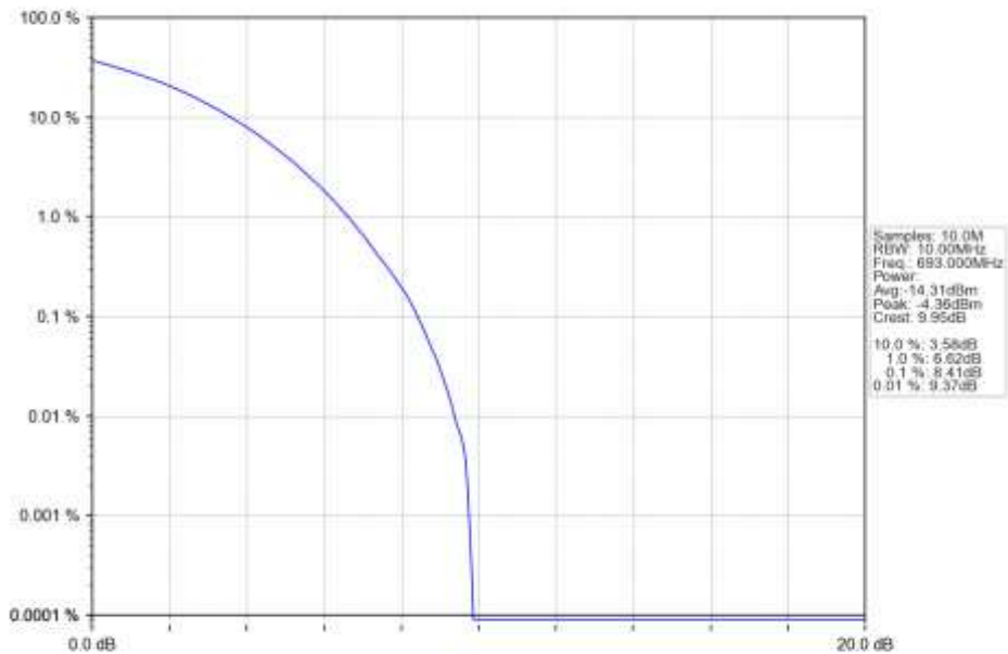
n71_30kHz_SISO_NTNV_10MHz_CP-OFDM_QPSK_693MHz_Outer_Full_Ant1
