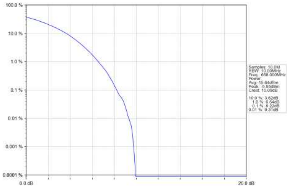
n71_30kHz_SISO_NTNV_10MHz_CP-OFDM_16_QAM_668MHz_Outer_Full_Ant1
