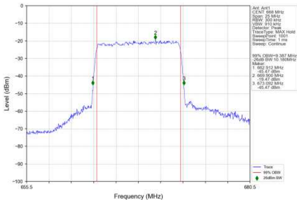
n71_15kHz_SISO_NTNV_10MHz_CP-OFDM_16_QAM_668MHz_Outer_Full_Ant1
