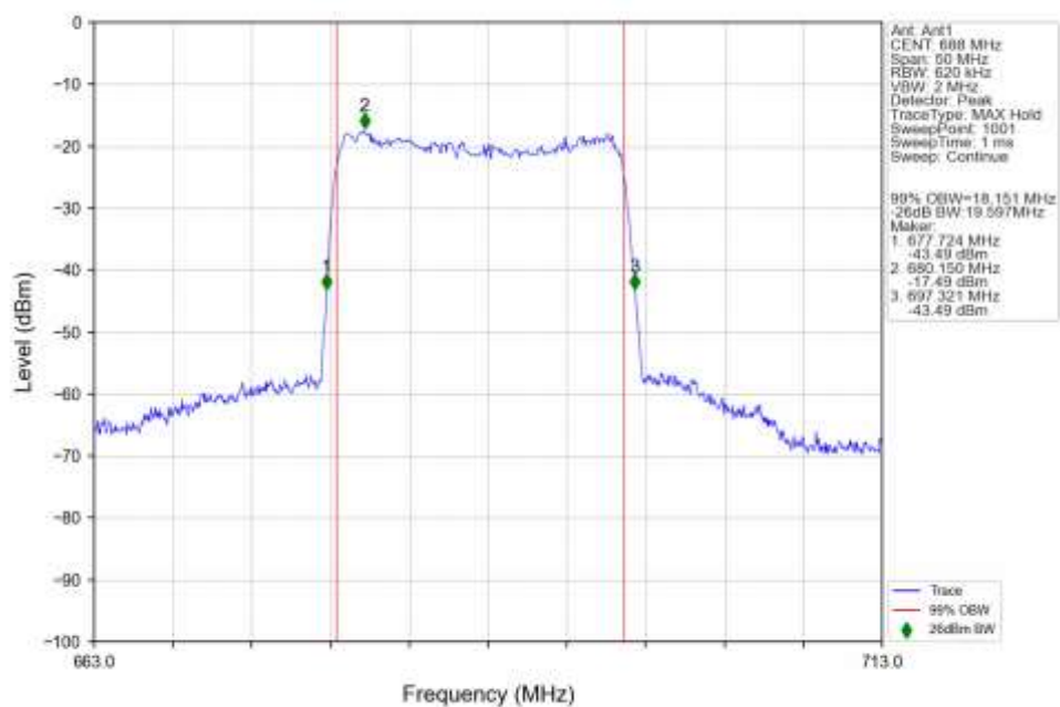
n71_15kHz_SISO_NTNV_20MHz_DFT-s-OFDM_16_QAM_688MHz_Outer_Full_Ant1
