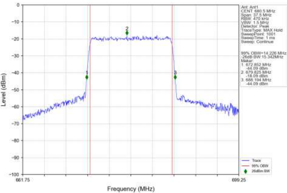
n71_15kHz_SISO_NTNV_15MHz_CP-OFDM_QPSK_680.5MHz_Outer_Full_Ant1
