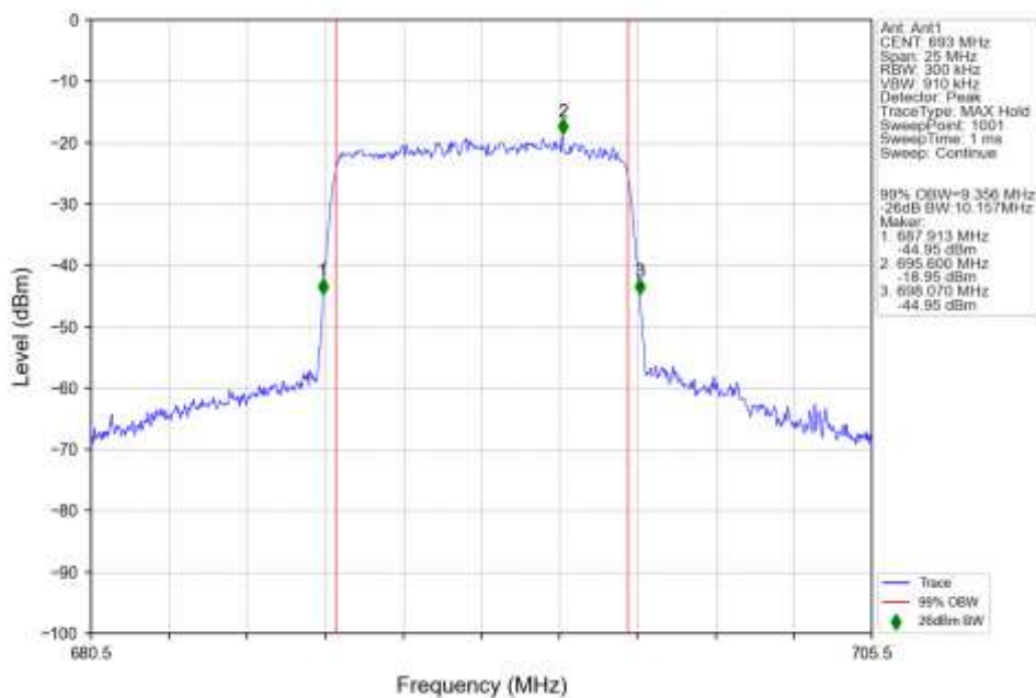
n71_15kHz_SISO_NTNV_10MHz_CP-OFDM_16_QAM_693MHz_Outer_Full_Ant1
