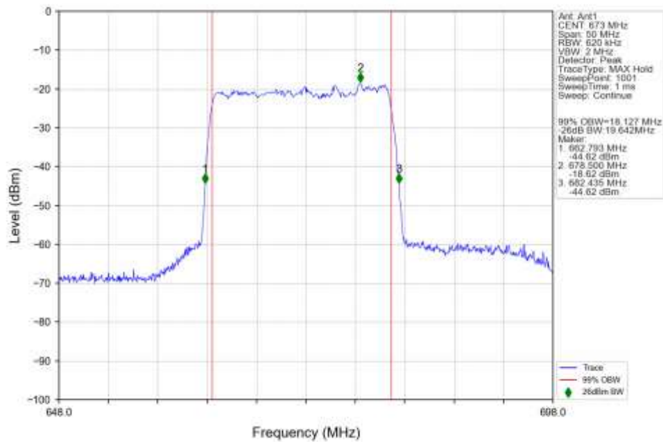
n71_15kHz_SISO_NTNV_20MHz_DFT-s-OFDM_256_QAM_673MHz_Outer_Full_Ant1
