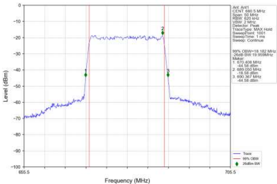
n71_30kHz_SISO_NTNV_20MHz_DFT-s-OFDM_64_QAM_680.5MHz_Outer_Full_Ant1
