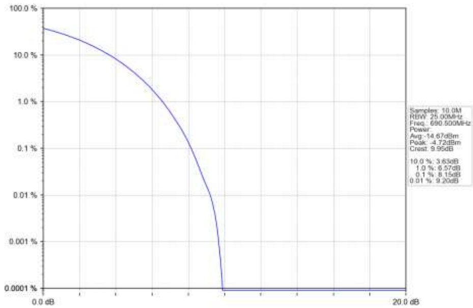
n71_15kHz_SISO_NTNV_15MHz_CP-OFDM_64_QAM_690.5MHz_Outer_Full_Ant1
