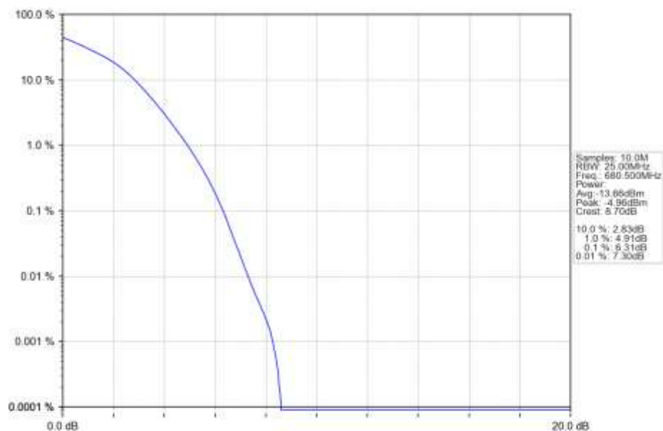
n71_15kHz_SISO_NTNV_20MHz_DFT-s-OFDM_16_QAM_680.5MHz_Outer_Full_Ant1
