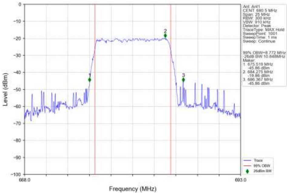
n71_30kHz_SISO_NTNV_10MHz_CP-OFDM_64_QAM_680.5MHz_Outer_Full_Ant1
