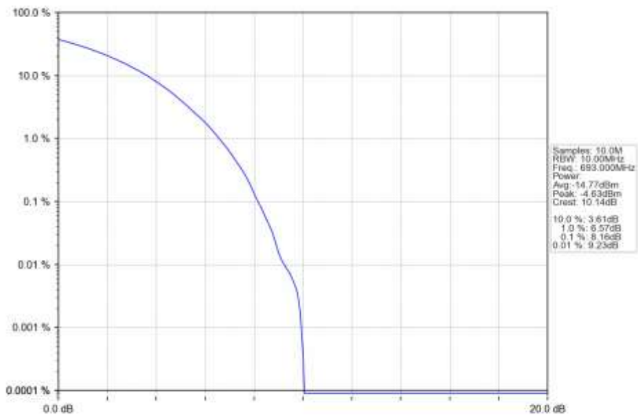
n71_30kHz_SISO_NTNV_10MHz_CP-OFDM_16_QAM_693MHz_Outer_Full_Ant1
