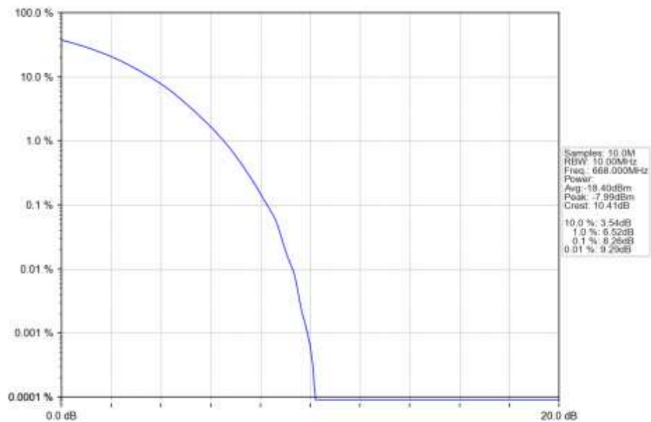
n71_30kHz_SISO_NTNV_10MHz_CP-OFDM 256 QAM 668MHz_Outer_Full_Ant1
