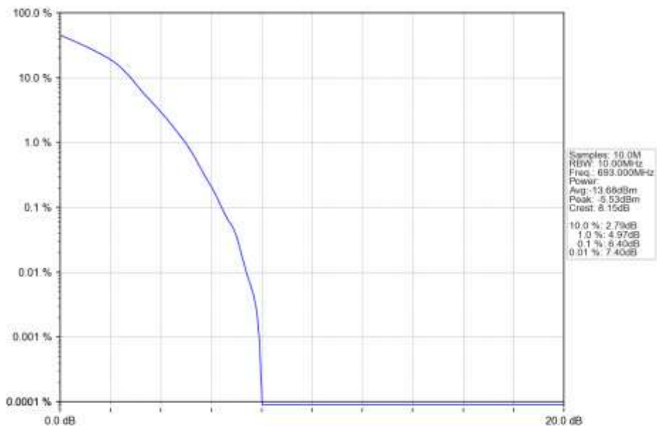
n71_30kHz_SISO_NTNV_10MHz_DFT-s-OFDM_16_QAM_693MHz_Outer_Full_Ant1
