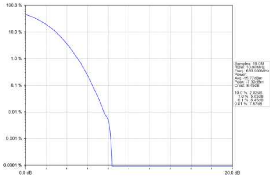
n71_15kHz_SISO_NTNV_10MHz_DFT-s-OFDM_256_QAM_693MHz_Outer_Full_Ant1
