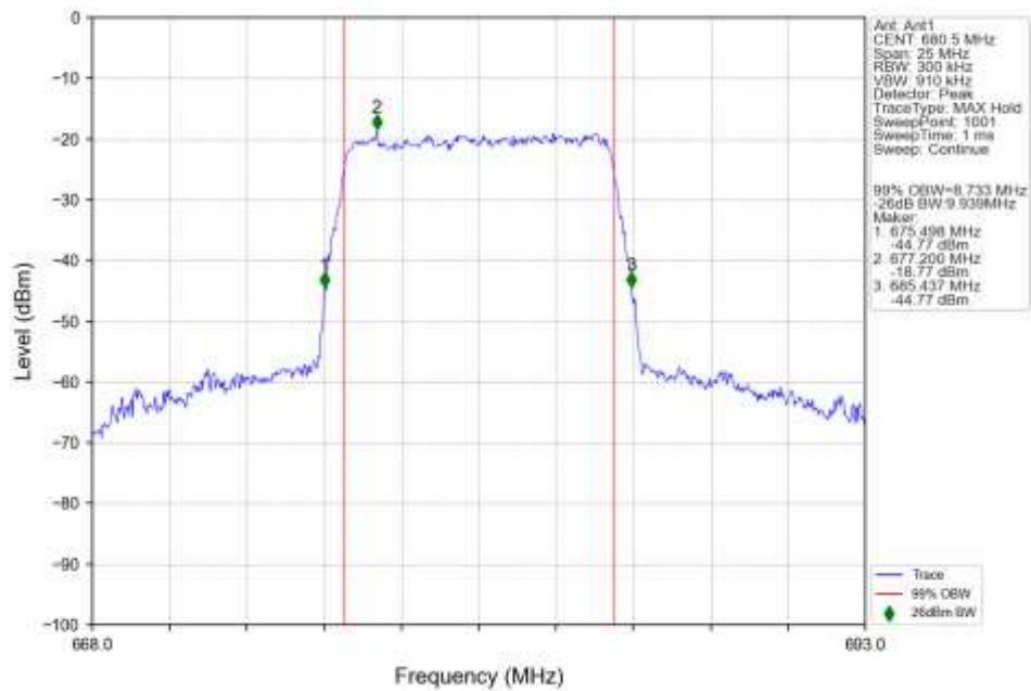
n71_30kHz_SISO_NTNV_10MHz_CP-OFDM_QPSK_680.5MHz_Outer_Full_Ant1
