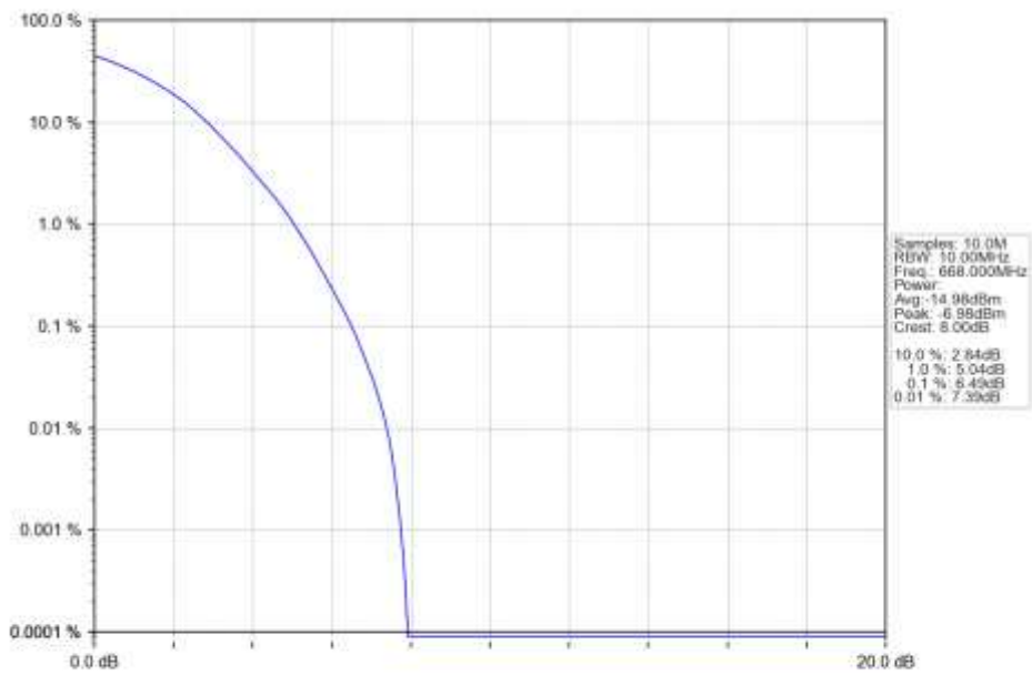
n71_15kHz_SISO_NTNV_10MHz_DFT-s-OFDM_64_QAM_668MHz_Outer_Full_Ant1
