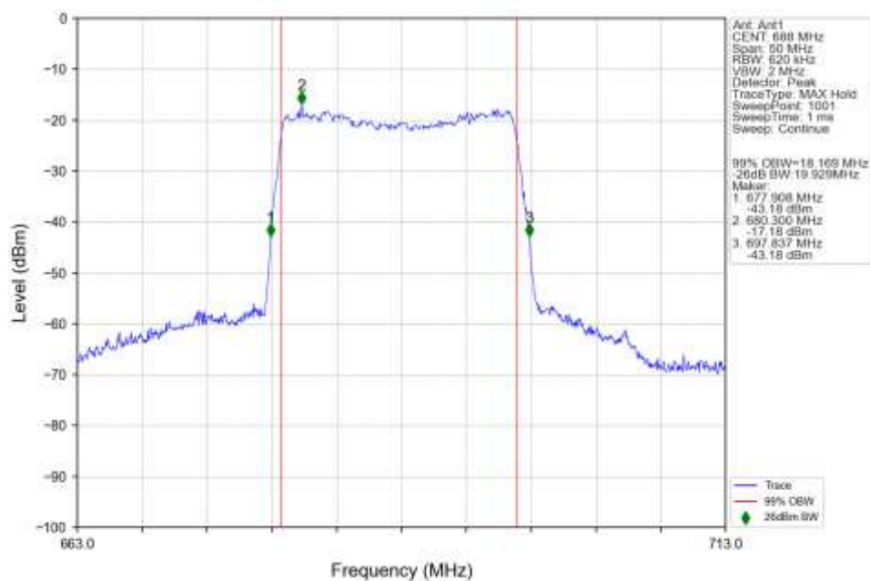
n71_30kHz_SISO_NTNV_20MHz_DFT-s-OFDM_16_QAM_688MHz_Outer_Full_Ant1
