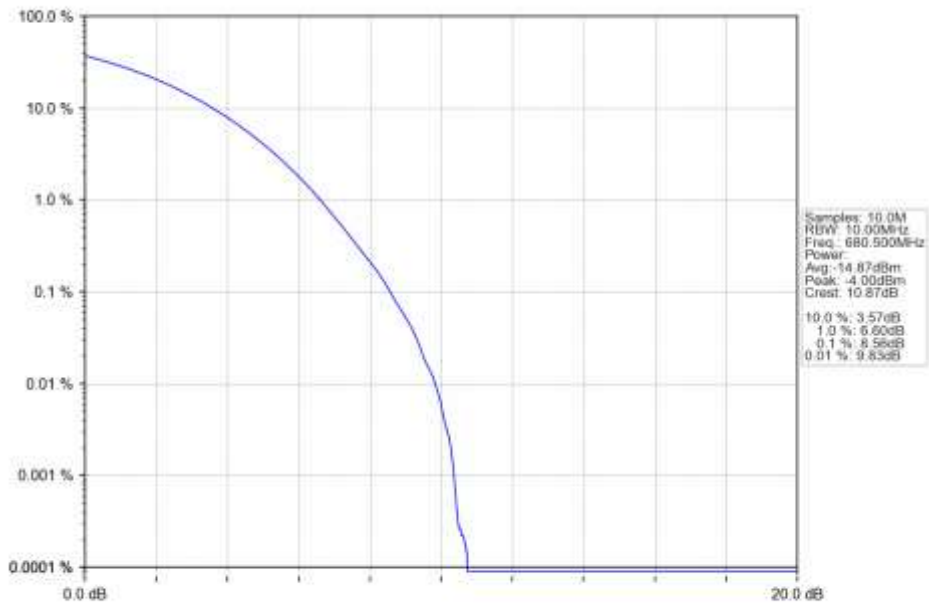
n71_15kHz_SISO_NTNV_10MHz_CP-OFDM_16_QAM_680.5MHz_Outer_Full_Ant1
