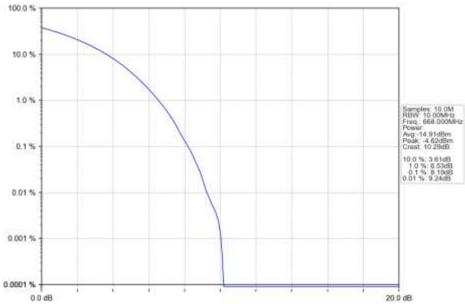
n71_15kHz_SISO_NTNV_10MHz_CP-OFDM_QPSK_668MHz_Outer_Full_Ant1
