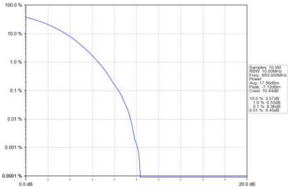
n71_30kHz_SISO_NTNV_10MHz_CP-OFDM_256_QAM_693MHz_Outer_Full_Ant1
