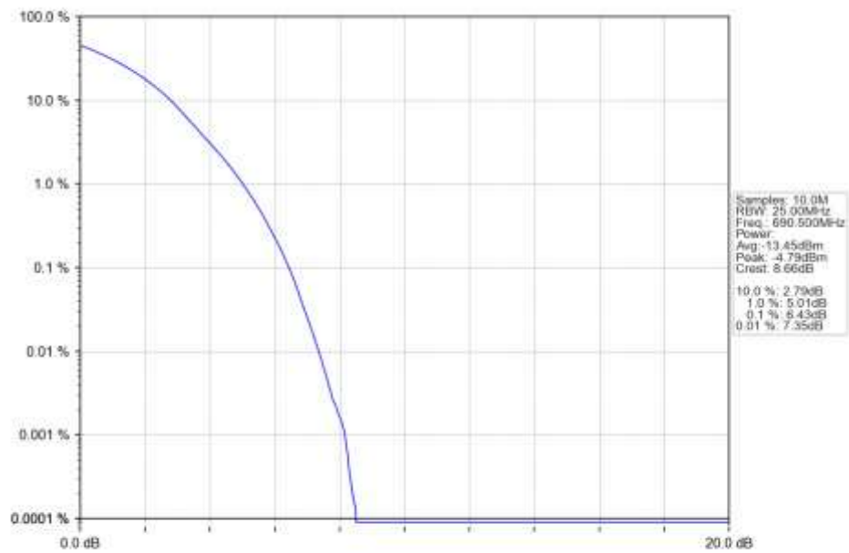
n71_15kHz_SISO_NTNV_15MHz_DFT-s-OFDM_16_QAM_690.5MHz_Outer_Full_Ant1
