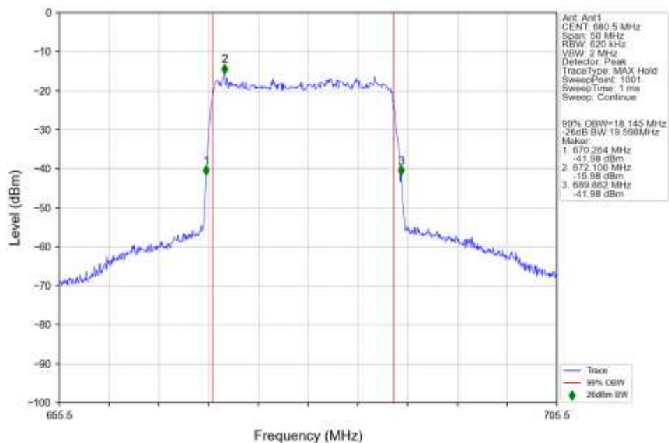
n71_15kHz_SISO_NTNV_20MHz_DFT-s-OFDM QPSK_680.5MHz_Outer_Full_Ant1
