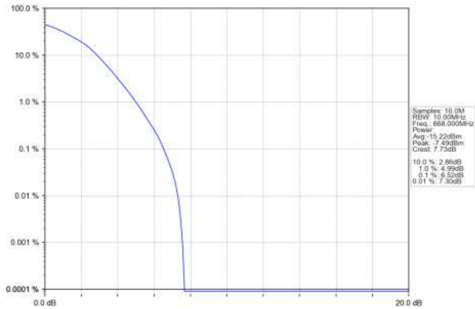
n71_30kHz_SISO_NTNV_10MHz_DFT-s-OFDM_64_QAM_668MHz_Outer_Full_Ant1
