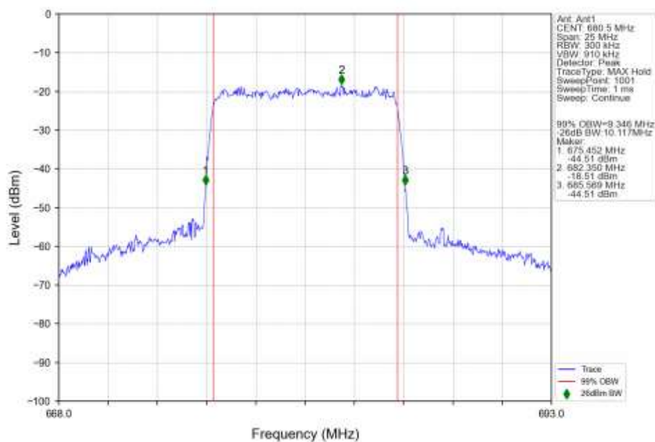
n71_15kHz_SISO_NTNV_10MHz_CP-OFDM_QPSK_680.5MHz_Outer_Full_Ant1
