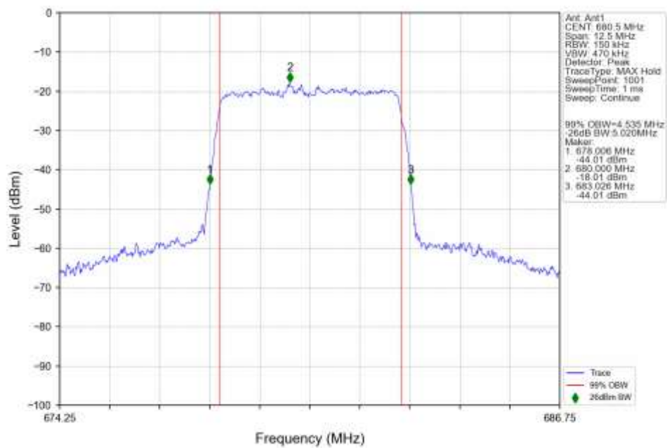
n71_15kHz_SISO_NTNV_5MHz_CP-OFDM_QPSK_680.5MHz_Outer_Full_Ant1
