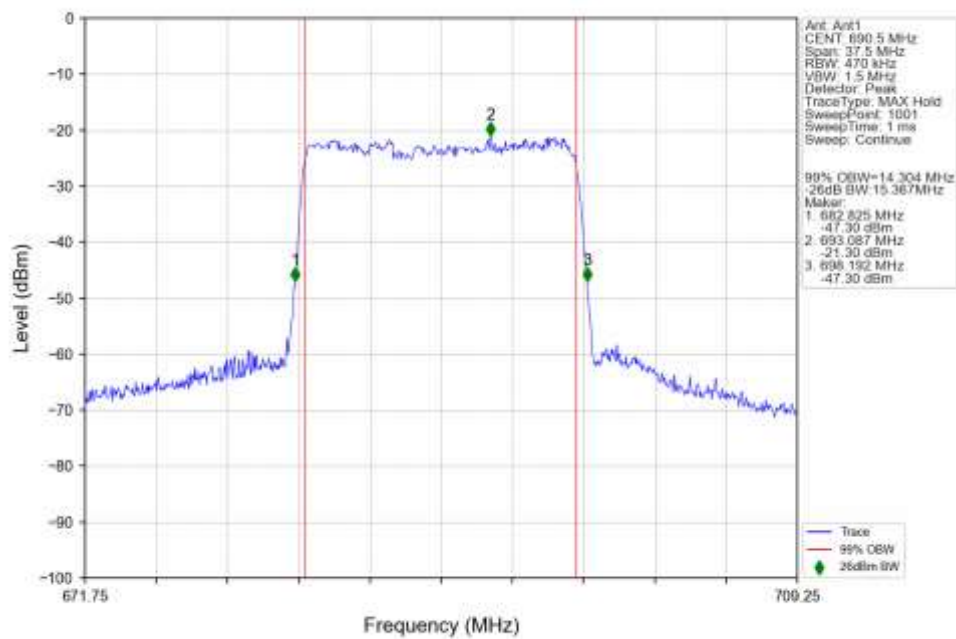
n71_15kHz_SISO_NTNV_15MHz_CP-OFDM_256_QAM_690.5MHz_Outer_Full_Ant1
