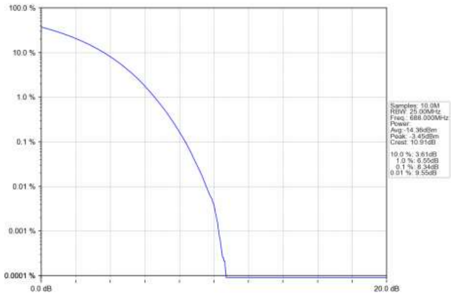
n71_15kHz_SISO_NTNV_20MHz_CP-OFDM_QPSK_688MHz_Outer_Full_Ant1
