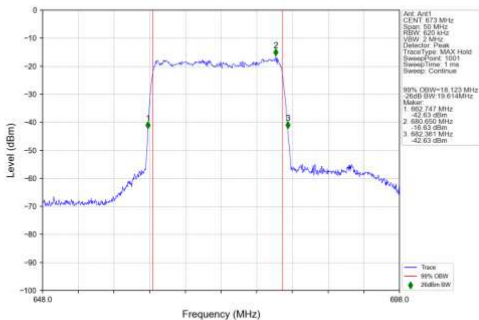
n71_15kHz_SISO_NTNV_20MHz_DFT-s-OFDM_16_QAM_673MHz_Outer_Full_Ant1
