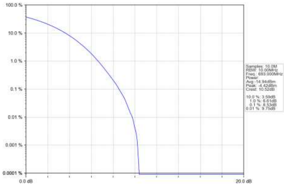
n71_15kHz_SISO_NTNV_10MHz_CP-OFDM_16_QAM_693MHz_Outer_Full_Ant1
