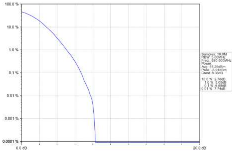
n71_15kHz_SISO_NTNV_5MHz_DFT-s-OFDM_256_QAM_680.5MHz_Outer_Full_Ant1
