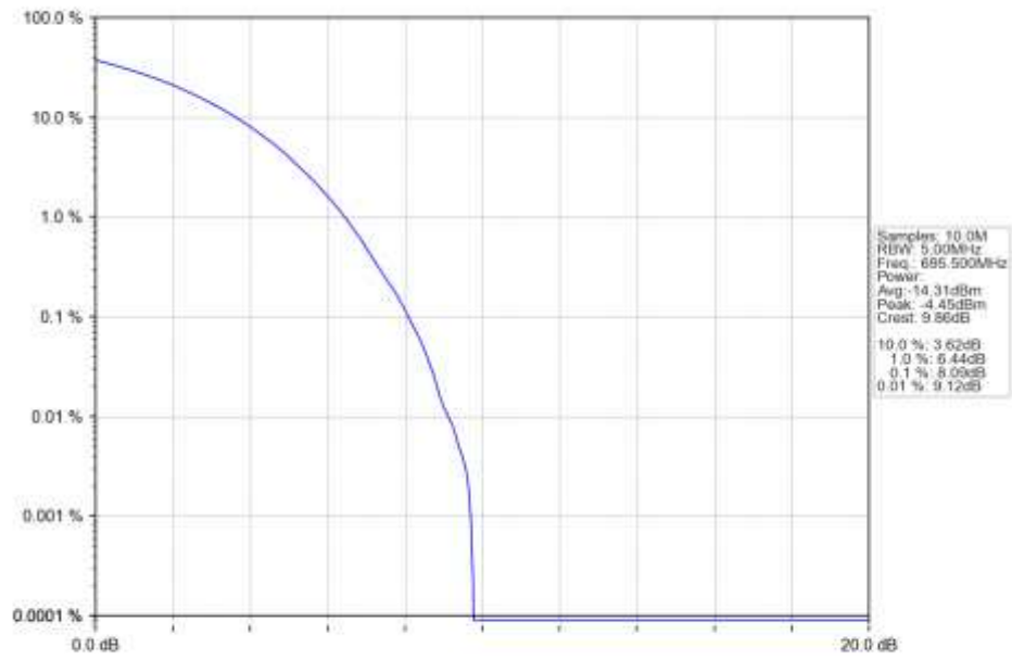
n71_15kHz_SISO_NTNV_5MHz_CP-OFDM_QPSK_695.5MHz_Outer_Full_Ant1
