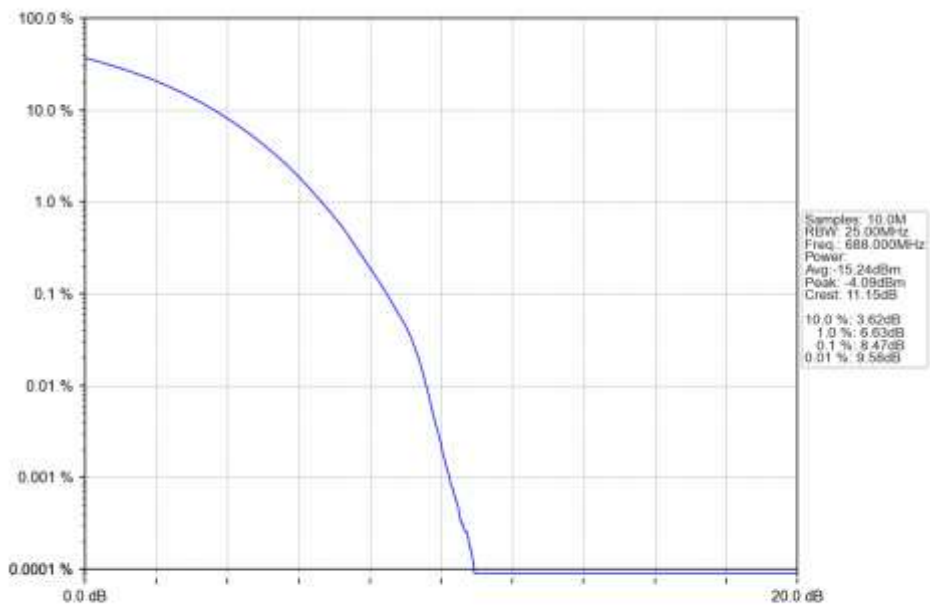
n71_15kHz_SISO_NTNV_20MHz_CP-OFDM_64_QAM_688MHz_Outer_Full_Ant1
