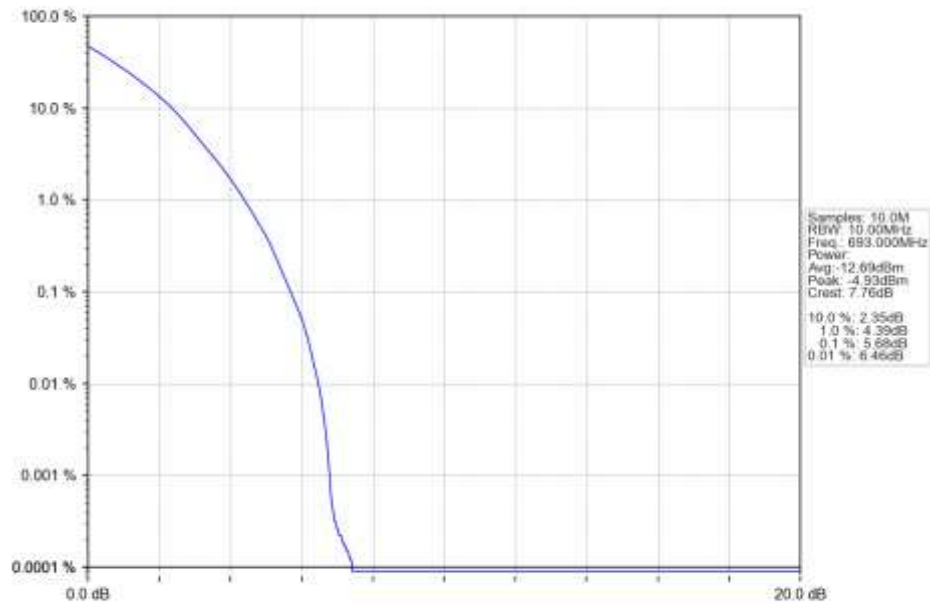
n71_30kHz_SISO_NTNV_10MHz_DFT-s-OFDM_QPSK_693MHz_Outer_Full_Ant1
