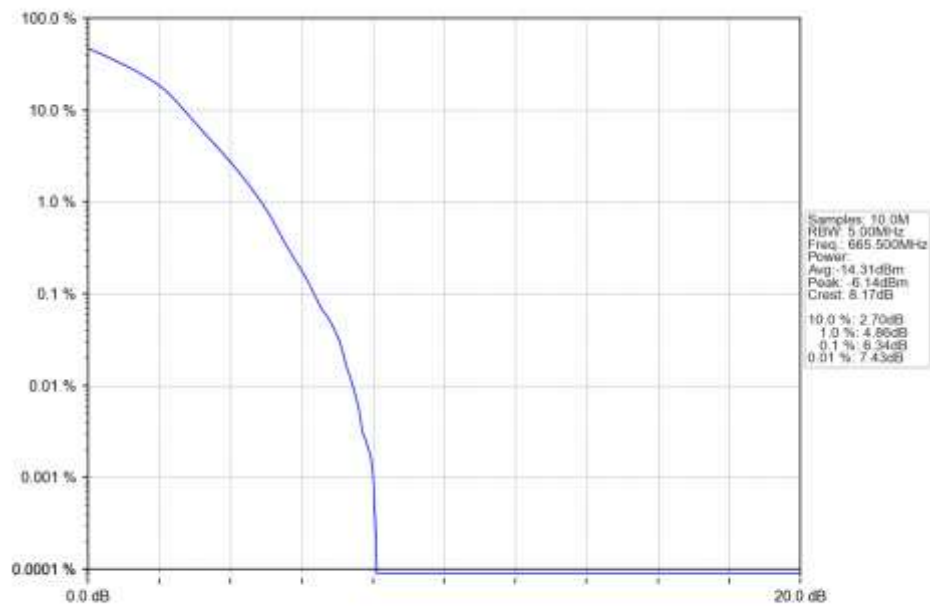
n71_15kHz_SISO_NTNV_5MHz_DFT-s-OFDM_16QAM_665.5MHz_Outer_Full_Ant1
