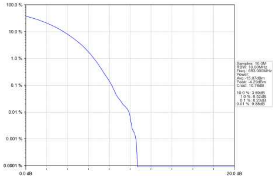
n71_30kHz_SISO_NTNV_10MHz_CP-OFDM 64 QAM 693MHz_Outer_Full_Ant1
