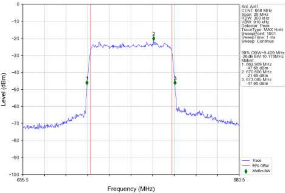
n71_15kHz_SISO_NTNV_10MHz_CP-OFDM_256_QAM_668MHz_Outer_Full_Ant1
