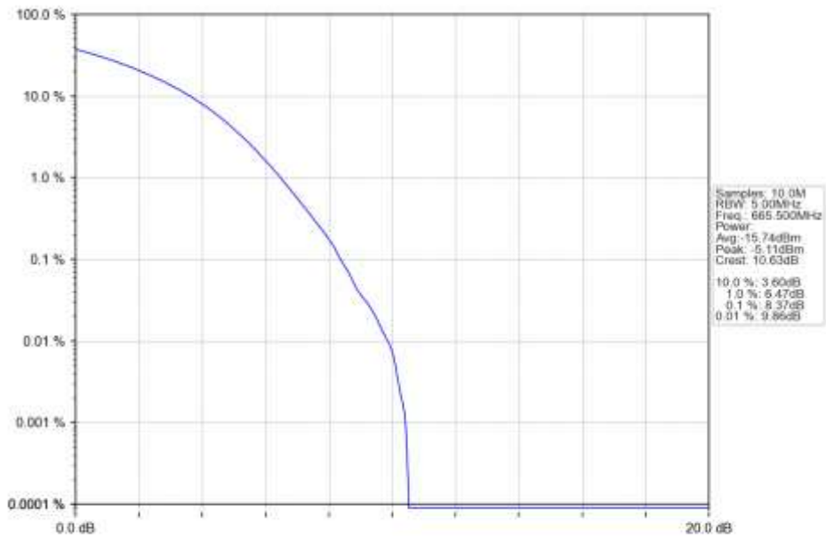
n71_15kHz_SISO_NTNV_5MHz_CP-OFDM_64_QAM_665.5MHz_Outer_Full_Ant1
