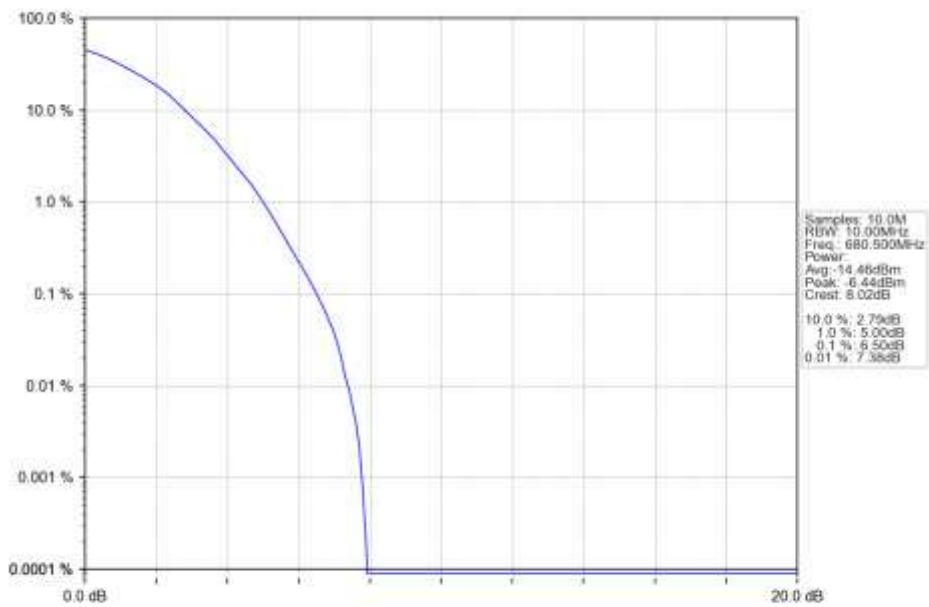
n71_15kHz_SISO_NTNV_10MHz_DFT-s-OFDM_64_QAM_680.5MHz_Outer_Full_Ant1
