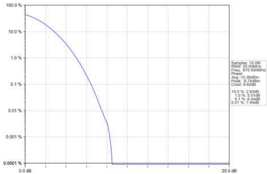
n71_15kHz_SISO_NTNV_15MHz_DFT-s-OFDM_256_QAM_670.5MHz_Outer_Full_Ant1
