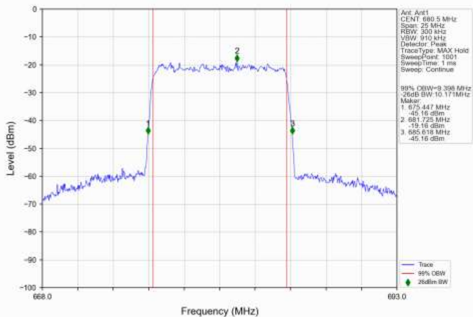
n71_15kHz_SISO_NTNV_10MHz_CP-OFDM_64_QAM_680.5MHz_Outer_Full_Ant1
