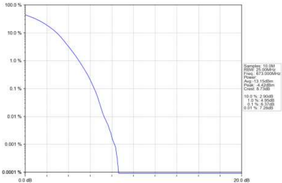
n71_15kHz_SISO_NTNV_20MHz_DFT-s-OFDM_16_QAM_673MHz_Outer_Full_Ant1
