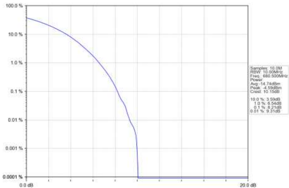
n71_30kHz_SISO_NTNV_10MHz_CP-OFDM_16_QAM_680.5MHz_Outer_Full_Ant1
