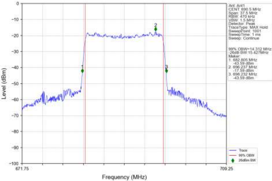
n71_15kHz_SISO_NTNV_15MHz_CP-OFDM_16_QAM_690.5MHz_Outer_Full_Ant1
