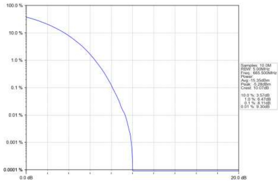
n71_15kHz_SISO_NTNV_5MHz_CP-OFDM_16_QAM_665.5MHz_Outer_Full_Ant1
