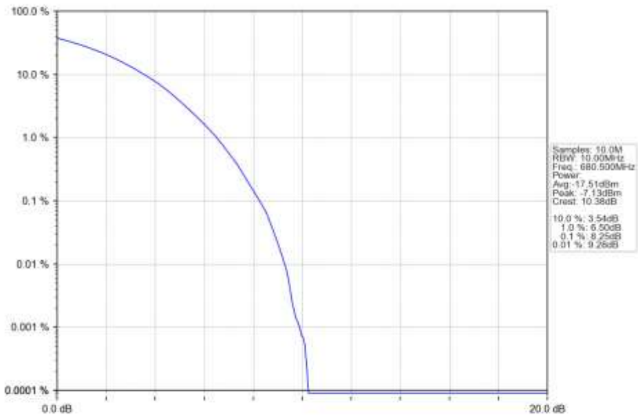
n71_30kHz_SISO_NTNV_10MHz_CP-OFDM_256_QAM_680.5MHz_Outer_Full_Ant1
