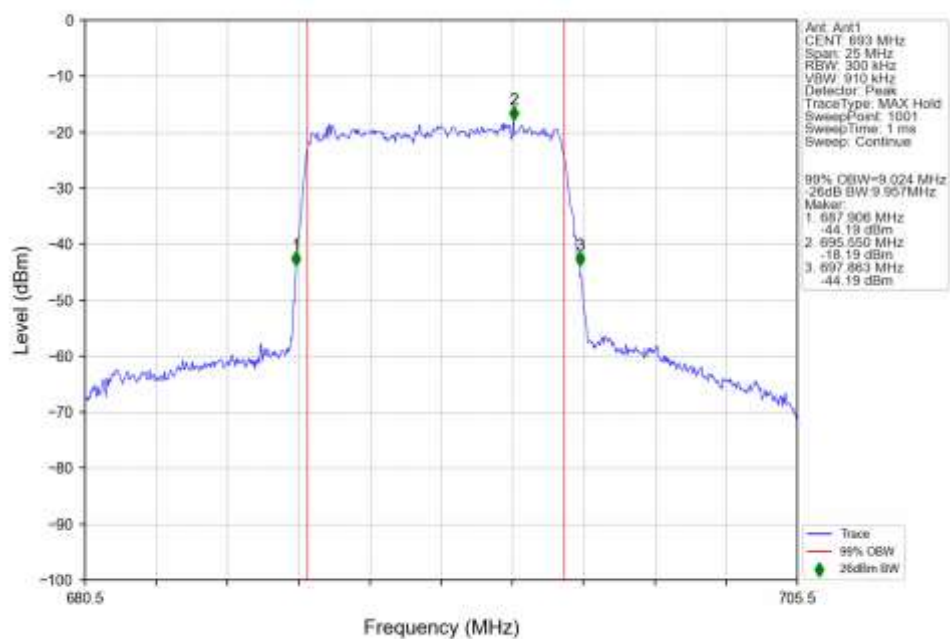
n71_15kHz_SISO_NTNV_10MHz_DFT-s-OFDM_16_QAM_693MHz_Outer_Full_Ant1
