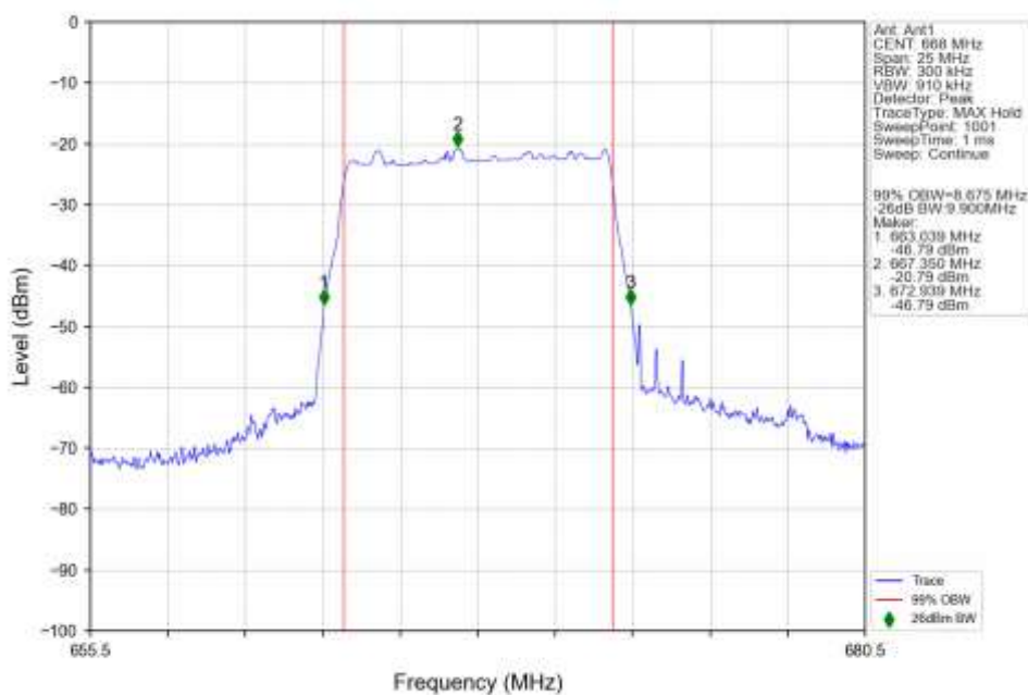
n71_30kHz_SISO_NTNV_10MHz_DFT-s-OFDM_256_QAM_668MHz_Outer_Full_Ant1
