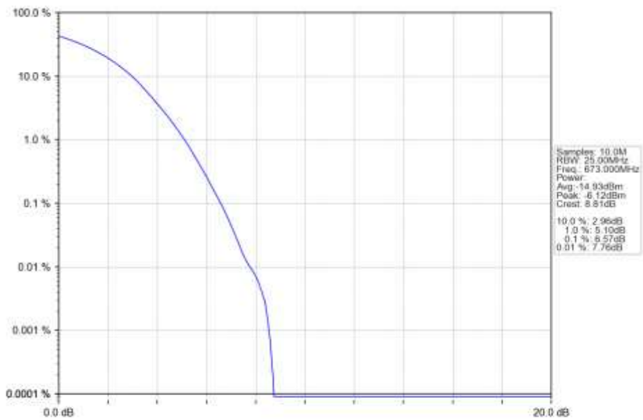
n71_15kHz_SISO_NTNV_20MHz_DFT-s-OFDM_256_QAM_673MHz_Outer_Full_Ant1
