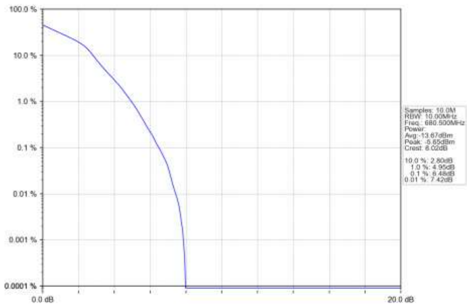
n71_30kHz_SISO_NTNV_10MHz_DFT-s-OFDM_16_QAM_680.5MHz_Outer_Full_Ant1
