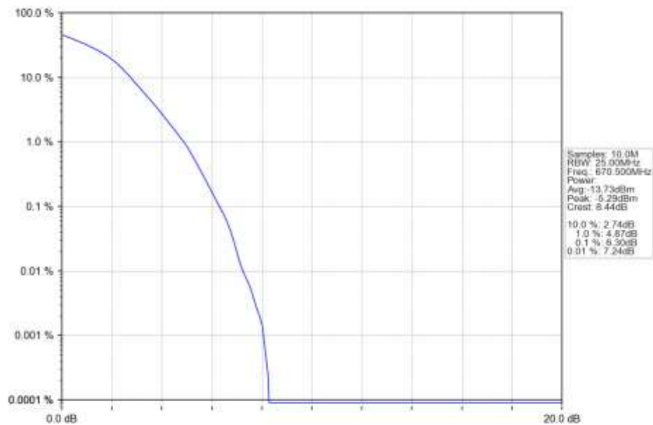
n71_30kHz_SISO_NTNV_15MHz_DFT-s-OFDM_16_QAM_670.5MHz_Outer_Full_Ant1
