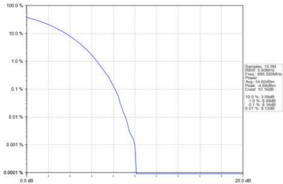
n71_15kHz_SISO_NTNV_5MHz_CP-OFDM_16_QAM_695.5MHz_Outer_Full_Ant1
