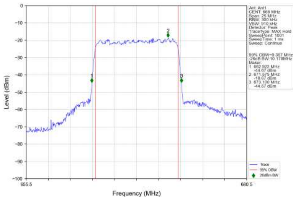
n71_15kHz_SISO_NTNV_10MHz_CP-OFDM_QPSK_680.5MHz_Outer_Full_Ant1
