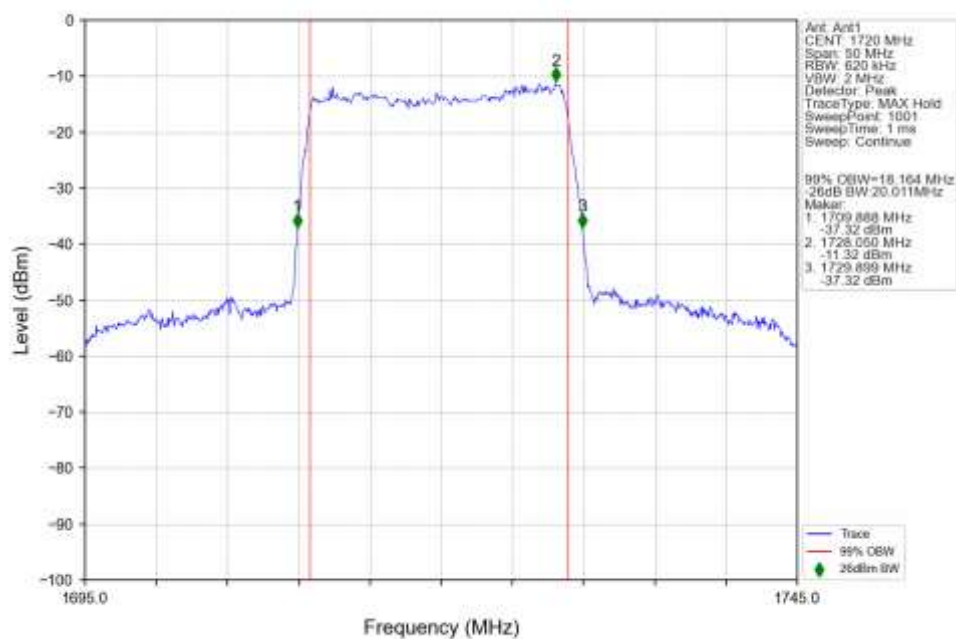
n66_30kHz_SISO_NTNV_20MHz_DFT-s-OFDM_16_QAM_1720MHz_Outer_Full_Ant1
