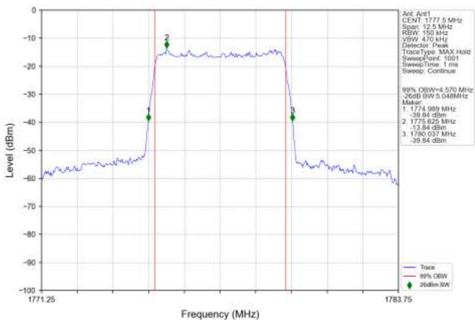
n66_15kHz_SISO_NTNV_5MHz_DFT-s-OFDM_16_QAM_1777.5MHz_Outer_Full_Ant1
