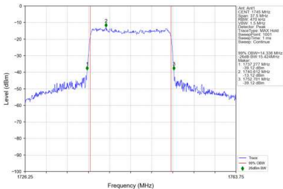
n66_15kHz_SISO_NTNV_15MHz_CP-OFDM_64_QAM_1745MHz_Outer_Full_Ant1
