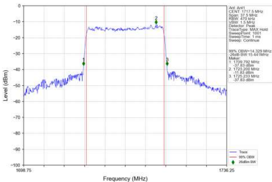
n66_15kHz_SISO_NTNV_15MHz_CP-OFDM_16_QAM_1717.5MHz_Outer_Full_Ant1
