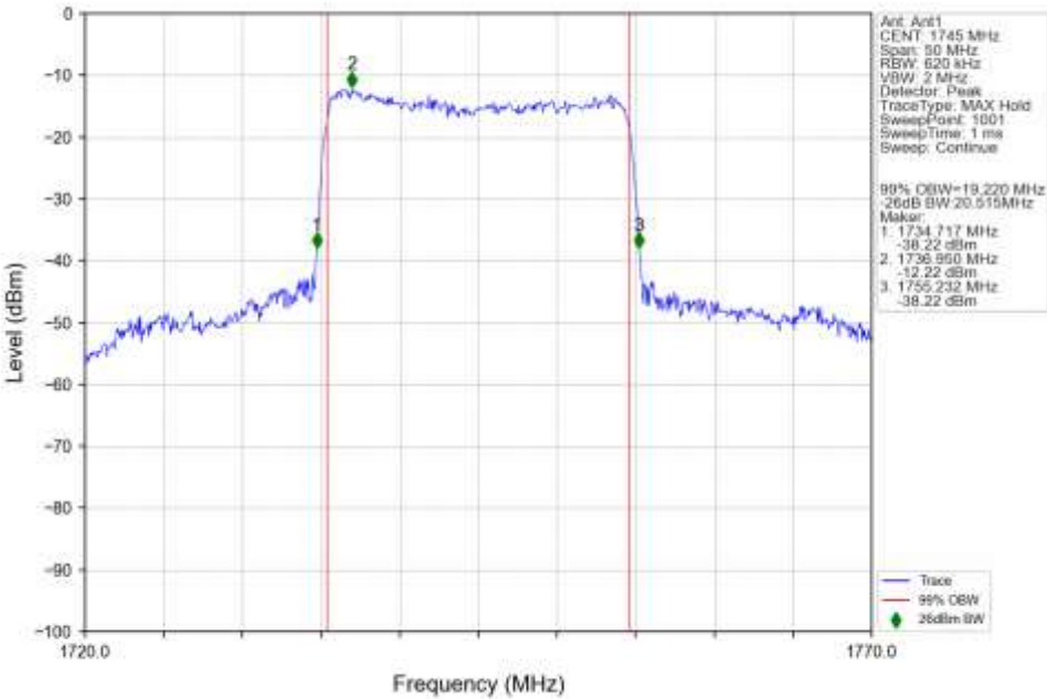
n66_15kHz_SISO_NTNV_20MHz_CP-OFDM_64_QAM_1745MHz_Outer_Full_Ant1
