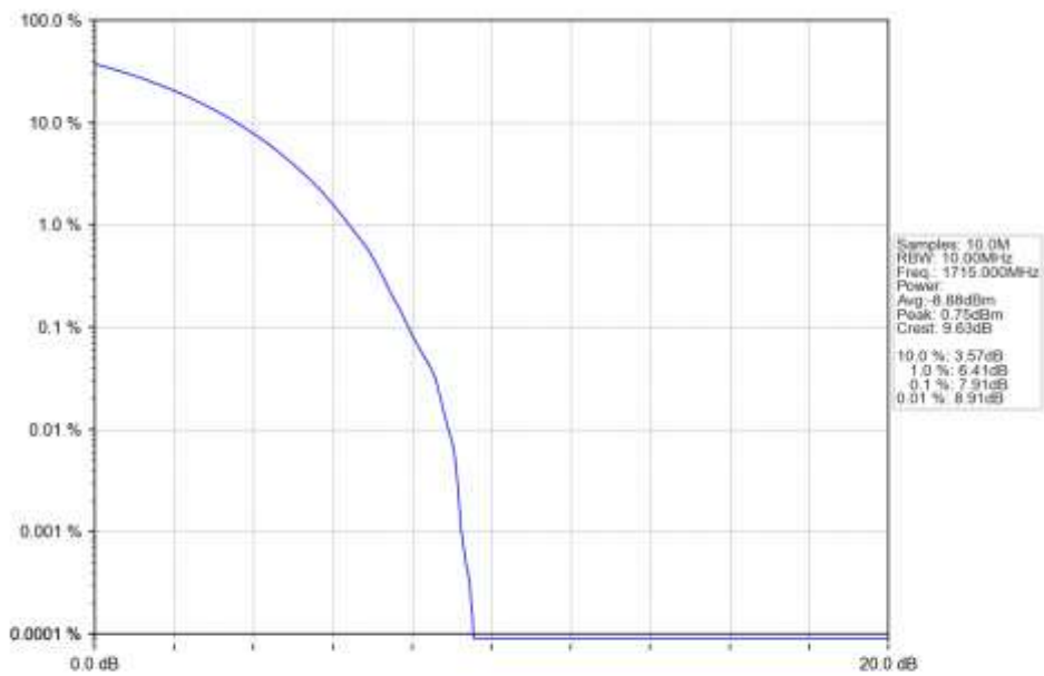
n66_15kHz_SISO_NTNV_10MHz_CP-OFDM_256_QAM_1715MHz_Outer_Full_Ant1
