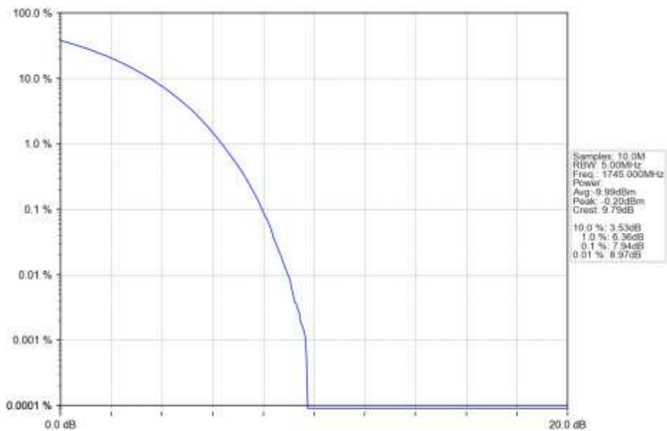
n66_15kHz_SISO_NTNV_5MHz_CP-OFDM_16_QAM_1745MHz_Outer_Full_Ant1
