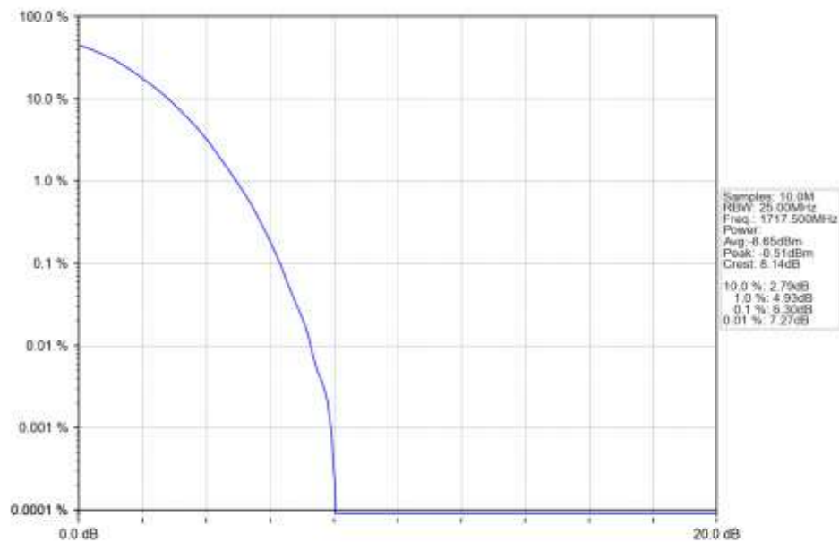
n66_15kHz_SISO_NTNV_15MHz_DFT-s-OFDM_256_QAM_1717.5MHz_Outer_Full_Ant1
