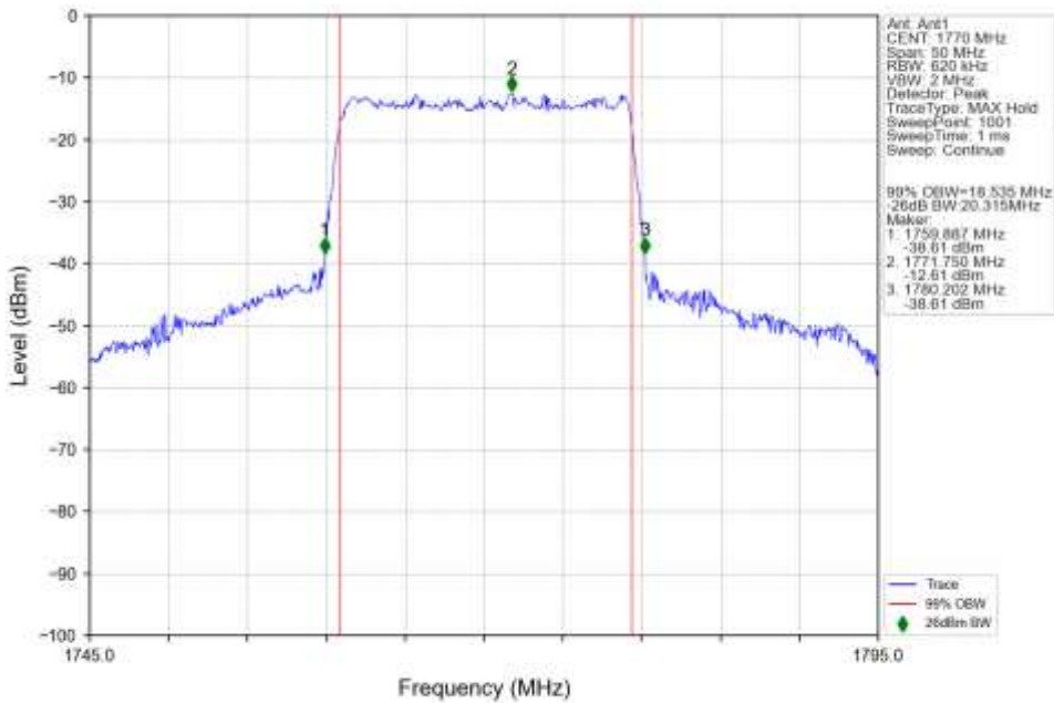
n66_30kHz_SISO_NTNV_20MHz_CP-OFDM_16_QAM_1770MHz_Outer_Full_Ant1
