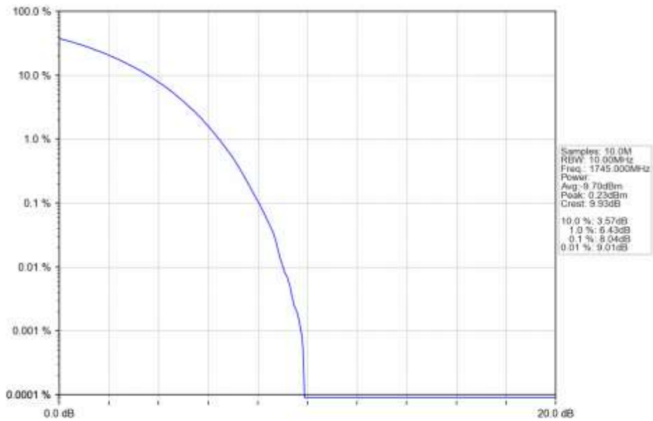
n66_15kHz_SISO_NTNV_10MHz_CP-OFDM_QPSK_1745MHz_Outer_Full_Ant1
