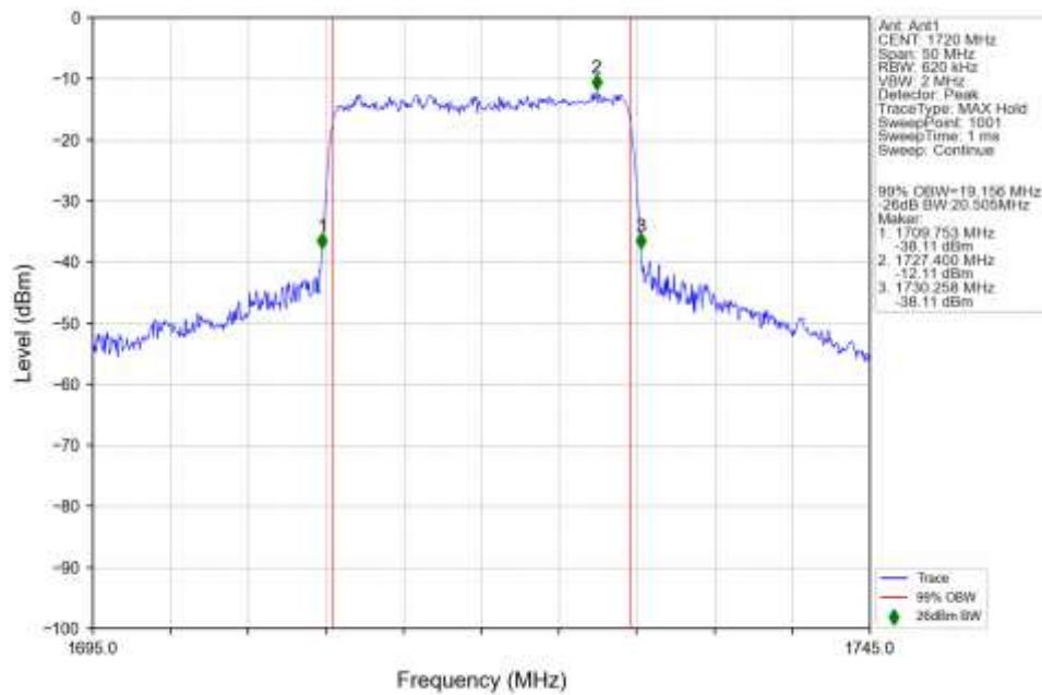
n66_15kHz_SISO_NTNV_20MHz_CP-OFDM_16_QAM_1720MHz_Outer_Full_Ant1
