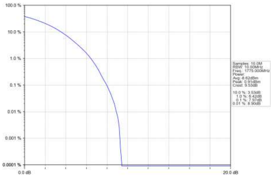
n66_15kHz_SISO_NTNV_10MHz_CP-OFDM_64_QAM_1775MHz_Outer_Full_Ant1
