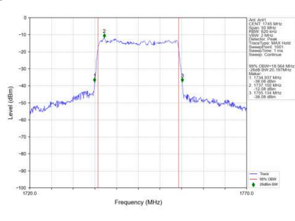
n66_30kHz_SISO_NTNV_20MHz_CP-OFDM_64_QAM_1745MHz_Outer_Full_Ant1
