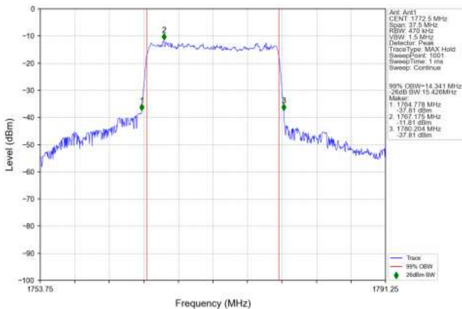
n66_15kHz_SISO_NTNV_15MHz_CP-OFDM_16_QAM_1772.5MHz_Outer_Full_Ant1
