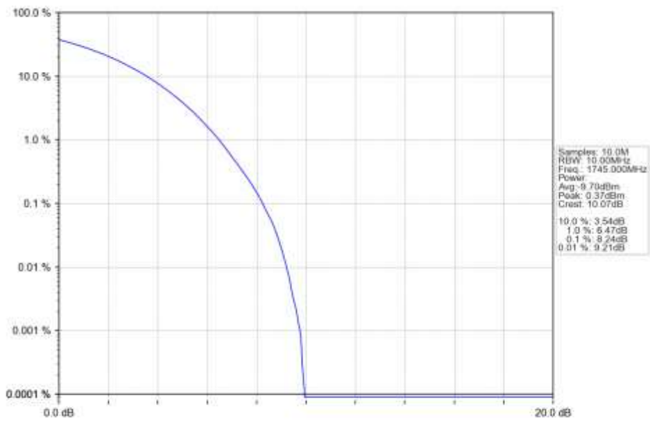
n66_15kHz_SISO_NTNV_10MHz_CP-OFDM_16_QAM_1745MHz_Outer_Full_Ant1
