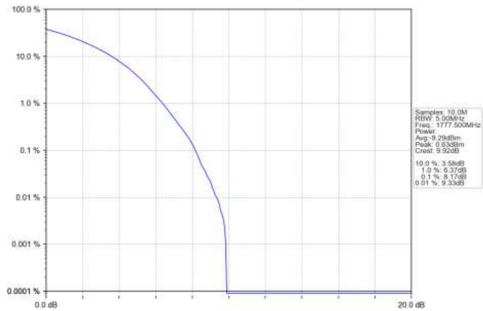
n66_15kHz_SISO_NTNV_5MHz_CP-OFDM_64_QAM_1777.5MHz_Outer_Full_Ant1
