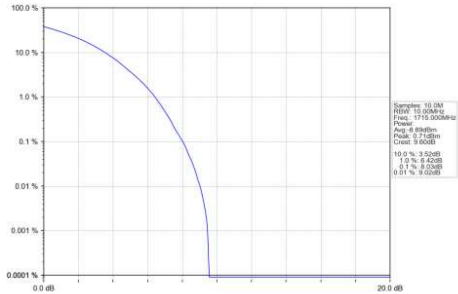
n66_15kHz_SISO_NTNV_10MHz_CP-OFDM_64_QAM_1715MHz_Outer_Full_Ant1
