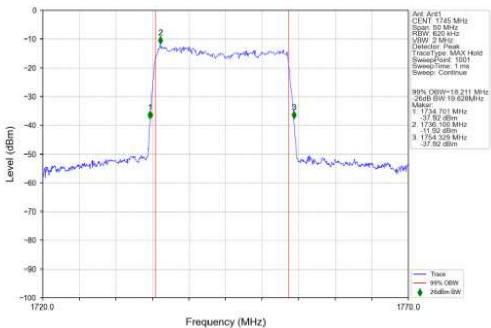
n66_15kHz_SISO_NTNV_20MHz_DFT-s-OFDM_64_QAM_1745MHz_Outer_Full_Ant1
