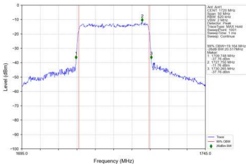
n66_15kHz_SISO_NTNV_20MHz_CP-OFDM_256_QAM_1720MHz_Outer_Full_Ant1
