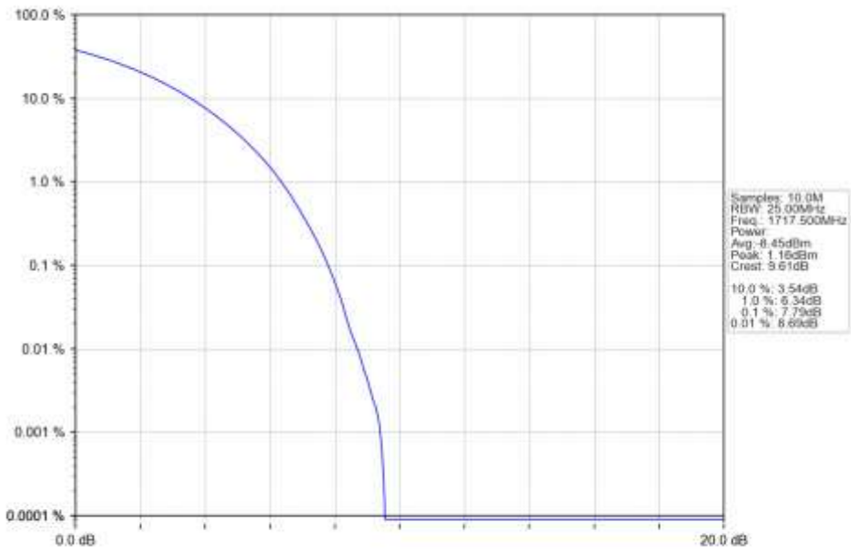
n66_15kHz_SISO_NTNV_15MHz_CP-OFDM_QPSK_1717.5MHz_Outer_Full_Ant1
