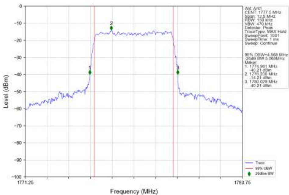
n66_15kHz_SISO_NTNV_5MHz_CP-OFDM_256_QAM_1777.5MHz_Outer_Full_Ant1
