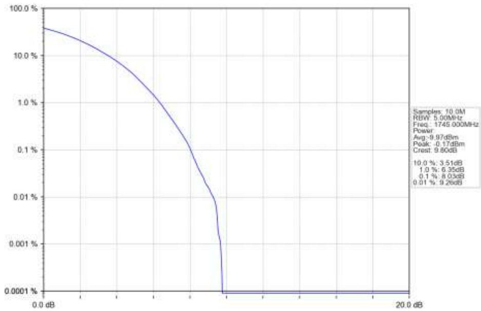
n66_15kHz_SISO_NTNV_5MHz_CP-OFDM_256_QAM_1745MHz_Outer_Full_Ant1
