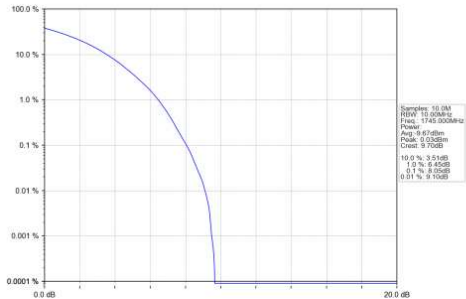
n66_15kHz_SISO_NTNV_10MHz_CP-OFDM_64_QAM_1745MHz_Outer_Full_Ant1
