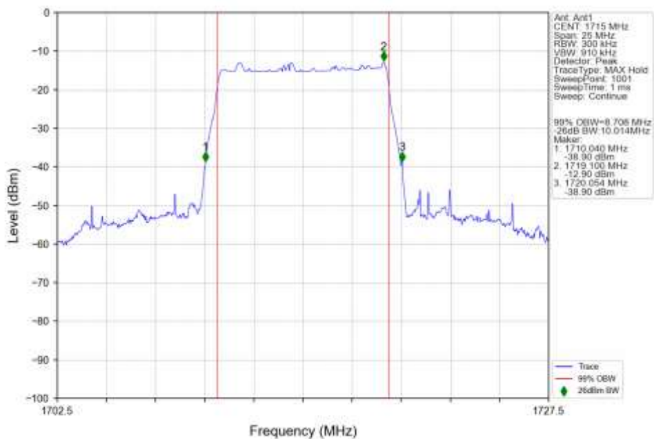
n66_30kHz_SISO_NTNV_10MHz_DFT-s-OFDM_256_QAM_1715MHz_Outer_Full_Ant1
