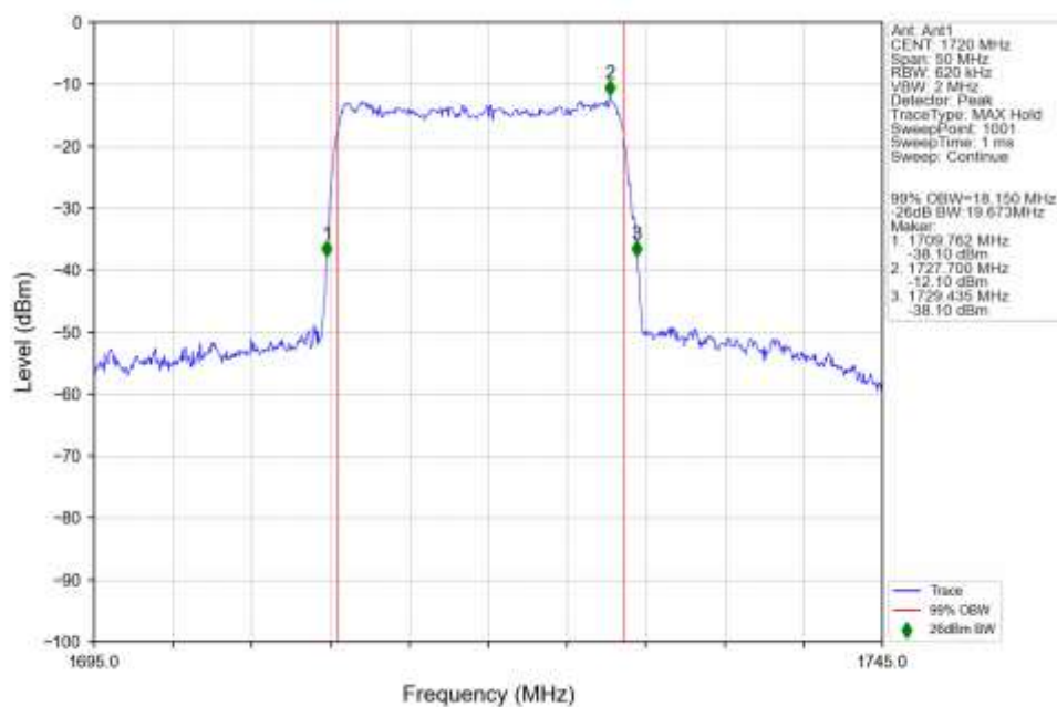
n66_15kHz_SISO_NTNV_20MHz_DFT-s-OFDM_16_QAM_1720MHz_Outer_Full_Ant1
