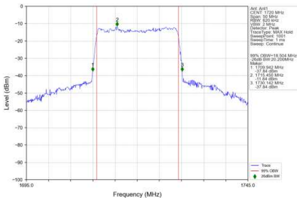
n66_30kHz_SISO_NTNV_20MHz_CP-OFDM_256_QAM_1720MHz_Outer_Full_Ant1
