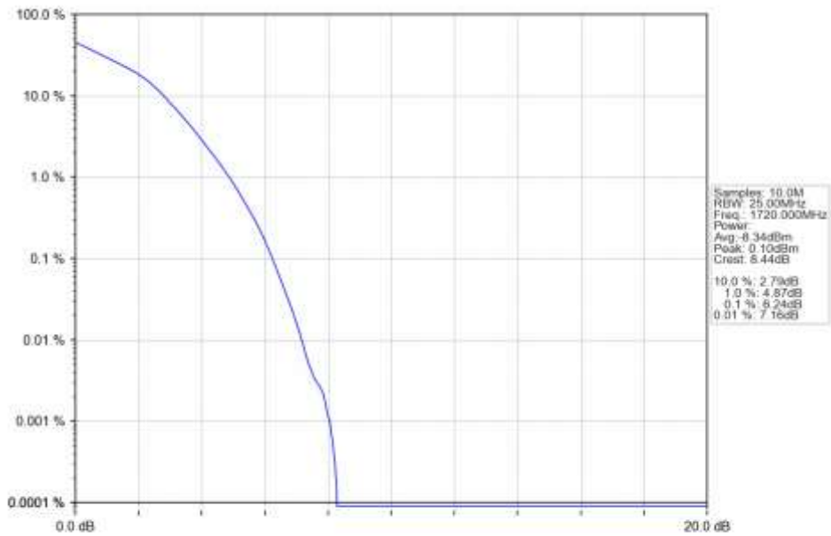
n66_15kHz_SISO_NTNV_20MHz_DFT-s-OFDM_16_QAM_1720MHz_Outer_Full_Ant1
