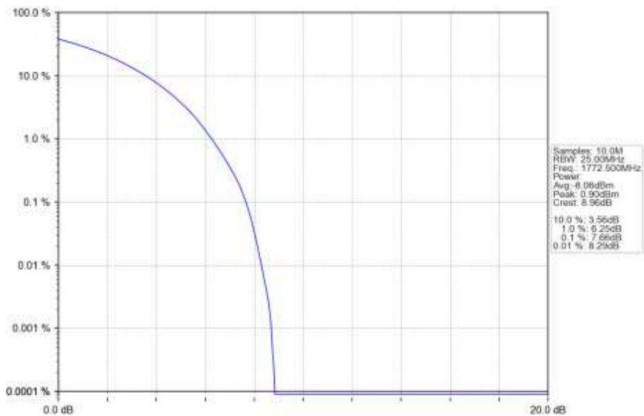
n66_15kHz_SISO_NTNV_15MHz_CP-OFDM_16_QAM_1772.5MHz_Outer_Full_Ant1
