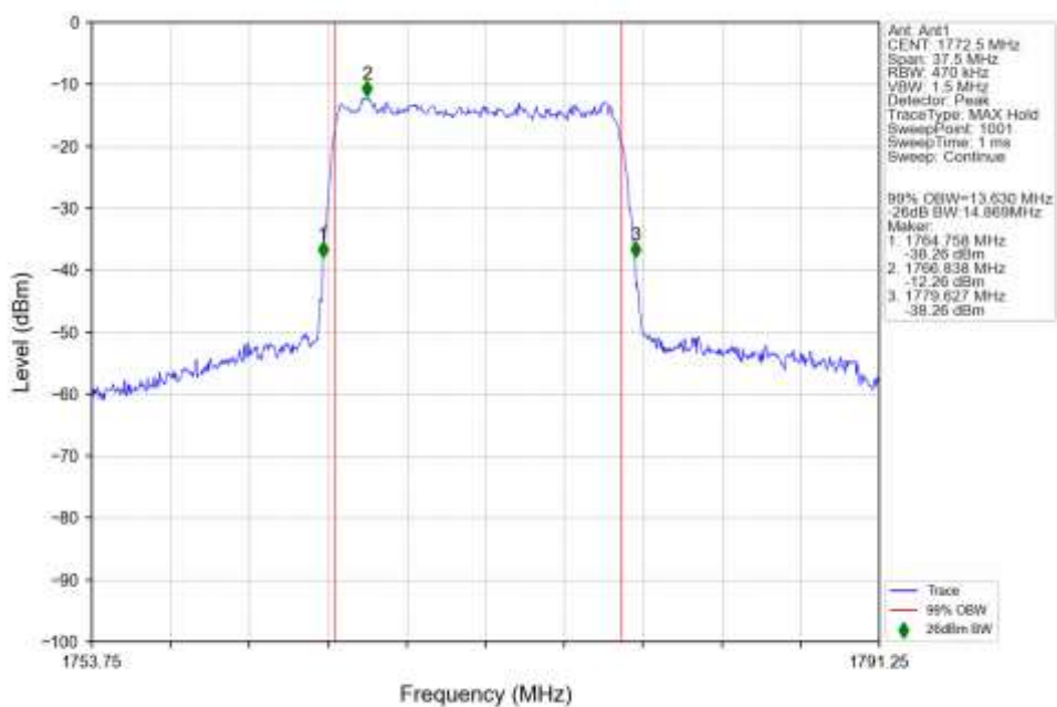
n66_15kHz_SISO_NTNV_15MHz_DFT-s-OFDM_16_QAM_1772.5MHz_Outer_Full_Ant1
