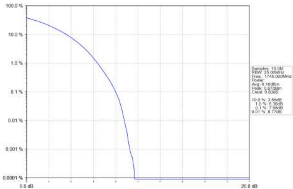
n66_15kHz_SISO_NTNV_15MHz_CP-OFDM_16_QAM_1745MHz_Outer_Full_Ant1
