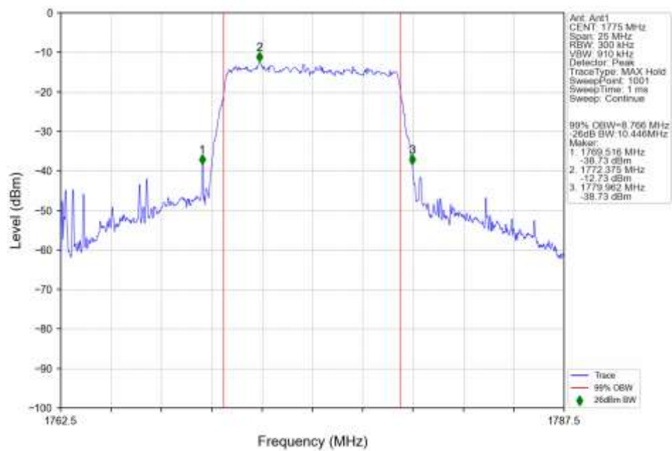
n66_30kHz_SISO_NTNV_10MHz_CP-OFDM_16_QAM_1775MHz_Outer_Full_Ant1
