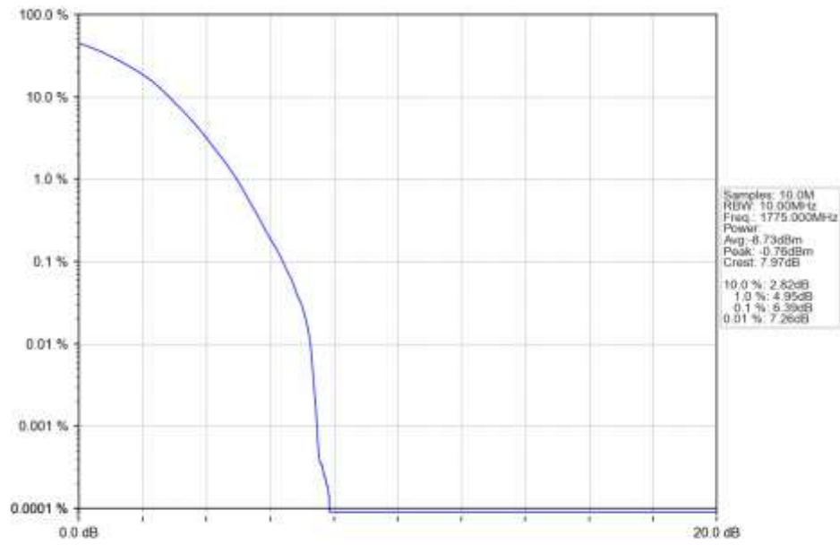
n66_15kHz_SISO_NTNV_10MHz_DFT-s-OFDM_64_QAM_1775MHz_Outer_Full_Ant1
