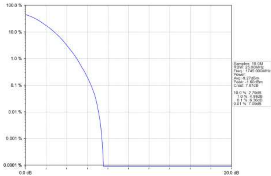
n66_15kHz_SISO_NTNV_15MHz_DFT-s-OFDM_64_QAM_1745MHz_Outer_Full_Ant1
