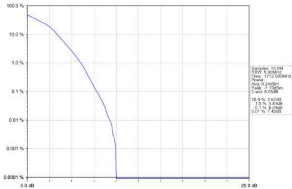
n66_15kHz_SISO_NTNV_5MHz_DFT-s-OFDM 16 QAM 1712.5MHz_Outer_Full_Ant1
