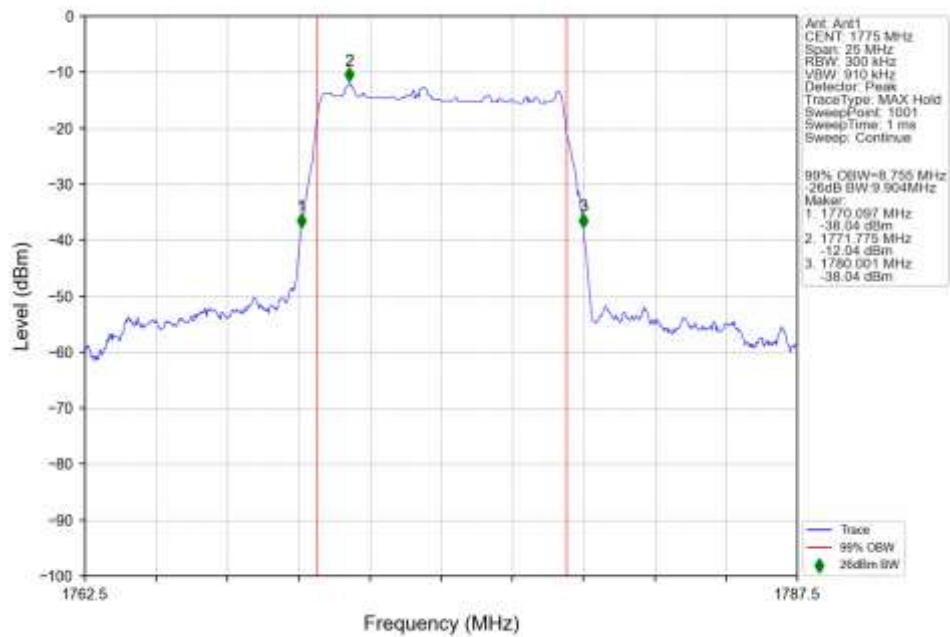
n66_30kHz_SISO_NTNV_10MHz_DFT-s-OFDM_256_QAM_1775MHz_Outer_Full_Ant1
