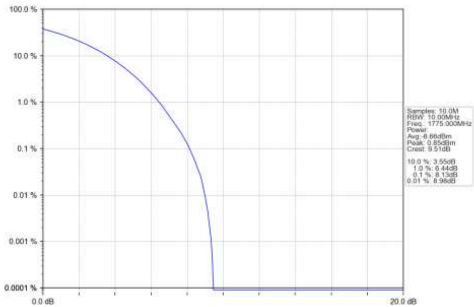
n66_15kHz_SISO_NTNV_10MHz_CP-OFDM_16_QAM_1775MHz_Outer_Full_Ant1
