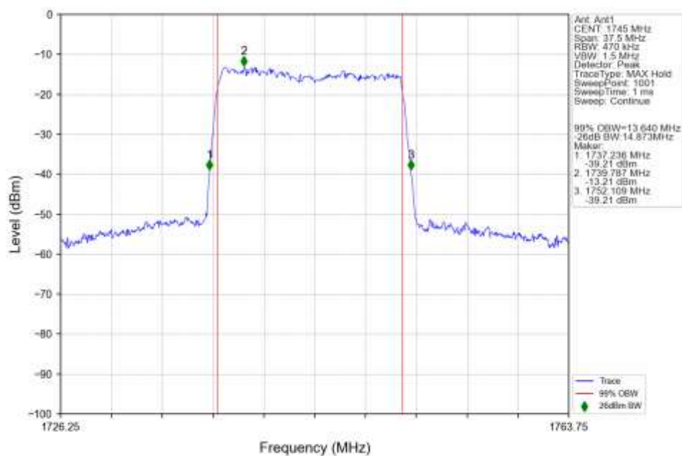
n66_15kHz_SISO_NTNV_15MHz_DFT-s-OFDM_64_QAM_1745MHz_Outer_Full_Ant1
