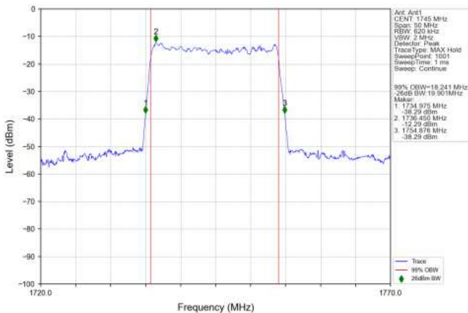
n66_30kHz_SISO_NTNV_20MHz_DFT-s-OFDM_64_QAM_1745MHz_Outer_Full_Ant1
