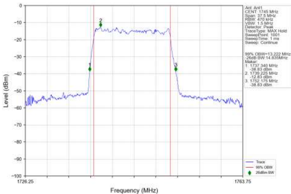
n66_30kHz_SISO_NTNV_15MHz_DFT-s-OFDM_64_QAM_1745MHz_Outer_Full_Ant1
