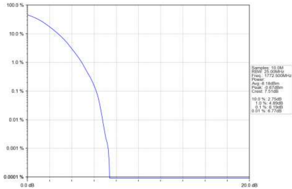
n66_15kHz_SISO_NTNV_15MHz_DFT-s-OFDM_64_QAM_1772.5MHz_Outer_Full_Ant1
