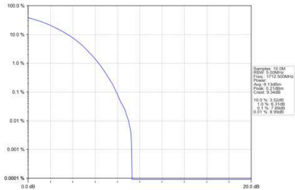
n66_15kHz_SISO_NTNV_5MHz_CP-OFDM_256_QAM_1712.5MHz_Outer_Full_Ant1
