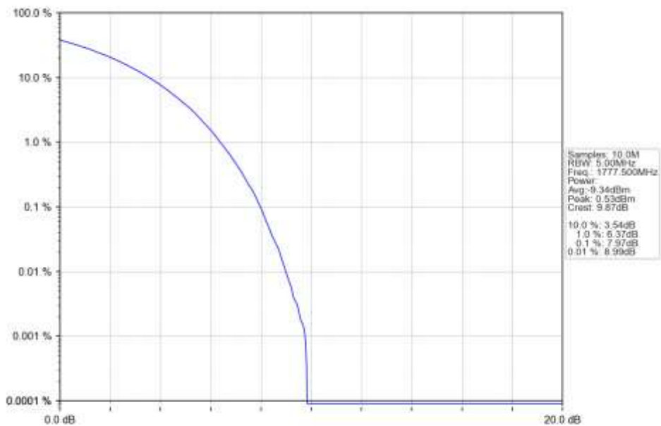
n66_15kHz_SISO_NTNV_5MHz_CP-OFDM_16_QAM_1777.5MHz_Outer_Full_Ant1
