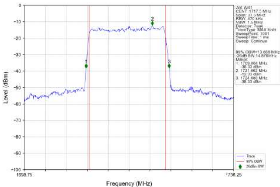
n66_15kHz_SISO_NTNV_15MHz_DFT-s-OFDM_256_QAM_1717.5MHz_Outer_Full_Ant1
