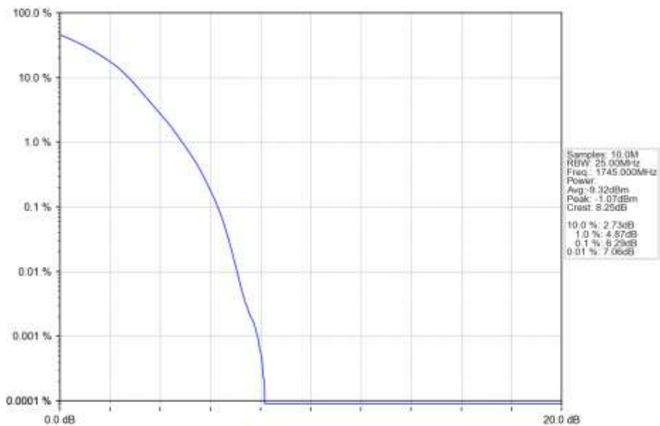
n66_15kHz_SISO_NTNV_15MHz_DFT-s-OFDM_16_QAM_1745MHz_Outer_Full_Ant1
