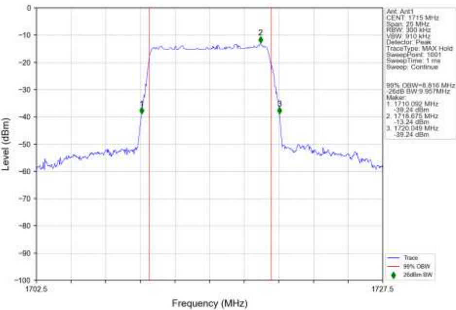
n66_30kHz_SISO_NTNV_10MHz_DFT-s-OFDM_16_QAM_1715MHz_Outer_Full_Ant1
