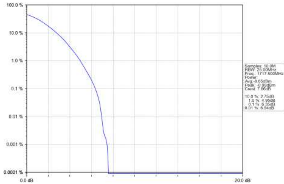
n66_15kHz_SISO_NTNV_15MHz_DFT-s-OFDM_64_QAM_1717.5MHz_Outer_Full_Ant1
