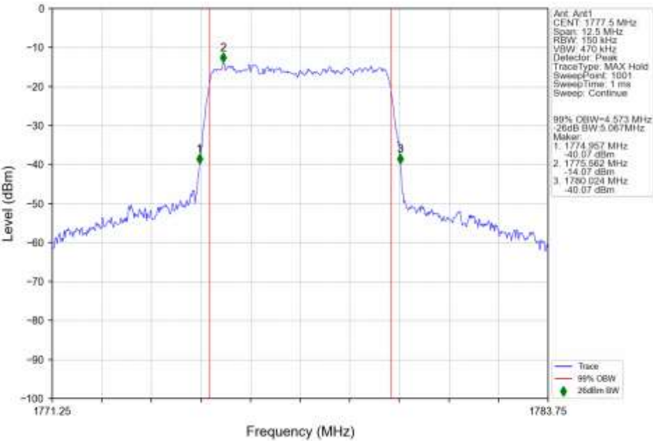
n66_15kHz_SISO_NTNV_5MHz_CP-OFDM_16_QAM_1777.5MHz_Outer_Full_Ant1
