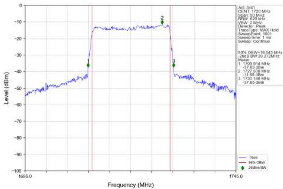
n66_30kHz_SISO_NTNV_20MHz_CP-OFDM_16_QAM_1720MHz_Outer_Full_Ant1
