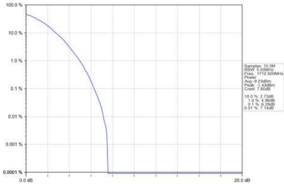
n66_15kHz_SISO_NTNV_5MHz_DFT-s-OFDM_64_QAM_1712.5MHz_Outer_Full_Ant1
