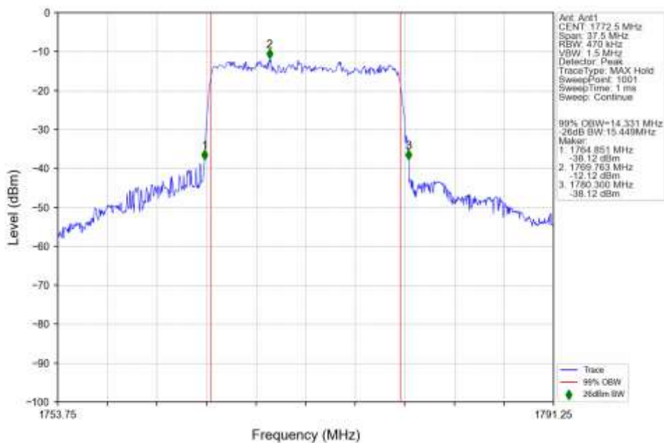
n66_15kHz_SISO_NTNV_15MHz_CP-OFDM_256_QAM_1772.5MHz_Outer_Full_Ant1
