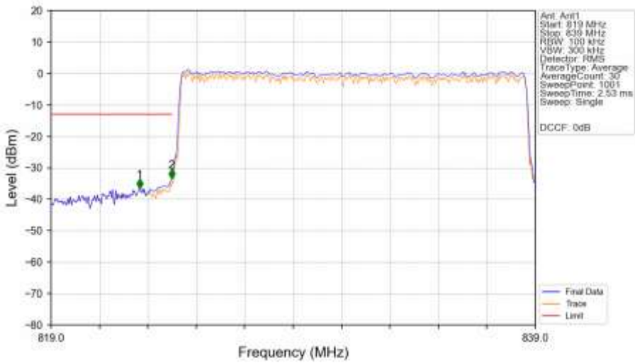
n5_15kHz_SISO_NTNV_15MHz_CP-OFDM_QPSK_831.5MHz_Outer_Full_Ant1
