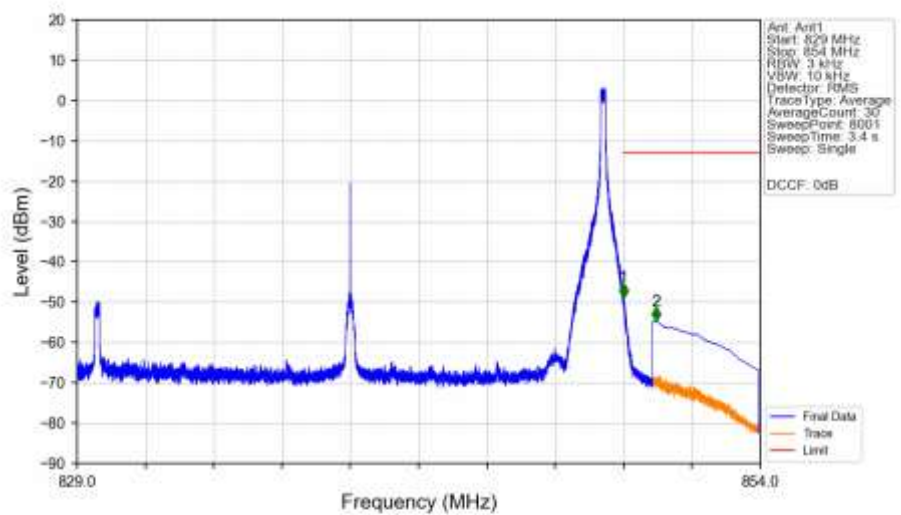
n5_15kHz_SISO_NTNV_20MHz_CP-OFDM_QPSK_839MHz_Inner_1RB_Right_Ant1
