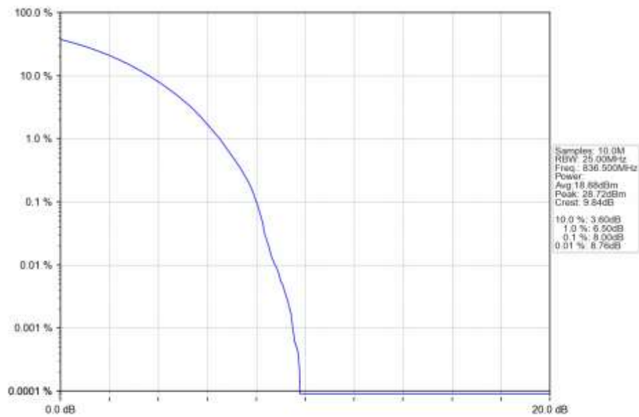
n5_30kHz_SISO_NTNV_15MHz_CP-OFDM_64_QAM_836.5MHz_Outer_Full_Ant1
