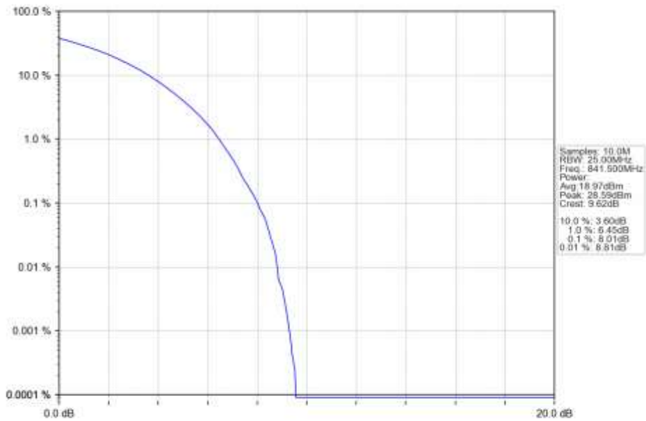
n5_30kHz_SISO_NTNV_15MHz_CP-OFDM_16_QAM_841.5MHz_Outer_Full_Ant1
