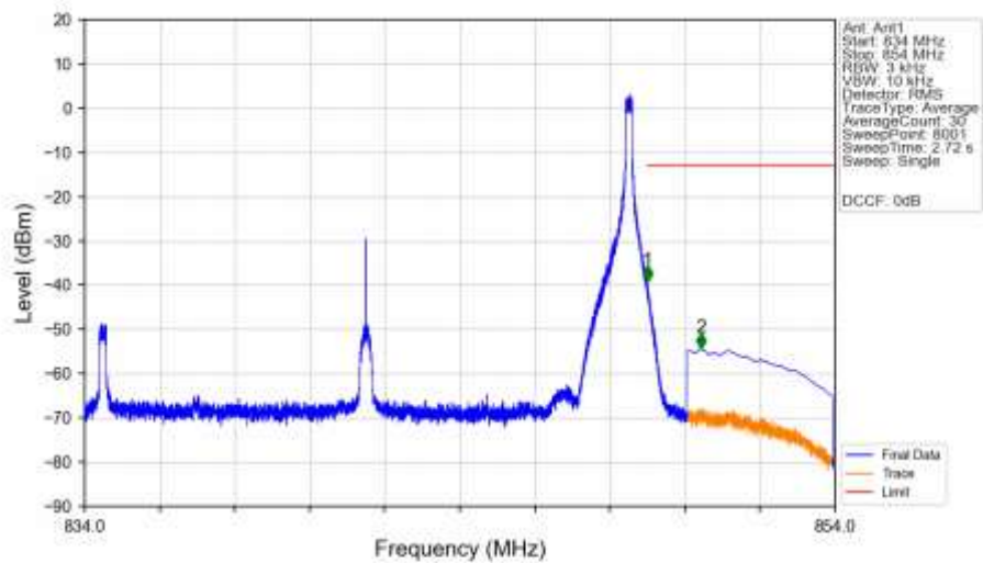
n5_15kHz_SISO_NTNV_15MHz_CP-OFDM_QPSK_841.5MHz_Edge_1RB_Right_Ant1
