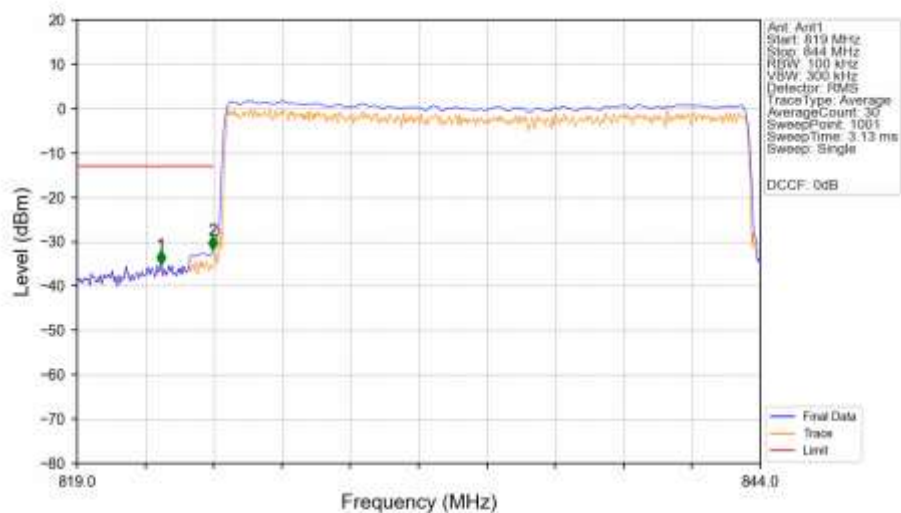
n5_15kHz_SISO_NTNV_20MHz_CP-OFDM_QPSK_834MHz_Outer_Full_Ant1
