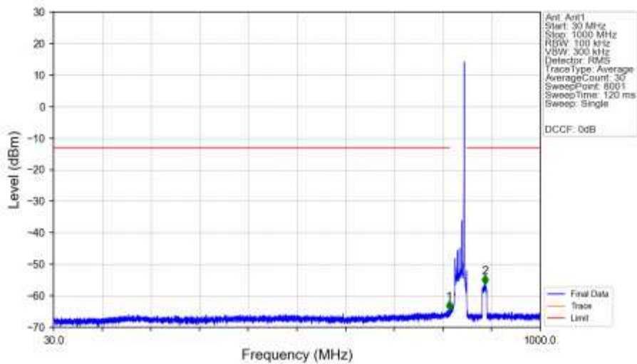
n5_15kHz_SISO_NTNV_10MHz_CP-OFDM_QPSK_844MHz_Edge_1RB_Right_Ant1
