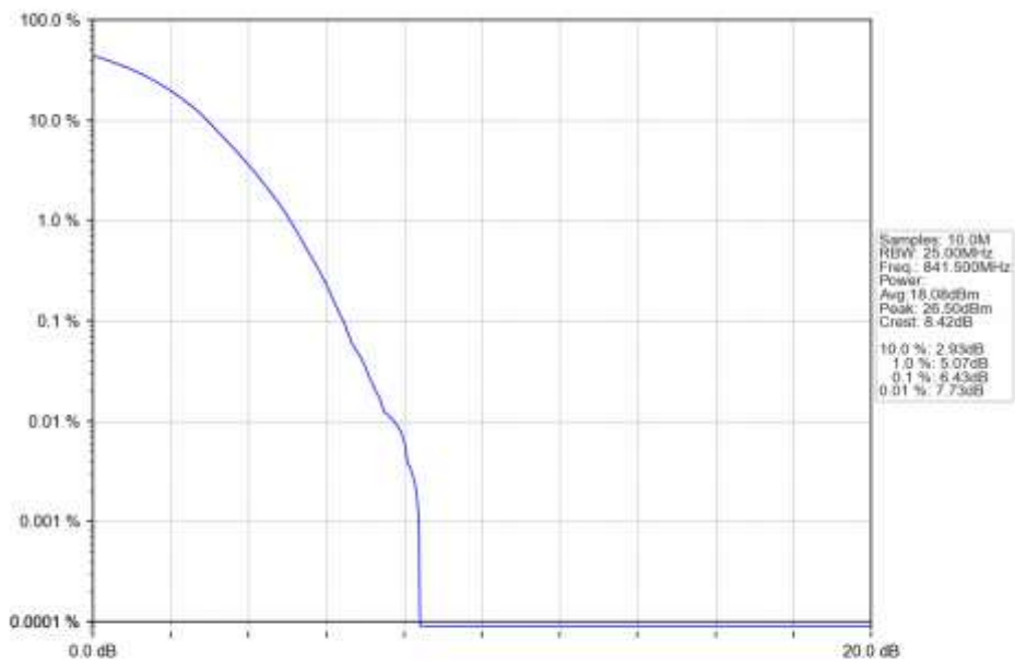
n5_30kHz_SISO_NTNV_15MHz_DFT-s-OFDM_256_QAM_841.5MHz_Outer_Full_Ant1
