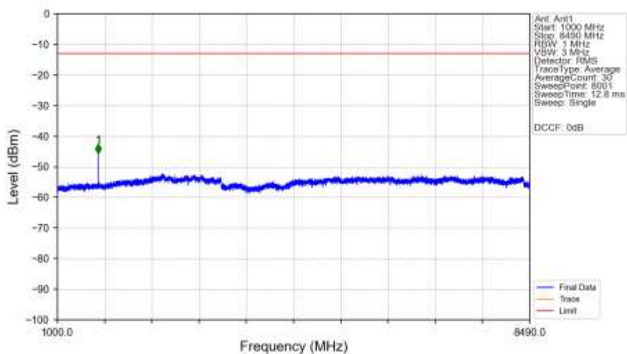
n5_15kHz_SISO_NTNV_20MHz_CP-OFDM_QPSK_834MHz_Edge_1RB_Left_Ant1
