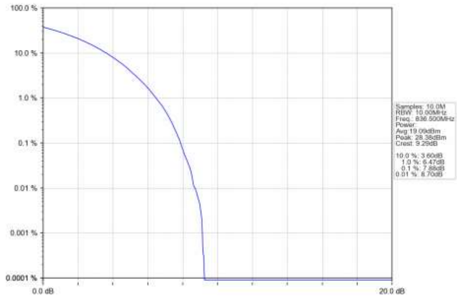
n5_30kHz_SISO_NTNV_10MHz_CP-OFDM_16_QAM_836.5MHz_Outer_Full_Ant1
