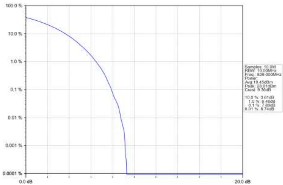
n5_30kHz_SISO_NTNV_10MHz_CP-OFDM_16_QAM_829MHz_Outer_Full_Ant1
