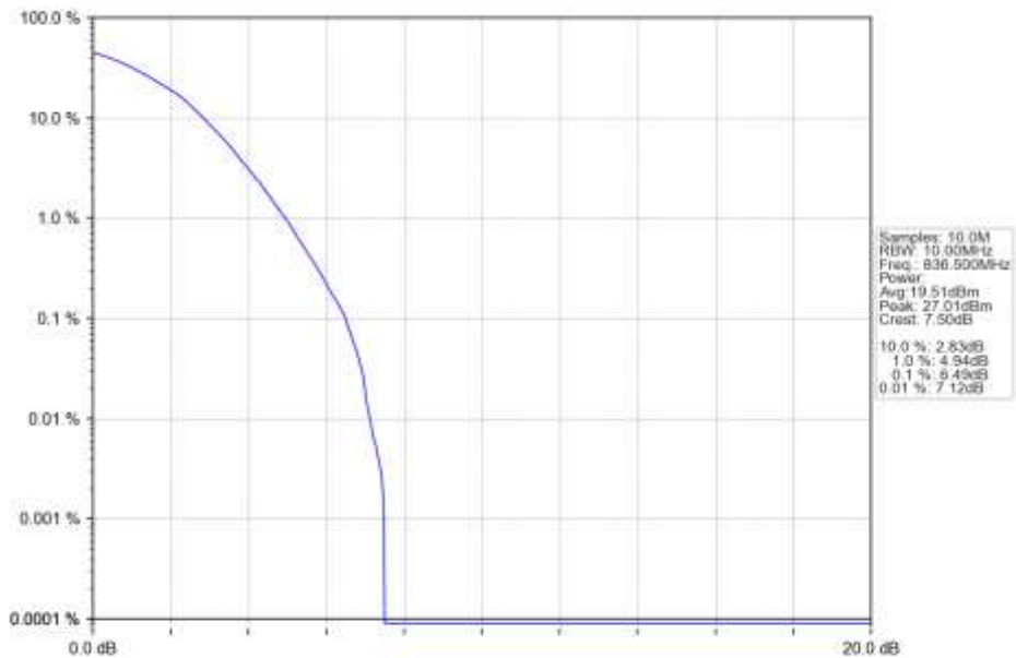
n5_30kHz_SISO_NTNV_10MHz_DFT-s-OFDM_64_QAM_836.5MHz_Outer_Full_Ant1
