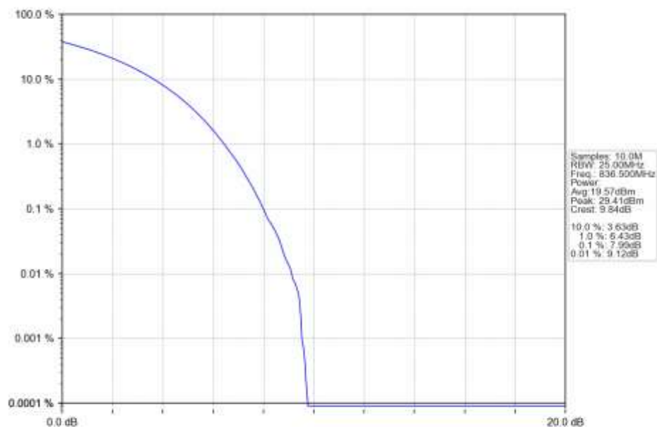
n5_30kHz_SISO_NTNV_20MHz_CP-OFDM_16_QAM_836.5MHz_Outer_Full_Ant1
