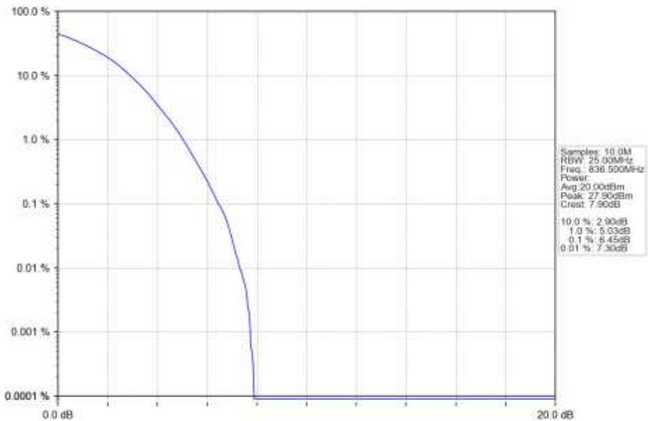
n5_30kHz_SISO_NTNV_20MHz_DFT-s-OFDM_64_QAM_836.5MHz_Outer_Full_Ant1
