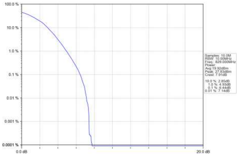
n5_30kHz_SISO_NTNV_10MHz_DFT-s-OFDM_64_QAM_829MHz_Outer_Full_Ant1
