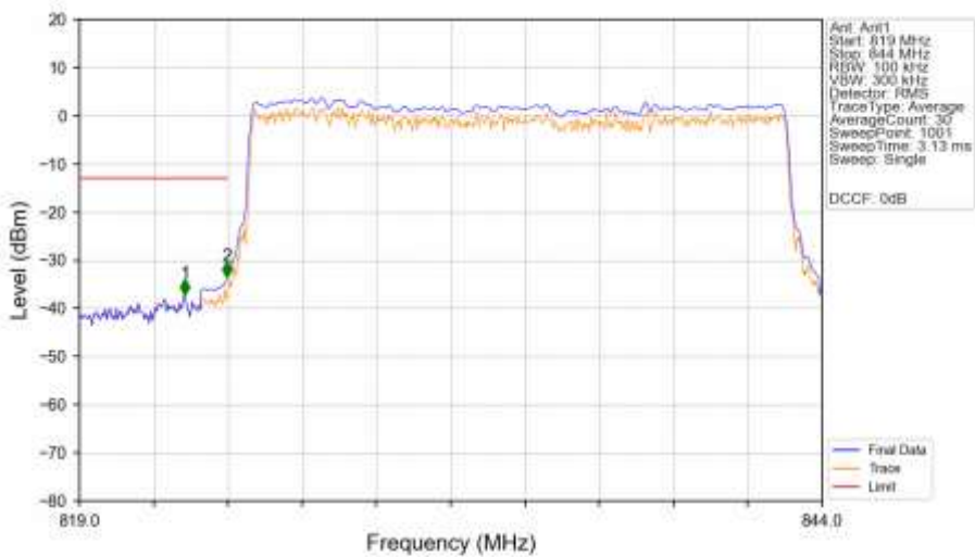
n5_30kHz_SISO_NTNV_20MHz_DFT-s-OFDM_QPSK_834MHz_Outer_Full_Ant1
