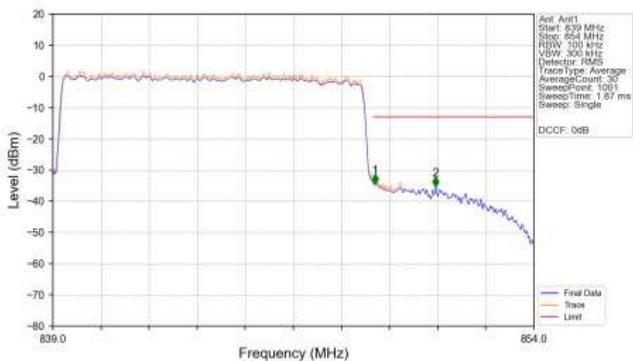
n5_15kHz_SISO_NTNV_10MHz_CP-OFDM_QPSK_844MHz_Outer_Full_Ant1
