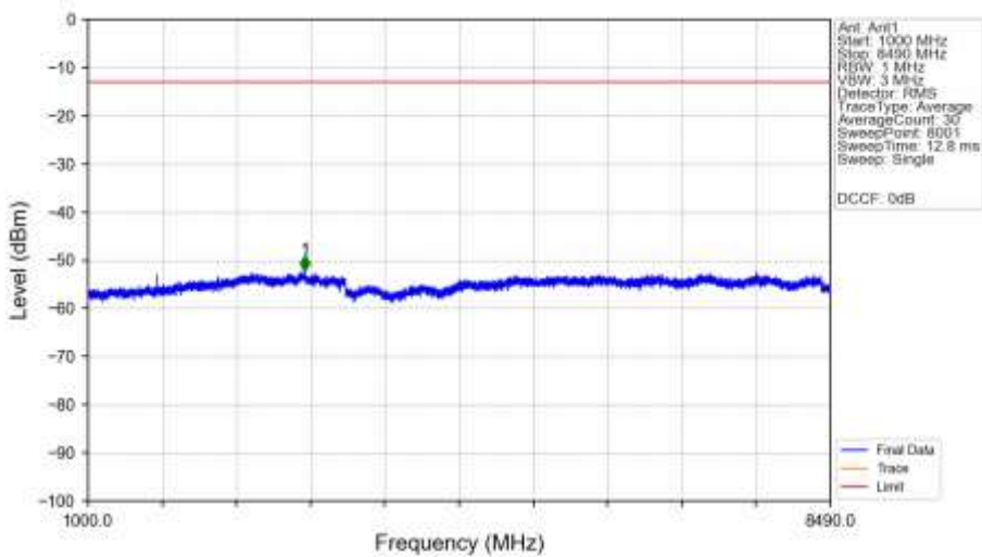
n5_15kHz_SISO_NTNV_20MHz_CP-OFDM_QPSK_839MHz_Edge_1RB_Right_Ant1
