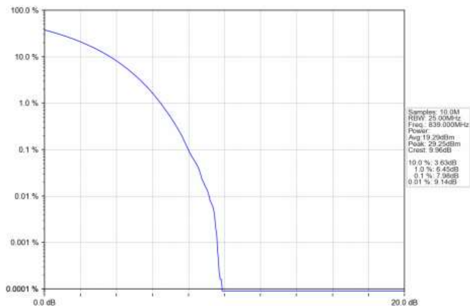
n5_30kHz_SISO_NTNV_20MHz_CP-OFDM_16_QAM_839MHz_Outer_Full_Ant1
