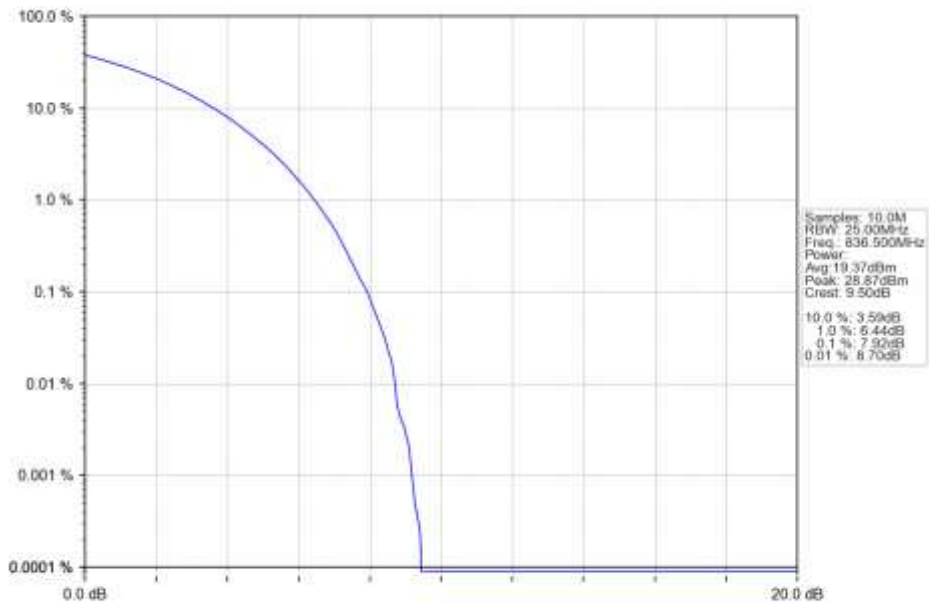
n5_30kHz_SISO_NTNV_15MHz_CP-OFDM_16_QAM_836.5MHz_Outer_Full_Ant1
