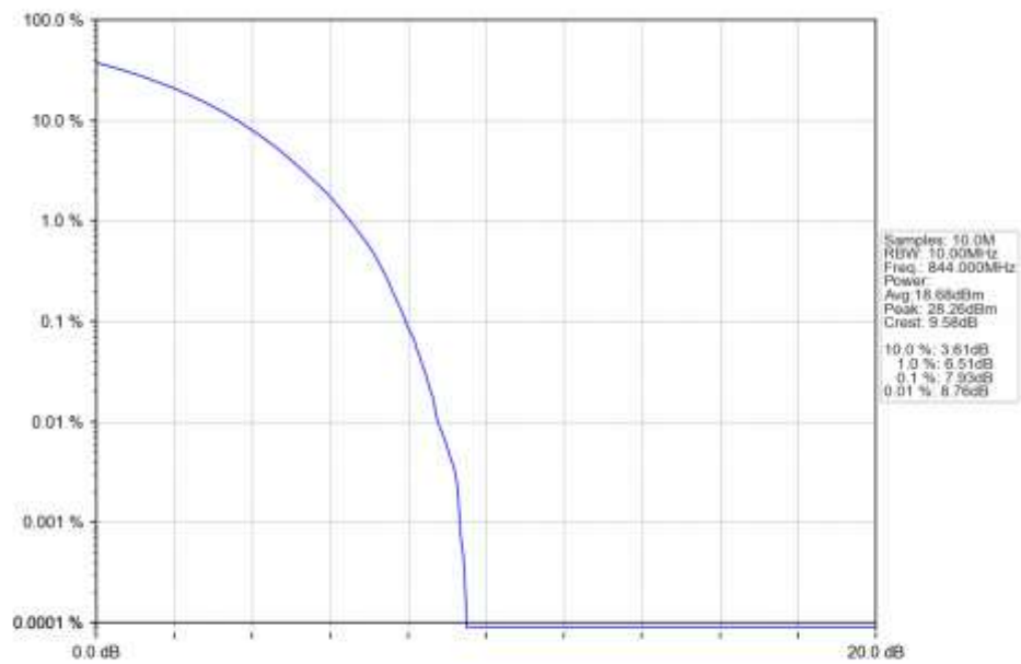
n5_30kHz_SISO_NTNV_10MHz_CP-OFDM_16_QAM_844MHz_Outer_Full_Ant1
