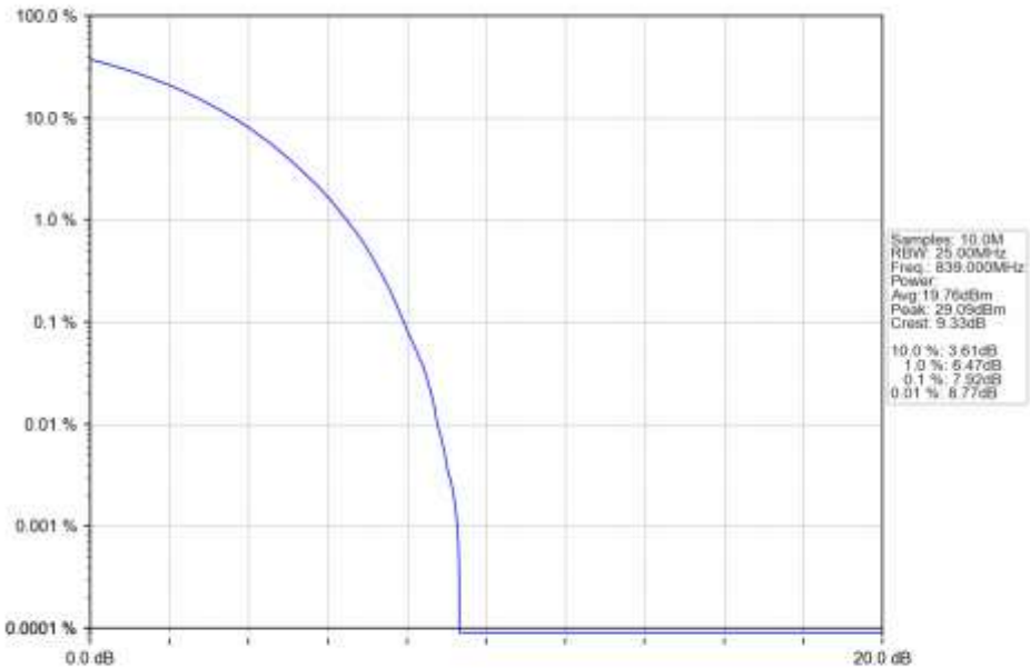
n5_30kHz_SISO_NTNV_20MHz_CP-OFDM_QPSK_839MHz_Outer_Full_Ant1
