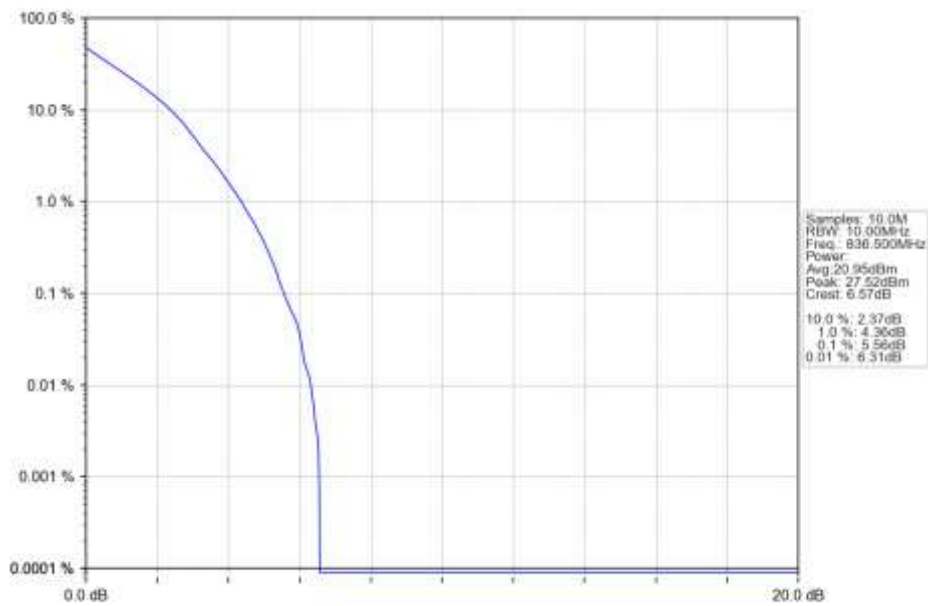
n5_30kHz_SISO_NTNV_10MHz_DFT-s-OFDM QPSK_836.5MHz_Outer_Full_Ant1
