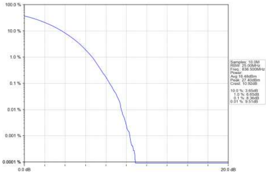
n5_30kHz_SISO_NTNV_15MHz_CP-OFDM_256_QAM_836.5MHz_Outer_Full_Ant1
