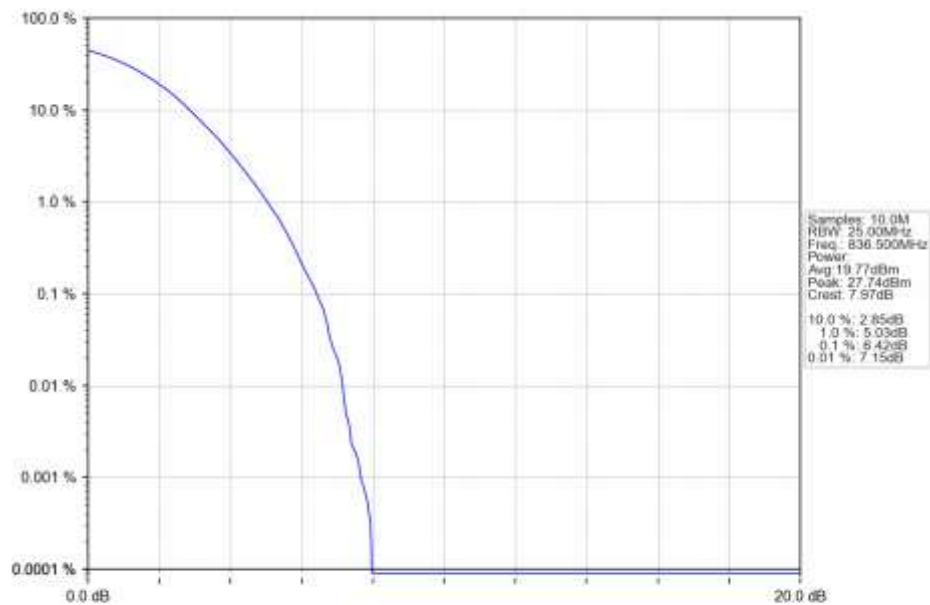
n5_30kHz_SISO_NTNV_15MHz_DFT-s-OFDM_64_QAM_836.5MHz_Outer_Full_Ant1
