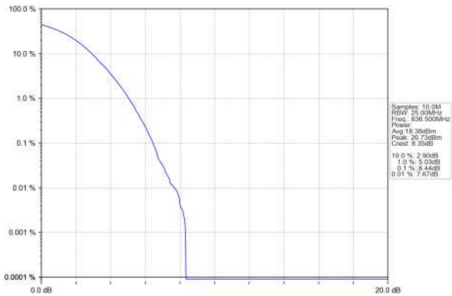
n5_30kHz_SISO_NTNV_15MHz_DFT-s-OFDM_256_QAM_836.5MHz_Outer_Full_Ant1
