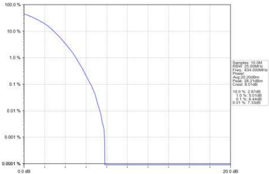
n5_30kHz_SISO_NTNV_20MHz_DFT-s-OFDM_64_QAM_834MHz_Outer_Full_Ant1
