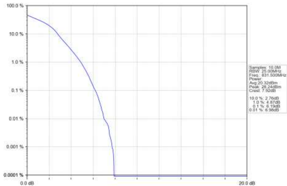
n5_30kHz_SISO_NTNV_15MHz_DFT-s-OFDM_16QAM_831.5MHz_Outer_Full_Ant1
