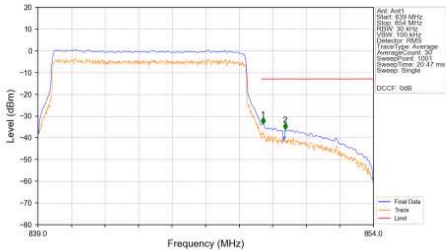
n5_30kHz_SISO_NTNV_10MHz_CP-OFDM_QPSK_844MHz_Outer_Full_Ant1
