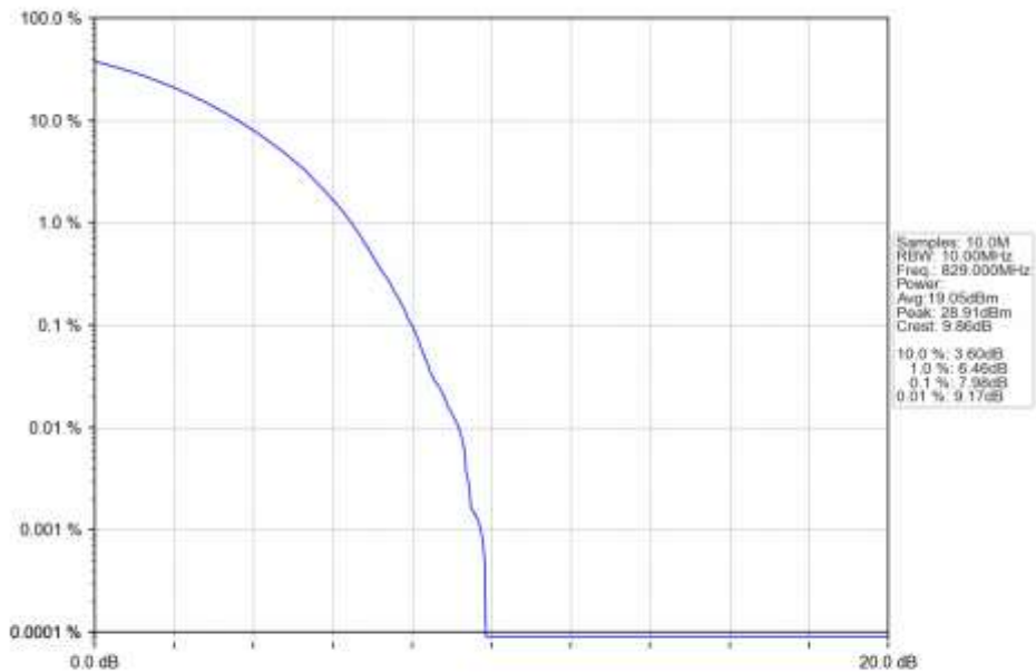
n5_30kHz_SISO_NTNV_10MHz_CP-OFDM_64_QAM_829MHz_Outer_Full_Ant1
