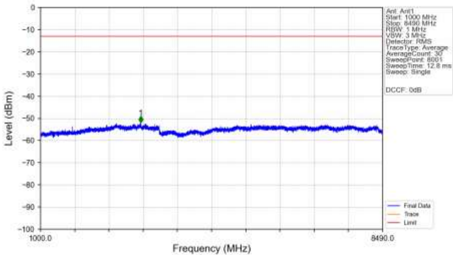
n5_15kHz_SISO_NTNV_10MHz_CP-OFDM_QPSK_844MHz_Edge_1RB_Right_Ant1
