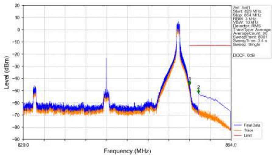
n5_30kHz_SISO_NTNV_20MHz_DFT-s-OFDM_QPSK_839MHz_Inner_1RB_Right_Ant1
