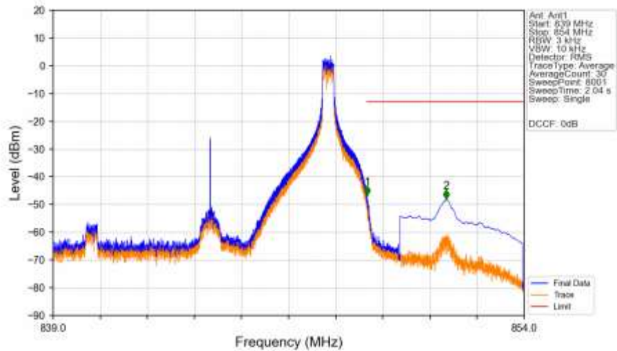
n5_30kHz_SISO_NTNV_10MHz_CP-OFDM_QPSK_844MHz_Inner_1RB_Right_Ant1
