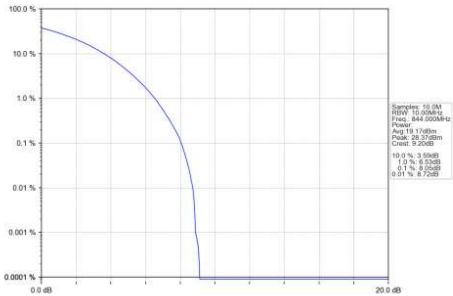
n5_30kHz_SISO_NTNV_10MHz_CP-OFDM_QPSK_844MHz_Outer_Full_Ant1
