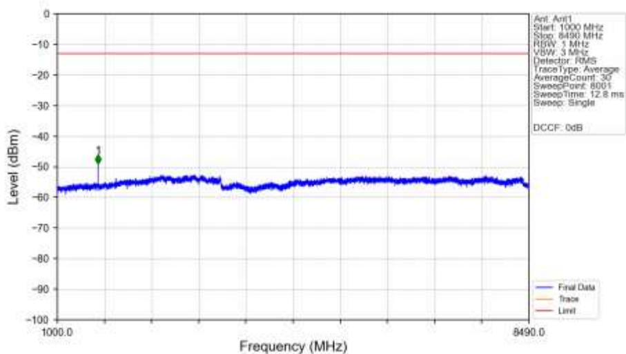
n5_30kHz_SISO_NTNV_10MHz_CP-OFDM_QPSK_829MHz_Edge_1RB_Left_Ant1
