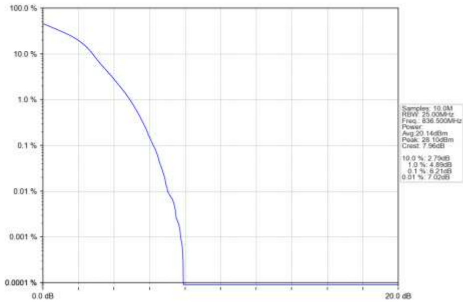
n5_30kHz_SISO_NTNV_15MHz_DFT-s-OFDM_16_QAM_836.5MHz_Outer_Full_Ant1
