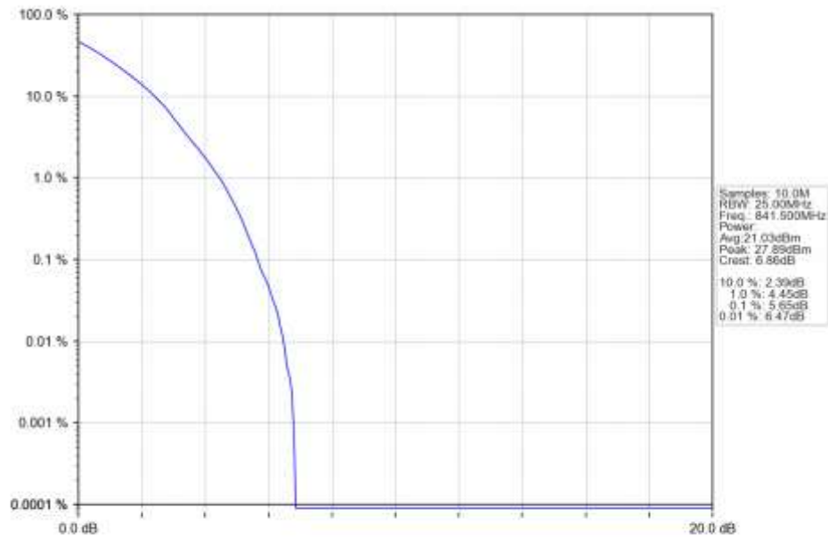
n5_30kHz_SISO_NTNV_15MHz_DFT-s-OFDM_QPSK_841.5MHz_Outer_Full_Ant1
