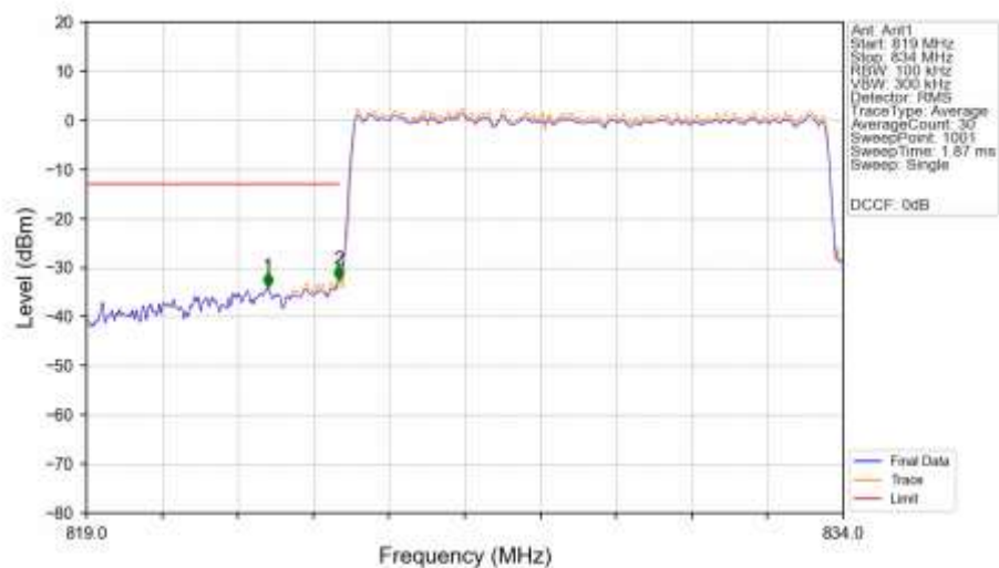
n5_15kHz_SISO_NTNV_10MHz_CP-OFDM_QPSK_829MHz_Outer_Full_Ant1
