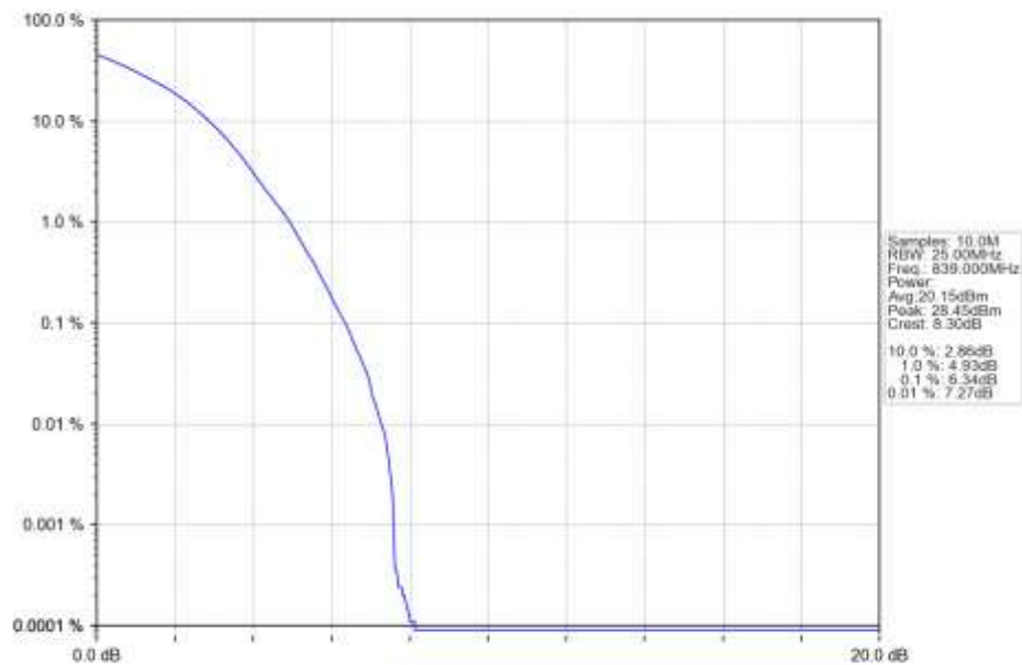
n5_30kHz_SISO_NTNV_20MHz_DFT-s-OFDM_16_QAM_839MHz_Outer_Full_Ant1
