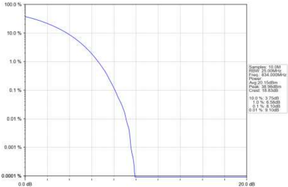
n5_30kHz_SISO_NTNV_20MHz_CP-OFDM_16_QAM_834MHz_Outer_Full_Ant1
