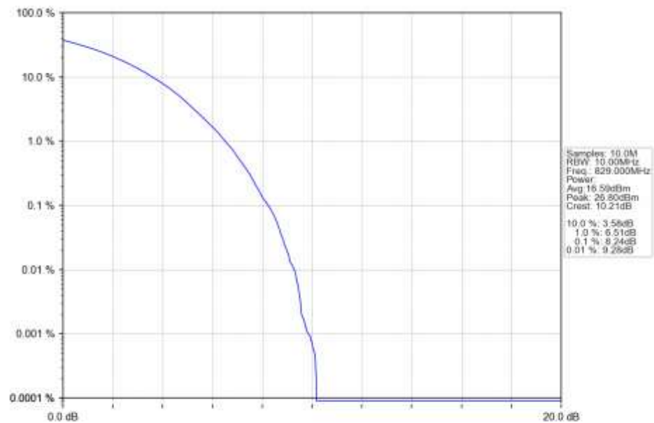
n5_30kHz_SISO_NTNV_10MHz_CP-OFDM_256_QAM_829MHz_Outer_Full_Ant1
