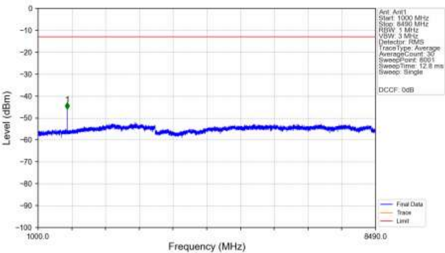
n5_15kHz_SISO_NTNV_15MHz_CP-OFDM_QPSK_831.5MHz_Edge_1RB_Left_Ant1
