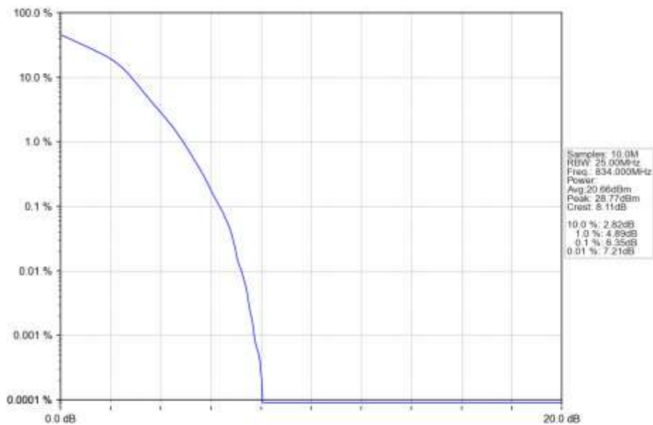
n5_30kHz_SISO_NTNV_20MHz_DFT-s-OFDM_16QAM_834MHz_Outer_Full_Ant1
