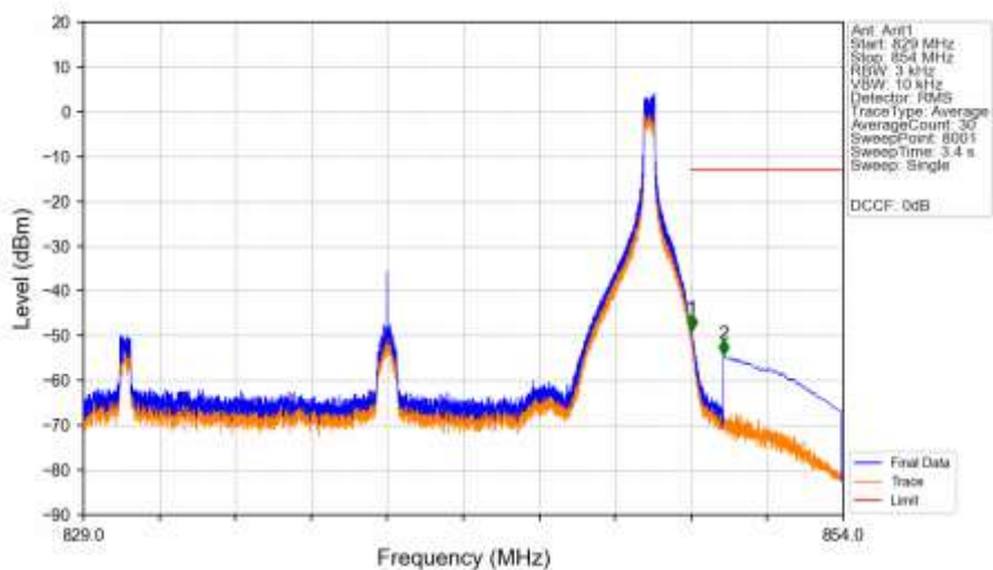
n5_30kHz_SISO_NTNV_20MHz_CP-OFDM_QPSK_839MHz_Inner_1RB_Right_Ant1
