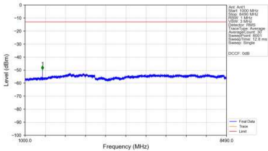
n5_15kHz_SISO_NTNV_5MHz_CP-OFDM_QPSK_826.5MHz_Edge_1RB_Left_Ant1
