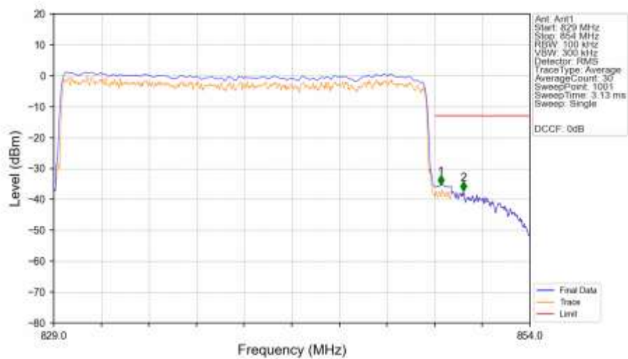
n5_15kHz_SISO_NTNV_20MHz_CP-OFDM_QPSK_839MHz_Outer_Full_Ant1
