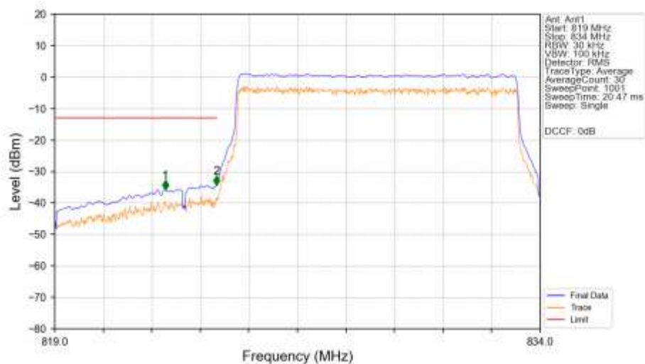
n5_30kHz_SISO_NTNV_10MHz_CP-OFDM_QPSK_829MHz_Outer_Full_Ant1
