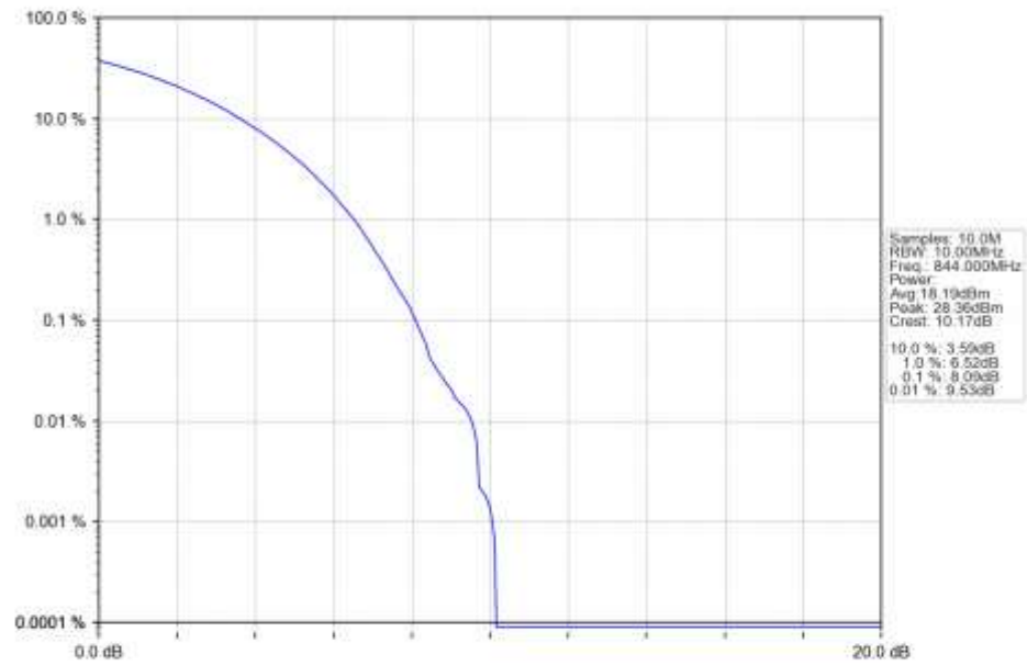
n5_30kHz_SISO_NTNV_10MHz_CP-OFDM_64_QAM_844MHz_Outer_Full_Ant1
