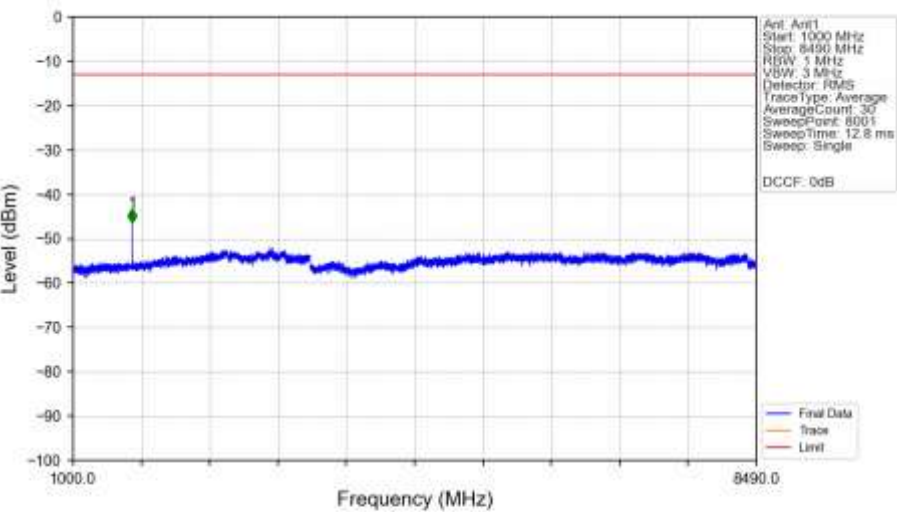
n5_30kHz_SISO_NTNV_20MHz_DFT-s-OFDM_QPSK_834MHz_Edge_1RB_Left_Ant1
