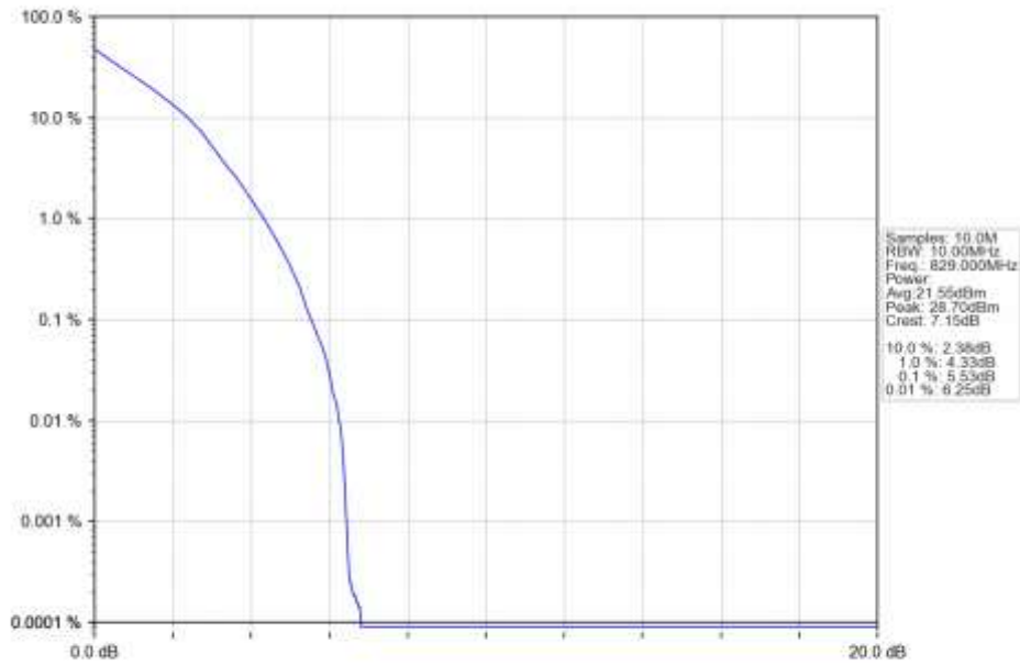
n5_30kHz_SISO_NTNV_10MHz_DFT-s-OFDM QPSK_829MHz_Outer_Full_Ant1
