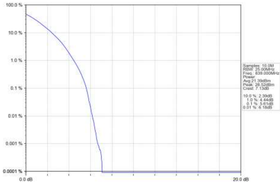
n5_30kHz_SISO_NTNV_20MHz_DFT-s-OFDM_QPSK_839MHz_Outer_Full_Ant1
