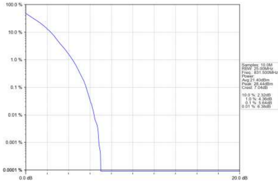
n5_30kHz_SISO_NTNV_15MHz_DFT-s-OFDM QPSK_831.5MHz_Outer_Full_Ant1
