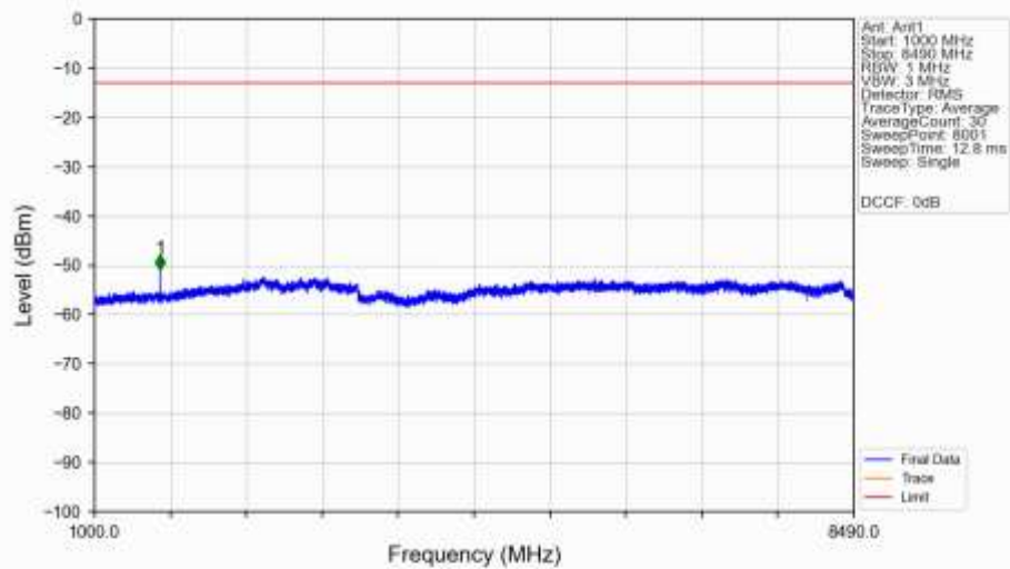
n5_15kHz_SISO_NTNV_10MHz_CP-OFDM_QPSK_829MHz_Edge_1RB_Left_Ant1
