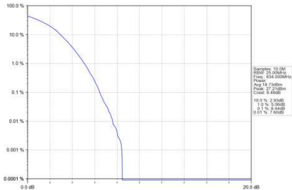
n5_30kHz_SISO_NTNV_20MHz_DFT-s-OFDM_256_QAM_834MHz_Outer_Full_Ant1
