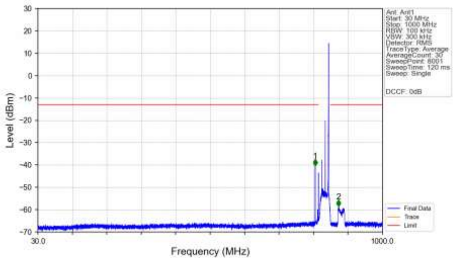
n5_15kHz_SISO_NTNV_20MHz_CP-OFDM_QPSK_839MHz_Edge_1RB_Right_Ant1
