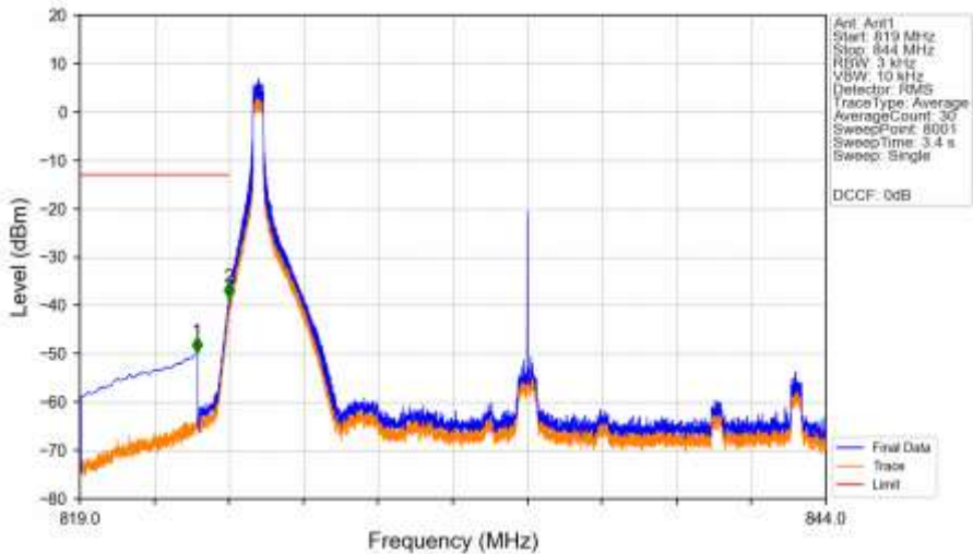
n5_30kHz_SISO_NTNV_20MHz_DFT-s-OFDM_QPSK_834MHz_Edge_1RB_Left_Ant1
