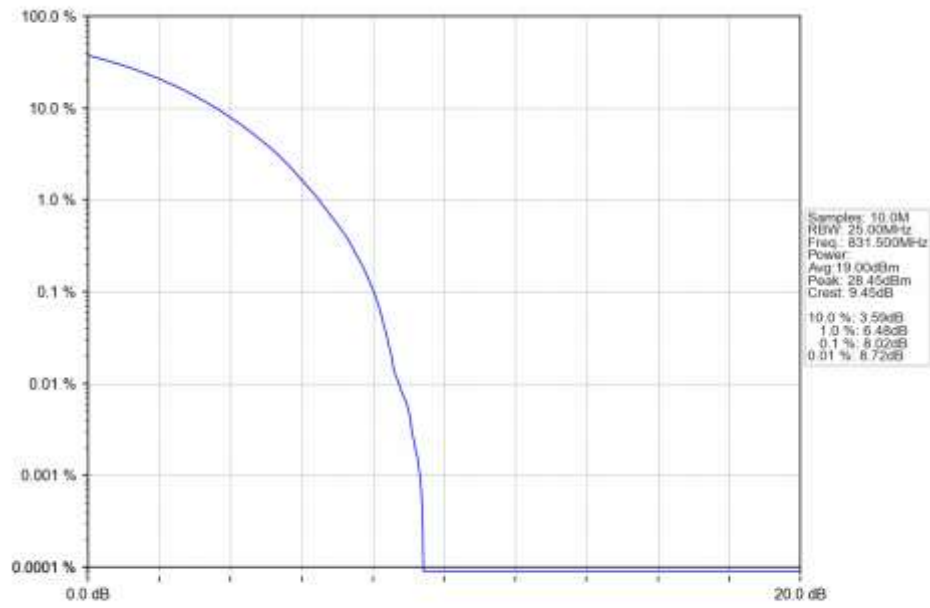
n5_30kHz_SISO_NTNV_15MHz_CP-OFDM_64_QAM_831.5MHz_Outer_Full_Ant1
