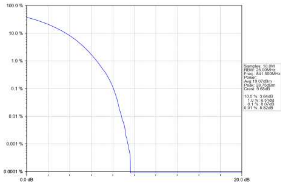
n5_15kHz_SISO_NTNV_15MHz_CP-OFDM_16_QAM_841.5MHz_Outer_Full_Ant1
