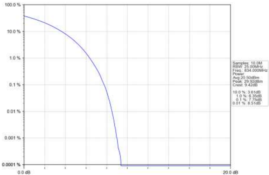
n5_15kHz_SISO_NTNV_20MHz_CP-OFDM_QPSK_834MHz_Outer_Full_Ant1
