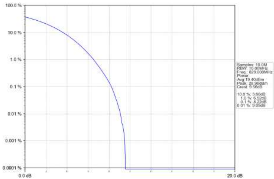
n5_15kHz_SISO_NTNV_10MHz_CP-OFDM_16_QAM_829MHz_Outer_Full_Ant1
