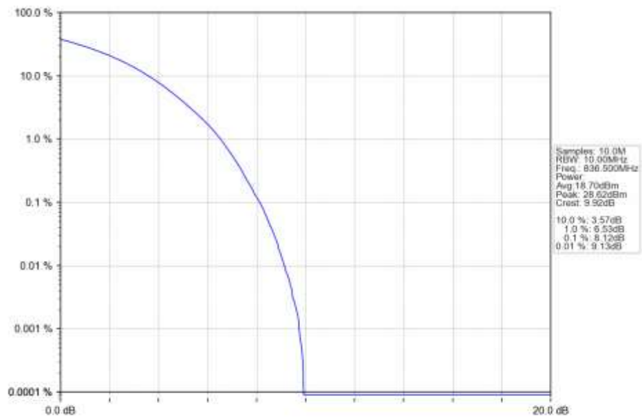
n5_15kHz_SISO_NTNV_10MHz_CP-OFDM_64_QAM_836.5MHz_Outer_Full_Ant1
