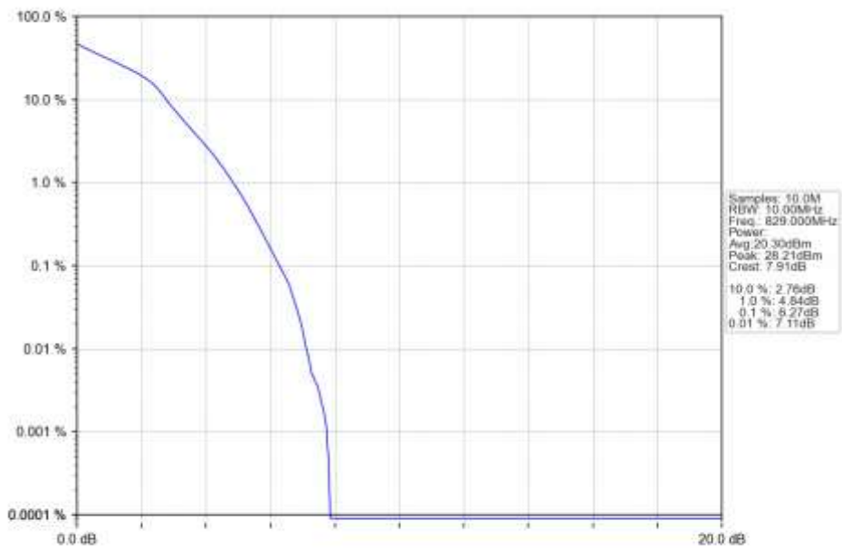
n5_15kHz_SISO_NTNV_10MHz_DFT-s-OFDM_16_QAM_829MHz_Outer_Full_Ant1
