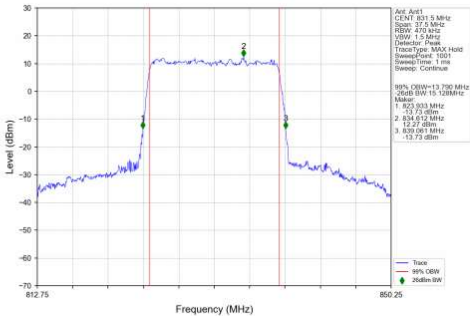
n5_30kHz_SISO_NTNV_15MHz_CP-OFDM_256_QAM_831.5MHz_Outer_Full_Ant1
