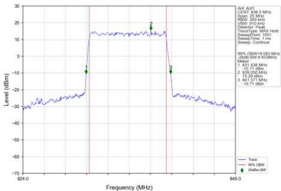
n5_15kHz_SISO_NTNV_10MHz_DFT-s-OFDM_64_QAM_836.5MHz_Outer_Full_Ant1
