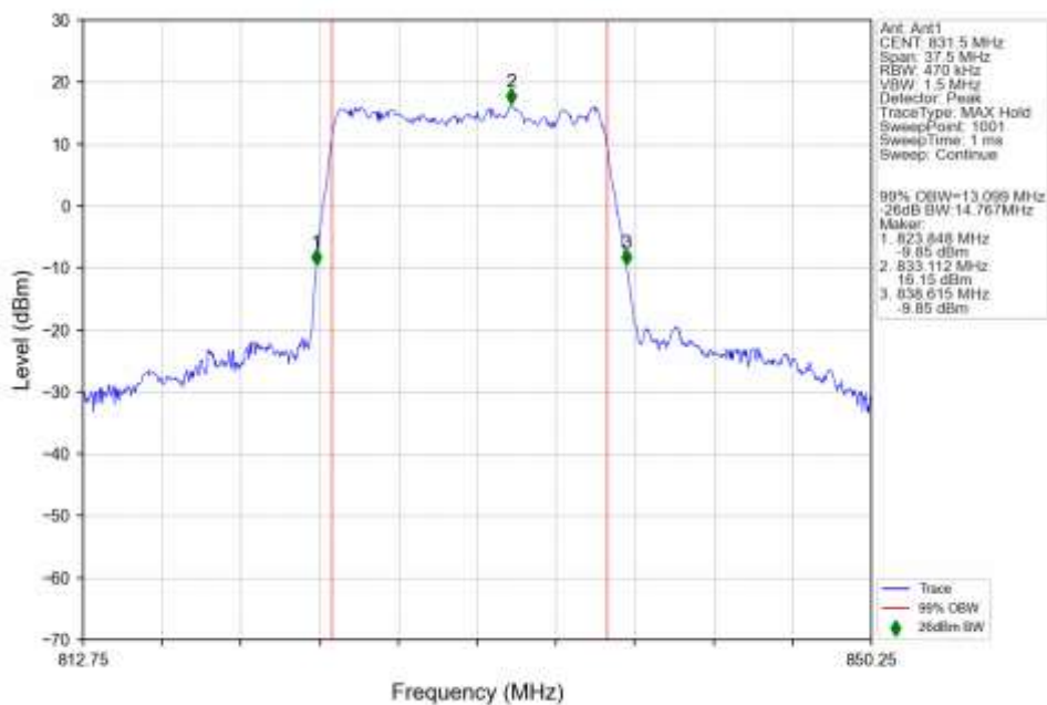
n5_30kHz_SISO_NTNV_15MHz_DFT-s-OFDM_16_QAM_831.5MHz_Outer_Full_Ant1
