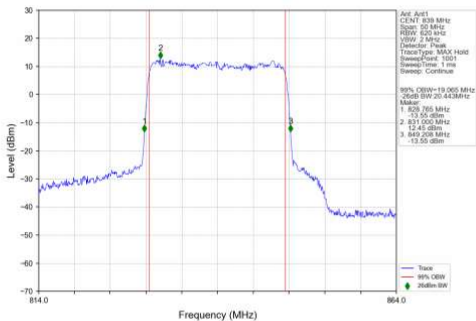
n5_15kHz_SISO_NTNV_20MHz_CP-OFDM_256_QAM_839MHz_Outer_Full_Ant1
