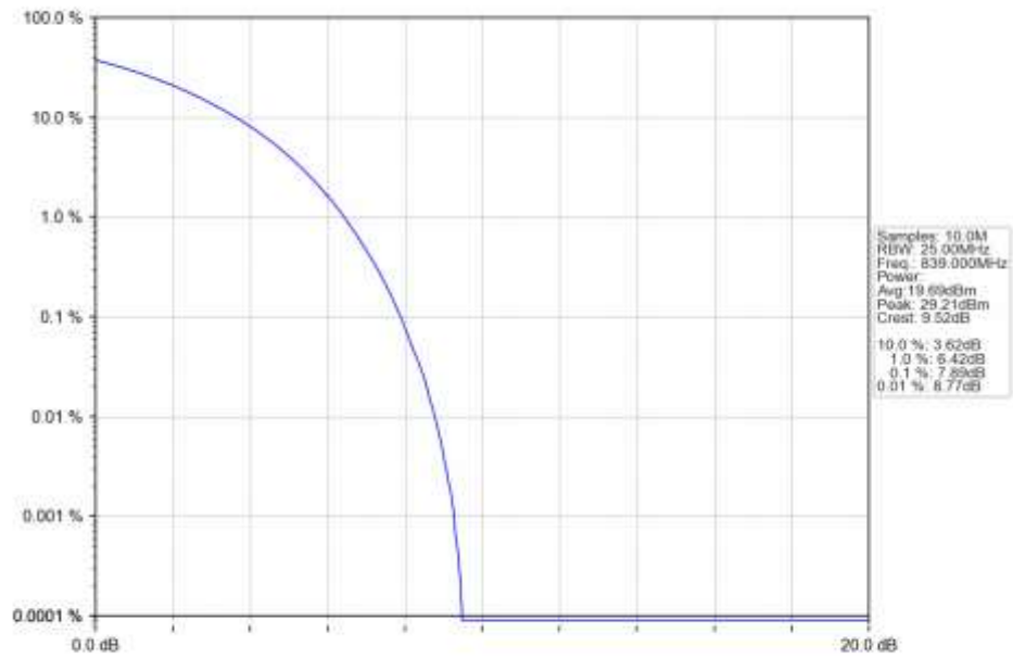
n5_15kHz_SISO_NTNV_20MHz_CP-OFDM_QPSK_839MHz_Outer_Full_Ant1
