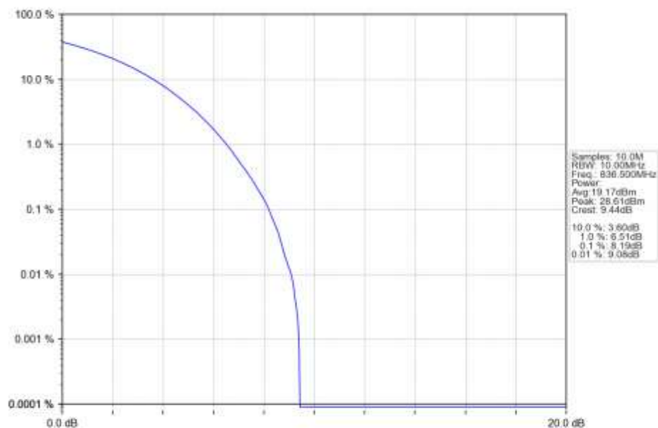
n5_15kHz_SISO_NTNV_10MHz_CP-OFDM_16_QAM_836.5MHz_Outer_Full_Ant1
