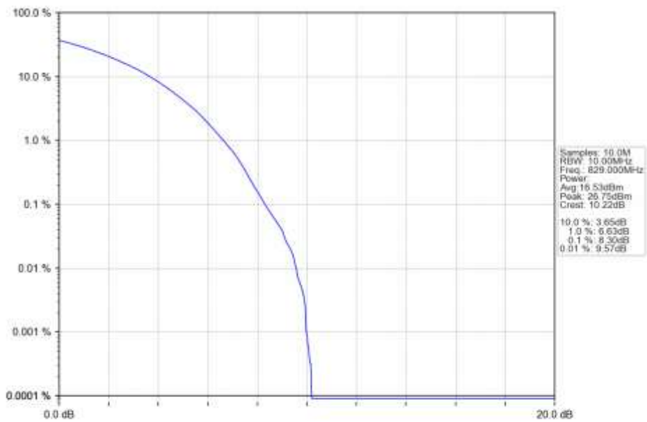
n5_15kHz_SISO_NTNV_10MHz_CP-OFDM_256_QAM_829MHz_Outer_Full_Ant1
