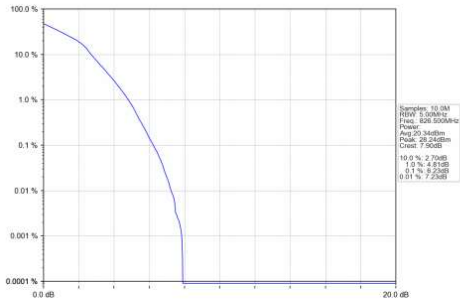
n5_15kHz_SISO_NTNV_5MHz_DFT-s-OFDM 16 QAM 826.5MHz_Outer_Full_Ant1
