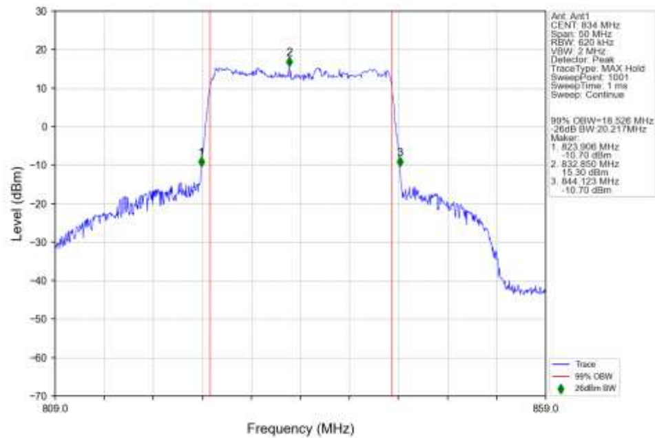
n5_30kHz_SISO_NTNV_20MHz_CP-OFDM_16_QAM_834MHz_Outer_Full_Ant1
