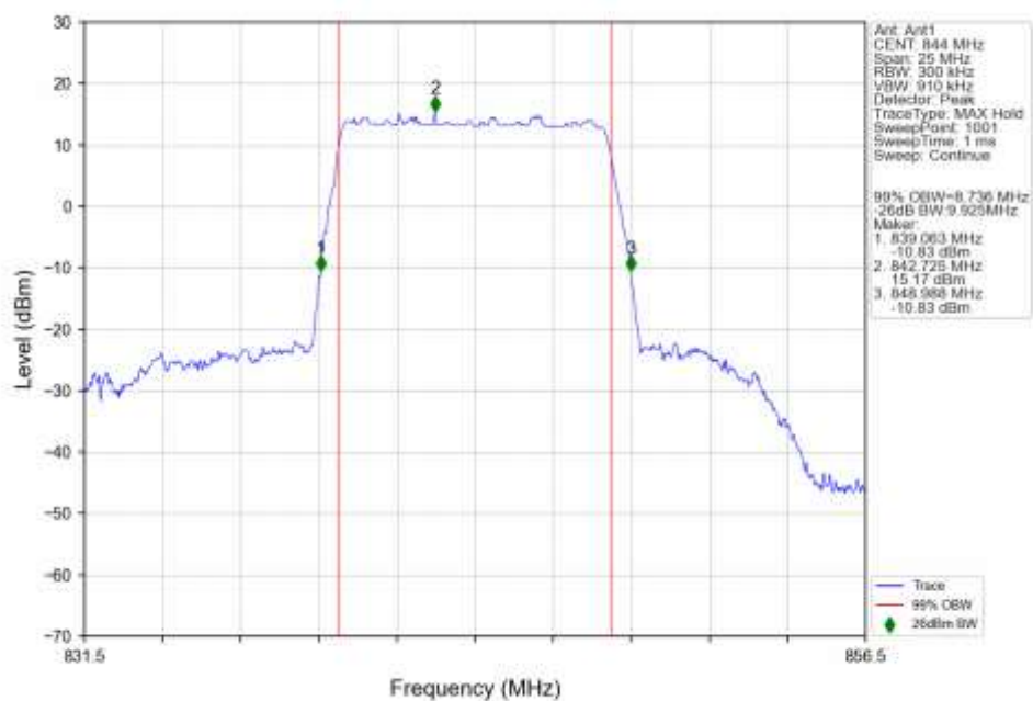
n5_30kHz_SISO_NTNV_10MHz_DFT-s-OFDM_16_QAM_844MHz_Outer_Full_Ant1
