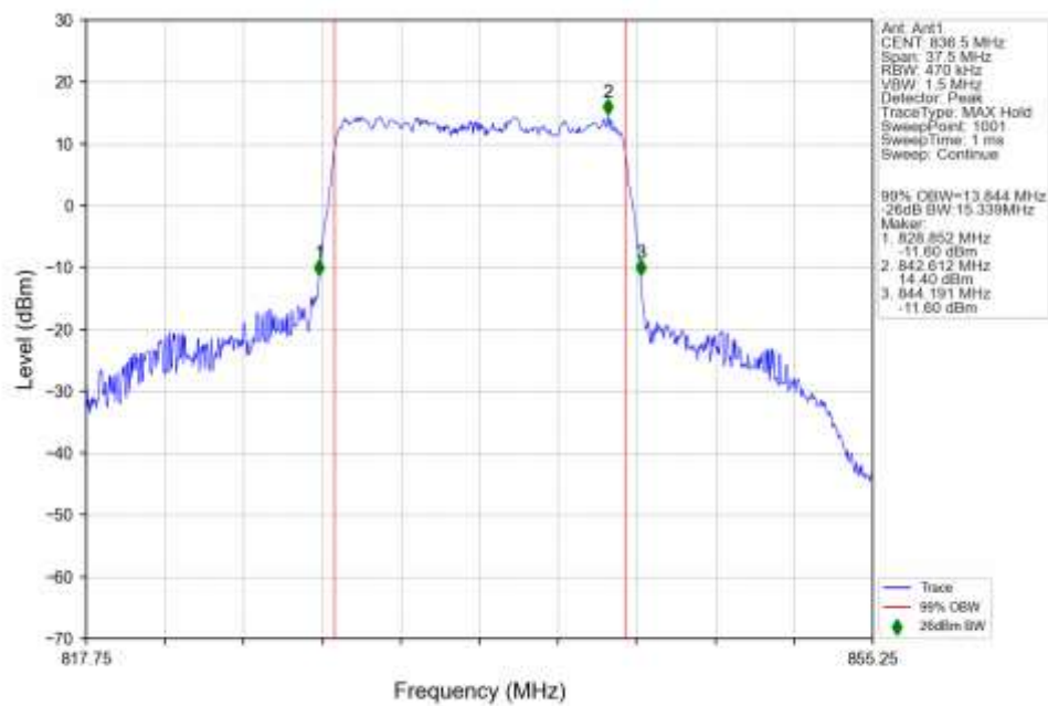
n5_30kHz_SISO_NTNV_15MHz_CP-OFDM_64_QAM_836.5MHz_Outer_Full_Ant1
