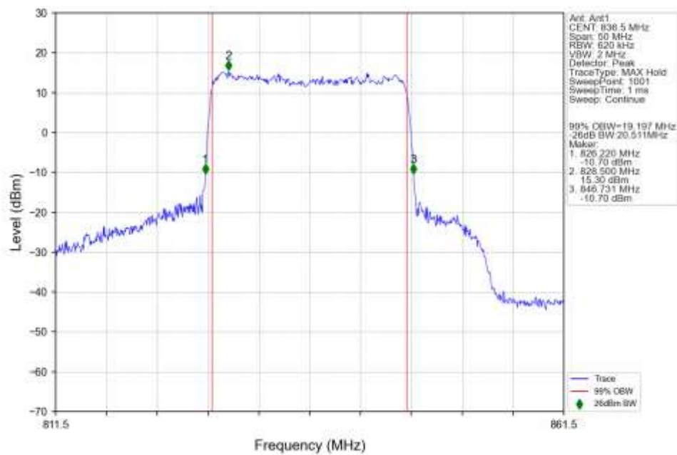
n5_15kHz_SISO_NTNV_20MHz_CP-OFDM_64_QAM_836.5MHz_Outer_Full_Ant1
