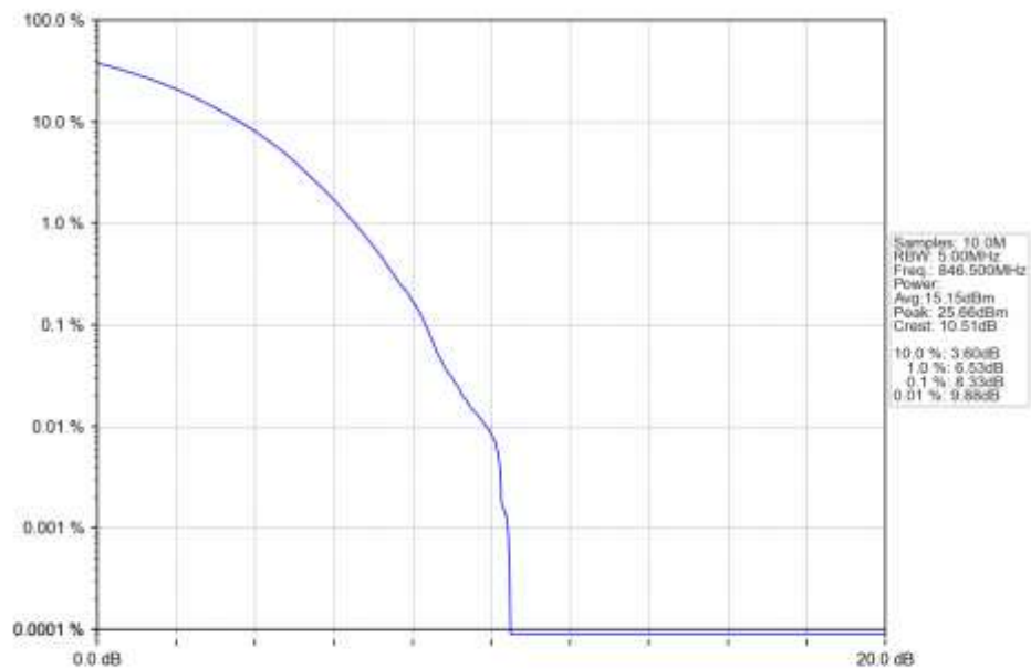
n5_15kHz_SISO_NTNV_5MHz_CP-OFDM_256_QAM_846.5MHz_Outer_Full_Ant1
