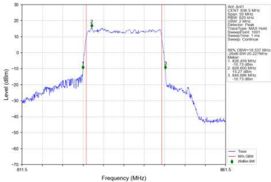
n5_30kHz_SISO_NTNV_20MHz_CP-OFDM_64_QAM_836.5MHz_Outer_Full_Ant1
