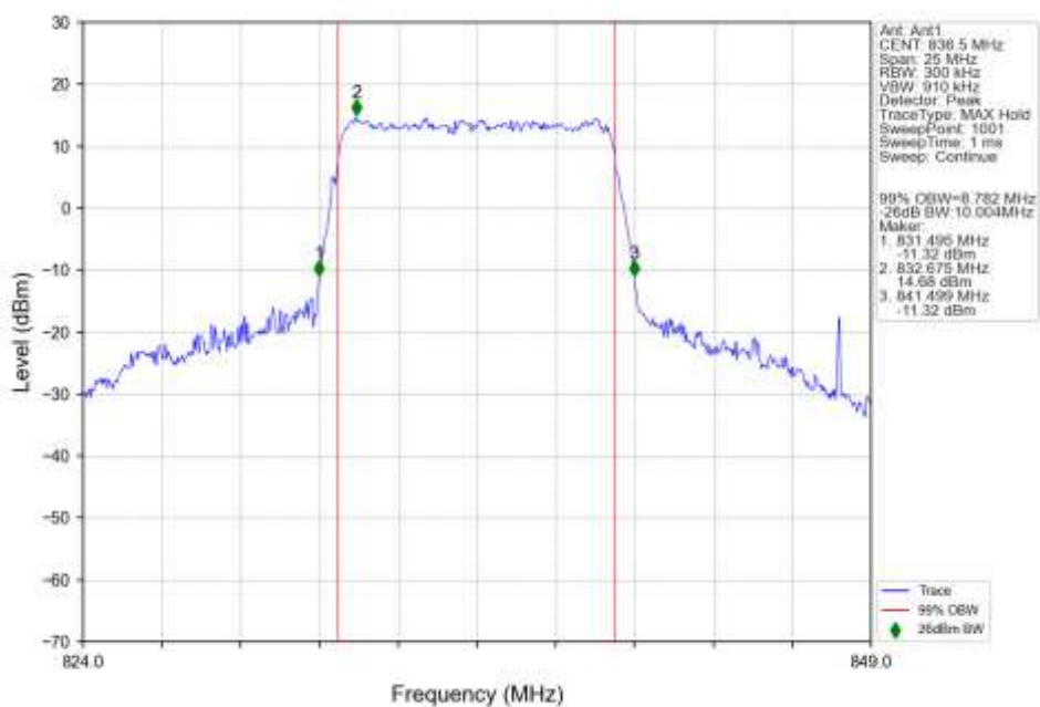
n5_30kHz_SISO_NTNV_10MHz_CP-OFDM_QPSK_836.5MHz_Outer_Full_Ant1
