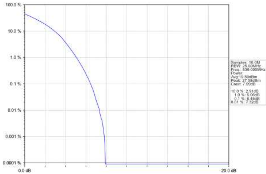
n5_15kHz_SISO_NTNV_20MHz_DFT-s-OFDM_64_QAM_839MHz_Outer_Full_Ant1
