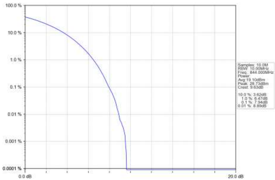
n5_15kHz_SISO_NTNV_10MHz_CP-OFDM_QPSK_844MHz_Outer_Full_Ant1
