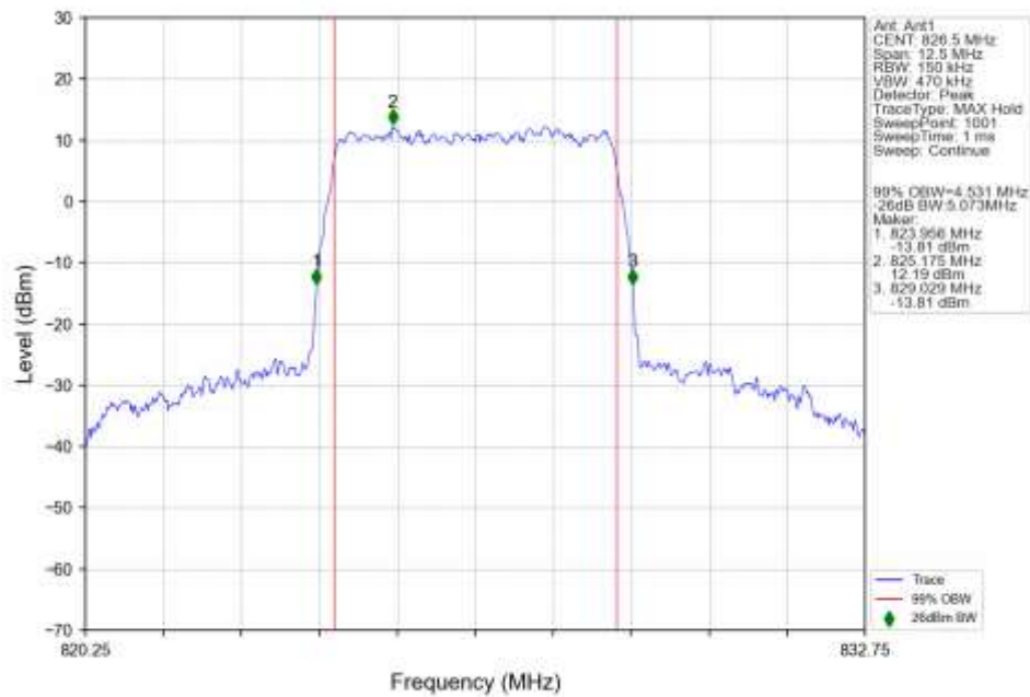
n5_15kHz_SISO_NTNV_5MHz_CP-OFDM_256_QAM_826.5MHz_Outer_Full_Ant1
