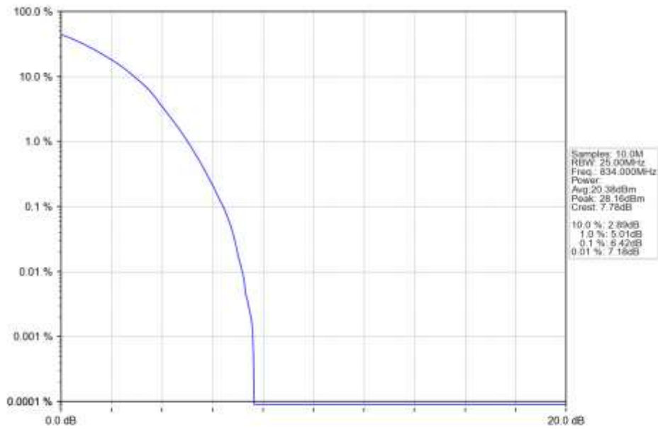
n5_15kHz_SISO_NTNV_20MHz_DFT-s-OFDM_64_QAM_834MHz_Outer_Full_Ant1
