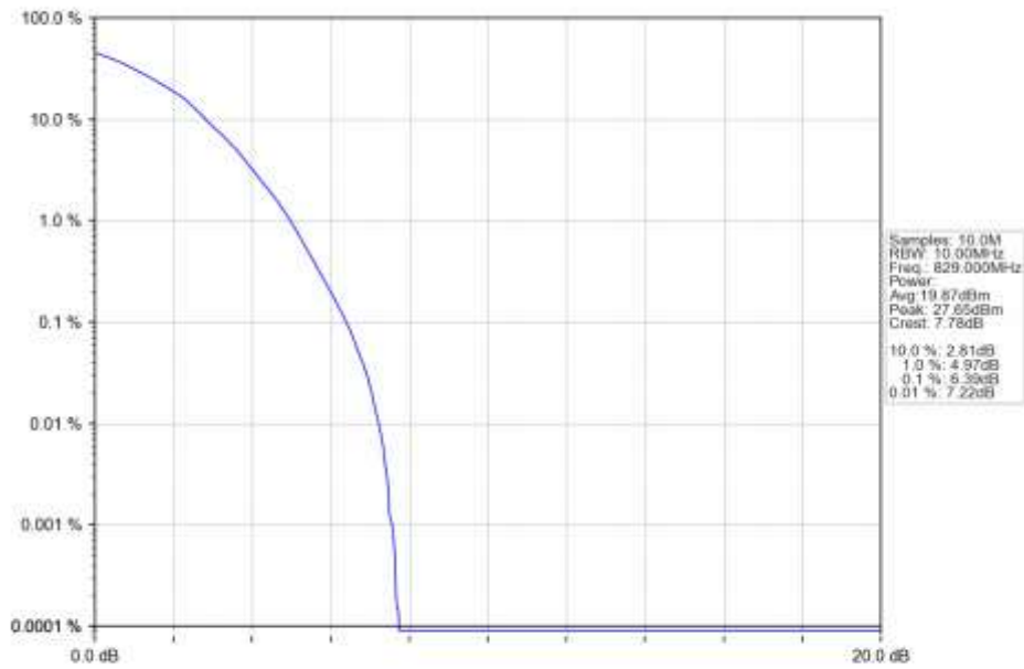
n5_15kHz_SISO_NTNV_10MHz_DFT-s-OFDM_64_QAM_829MHz_Outer_Full_Ant1
