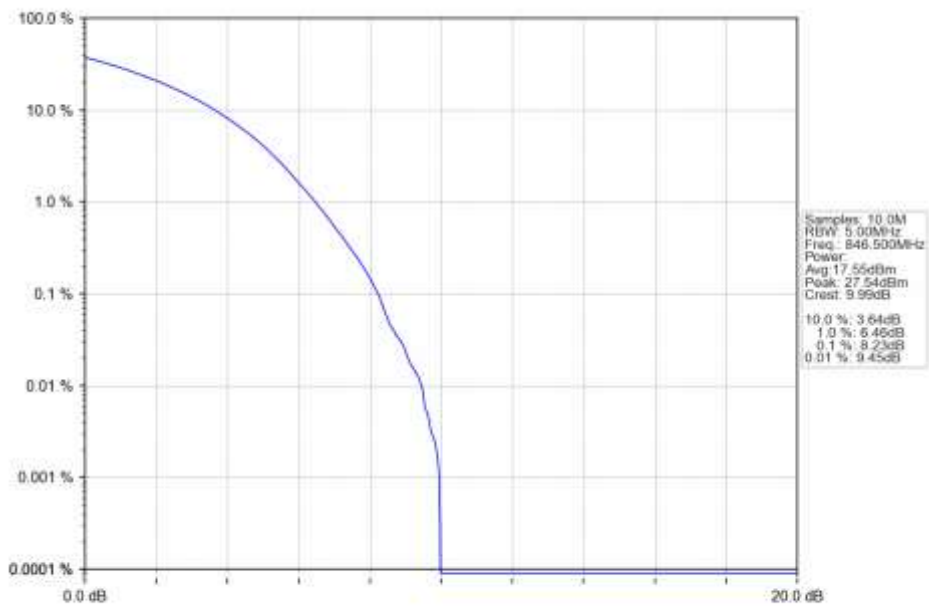
n5_15kHz_SISO_NTNV_5MHz_CP-OFDM_64_QAM_846.5MHz_Outer_Full_Ant1
