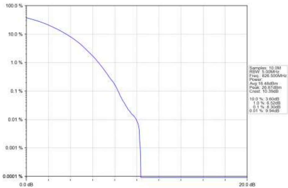
n5_15kHz_SISO_NTNV_5MHz_CP-OFDM_256_QAM_826.5MHz_Outer_Full_Ant1
