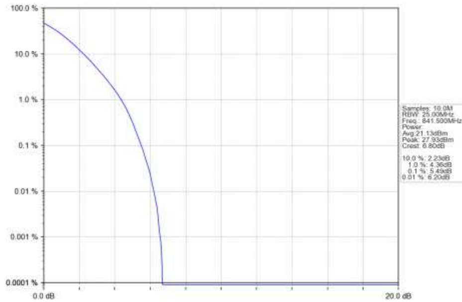
n5_15kHz_SISO_NTNV_15MHz_DFT-s-OFDM_QPSK_841.5MHz_Outer_Full_Ant1
