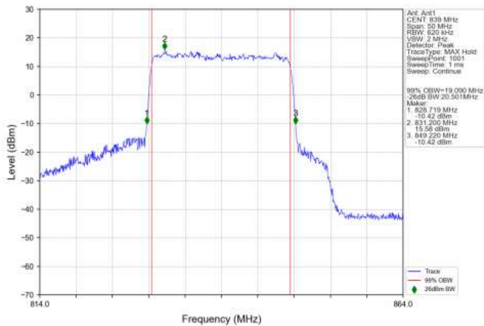
n5_15kHz_SISO_NTNV_20MHz_CP-OFDM_16_QAM_839MHz_Outer_Full_Ant1
