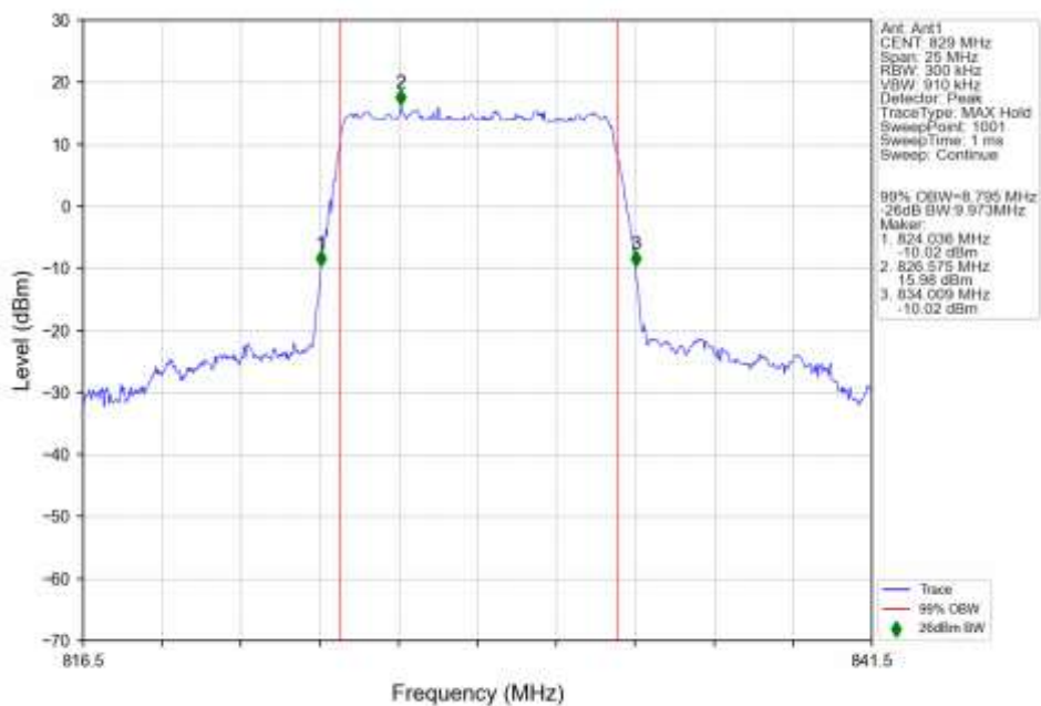
n5_30kHz_SISO_NTNV_10MHz_DFT-s-OFDM_16_QAM_829MHz_Outer_Full_Ant1
