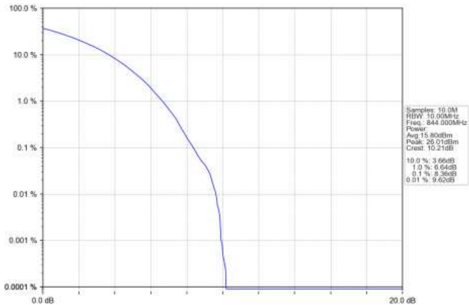
n5_15kHz_SISO_NTNV_10MHz_CP-OFDM_256_QAM_844MHz_Outer_Full_Ant1
