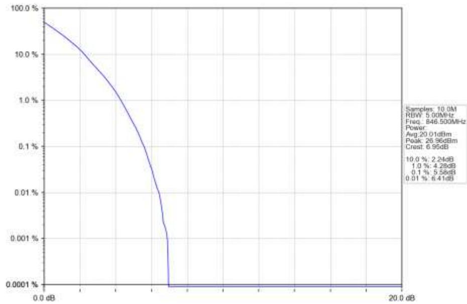
n5_15kHz_SISO_NTNV_5MHz_DFT-s-OFDM QPSK 846.5MHz_Outer_Full_Ant1
