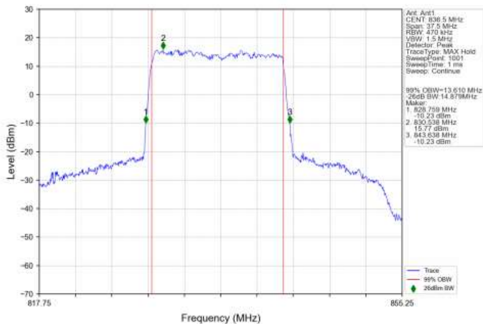
n5_15kHz_SISO_NTNV_15MHz_DFT-s-OFDM_64_QAM_836.5MHz_Outer_Full_Ant1
