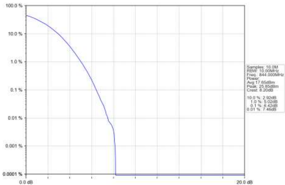
n5_15kHz_SISO_NTNV_10MHz_DFT-s-OFDM_256_QAM_844MHz_Outer_Full_Ant1
