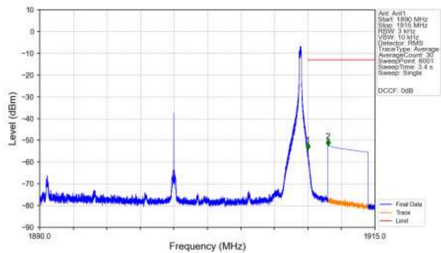
n2_15kHz_SISO_NTNV_20MHz_DFT-s-OFDM_QPSK_1900MHz_Edge_1RB_Right_Ant1
