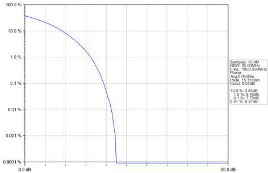
n2_30kHz_SISO_NTNV_15MHz_CP-OFDM QPSK_1902.5MHz_Outer_Full_Ant1
