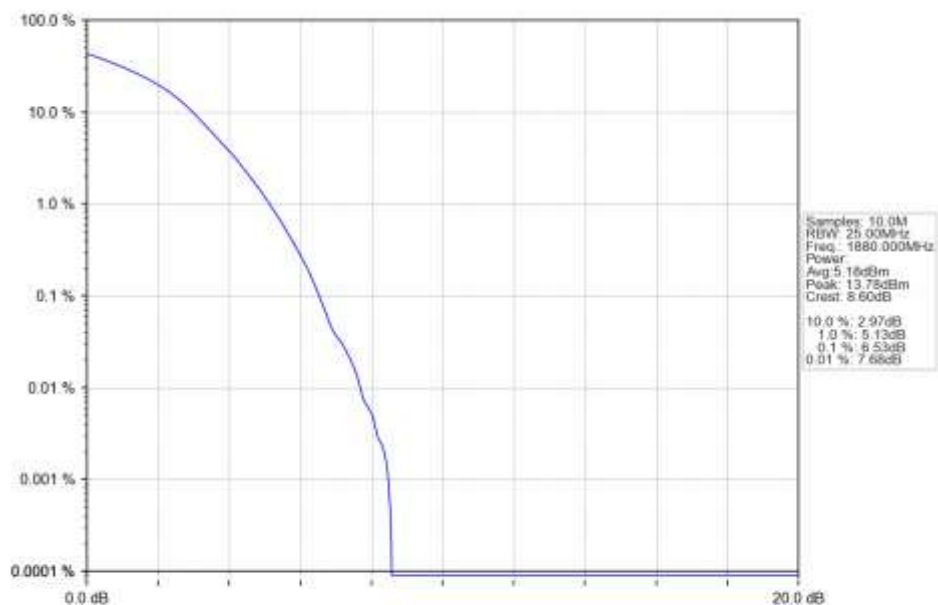
n2_30kHz_SISO_NTNV_20MHz_DFT-s-OFDM_256_QAM_1880MHz_Outer_Full_Ant1
