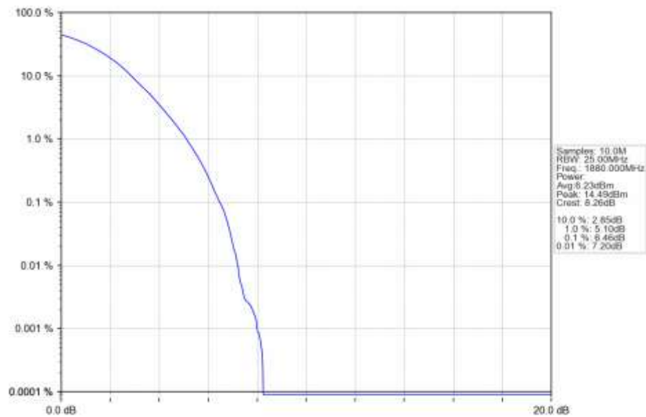
n2_30kHz_SISO_NTNV_15MHz_DFT-s-OFDM_64_QAM_1880MHz_Outer_Full_Ant1
