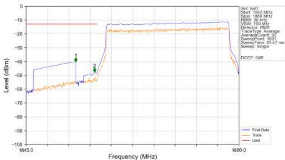
n2_30kHz_SISO_NTNV_10MHz_CP-OFDM_QPSK_1855MHz_Outer_Full_Ant1
