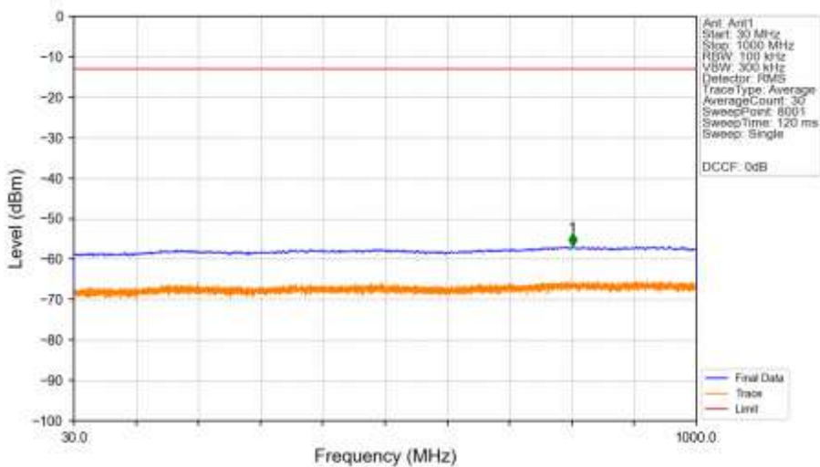
n2_15kHz_SISO_NTNV_15MHz_DFT-s-OFDM QPSK_1857.5MHz_Edge_1RB_Left_Ant1
