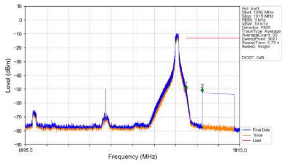
n2_30kHz_SISO_NTNV_15MHz_DFT-s-OFDM_QPSK_1902.5MHz_Edge_1RB_Right_Ant1
