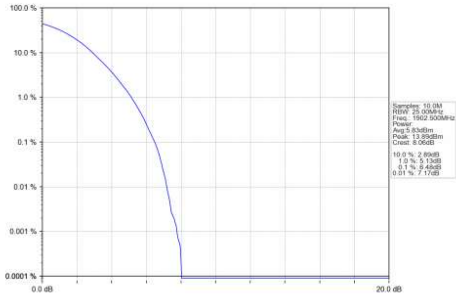
n2_30kHz_SISO_NTNV_15MHz_DFT-s-OFDM 64 QAM_1902.5MHz_Outer_Full_Ant1
