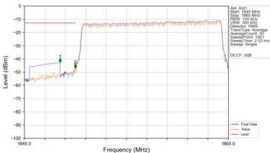
n2_30kHz_SISO_NTNV_15MHz_CP-OFDM_QPSK_1857.5MHz_Outer_Full_Ant1
