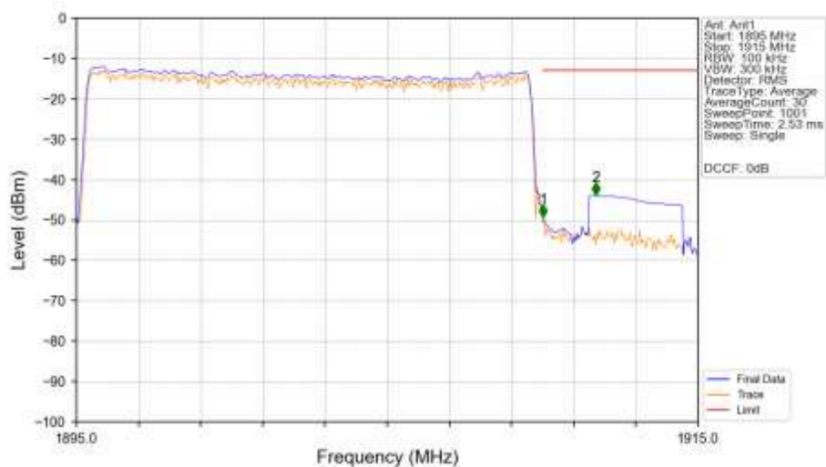
n2_15kHz_SISO_NTNV_15MHz_CP-OFDM_QPSK_1902.5MHz_Outer_Full_Ant1
