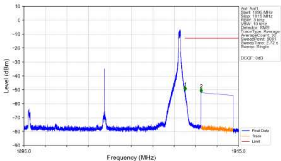
n2_15kHz_SISO_NTNV_15MHz_DFT-s-OFDM_QPSK_1902.5MHz_Edge_1RB_Right_Ant1
