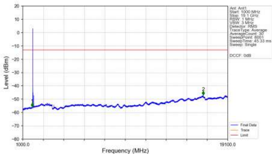
n2_30kHz_SISO_NTNV_15MHz_CP-OFDM_QPSK_1880MHz_Edge_1RB_Left_Ant1
