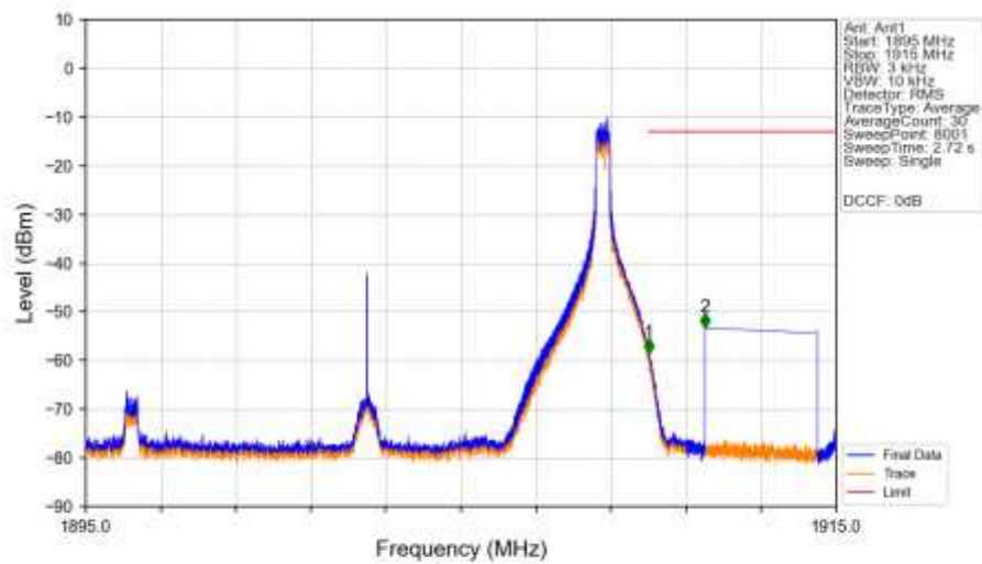
n2_30kHz_SISO_NTNV_15MHz_CP-OFDM_QPSK_1902.5MHz_Inner_1RB_Right_Ant1
