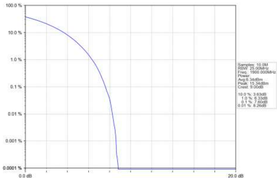
n2_30kHz_SISO_NTNV_20MHz_CP-OFDM QPSK_1900MHz_Outer_Full_Ant1
