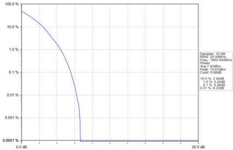
n2_30kHz_SISO_NTNV_15MHz_DFT-s-OFDM_QPSK_1902.5MHz_Outer_Full_Ant1
