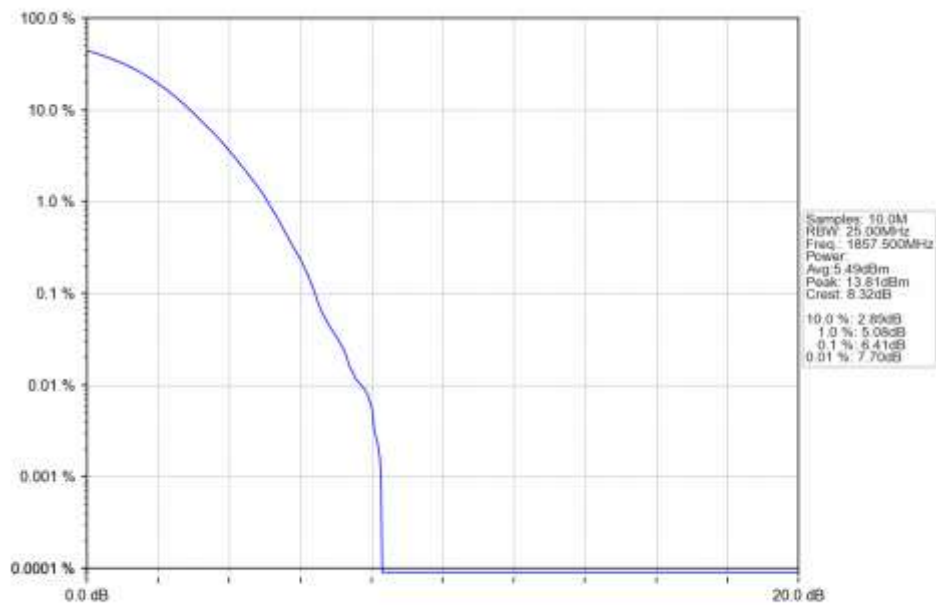
n2_30kHz_SISO_NTNV_15MHz_DFT-s-OFDM 256 QAM_1857.5MHz_Outer_Full_Ant1
