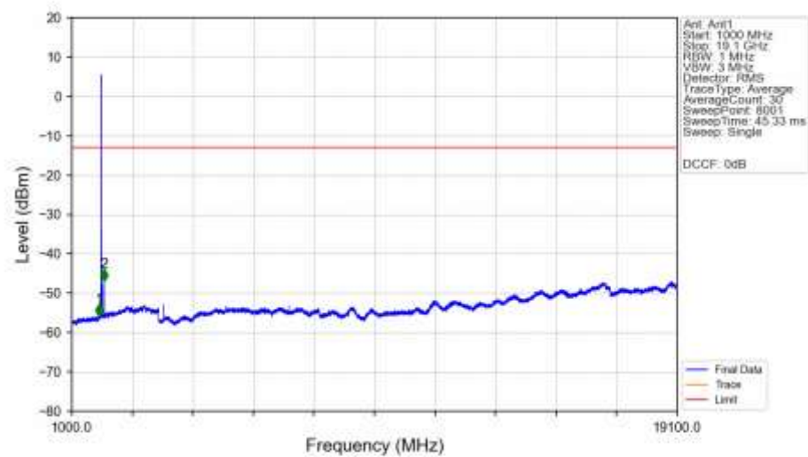
n2_30kHz_SISO_NTNV_15MHz_DFT-s-OFDM_QPSK_1880MHz_Edge_1RB_Left_Ant1
