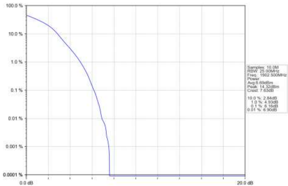
n2_30kHz_SISO_NTNV_15MHz_DFT-s-OFDM_16_QAM_1902.5MHz_Outer_Full_Ant1
