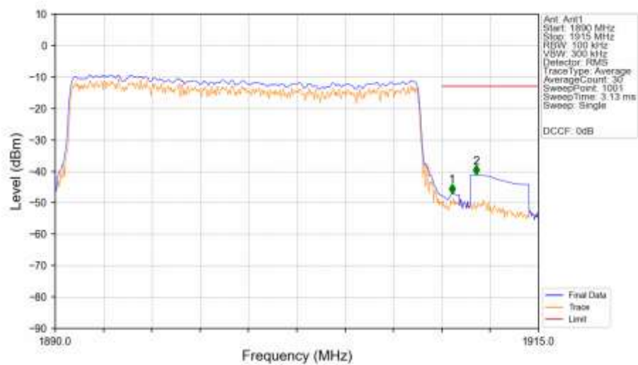
n2_30kHz_SISO_NTNV_20MHz_DFT-s-OFDM_QPSK_1900MHz_Outer_Full_Ant1
