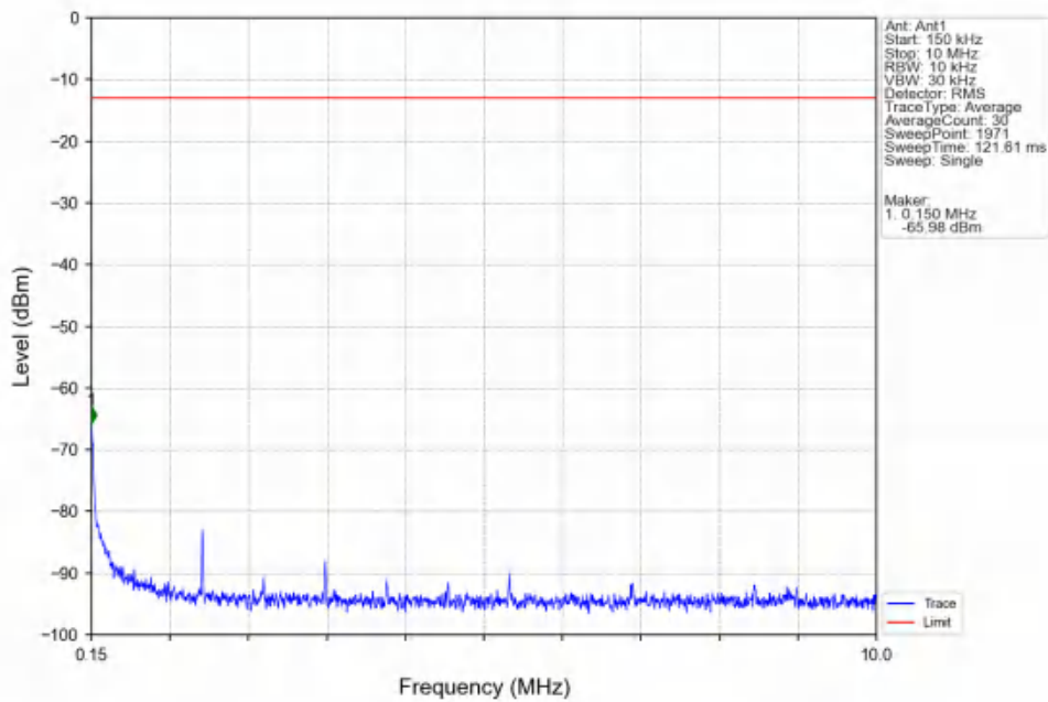
Band25_20MHz_16QAM_MCH_1882.5MHz_RB_1_0_NTNV
