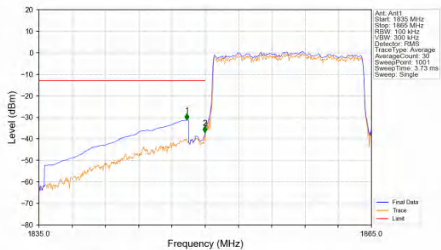
Band25_15MHz_QPSK_LCH_1857.5MHz_RB_75_0_NTNV
