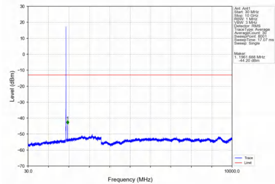
Band25_5MHz_16QAM_MCH_1882.5MHz_RB_1_0_NTNV
