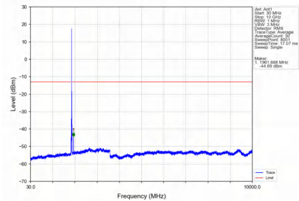
Band25_15MHz_16QAM_MCH_1882.5MHz_RB_1_0_NTNV
