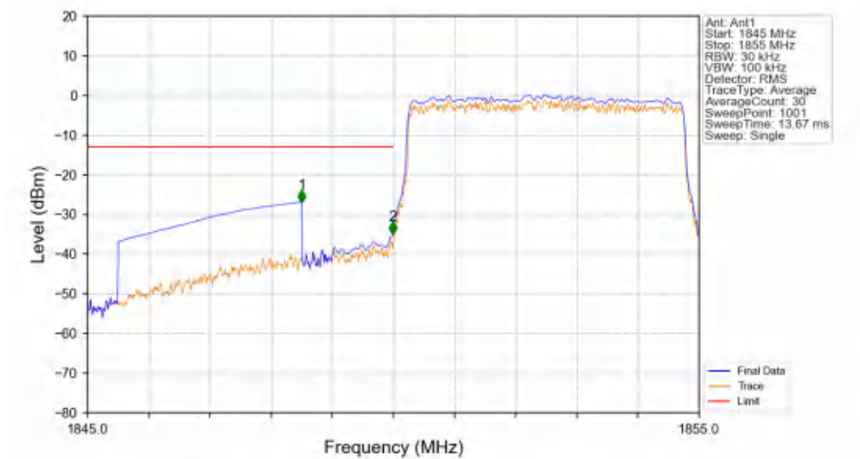
Band25_5MHz_16QAM_LCH_1852.5MHz_RB_25_0_NTNV
