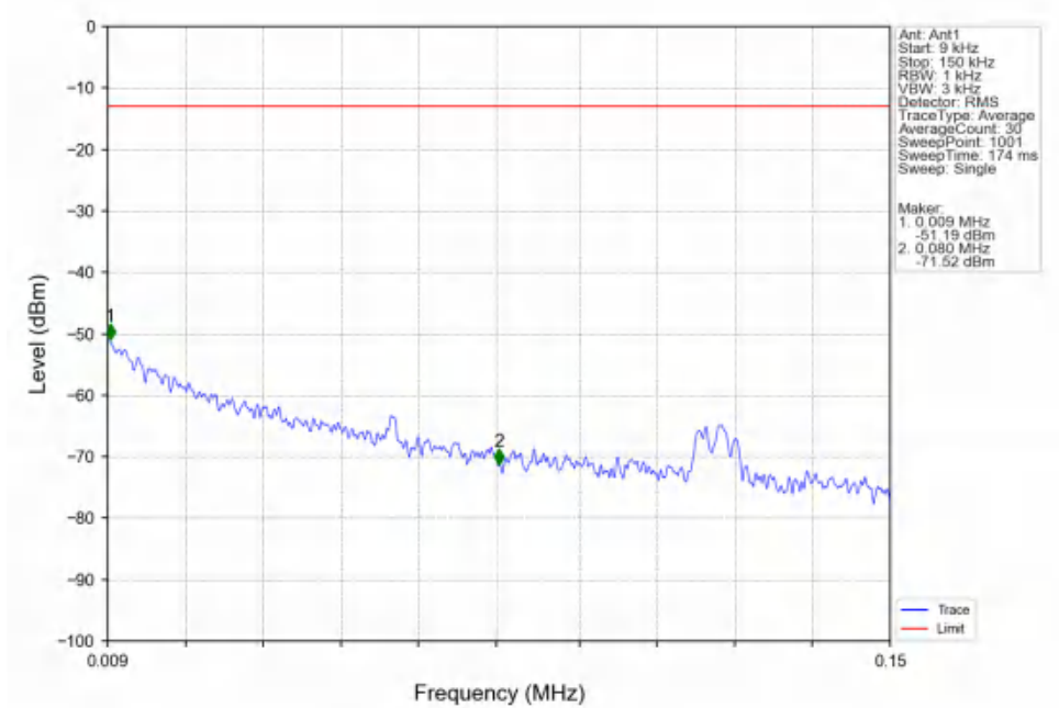
Band25_5MHz_QPSK_HCH_1912.5MHz_RB_1_0_NTNV
