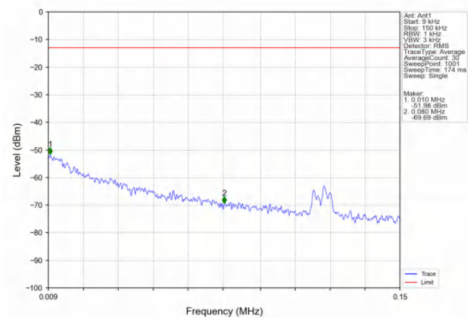
Band25_15MHz_16QAM_MCH_1882.5MHz_RB_1_0_NTNV
