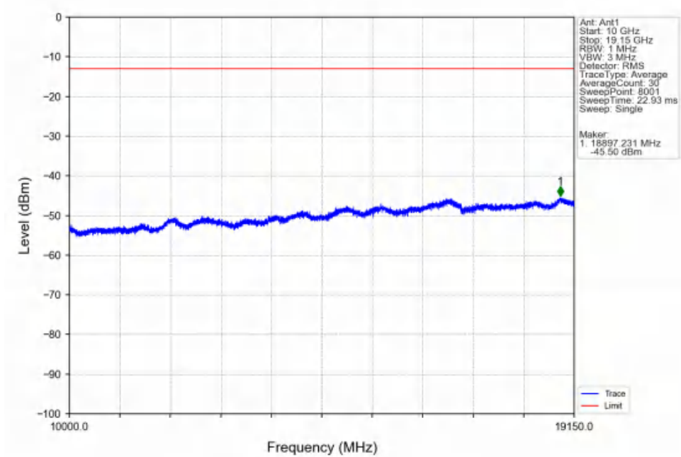
Band25_5MHz_16QAM_HCH_1912.5MHz_RB_1_0_NTNV
