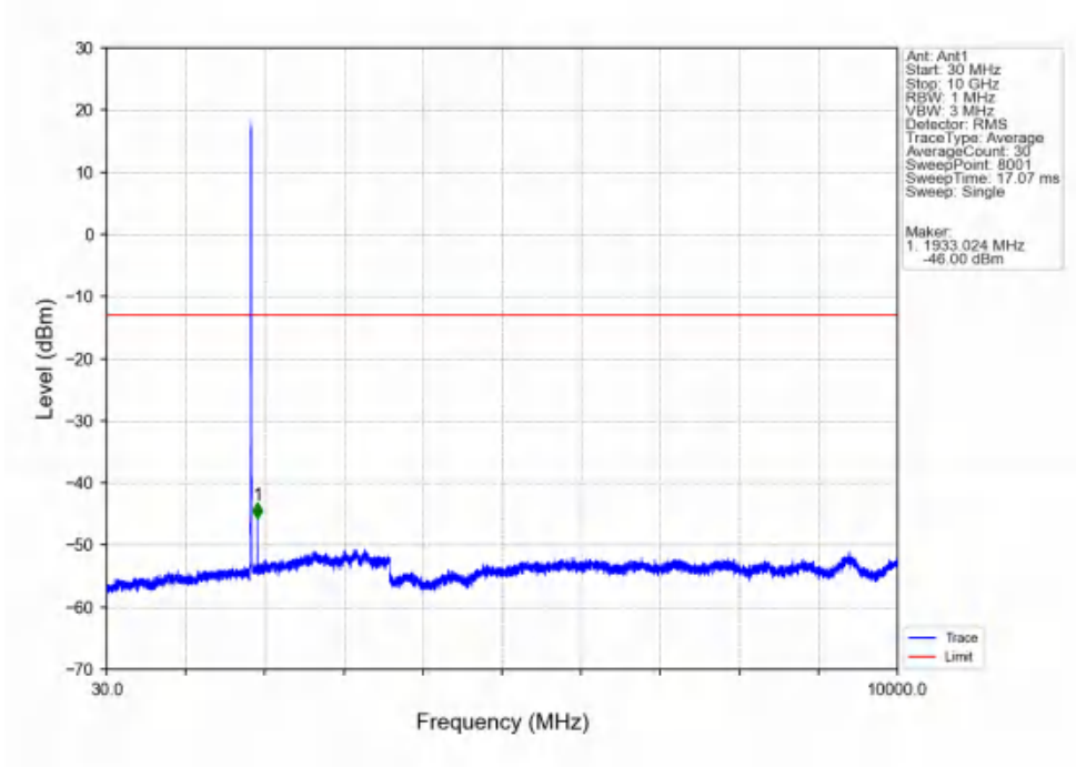
Band25_5MHz_QPSK_LCH_1852.5MHz_RB_1_0_NTNV
