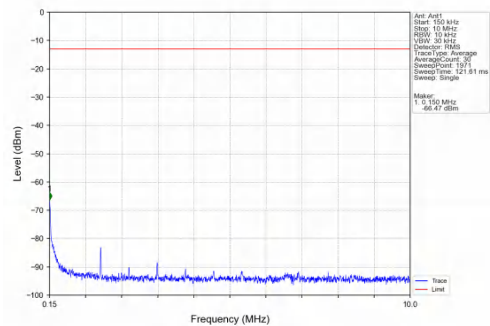
Band25_15MHz_QPSK_MCH_1882.5MHz_RB_1_0_NTNV
