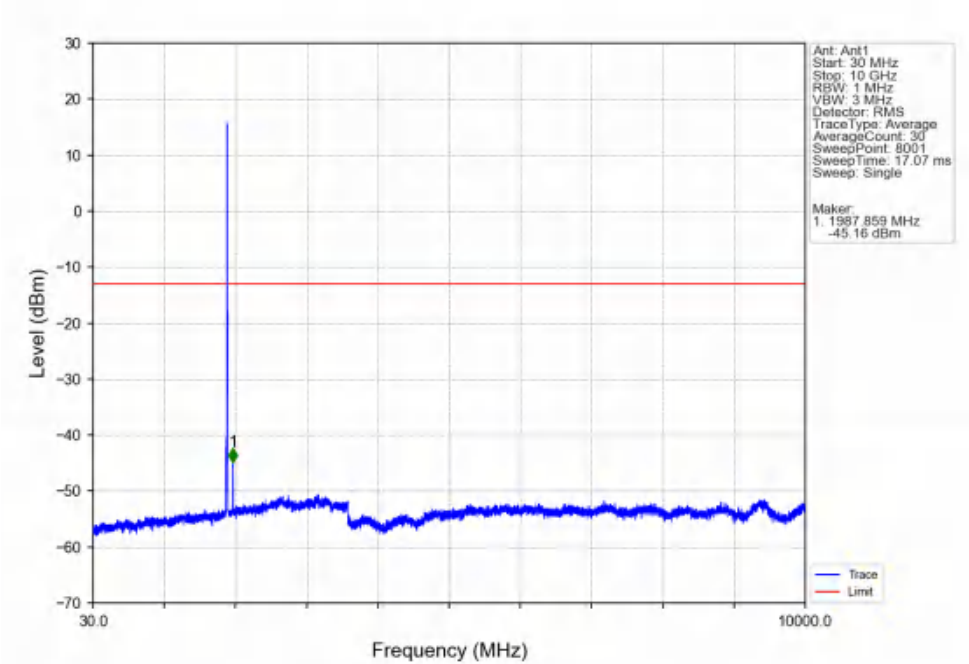
Band25_10MHz_16QAM_HCH_1910MHz_RB_1_0_NTNV
