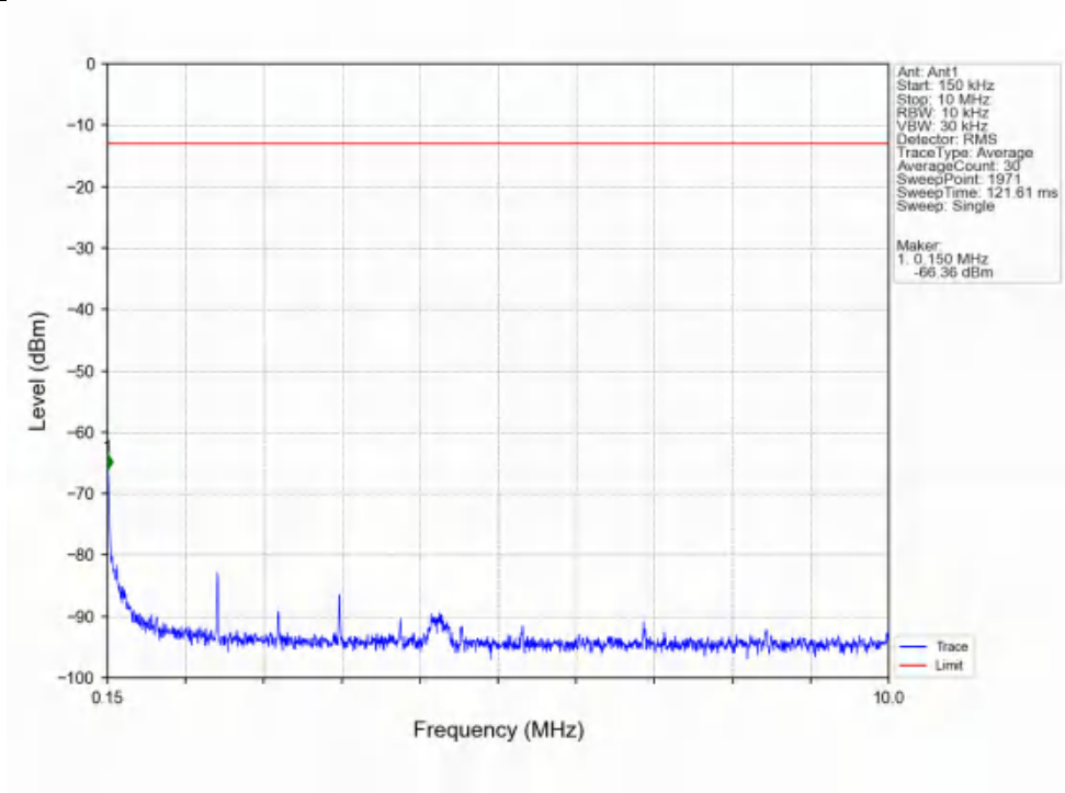
Band25_5MHz_16QAM_HCH_1912.5MHz_RB_1_0_NTNV
