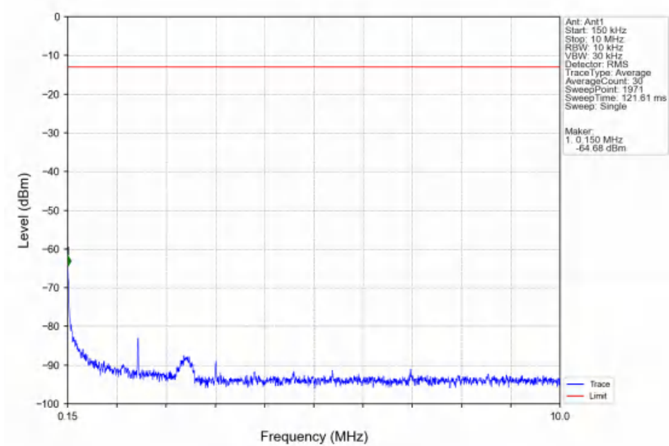
Band25_3MHz_16QAM_HCH_1913.5MHz_RB_1_0_NTNV
