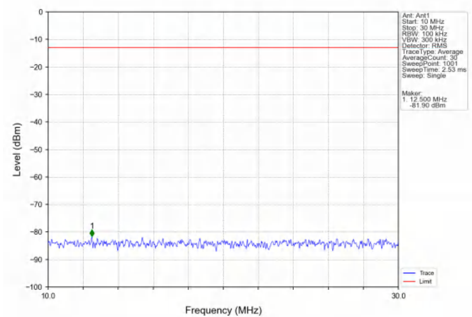
Band25_5MHz_16QAM_LCH_1852.5MHz_RB_1_0_NTNV
