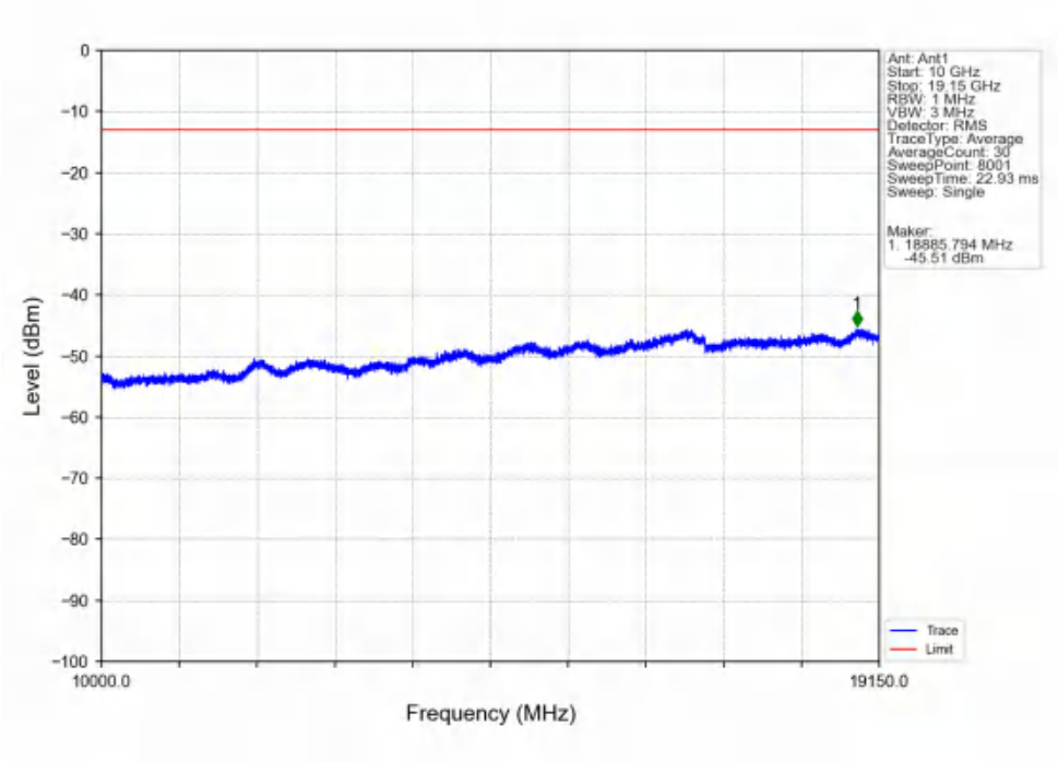
Band25_3MHz_16QAM_HCH_1913.5MHz_RB_1_0_NTNV
