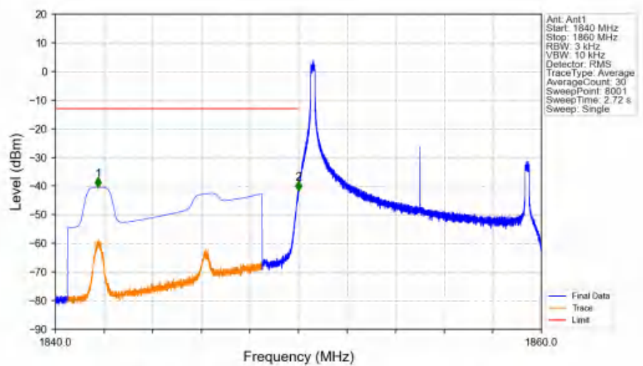
Band25_10MHz_16QAM_LCH_1855MHz_RB_1_0_NTNV
