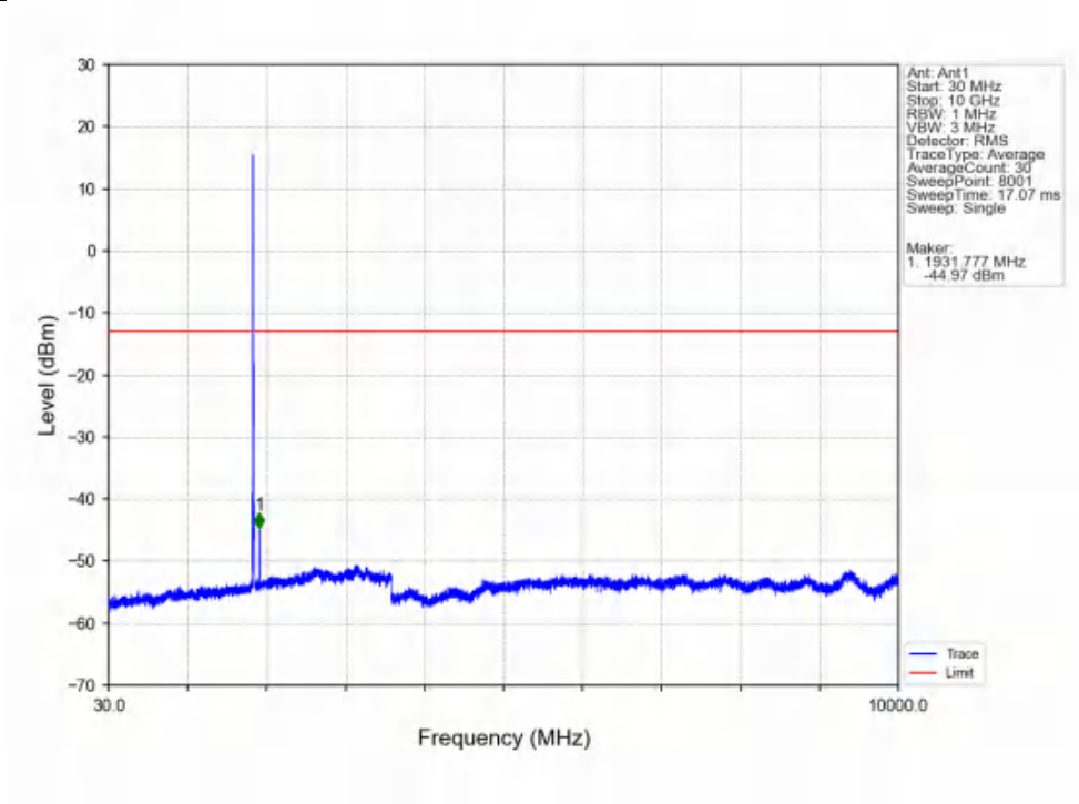
Band25_10MHz_16QAM_LCH_1855MHz_RB_1_0_NTNV
