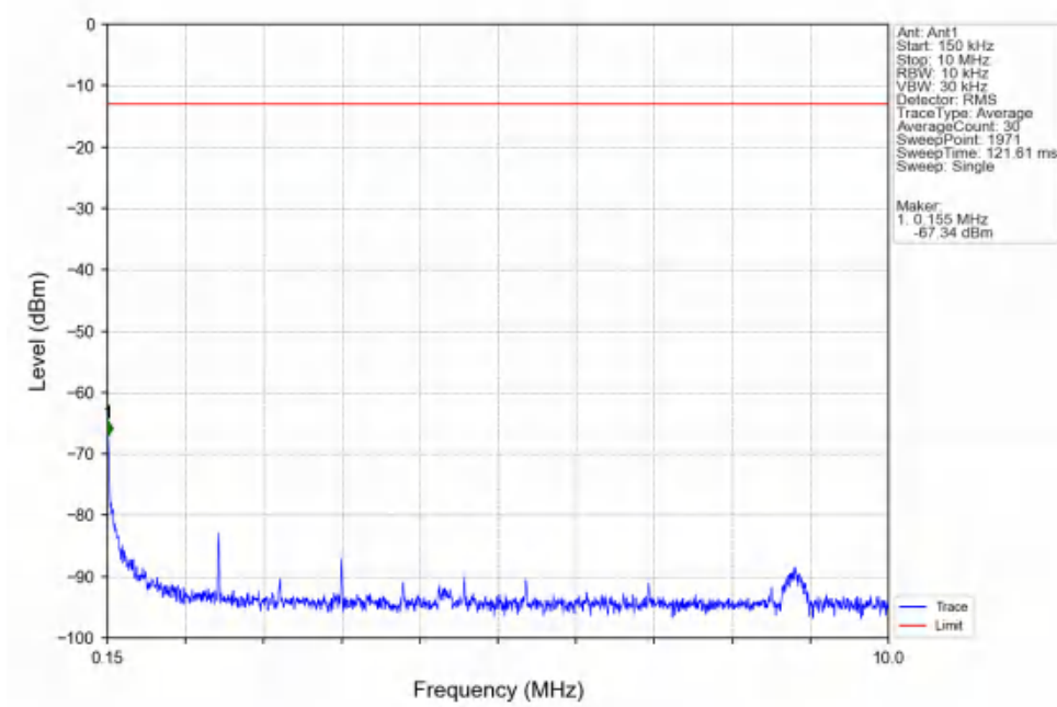
Band25_10MHz_16QAM_LCH_1855MHz_RB_1_0_NTNV
