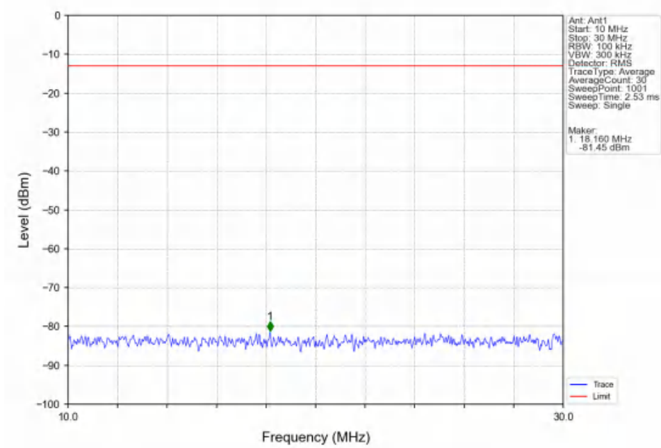
Band25_3MHz_16QAM_HCH_1913.5MHz_RB_1_0_NTNV
