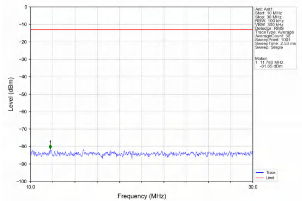
Band25_10MHz_16QAM_HCH_1910MHz_RB_1_0_NTNV
