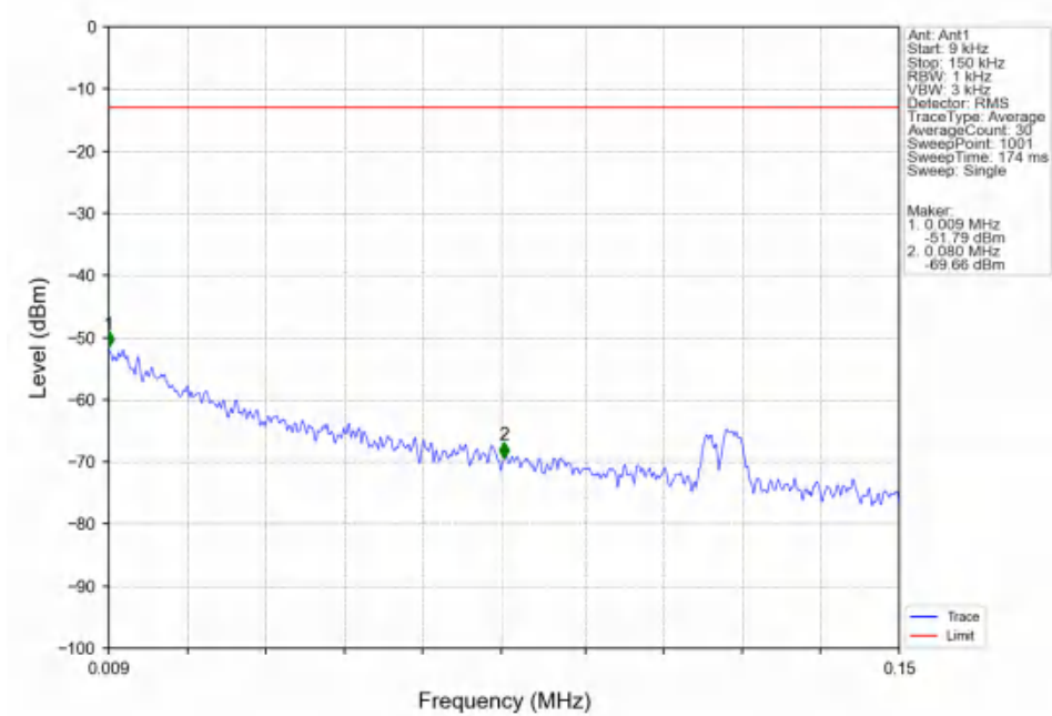
Band25_20MHz_16QAM_LCH_1860MHz_RB_1_0_NTNV
