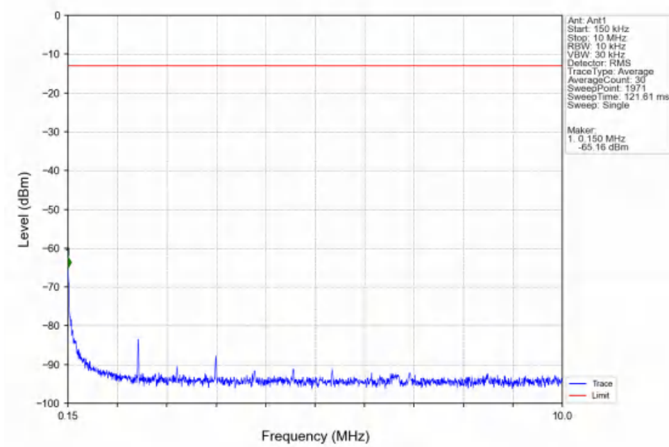
Band25_15MHz_16QAM_MCH_1882.5MHz_RB_1_0_NTNV
