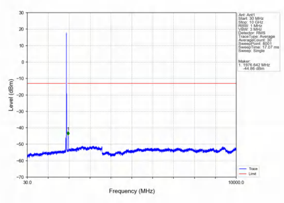
Band25_20MHz_16QAM_HCH_1905MHz_RB_1_0_NTNV
