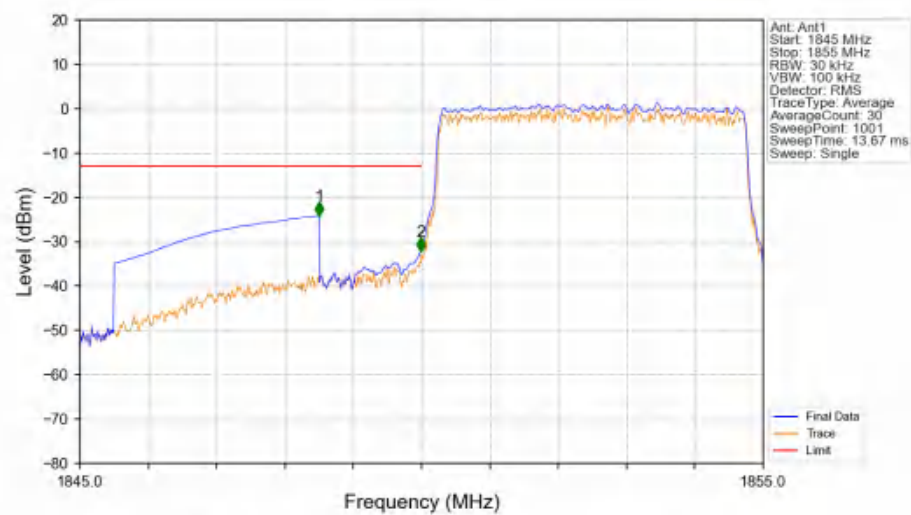
Band25_5MHz_QPSK_LCH_1852.5MHz_RB_25_0_NTNV
