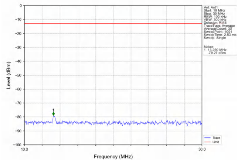
Band25_15MHz_QPSK_MCH_1882.5MHz_RB_1_0_NTNV
