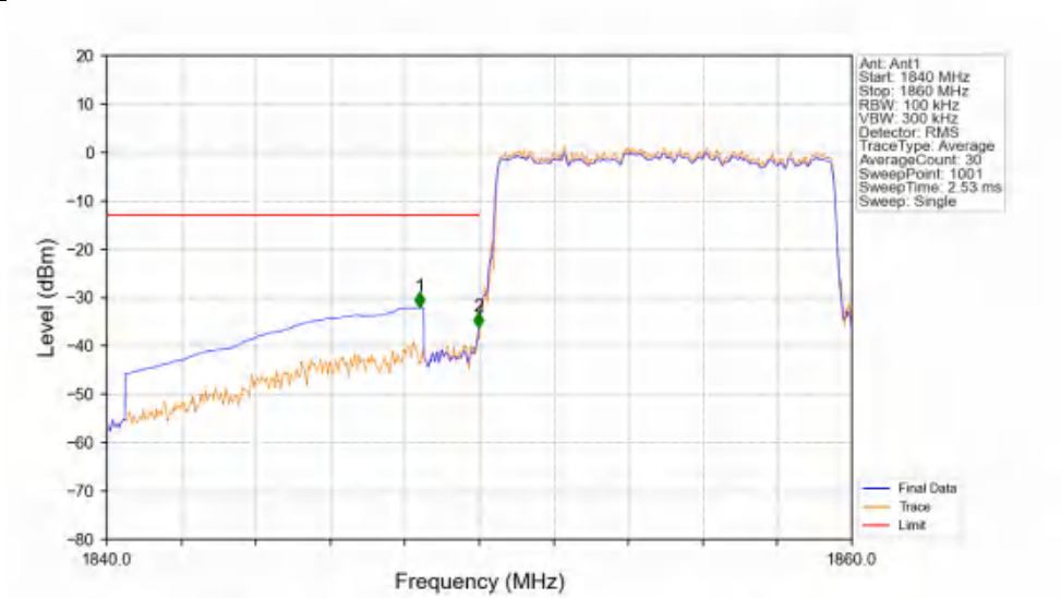
Band25_10MHz_16QAM_LCH_1855MHz_RB_50_0_NTNV
