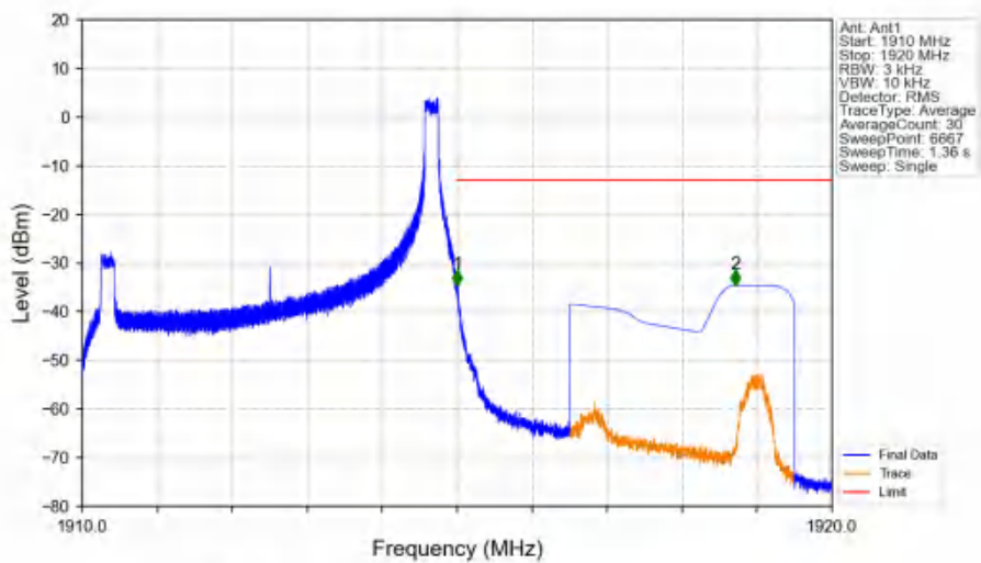
Band25_5MHz_QPSK_HCH_1912.5MHz_RB_1_24_NTNV
