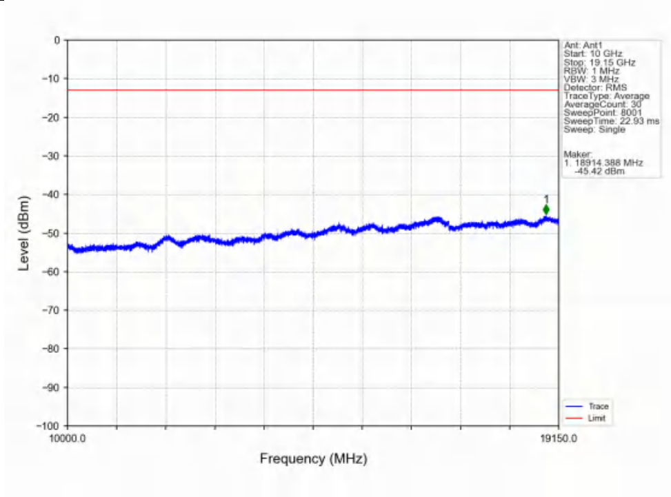
Band25_10MHz_16QAM_LCH_1855MHz_RB_50_0_NTNV
