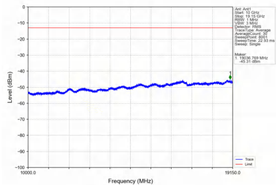
Band25_5MHz_16QAM_LCH_1852.5MHz_RB_25_0_NTNV
