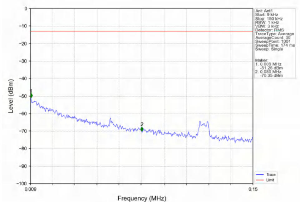
Band25_5MHz_16QAM_HCH_1912.5MHz_RB_1_0_NTNV
