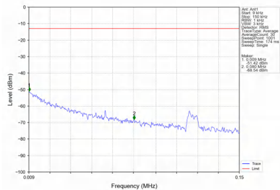
Band25_10MHz_16QAM_LCH_1855MHz_RB_1_0_NTNV
