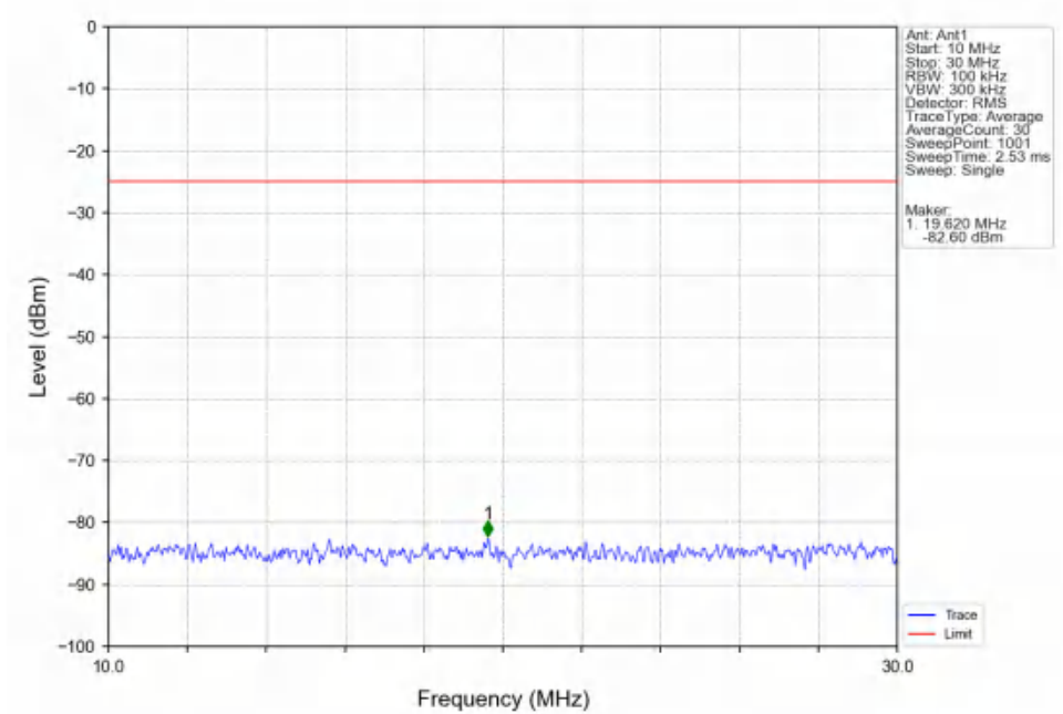
Band7_15MHz_QPSK_MCH_2535MHz_RB_1_0_NTNV
