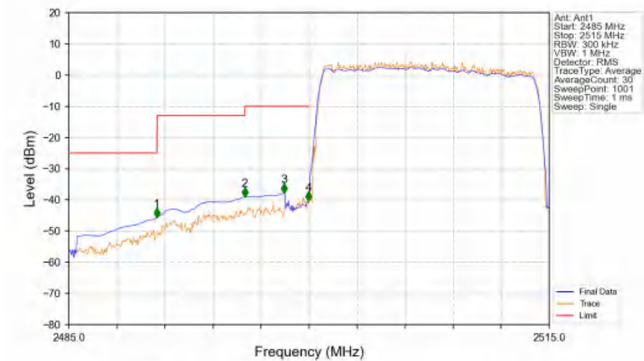
Band7_15MHz_QPSK_LCH_2507.5MHz_RB_75_0_NTNV
