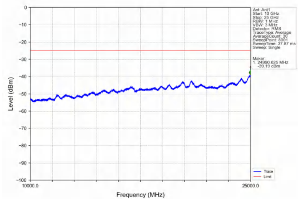
Band7_15MHz_16QAM_MCH_2535MHz_RB_1_0_NTNV
