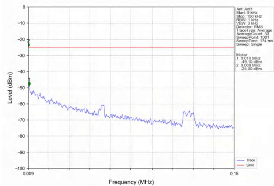
Band7_15MHz_16QAM_HCH_2562.5MHz_RB_1_0_NTNV
