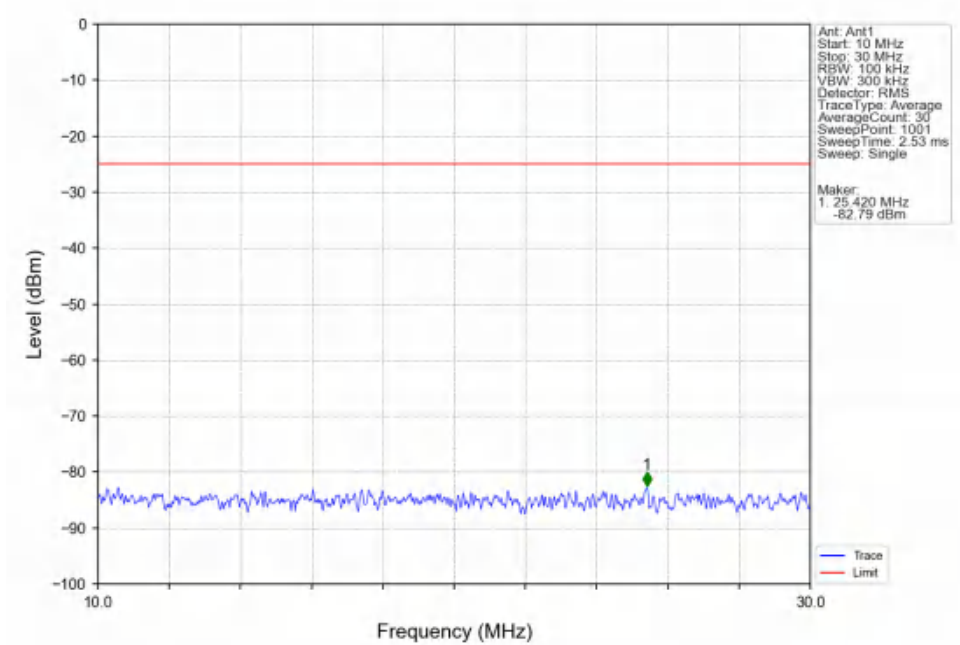
Band7_10MHz_16QAM_MCH_2535MHz_RB_1_0_NTNV
