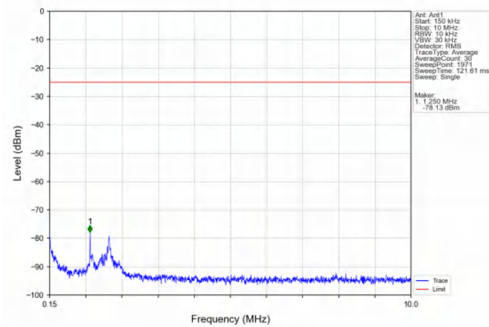
Band7_15MHz_16QAM_HCH_2562.5MHz_RB_1_0_NTNV
