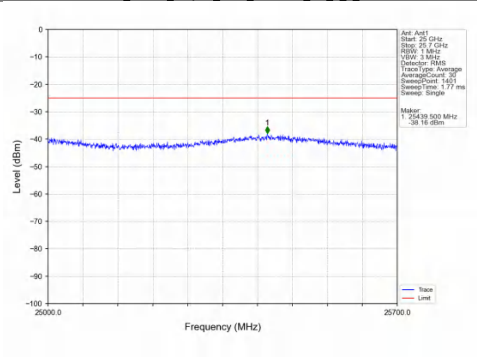
Band7_10MHz_16QAM_MCH_2535MHz_RB_1_0_NTNV
