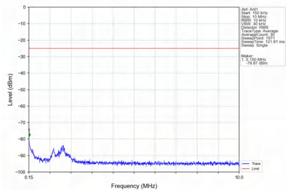
Band7_15MHz_QPSK_LCH_2507.5MHz_RB_1_0_NTNV
