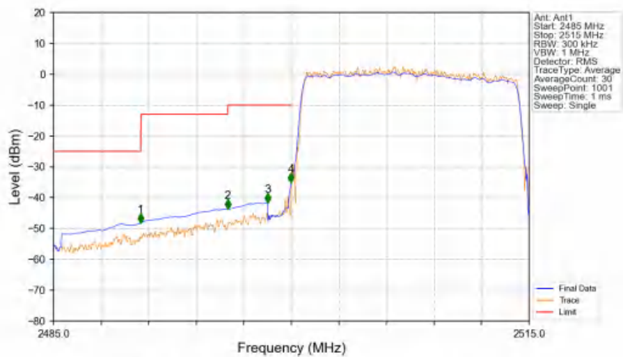
Band7_15MHz_16QAM_LCH_2507.5MHz_RB_75_0_NTNV
