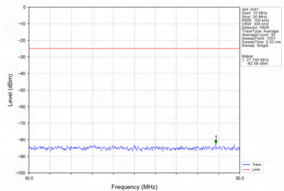
Band7_15MHz_16QAM_MCH_2535MHz_RB_1_0_NTNV
