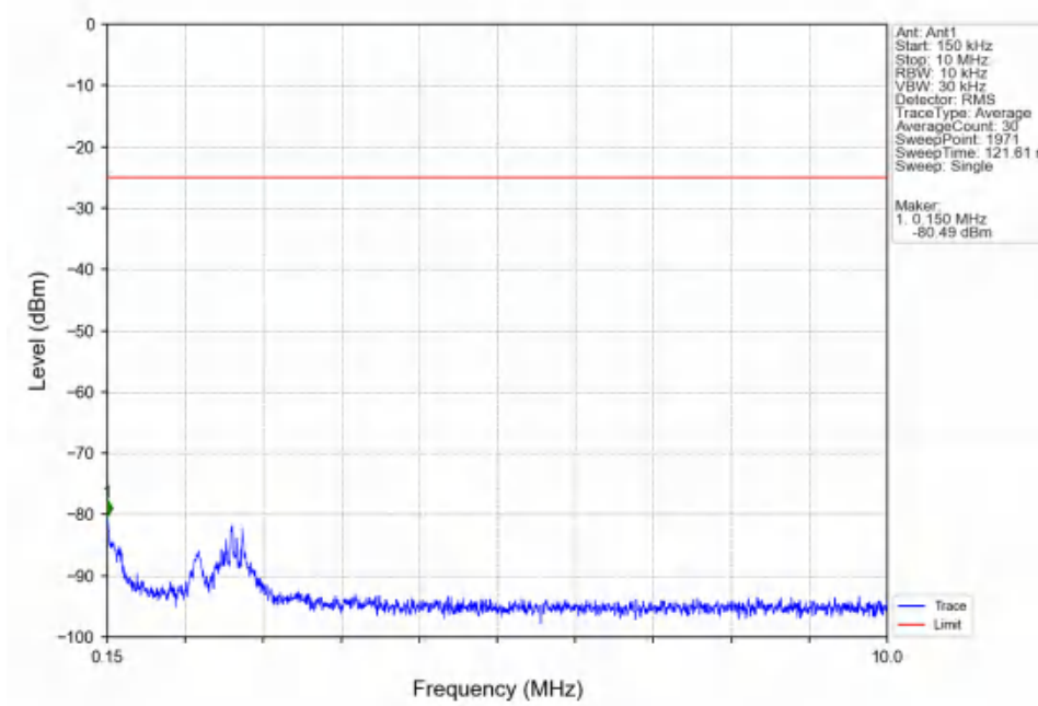
Band7_15MHz_16QAM_MCH_2535MHz_RB_1_0_NTNV
