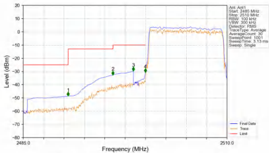
Band7_10MHz_16QAM_LCH_2505MHz_RB_50_0_NTNV
