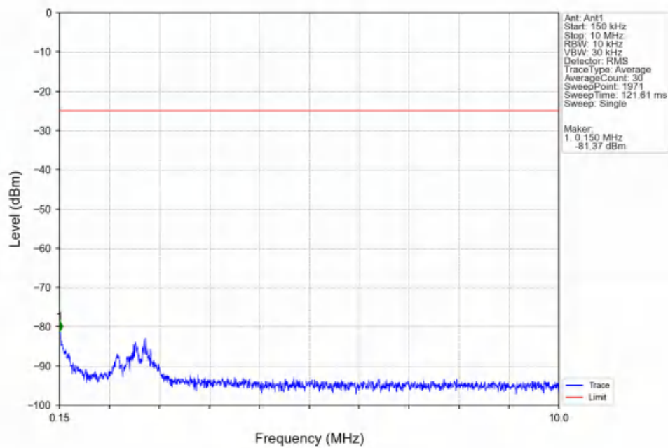
Band7_15MHz_QPSK_MCH_2535MHz_RB_1_0_NTNV
