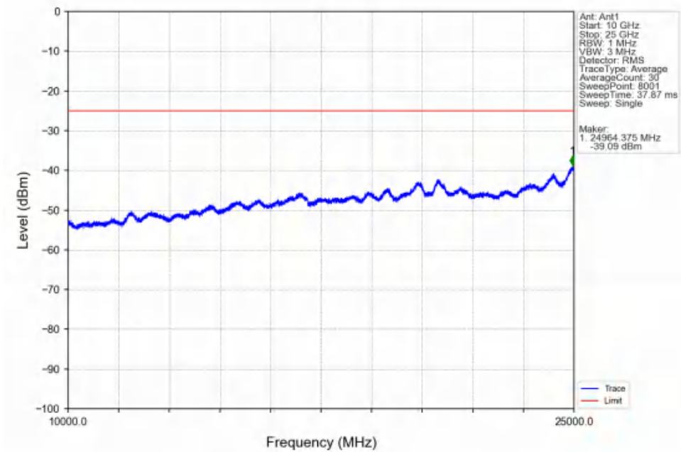
Band7_10MHz_16QAM_HCH_2565MHz_RB_1_0_NTNV
