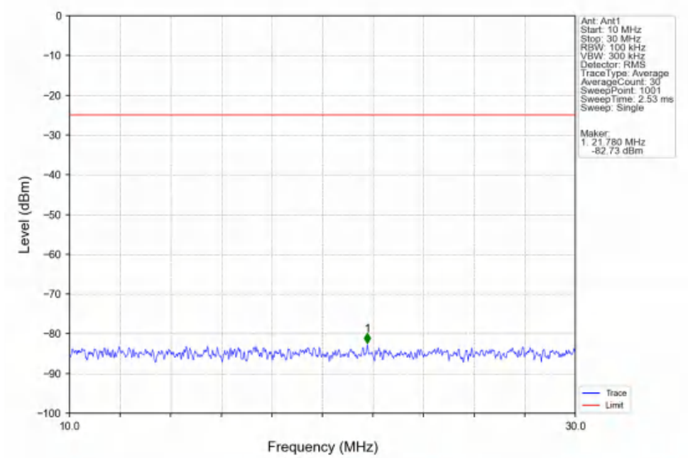
Band7_15MHz_16QAM_LCH_2507.5MHz_RB_1_0_NTNV
