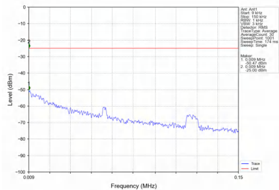
Band7_10MHz_16QAM_MCH_2535MHz_RB_1_0_NTNV
