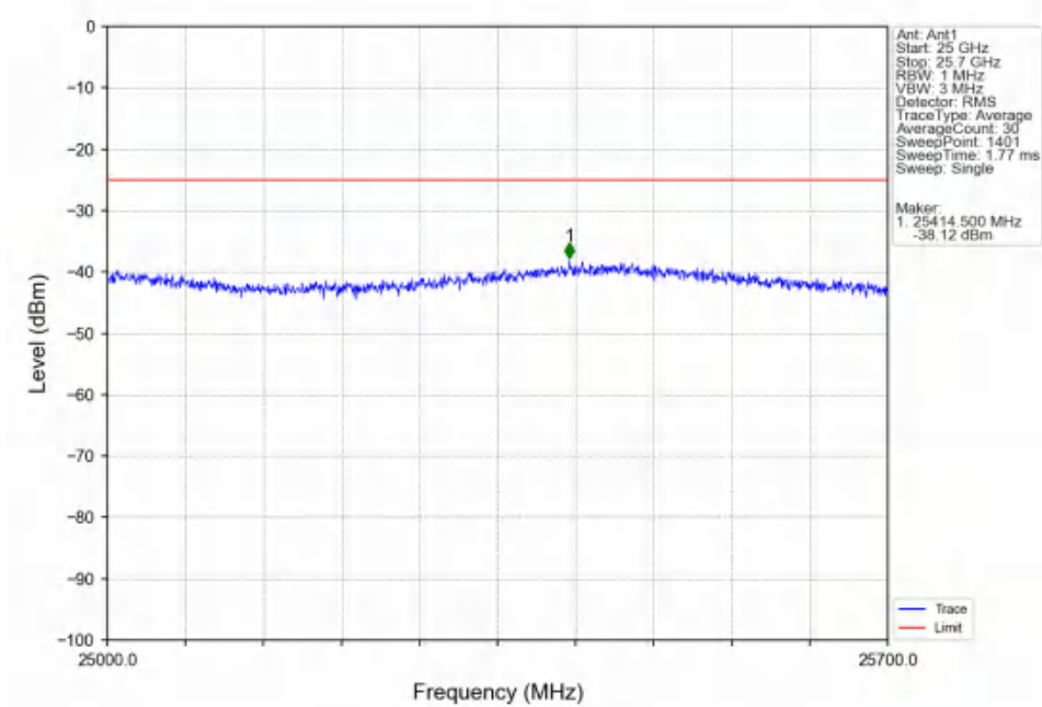
Band7_15MHz_QPSK_LCH_2507.5MHz_RB_75_0_NTNV
