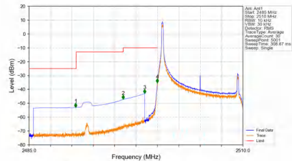
Band7_10MHz_16QAM_LCH_2505MHz_RB_1_0_NTNV
