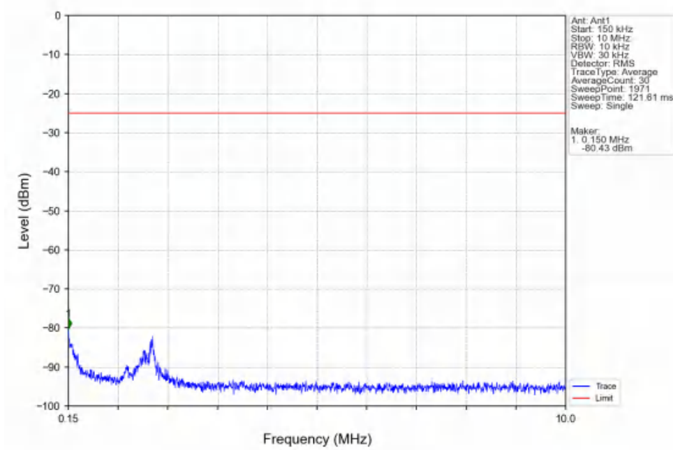
Band7_10MHz_16QAM_MCH_2535MHz_RB_1_0_NTNV
