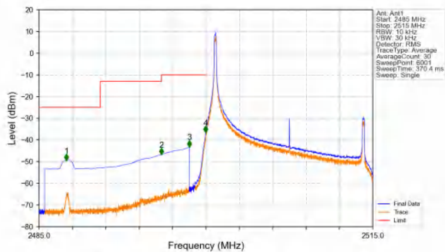
Band7_15MHz_16QAM_LCH_2507.5MHz_RB_1_0_NTNV
