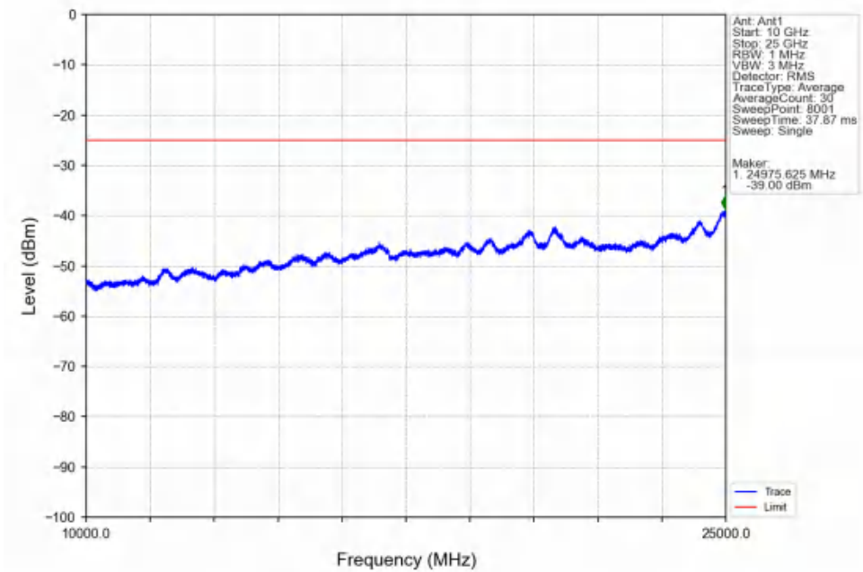
Band7_15MHz_16QAM_HCH_2562.5MHz_RB_1_0_NTNV
