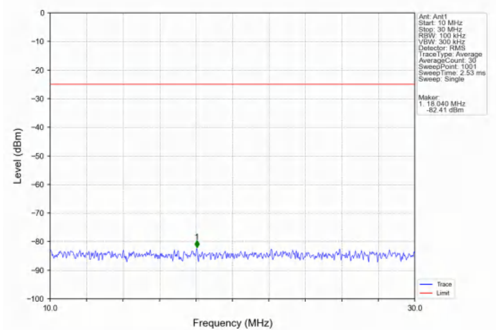
Band7_15MHz_QPSK_LCH_2507.5MHz_RB_1_0_NTNV
