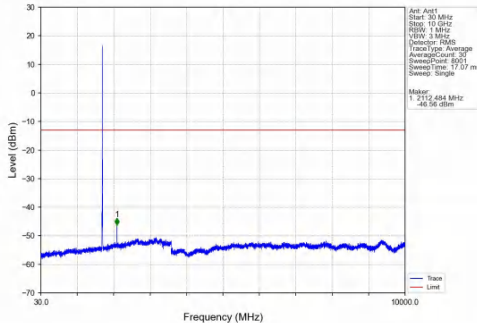
Band4_5MHz_16QAM_LCH_1712.5MHz_RB_1_0_NTNV
