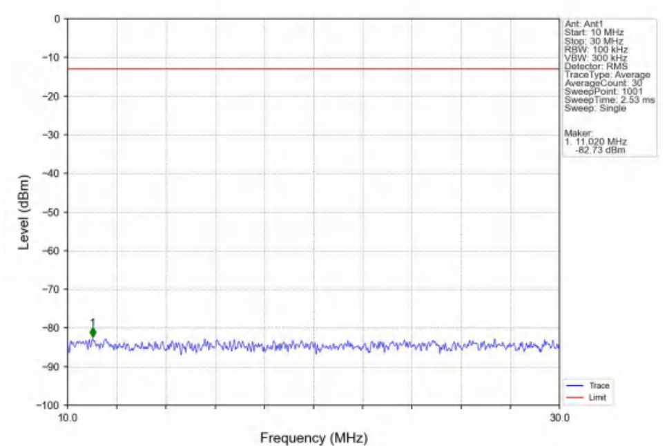
Band4_10MHz_QPSK_MCH_1732.5MHz_RB_1_0_NTNV
