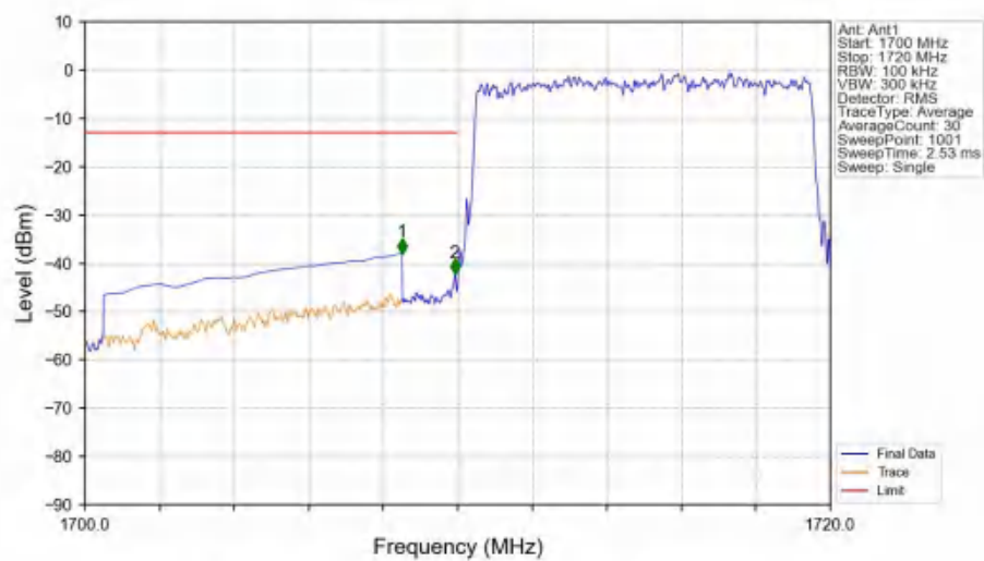
Band4_10MHz_16QAM_LCH_1715MHz_RB_50_0_NTNV
