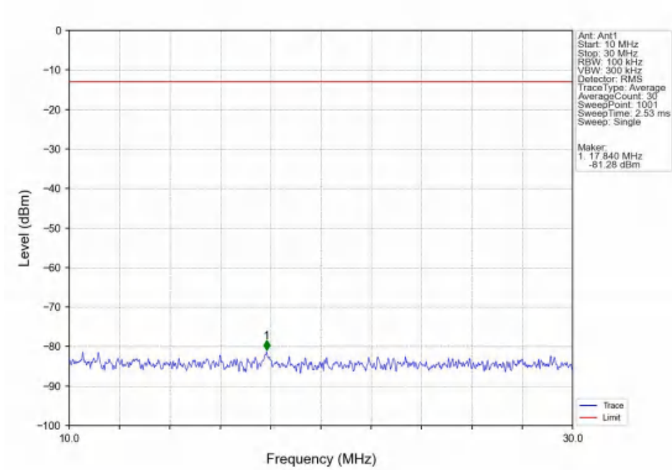
Band4_20MHz_16QAM_HCH_1745MHz_RB_1_0_NTNV
