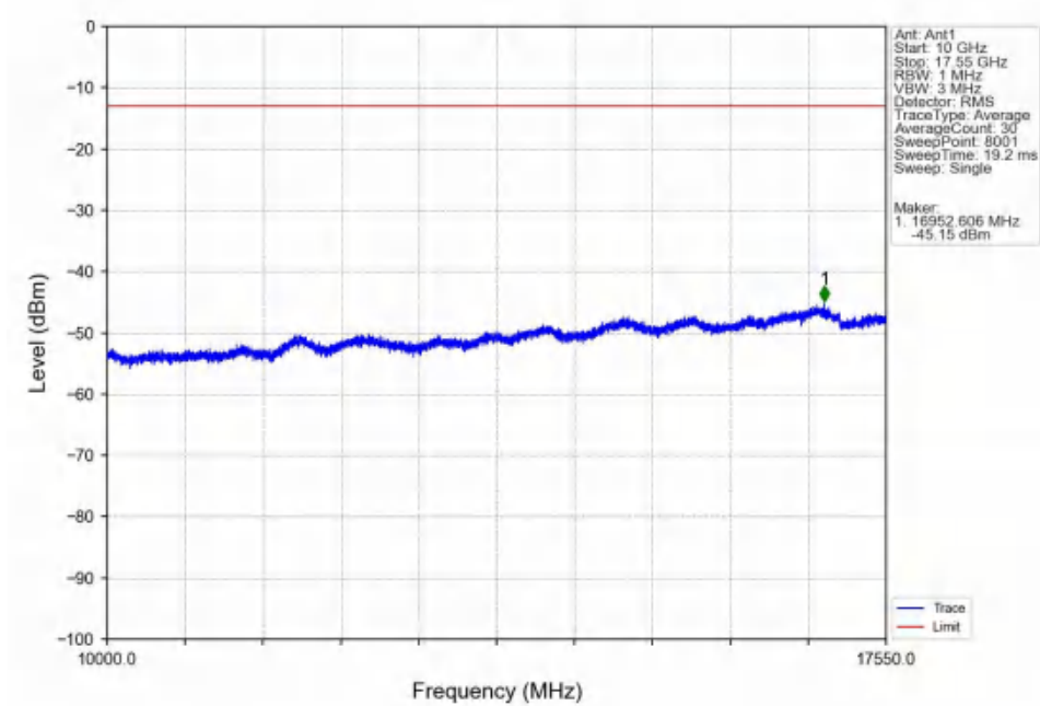
Band4_5MHz_16QAM_LCH_1712.5MHz_RB_25_0_NTNV
