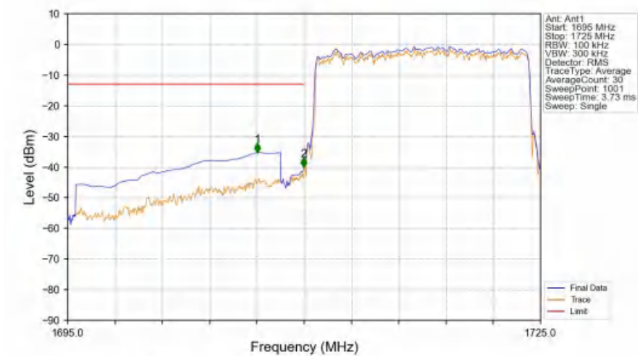
Band4_15MHz_16QAM_LCH_1717.5MHz_RB_75_0_NTNV
