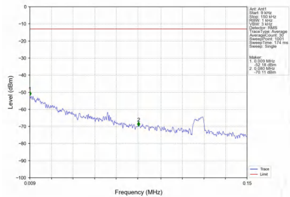
Band4_20MHz_16QAM_HCH_1745MHz_RB_1_0_NTNV
