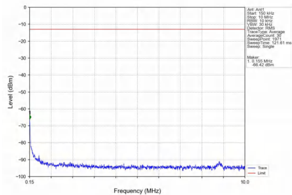
Band4_10MHz_QPSK_MCH_1732.5MHz_RB_1_0_NTNV
