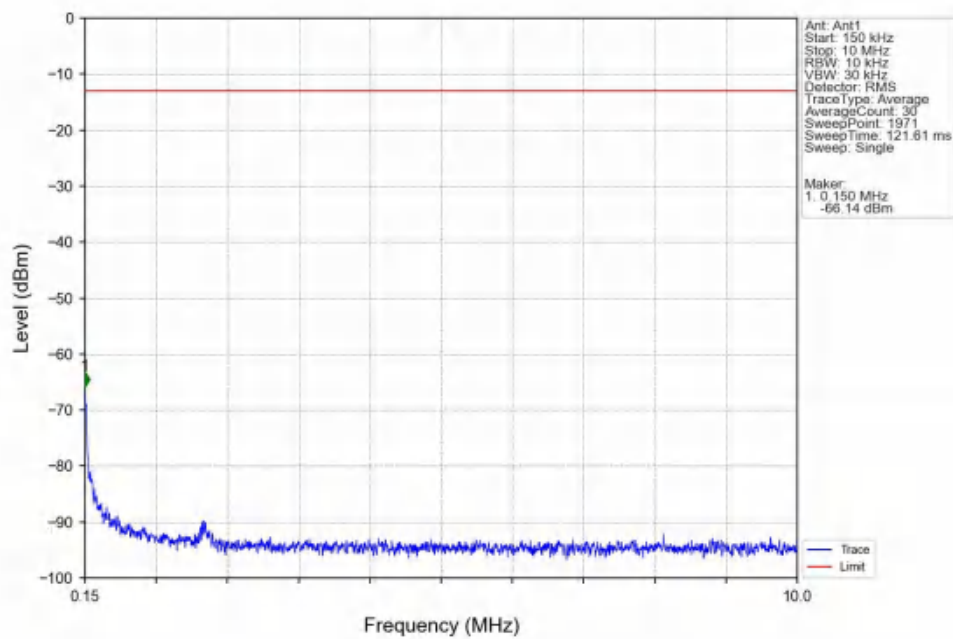
Band4_20MHz_16QAM_MCH_1732.5MHz_RB_1_0_NTNV
