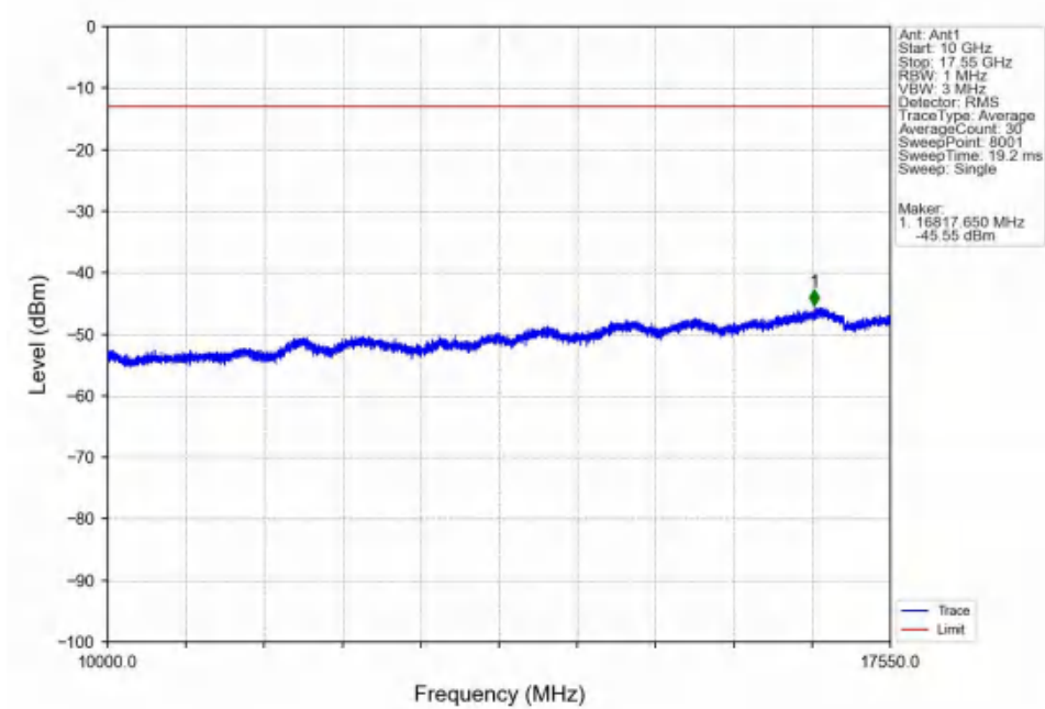
Band4_5MHz_16QAM_HCH_1752.5MHz_RB_1_0_NTNV
