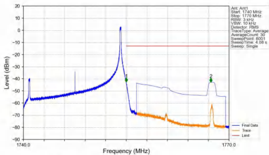
Band4_15MHz_16QAM_HCH_1747.5MHz_RB_1_74_NTNV
