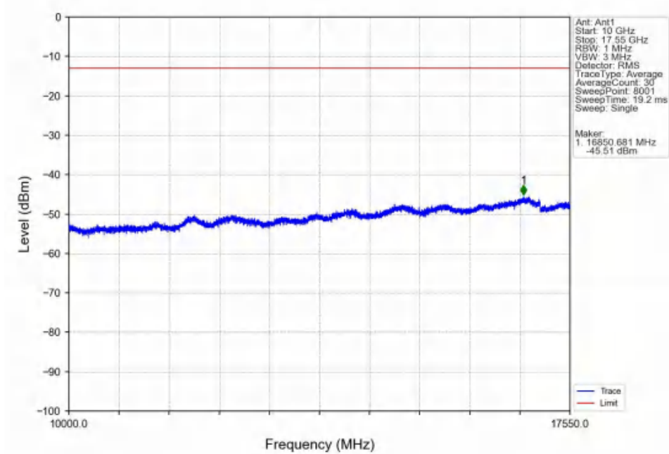
Band4_15MHz_16QAM_LCH_1717.5MHz_RB_75_0_NTNV
