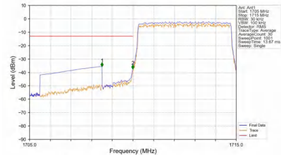
Band4_5MHz_16QAM_LCH_1712.5MHz_RB_25_0_NTNV
