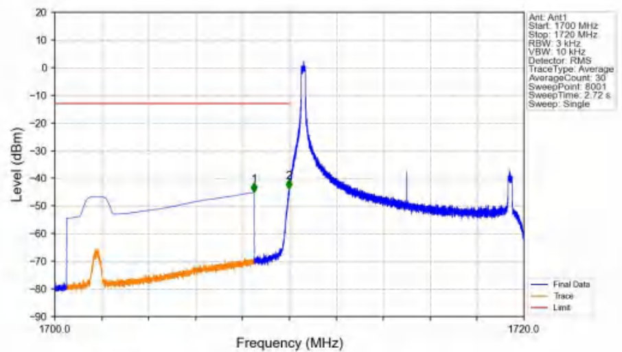
Band4_10MHz_16QAM_LCH_1715MHz_RB_1_0_NTNV
