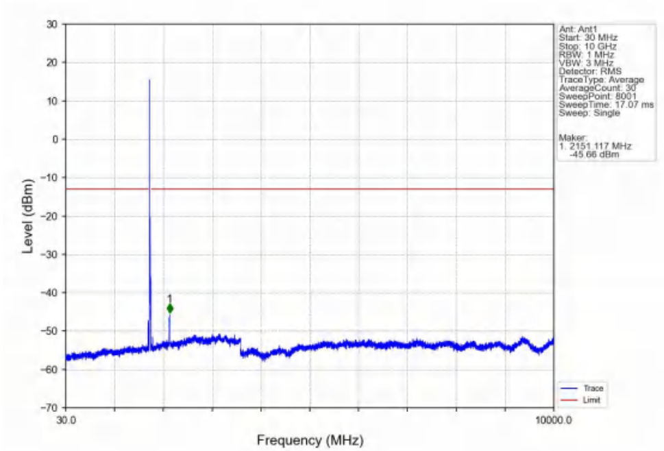
Band4_15MHz_16QAM_HCH_1747.5MHz_RB_1_0_NTNV
