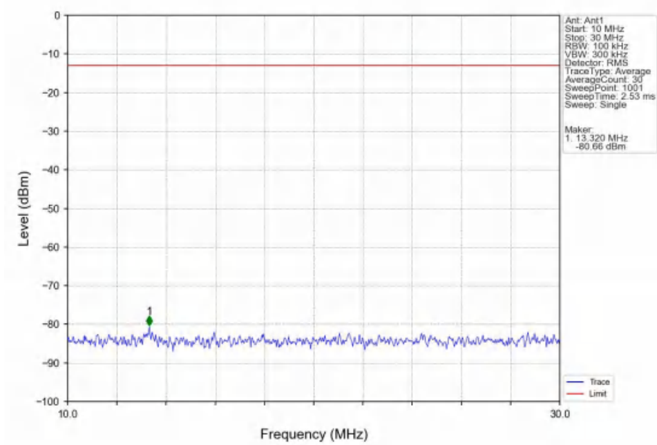
Band4_15MHz_16QAM_HCH_1747.5MHz_RB_1_0_NTNV
