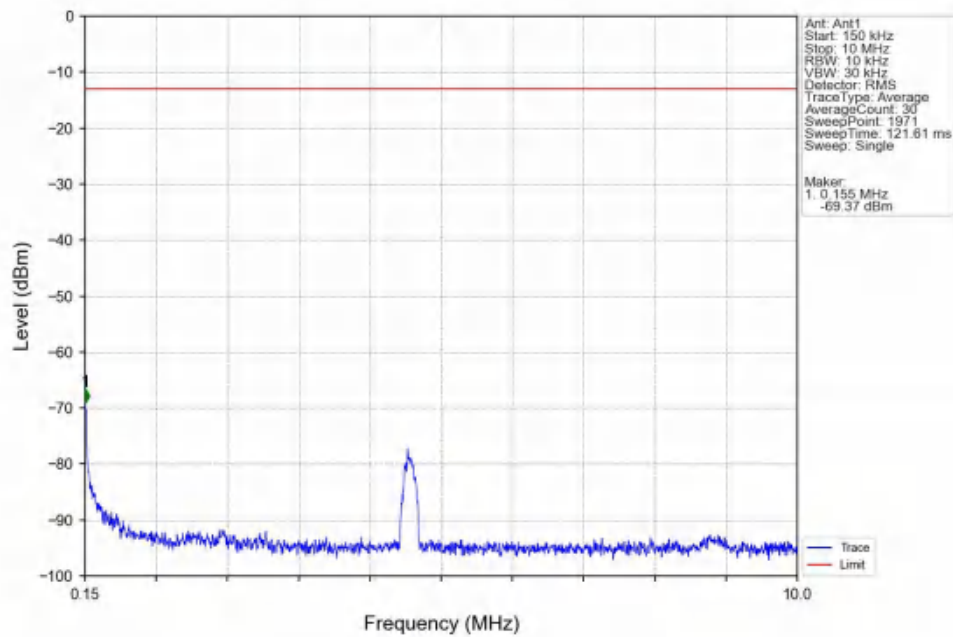
Band4_10MHz_16QAM_LCH_1715MHz_RB_1_0_NTNV
