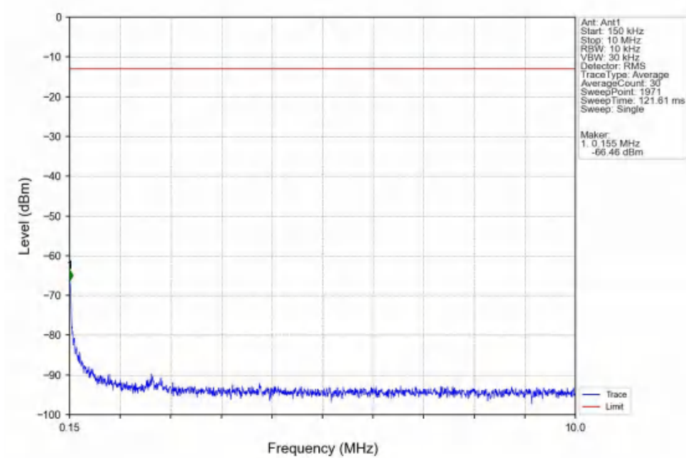
Band4_15MHz_16QAM_HCH_1747.5MHz_RB_1_0_NTNV
