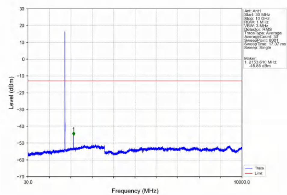
Band4_5MHz_16QAM_HCH_1752.5MHz_RB_1_0_NTNV
