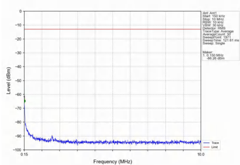
Band4_20MHz_16QAM_HCH_1745MHz_RB_1_0_NTNV
