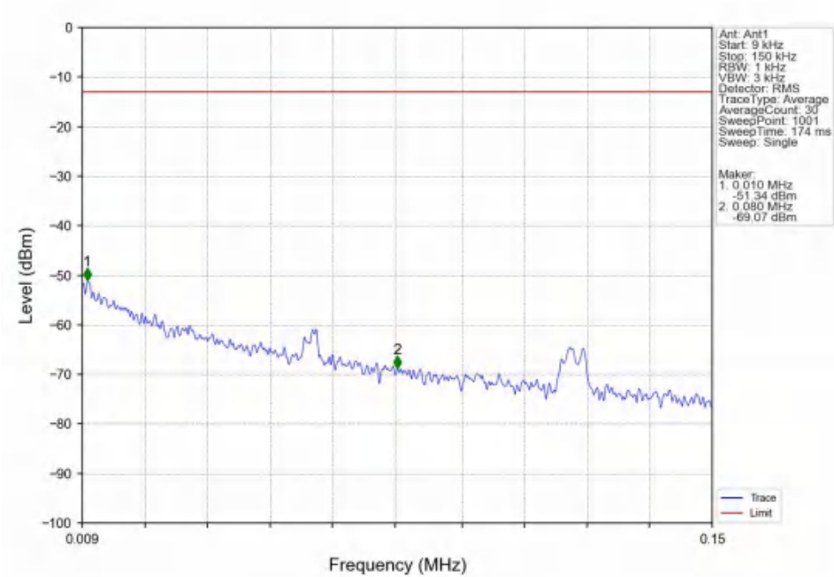
Band4_10MHz_QPSK_MCH_1732.5MHz_RB_1_0_NTNV
