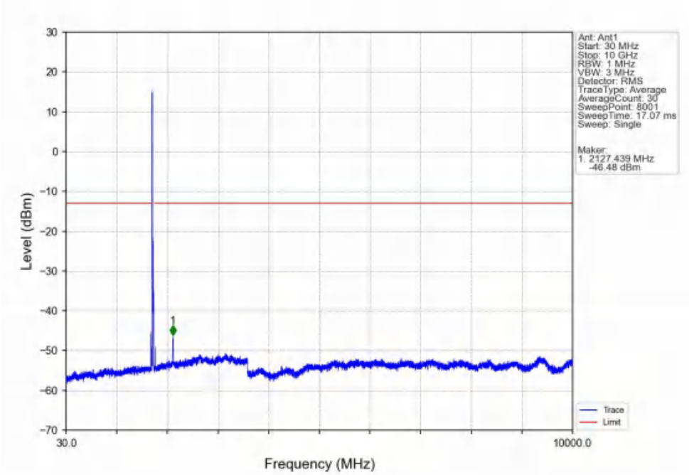
Band4_15MHz_QPSK_MCH_1732.5MHz_RB_1_0_NTNV
