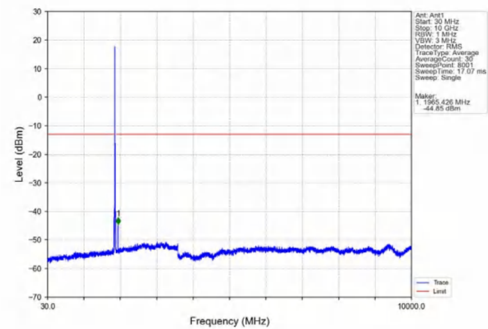
Band2_15MHz_16QAM_MCH_1880MHz_RB_1_0_NTNV
