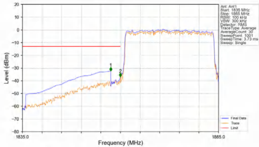
Band2_15MHz_16QAM_LCH_1857.5MHz_RB_75_0_NTNV
