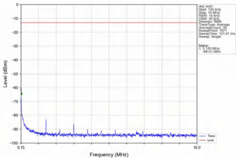
Band2_15MHz_16QAM_MCH_1880MHz_RB_1_0_NTNV
