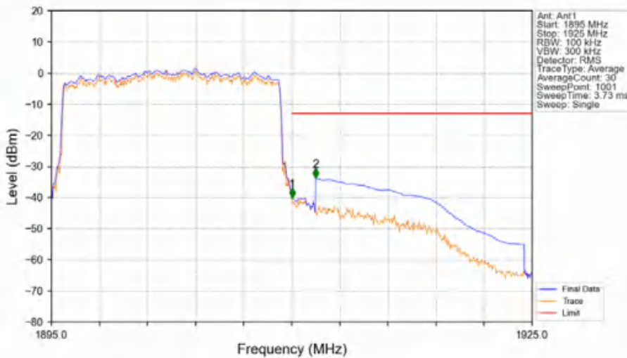
Band2_15MHz_16QAM_HCH_1902.5MHz_RB_75_0_NTNV
