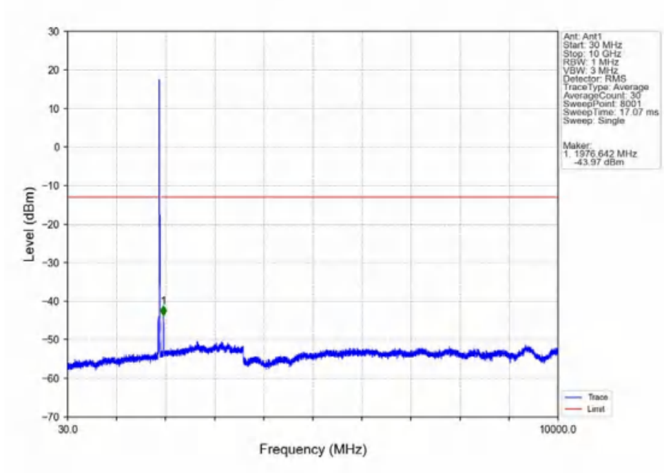
Band2_15MHz_16QAM_HCH_1902.5MHz_RB_1_0_NTNV
