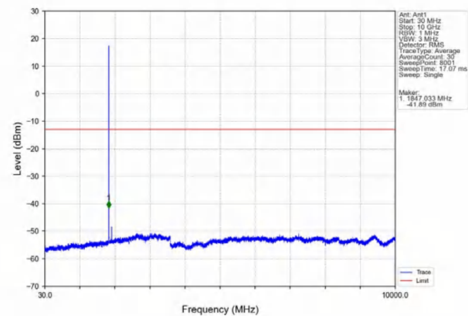
Band2_1.4MHz_16QAM_LCH_1850.7MHz_RB_1_0_NTNV
