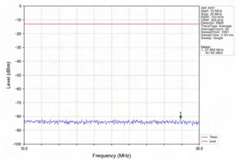
Band2_1.4MHz_16QAM_MCH_1880MHz_RB_1_0_NTNV
