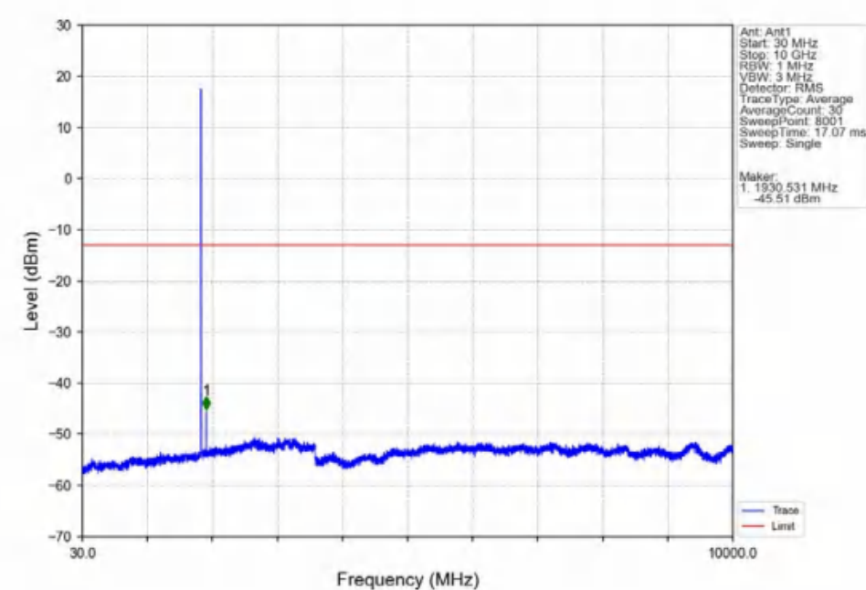
Band2_3MHz_16QAM_LCH_1851.5MHz_RB_1_0_NTNV
