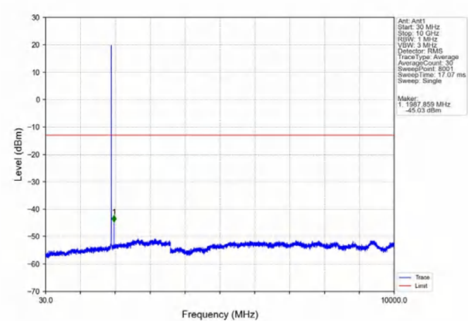
Band2_3MHz_16QAM_HCH_1908.5MHz_RB_1_0_NTNV
