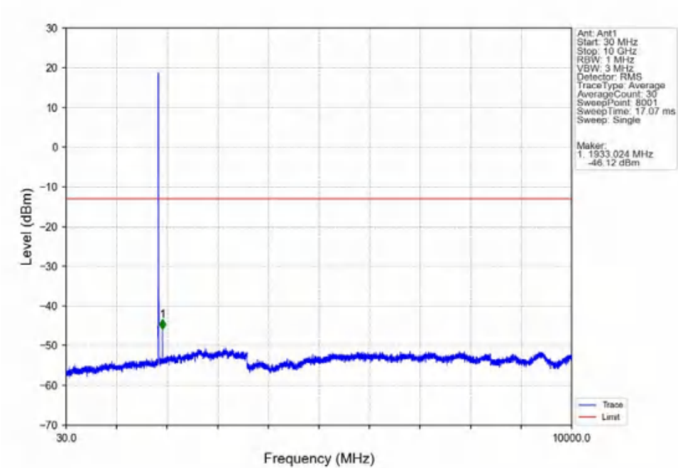
Band2_5MHz_QPSK_LCH_1852.5MHz_RB_1_0_NTNV
