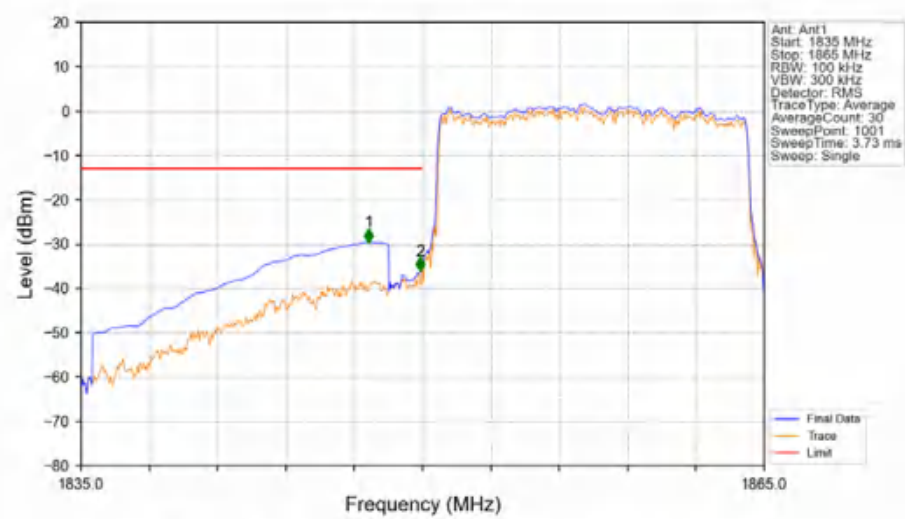
Band2_15MHz_QPSK_LCH_1857.5MHz_RB_75_0_NTNV
