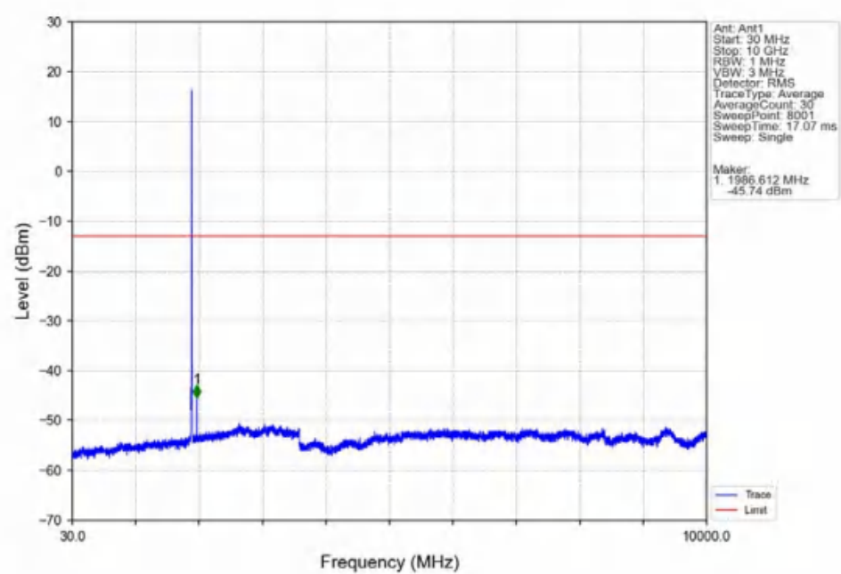
Band2_5MHz_16QAM_HCH_1907.5MHz_RB_1_0_NTNV
