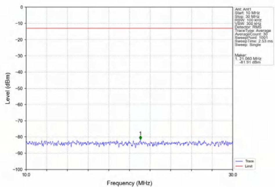
Band2_3MHz_16QAM_LCH_1851.5MHz_RB_1_0_NTNV
