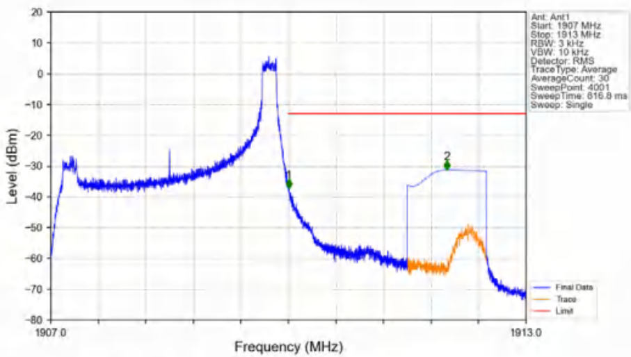
Band2_3MHz_16QAM_HCH_1908.5MHz_RB_1_14_NTNV
