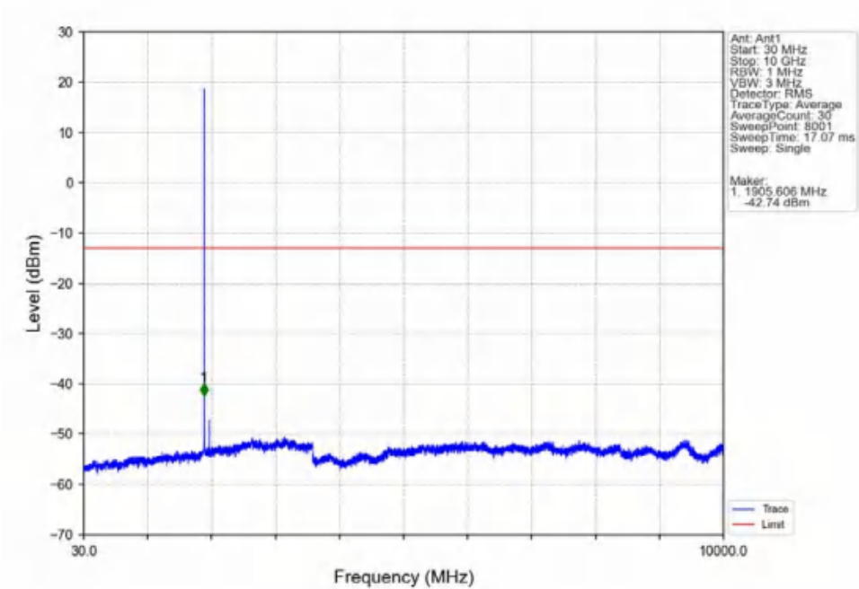
Band2_1.4MHz_16QAM_HCH_1909.3MHz_RB_1_0_NTNV
