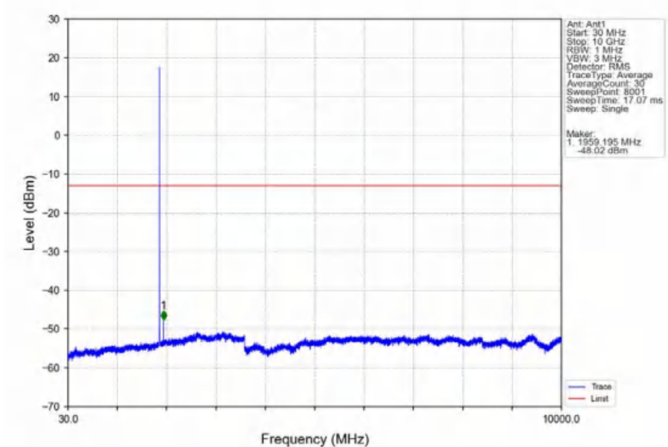
Band2_1.4MHz_16QAM_MCH_1880MHz_RB_1_0_NTNV
