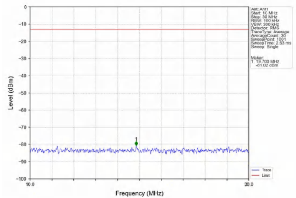
Band2_5MHz_QPSK_LCH_1852.5MHz_RB_1_0_NTNV
