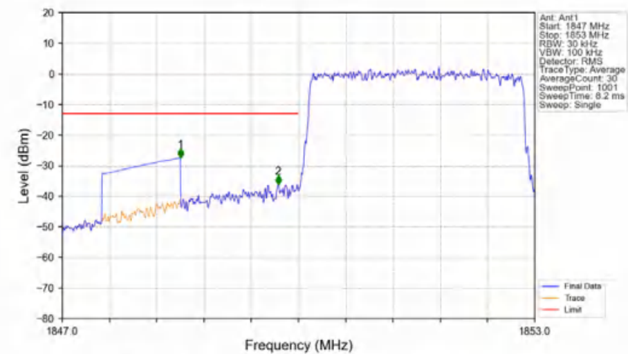
Band2_3MHz_16QAM_LCH_1851.5MHz_RB_15_0_NTNV
