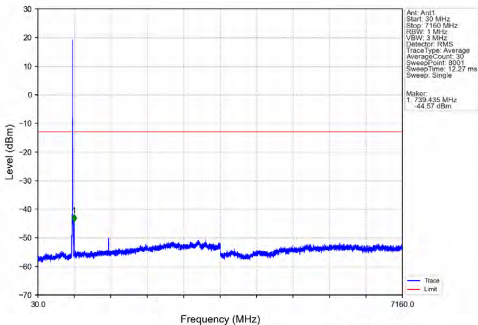
Band12 10MHz QPSK HCH 711MHz RB 1 49 NTNV
