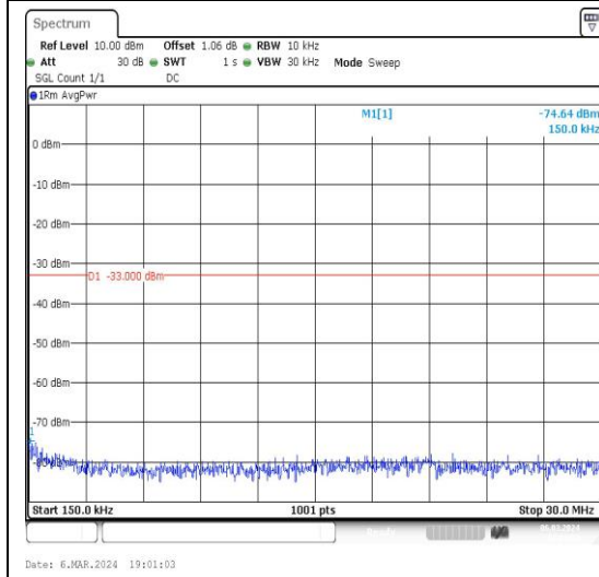
Band4_1.4MHz_16QAM_20393_1RB#0_0.15~30_0.15~30
