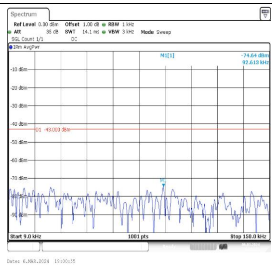
Band4_1.4MHz_16QAM_20393_1RB#0_0.009~0.15_0.009~0.15
