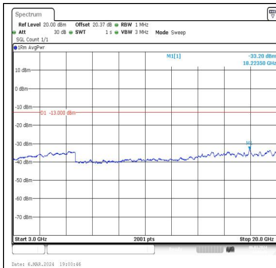
Band4_1.4MHz_QPSK_20393_1RB#0_3000~20000_3000~20000
