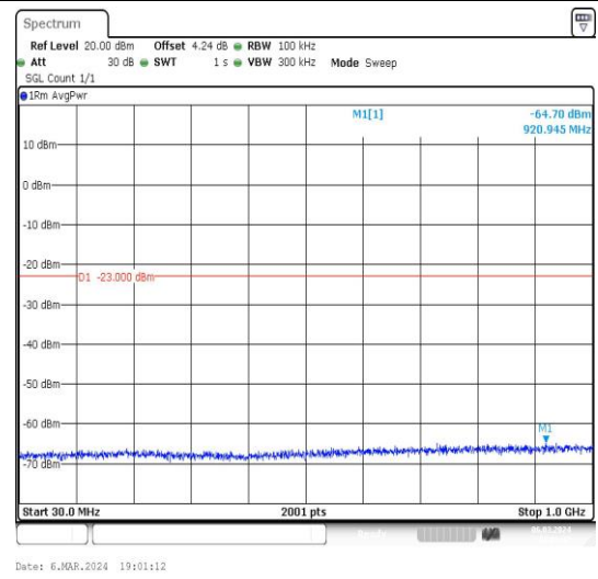
Band4_1.4MHz_16QAM_20393_1RB#0_30~1000_30~1000
